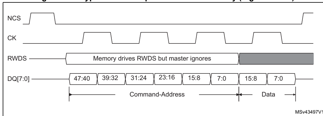
Figure 153. HyperBus write operation with no latency (register write)
