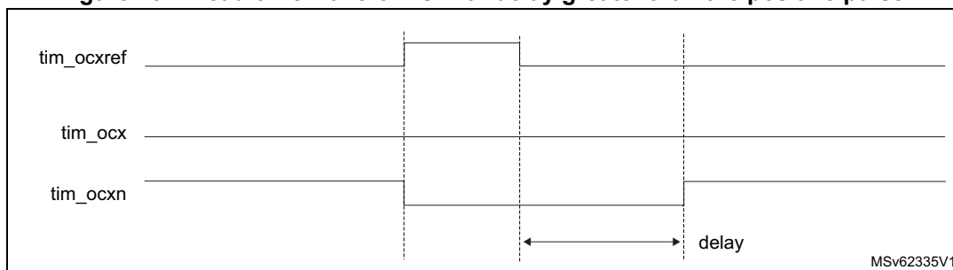
Figure 704. Dead-time waveforms with delay greater than the positive pulse.
