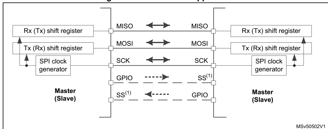
Figure 842. Multimaster application
