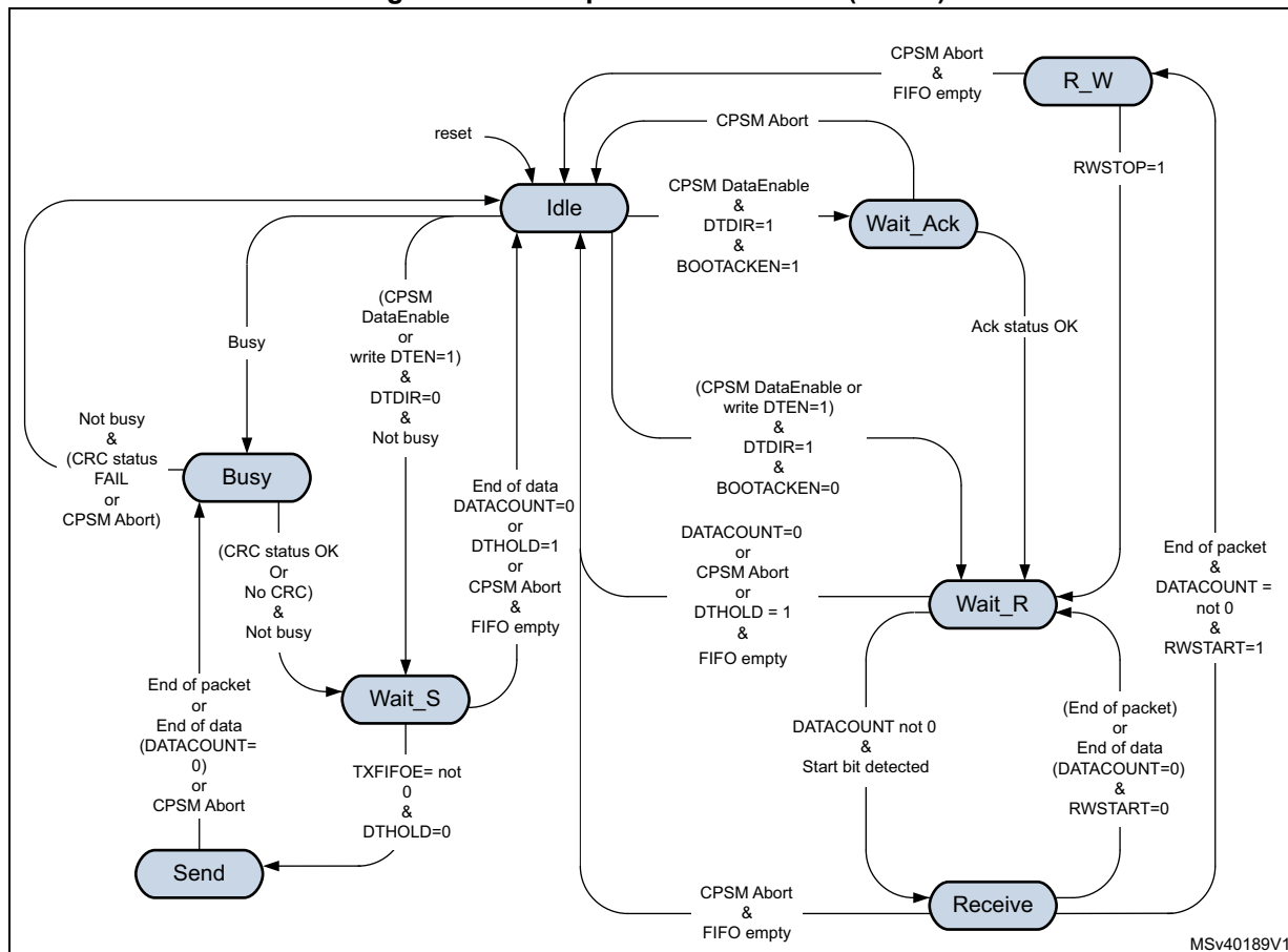
Figure 193. Data path state machine (DPSM)
