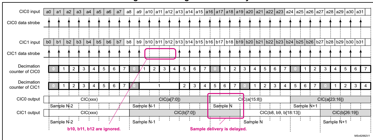
Figure 362. Programmable delay
