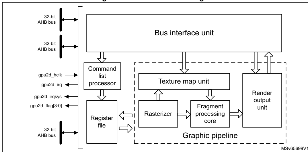
Figure 443. GPU2D block diagram
