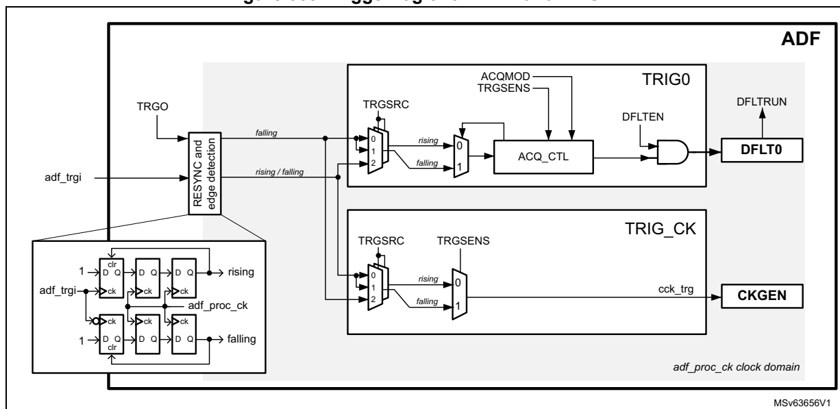
Figure 365. Trigger logic for DFLT and CKGEN
