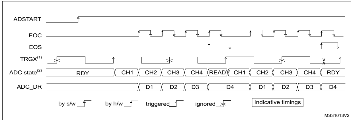
Figure 229. Single conversions of a sequence, hardware trigger
