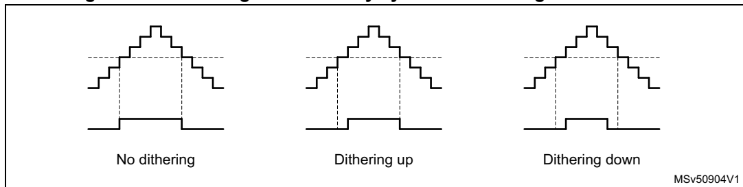
Figure 542. Dithering effect on duty cycle in center-aligned PWM mode
