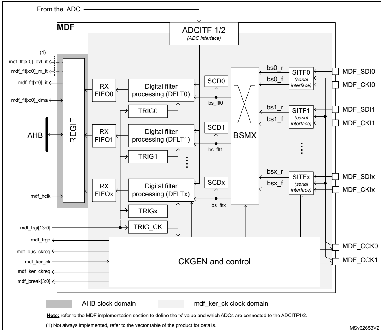
Figure 321. MDF block diagram
