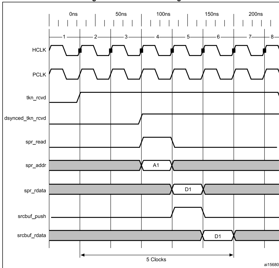
Figure 904. TRDT max timing case
