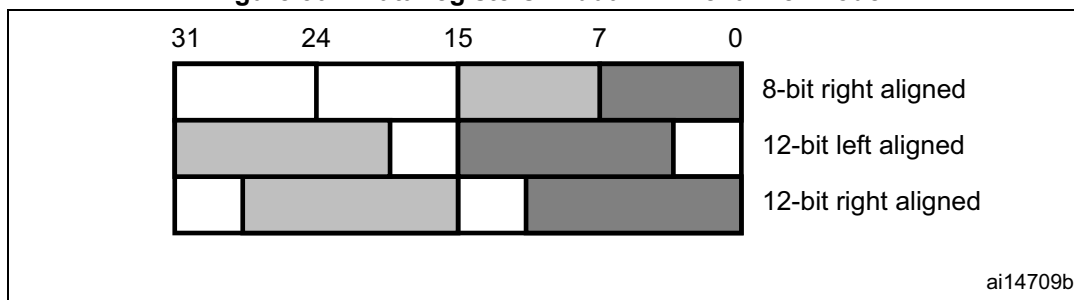
Figure 304. Data registers in dual DAC channel mode
