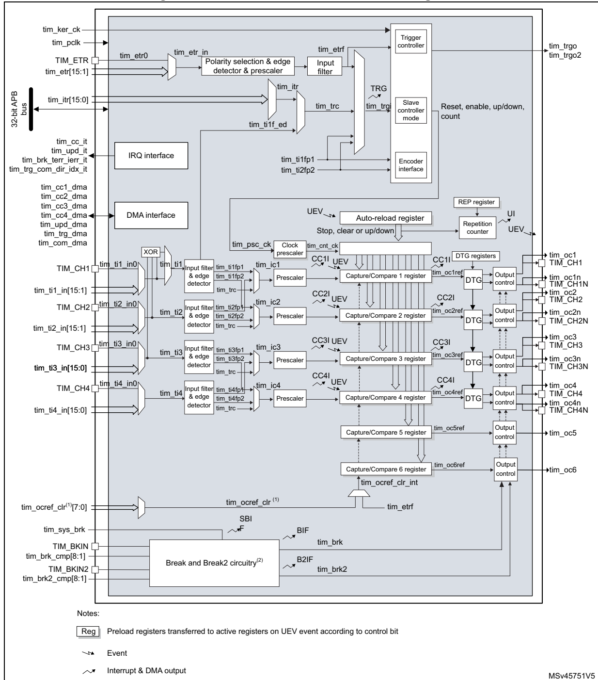
Figure 503. Advanced-control timer block diagram
