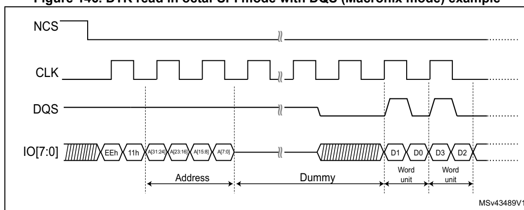
Figure 146. DTR read in octal-SPI mode with DQS (Macronix mode) example
