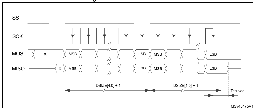
Figure 849. TI mode transfer
