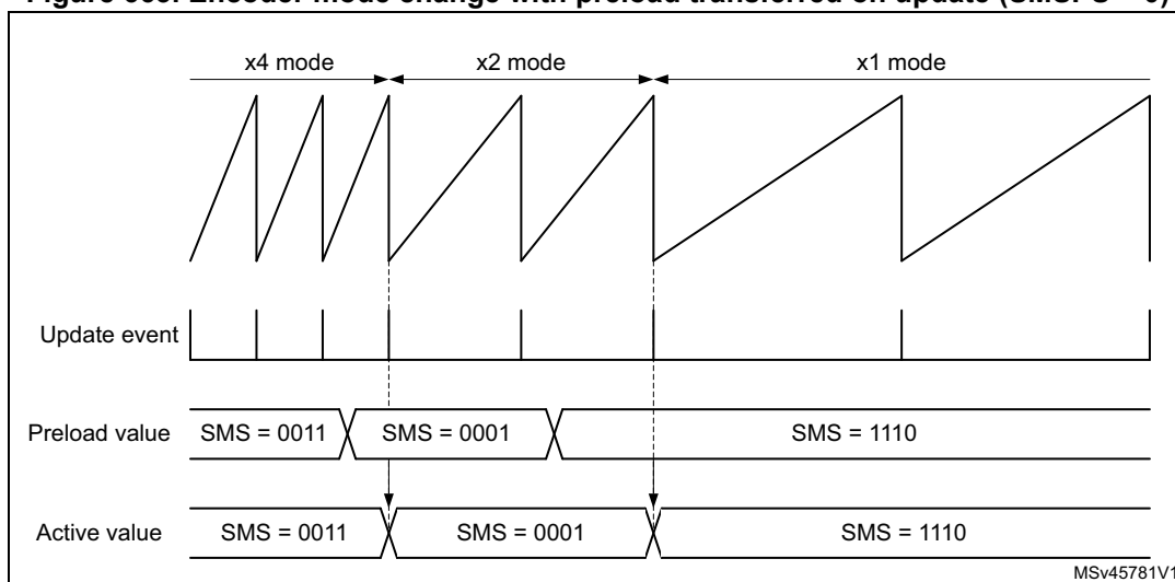
Figure 663. Encoder mode change with preload transferred on update (SMSPS = 0)
