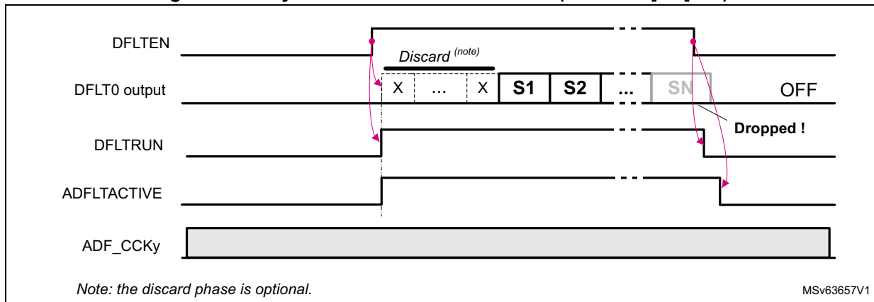
Figure 366. Asynchronous continuous mode (ACQMOD[2:0] = 0)
