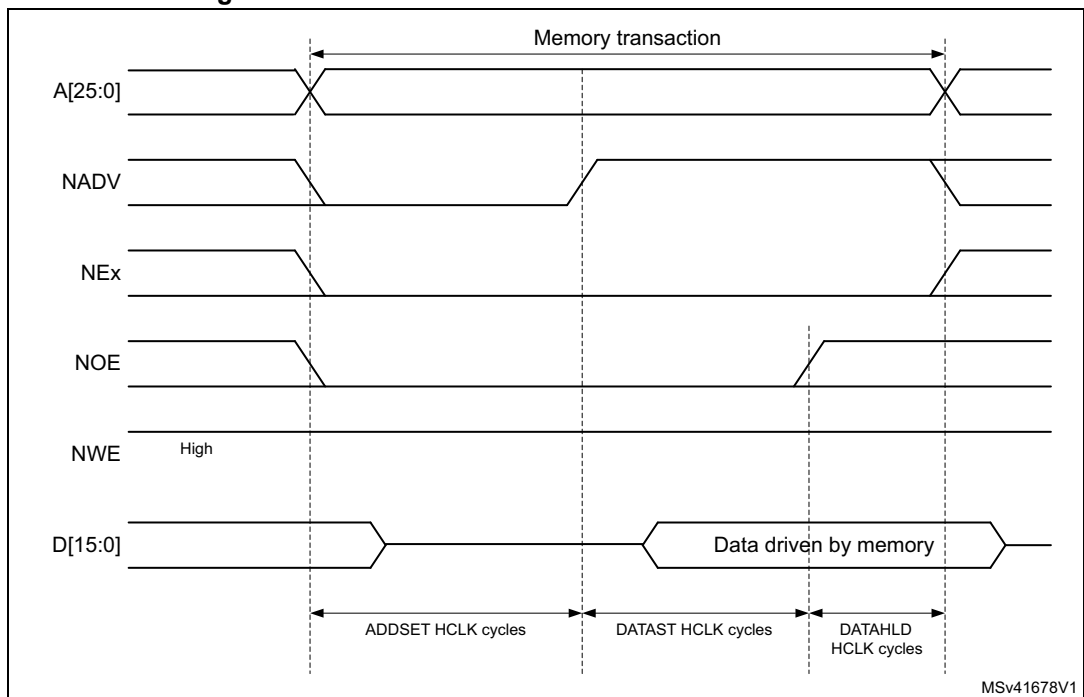
Figure 123. Mode 2 and mode B read access waveforms
