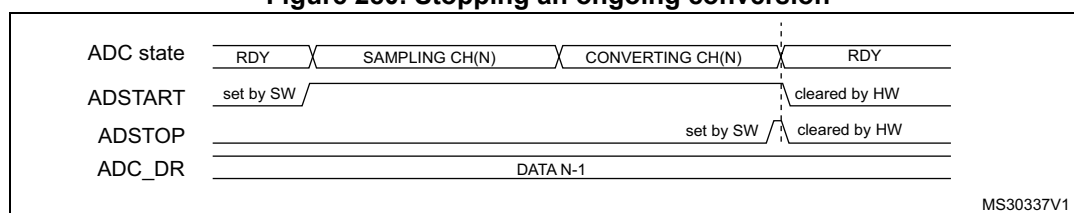
Figure 280. Stopping an ongoing conversion
