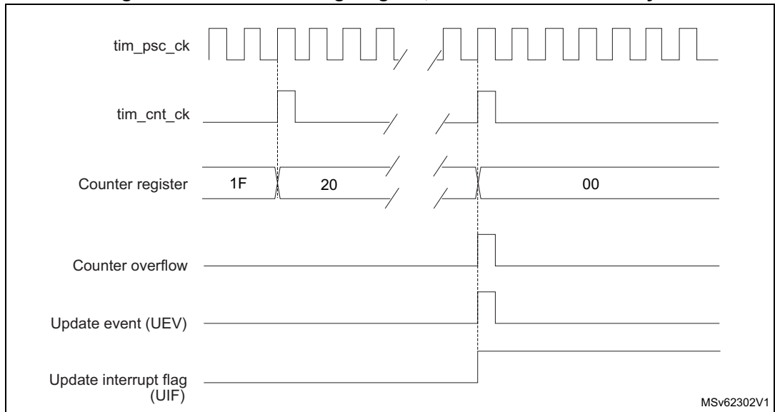
Figure 510. Counter timing diagram, update event when ARPE=0 (TIMx_ARR not preloaded)
