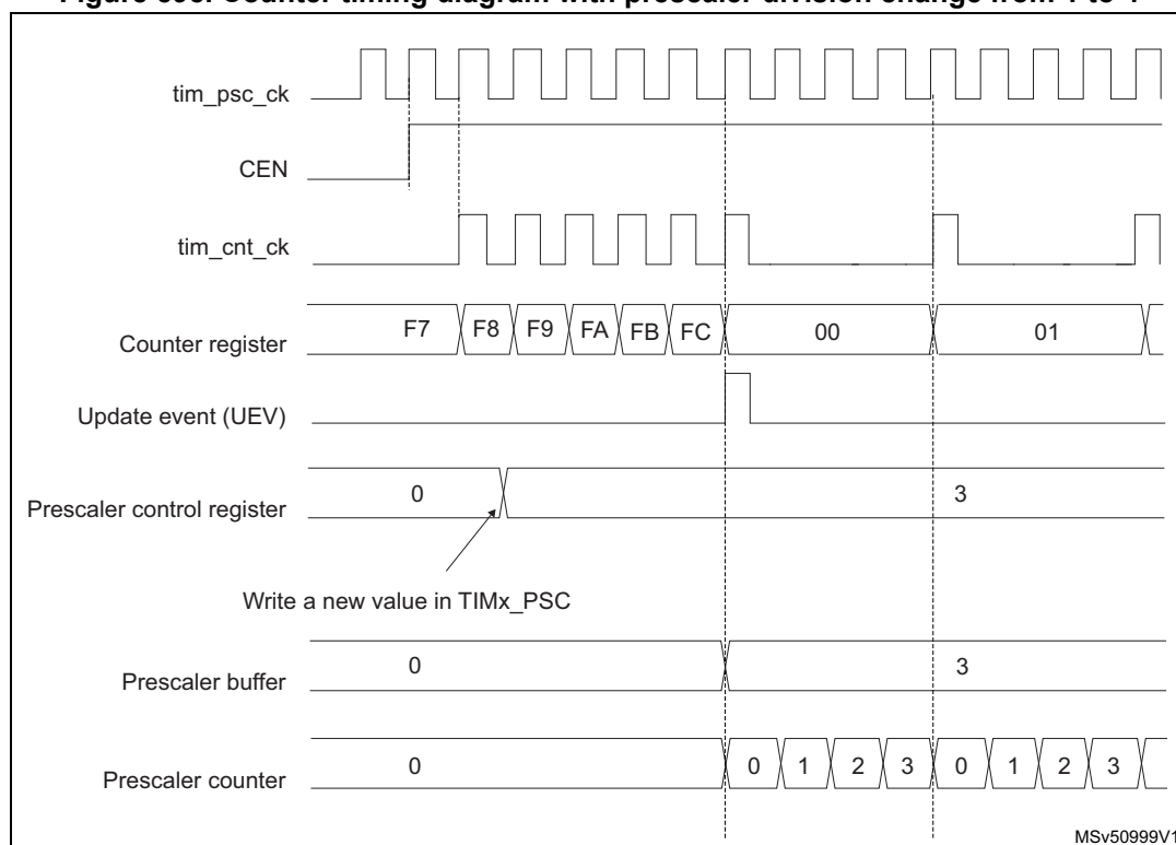
Figure 595. Counter timing diagram with prescaler division change from 1 to 4
