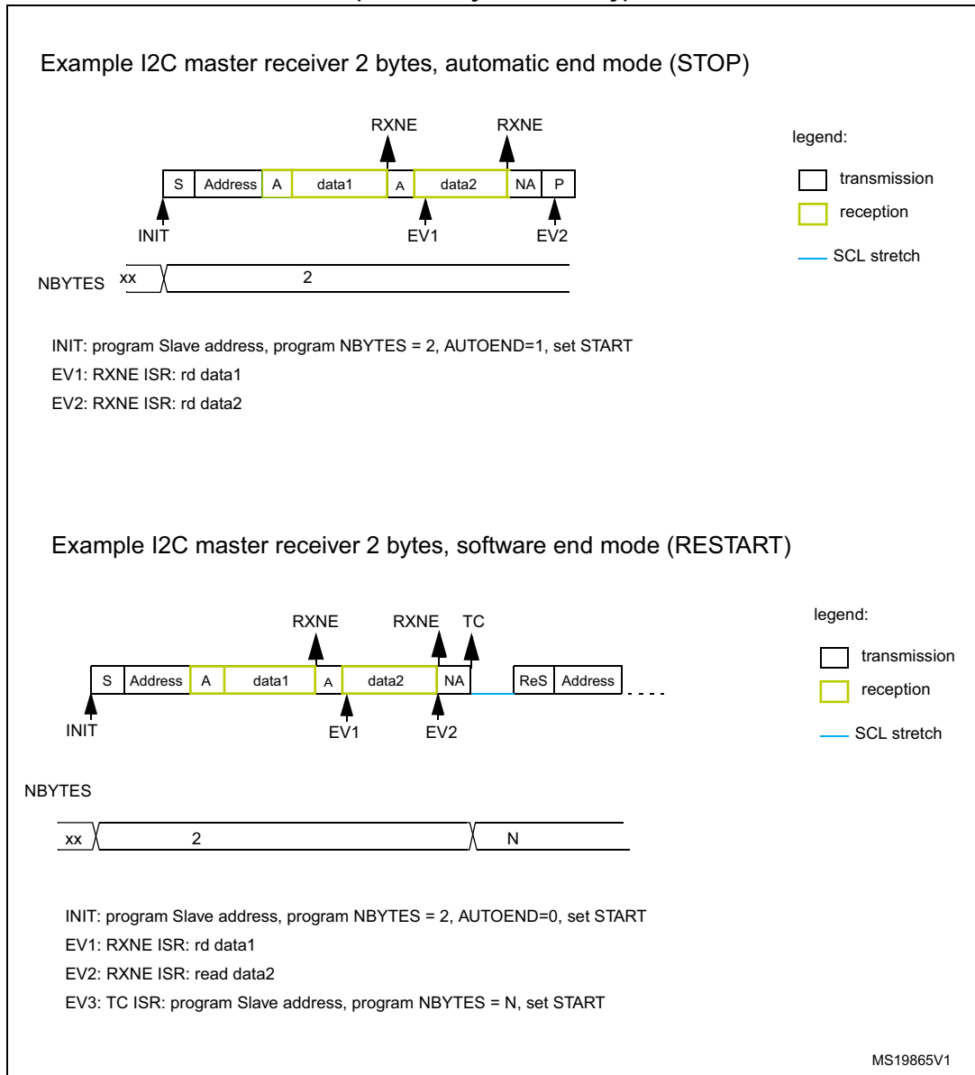
Figure 792. Transfer bus diagrams for I2C master receiver (mandatory events only)
