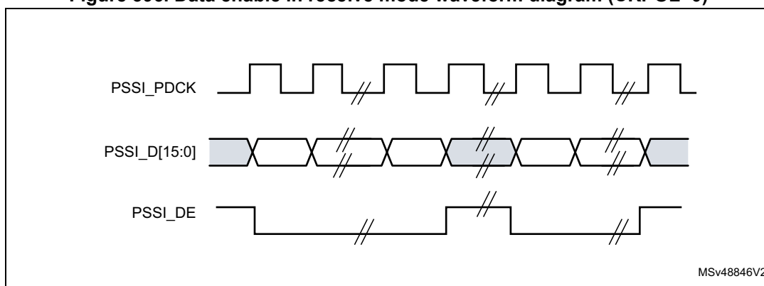
Figure 396. Data enable in receive mode waveform diagram (CKPOL=0)
