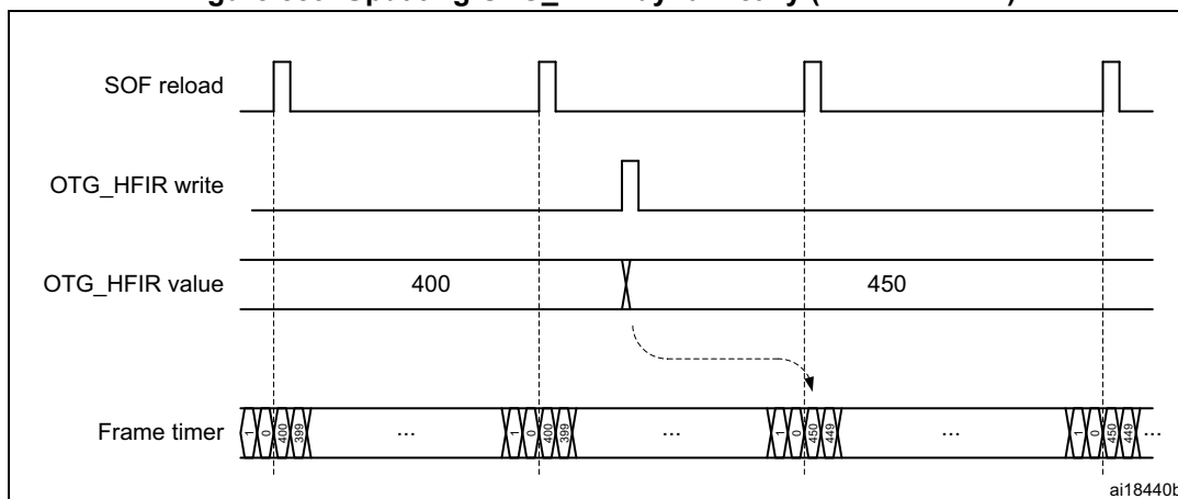
Figure 889. Updating OTG_HFIR dynamically (RLDCTRL = 1)
