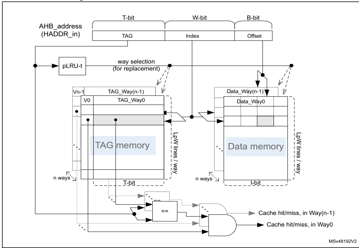
Figure 28. ICACHE TAG and data memories functional view
