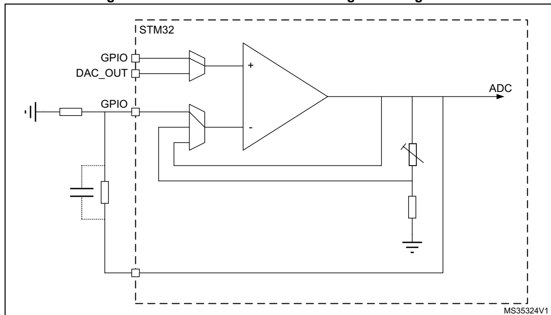
Figure 317. Standalone mode: external gain setting mode
