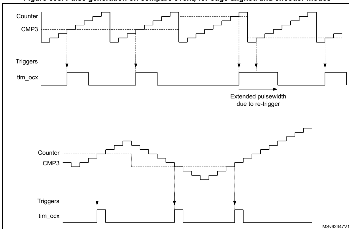
Figure 638. Pulse generation on compare event, for edge-aligned and encoder modes
