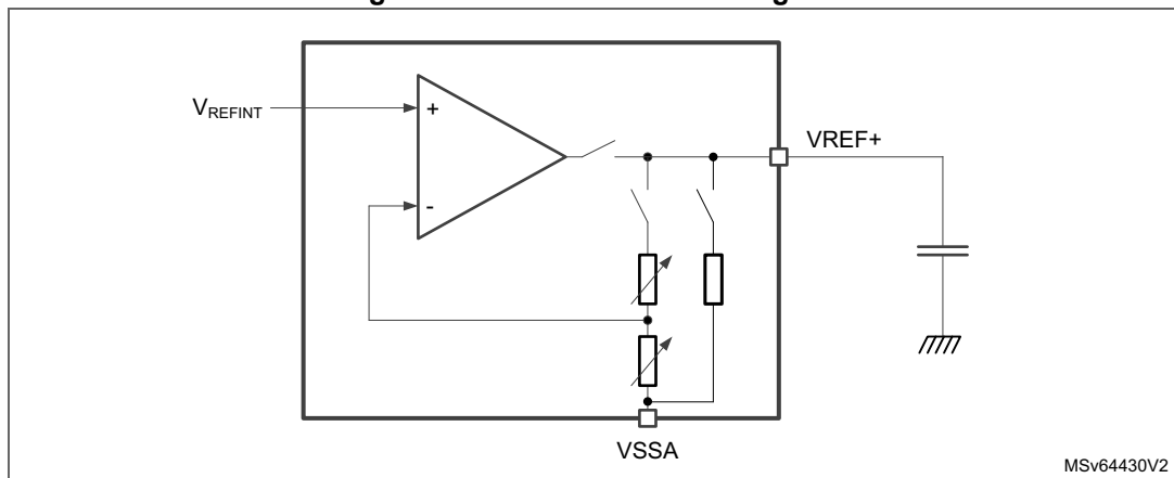
Figure 311. VREFBUF block diagram
