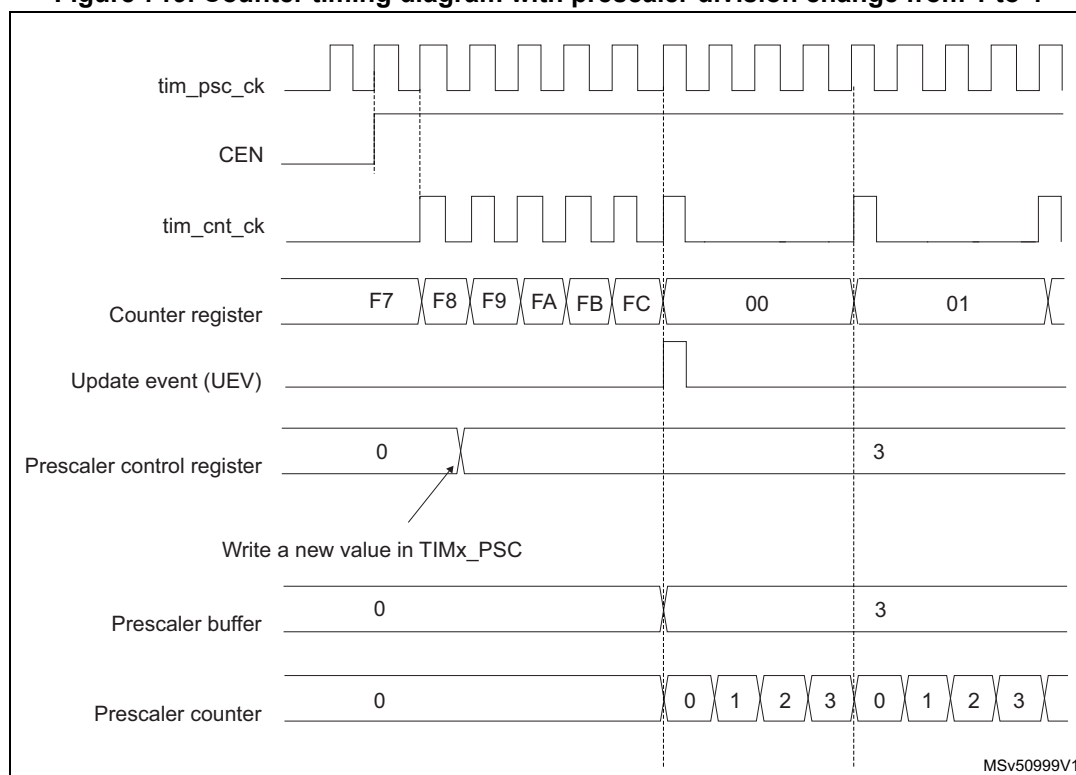
Figure 719. Counter timing diagram with prescaler division change from 1 to 4
