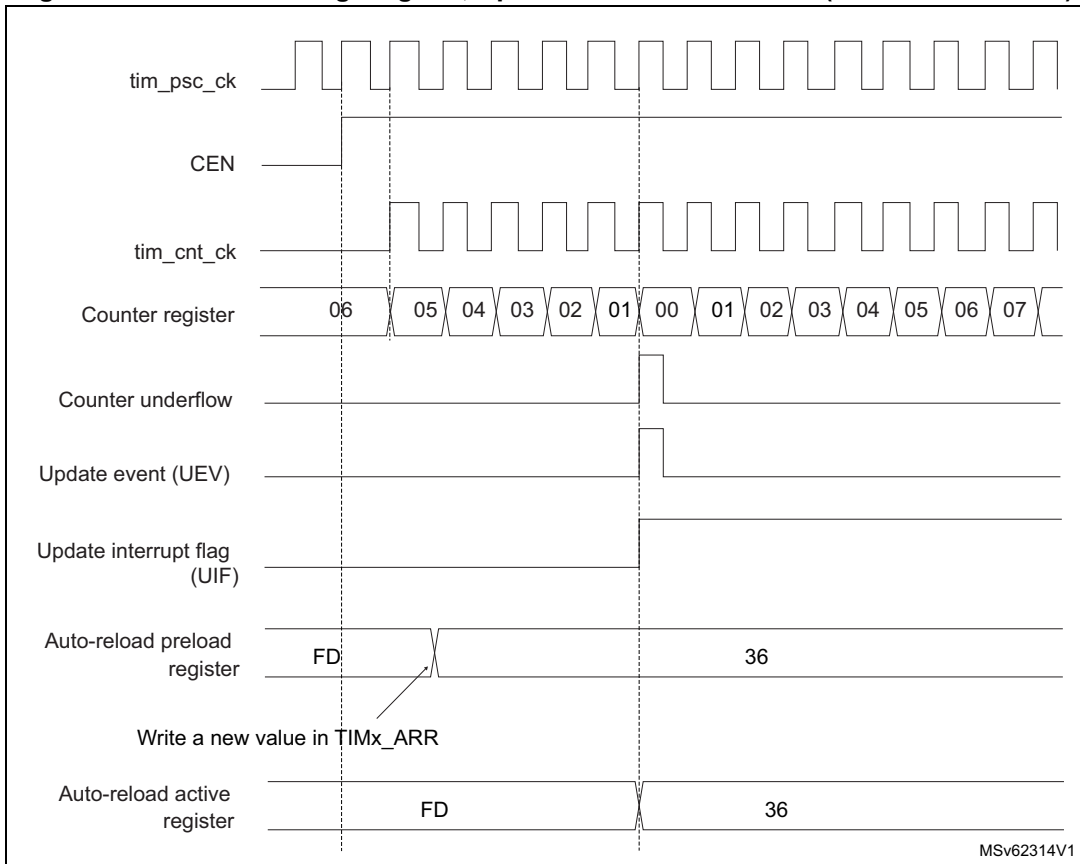
Figure 611. Counter timing diagram, Update event with ARPE=1 (counter underflow)
