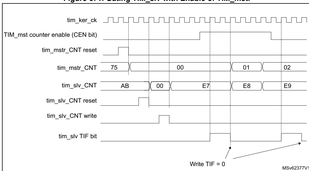
Figure 671. Gating TIM_slv with Enable of TIM_mstr
