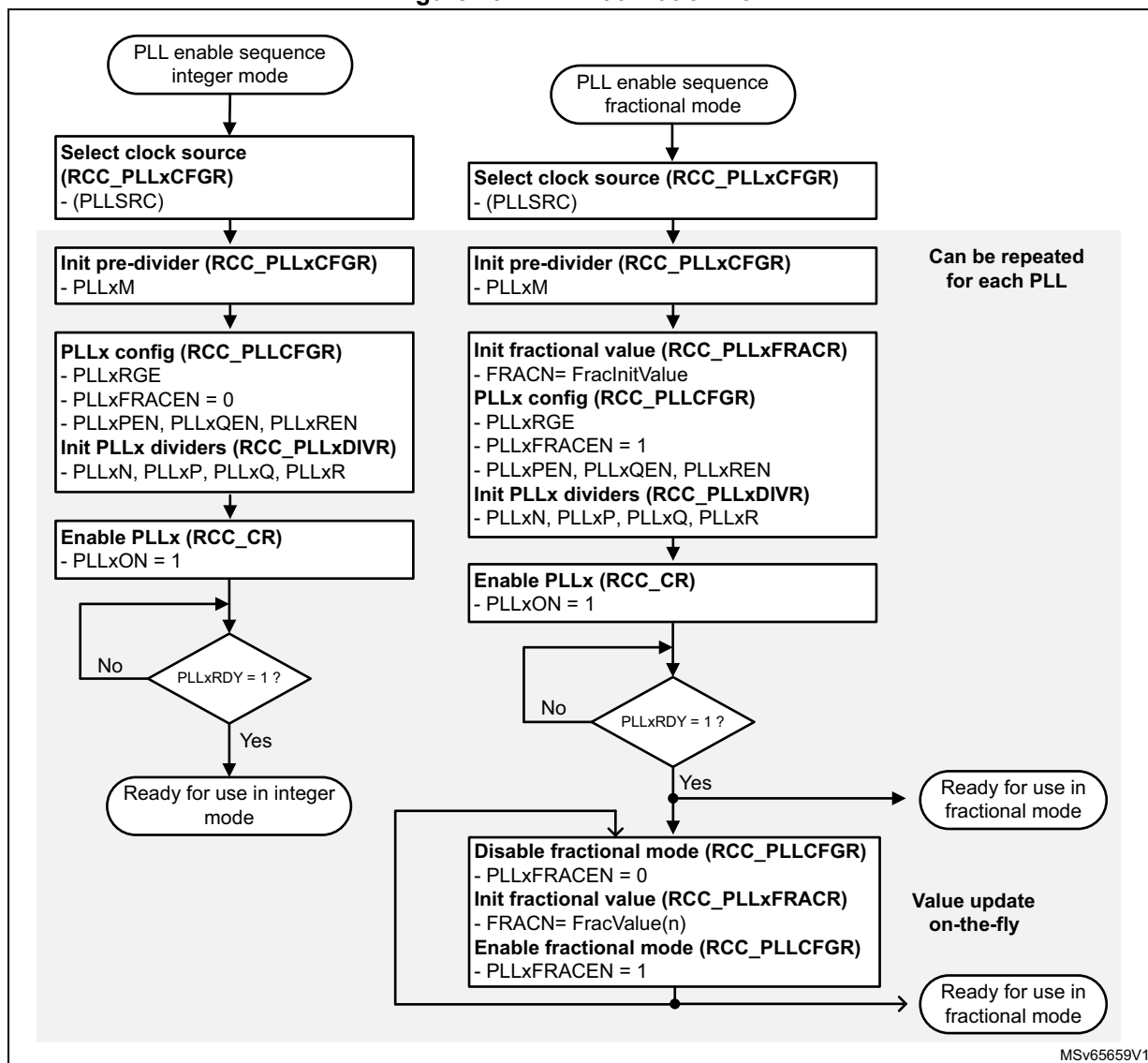
Figure 40. PLL initialization flow
