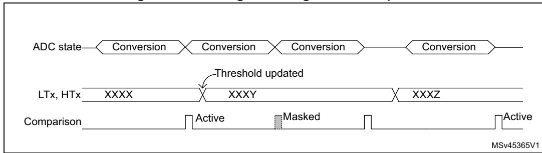
Figure 296. Analog watchdog threshold update
