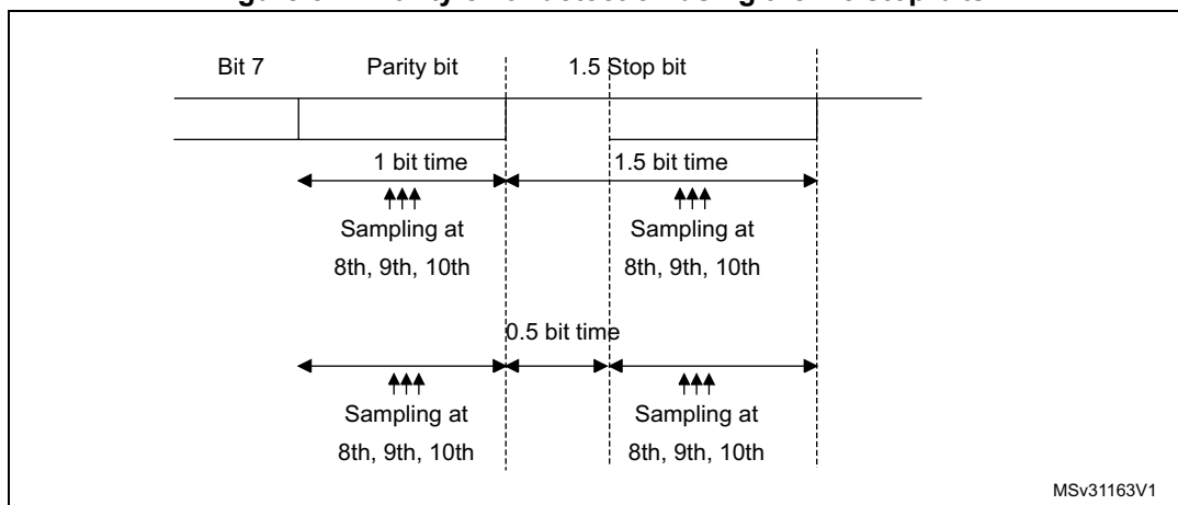
Figure 817. Parity error detection using the 1.5 stop bits
