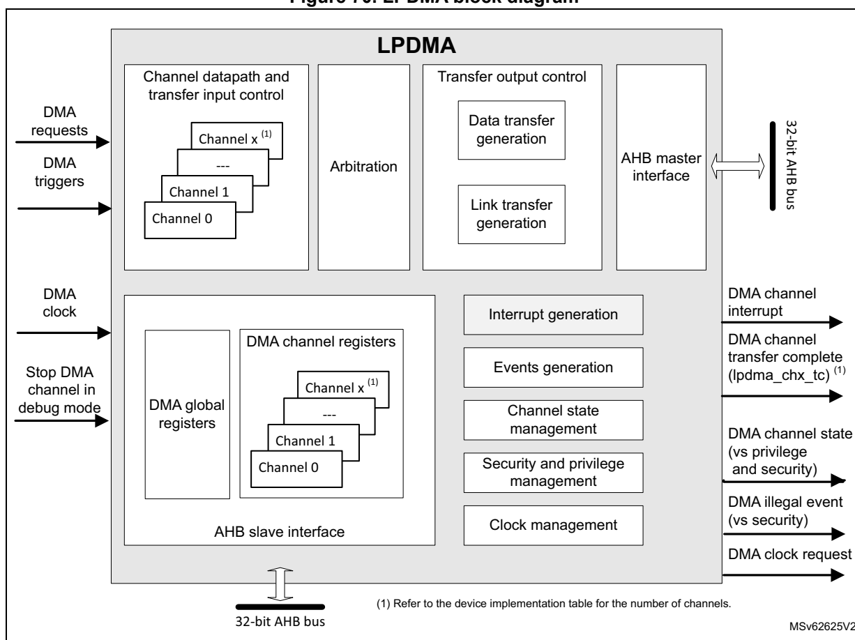
Figure 70. LPDMA block diagram
