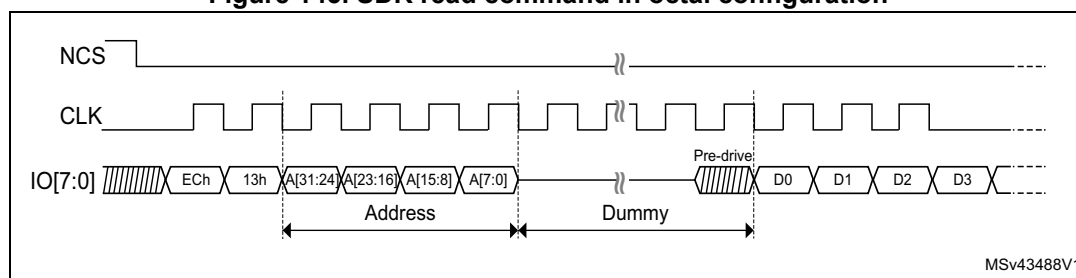
Figure 145. SDR read command in octal configuration
