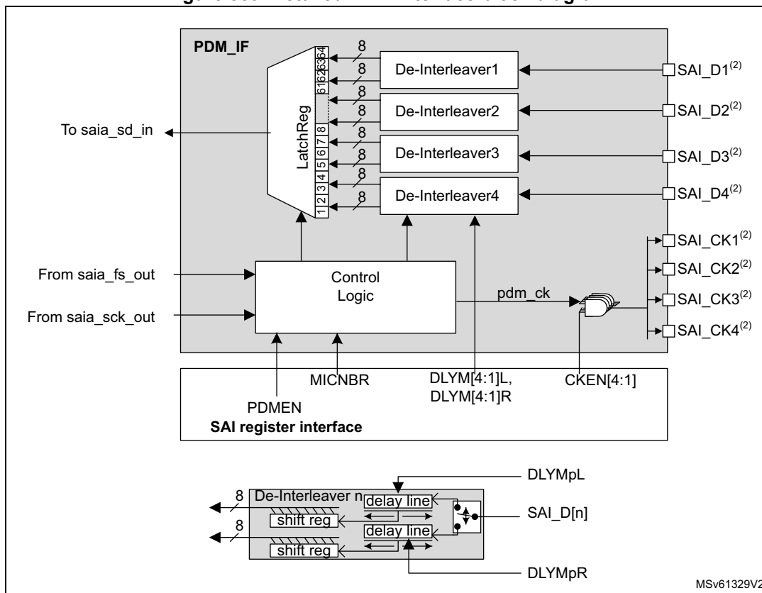
Figure 859. Detailed PDM interface block diagram
