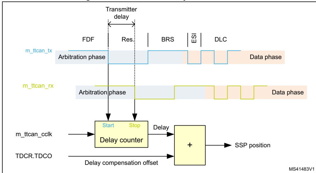
Figure 876. Transceiver delay measurement
