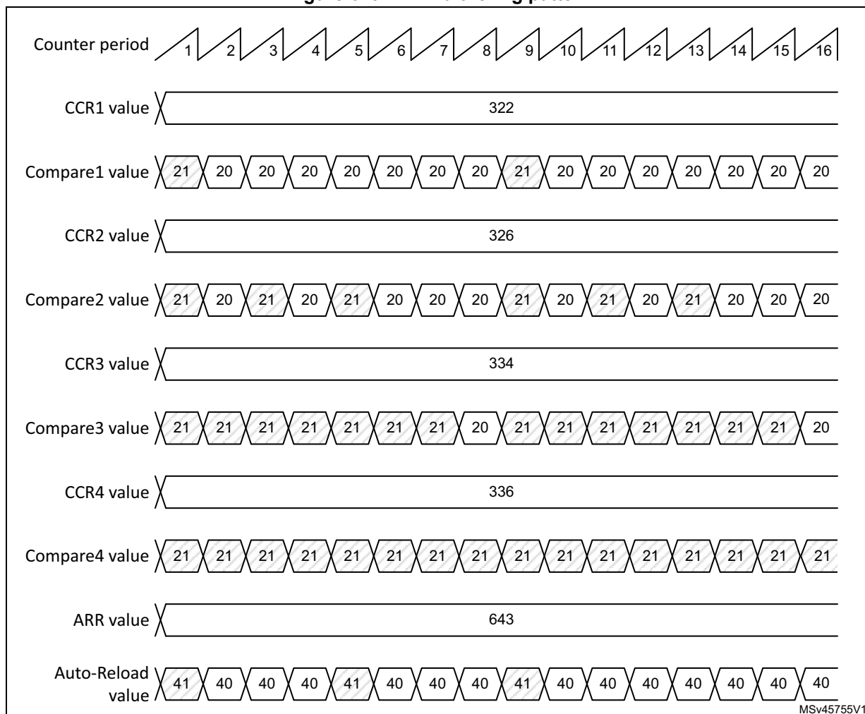
Figure 629. PWM dithering pattern
