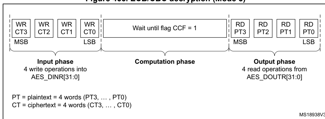
Figure 466. ECB/CBC decryption (Mode 3)
