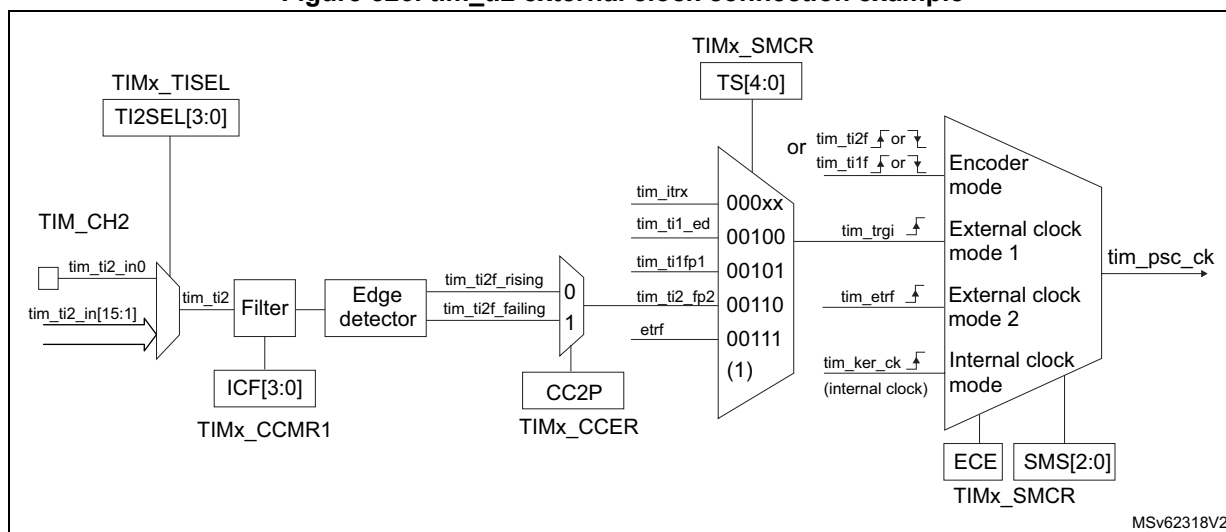
Figure 526. tim_ti2 external clock connection example
