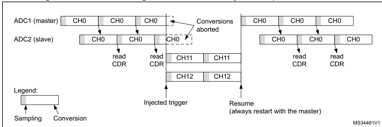
Figure 264. Two interleaved channels (CH1, CH2) with injected sequence CH11, CH12 - case 1: Master interrupted first
