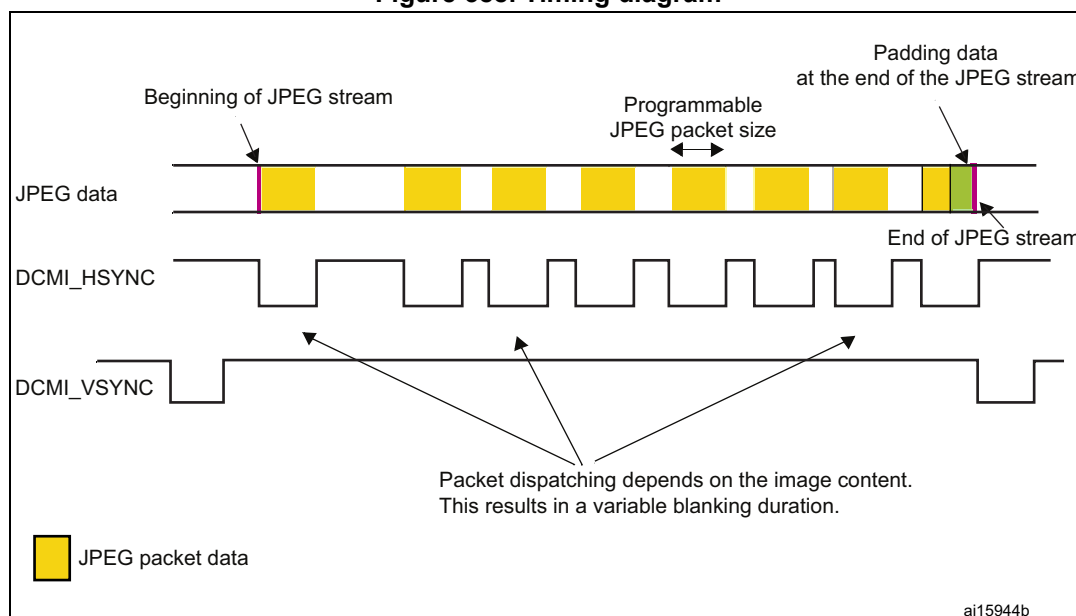
Figure 388. Timing diagram
