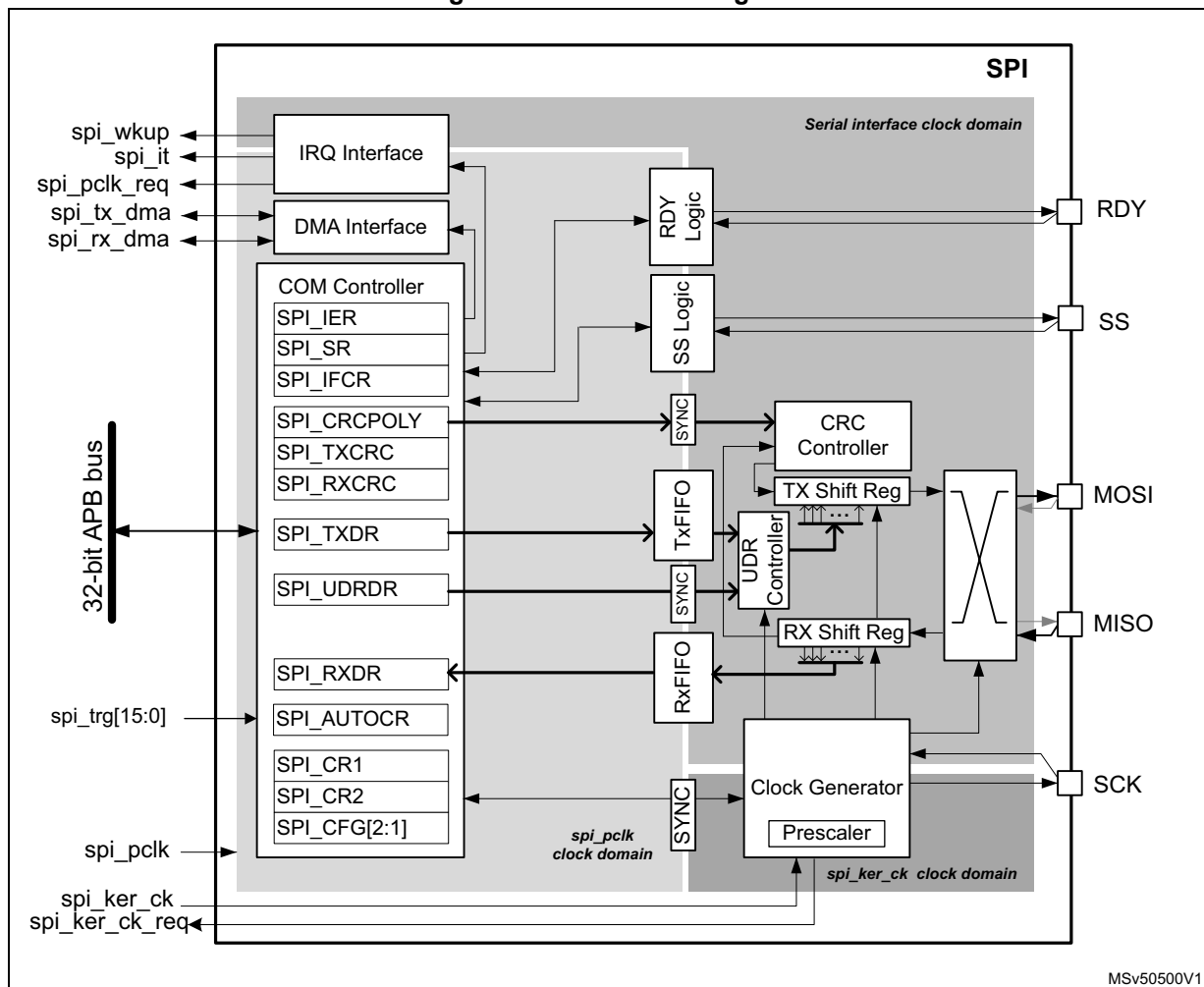
Figure 837. SPI block diagram
