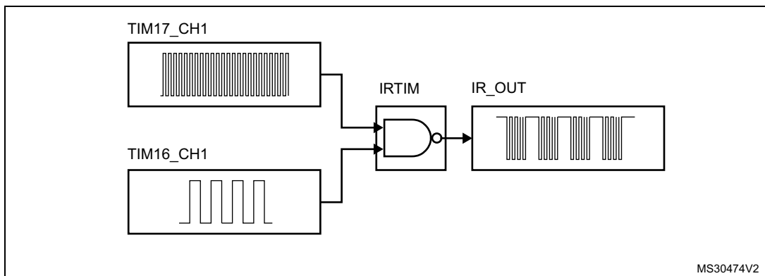
Figure 759. IRTIM internal hardware connections with TIM16 and TIM17
