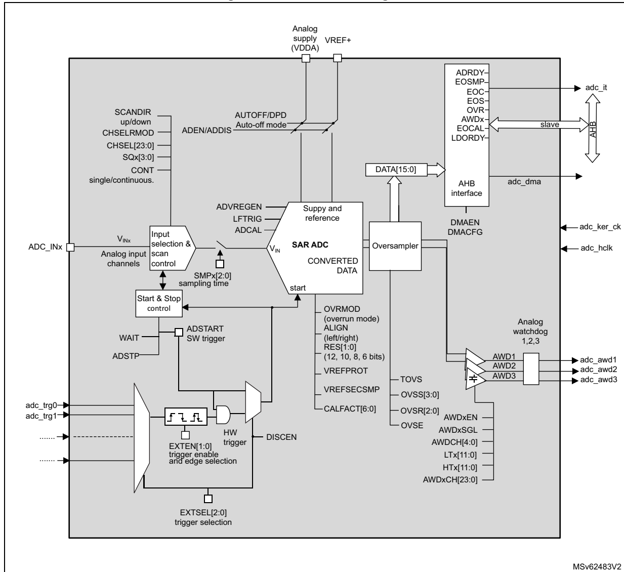
Figure 272. ADC block diagram
