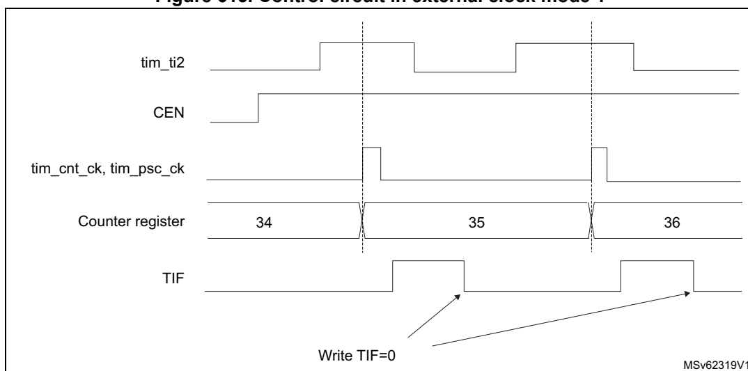
Figure 615. Control circuit in external clock mode 1
