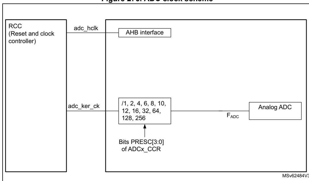
Figure 276. ADC clock scheme
