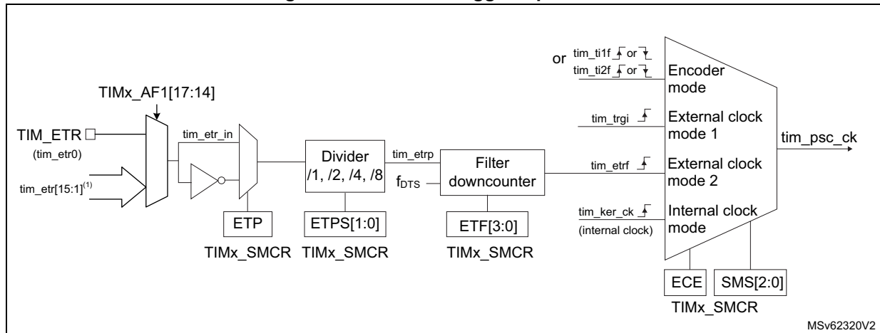
Figure 528. External trigger input block
