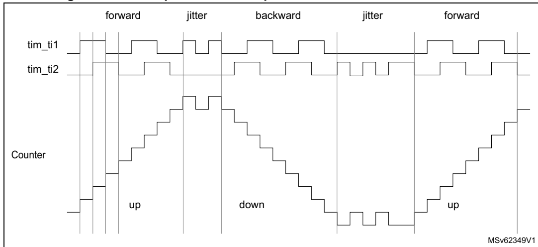
Figure 563. Example of counter operation in encoder interface mode.
