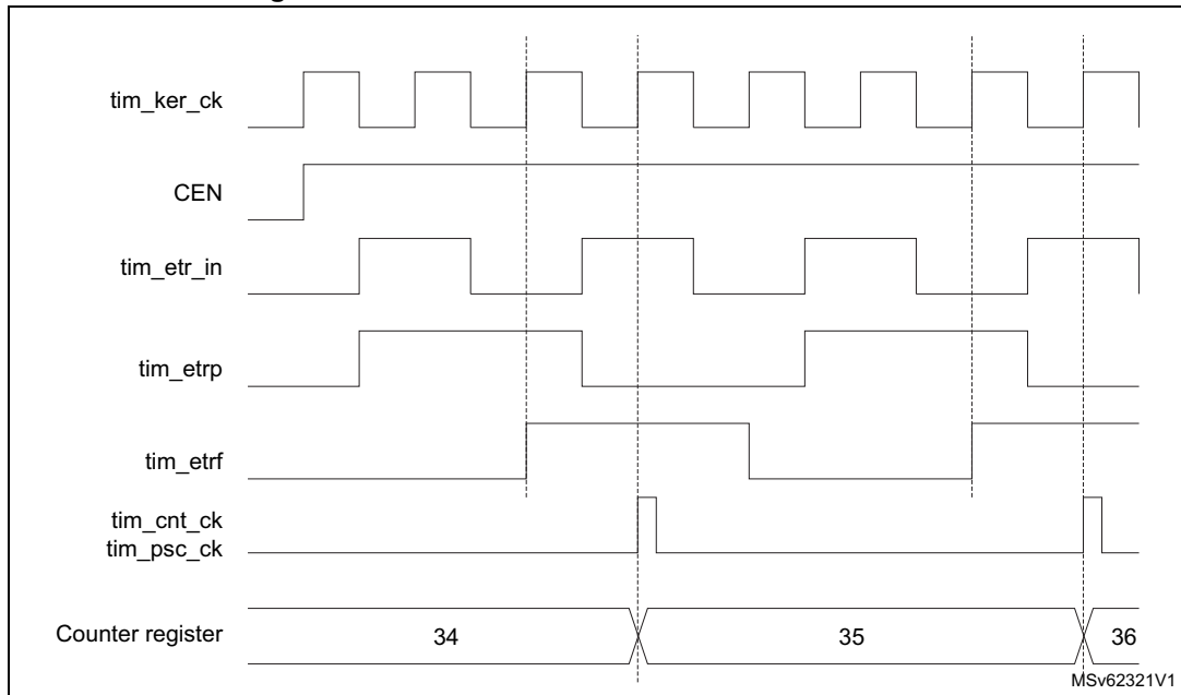
Figure 529. Control circuit in external clock mode 2
