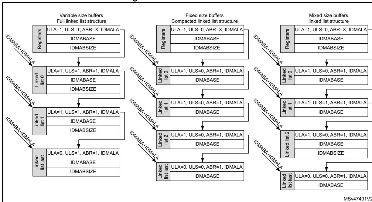
Figure 195. Linked list structures
