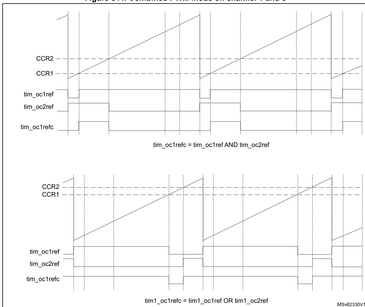
Figure 544. Combined PWM mode on channel 1 and 3
