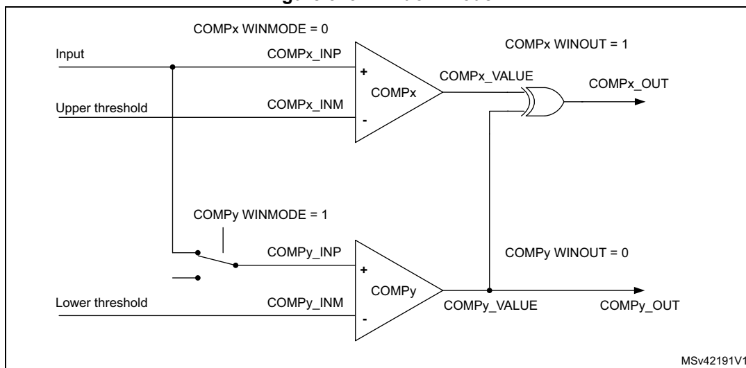
Figure 313. Window mode
