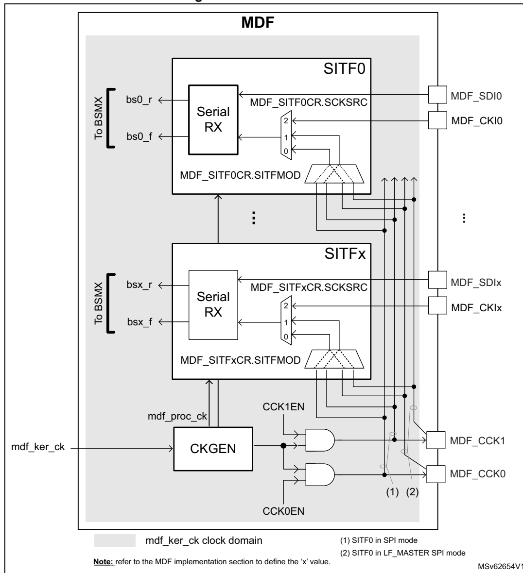
Figure 322. SITF x overview
