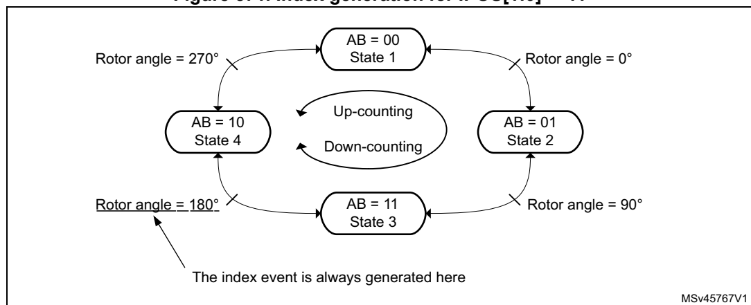
Figure 571. Index generation for IPOS[1:0] = 11
