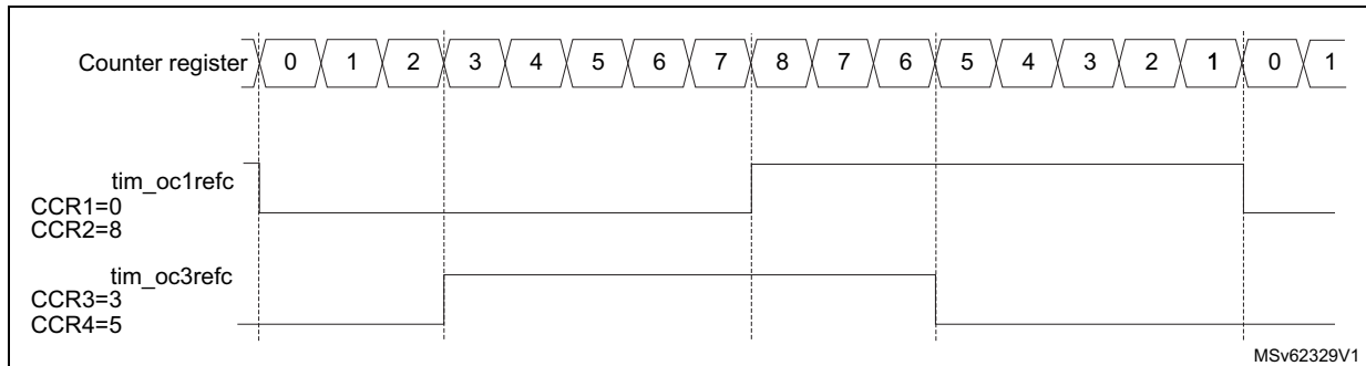
Figure 631. Generation of 2 phase-shifted PWM signals with 50% duty cycle
