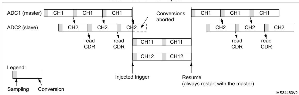
Figure 265. Two Interleaved channels (CH1, CH2) with injected sequence CH11, CH12 - case 2: Slave interrupted first
