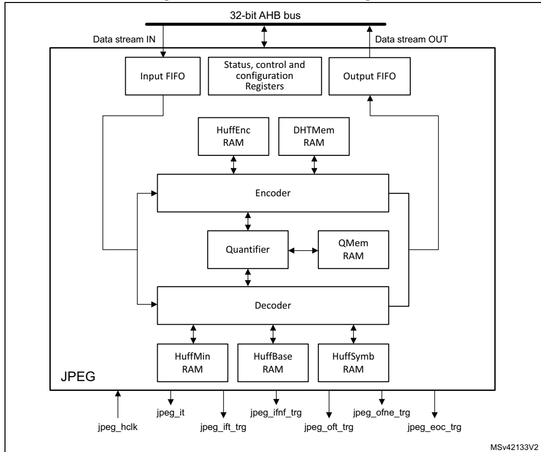
Figure 444. JPEG codec block diagram
