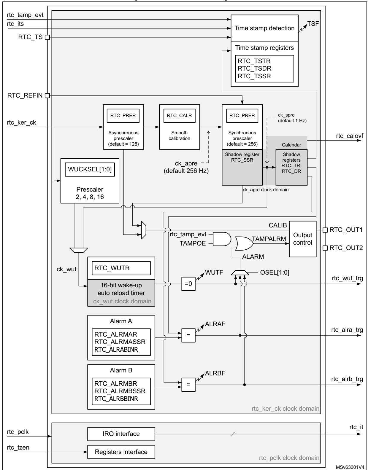
Figure 766. RTC block diagram
