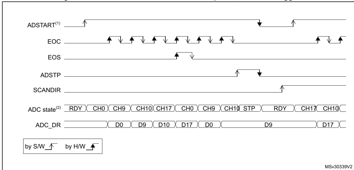
Figure 282. Continuous conversion of a sequence, software trigger
