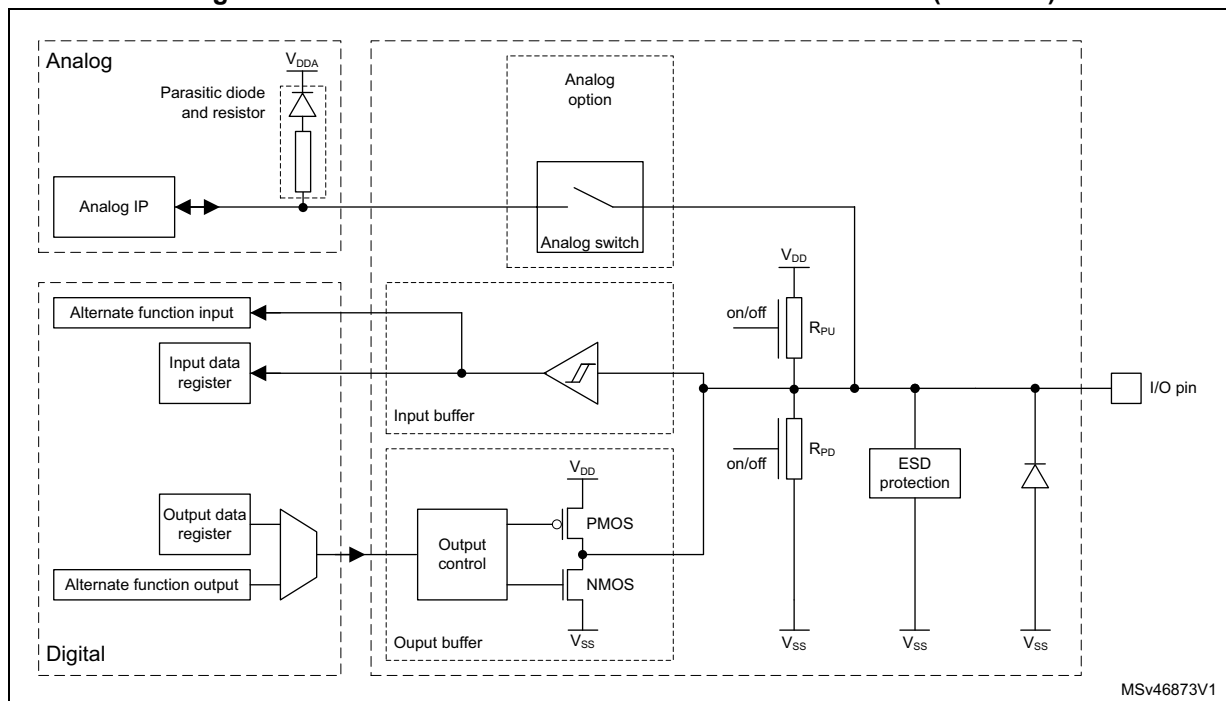
Figure 43. Structure of three-volt or five-volt tolerant GPIO (TT or FT)
