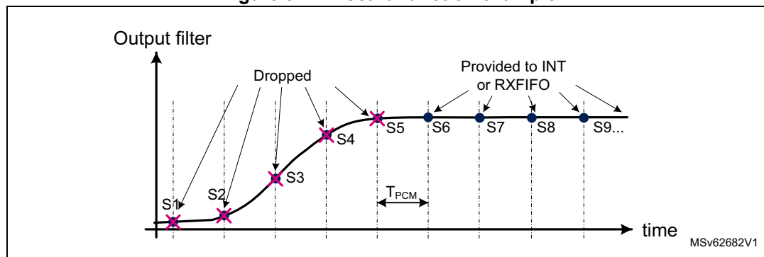
Figure 341. Discard function example
