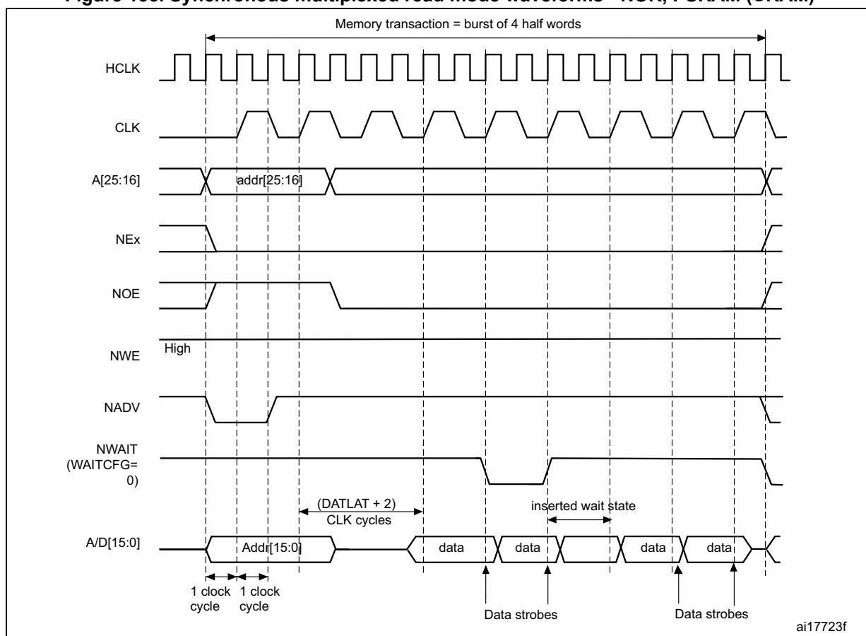
Figure 135. Synchronous multiplexed read mode waveforms - NOR, PSRAM (CRAM)
