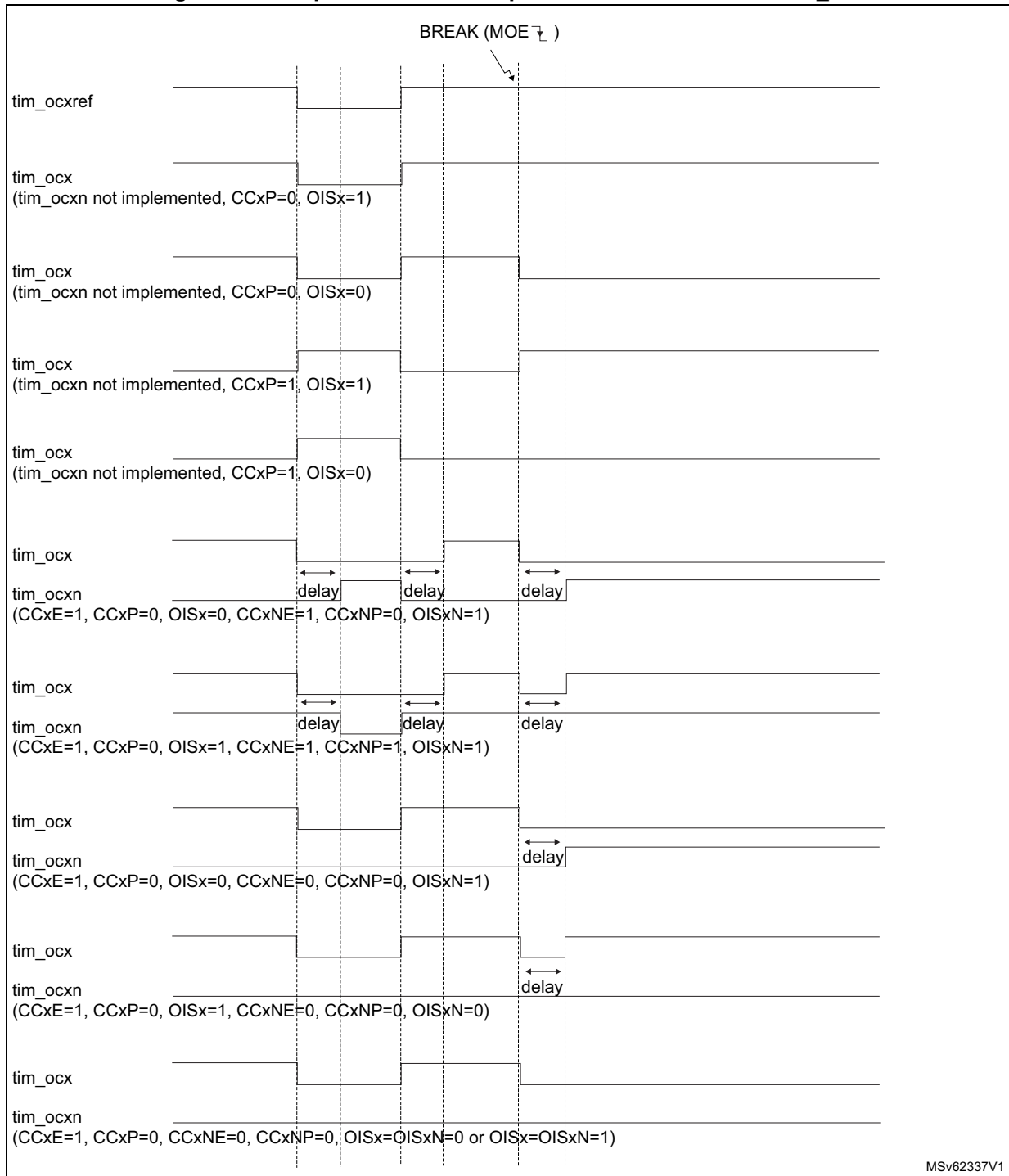
Figure 706. Output behavior in response to a break event on tim_brk
