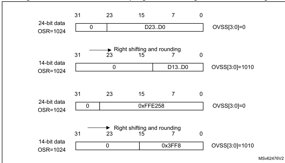
Figure 247. 14-bit result oversampling with 10-bits right shift and rounding
