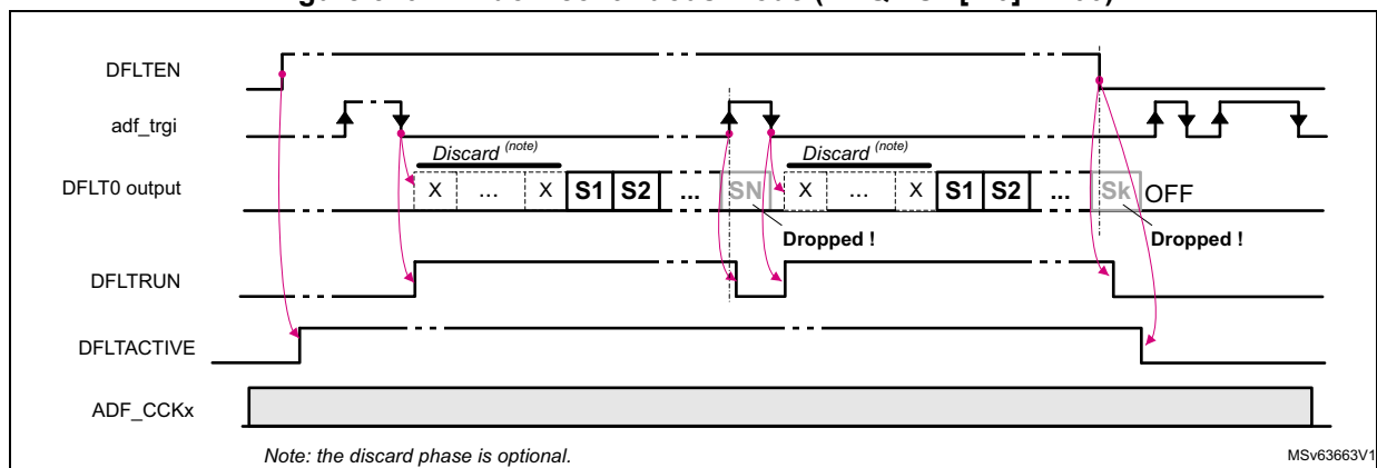
Figure 370. Window continuous mode (ACQMOD[2:0] = 100)
