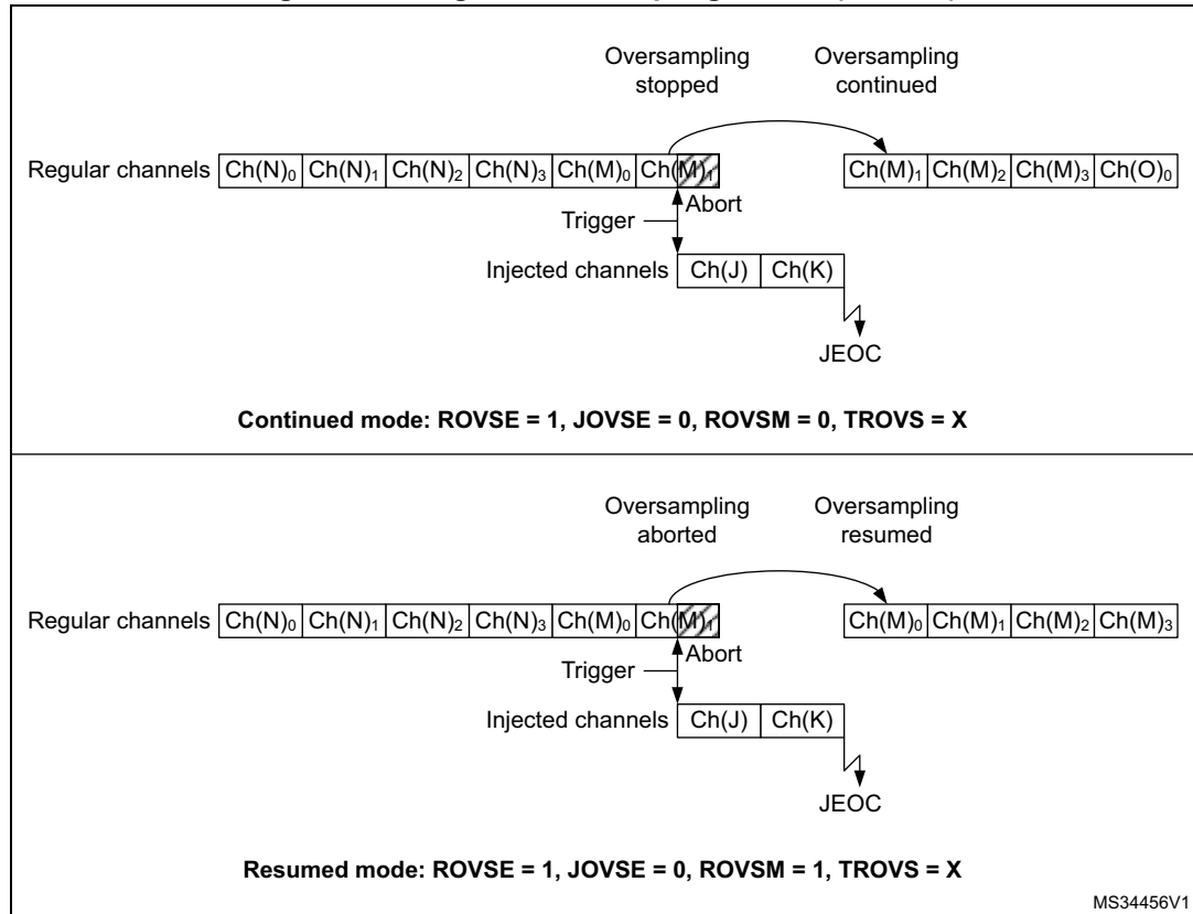
Figure 249. Regular oversampling modes (4x ratio)
