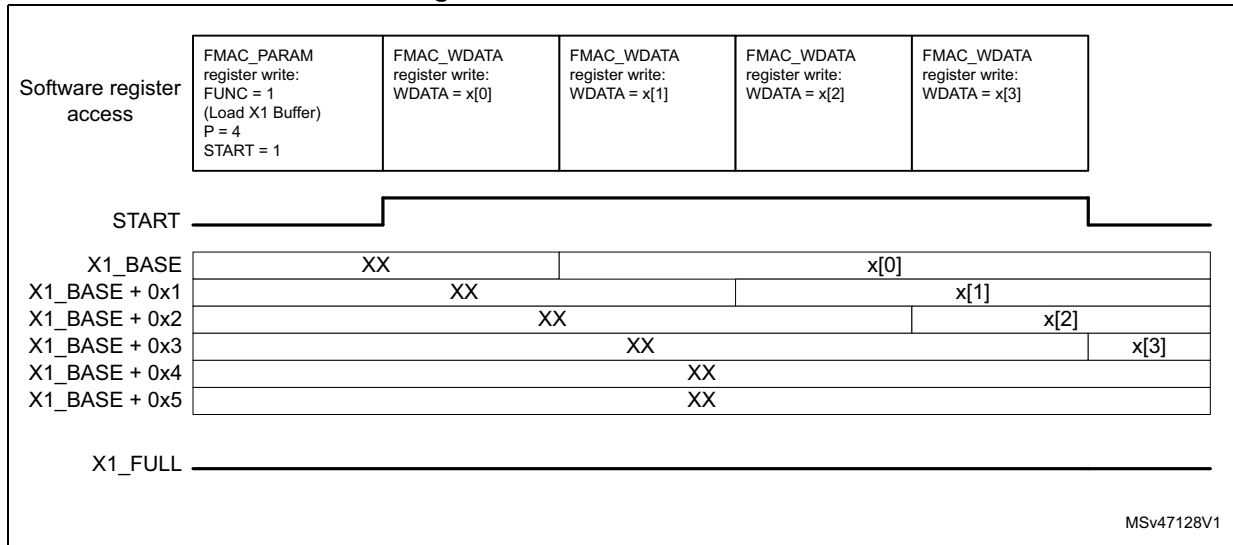
Figure 114. X1 buffer initialization
