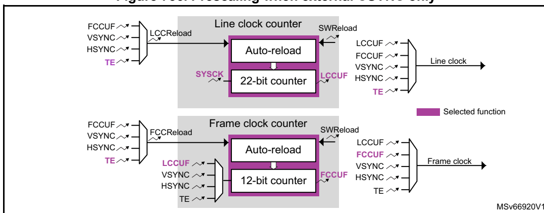
Figure 756. Prescaling when external CSYNC only
