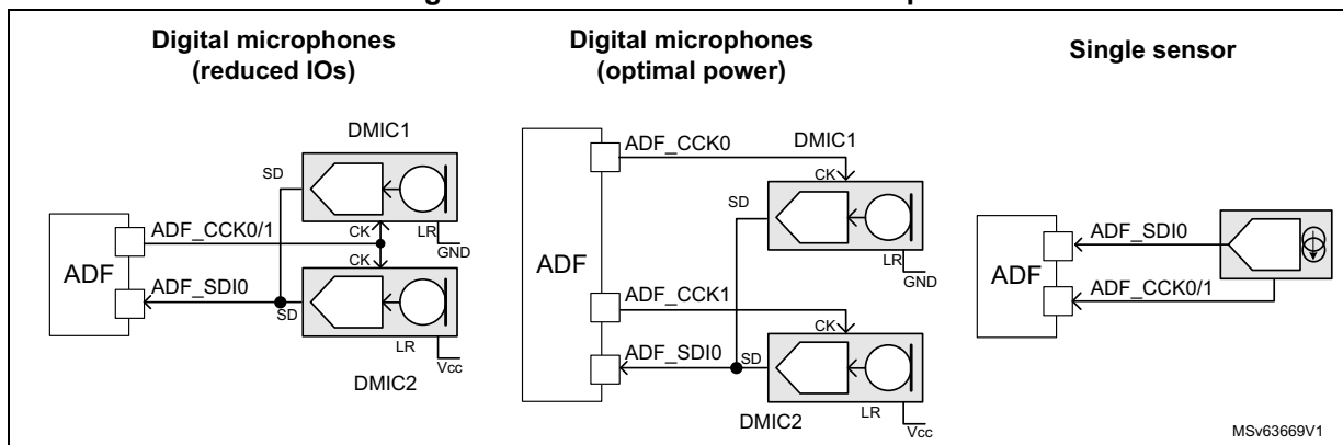
Figure 380. Sensor connection examples
