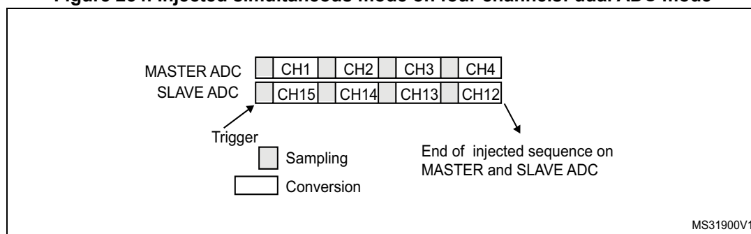
Figure 254. Injected simultaneous mode on four channels: dual ADC mode
