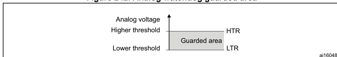
Figure 242. Analog watchdog guarded area
