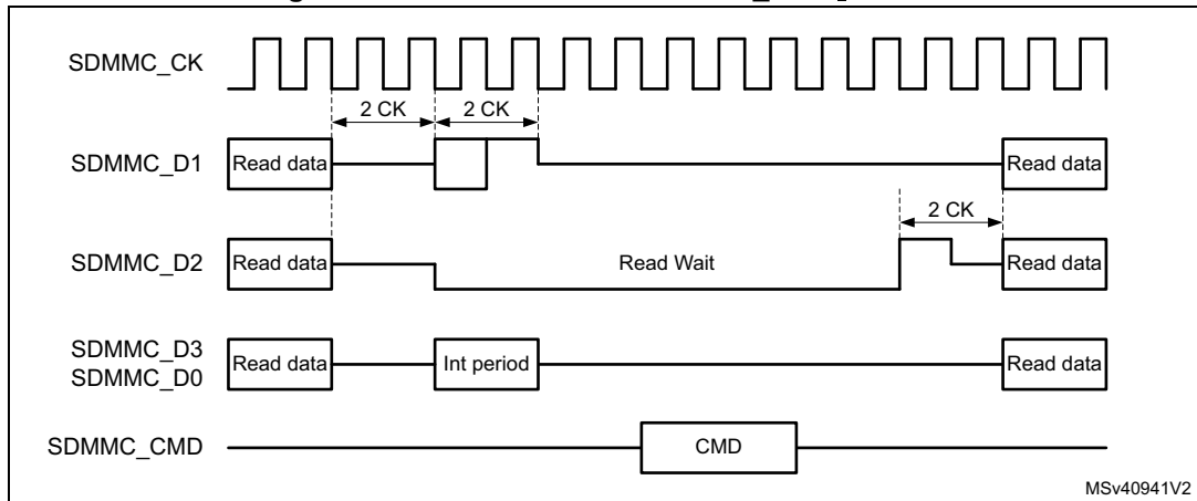
Figure 203. Read Wait with SDMMC_CK < 50 MHz
