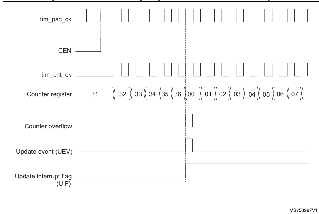
Figure 679. Counter timing diagram, internal clock divided by 1
