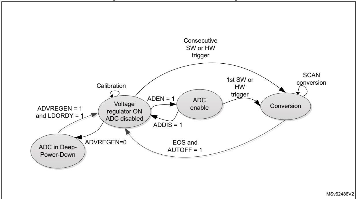
Figure 289. ADC behavior with WAIT = 0 and AUTOFF = 1
