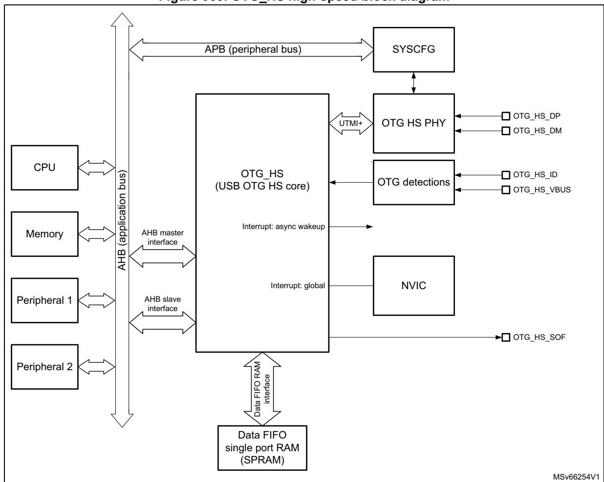
Figure 909. OTG_HS high-speed block diagram
