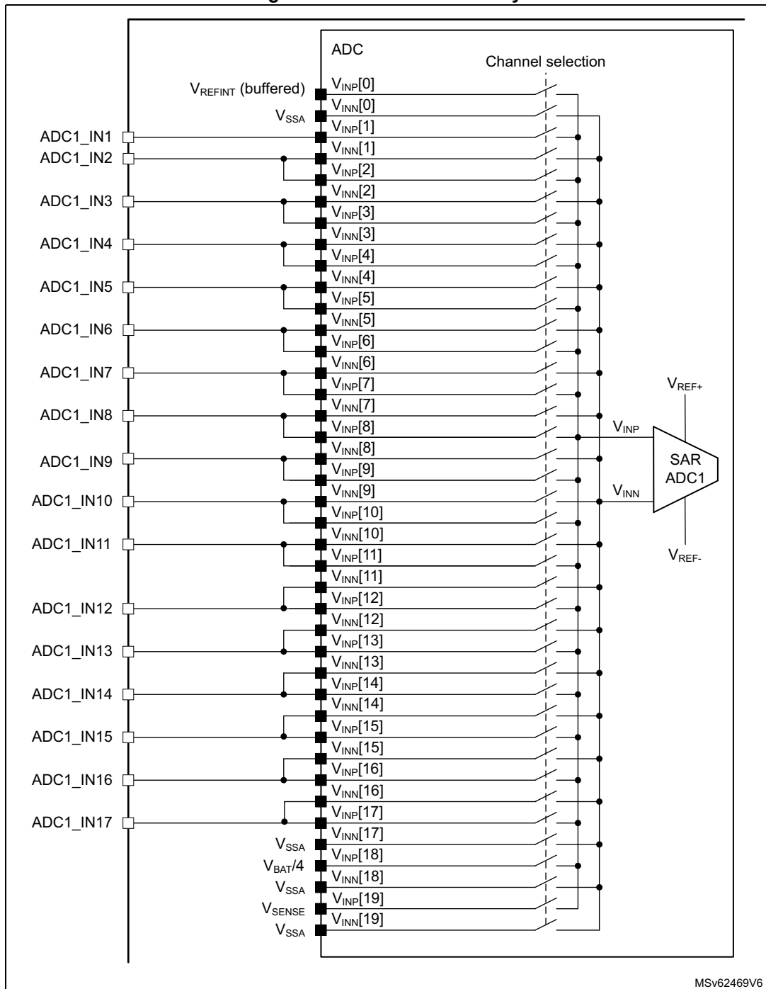
Figure 217. ADC1 connectivity
