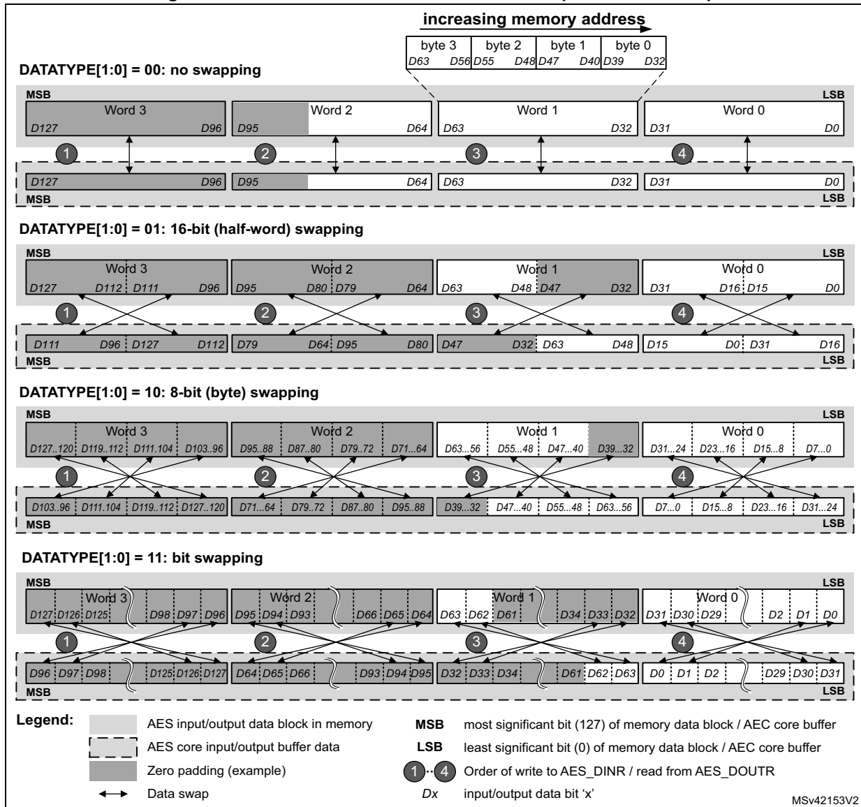
Figure 491. 128-bit block construction with respect to data swap
