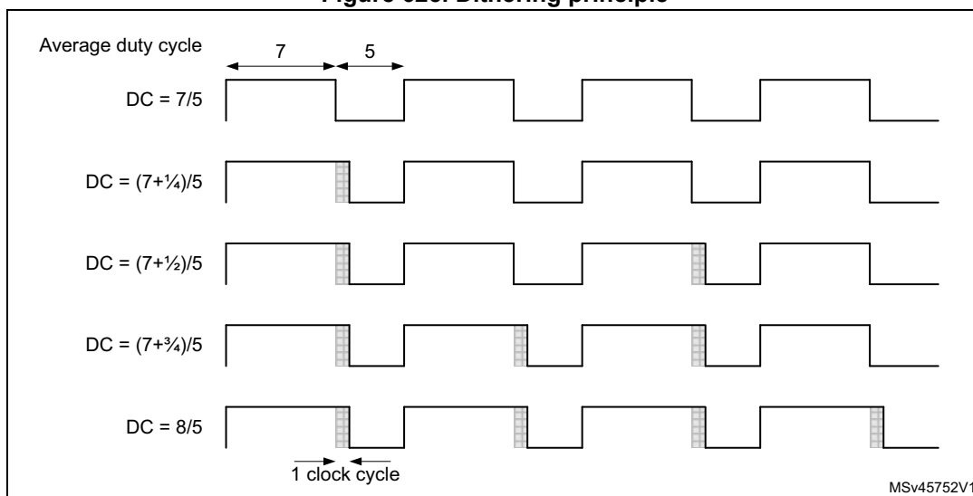
Figure 625. Dithering principle
