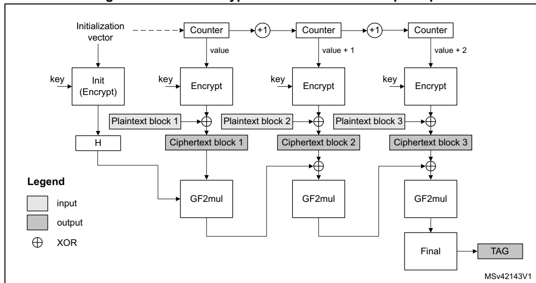
Figure 457. GCM encryption and authentication principle
