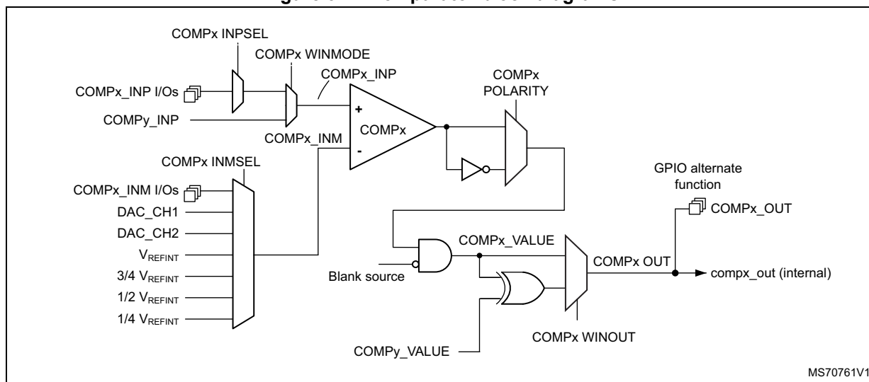
Figure 312. Comparator block diagrams
