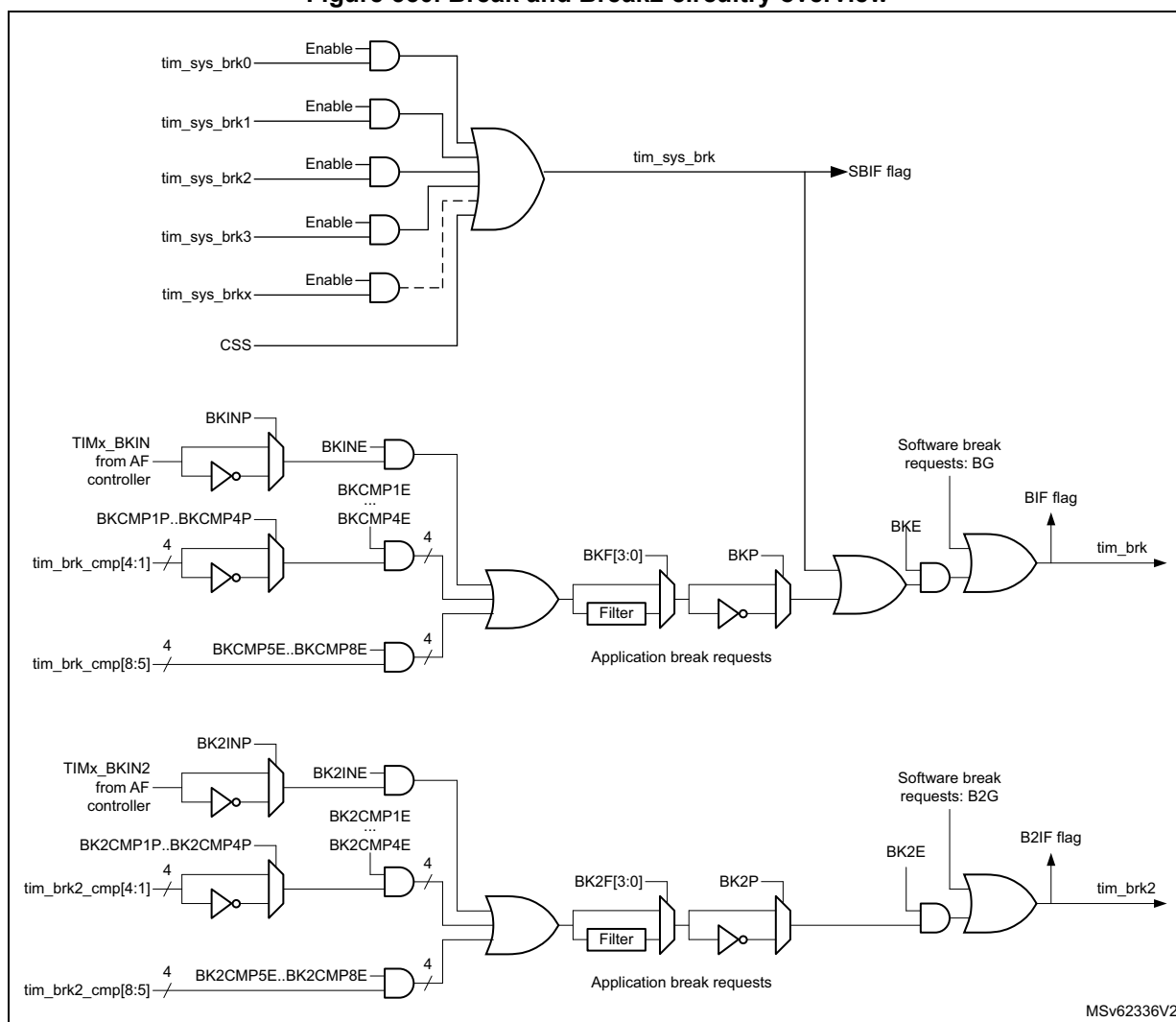
Figure 550. Break and Break2 circuitry overview
