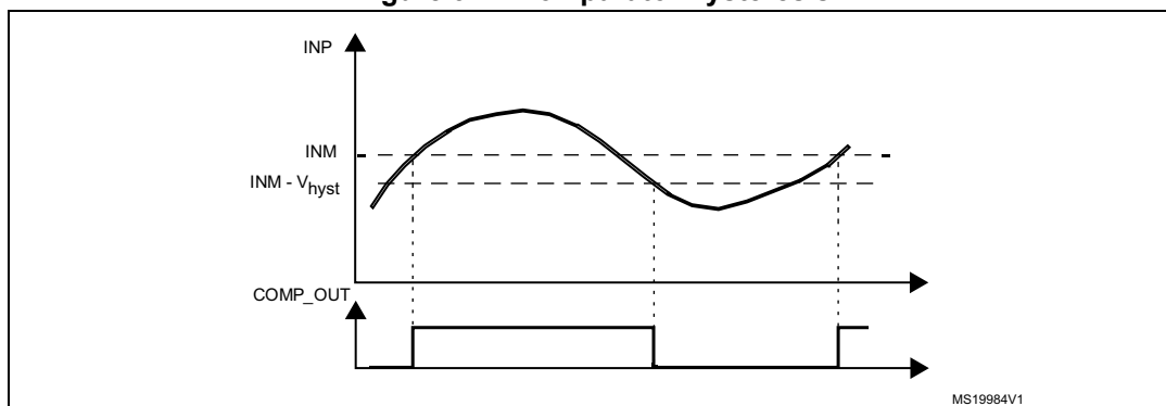
Figure 314. Comparator hysteresis
