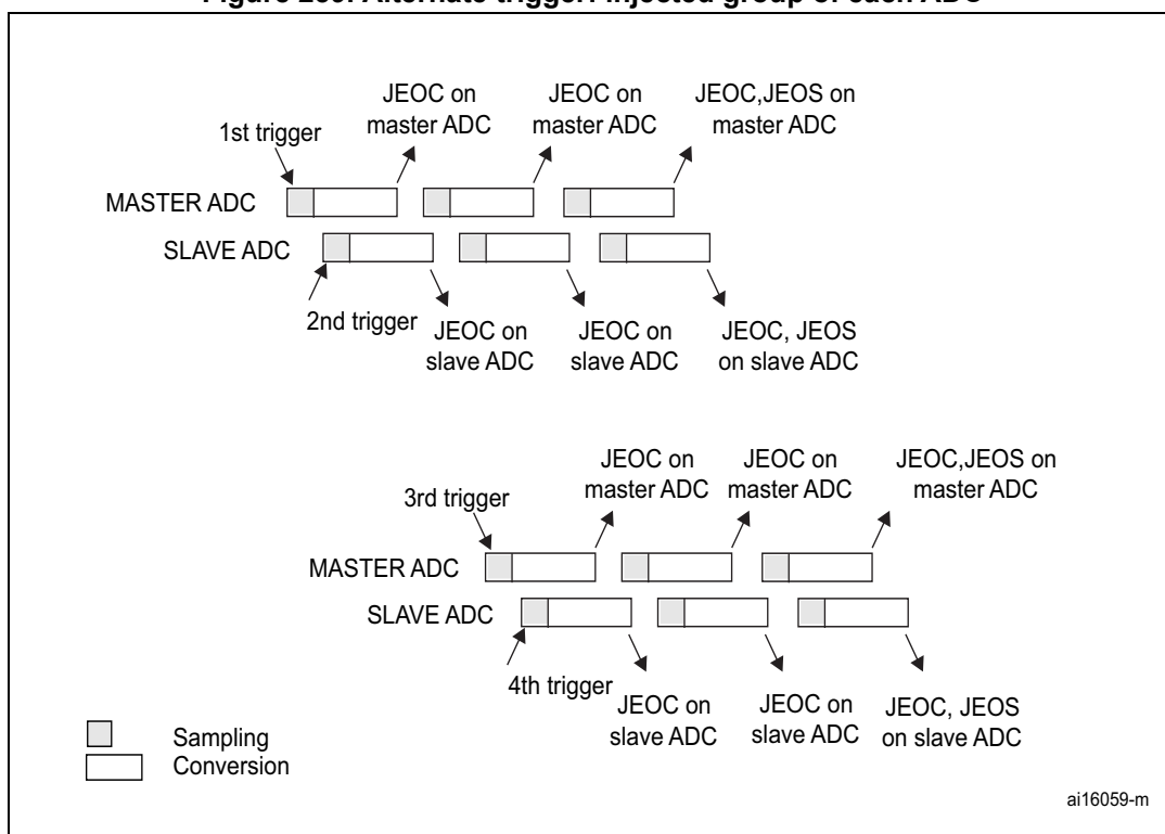
Figure 259. Alternate trigger: injected group of each ADC
