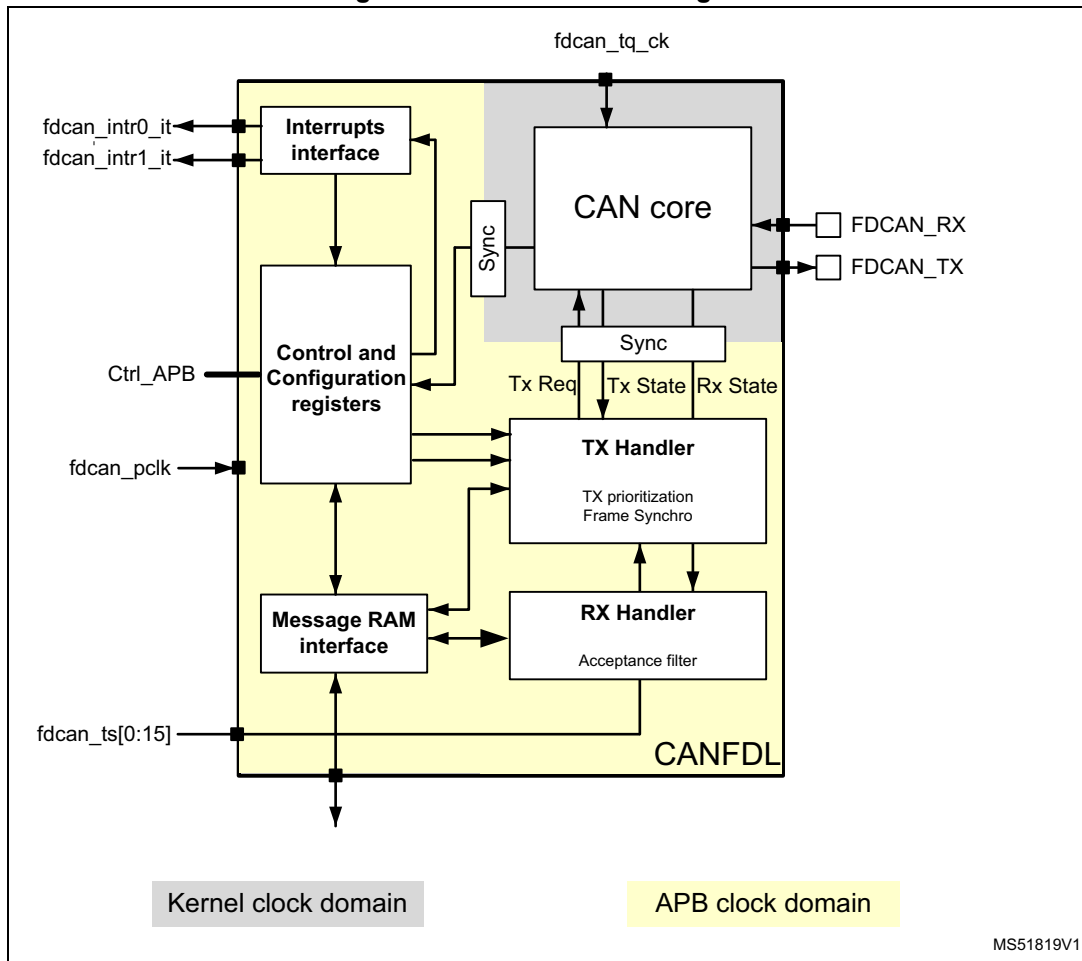
Figure 874. FDCAN block diagram
