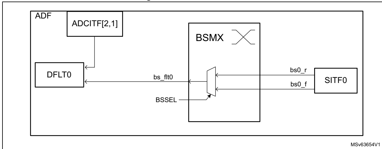
Figure 360. BSMX overview
