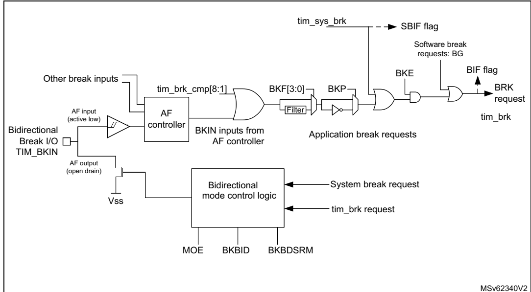
Figure 554. Output redirection (tim_brk2 request not represented)
