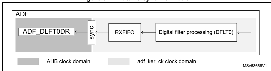
Figure 377. Data re-synchronization
