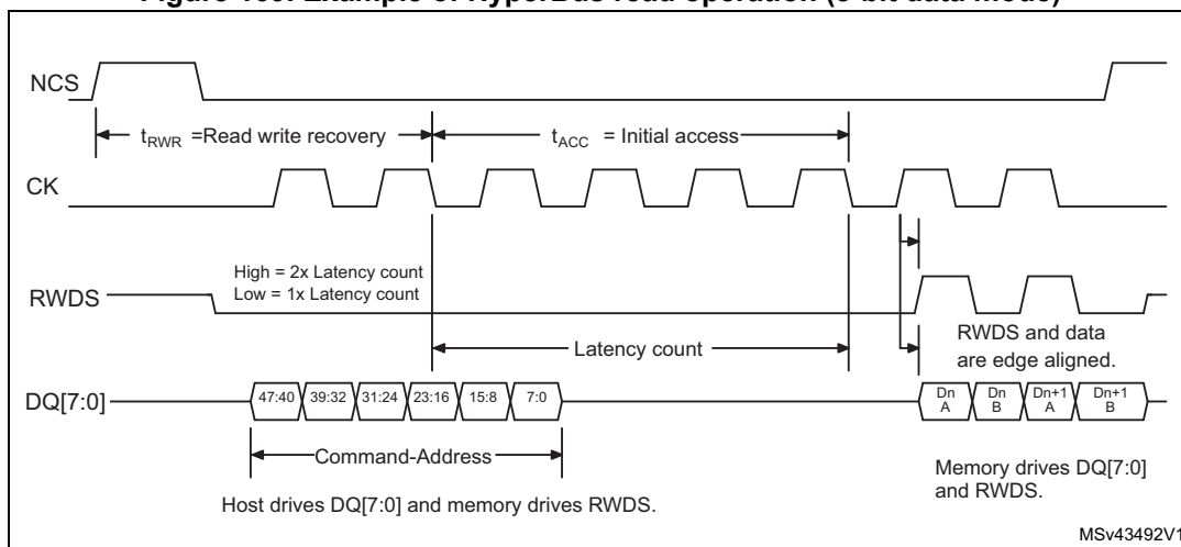
Figure 169. Example of HyperBus read operation (8-bit data mode)
