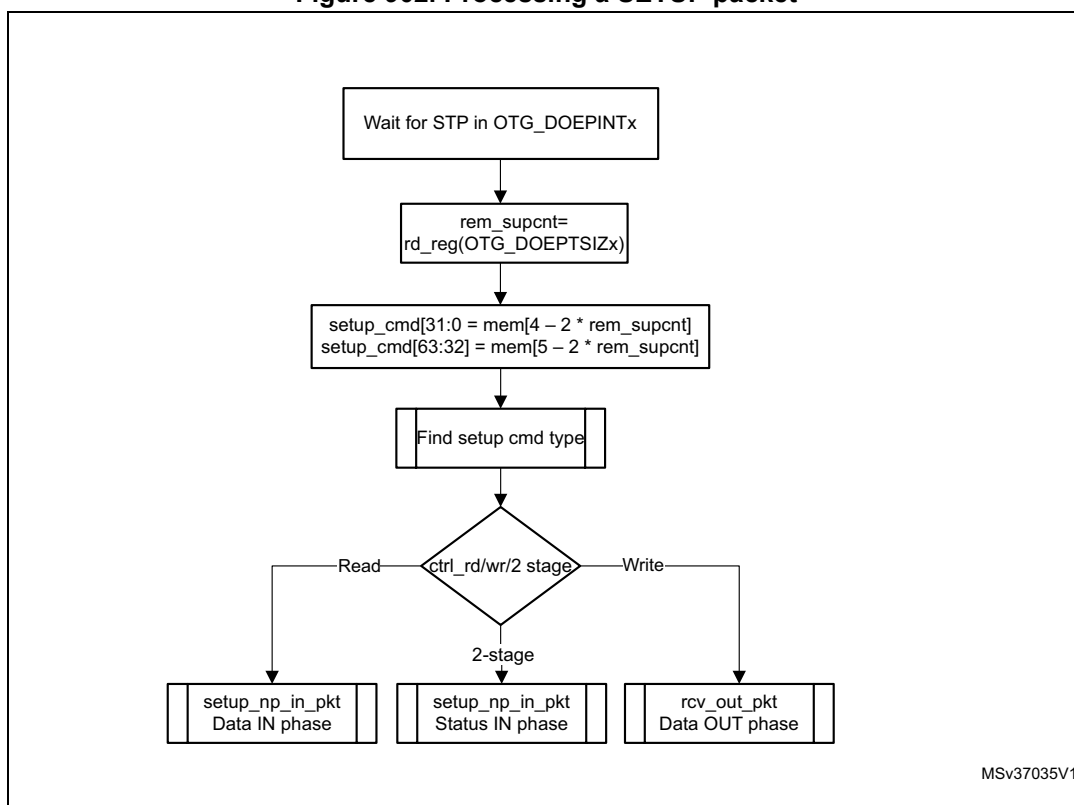
Figure 902. Processing a SETUP packet
