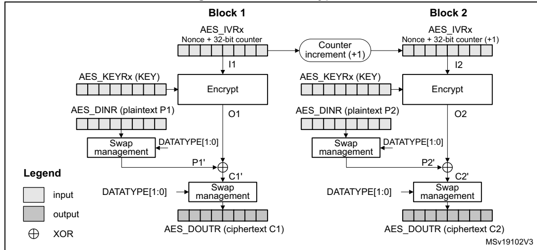
Figure 468. CTR encryption
