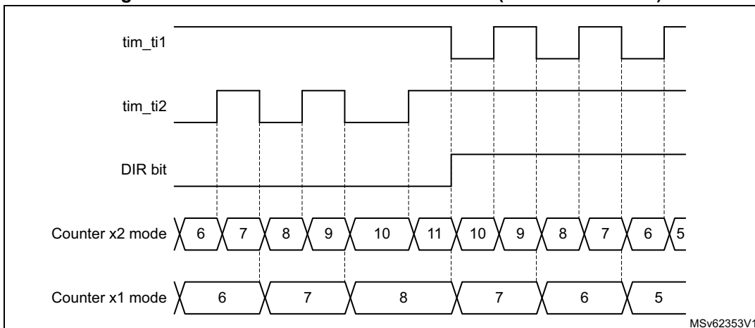
Figure 644. Directional clock encoder mode (CC1P = CC2P = 0)
