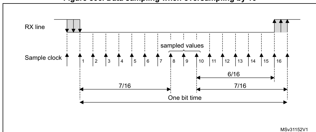
Figure 806. Data sampling when oversampling by 16
