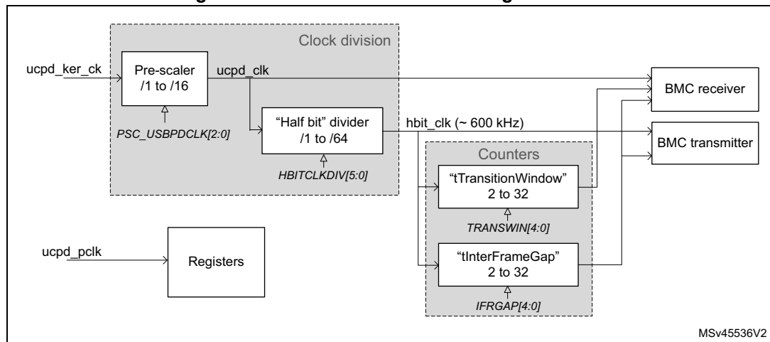
Figure 937. Clock division and timing elements
