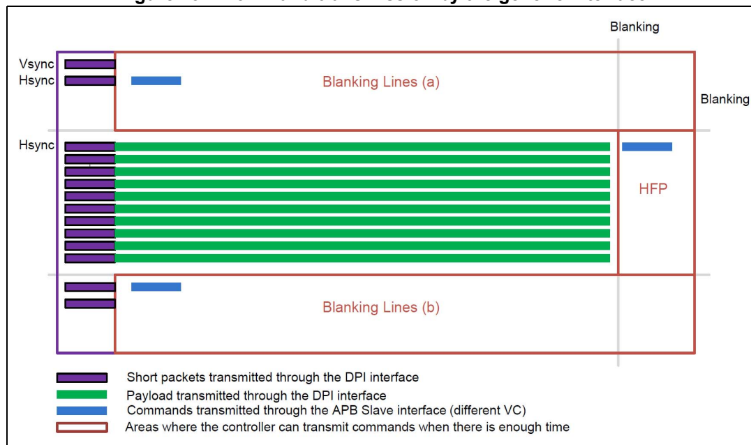
Figure 432. Command transmission by the generic interface
