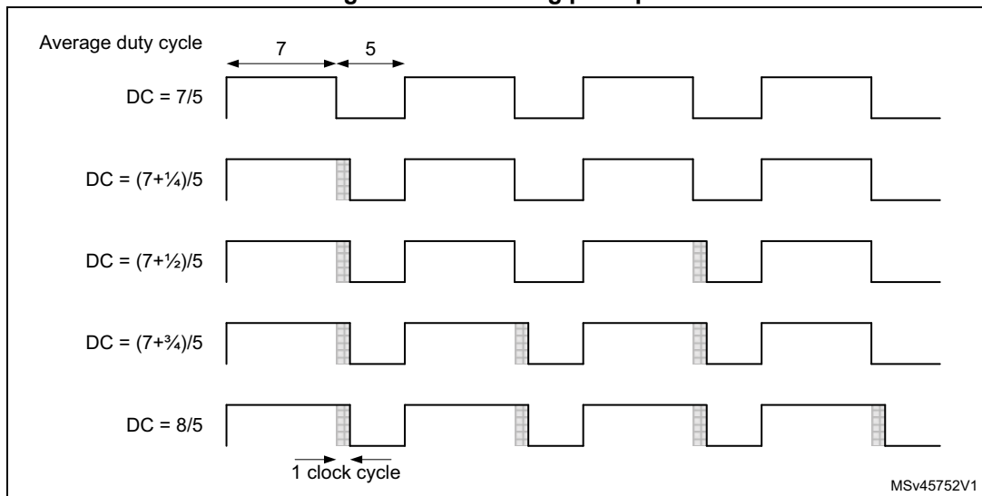
Figure 538. Dithering principle
