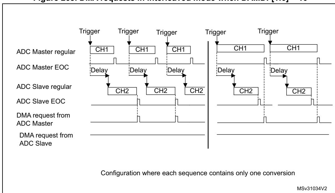
Figure 268. DMA requests in interleaved mode when DAMDF[1:0] = 10
