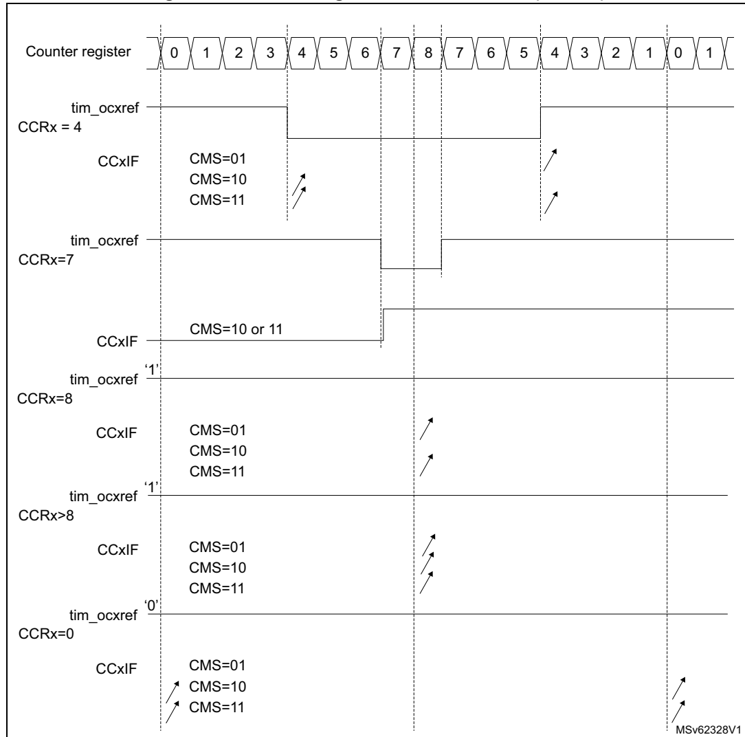
Figure 537. Center-aligned PWM waveforms (ARR=8)
