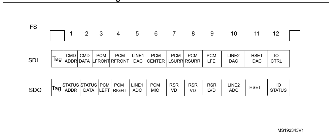
Figure 864. AC'97 audio frame
