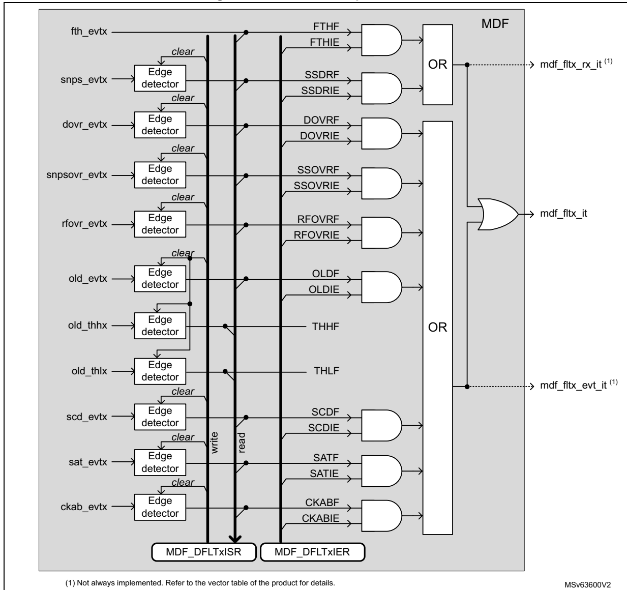
Figure 350. MDF interrupt interface
