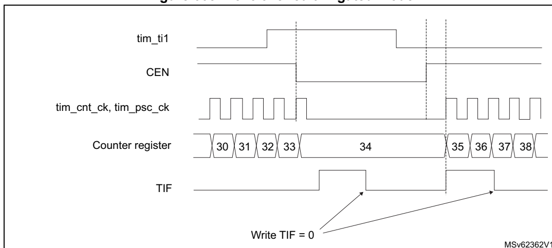
Figure 665. Control circuit in gated mode
