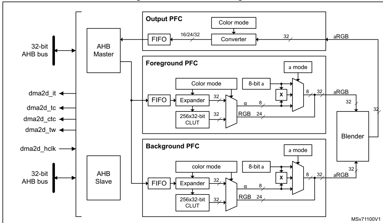
Figure 91. DMA2D block diagram
