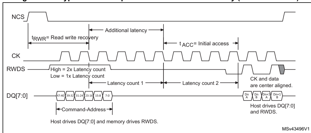
Figure 172. HyperBus write operation with additional latency (8-bit data mode)
