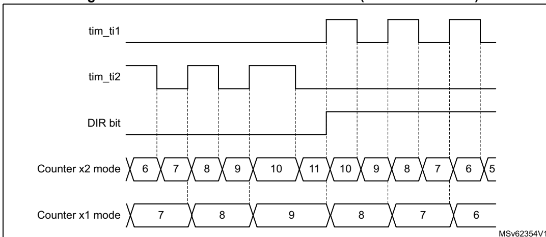
Figure 645. Directional clock encoder mode (CC1P = CC2P = 1)
