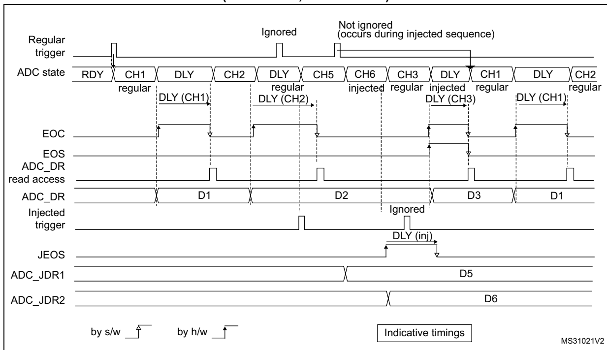
Figure 238. AUTDLY = 1, regular hardware conversions interrupted by injected conversions (DISCEN = 0; JDISCEN = 0)
