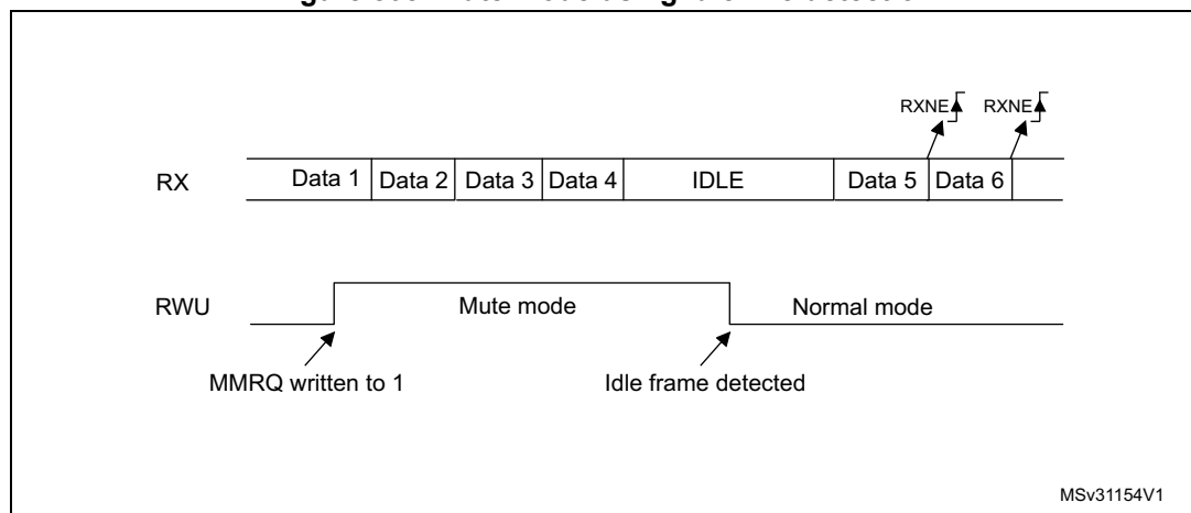
Figure 808. Mute mode using Idle line detection
