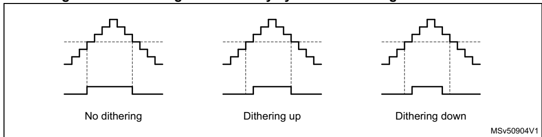
Figure 630. Dithering effect on duty cycle in center-aligned PWM mode
