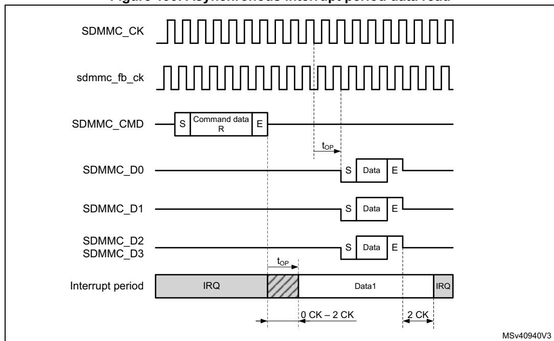
Figure 199. Asynchronous interrupt period data read
