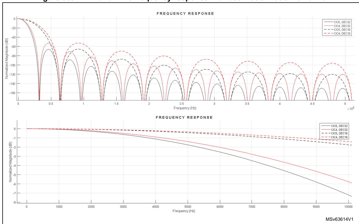
Figure 363. CIC4 and CIC5 frequency response with decimation ratio = 32 or 16
