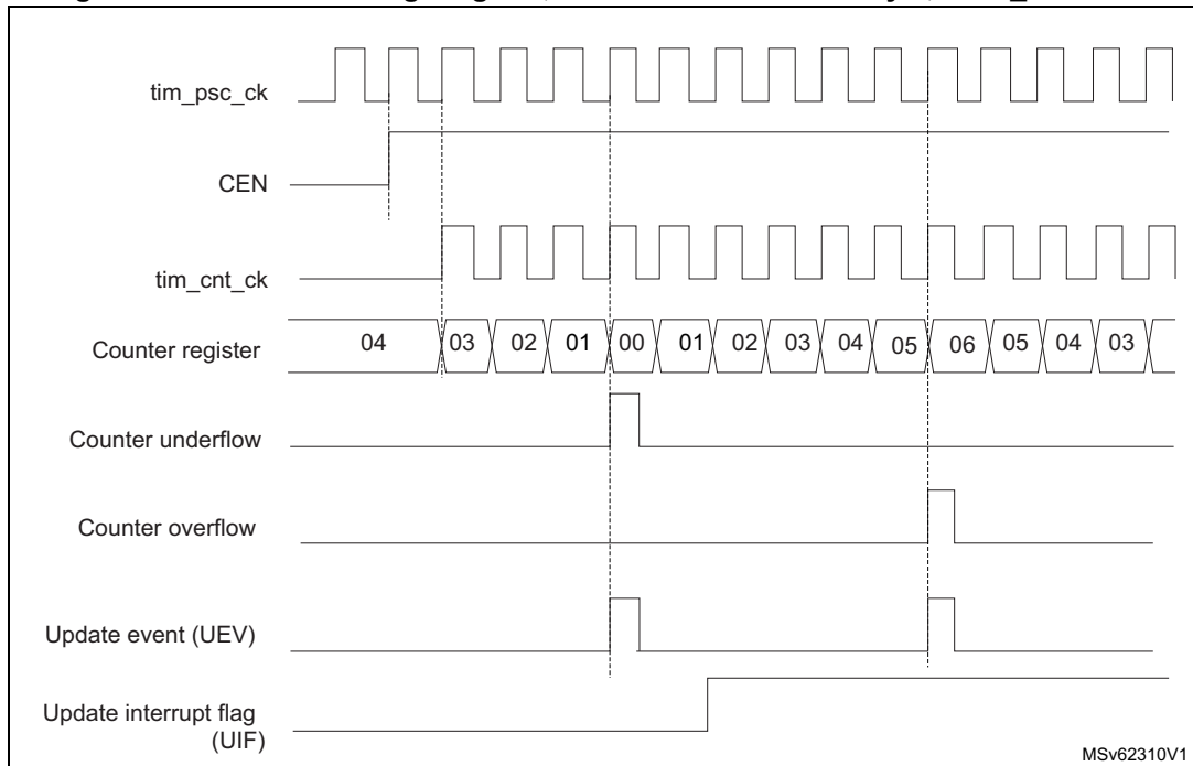
Figure 607. Counter timing diagram, internal clock divided by 1, TIMx_ARR=0x6
