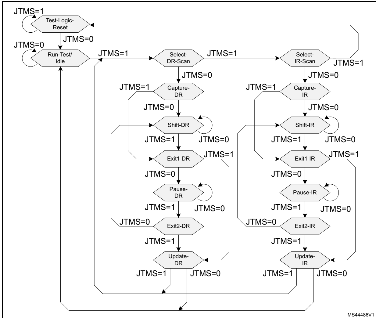
Figure 948. JTAG TAP state machine
