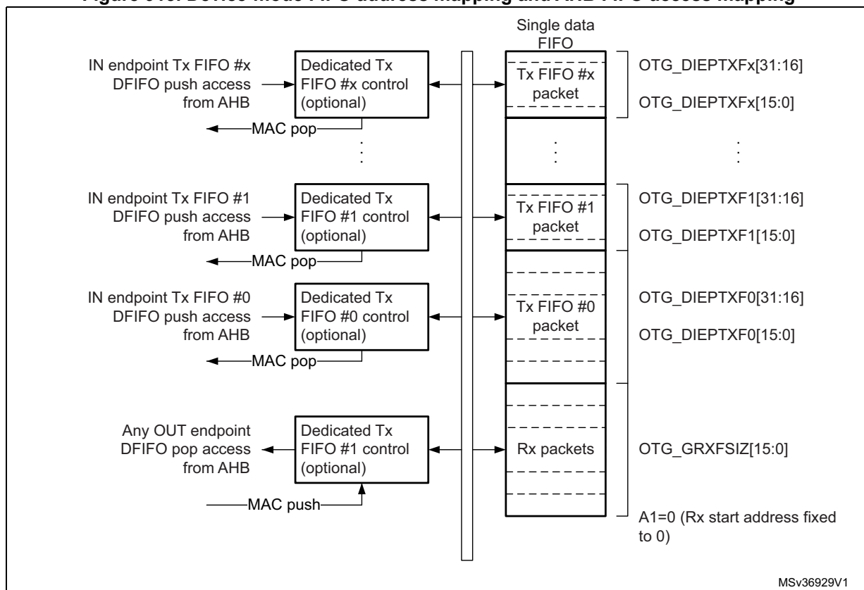
Figure 915. Device-mode FIFO address mapping and AHB FIFO access mapping
