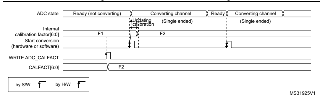
Figure 274. Calibration factor forcing
