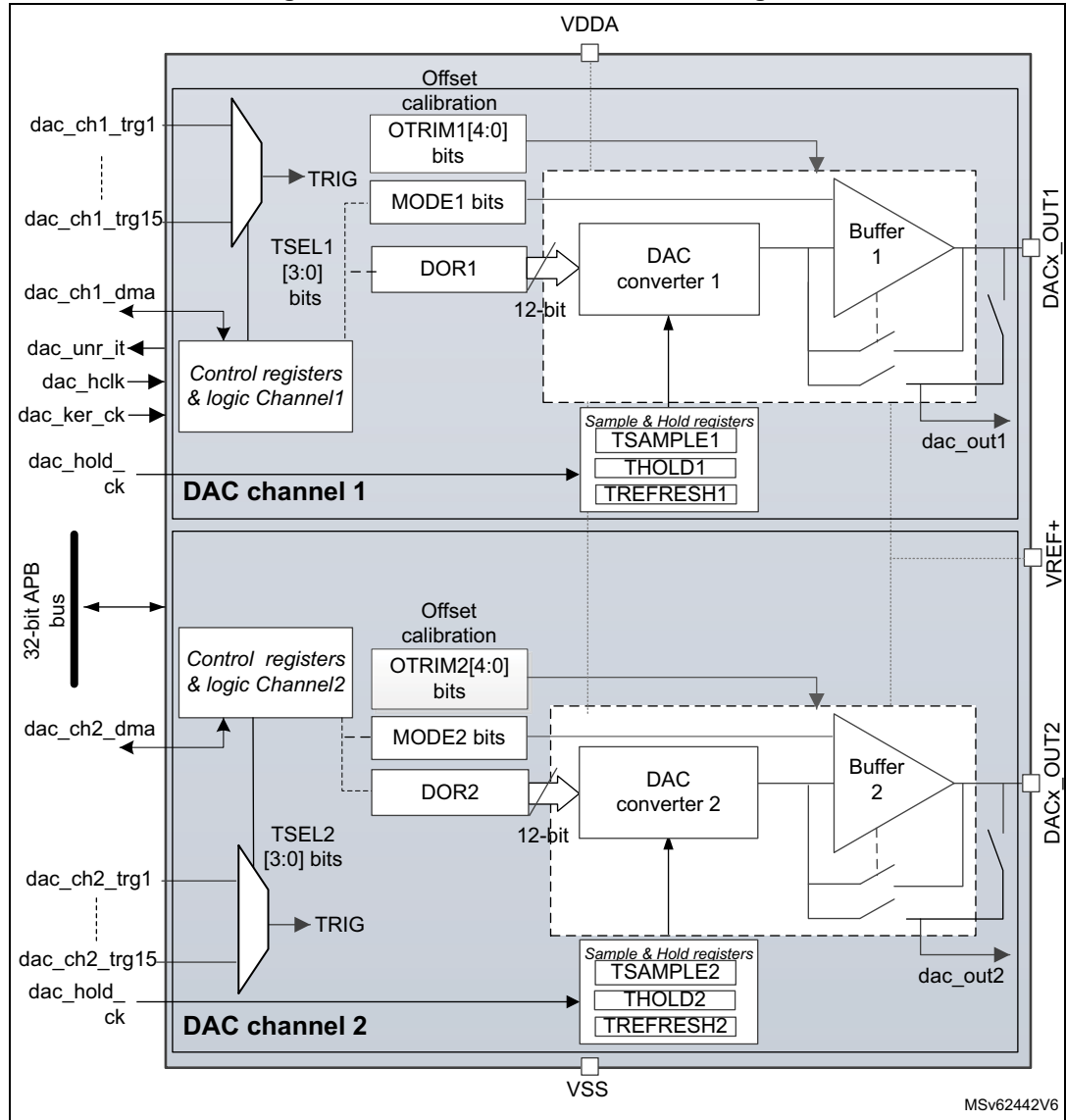
Figure 302. Dual-channel DAC block diagram
