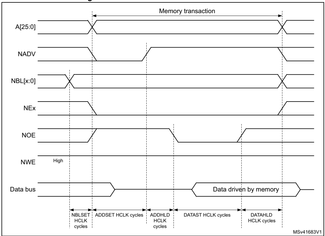
Figure 128. Mode D read access waveforms
