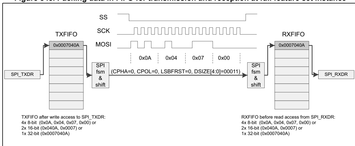
Figure 848. Packing data in FIFO for transmission and reception at full feature set instance
