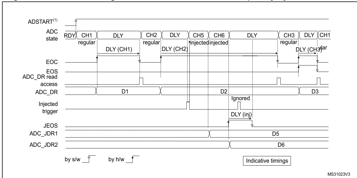
Figure 240. AUTODLY = 1, regular continuous conversions interrupted by injected conversions
