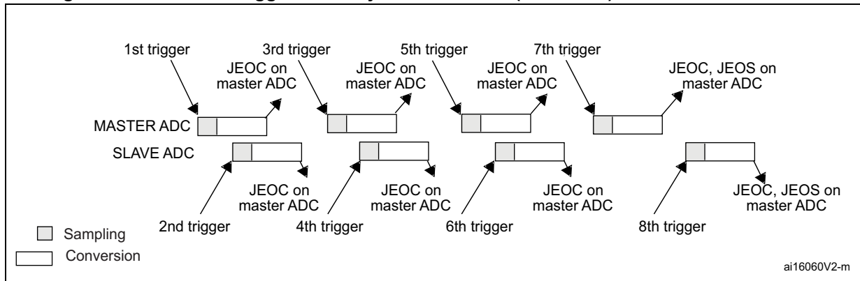
Figure 260. Alternate trigger: Four injected channels (each ADC) in discontinuous mode
