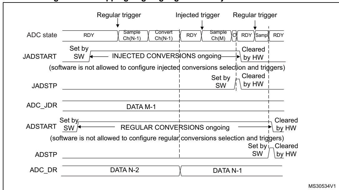
Figure 224. Stopping ongoing regular and injected conversions
