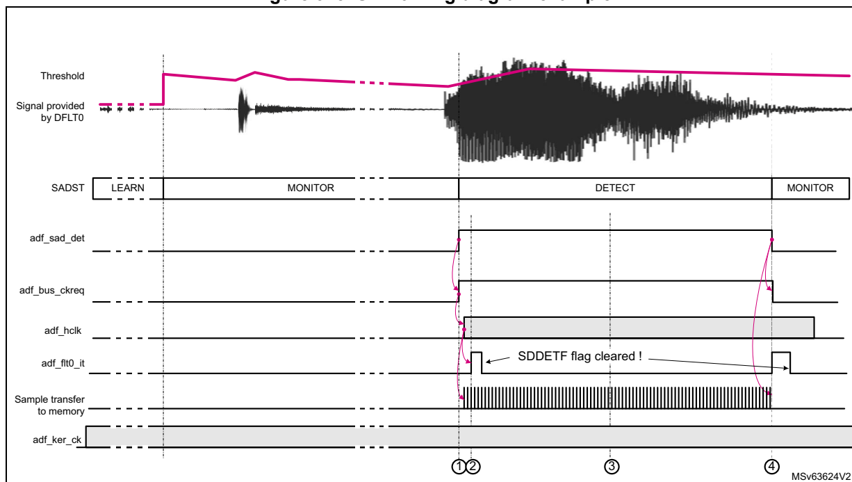
Figure 375. SAD timing diagram example
