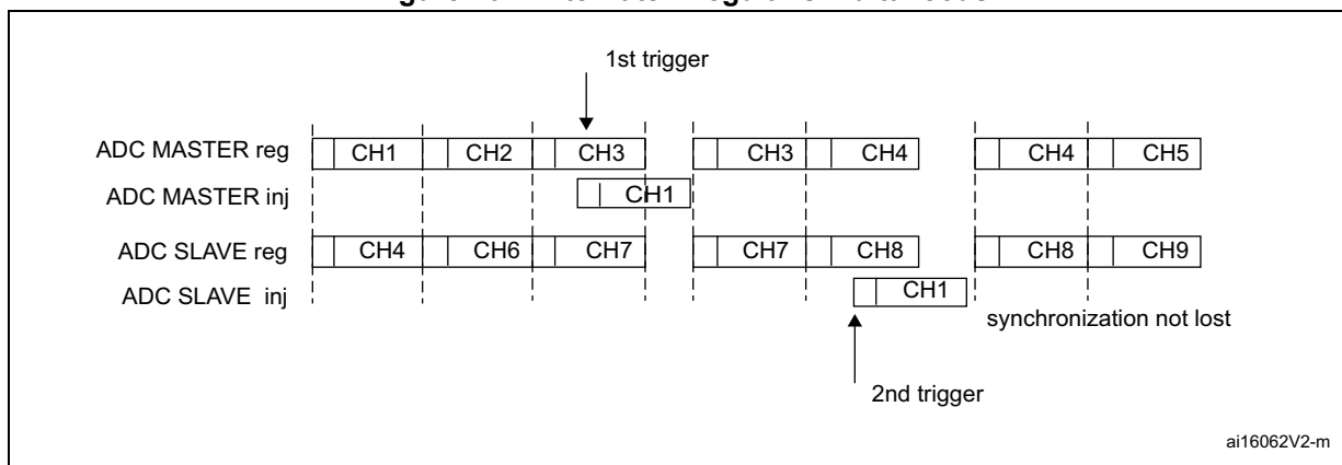
Figure 261. Alternate + regular simultaneous
