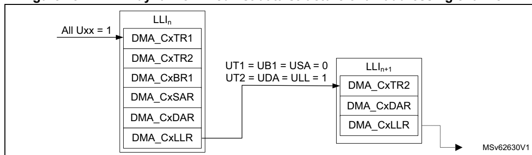
Figure 75. LPDMA dynamic linked-list data structure of an addressing channel x
