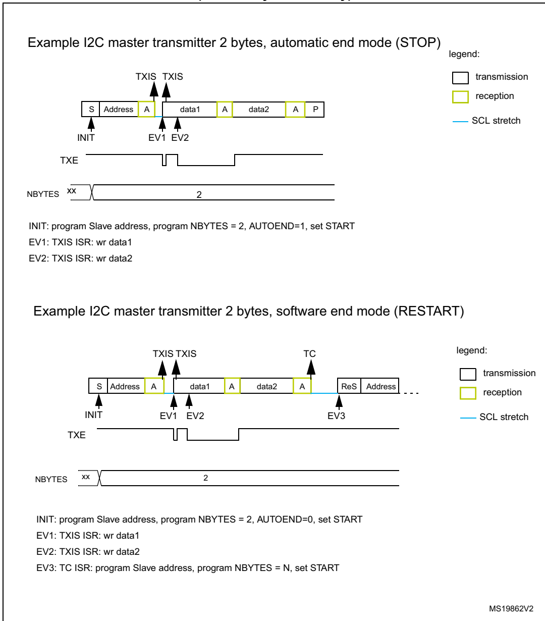
Figure 789. Transfer bus diagrams for I2C master transmitter (mandatory events only)
