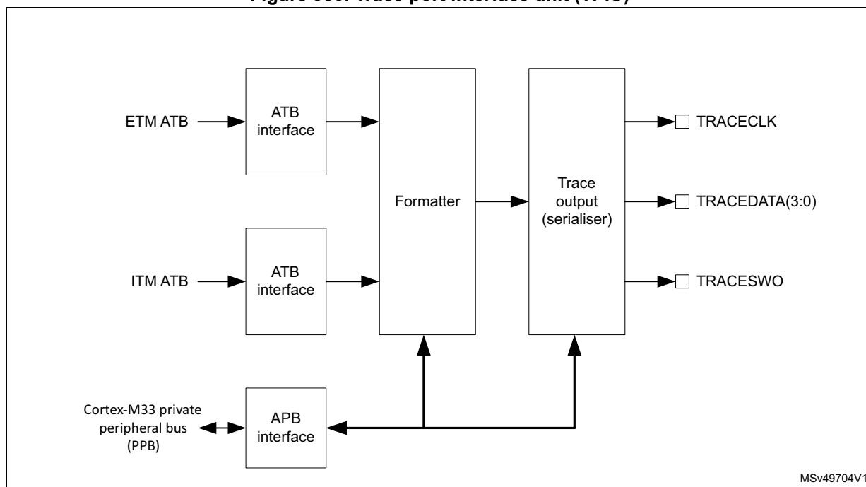
Figure 950. Trace port interface unit (TPIU)
