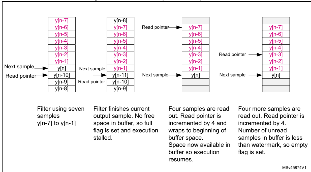
Figure 111. Circular output buffer operation
