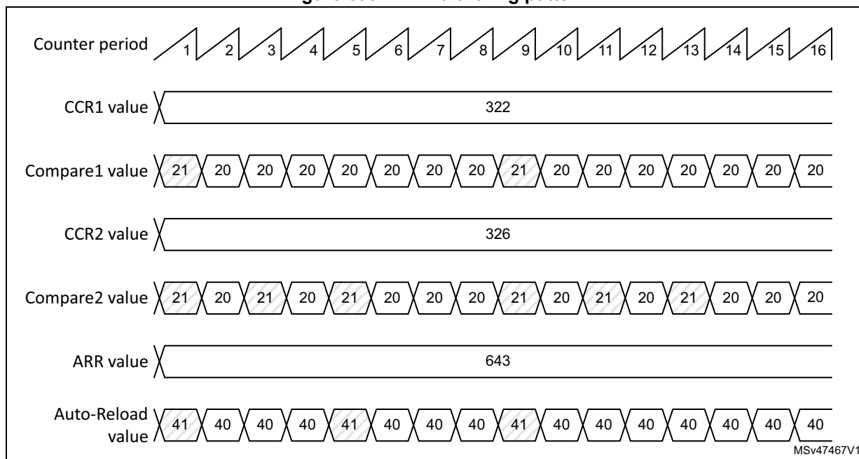
Figure 699. PWM dithering pattern
