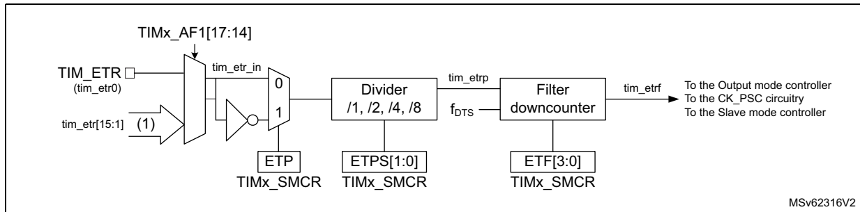
Figure 524. External trigger input block
