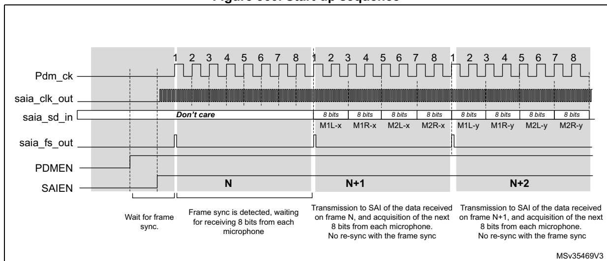
Figure 860. Start-up sequence
