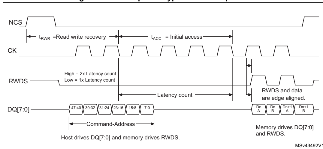
Figure 149. Example of HyperBus read operation
