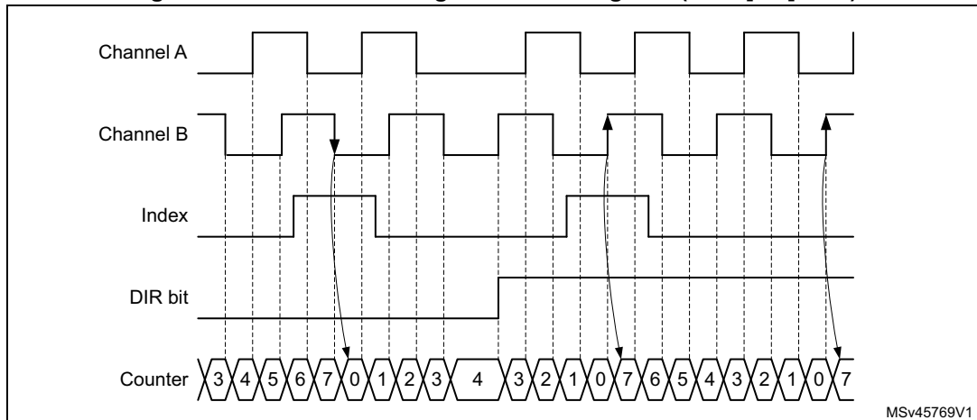
Figure 650. Counter reading with index ungated (IPOS[1:0] = 00)
