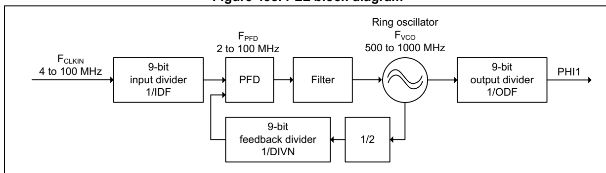
Figure 438. PLL block diagram
