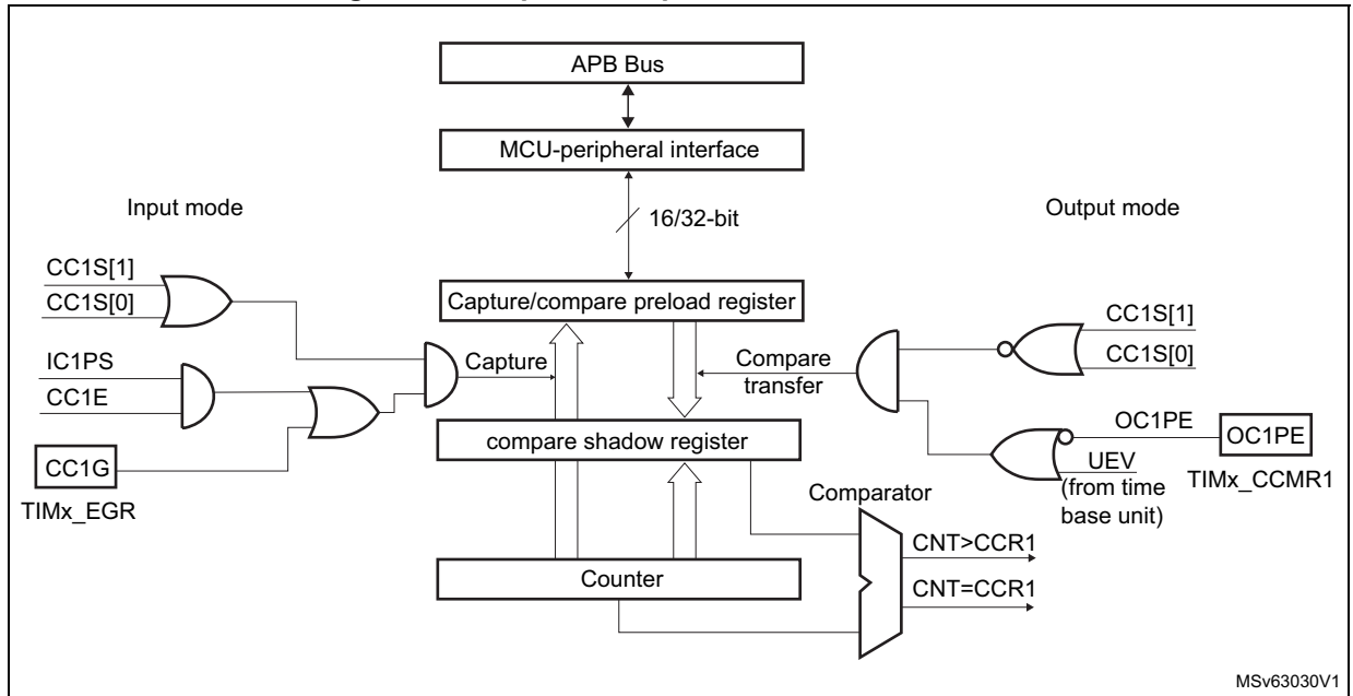
Figure 531. Capture/compare channel 1 main circuit
