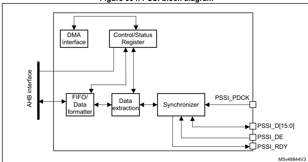
Figure 395. Top-level block diagram
