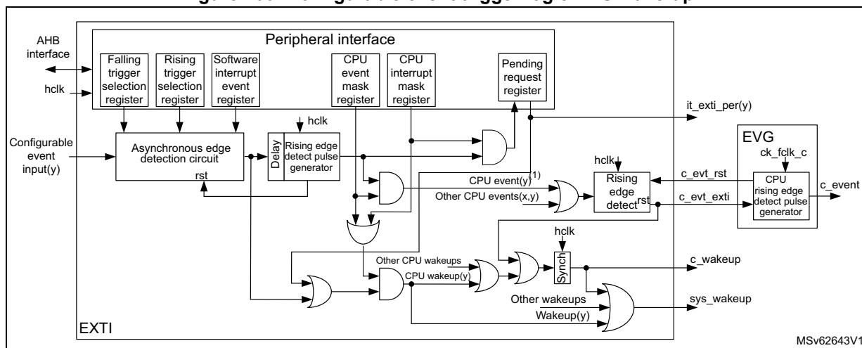
Figure 100. Configurable event trigger logic CPU wake-up
