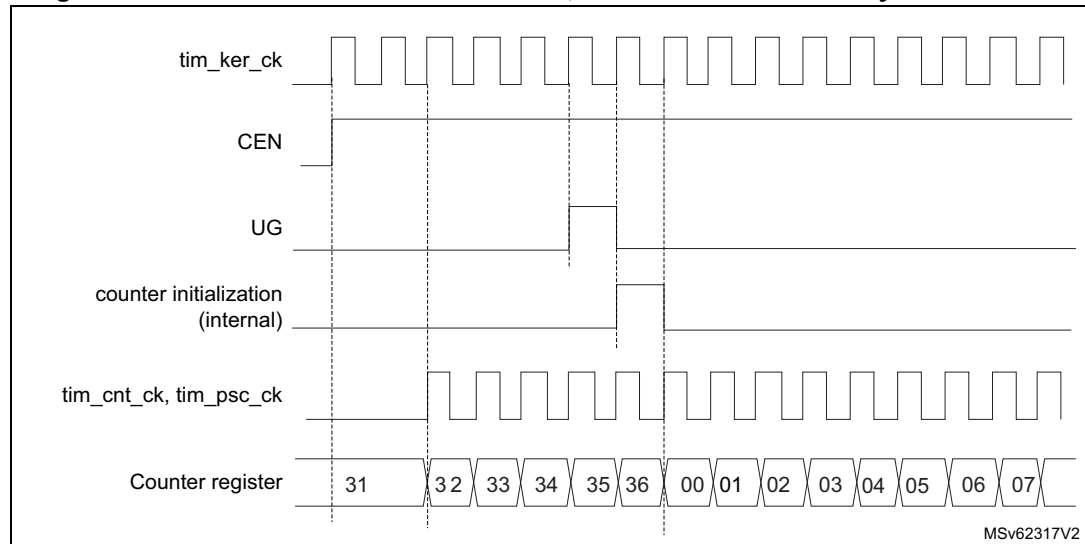
Figure 686. Control circuit in normal mode, internal clock divided by 1
