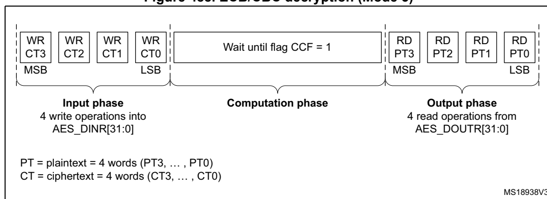
Figure 488. ECB/CBC decryption (Mode 3)
