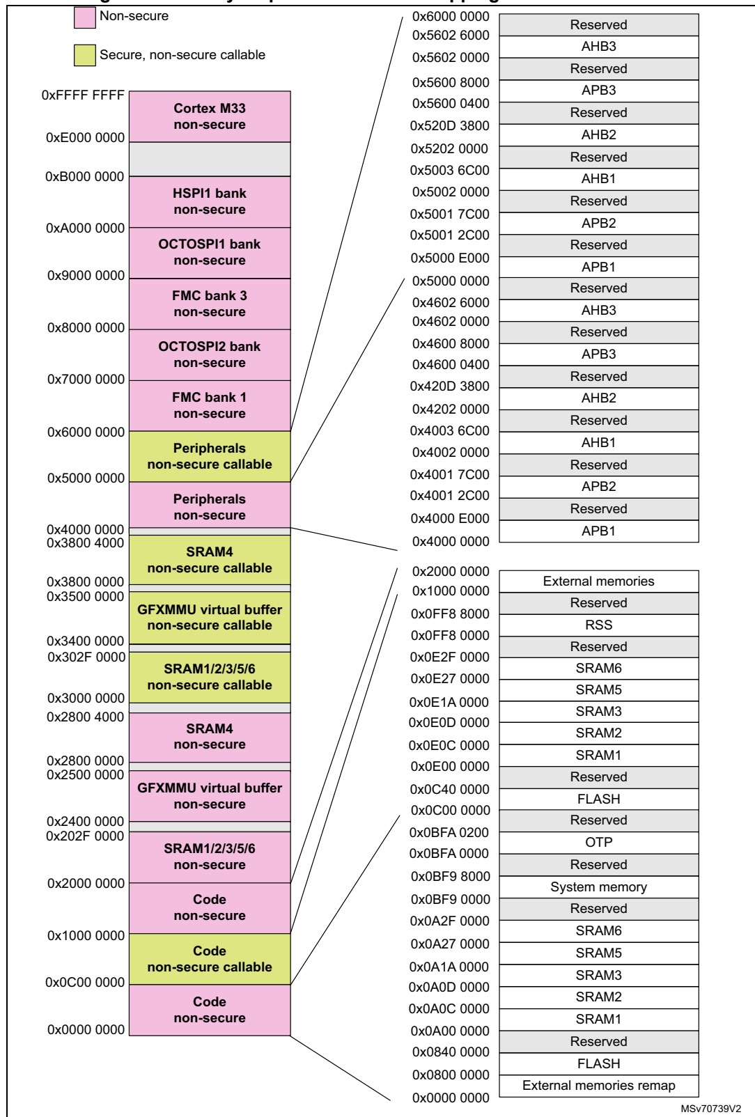
Figure 6. Memory map based on IDAU mapping for STM32U5Fx/5Gx
