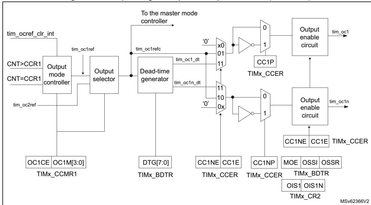
Figure 691. Output stage of capture/compare channel (channel 1)
