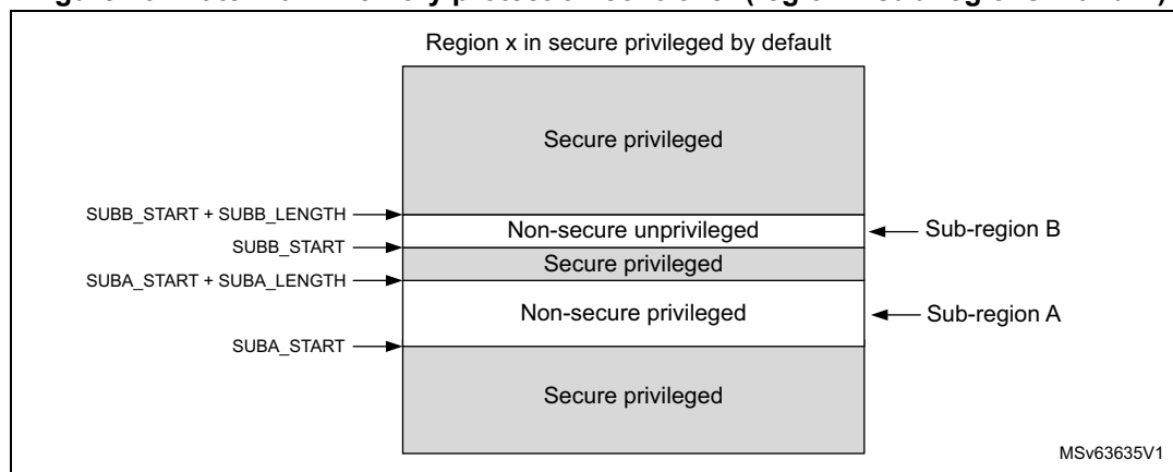
Figure 20. Watermark memory protection controller (region x/sub-regions A and B)
