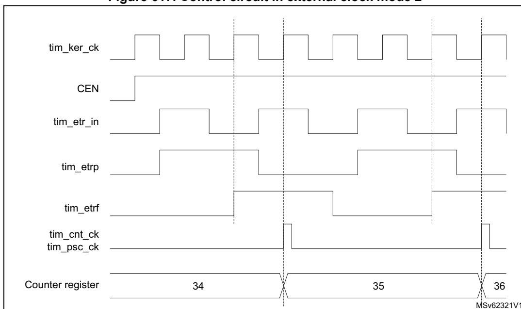
Figure 617. Control circuit in external clock mode 2
