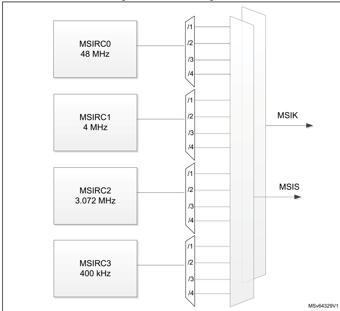
Figure 38. MSI block diagram
