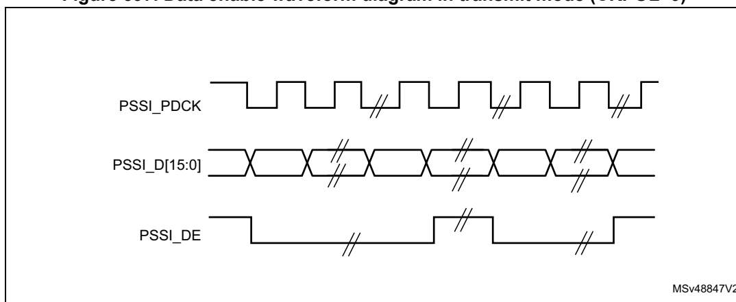
Figure 397. Data enable waveform diagram in transmit mode (CKPOL=0)
