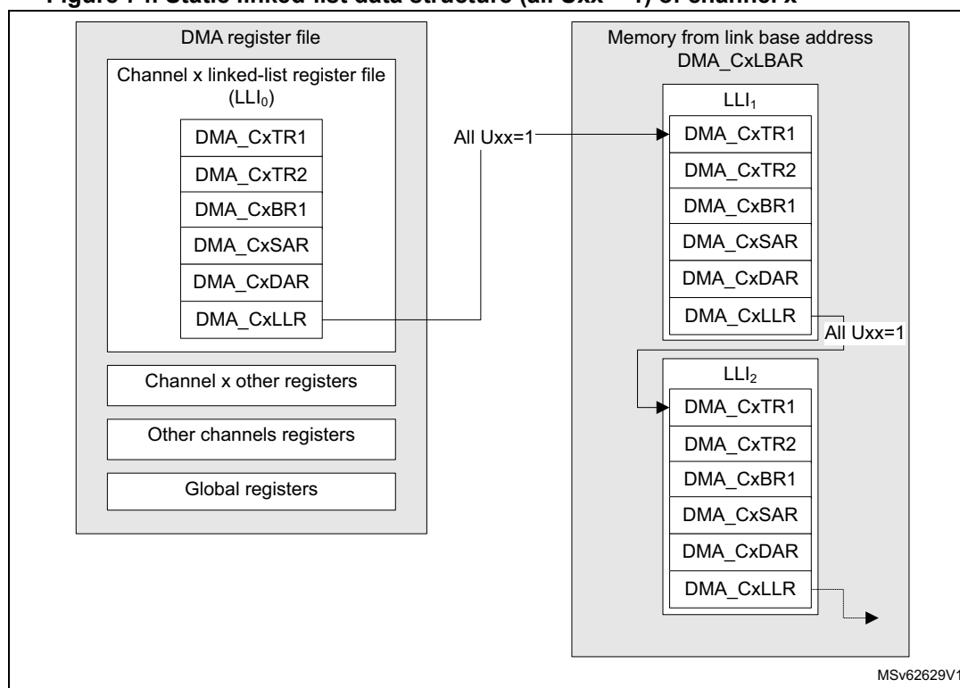
Figure 74. Static linked-list data structure (all U_{xx} = 1 ) of channel x
