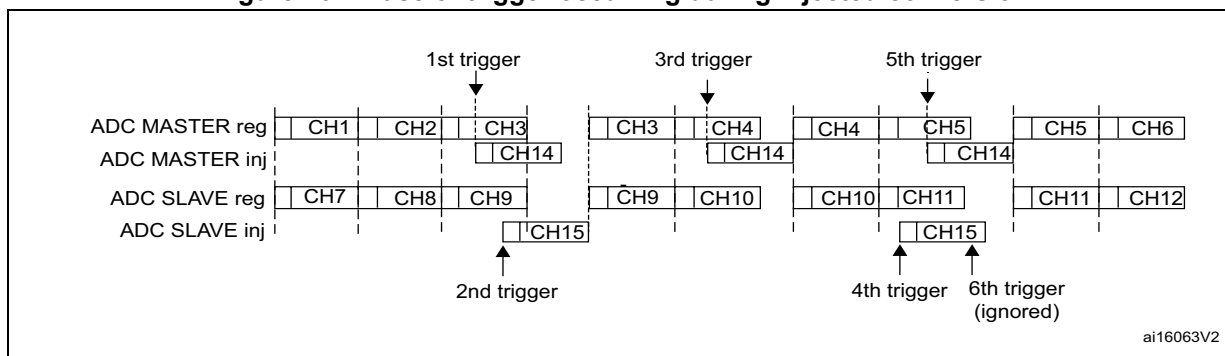
Figure 262. Case of trigger occurring during injected conversion
