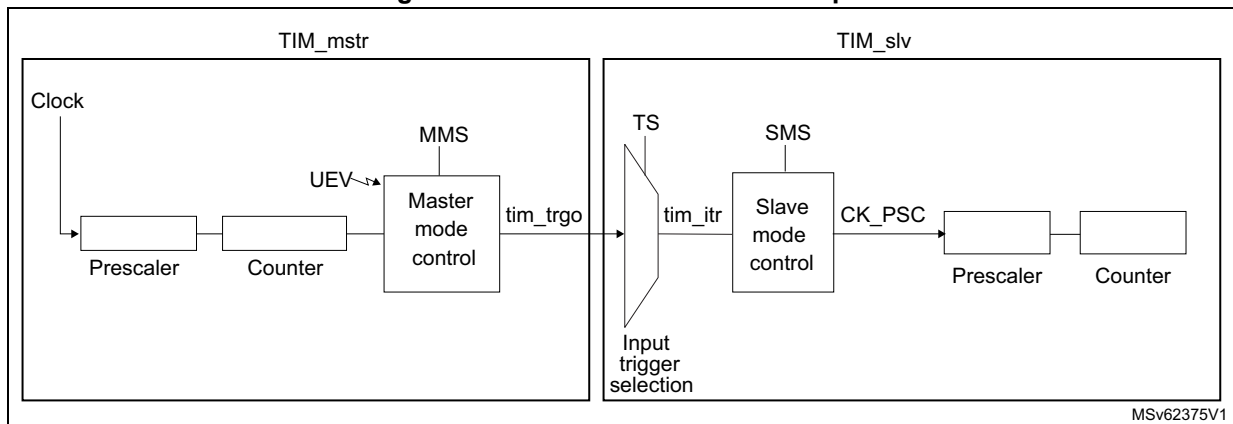
Figure 668. Master/Slave timer example
