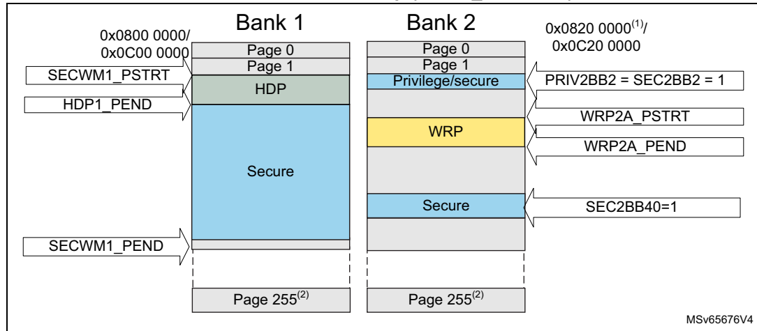
Figure 23. Flash memory security attributes and protections in case of no bank swap (SWAP_BANK = 0)
