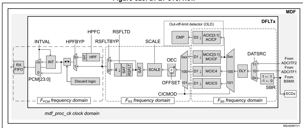
Figure 329. DFLT overview
