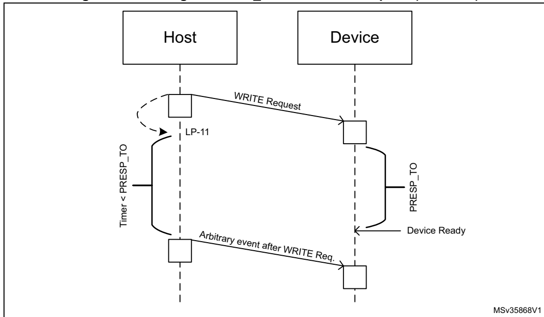
Figure 419. Timing of PRESP_TO after a write request (HS or LP)
