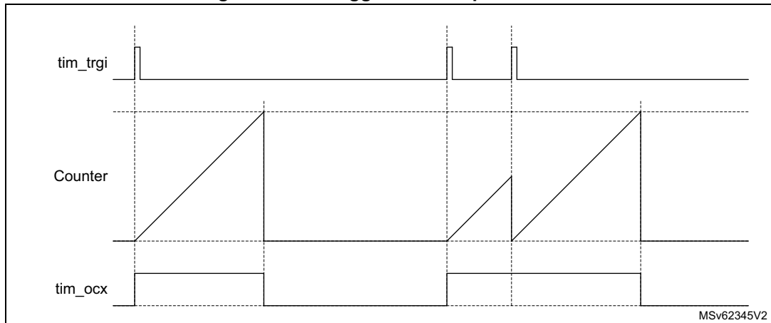
Figure 711. Retriggerable one pulse mode
