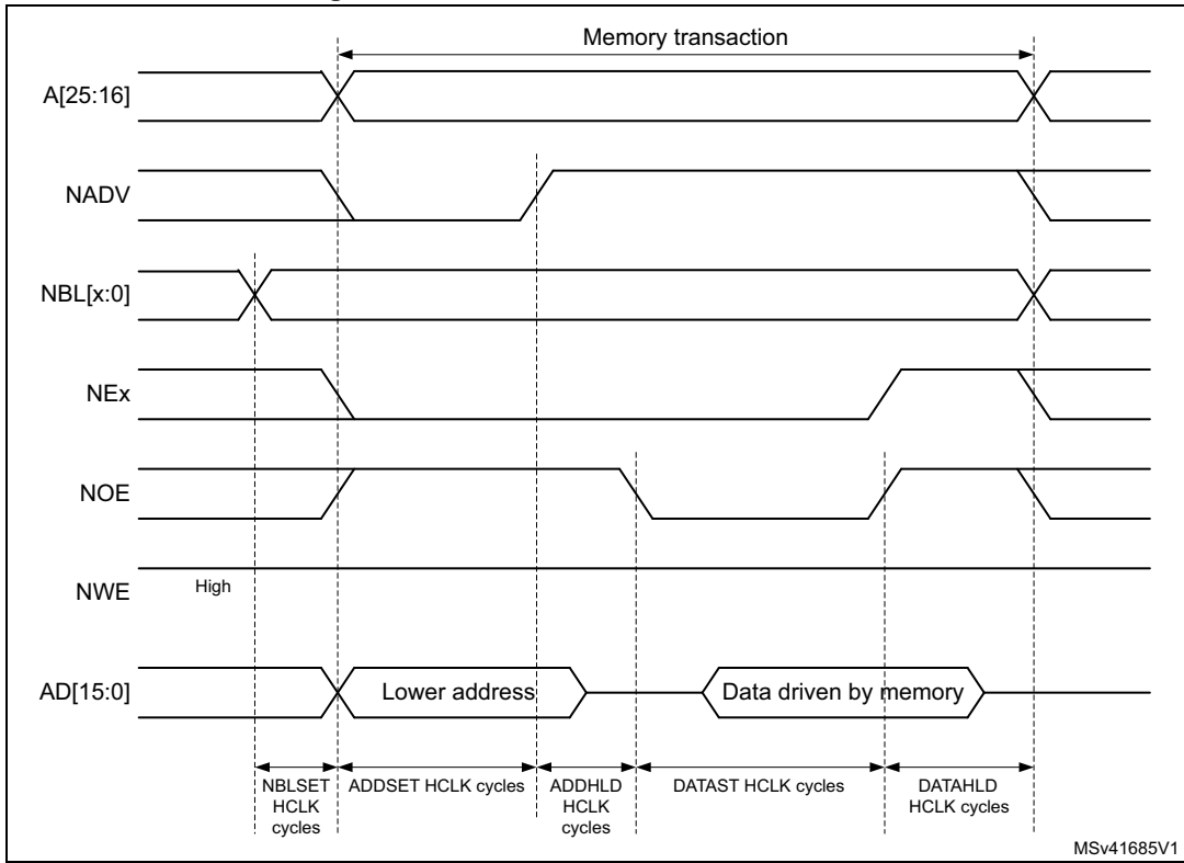
Figure 130. Muxed read access waveforms
