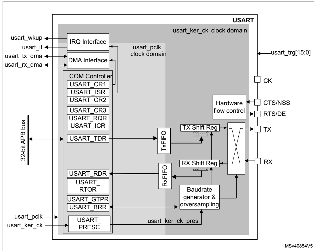
Figure 800. USART block diagram
