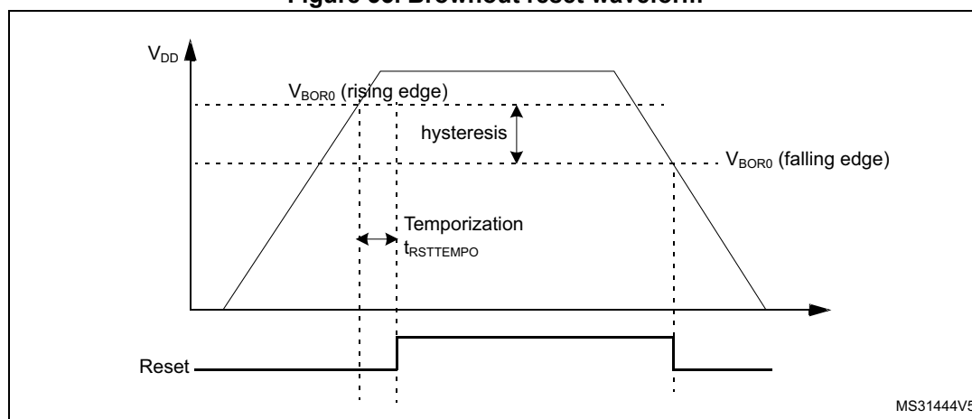
Figure 33. Brownout reset waveform
