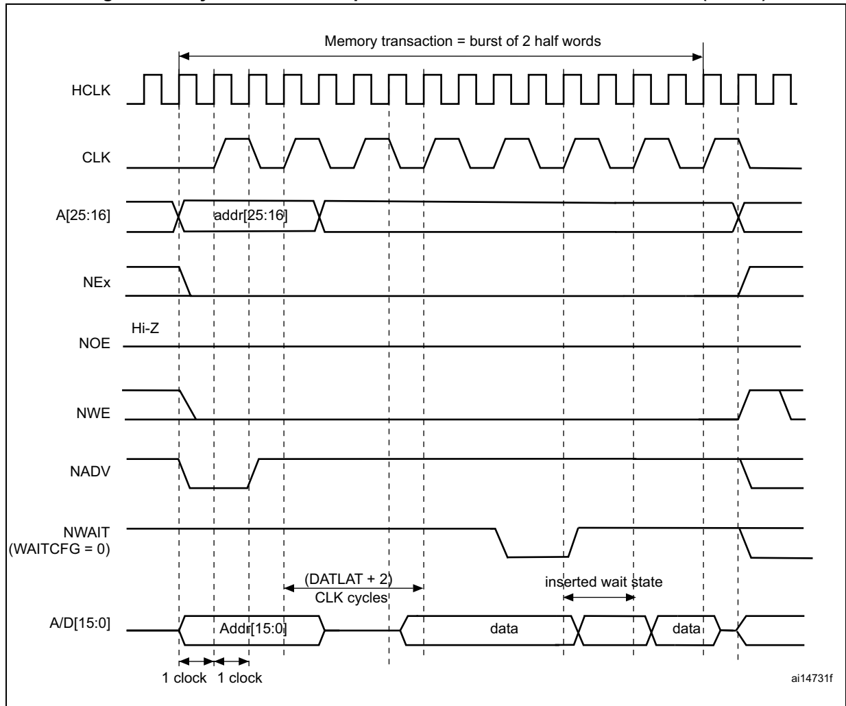
Figure 136. Synchronous multiplexed write mode waveforms - PSRAM (CRAM)
