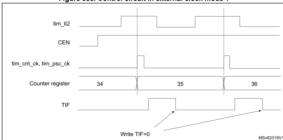
Figure 688. Control circuit in external clock mode 1
