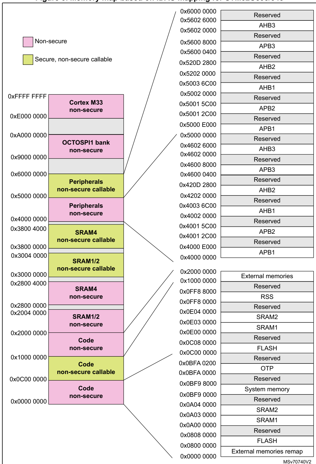
Figure 3. Memory map based on IDAU mapping for STM32U535/545
