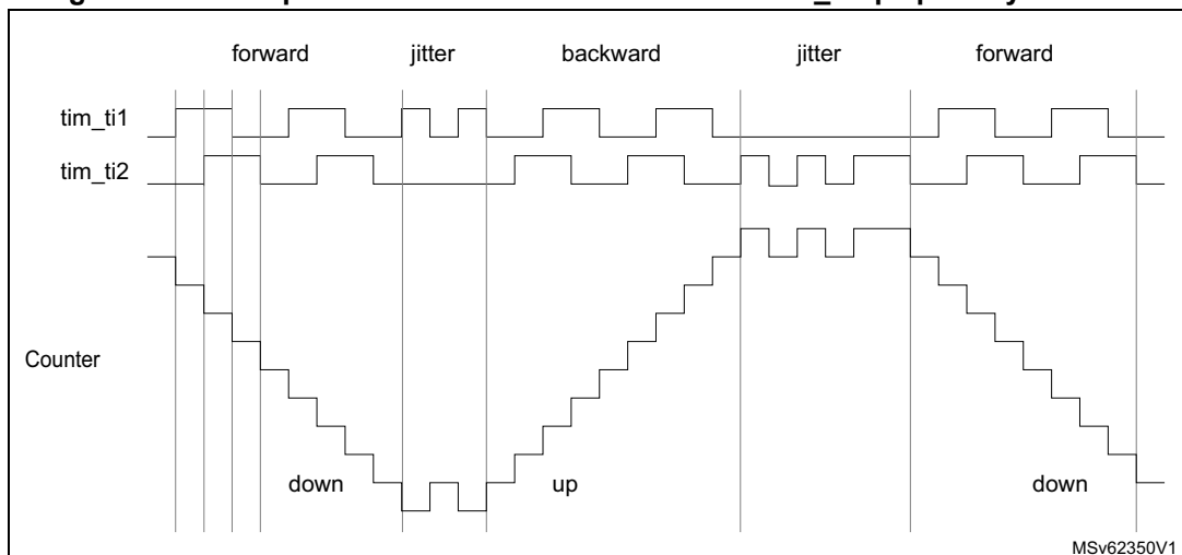
Figure 564. Example of encoder interface mode with tim_ti1fp1 polarity inverted.
