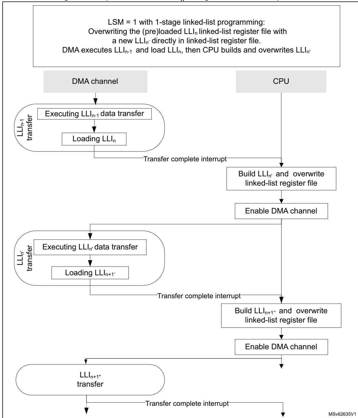
Figure 80. Replace with a new LLI n' in register file in link step mode
