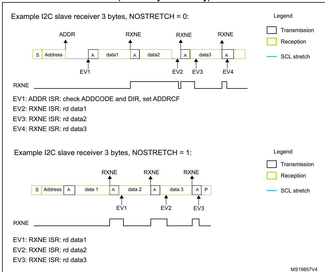
Figure 782. Transfer bus diagrams for I2C slave receiver (mandatory events only)
