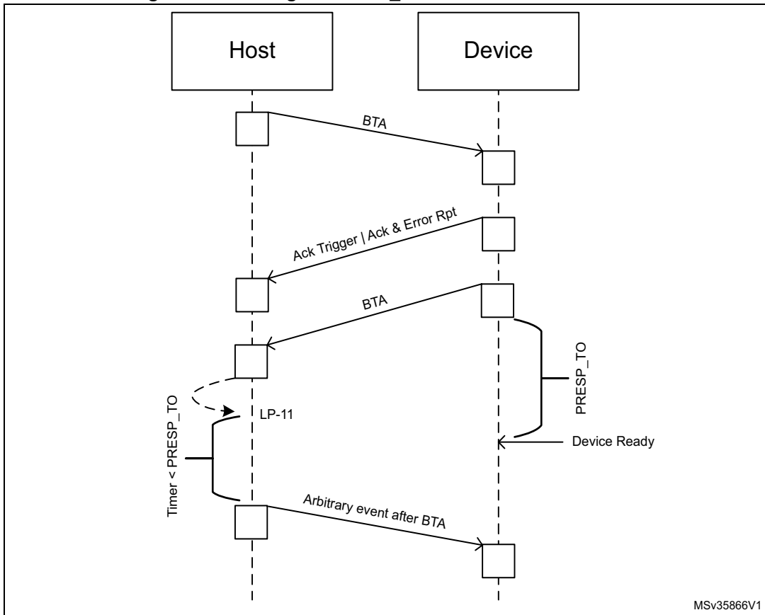
Figure 417. Timing of PRESP_TO after a bus-turn-around
