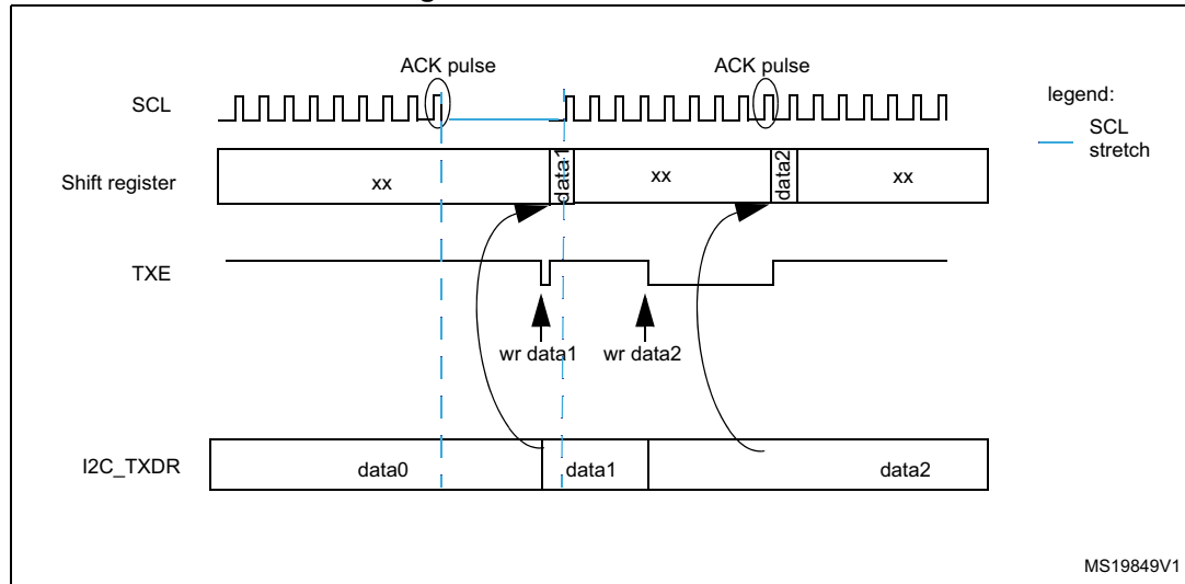
Figure 775. Data transmission
