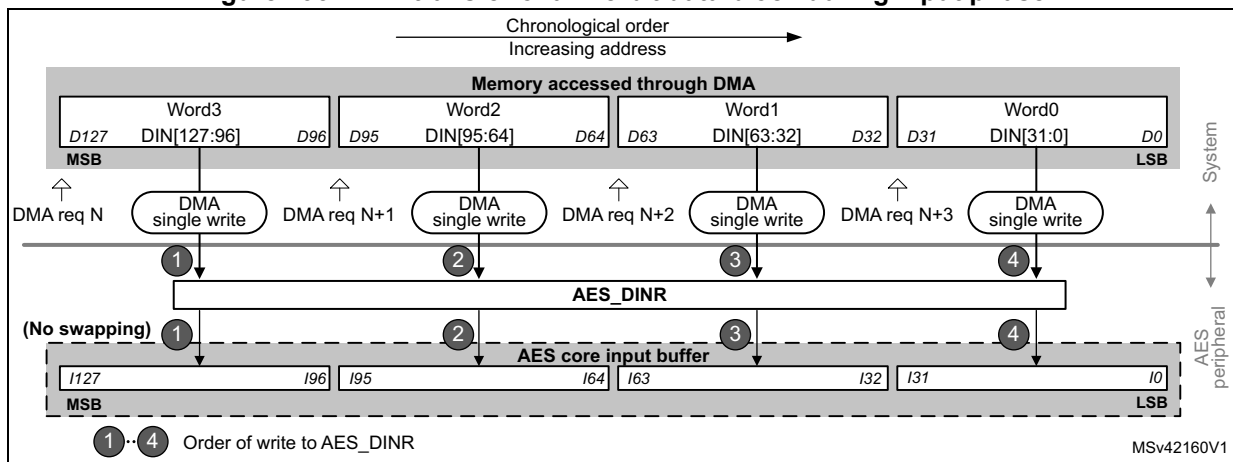
Figure 493. DMA transfer of a 128-bit data block during input phase
