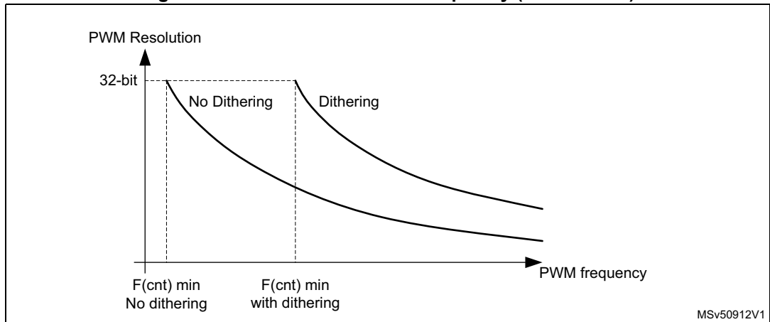
Figure 628. PWM resolution vs frequency (32-bit mode)
