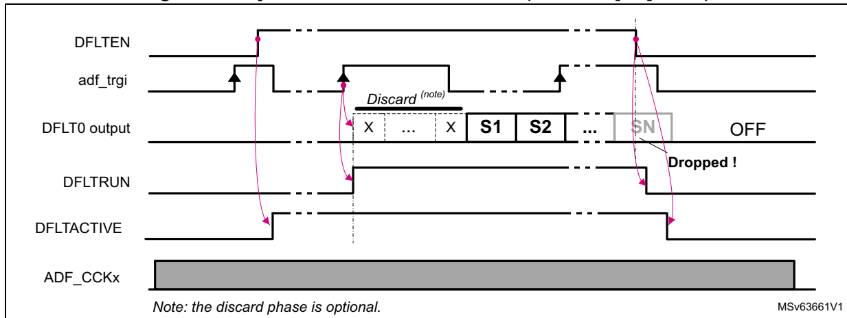
Figure 368. Synchronous continuous mode (ACQMOD[2:0] = 010)
