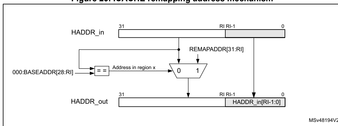
Figure 29. ICACHE remapping address mechanism
