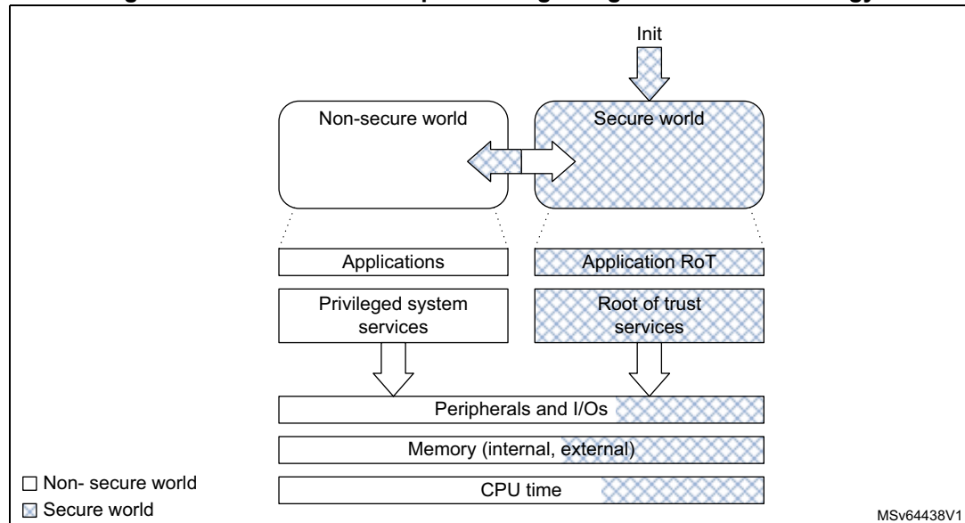
Figure 7. Secure/nonsecure partitioning using TrustZone technology
