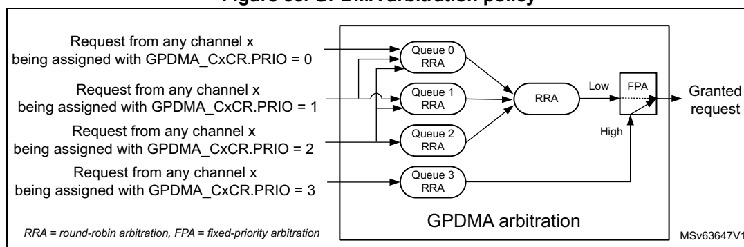
Figure 66. GPDMA arbitration policy
