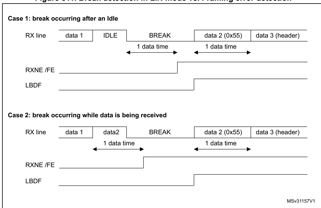
Figure 811. Break detection in LIN mode vs. Framing error detection
