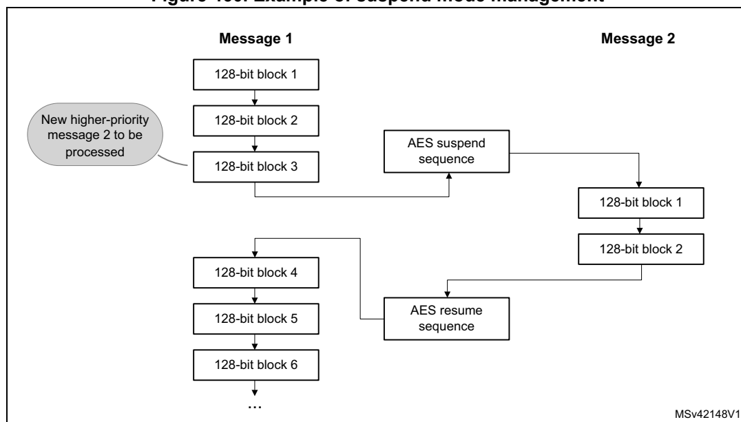
Figure 460. Example of suspend mode management
