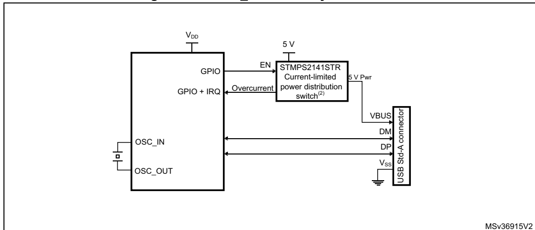
Figure 887. OTG_FS host-only connection
