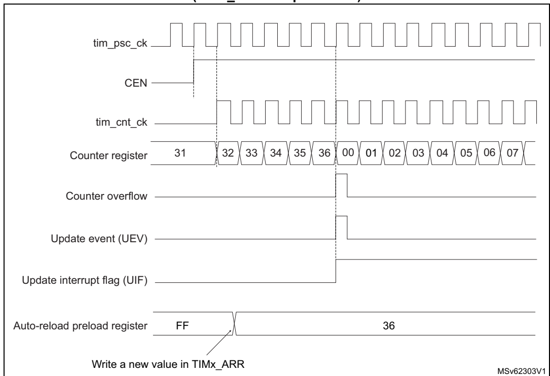
Figure 510. Counter timing diagram, update event when ARPE=0 (TIMx_ARR not preloaded)
