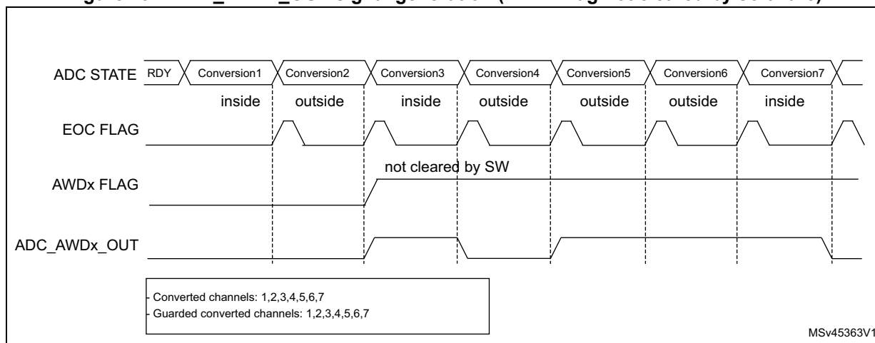
Figure 294. ADC_AWDx_OUT signal generation (AWDx flag not cleared by software)
