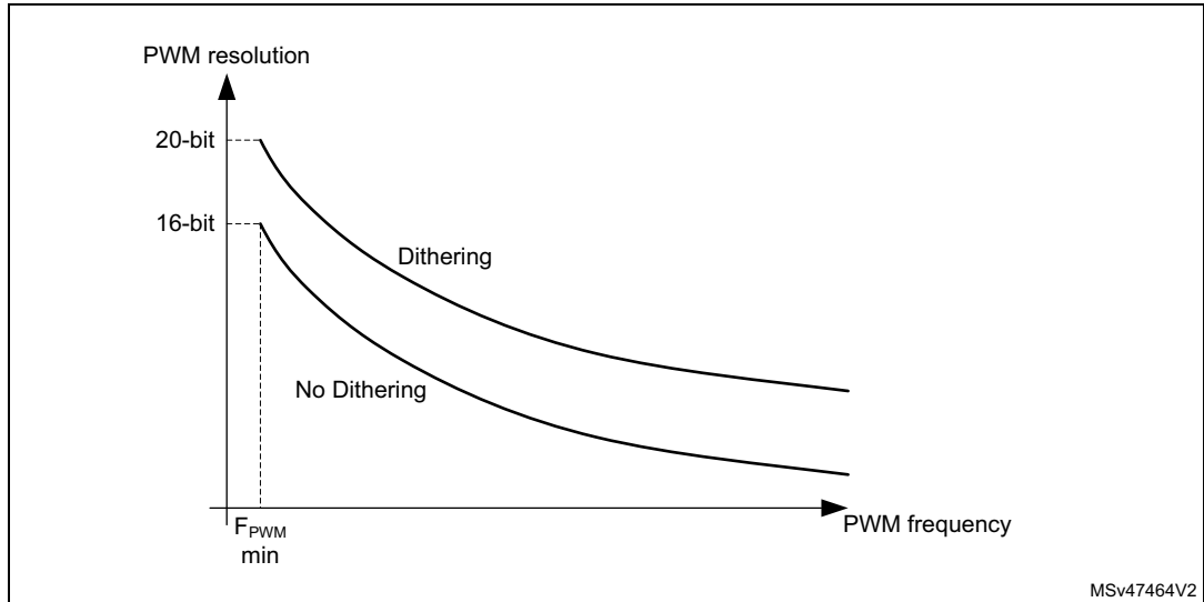
Figure 627. PWM resolution vs frequency (16-bit mode)
