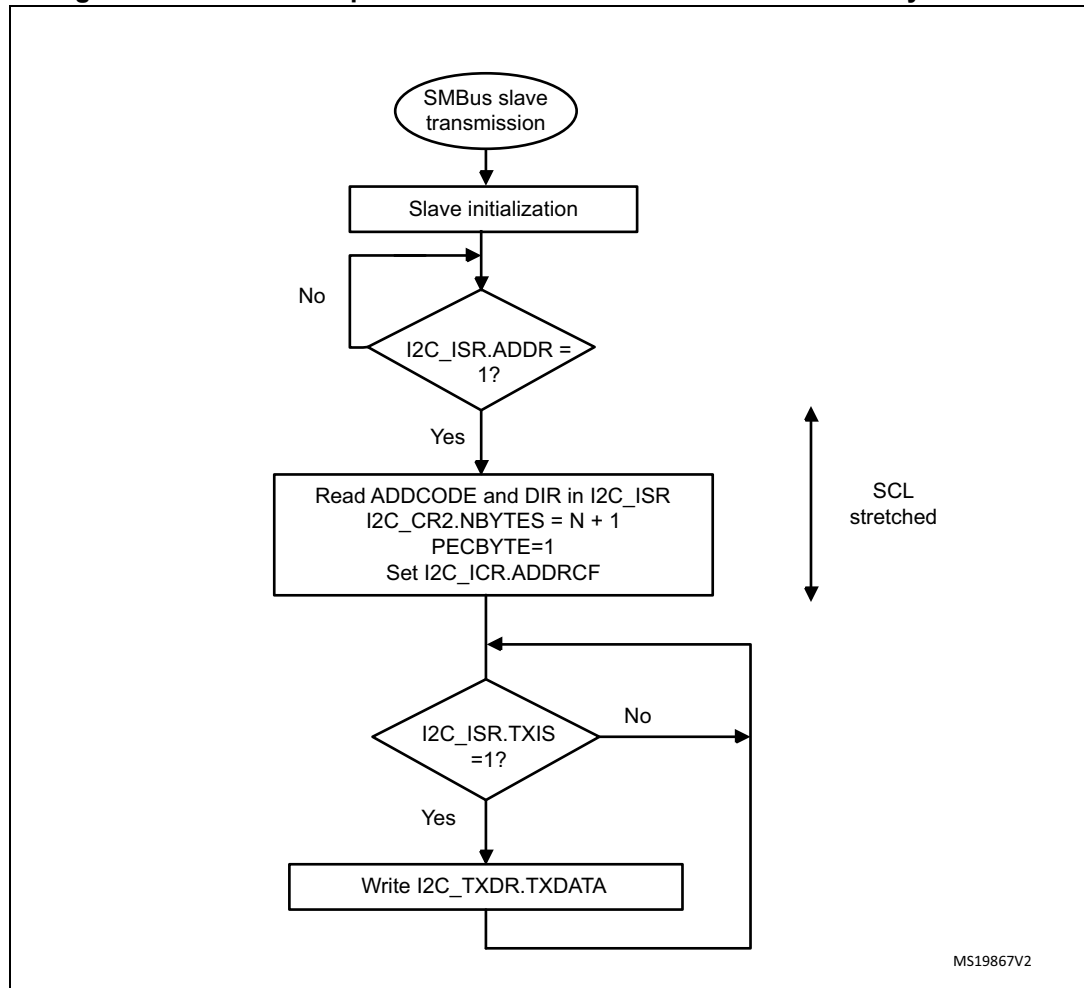
Figure 794. Transfer sequence flow for SMBus slave transmitter N bytes + PEC
