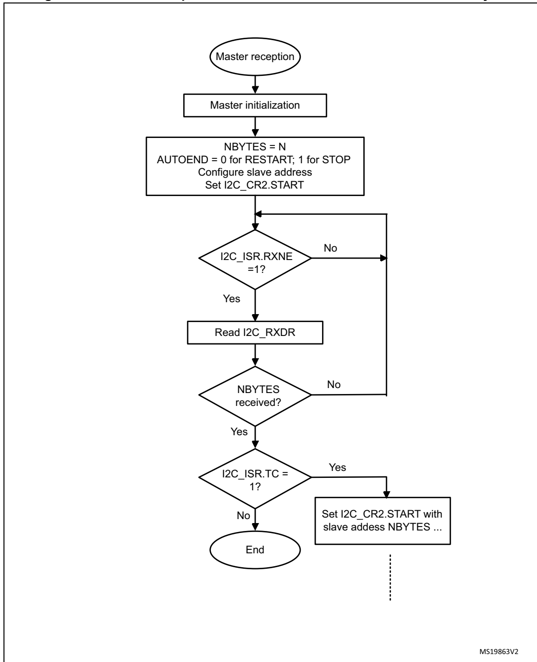
Figure 790. Transfer sequence flow for I2C master receiver for N \leq 255 bytes
