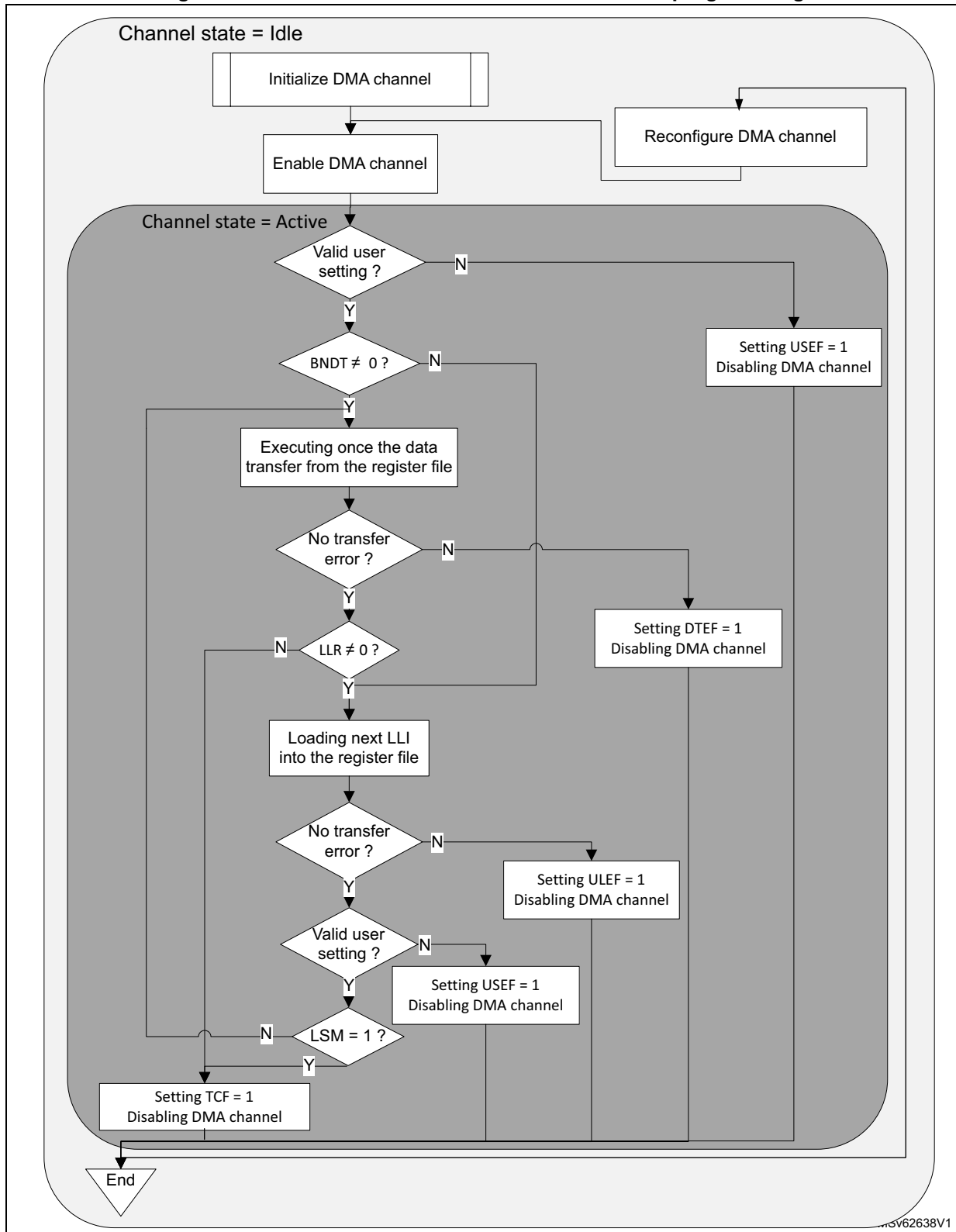
Figure 83. LPDMA channel execution and linked-list programming
