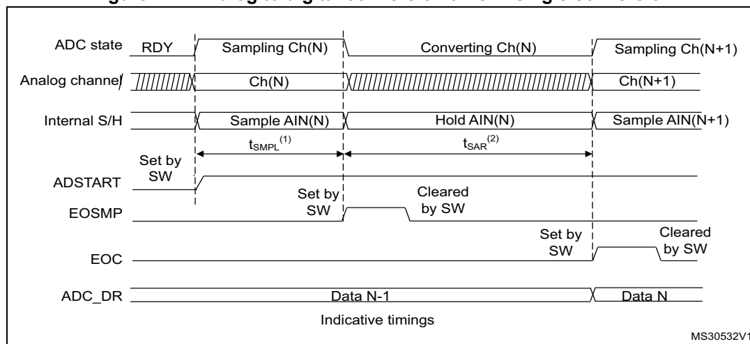
Figure 222. Analog to digital conversion time in single conversion
