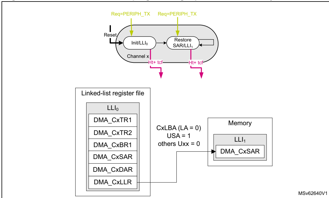
Figure 86. LPDMA circular buffer programming: update of the memory start address
