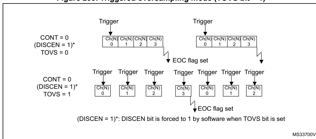
Figure 299. Triggered oversampling mode (TOVS bit = 1)
