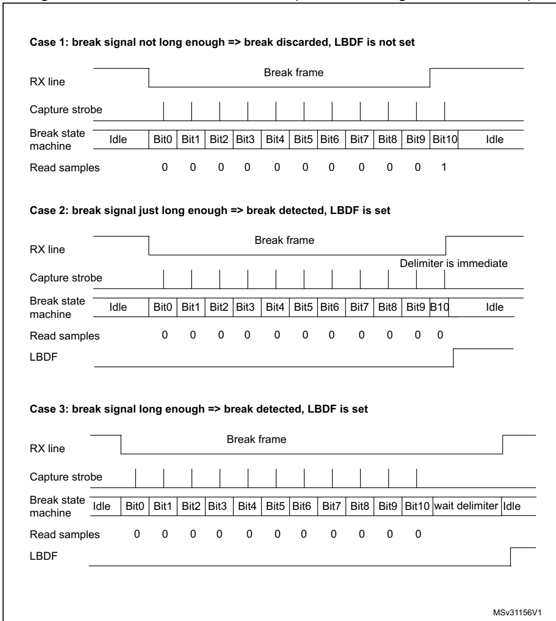
Figure 810. Break detection in LIN mode (11-bit break length - LBDL bit is set)
