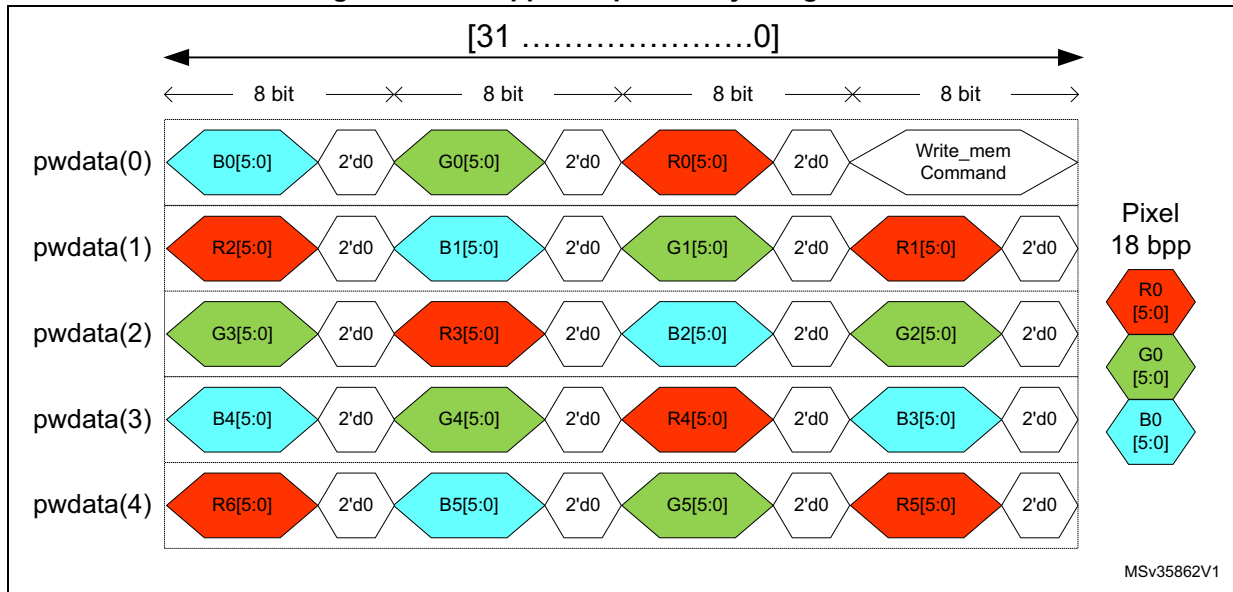
Figure 413. 18 bpp APB pixel to byte organization
