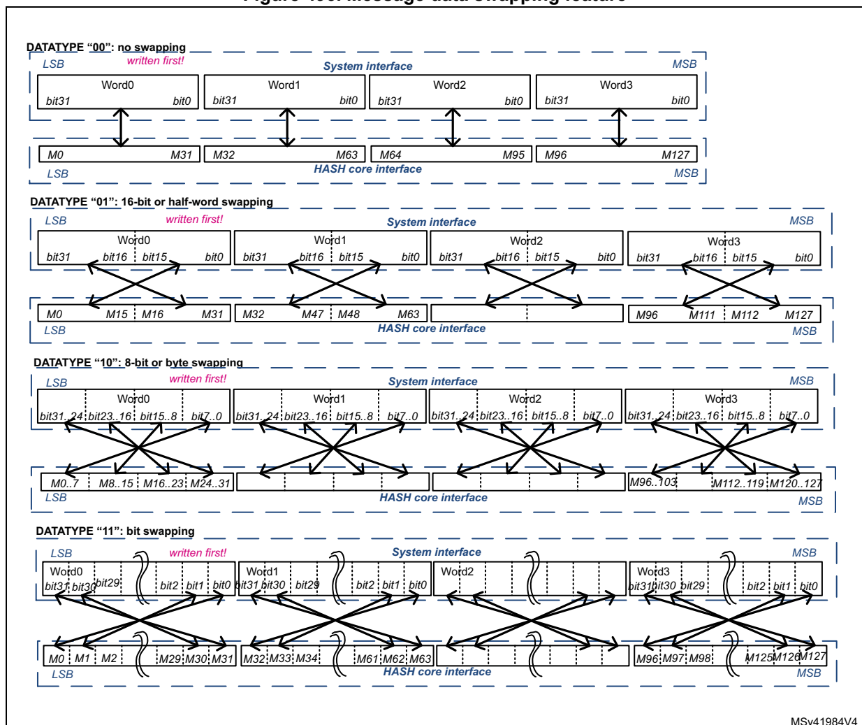
Figure 496. Message data swapping feature
