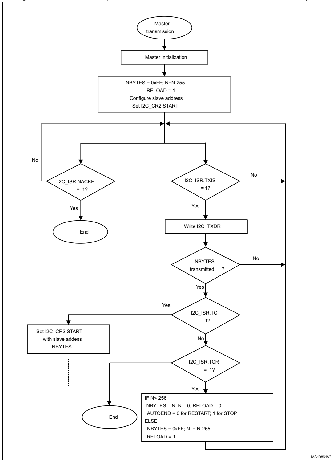
Figure 788. Transfer sequence flow for I2C master transmitter for N > 255 bytes
