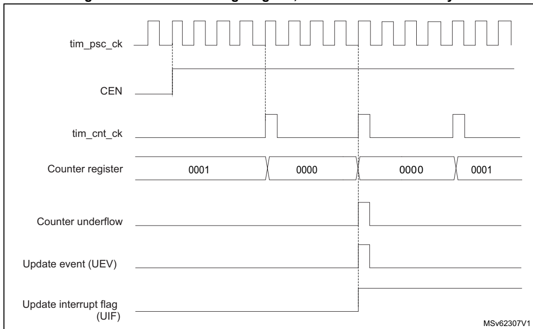
Figure 514. Counter timing diagram, internal clock divided by 4
