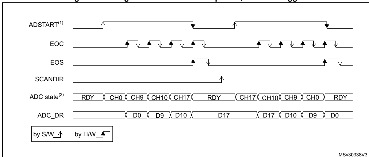
Figure 281. Single conversions of a sequence, software trigger
