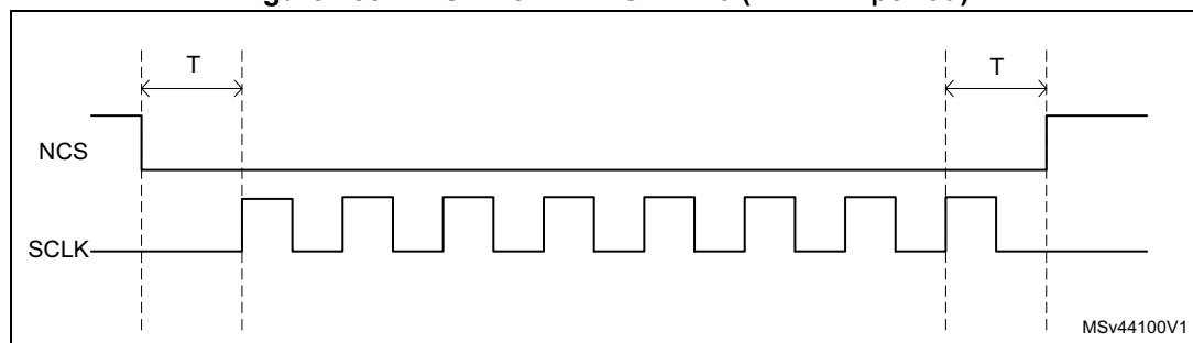
Figure 155. NCS when CKMODE = 0 (T = CLK period)
