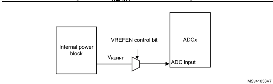
Figure 271. V_{REFINT} channel block diagram
