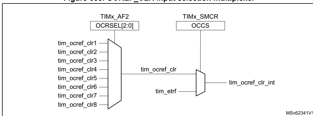
Figure 633. OCREF_CLR input selection multiplexer
