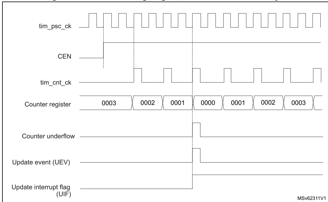
Figure 518. Counter timing diagram, internal clock divided by 2
