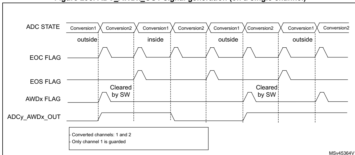
Figure 295. ADC_AWDx_OUT signal generation (on a single channel)
