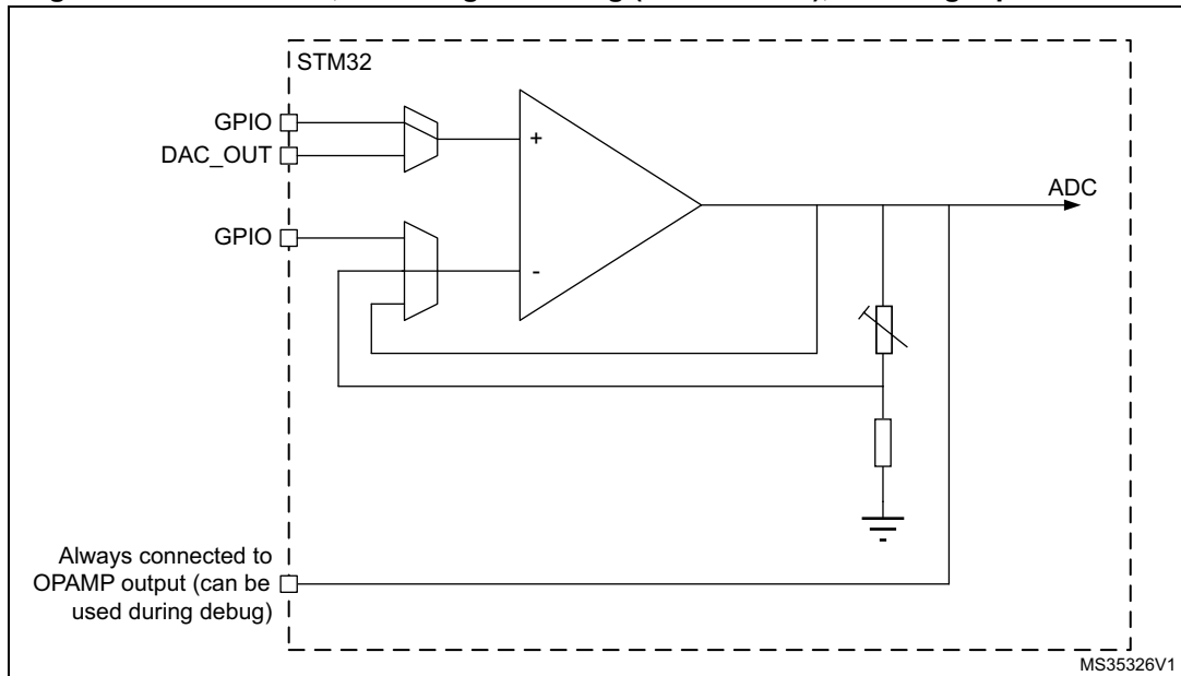
Figure 319. PGA mode, internal gain setting (x2/x4/x8/x16), inverting input not used
