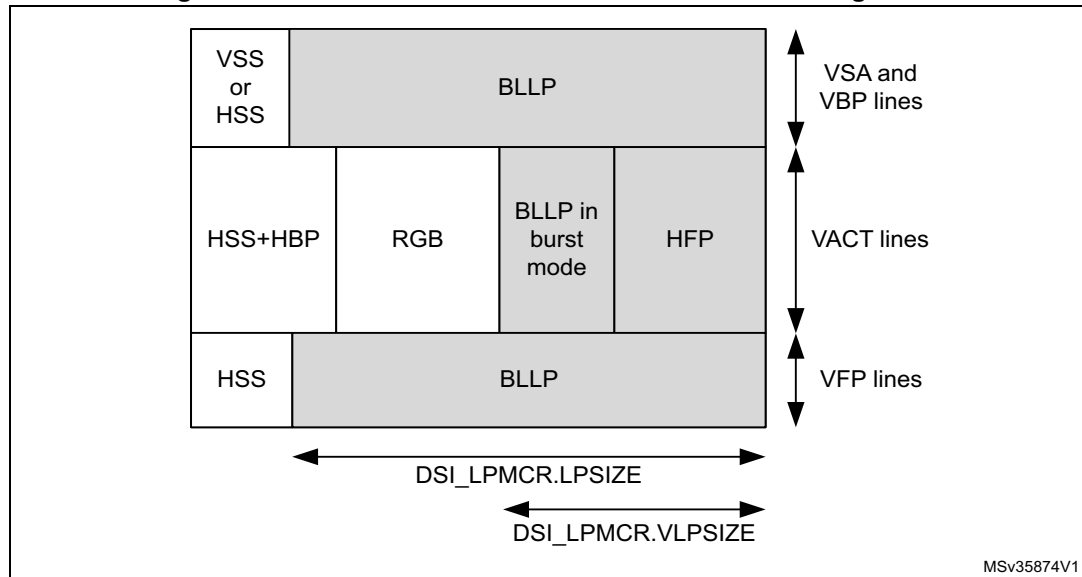
Figure 428. Location of LPSIZE and VLPSIZE in the image area
