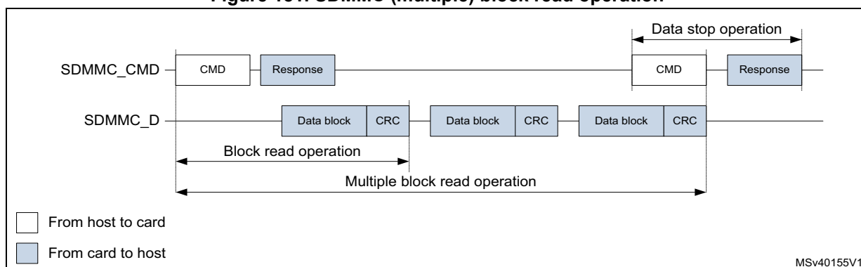
Figure 181. SDMMC (multiple) block read operation
