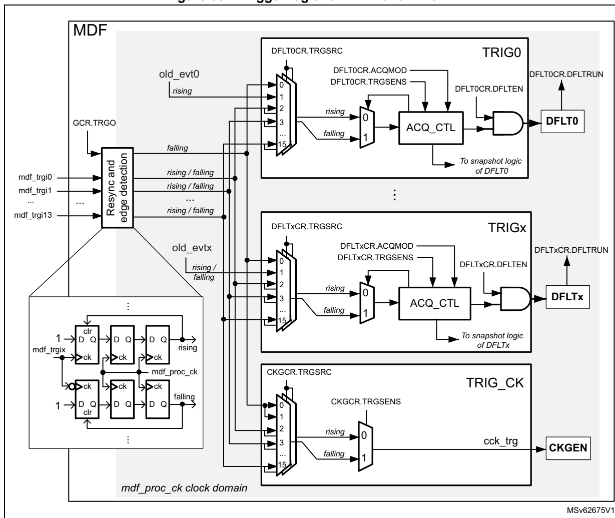
Figure 334. Trigger logic for DFLT and CKGEN
