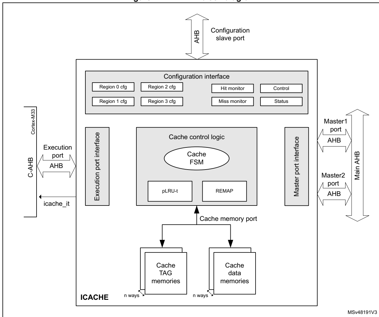
Figure 27. ICACHE block diagram
