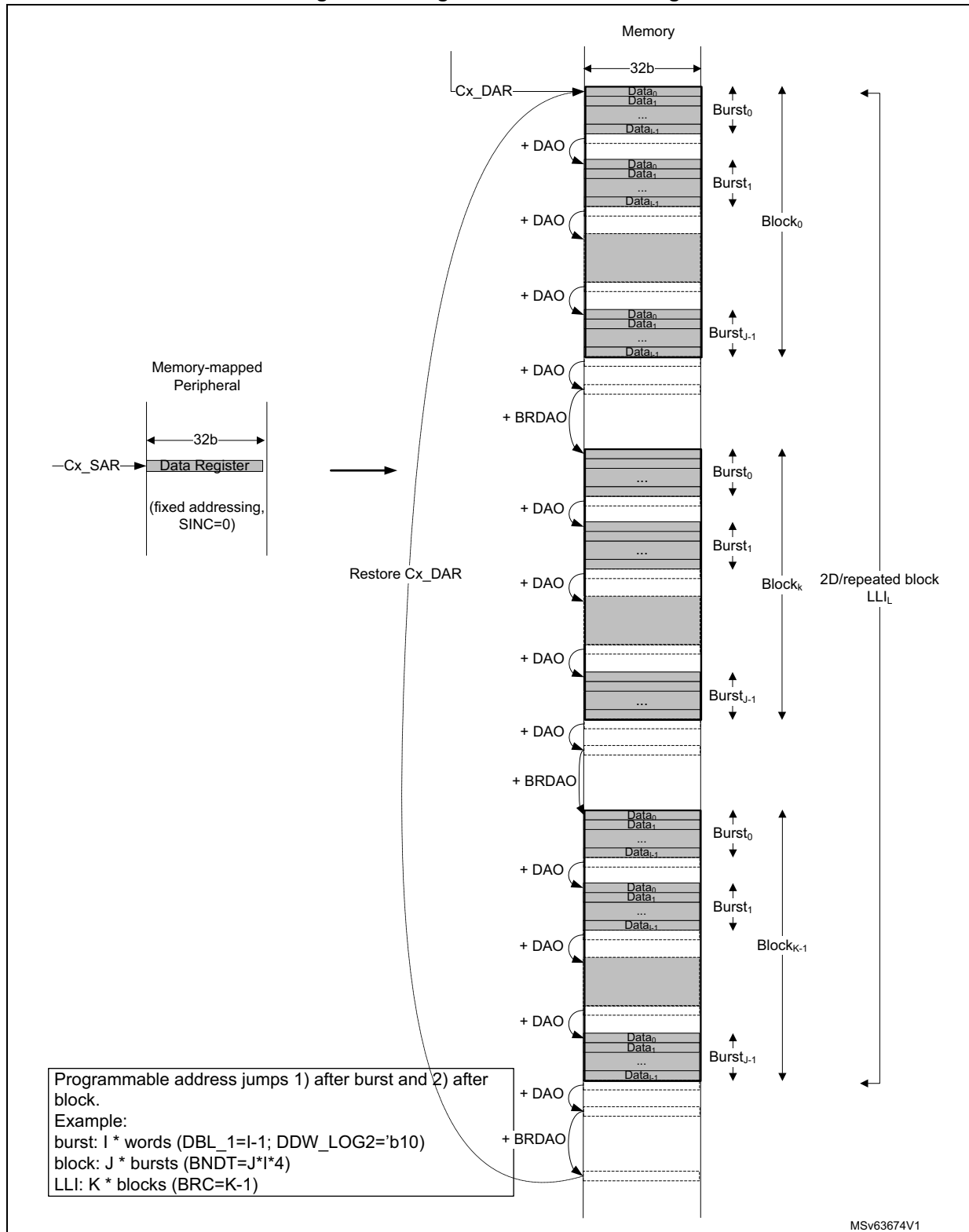
Figure 65. Programmed 2D addressing
