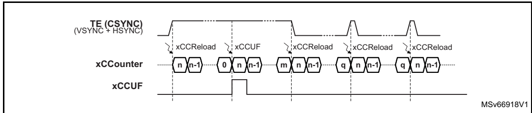
Figure 754. Waveforms with external CSYNC only
