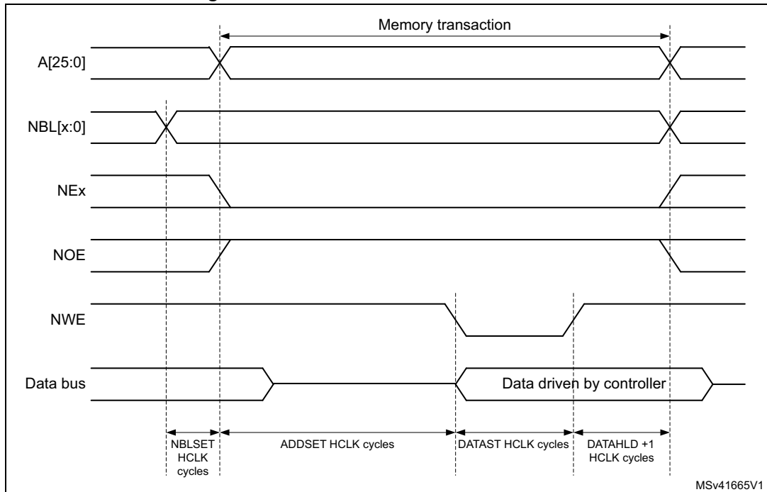
Figure 122. Mode A write access waveforms
