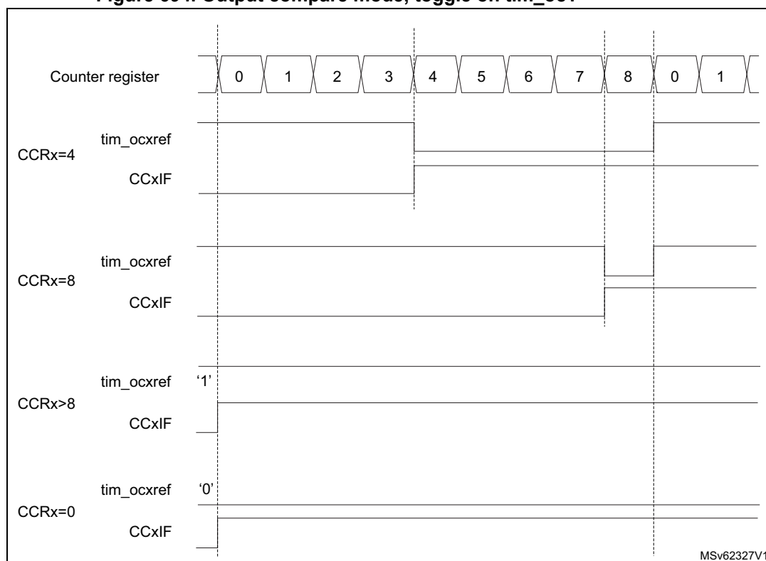
Figure 694. Output compare mode, toggle on tim_oc1
