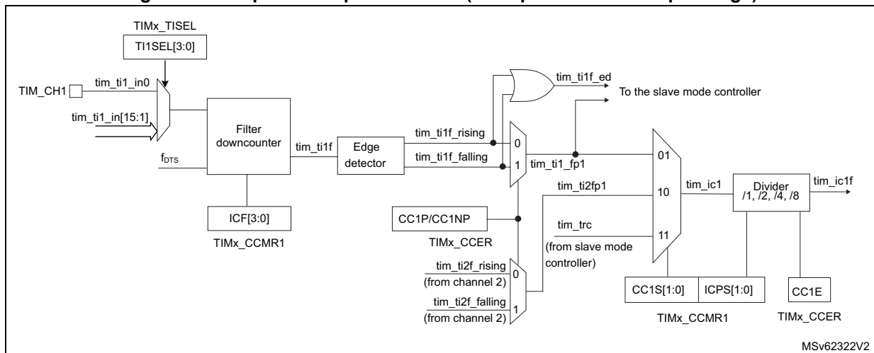
Figure 530. Capture/compare channel (example: channel 1 input stage)
