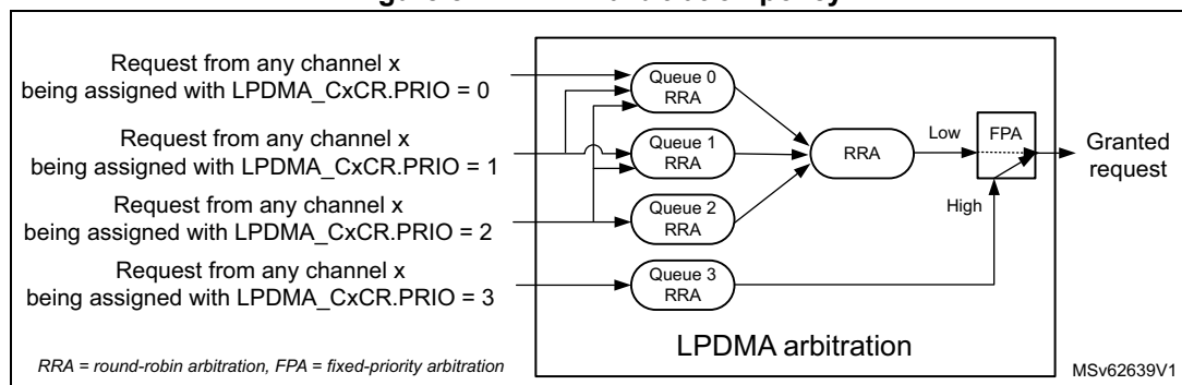
Figure 84. LPDMA arbitration policy
