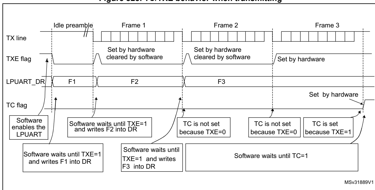
Figure 828. TC/TXE behavior when transmitting
