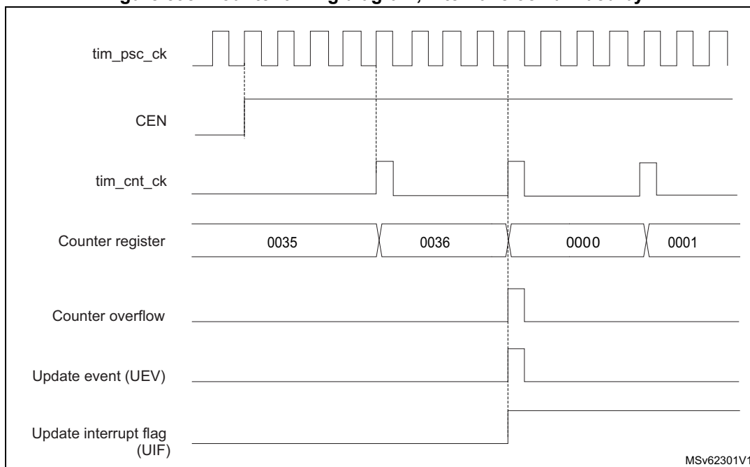
Figure 598. Counter timing diagram, internal clock divided by 4
