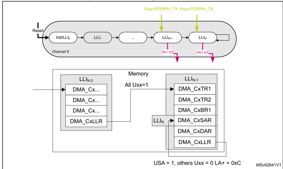
Figure 87. Shared LPDMA channel with circular buffering: update of the memory start address
