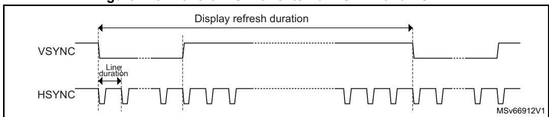
Figure 748. Waveforms with external HSYNC and VSYNC
