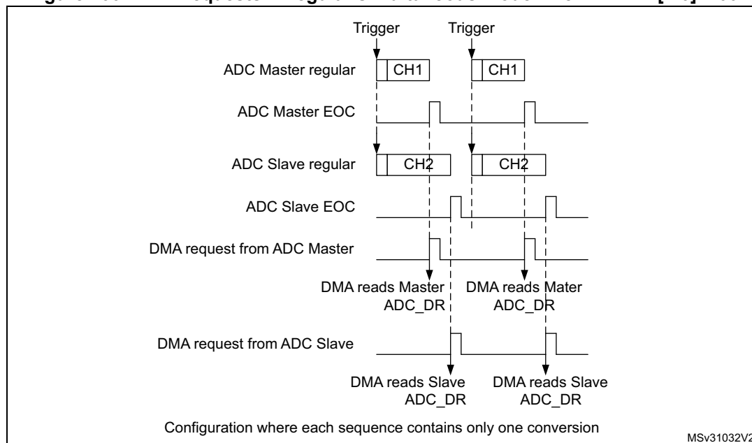
Figure 266. DMA Requests in regular simultaneous mode when DAMDF[1:0] = 00
