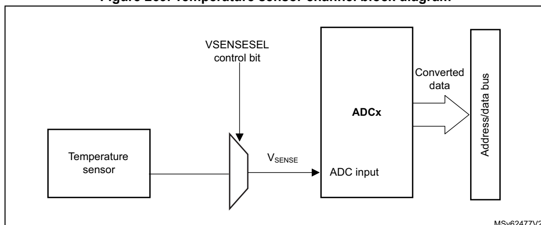
Figure 269. Temperature sensor channel block diagram
