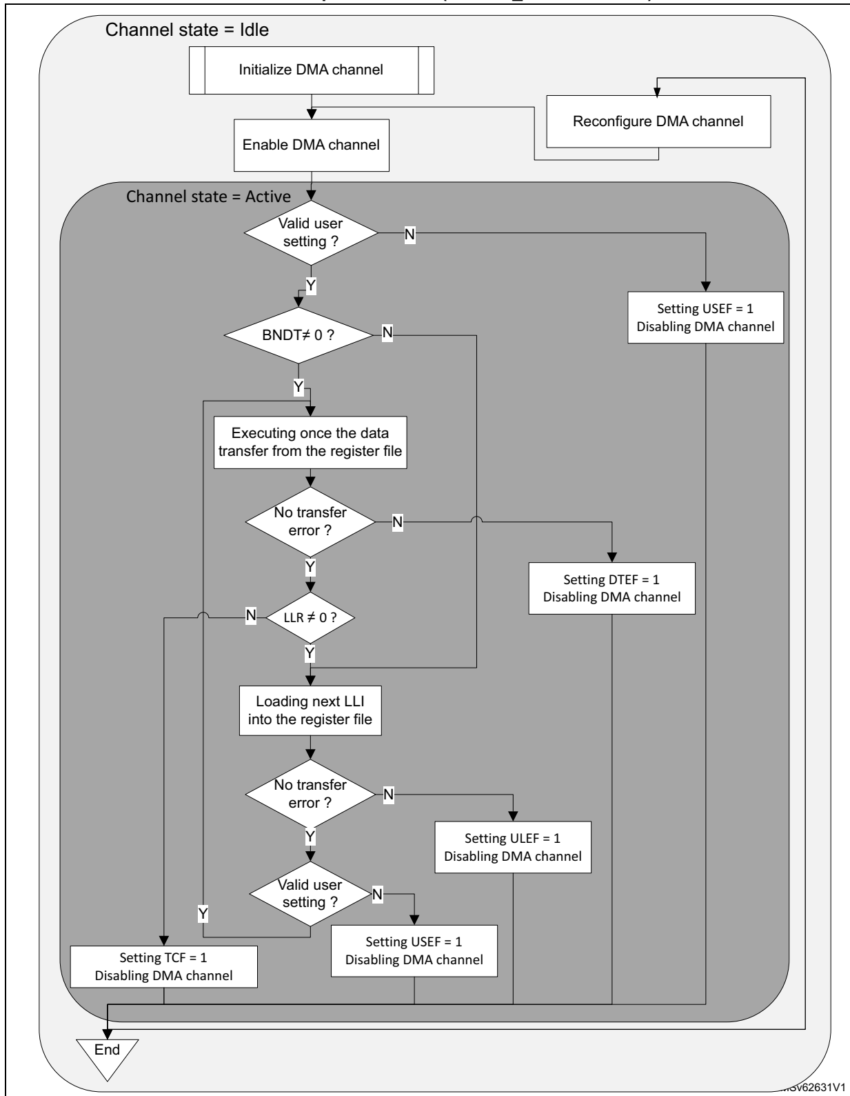
Figure 76. LPDMA channel execution and linked-list programming in run-to-completion mode (LPDMA_CxCR.LSM = 0)
