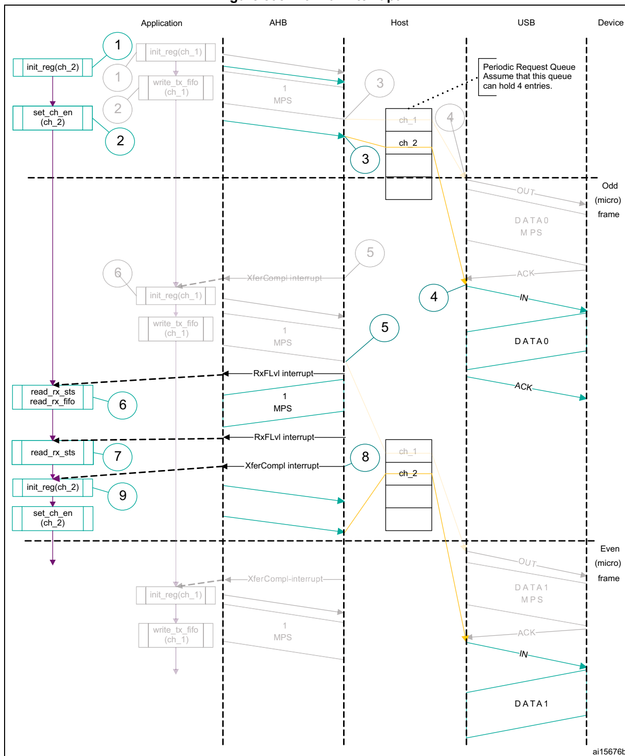
Figure 898. Normal interrupt IN
