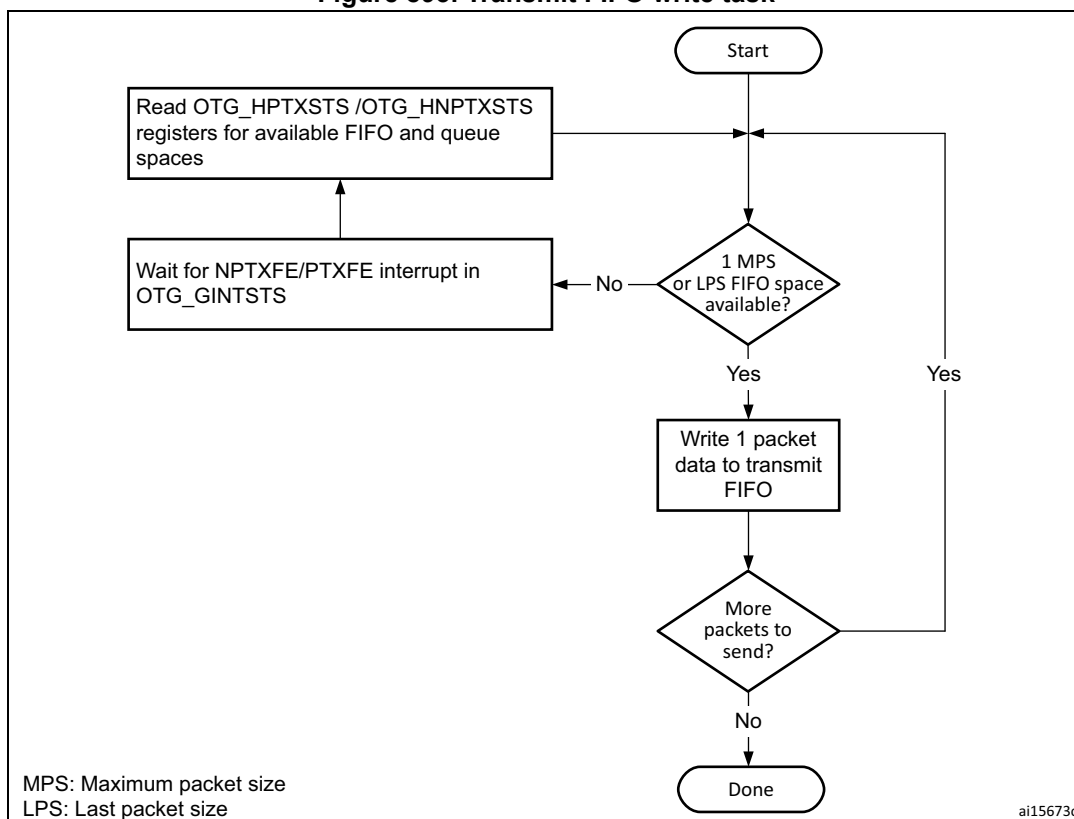
Figure 893. Transmit FIFO write task
