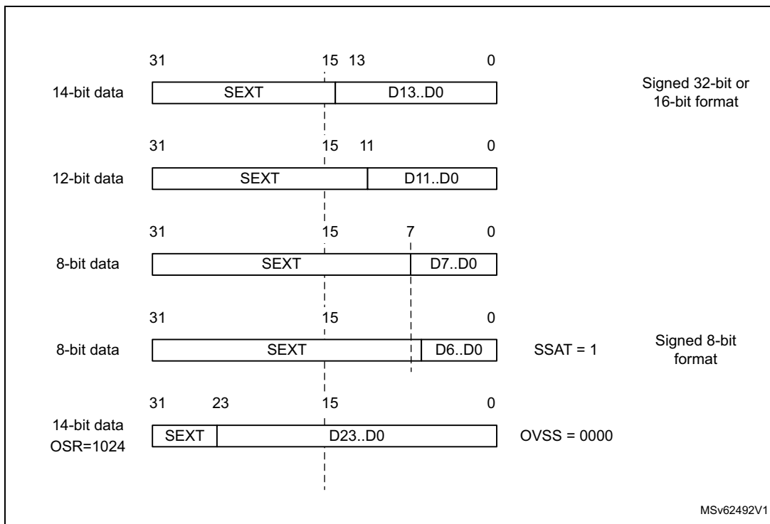
Figure 232. Right alignment (offset enabled, signed value)
