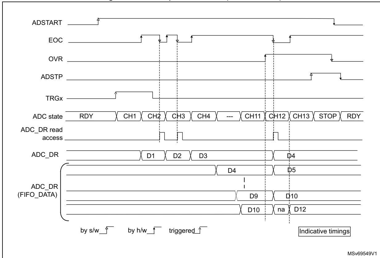
Figure 236. Example of overrun (OVRMOD = 1)
