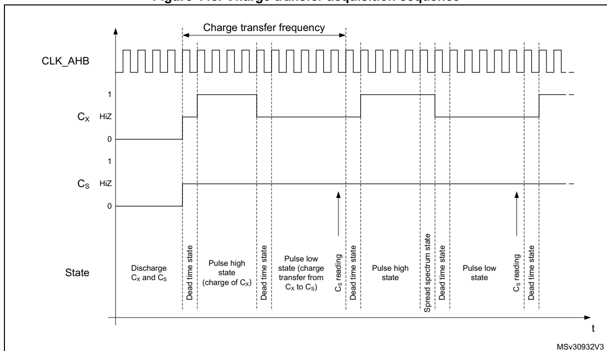
Figure 448. Charge transfer acquisition sequence
