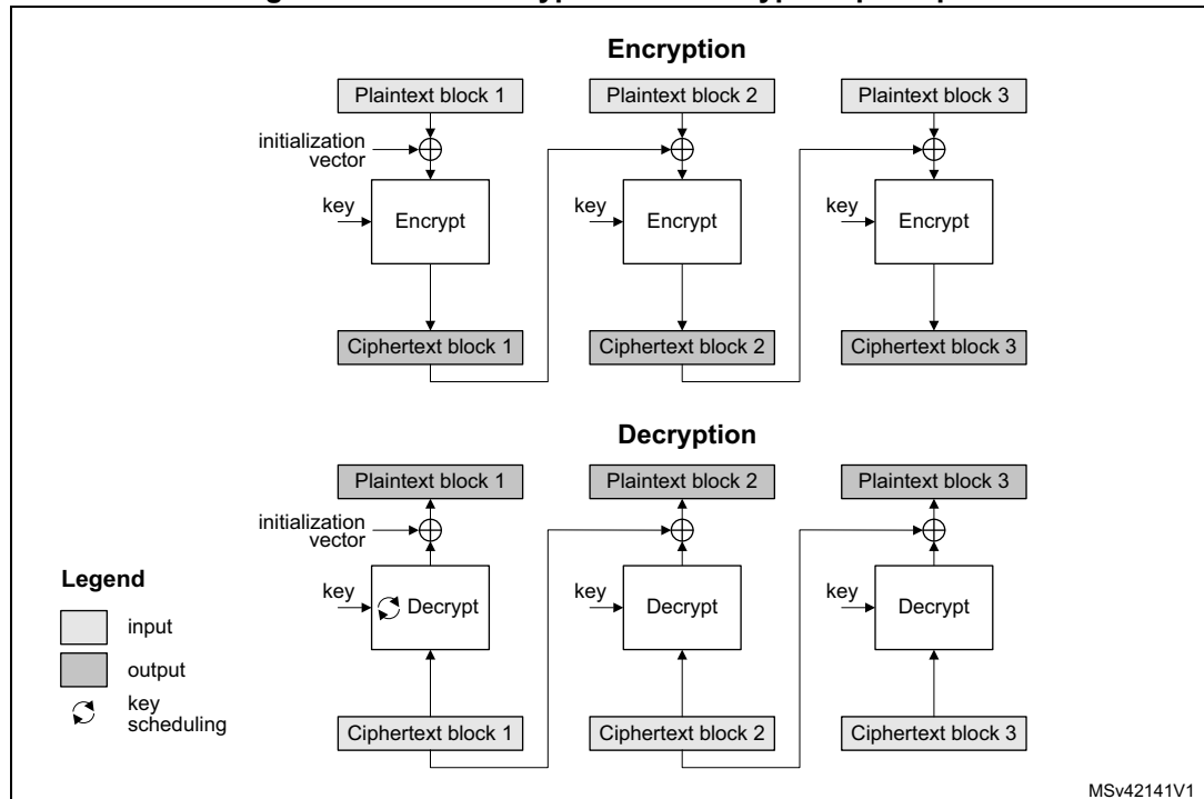
Figure 455. CBC encryption and decryption principle
