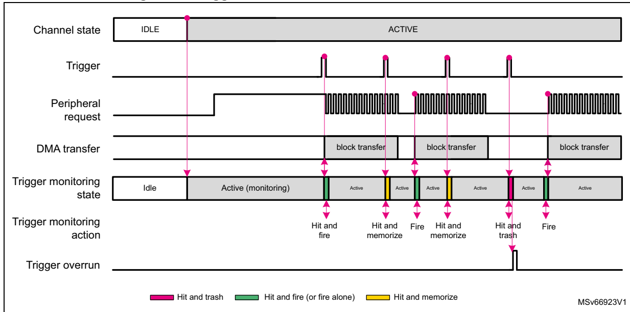
Figure 85. Trigger hit, memorization and overrun waveform
