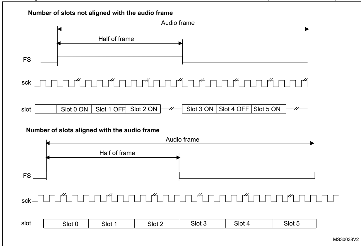
Figure 853. FS role is start of frame + channel side identification (FSDEF = TRIS = 1)
