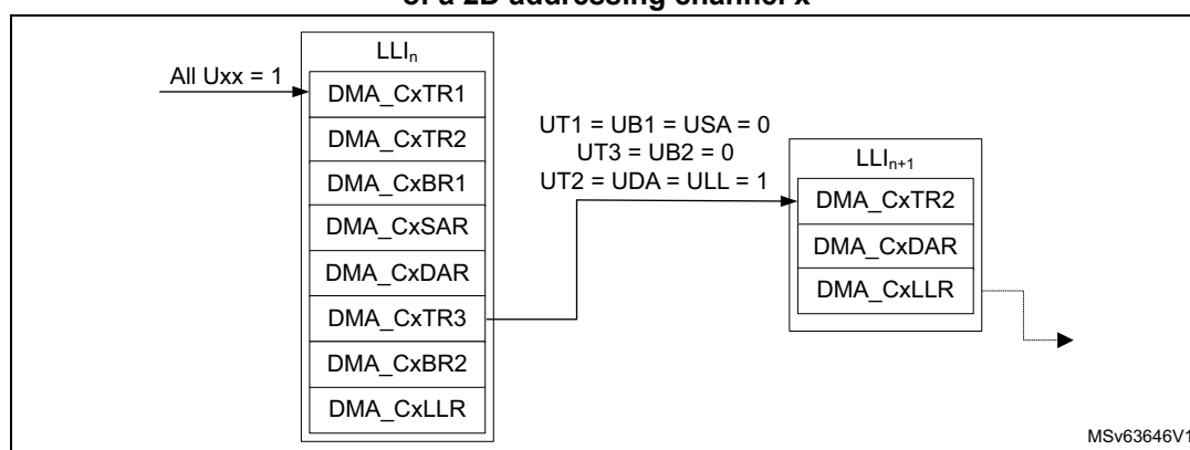
Figure 56. GPDMA dynamic linked-list data structure of a 2D addressing channel x
