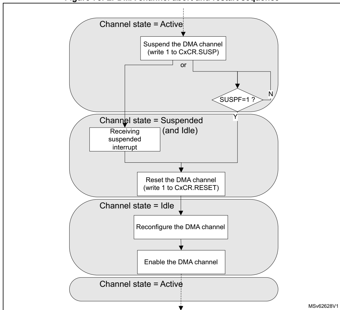
Figure 73. LPDMA channel abort and restart sequence
