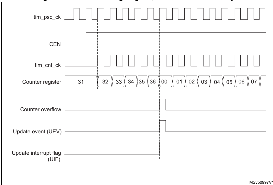
Figure 596. Counter timing diagram, internal clock divided by 1
