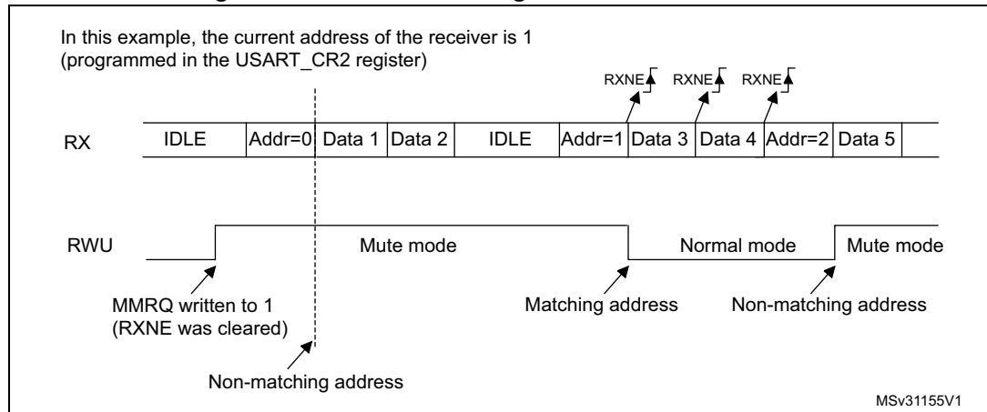
Figure 809. Mute mode using address mark detection
