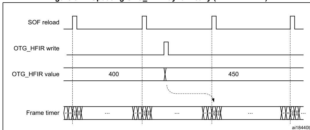
Figure 914. Updating OTG_HFIR dynamically (RLDCTRL = 1)
