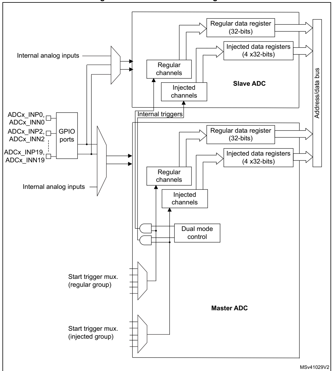
Figure 253. Dual ADC block diagram (1)
