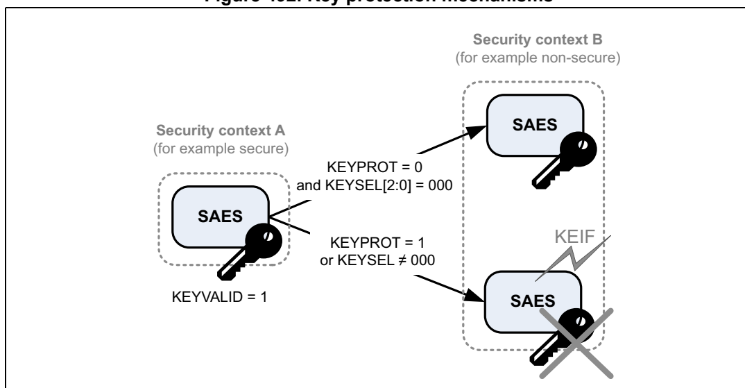
Figure 492. Key protection mechanisms
