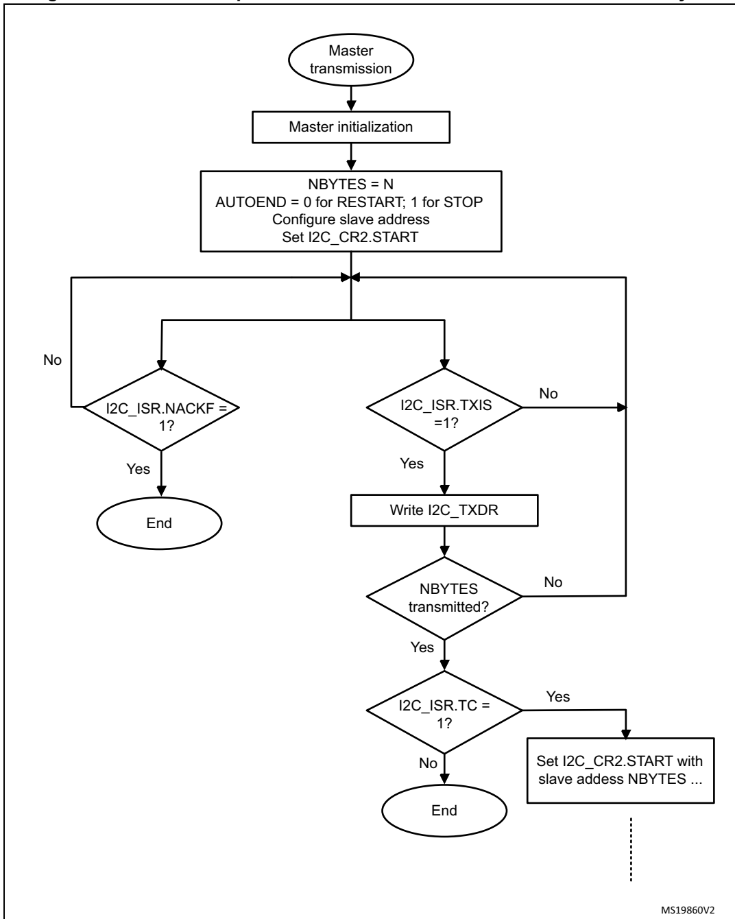
Figure 787. Transfer sequence flow for I2C master transmitter for N \leq 255 bytes
