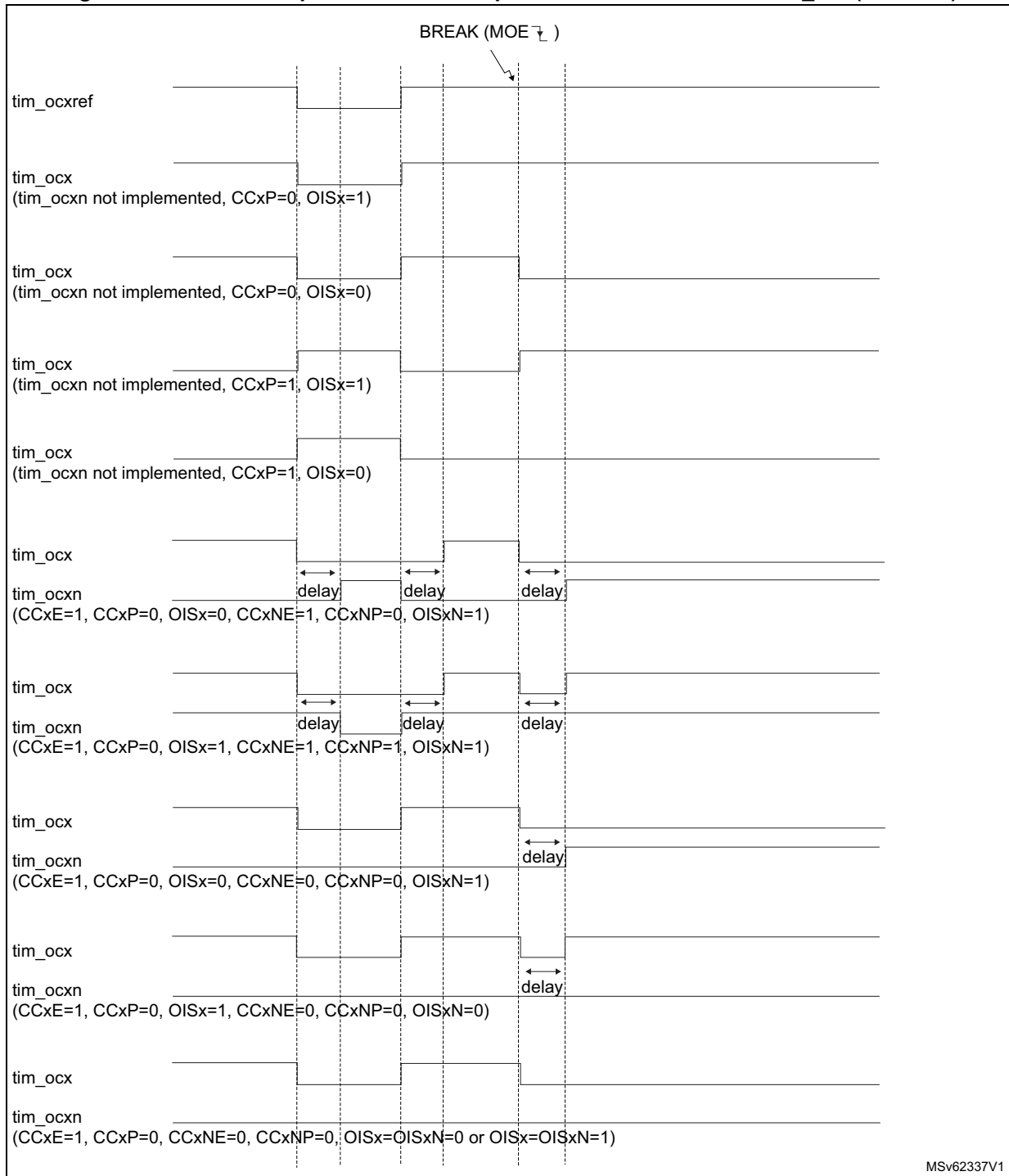
Figure 551. Various output behavior in response to a break event on tim_brk (OSSI = 1)
