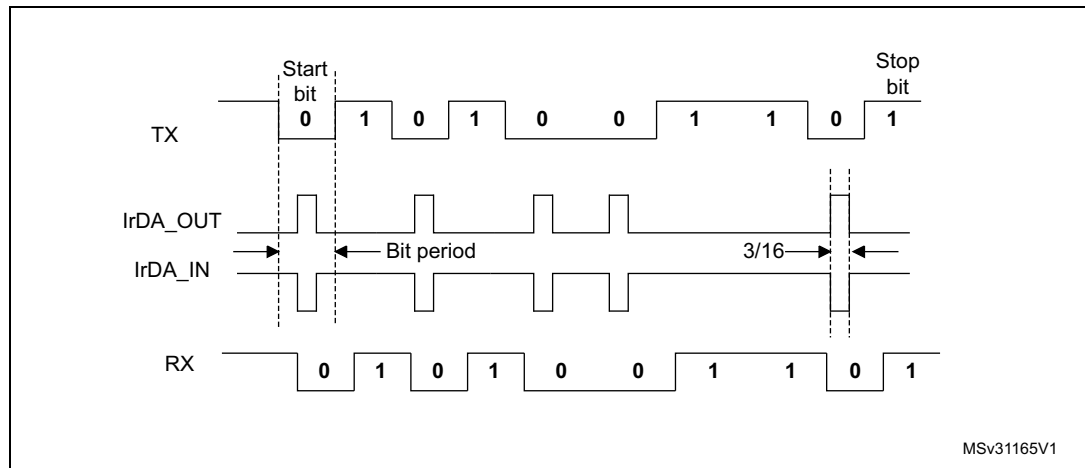
Figure 819. IrDA data modulation (3/16) - Normal mode
