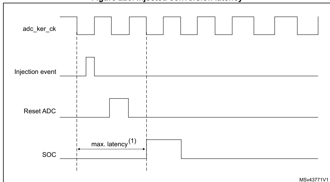
Figure 226. Injected conversion latency
