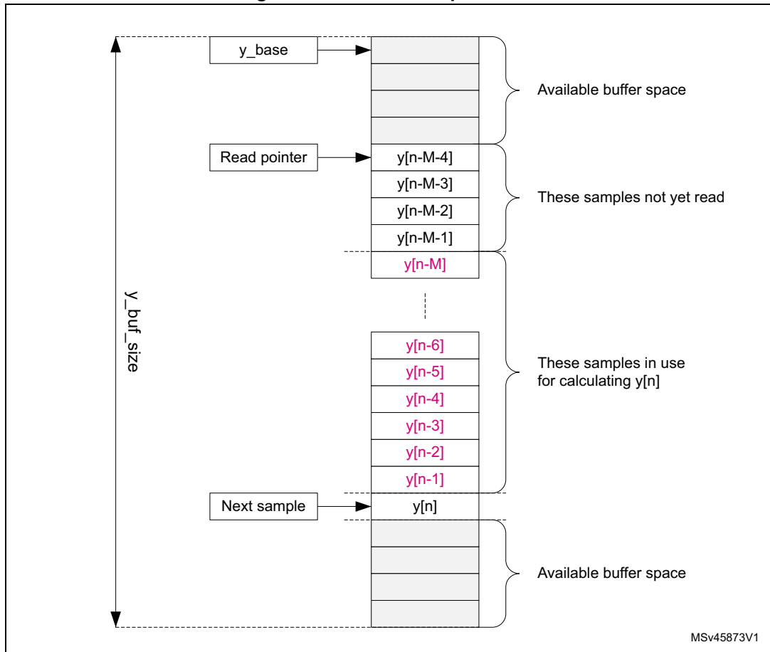
Figure 110. Circular output buffer
