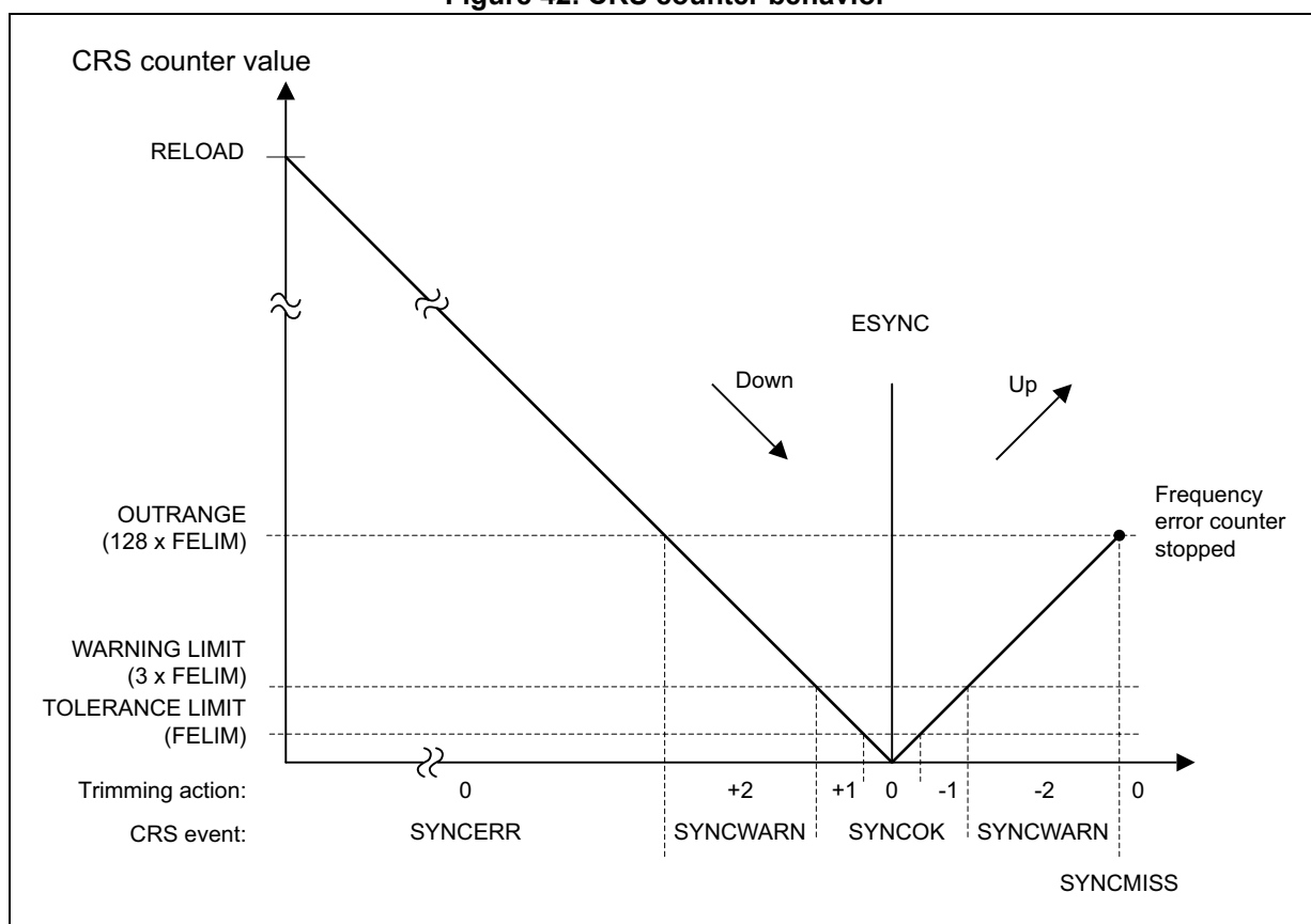
Figure 42. CRS counter behavior
