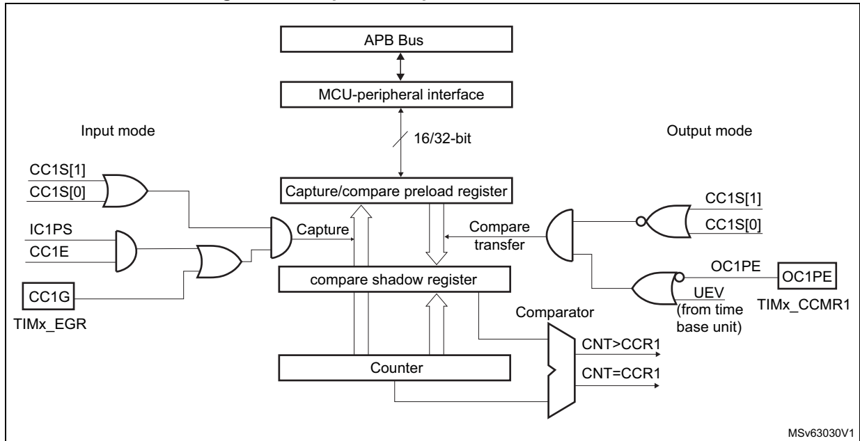
Figure 619. Capture/compare channel 1 main circuit
