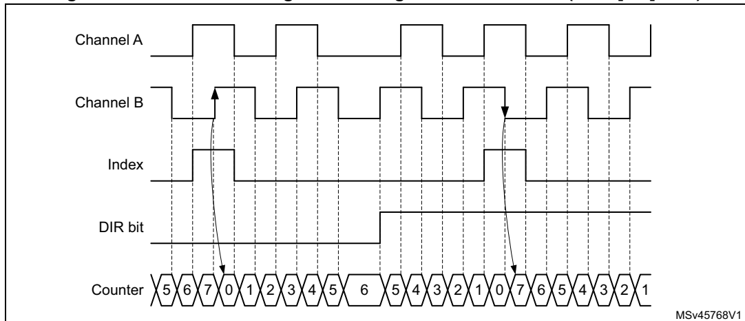
Figure 572. Counter reading with index gated on channel A (IPOS[1:0] = 11)
