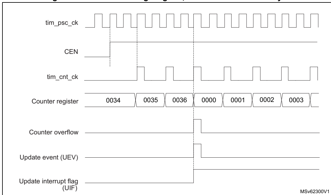
Figure 721. Counter timing diagram, internal clock divided by 2
