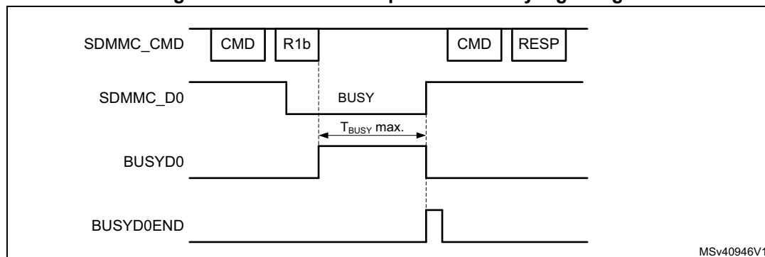
Figure 209. Command response R1b busy signaling
