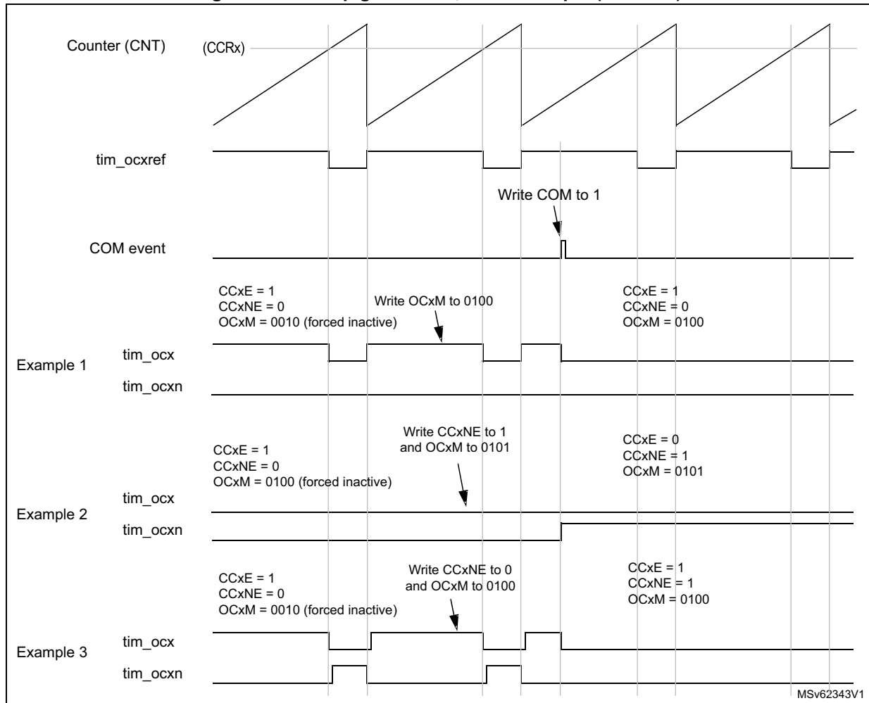
Figure 709. 6-step generation, COM example (OSSR=1)
