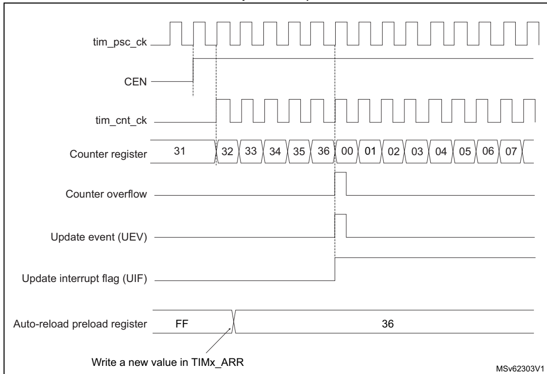
Figure 724. Counter timing diagram, update event when ARPE = 0 (TIMx_ARR not preloaded)
