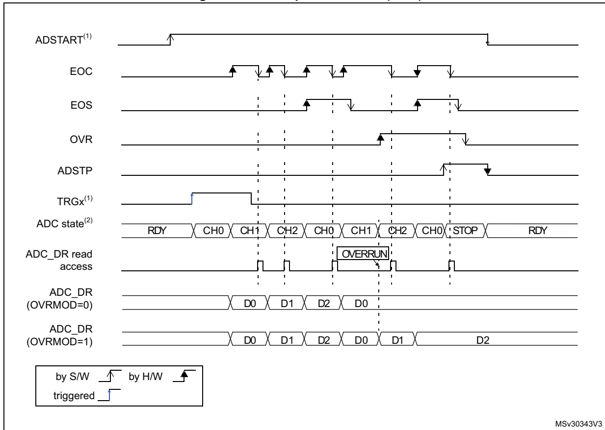
Figure 286. Example of overrun (OVR)
