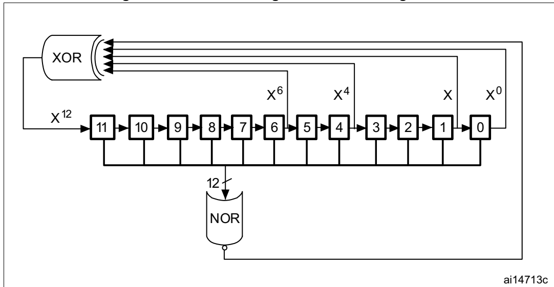
Figure 306. DAC LFSR register calculation algorithm
