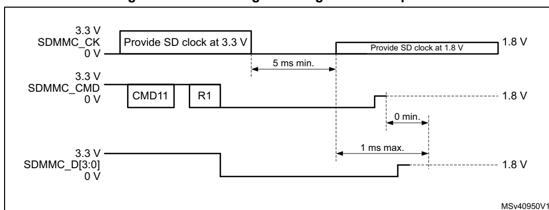
Figure 212. CMD11 signal voltage switch sequence
