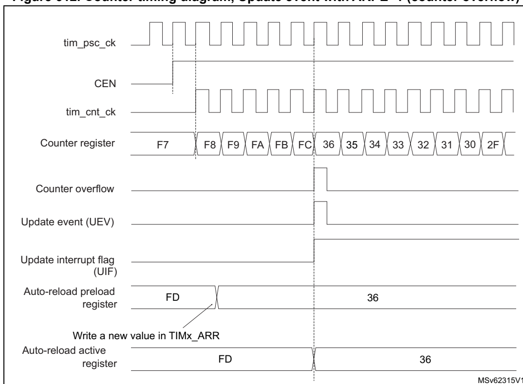
Figure 612. Counter timing diagram, Update event with ARPE=1 (counter overflow)
