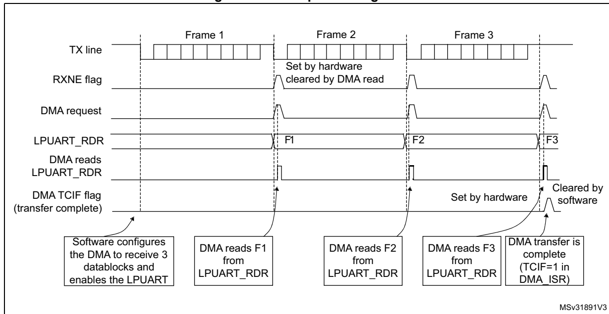
Figure 833. Reception using DMA
