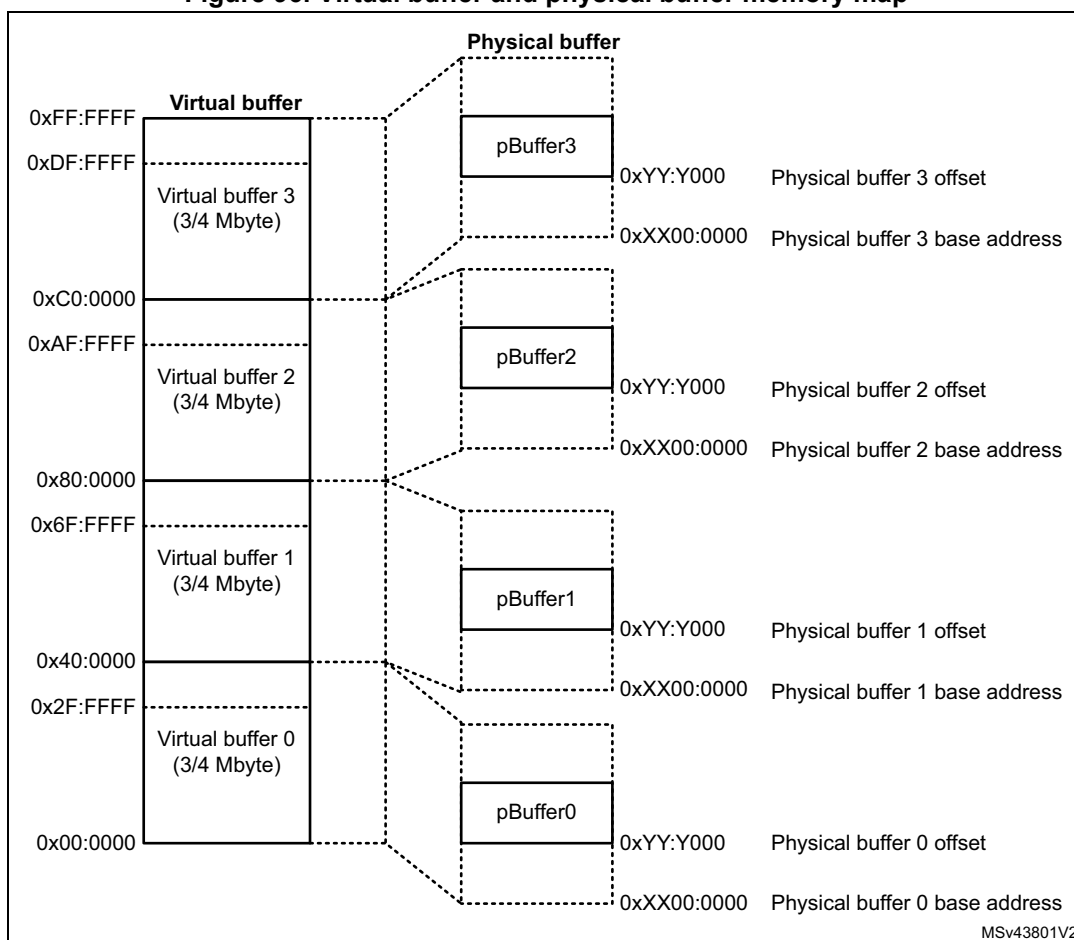
Figure 96. Virtual buffer and physical buffer memory map
