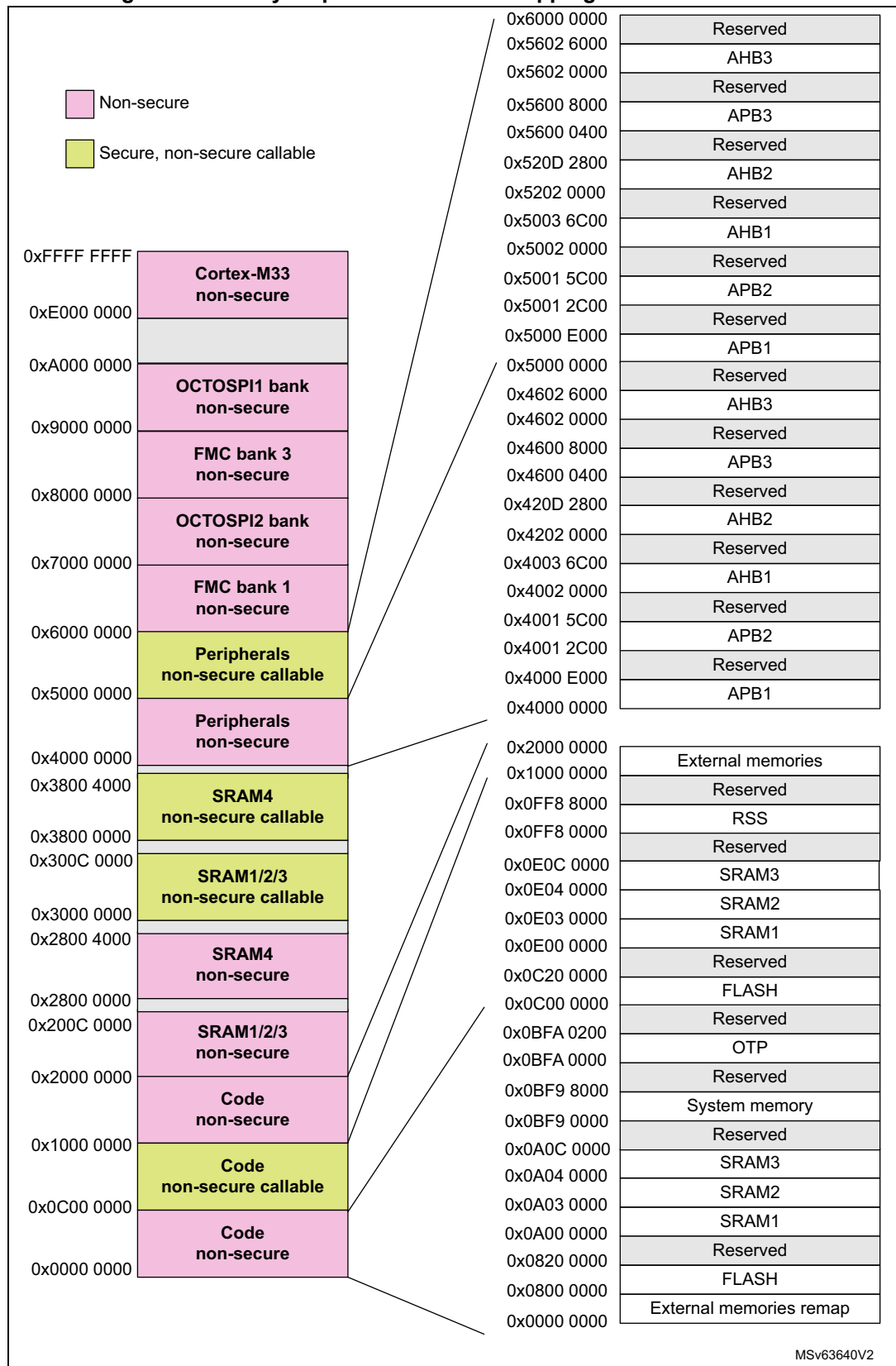
Figure 4. Memory map based on IDAU mapping for STM32U575/585
