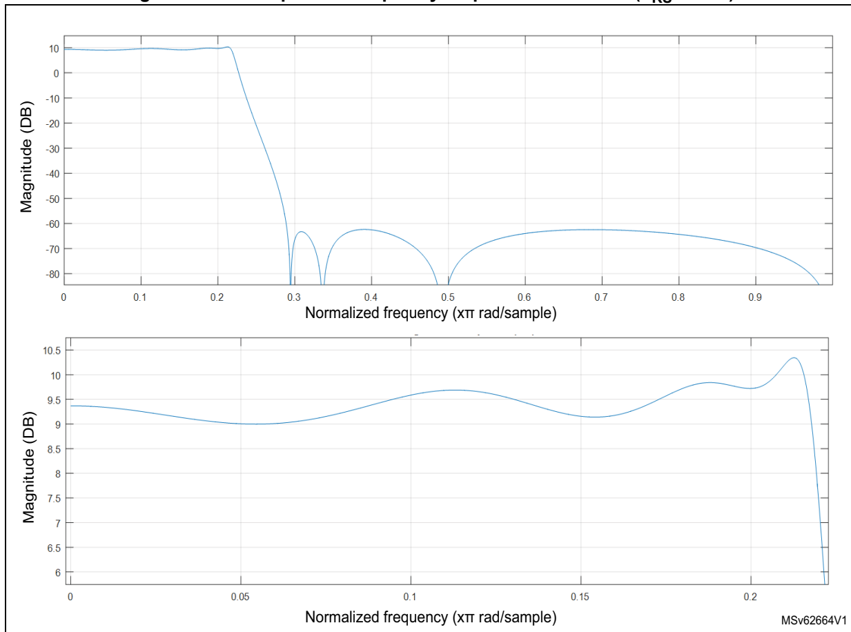
Figure 332. Reshape filter frequency response normalized ( F_{RS} / 2 = 1 )
