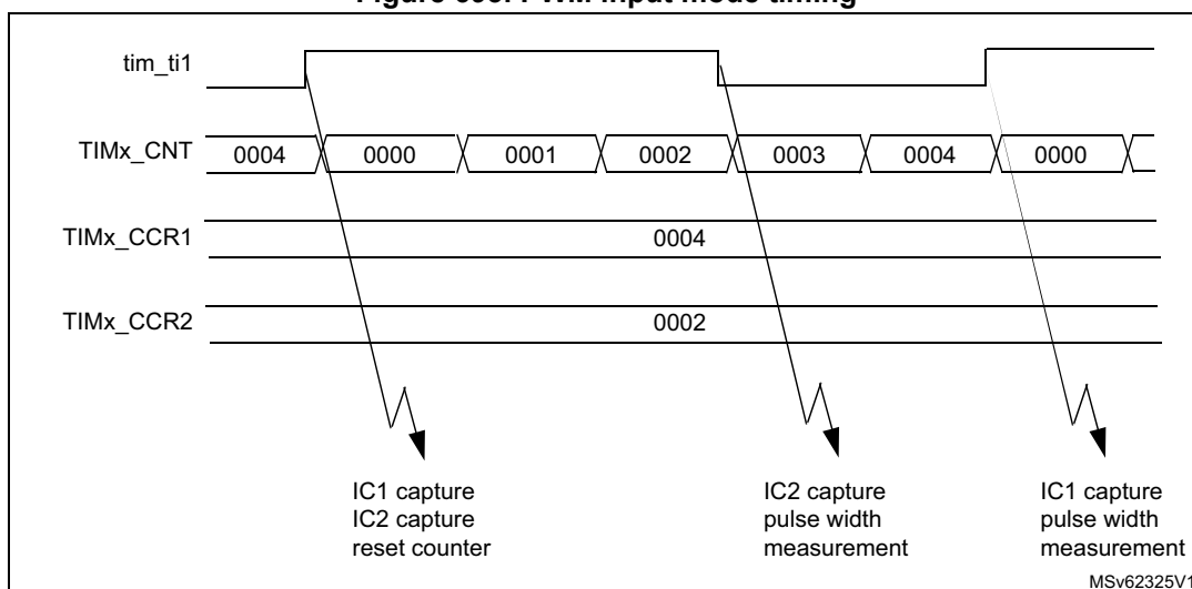
Figure 693. PWM input mode timing
