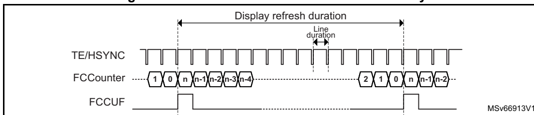
Figure 749. Waveforms with external HSYNC only
