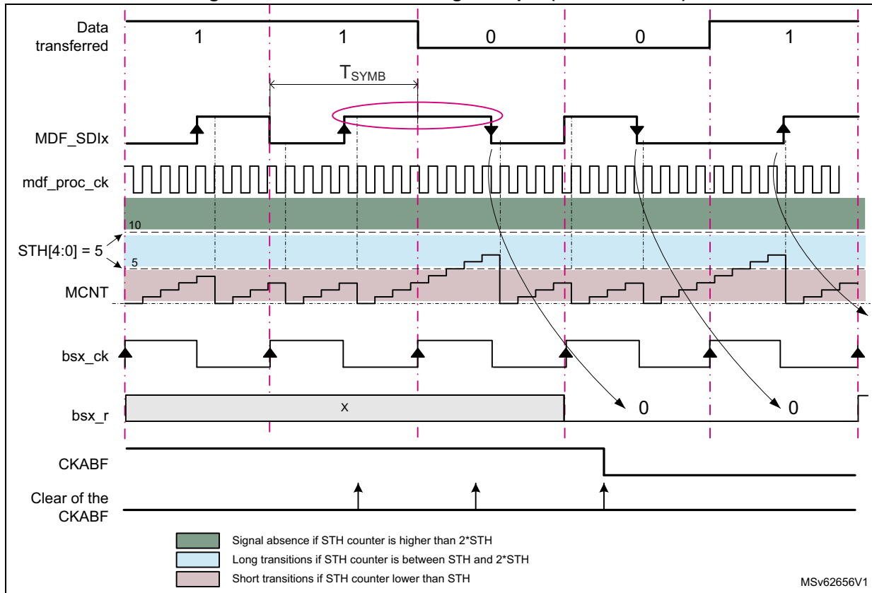
Figure 324. Manchester timing example (SITFMOD = 11)
