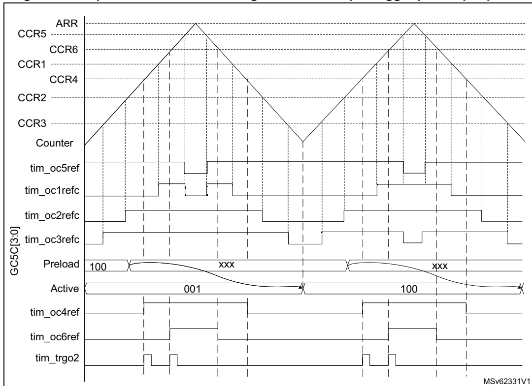
Figure 545. 3-phase combined PWM signals with multiple trigger pulses per period
