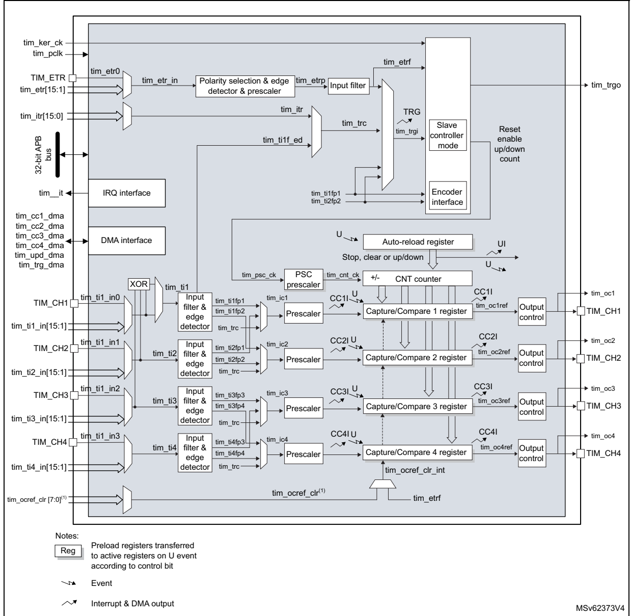
Figure 593. General-purpose timer block diagram
