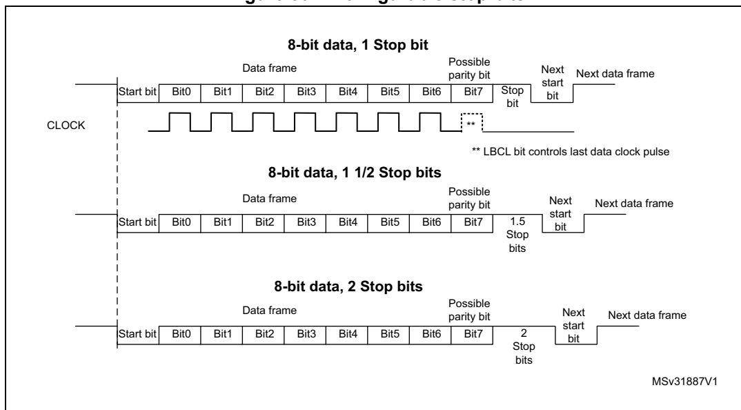
Figure 802. Configurable stop bits
