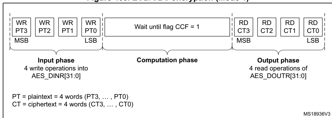
Figure 465. ECB/CBC encryption (Mode 1)
