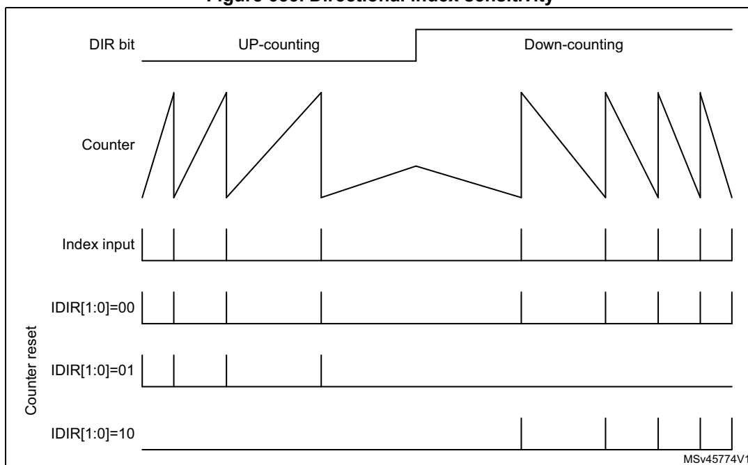
Figure 655. Directional index sensitivity
