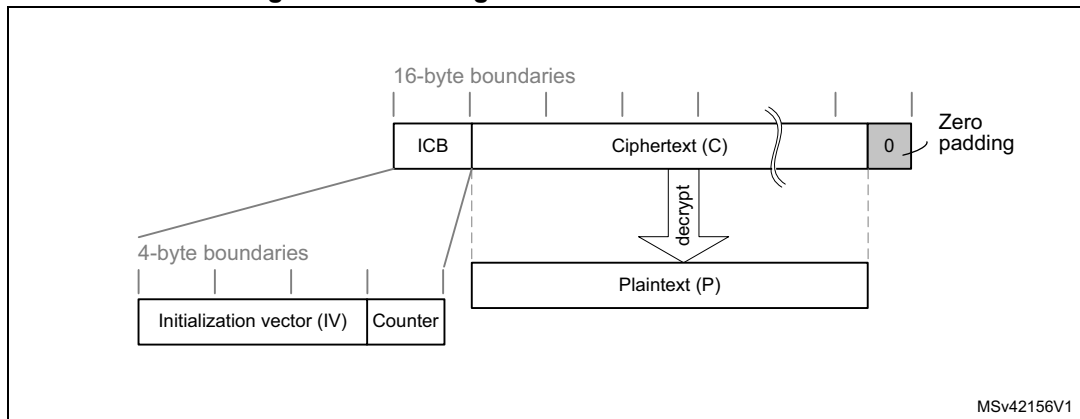
Figure 467. Message construction in CTR mode
