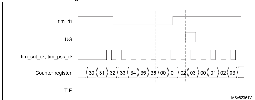
Figure 589. Control circuit in reset mode
