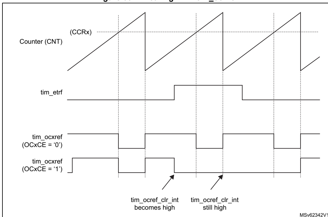
Figure 634. Clearing TIMx tim_ocxref
