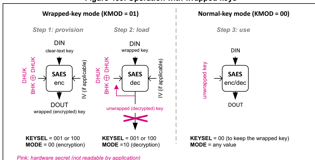
Figure 489. Operation with wrapped keys
