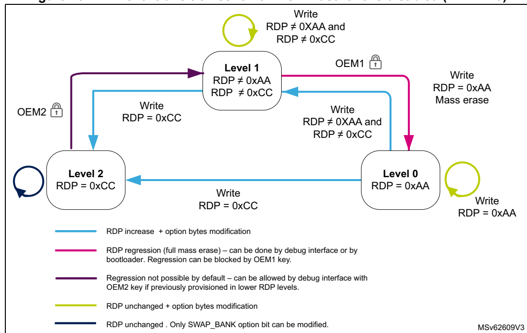
Figure 25. RDP level transition scheme when TrustZone is disabled (TZEN = 0)
