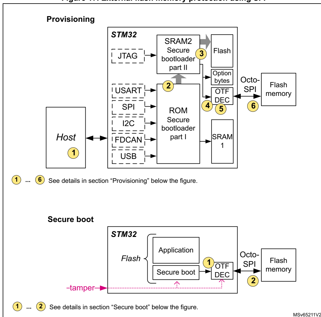
Figure 17. External flash memory protection using SFI
