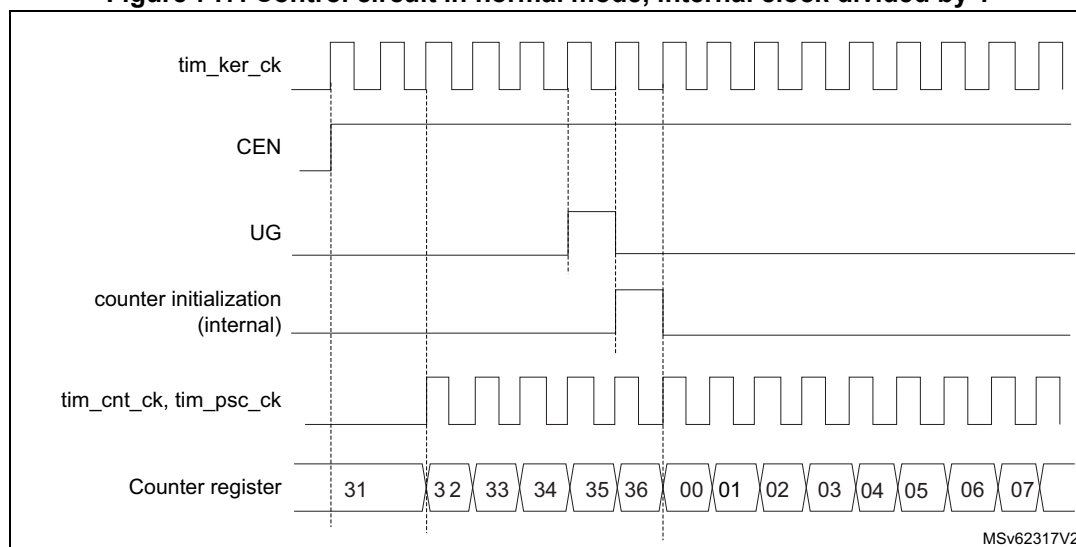
Figure 717. Control circuit in normal mode, internal clock divided by 1
