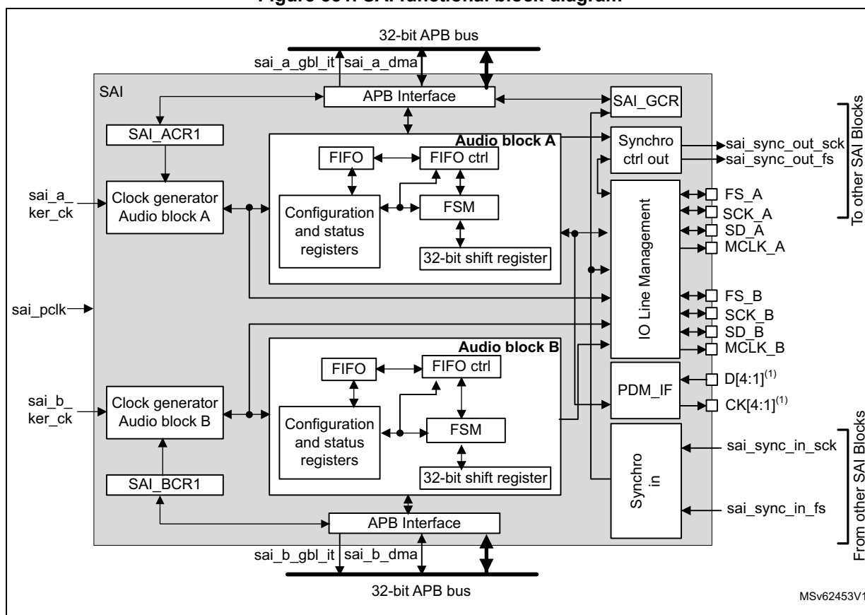
Figure 851. SAI functional block diagram
