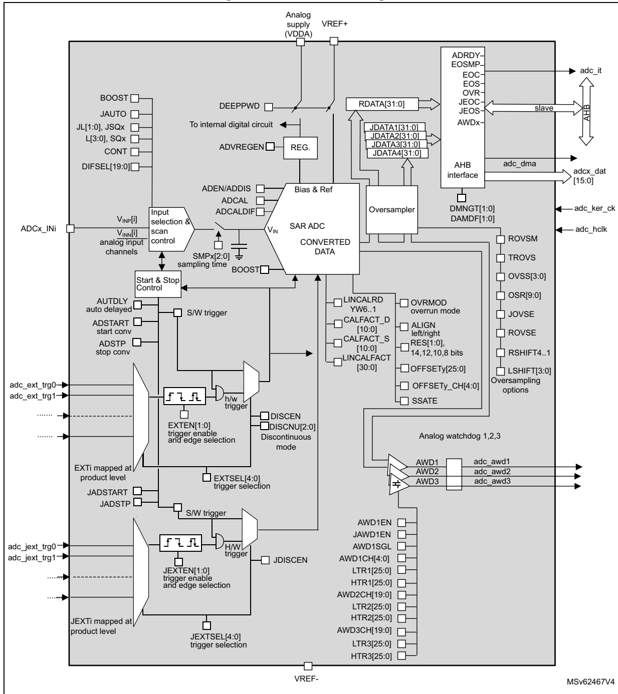
Figure 215. ADC block diagram
