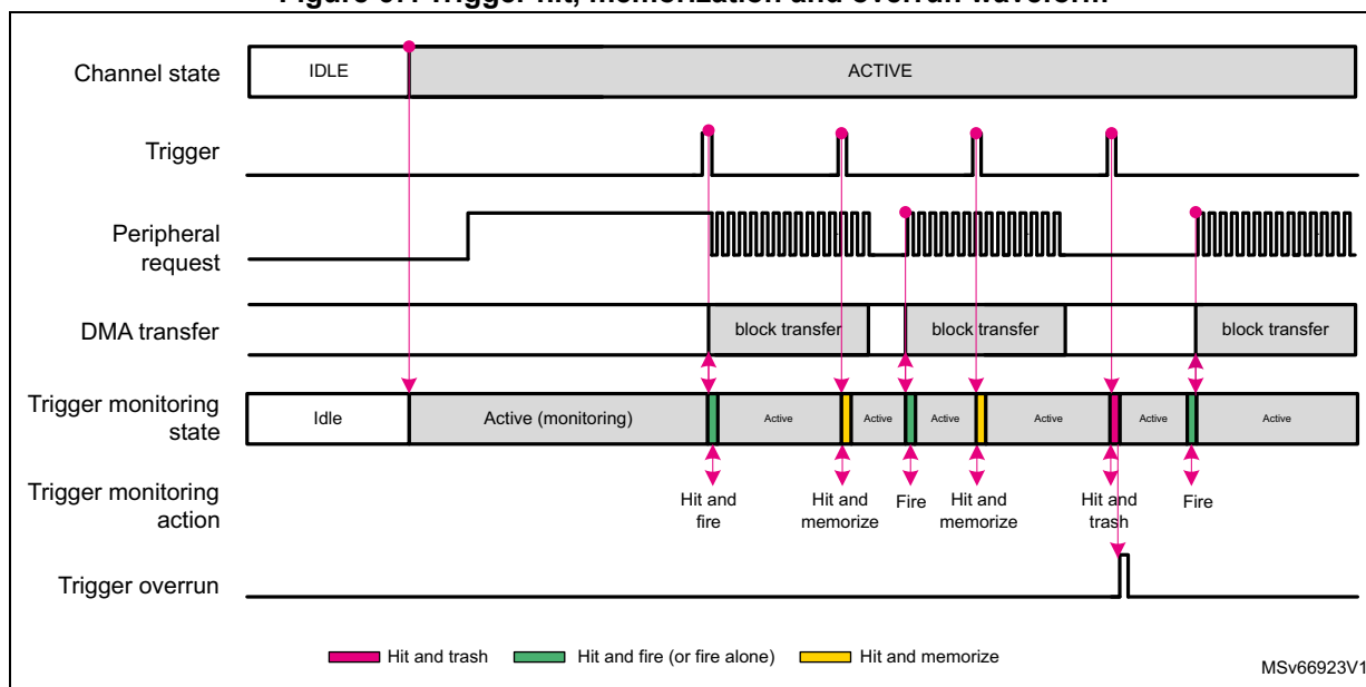
Figure 67. Trigger hit, memorization and overrun waveform
