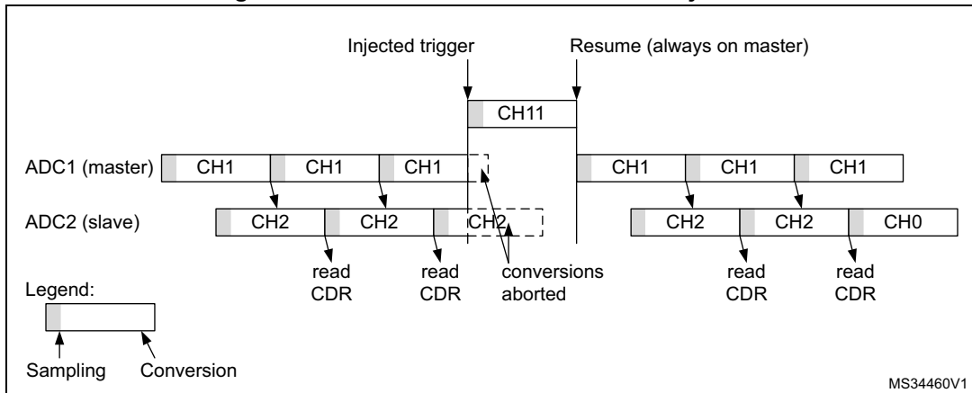
Figure 258. Interleaved conversion with injection
