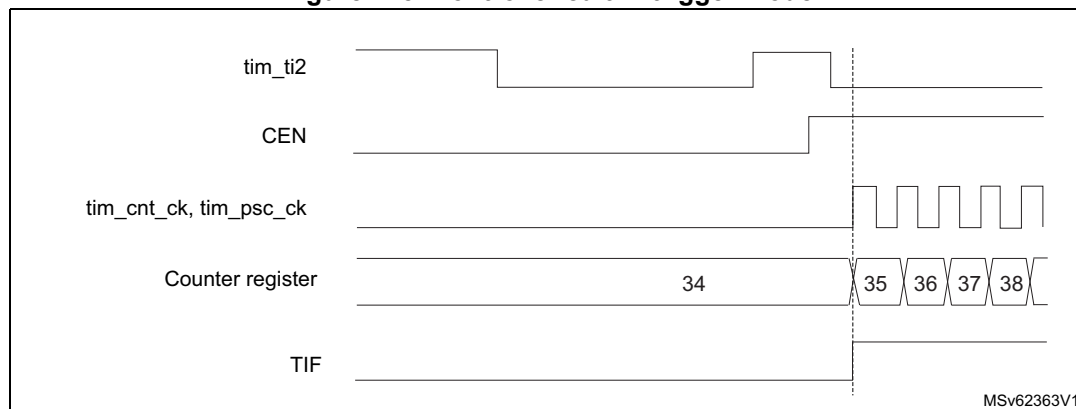
Figure 715. Control circuit in trigger mode
