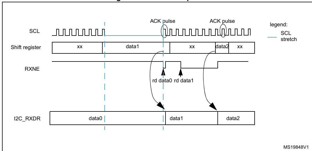
Figure 774. Data reception
