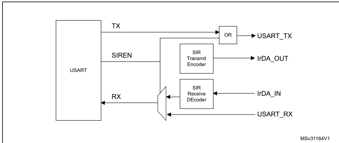
Figure 818. IrDA SIR ENDEC block diagram
