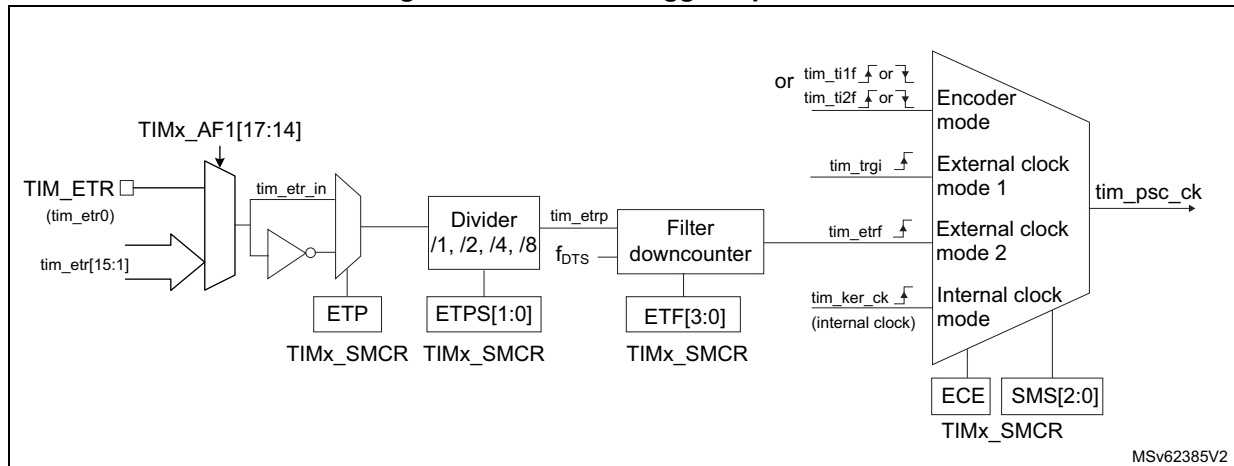
Figure 616. External trigger input block
