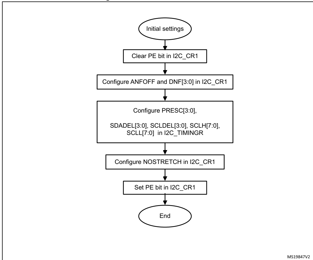
Figure 773. I2C initialization flow
