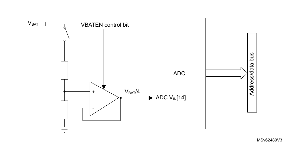
Figure 301. V_{BAT} channel block diagram
