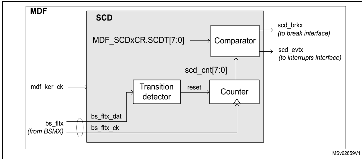
Figure 327. SCD functional view
