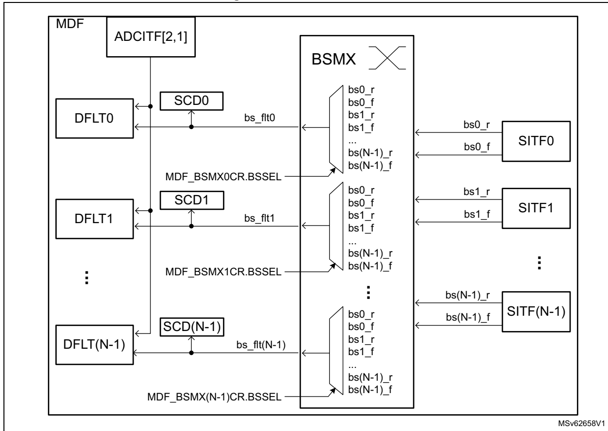
Figure 326. BSMX overview
