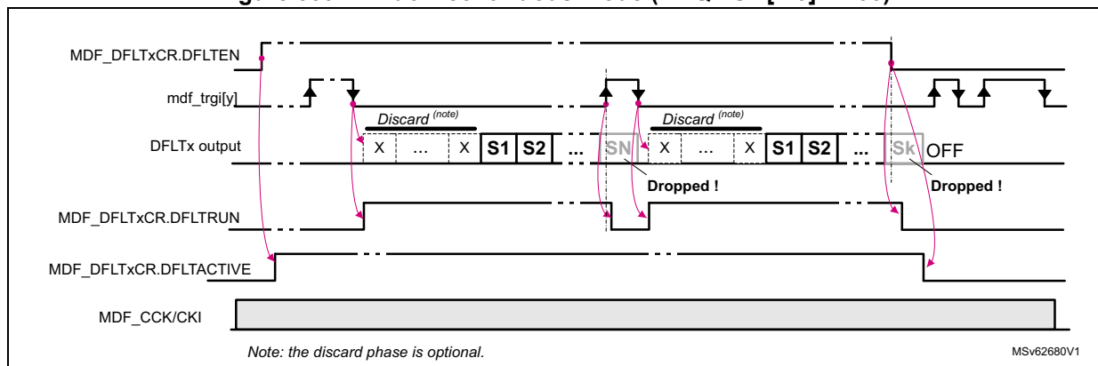
Figure 339. Window continuous mode (ACQMOD[2:0] = 100)
