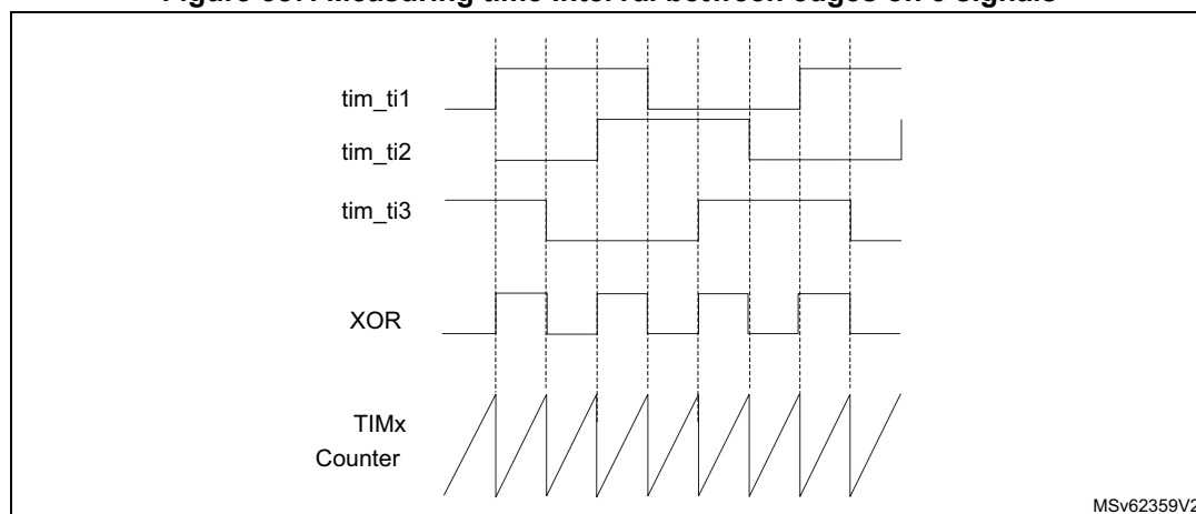
Figure 587. Measuring time interval between edges on 3 signals
