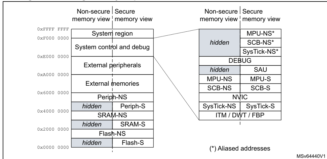
Figure 8. Sharing memory map between CPU in secure and nonsecure state
