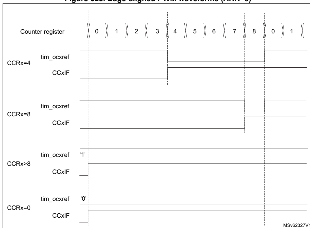
Figure 623. Edge-aligned PWM waveforms (ARR=8)
