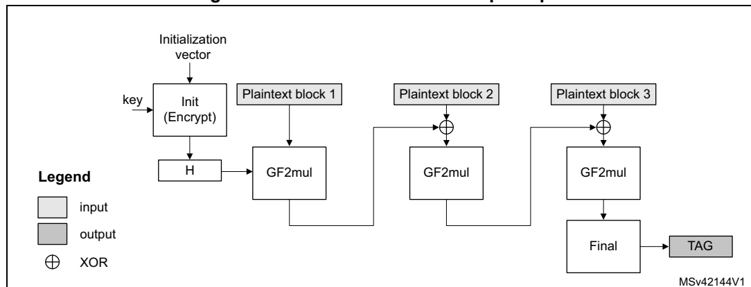
Figure 458. GMAC authentication principle
