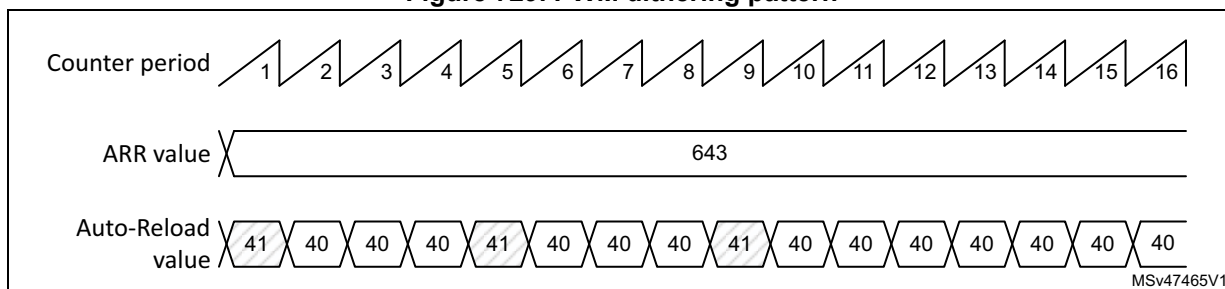
Figure 729. PWM dithering pattern
