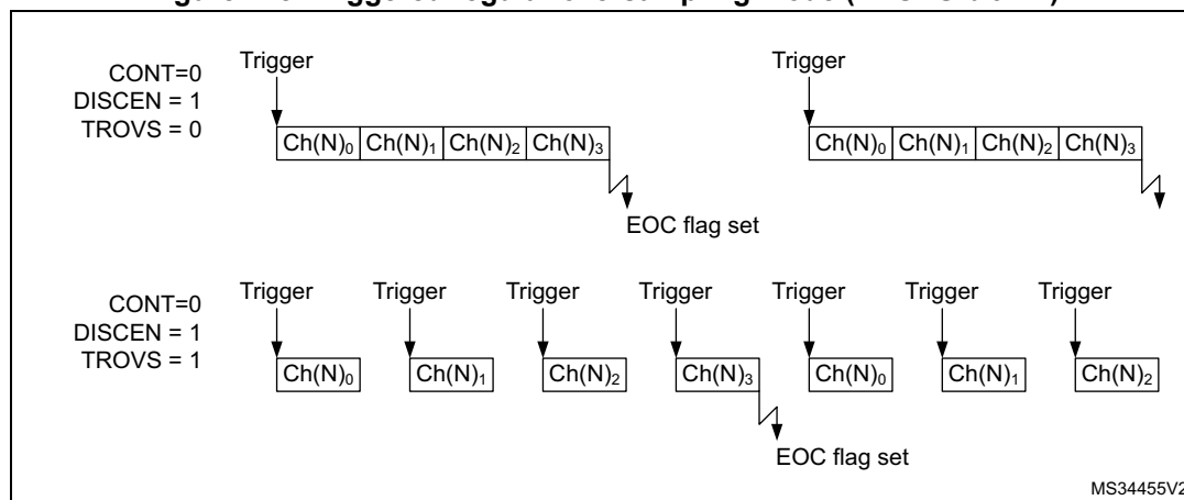
Figure 248. Triggered regular oversampling mode (TROVS bit = 1)
