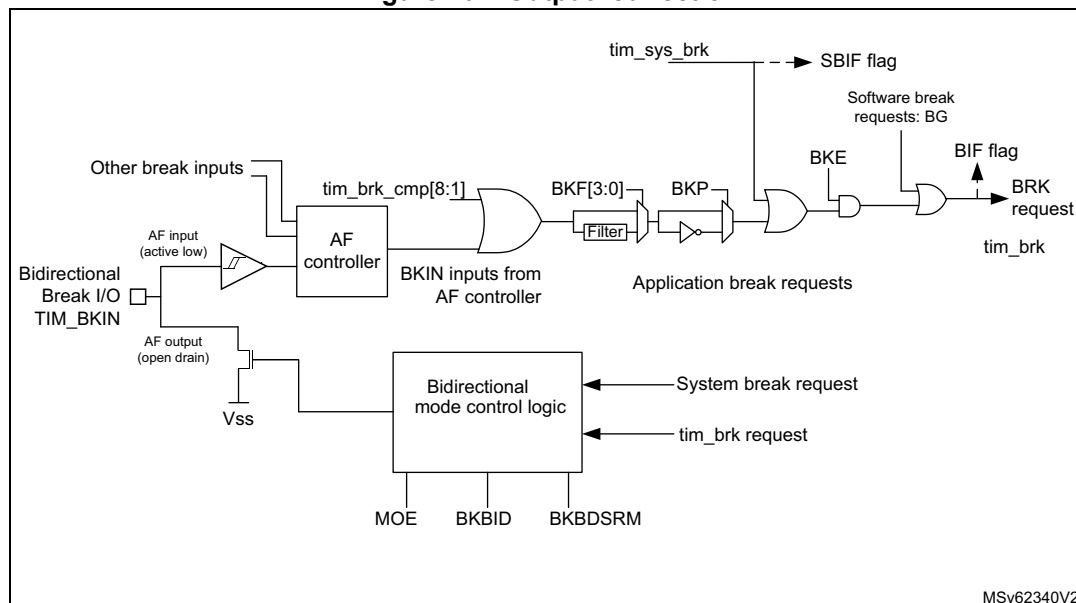
Figure 707. Output redirection
