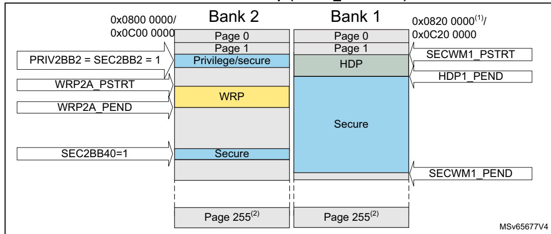
Figure 24. Flash memory security attributes and protections in case of bank swap (SWAP_BANK = 1)
