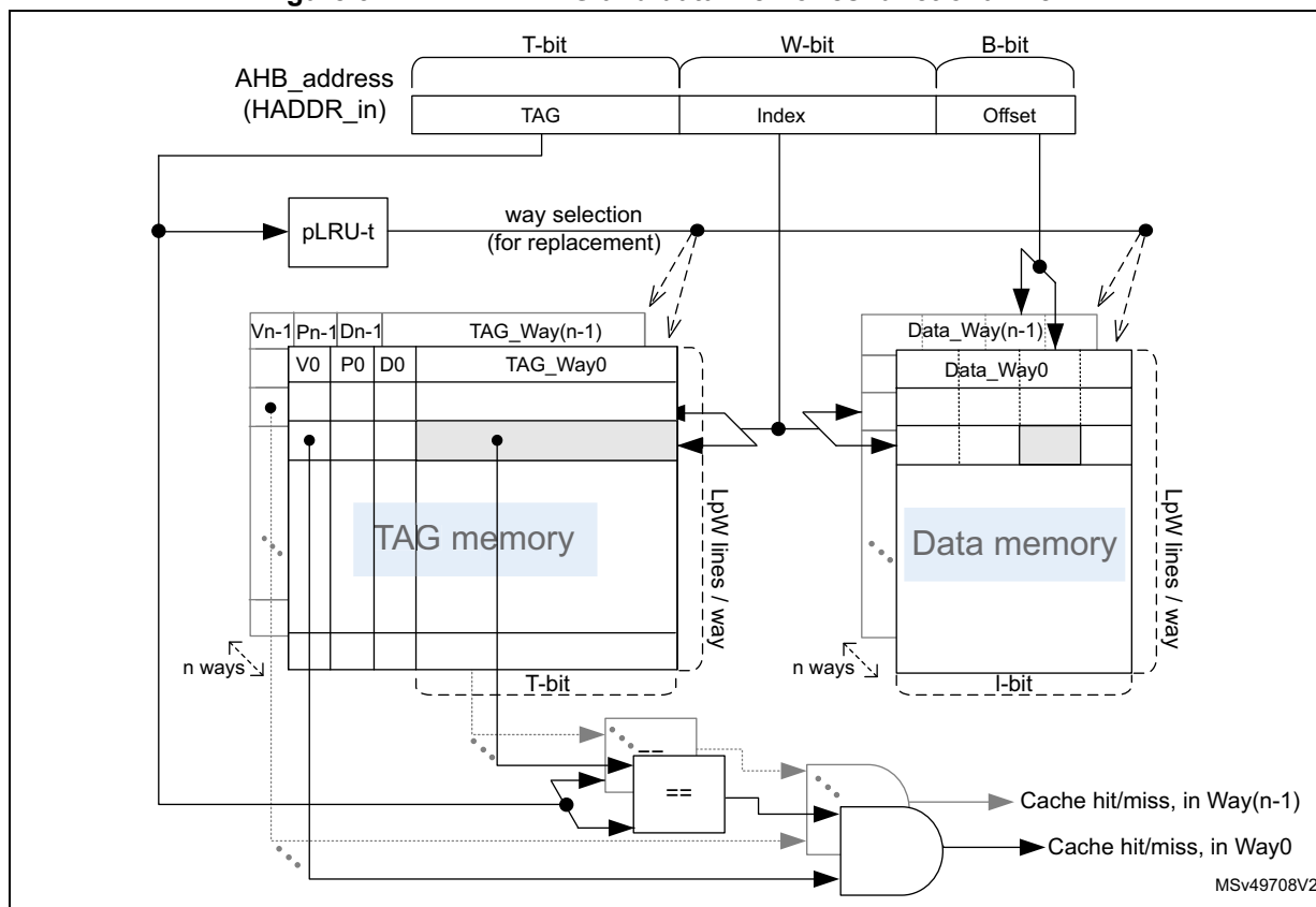
Figure 31. DCACHE TAG and data memories functional view
