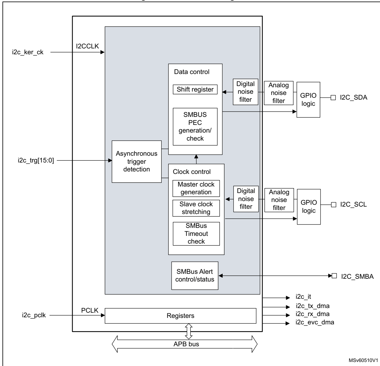
Figure 770. I2C block diagram
