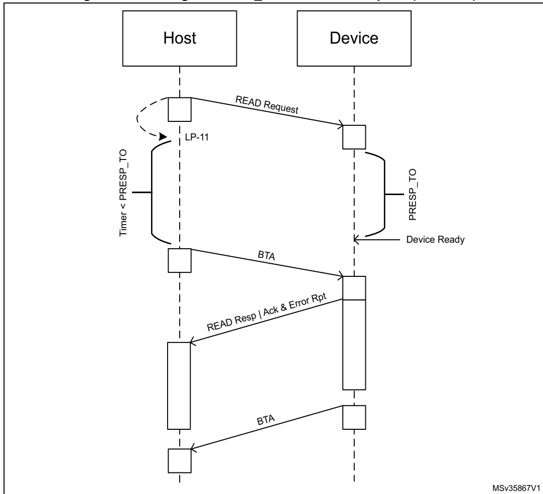
Figure 418. Timing of PRESP_TO after a read request (HS or LP)
