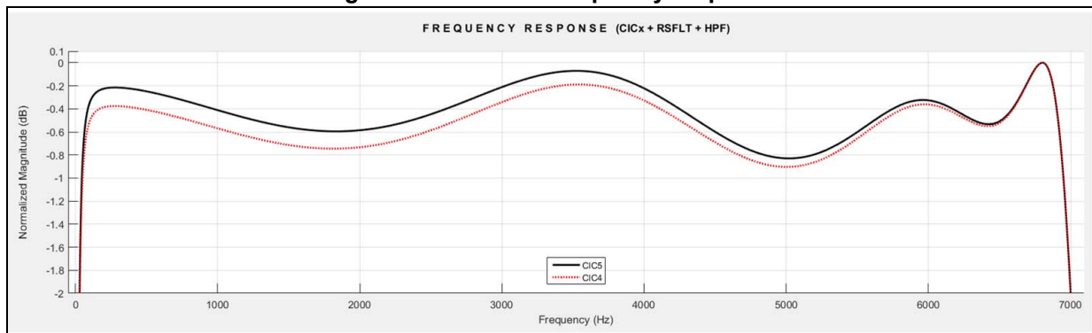
Figure 353. Detailed frequency response
