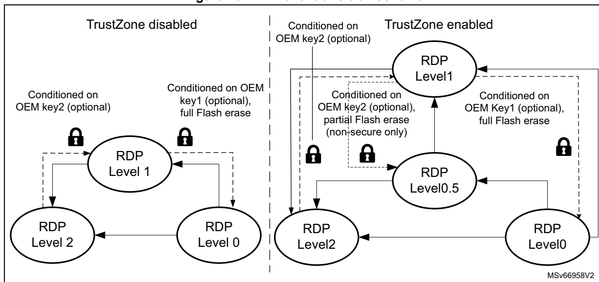
Figure 15. RDP level transition scheme
