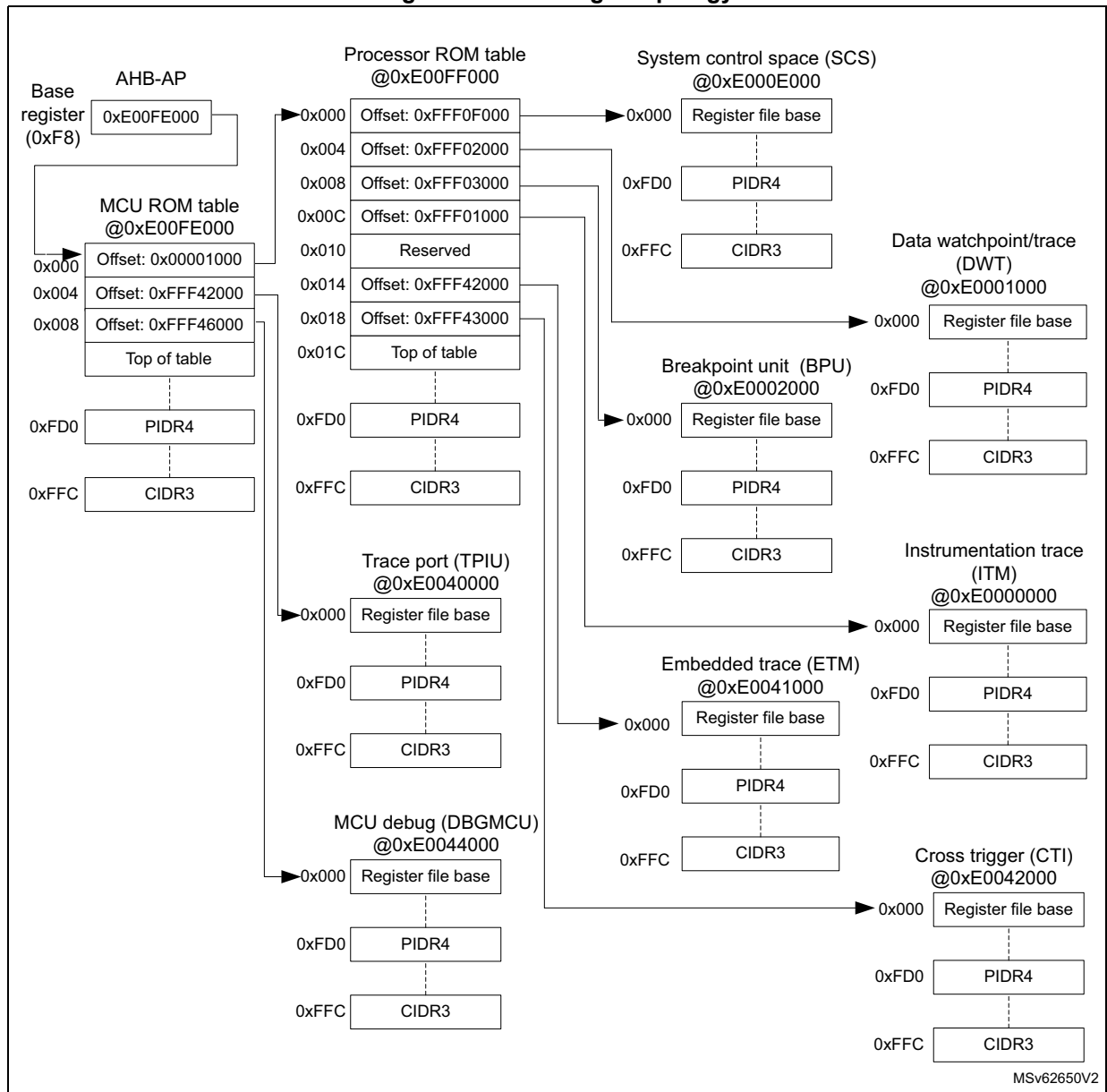
Figure 949. CoreSight topology
