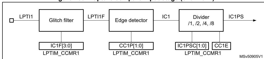
Figure 739. Capture/compare input stage (channel 1)
