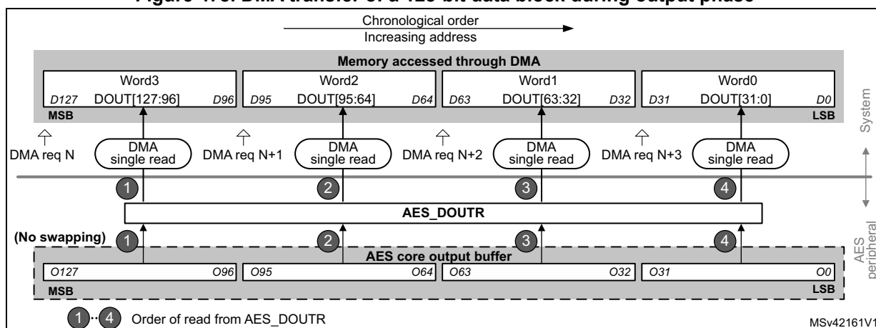
Figure 478. DMA transfer of a 128-bit data block during output phase
