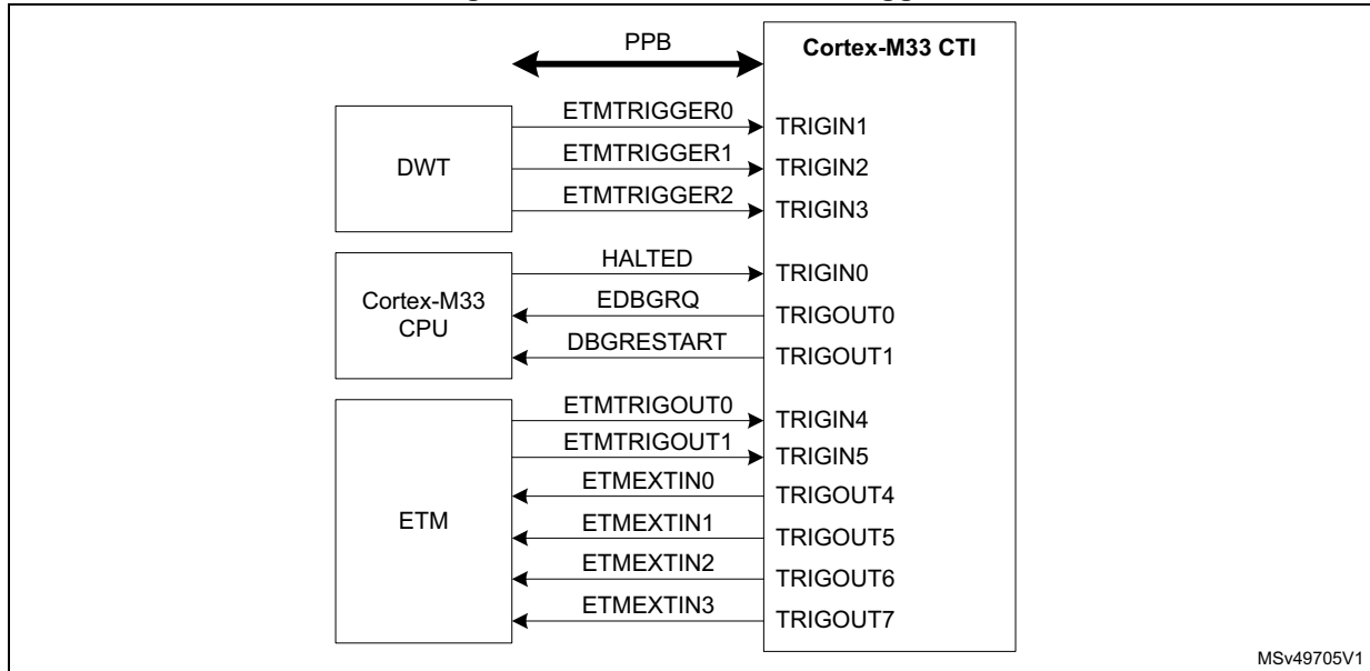
Figure 951. Embedded cross trigger
