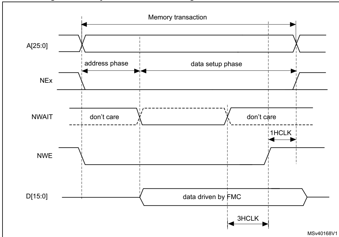
Figure 133. Asynchronous wait during a write access waveforms
