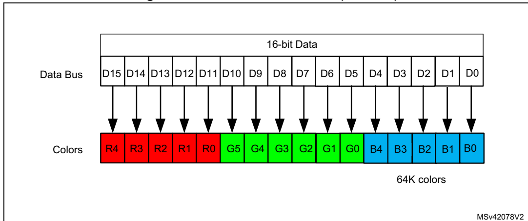
Figure 92. Intel 8080 16-bit mode (RGB565)
