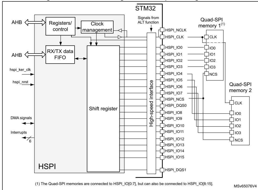
Figure 164. HSPI block diagram for dual-quad configuration
