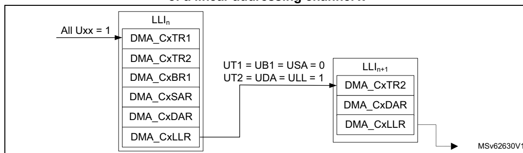
Figure 55. GPDMA dynamic linked-list data structure of a linear addressing channel x
