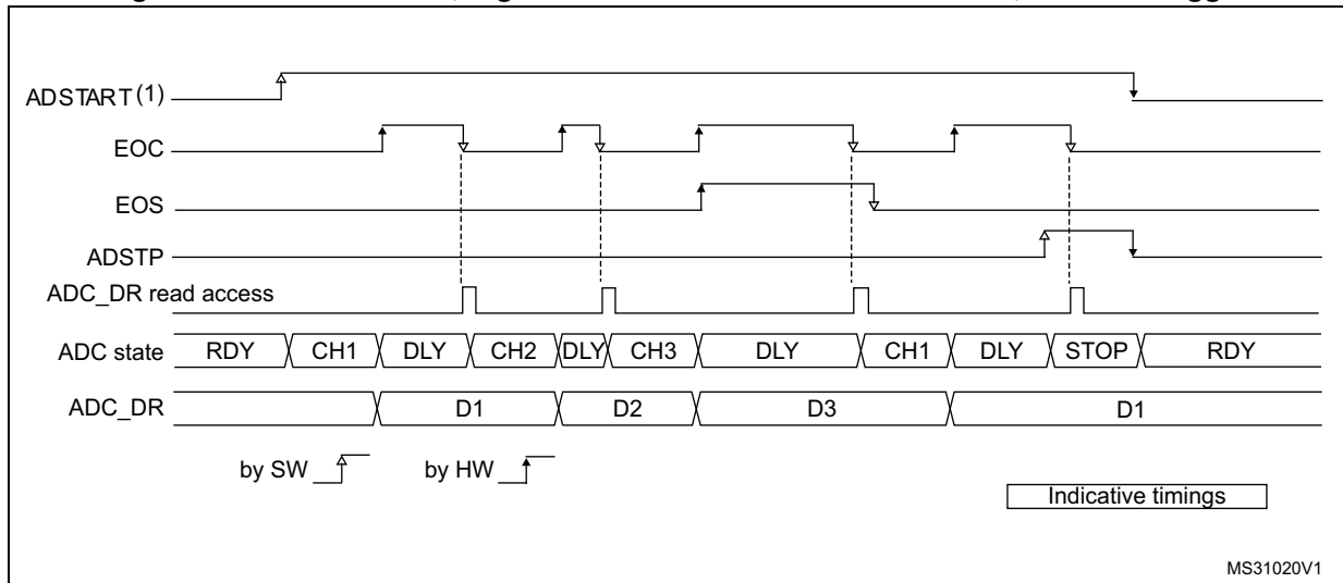
Figure 237. AUTDLY = 1, regular conversion in continuous mode, software trigger
