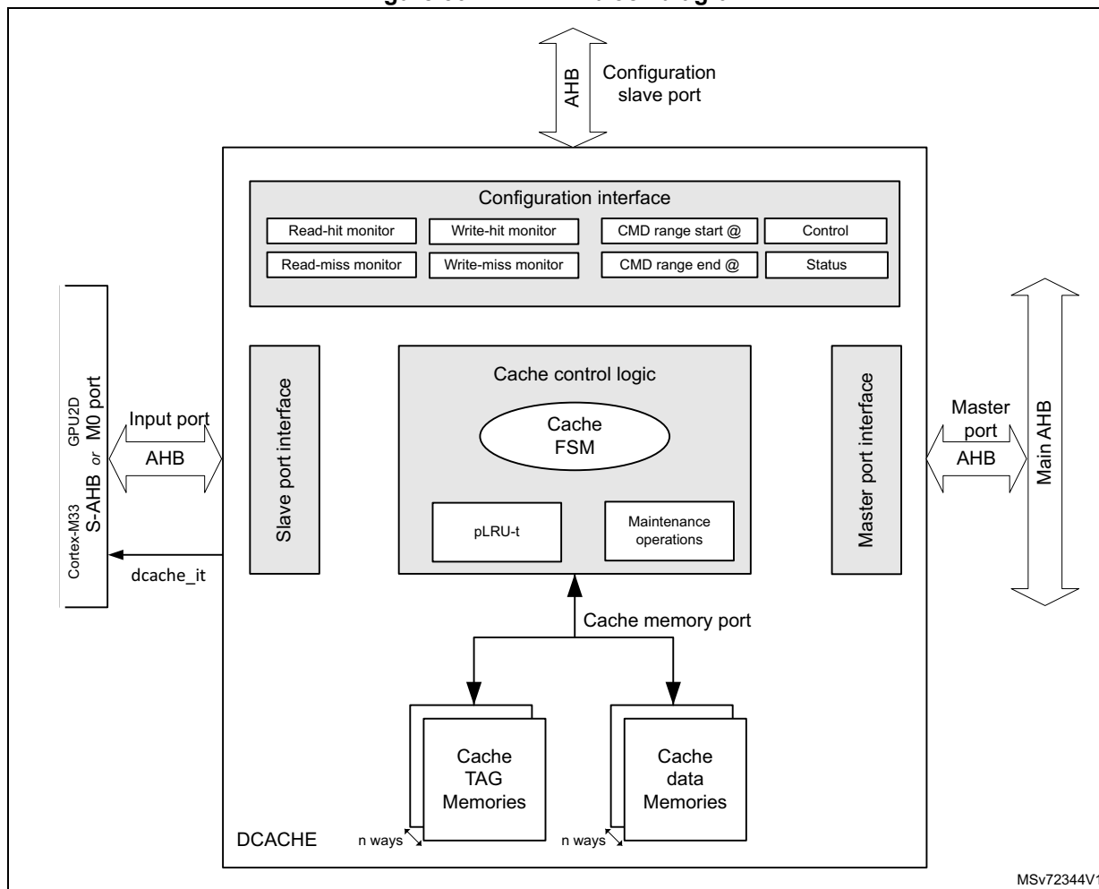
Figure 30. DCACHE block diagram
