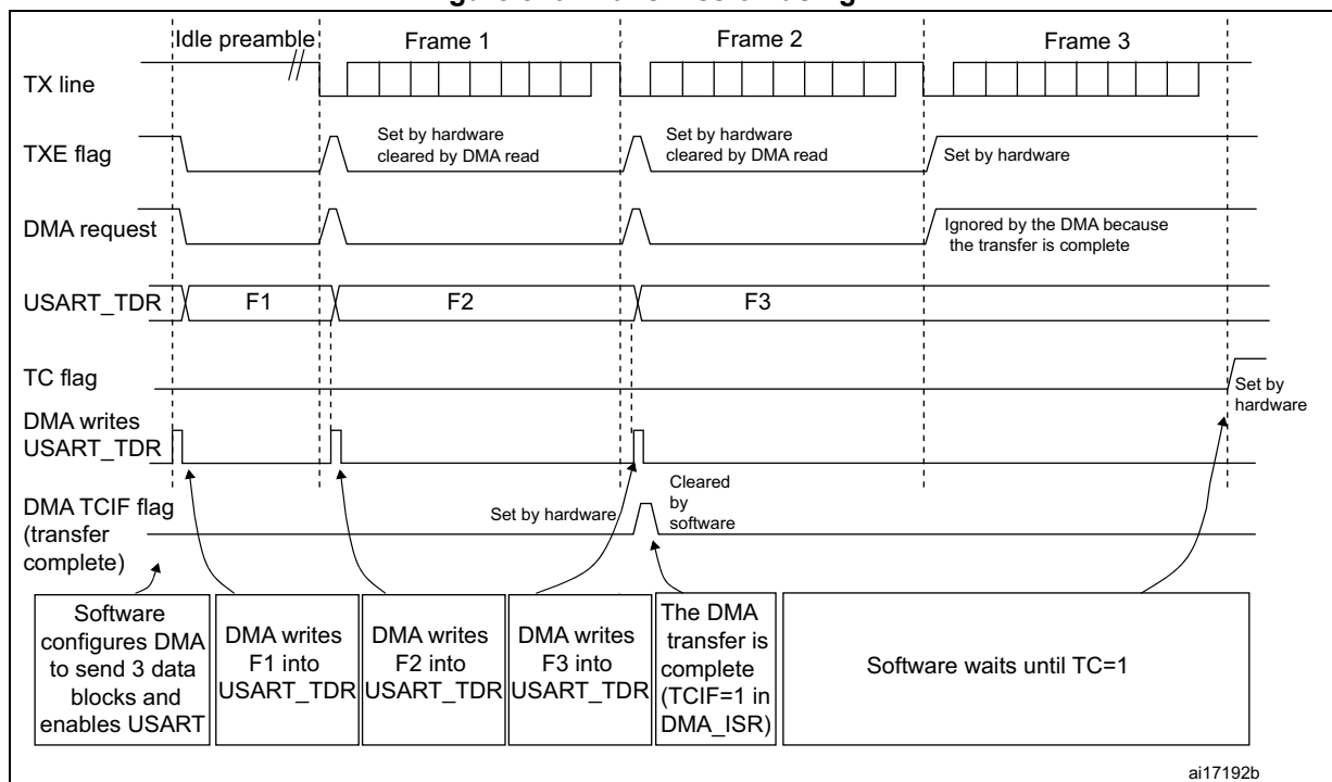
Figure 820. Transmission using DMA
