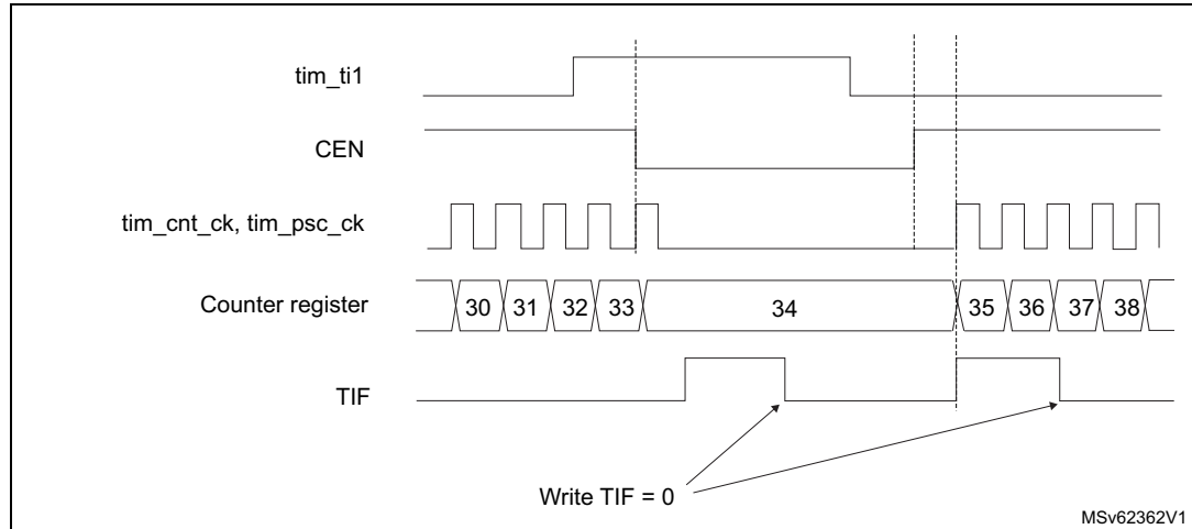
Figure 590. Control circuit in Gated mode
