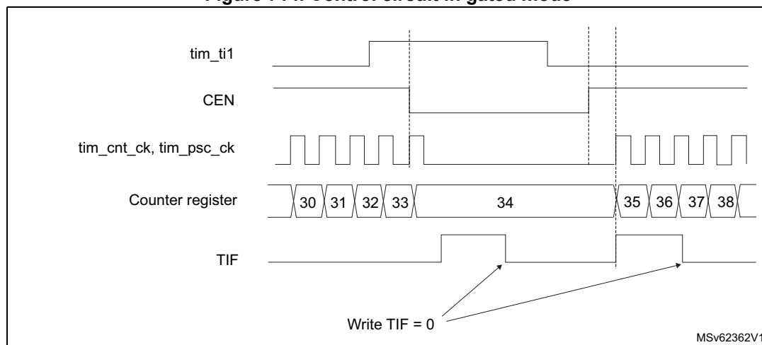
Figure 714. Control circuit in gated mode
