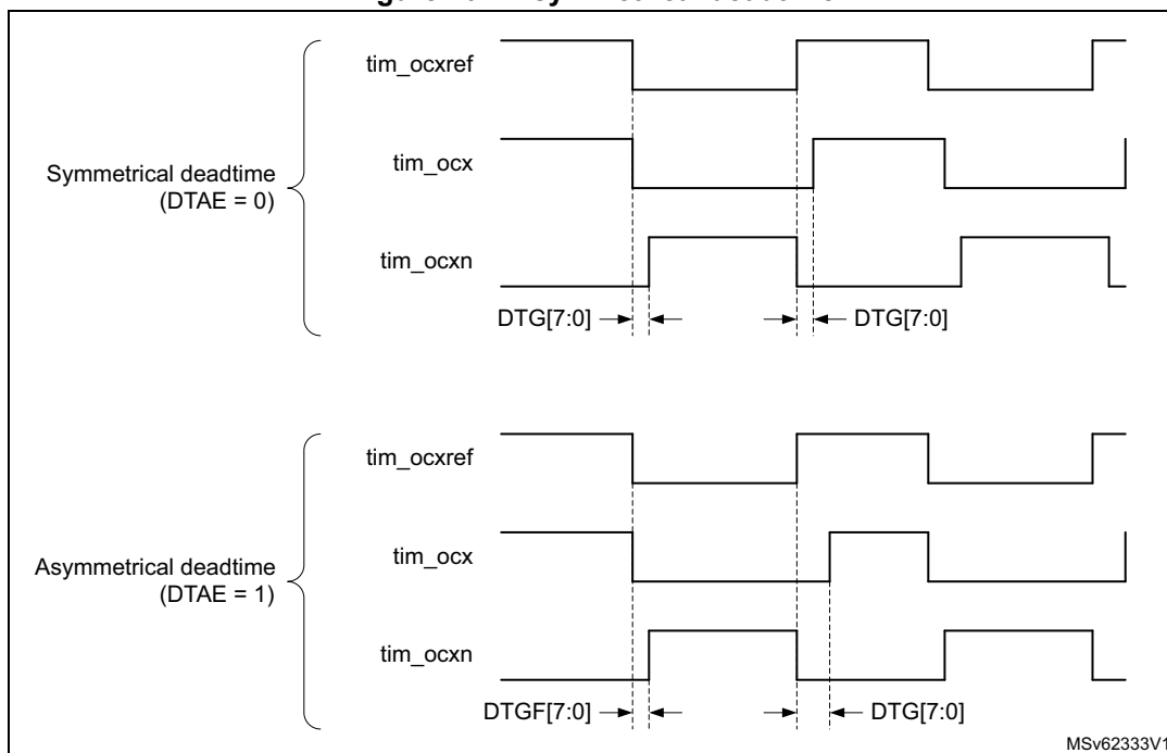
Figure 702. Asymmetrical deadtime
