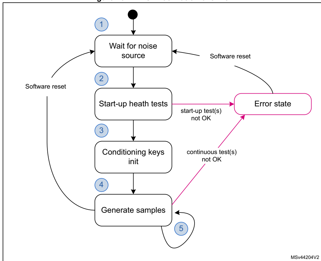
Figure 452. RNG initialization overview
