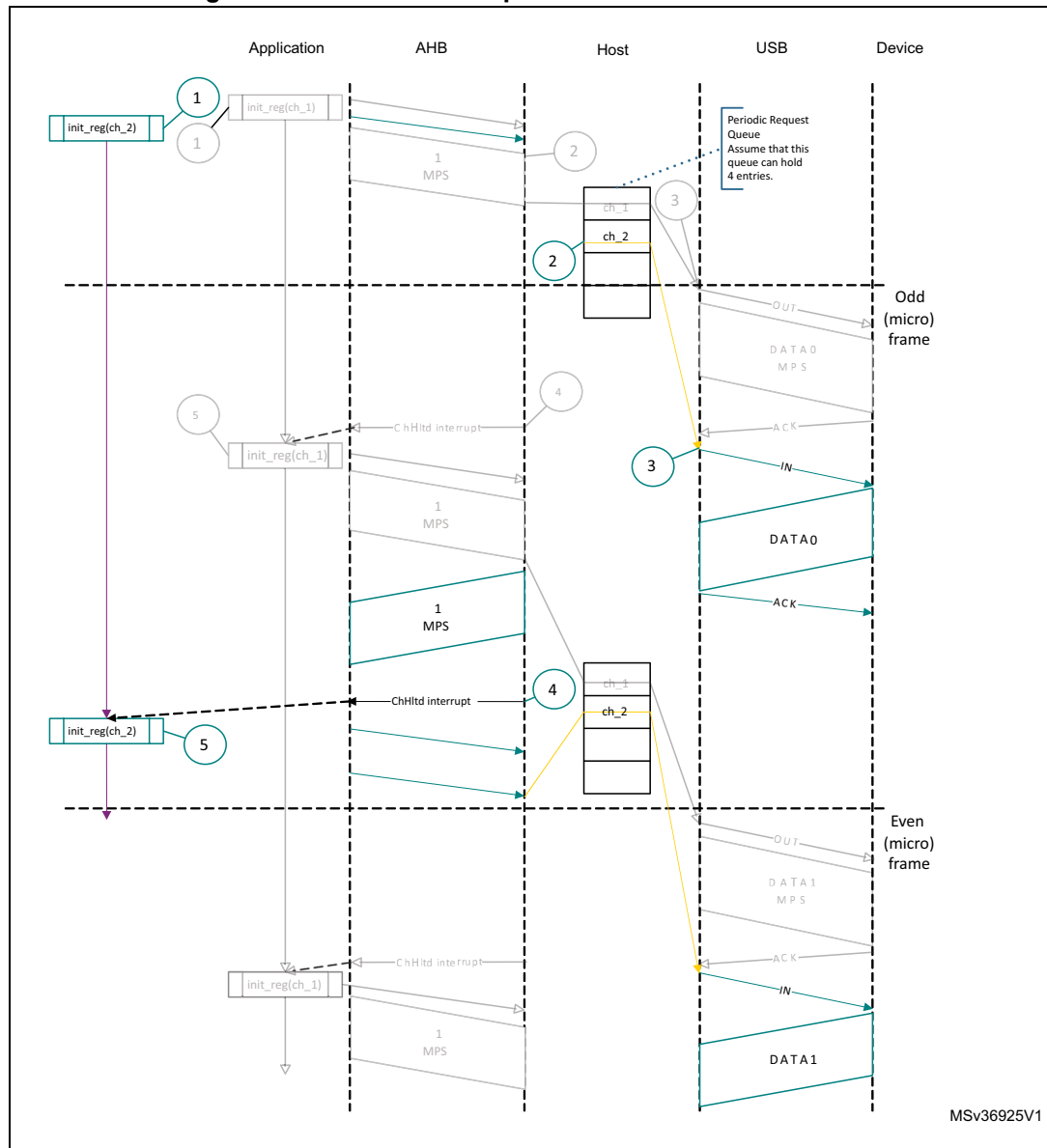
Figure 929. Normal interrupt IN transactions - DMA mode
