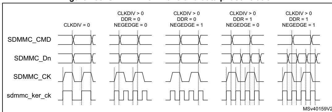
Figure 186. SDMMC Command and data phase relation
