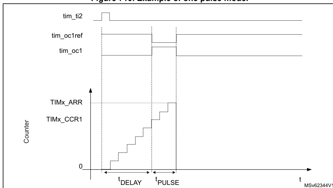
Figure 710. Example of one pulse mode.
