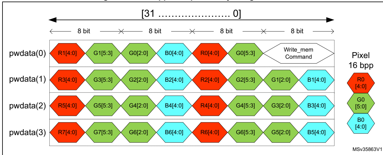
Figure 414. 16 bpp APB pixel to byte organization
