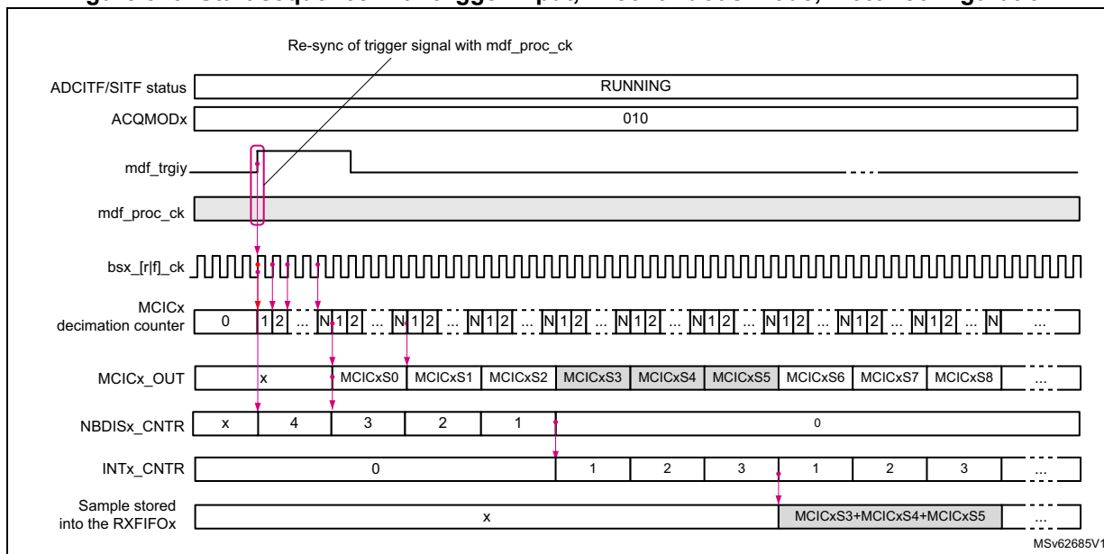
Figure 343. Start sequence with trigger input, in continuous mode, motor configuration
