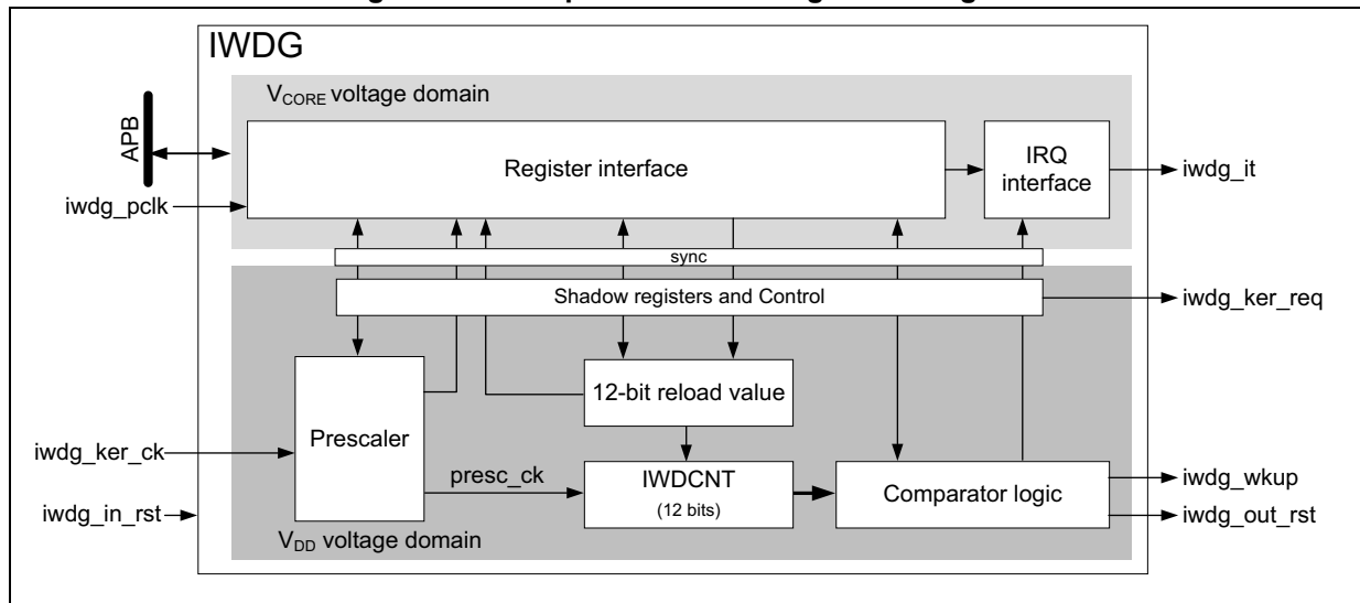
Figure 760. Independent watchdog block diagram
