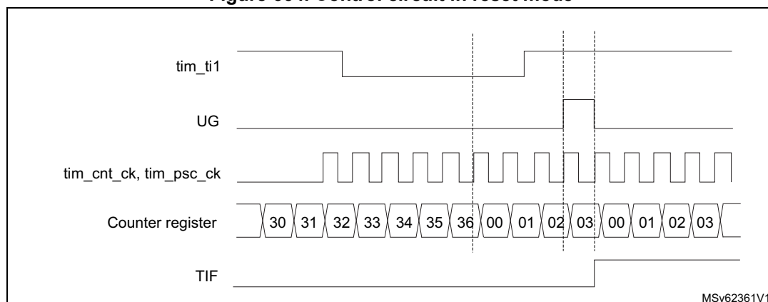
Figure 664. Control circuit in reset mode
