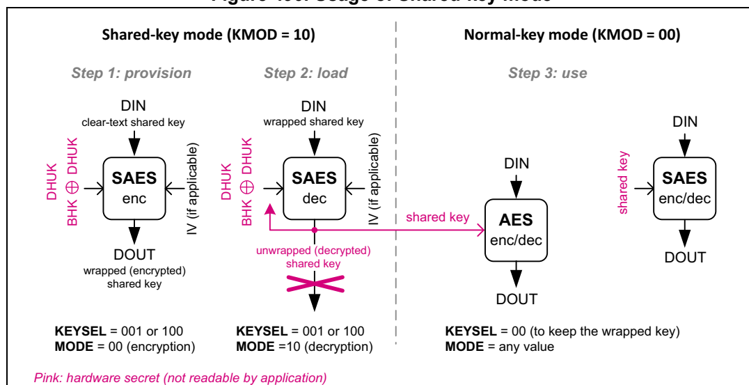
Figure 490. Usage of Shared-key mode
