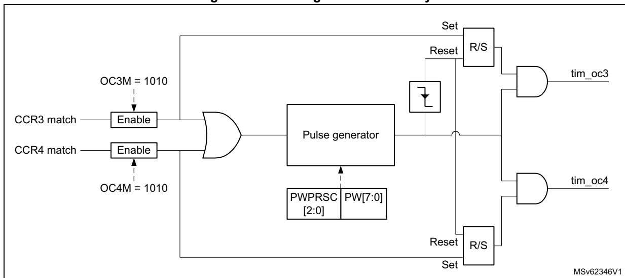
Figure 637. Pulse generator circuitry
