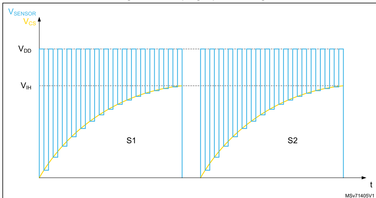
Figure 447. Sampling capacitor voltage variation
