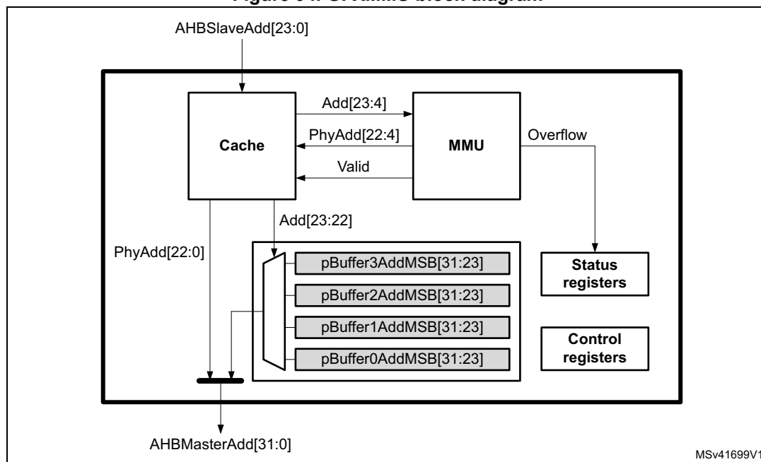
Figure 94. GFXMMU block diagram
