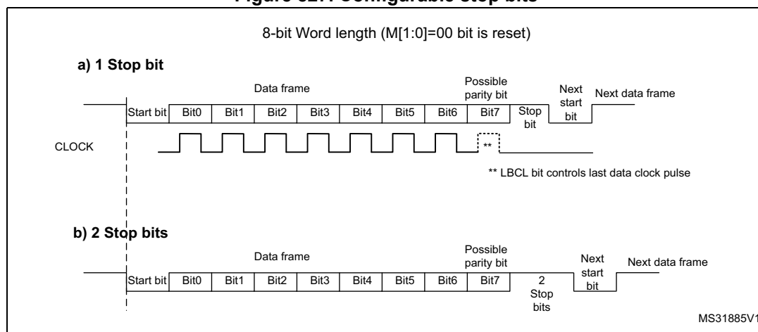
Figure 827. Configurable stop bits
