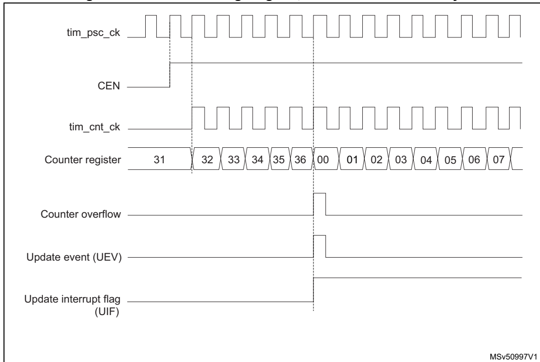
Figure 506. Counter timing diagram, internal clock divided by 1
