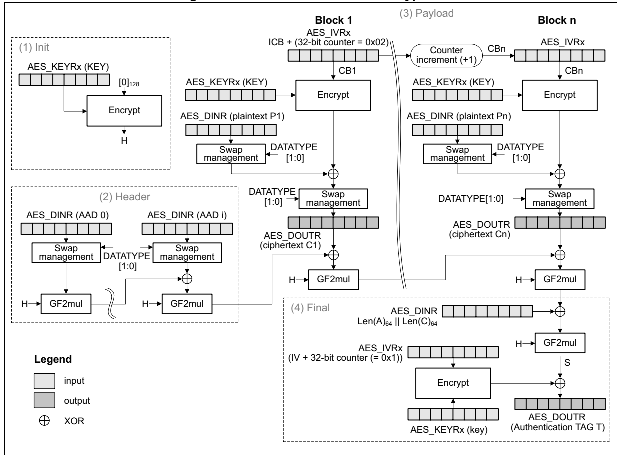
Figure 471. GCM authenticated encryption
