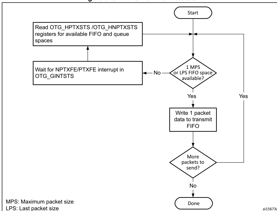
Figure 918. Transmit FIFO write task
