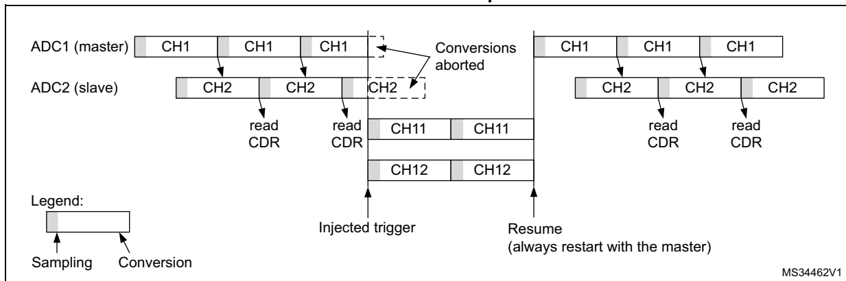
Figure 265. Two Interleaved channels (CH1, CH2) with injected sequence CH11, CH12 - case 2: Slave interrupted first
