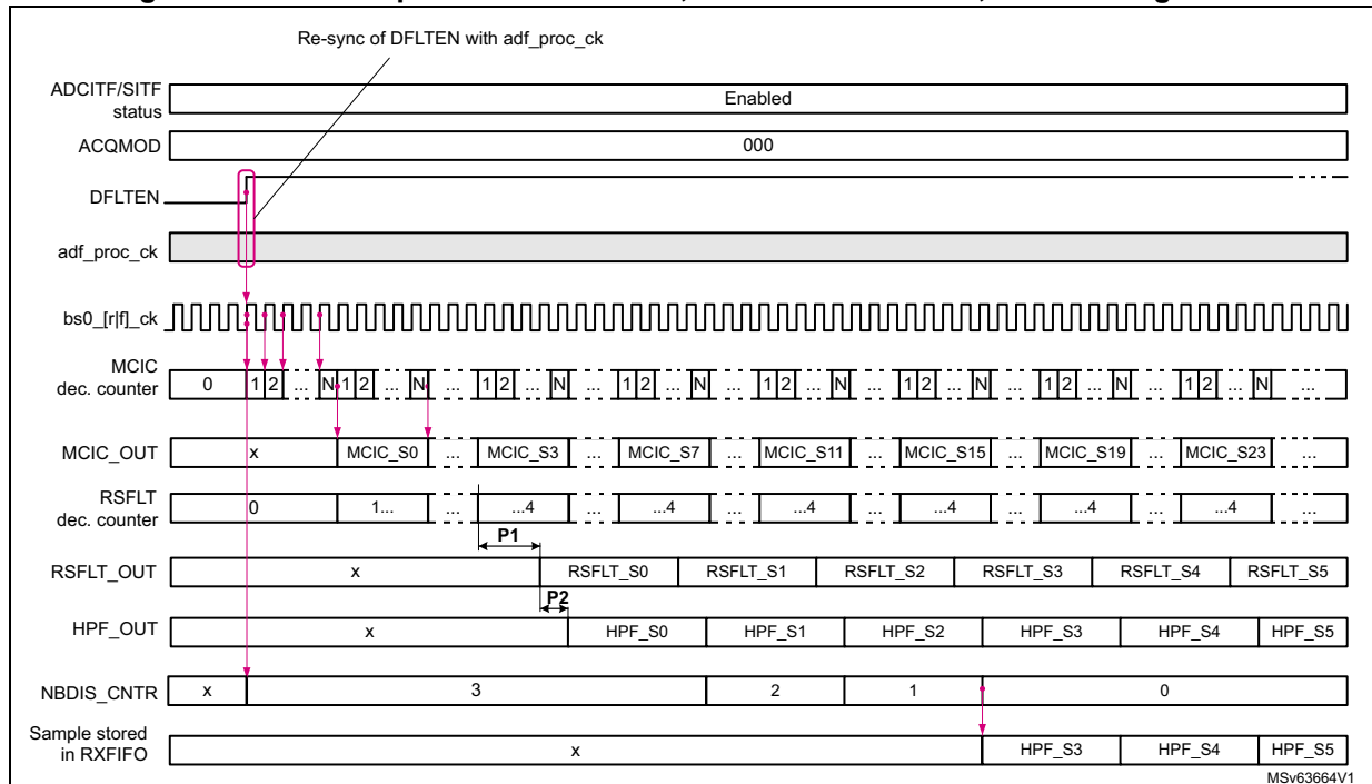
Figure 372. Start sequence with DFLTEN, in continuous mode, audio configuration
