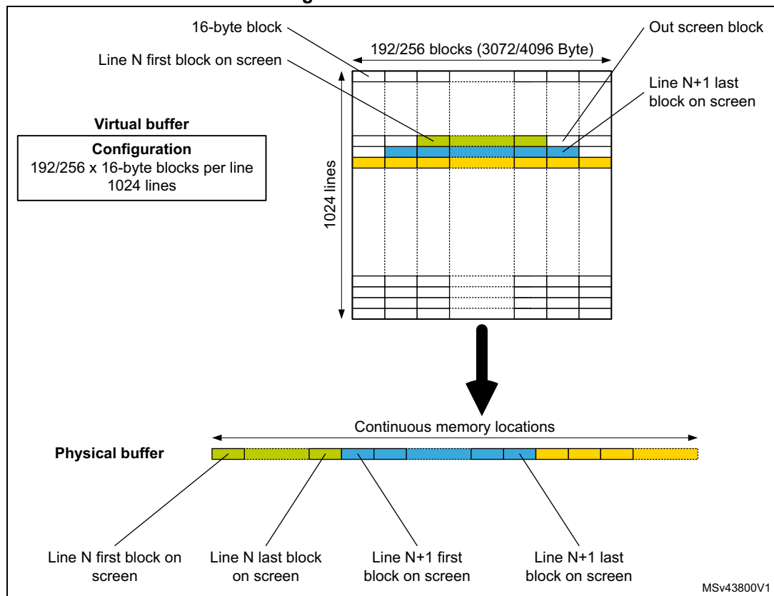
Figure 95. Virtual buffer
