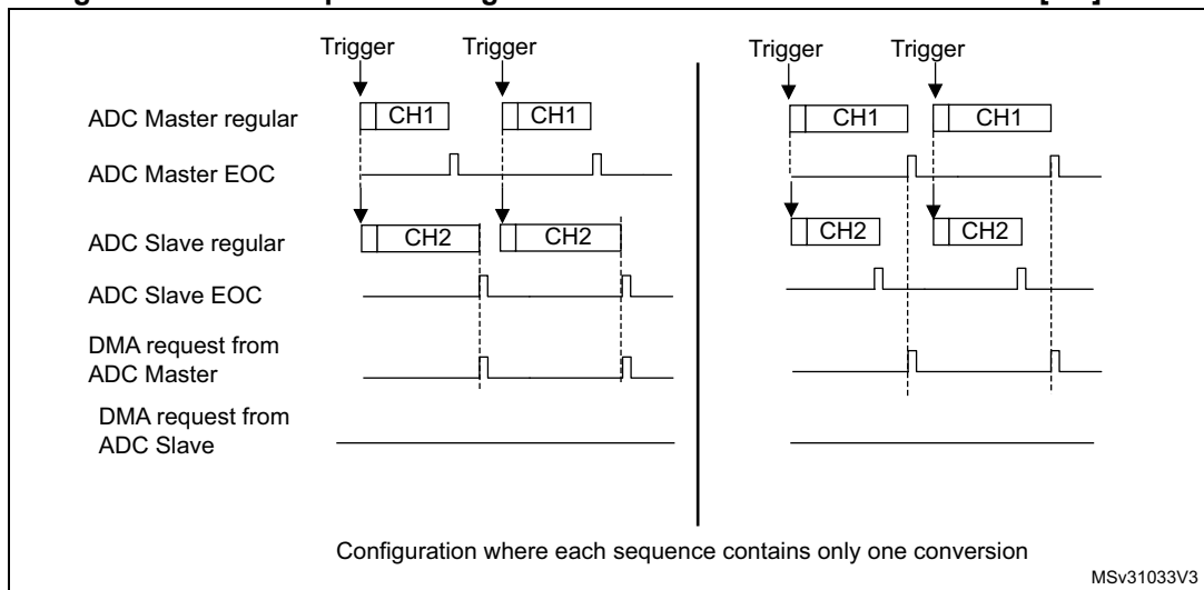
Figure 267. DMA requests in regular simultaneous mode when DAMDF[1:0] = 10
