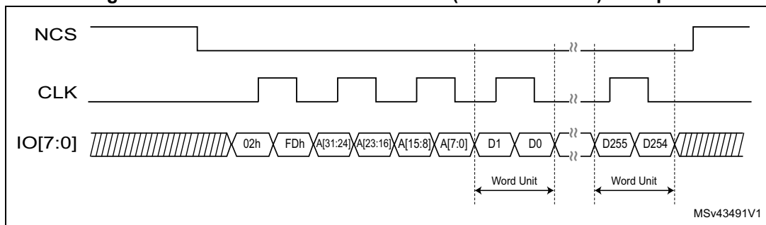
Figure 148. DTR write in octal-SPI mode (Macronix mode) example
