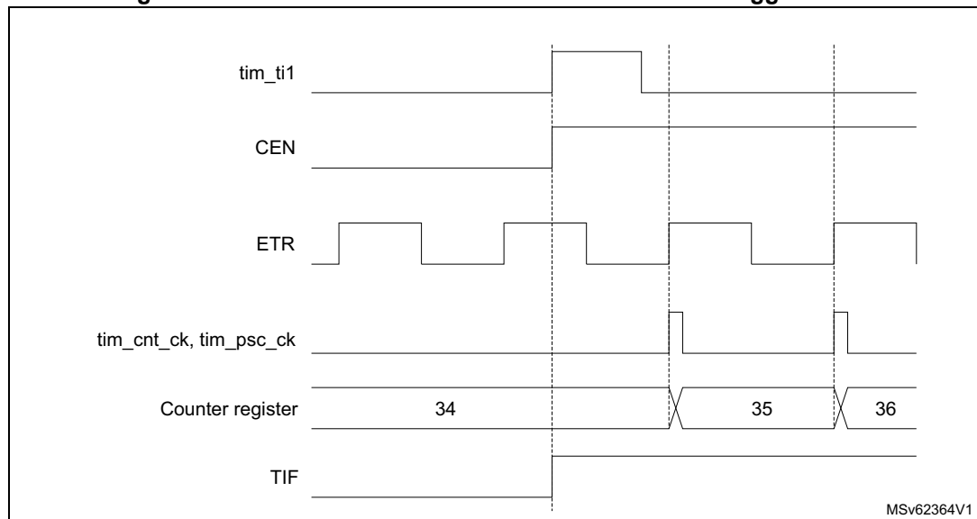
Figure 592. Control circuit in external clock mode 2 + trigger mode
