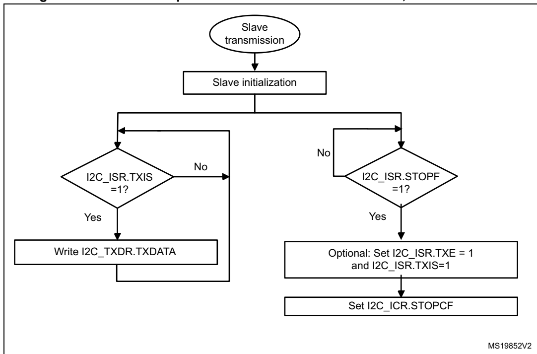
Figure 778. Transfer sequence flow for I2C slave transmitter, NOSTRETCH = 1
