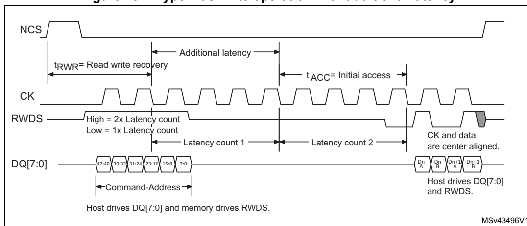
Figure 152. HyperBus write operation with additional latency
