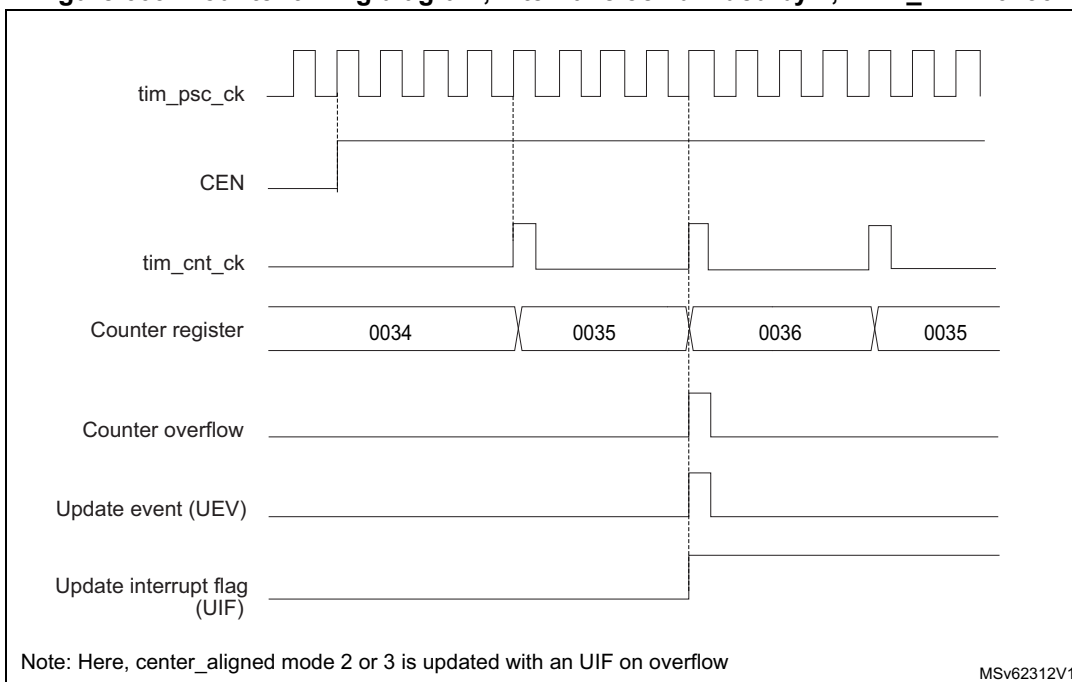
Figure 609. Counter timing diagram, internal clock divided by 4, TIMx_ARR=0x36
