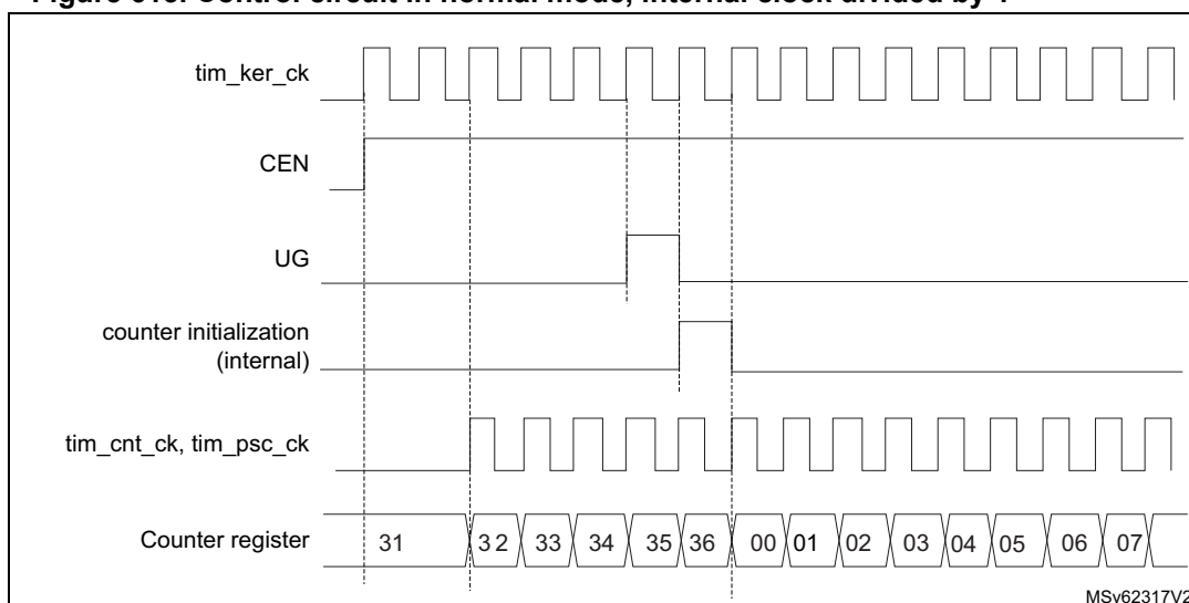
Figure 613. Control circuit in normal mode, internal clock divided by 1
