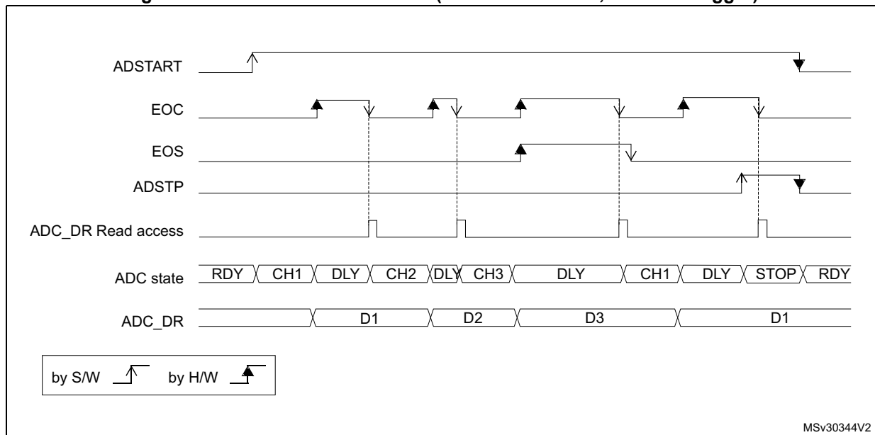
Figure 287. Wait conversion mode (continuous mode, software trigger)
