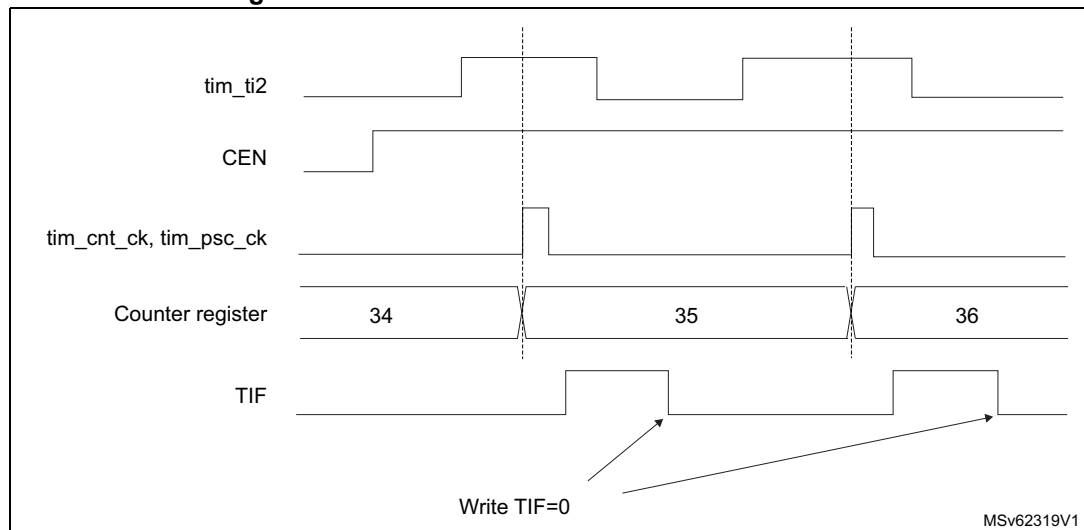
Figure 527. Control circuit in external clock mode 1
