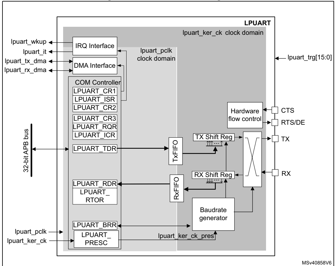
Figure 825. LPUART block diagram
