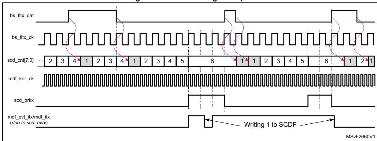
Figure 328. SCD timing example
