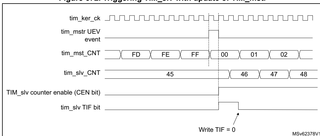
Figure 672. Triggering TIM_slv with update of TIM_mstr
