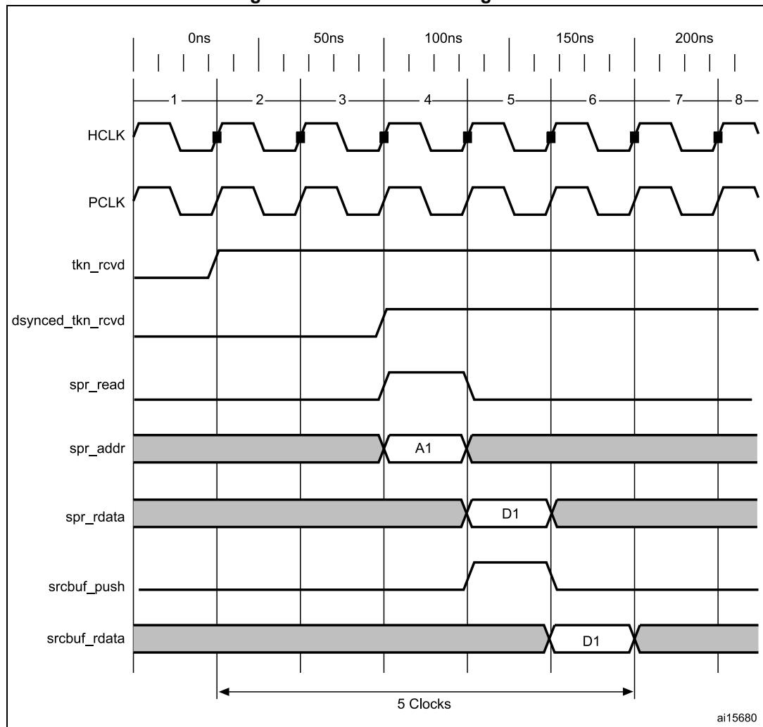
Figure 935. TRDT max timing case
