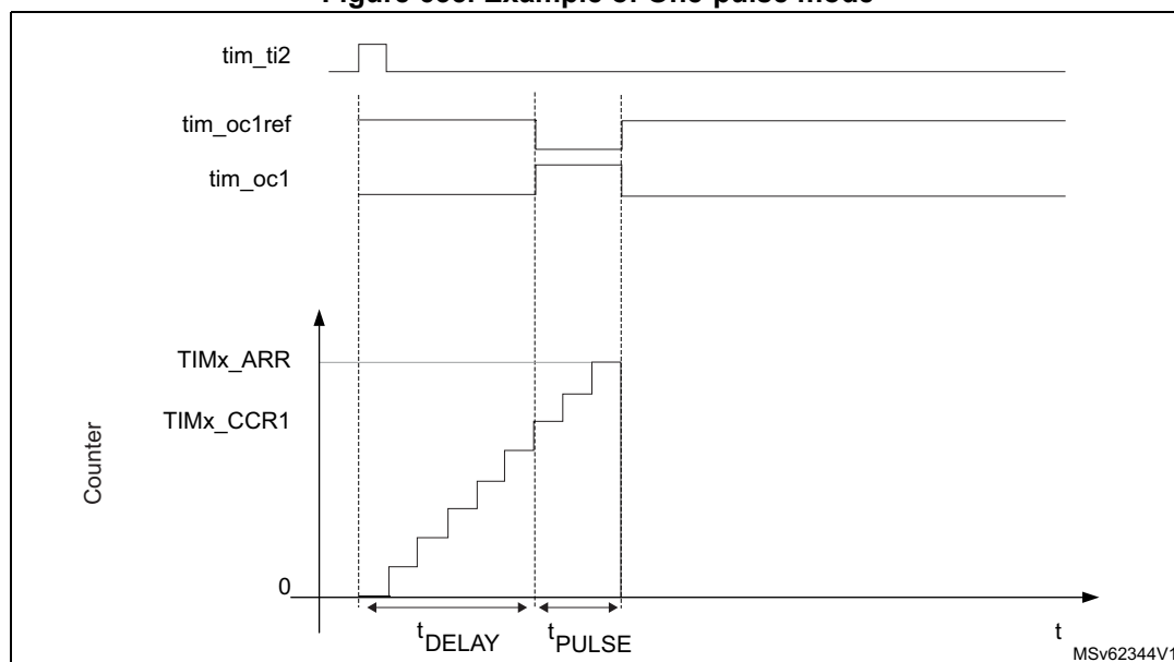
Figure 635. Example of One-pulse mode
