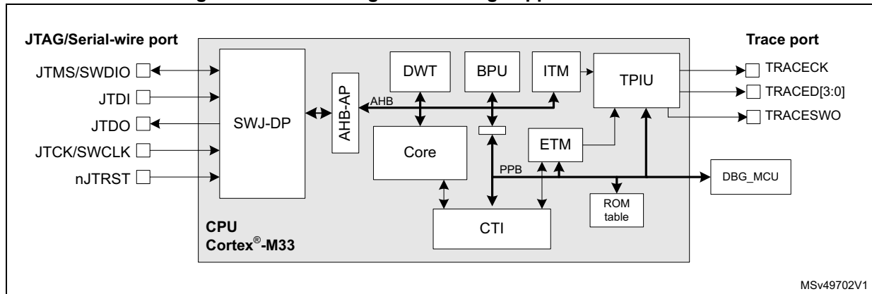
Figure 947. Block diagram of debug support infrastructure
