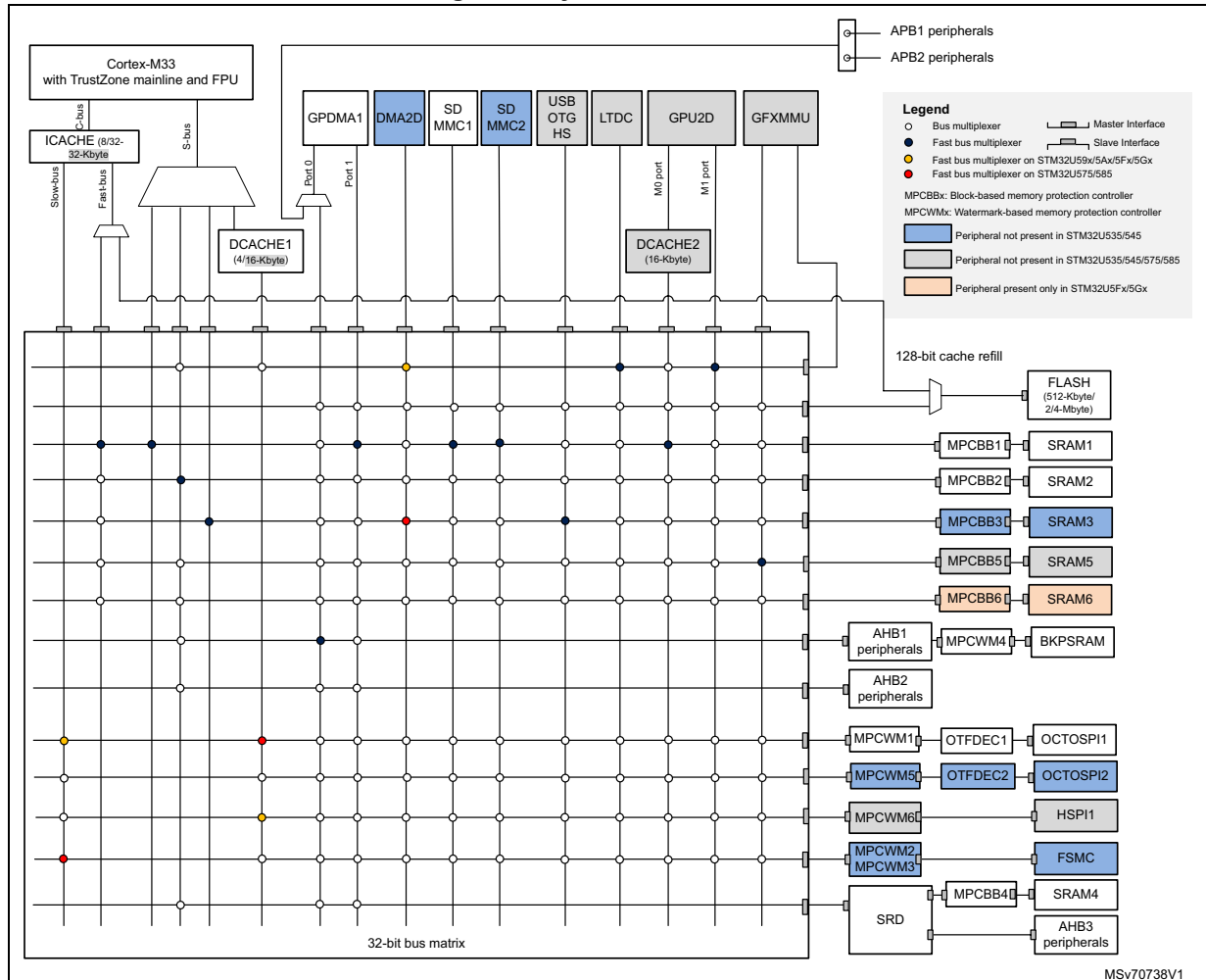
Figure 1. System architecture
