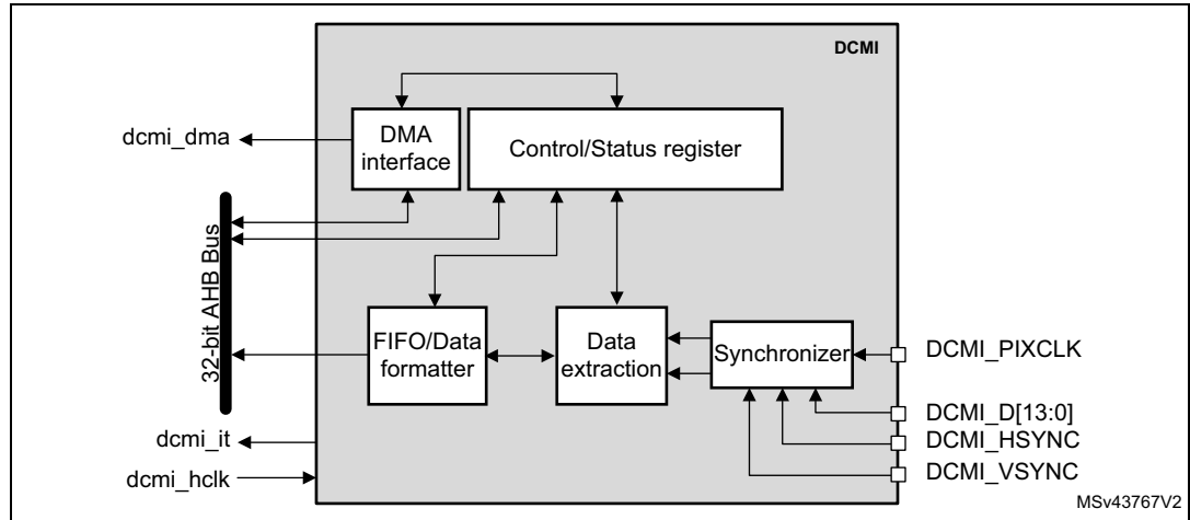
Figure 386. DCMI block diagram
