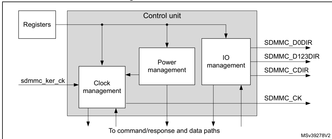
Figure 187. Control unit
