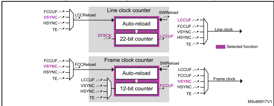
Figure 753. Prescaling when external VSYNC only
