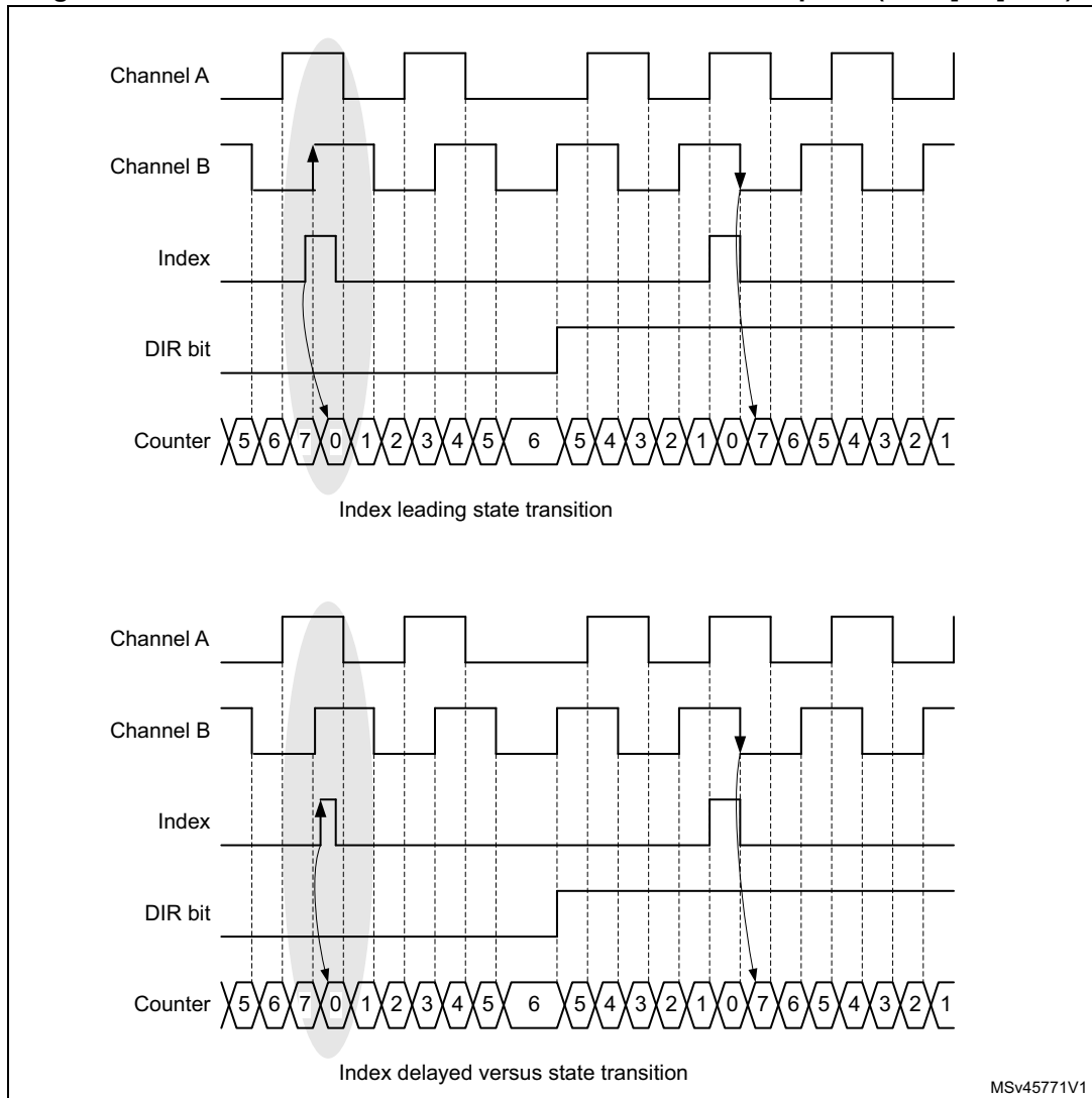
Figure 575. Encoder mode behavior in case of narrow index pulse (IPOS[1:0] = 11)
