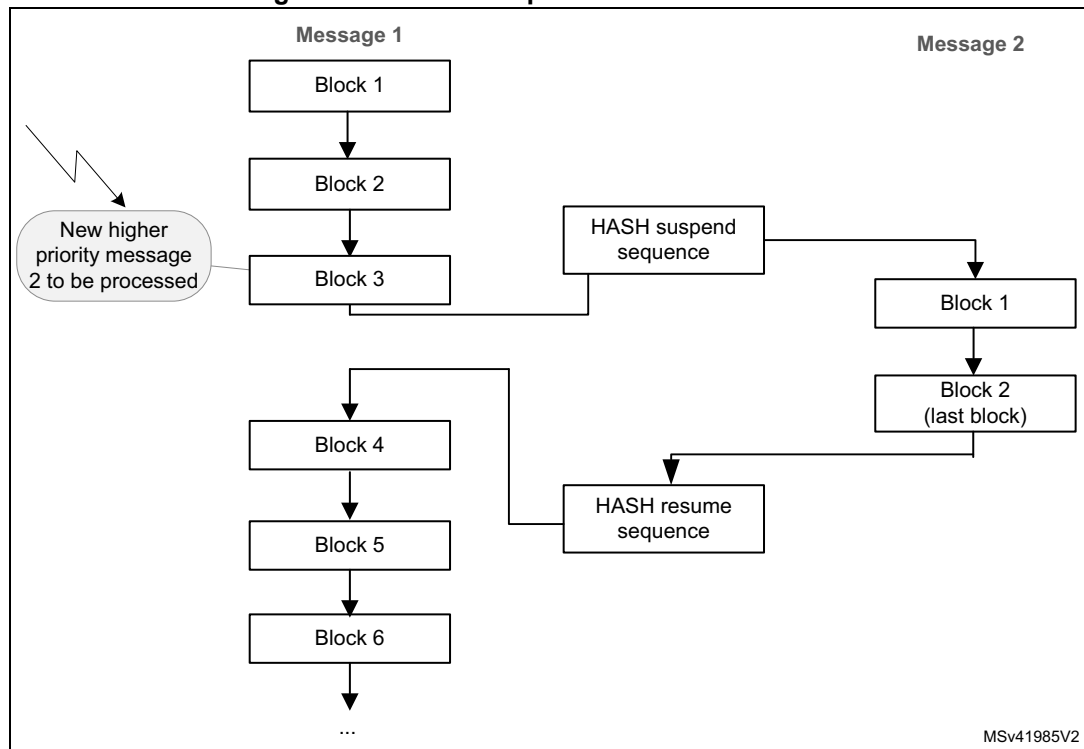
Figure 497. HASH suspend/resume mechanism
