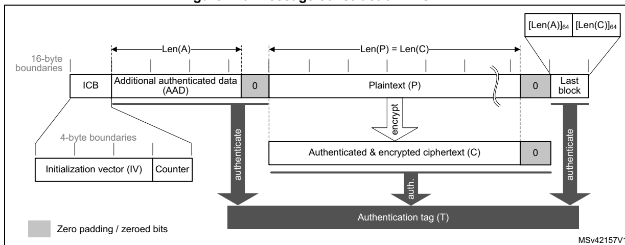
Figure 470. Message construction in GCM
