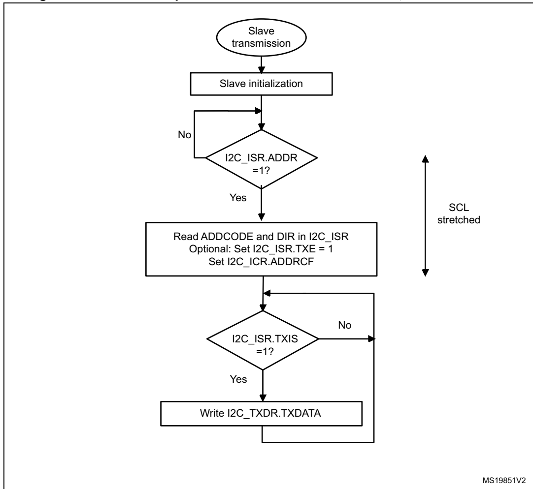
Figure 777. Transfer sequence flow for I2C slave transmitter, NOSTRETCH = 0
