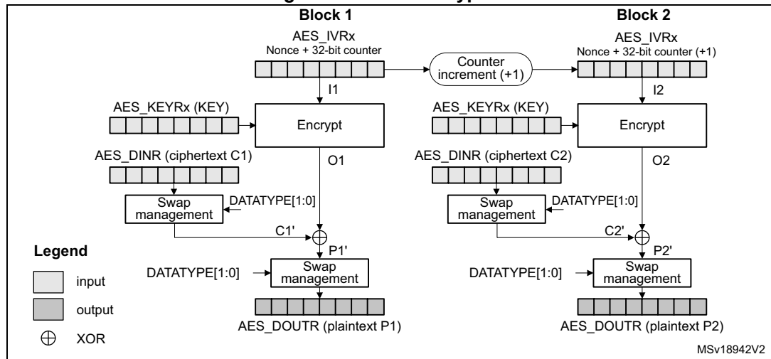
Figure 469. CTR decryption
