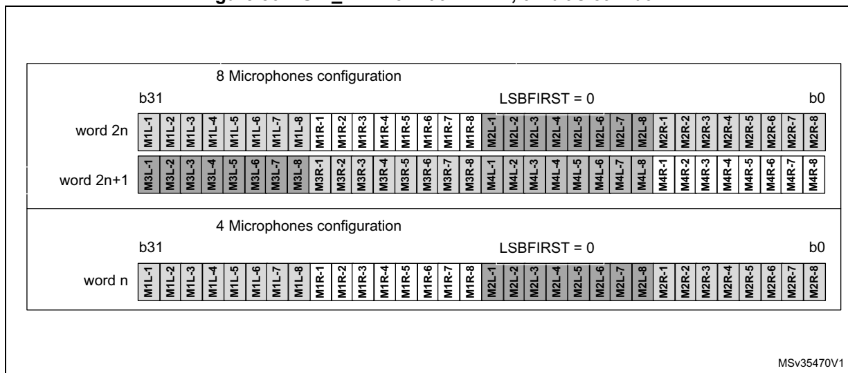
Figure 861. SAI_ADR format in TDM, 32-bit slot width
