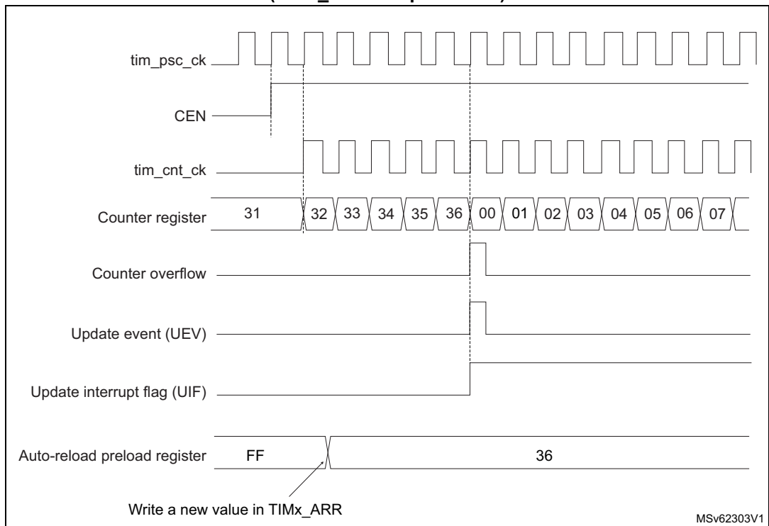
Figure 683. Counter timing diagram, update event when ARPE=0 (TIMx_ARR not preloaded)
