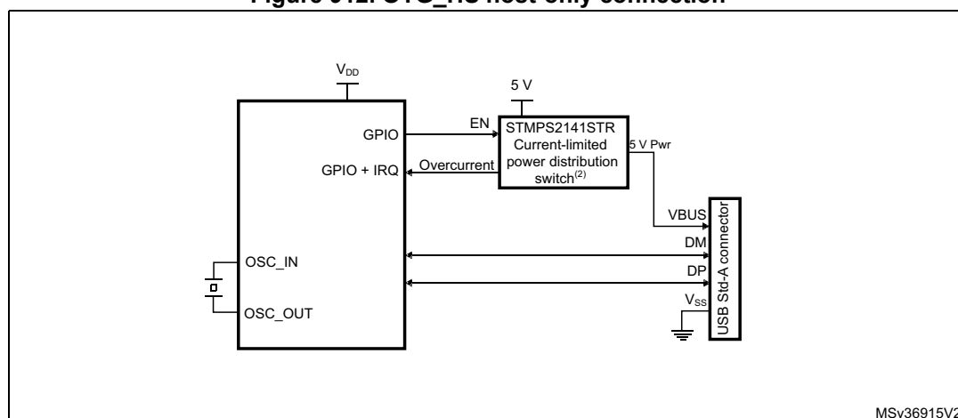
Figure 912. OTG_HS host-only connection
