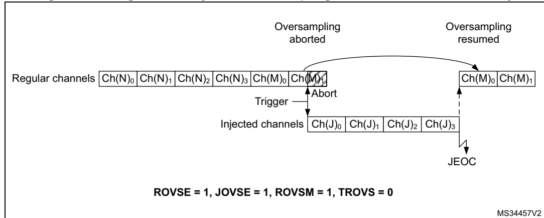
Figure 250. Regular and injected oversampling modes used simultaneously
