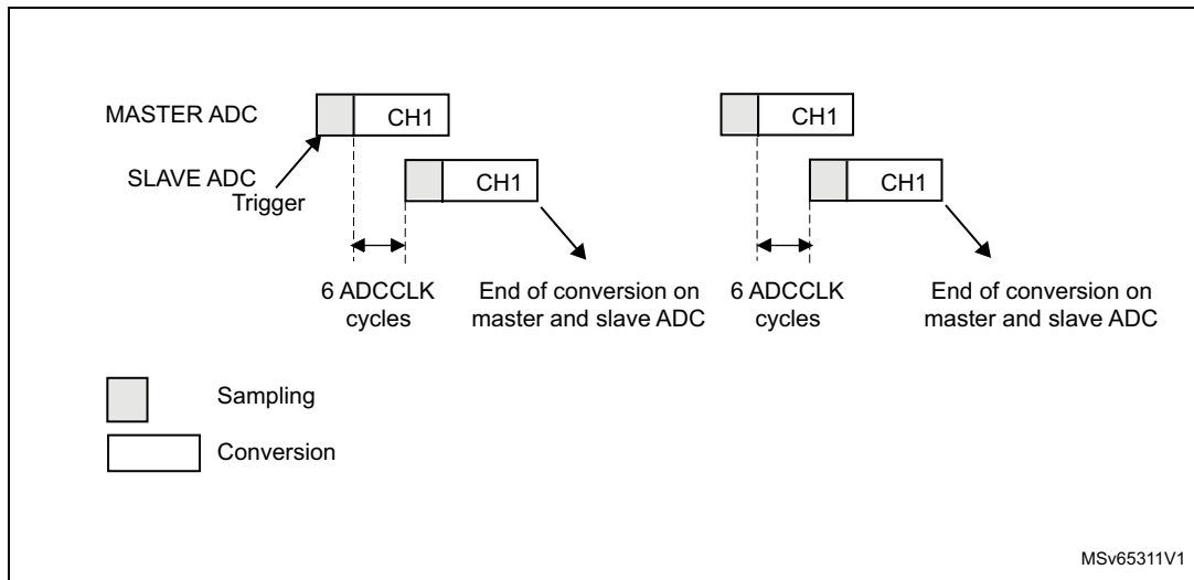
Figure 257. Interleaved mode on one channel in single conversion mode: dual ADC mode
