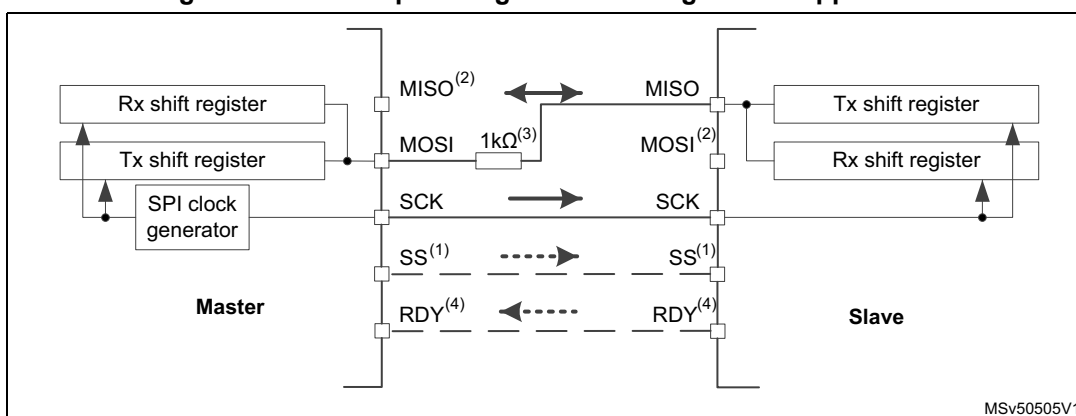
Figure 839. Half-duplex single master/ single slave application
