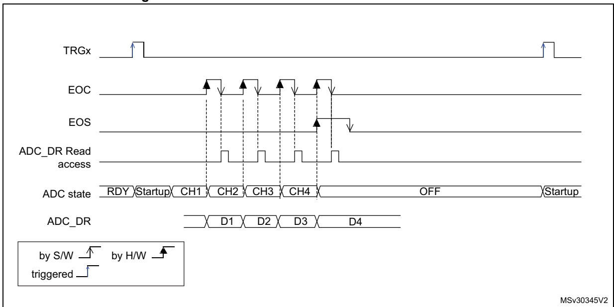
Figure 289. ADC behavior with WAIT = 0 and AUTOFF = 1
