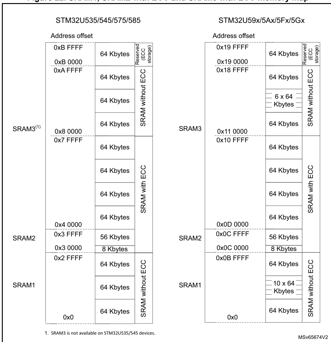
Figure 22. SRAM1, SRAM2 with ECC and SRAM3 with ECC memory map
