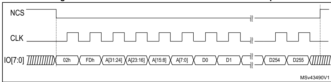
Figure 147. SDR write command in octo-SPI mode example
