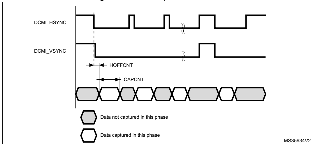
Figure 392. Data capture waveforms
