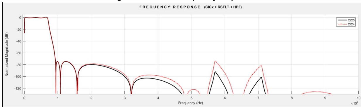
Figure 352. Global frequency response
