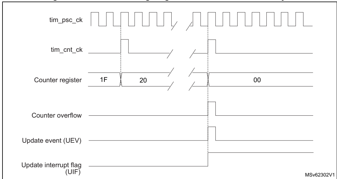
Figure 683. Counter timing diagram, update event when ARPE=0 (TIMx_ARR not preloaded)
