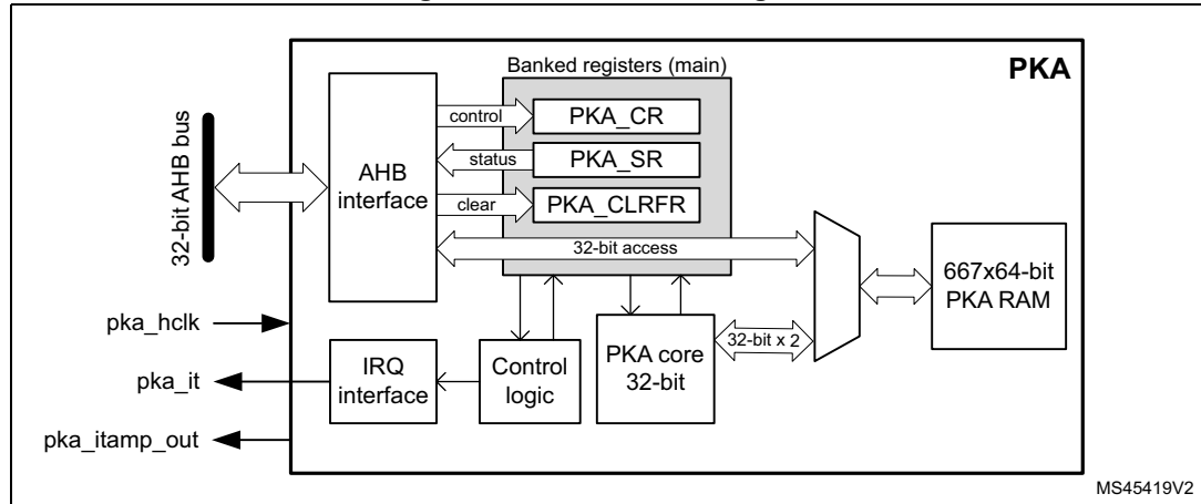
Figure 502. PKA block diagram
