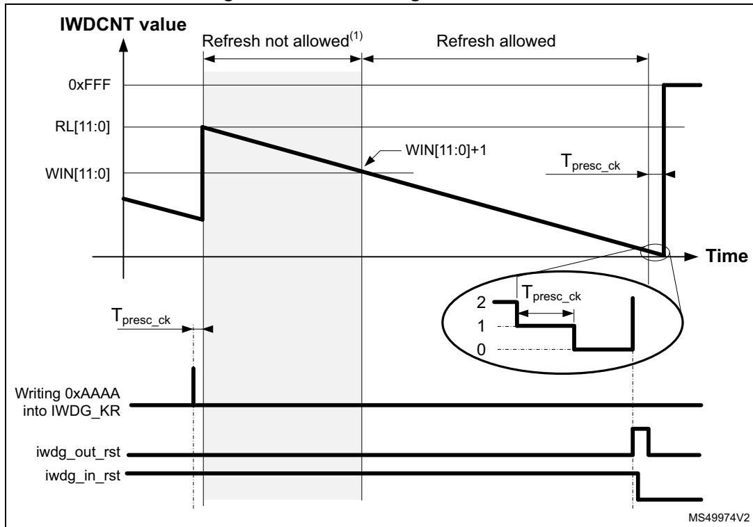
Figure 761. Reset timing due to timeout
