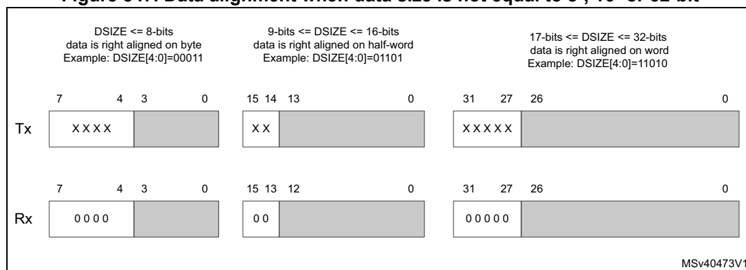
Figure 847. Data alignment when data size is not equal to 8-, 16- or 32-bit
