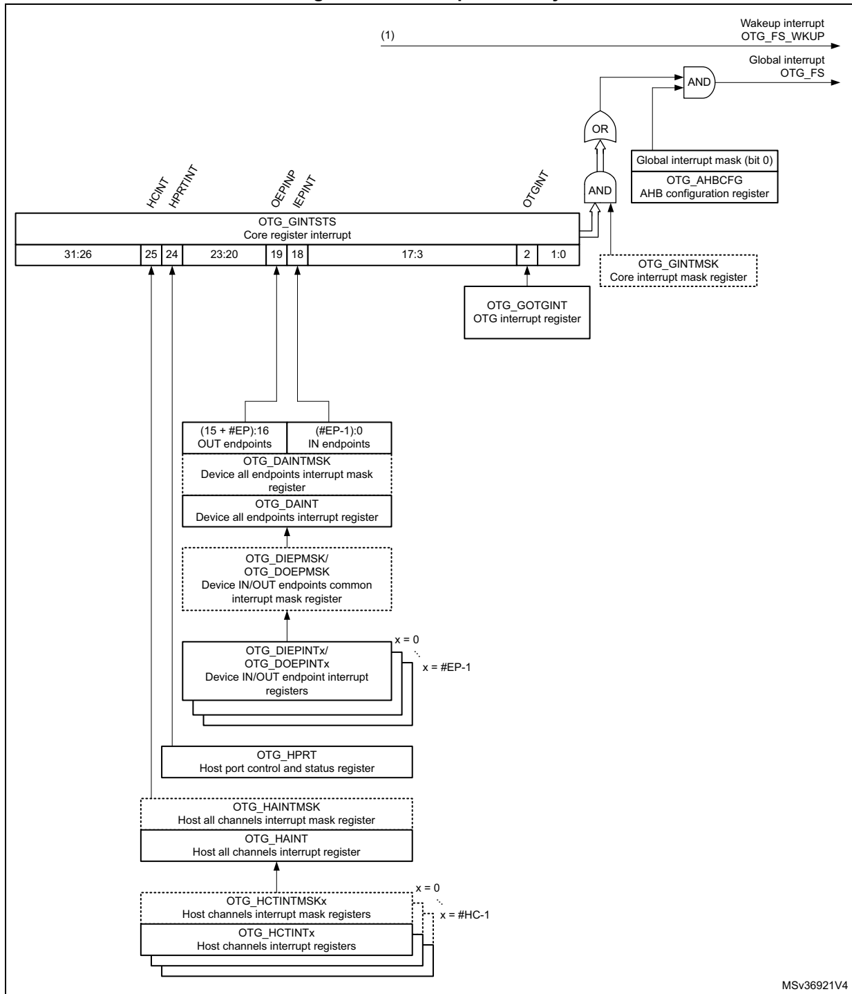
Figure 892. Interrupt hierarchy
