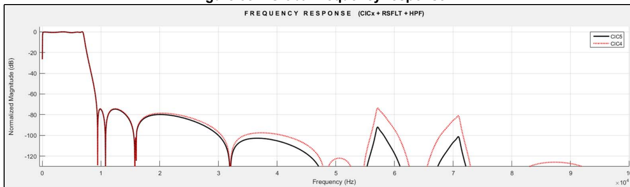
Figure 381. Global frequency response
