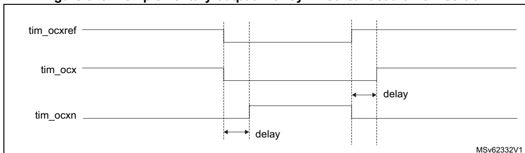
Figure 546. Complementary output with symmetrical dead-time insertion
