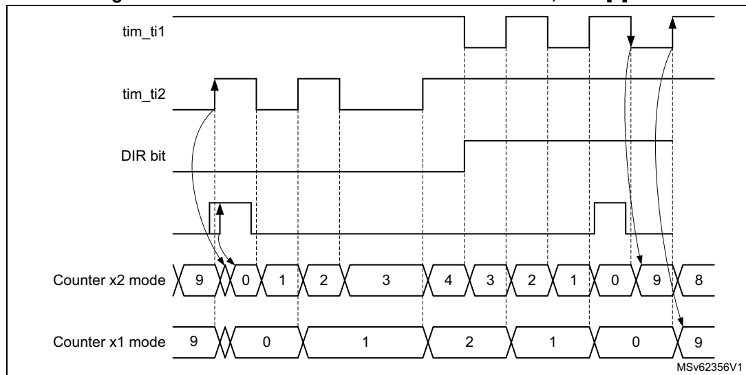
Figure 582. Index behavior in directional clock mode, IPOS[0] = 1
