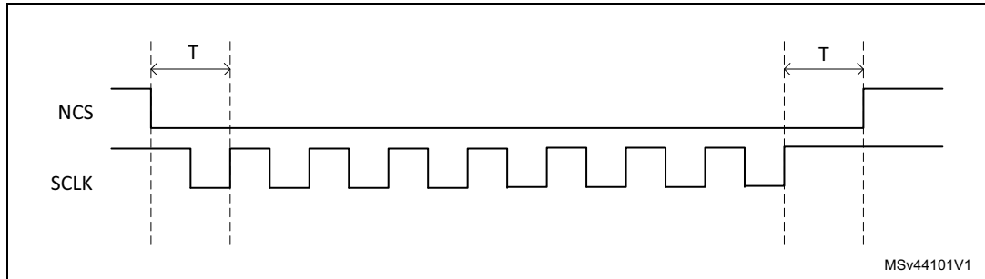
Figure 177. NCS when CKMODE = 1 in SDR mode (T = CLK period)
