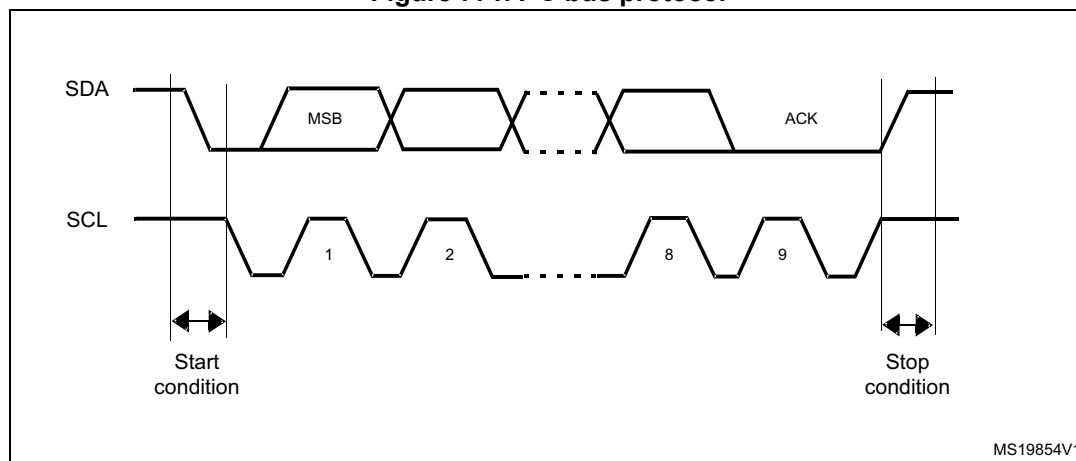
Figure 771. I 2 C bus protocol
