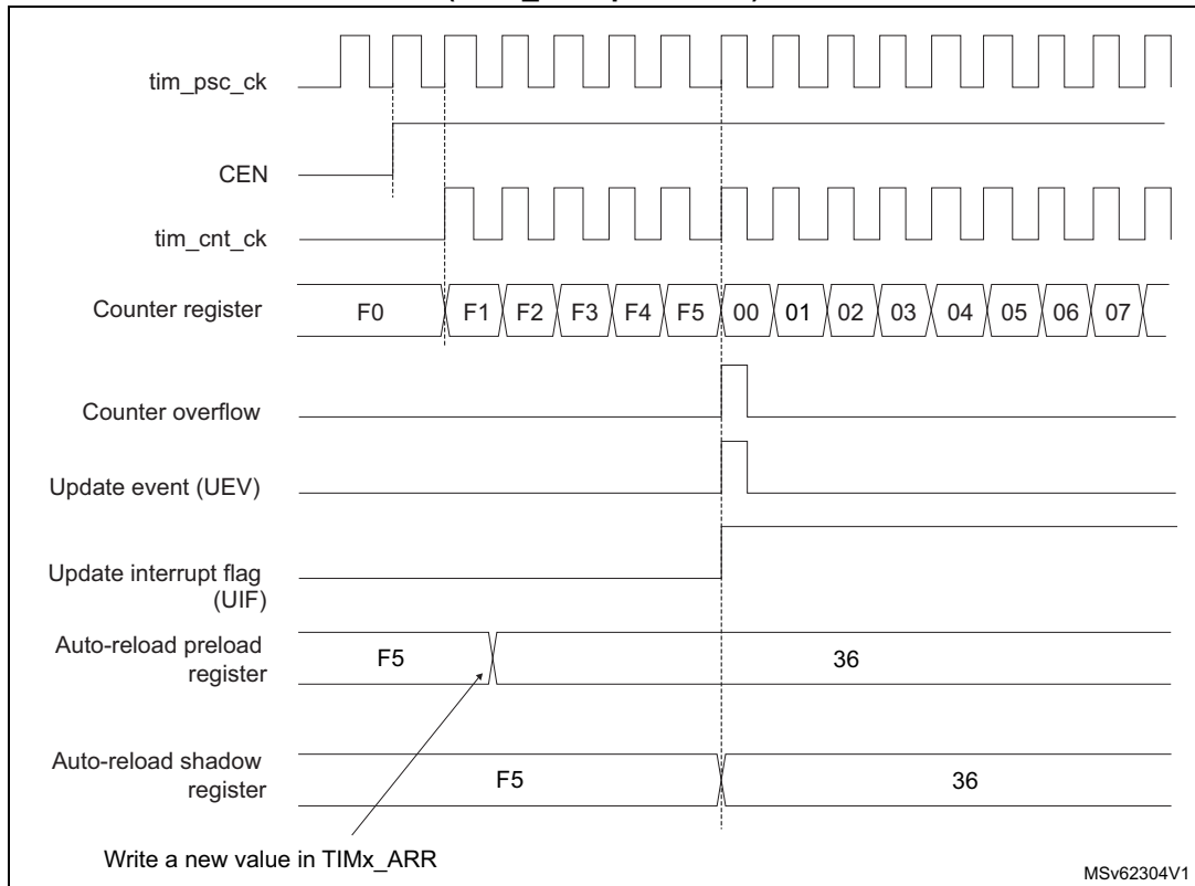
Figure 511. Counter timing diagram, update event when ARPE=1 (TIMx_ARR preloaded)
