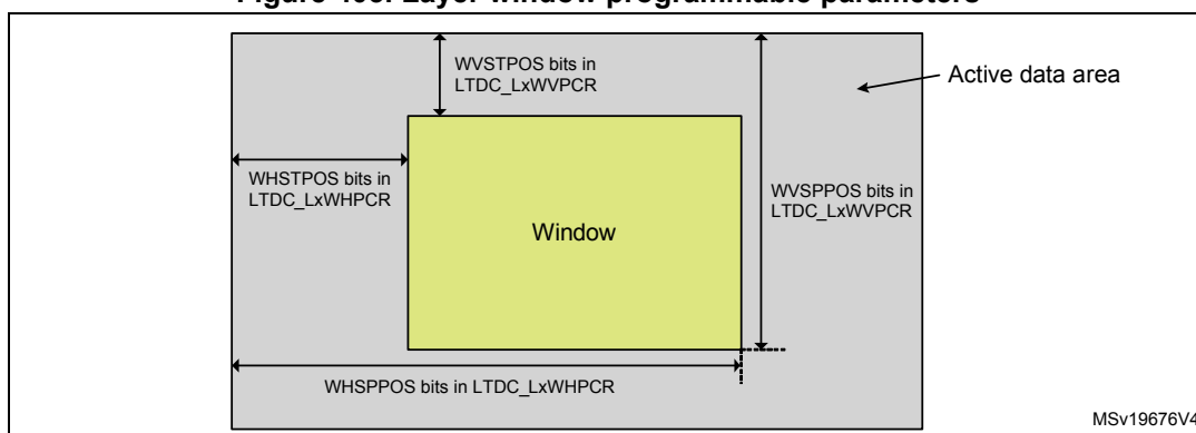
Figure 403. Layer window programmable parameters
