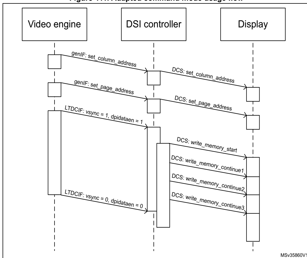
Figure 411. Adapted command mode usage flow
