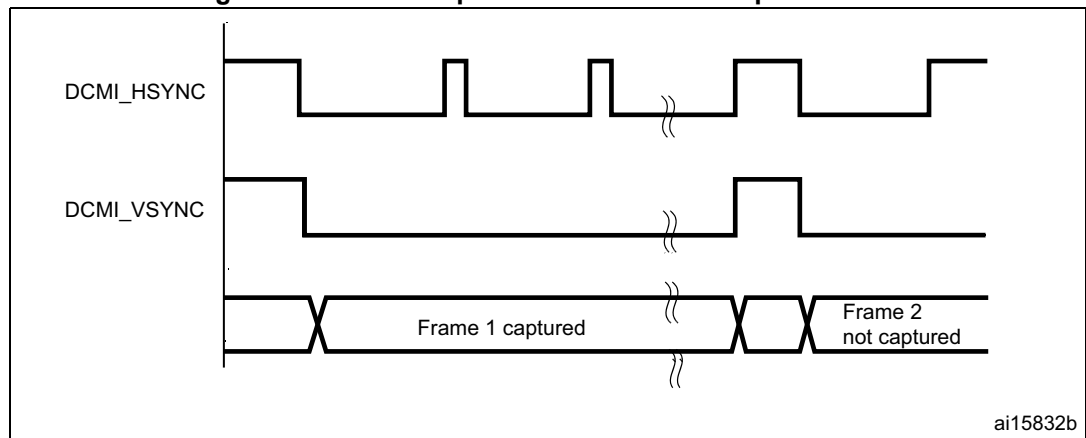
Figure 389. Frame capture waveforms in snapshot mode
