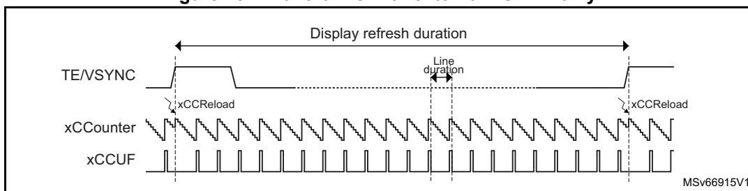
Figure 751. Waveforms with external VSYNC only
