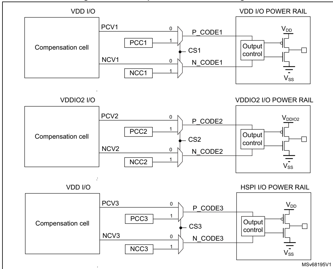
Figure 48. I/O compensation cell block diagram
