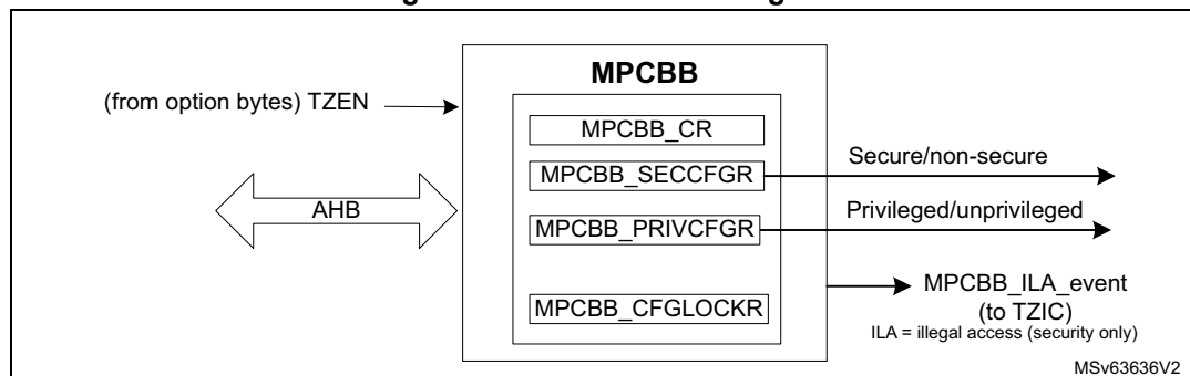
Figure 21. MPCBB block diagram
