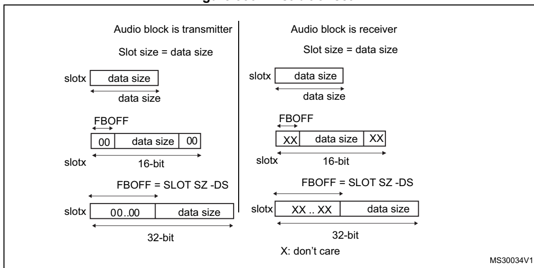
Figure 856. First bit offset
