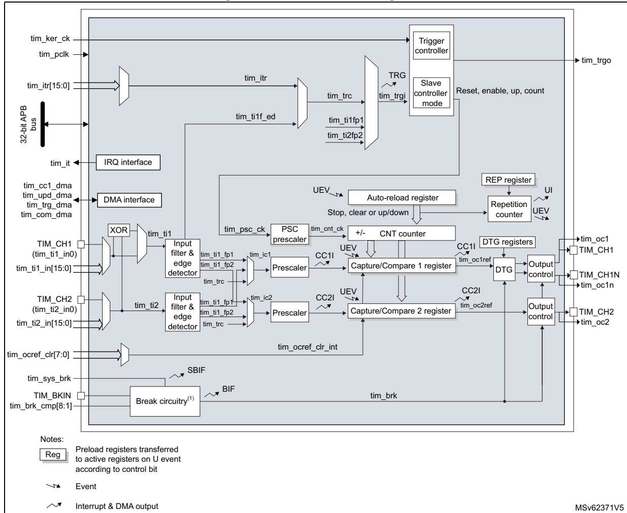
Figure 675. TIM15 block diagram
