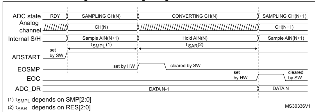
Figure 278. Analog to digital conversion time
