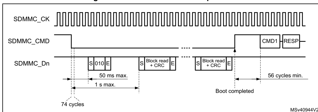
Figure 207. Normal boot mode operation
