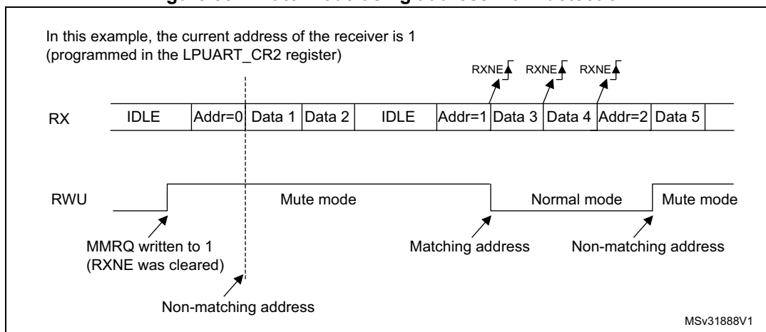
Figure 831. Mute mode using address mark detection
