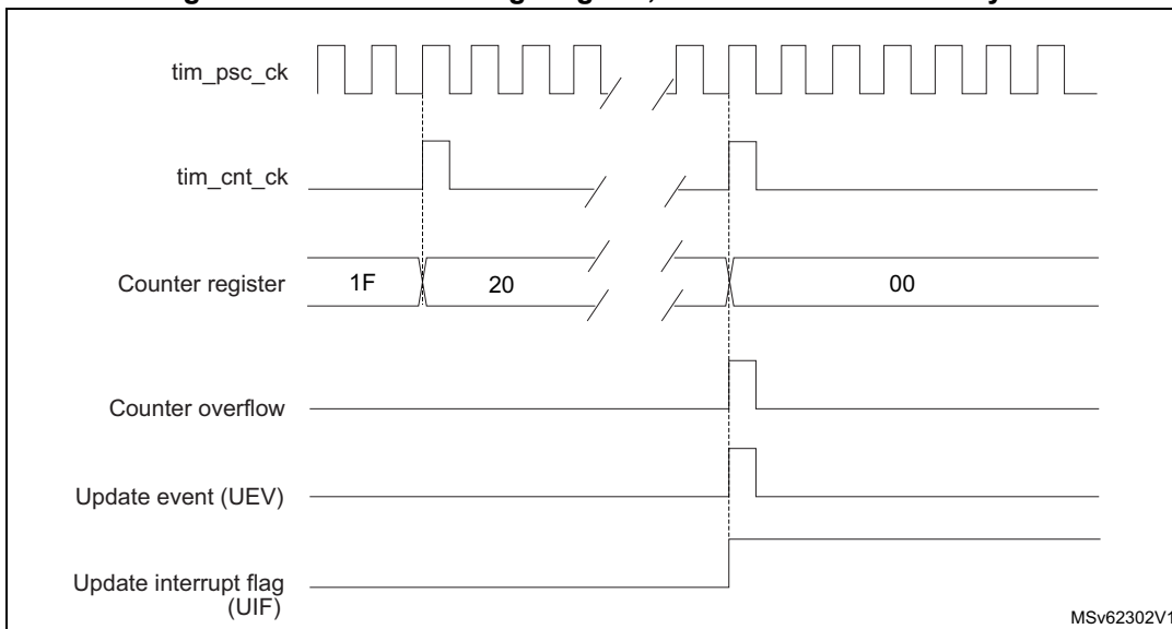
Figure 723. Counter timing diagram, internal clock divided by N
