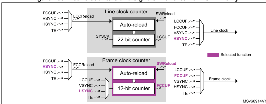
Figure 750. Active counters and signals with external HSYNC only
