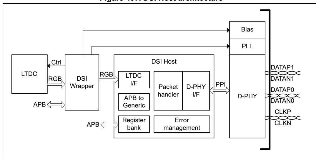
Figure 407. DSI Host architecture
