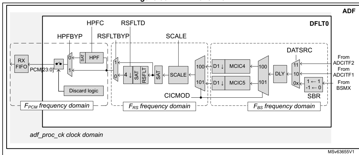
Figure 361. DFLT overview
