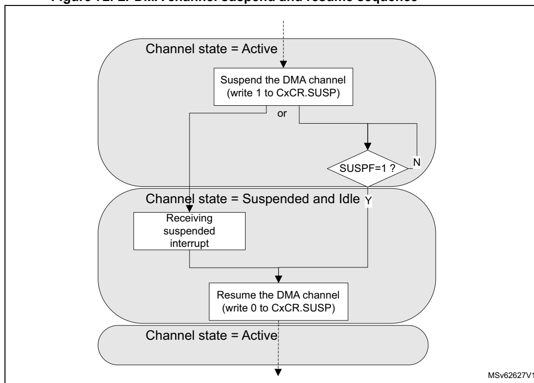
Figure 72. LPDMA channel suspend and resume sequence
