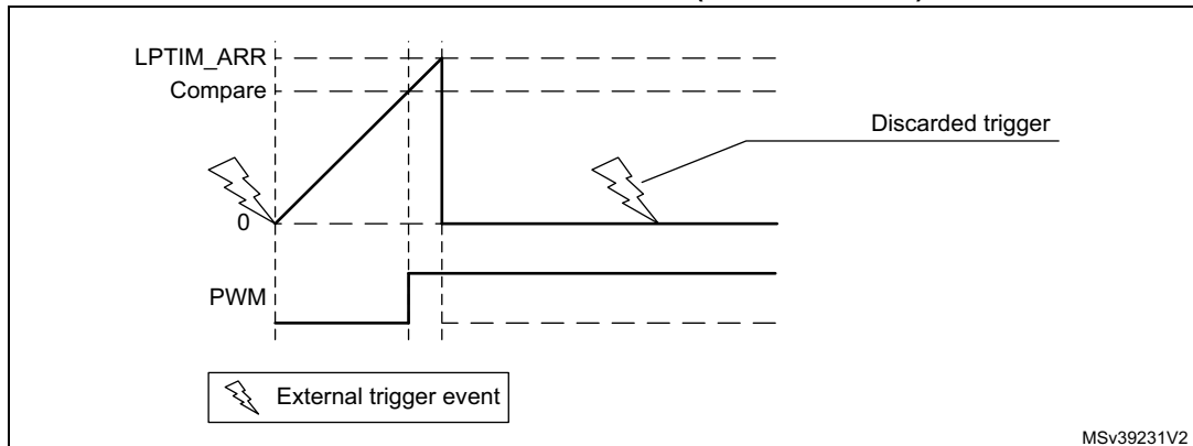
Figure 734. LPTIM output waveform, Single counting mode configuration and Set-once mode activated (WAVE bit is set)
