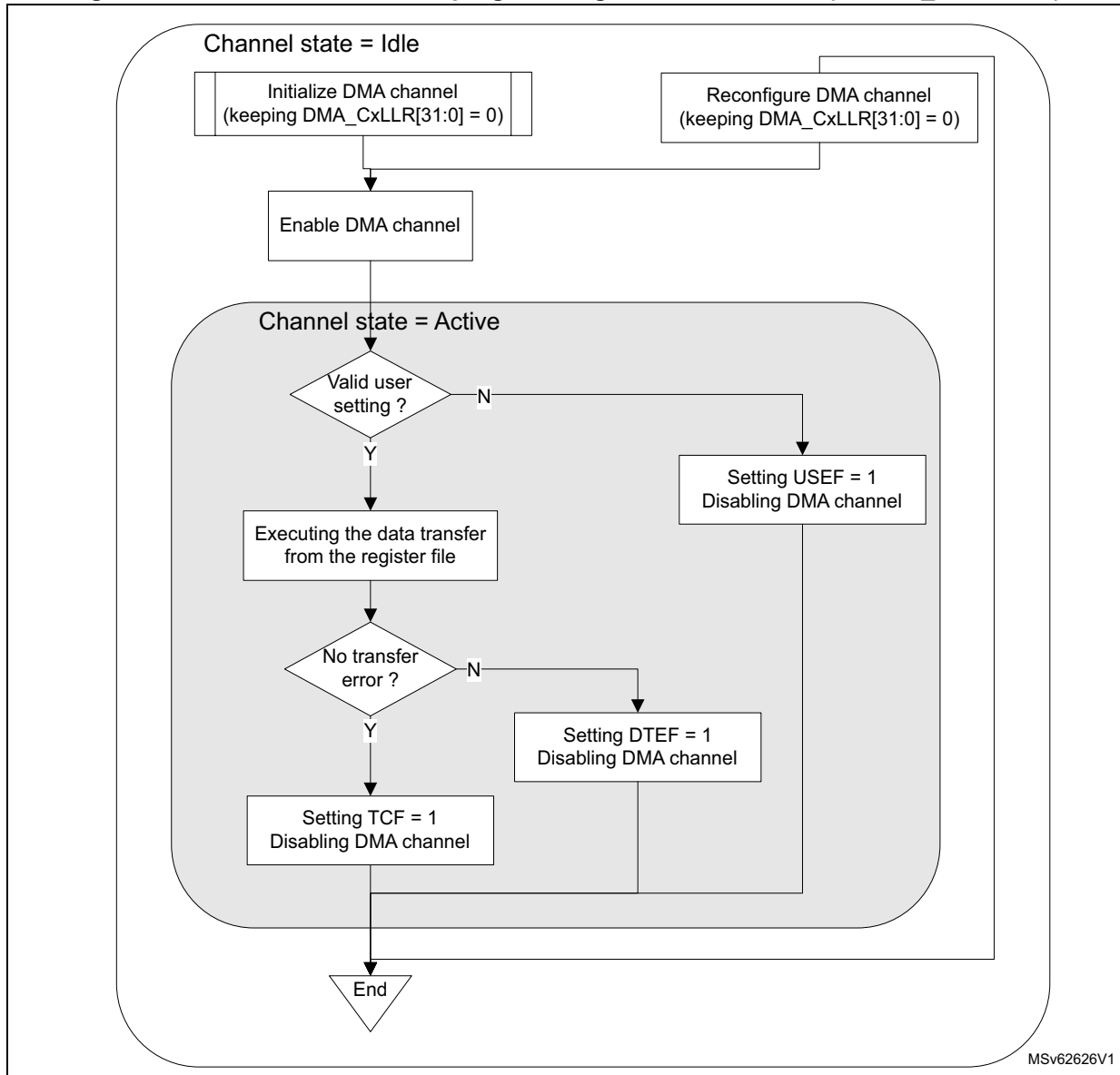
Figure 71. LPDMA channel direct programming without linked-list (LPDMA_CxLLR = 0)
