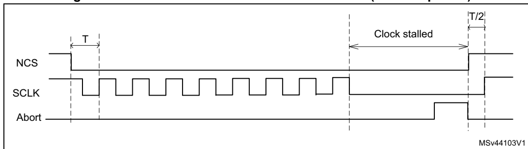
Figure 179. NCS when CKMODE =1 with an abort (T = CLK period)
