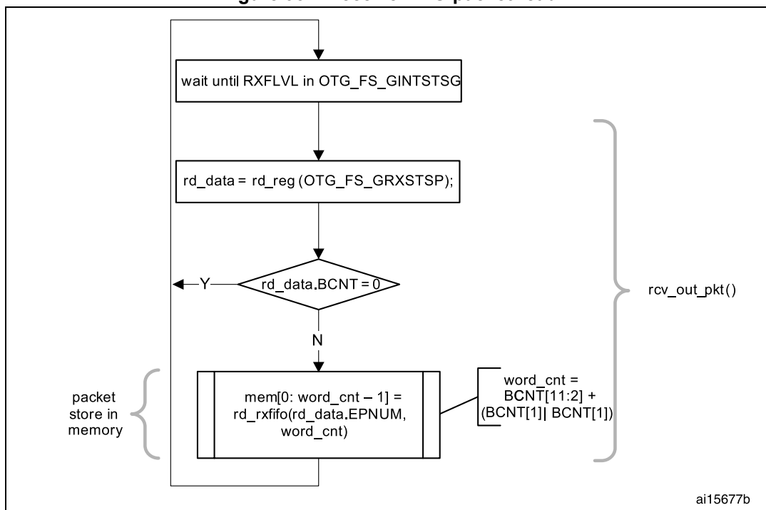
Figure 932. Receive FIFO packet read
