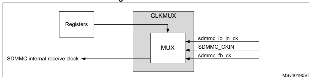
Figure 194. CLKMUX unit
