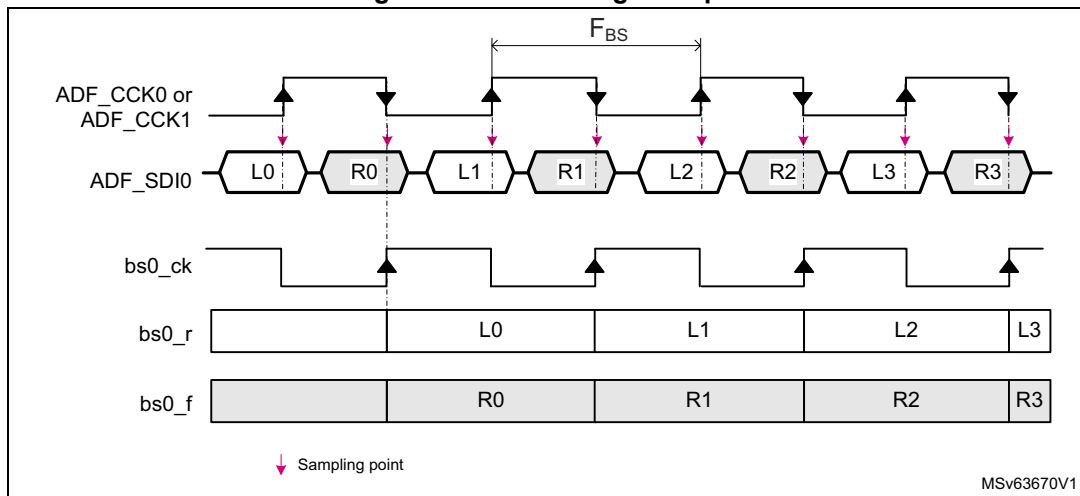
Figure 357. SPI timing example
