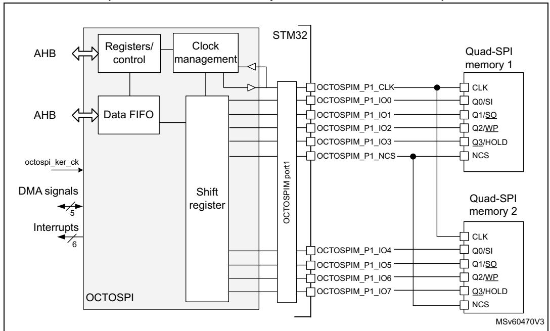
Figure 141. OCTOSPI block diagram in dual-quad configuration (for STM32U5 series except STM32U535/545 devices)
