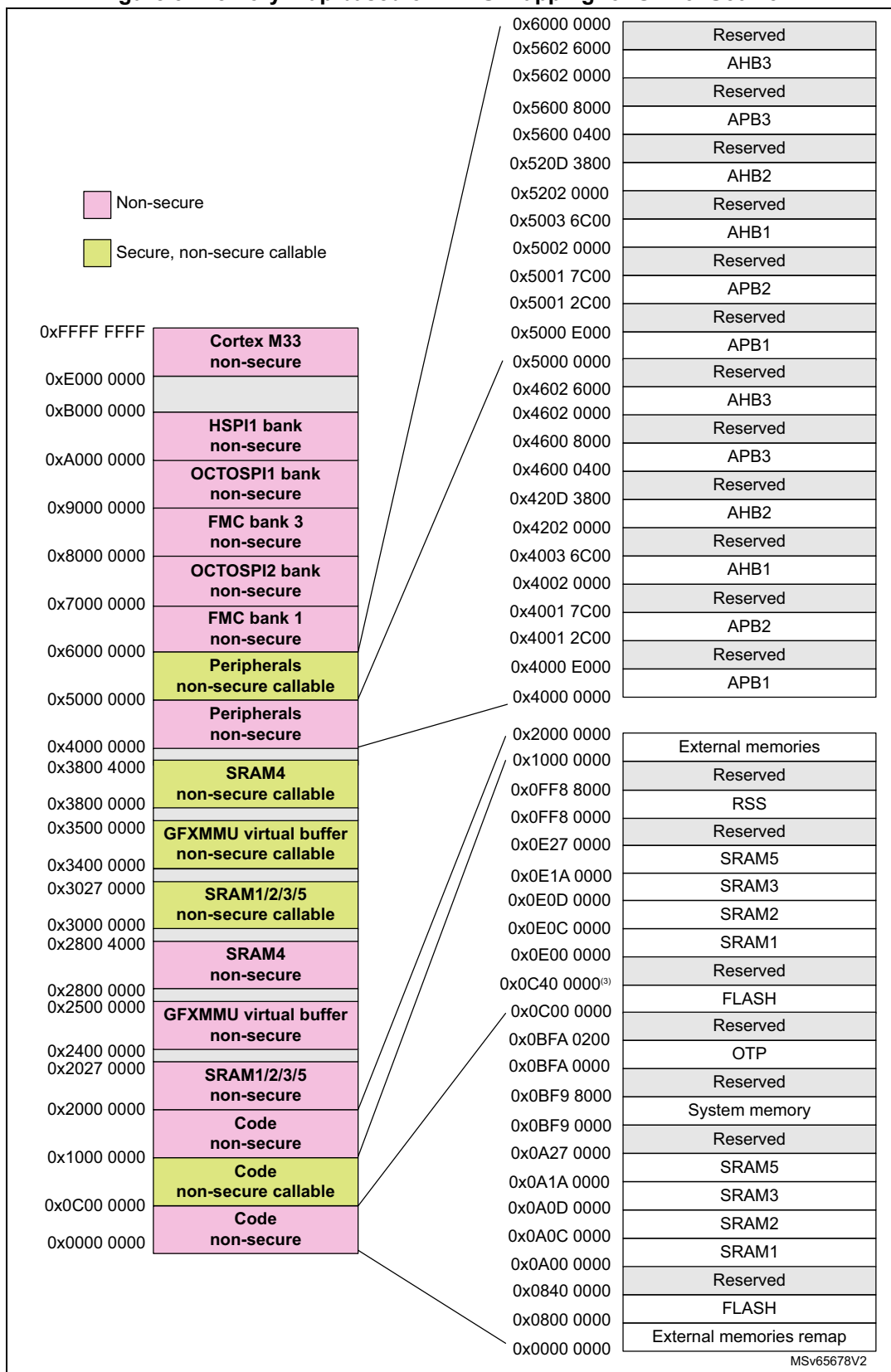
Figure 5. Memory map based on IDAU mapping for STM32U59x/5Ax
