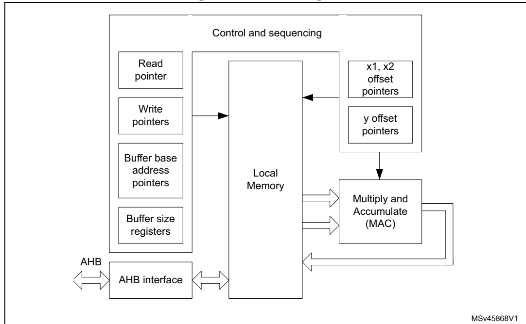
Figure 106. Block diagram
