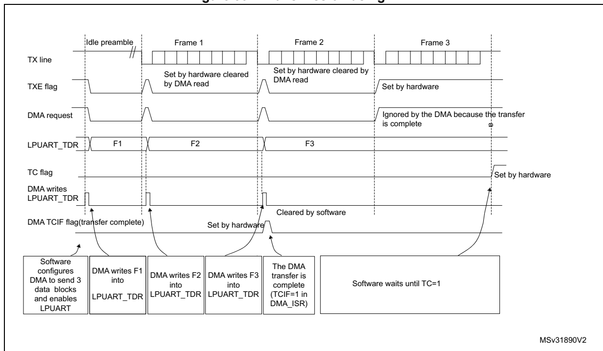
Figure 832. Transmission using DMA
