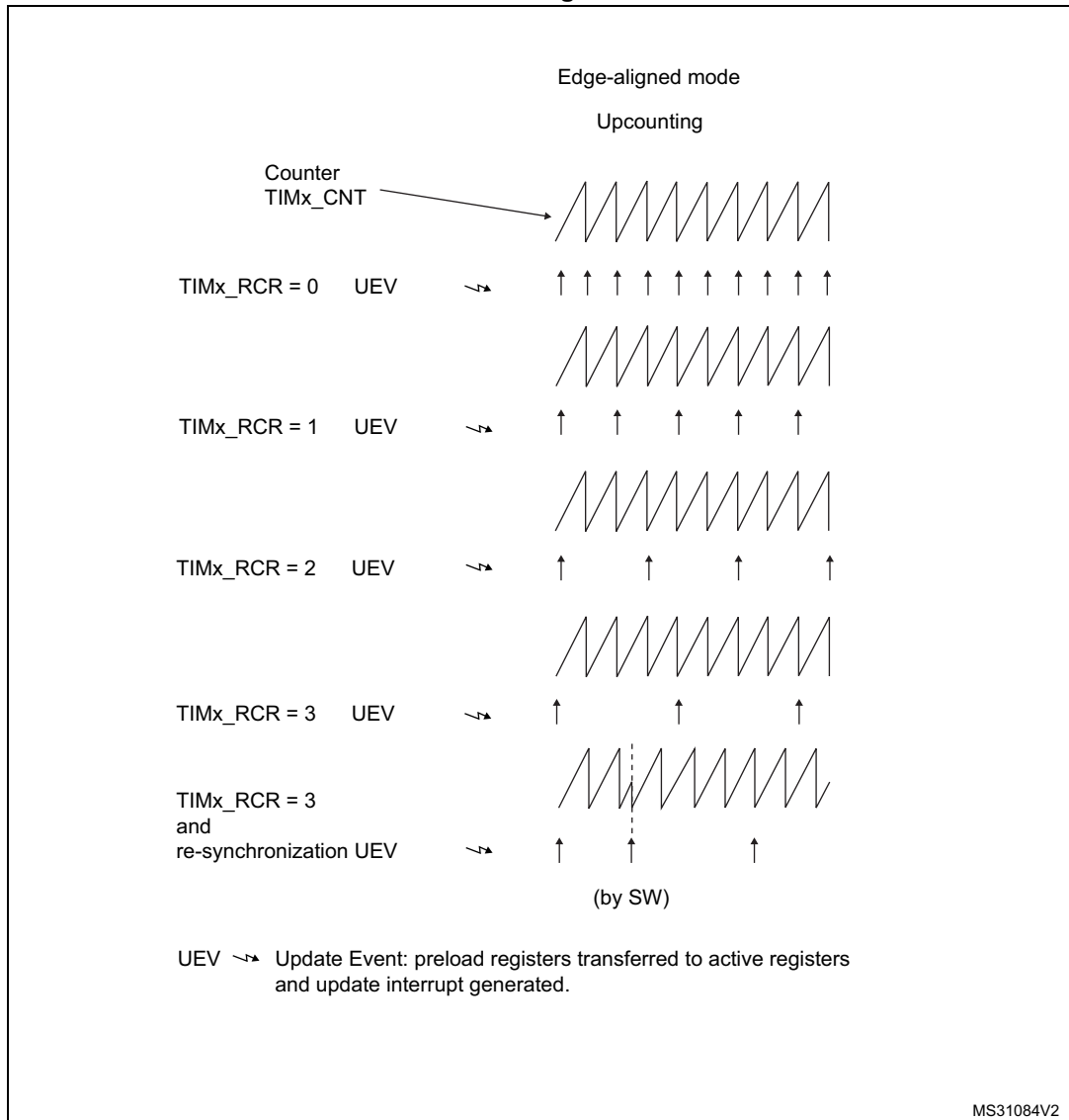
Figure 685. Update rate examples depending on mode and TIMx_RCR register settings
