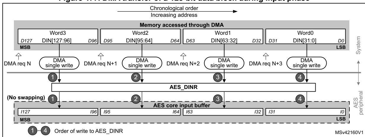
Figure 477. DMA transfer of a 128-bit data block during input phase
