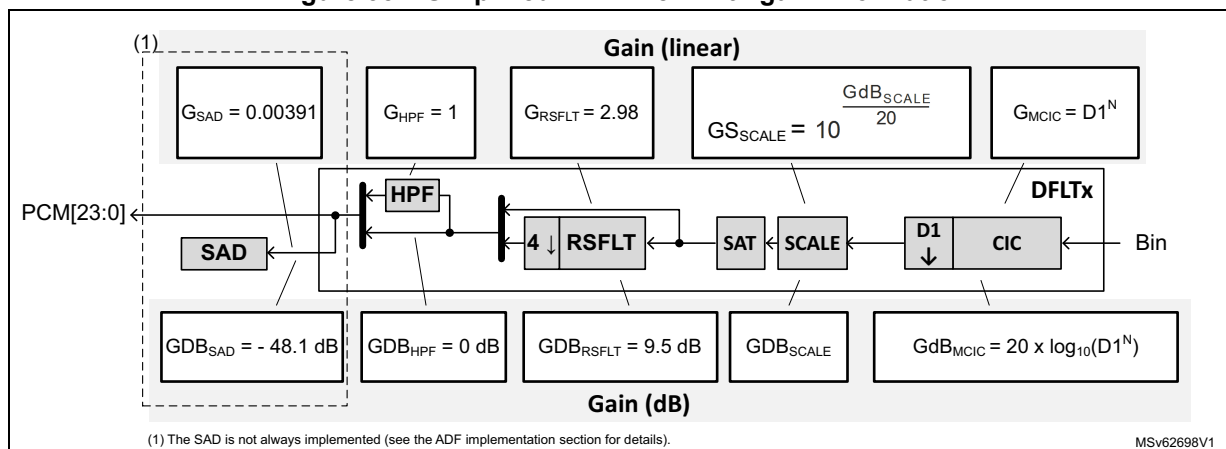
Figure 354. Simplified DFLT view with gain information
