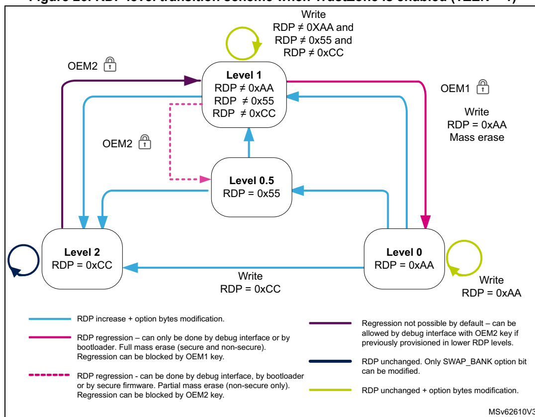
Figure 26. RDP level transition scheme when TrustZone is enabled (TZEN = 1)
