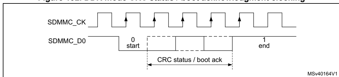
Figure 192. DDR mode CRC status / boot acknowledgment clocking
