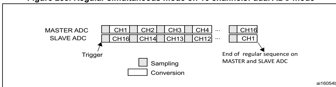
Figure 255. Regular simultaneous mode on 16 channels: dual ADC mode
