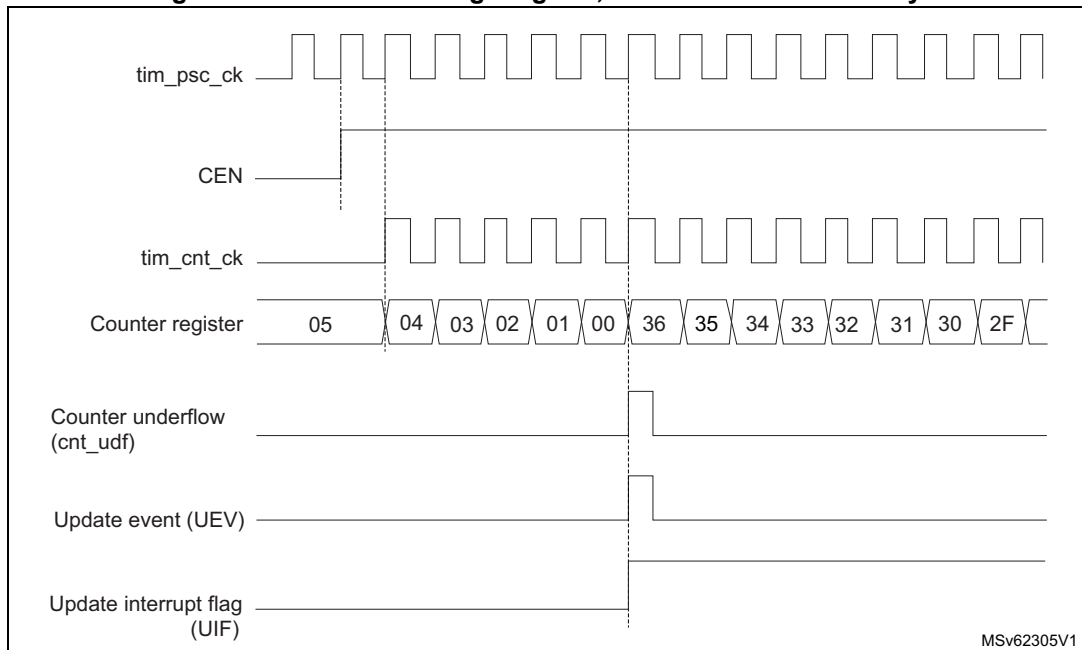
Figure 512. Counter timing diagram, internal clock divided by 1
