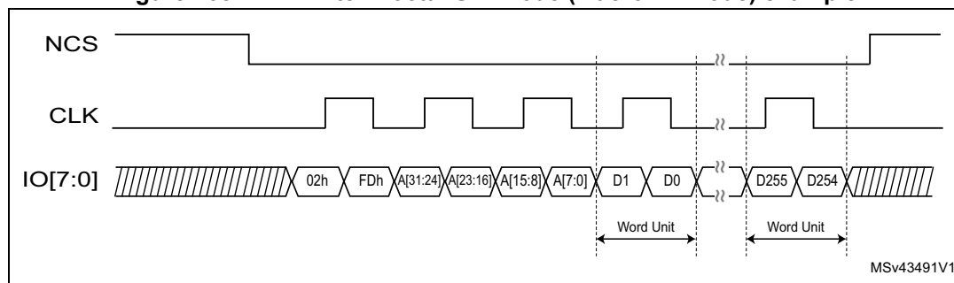
Figure 168. DTR write in octal-SPI mode (Macronix mode) example
