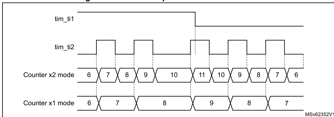
Figure 643. Direction plus clock encoder mode
