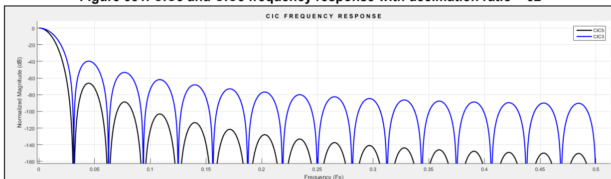
Figure 331. CIC3 and CIC5 frequency response with decimation ratio = 32
