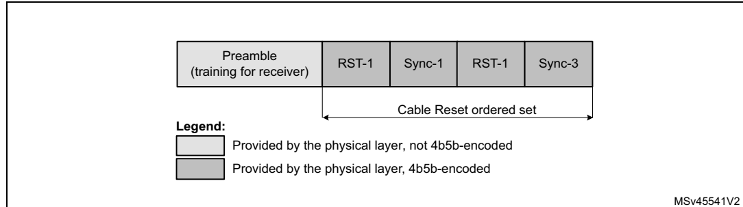
Figure 942. Line format of Cable Reset
