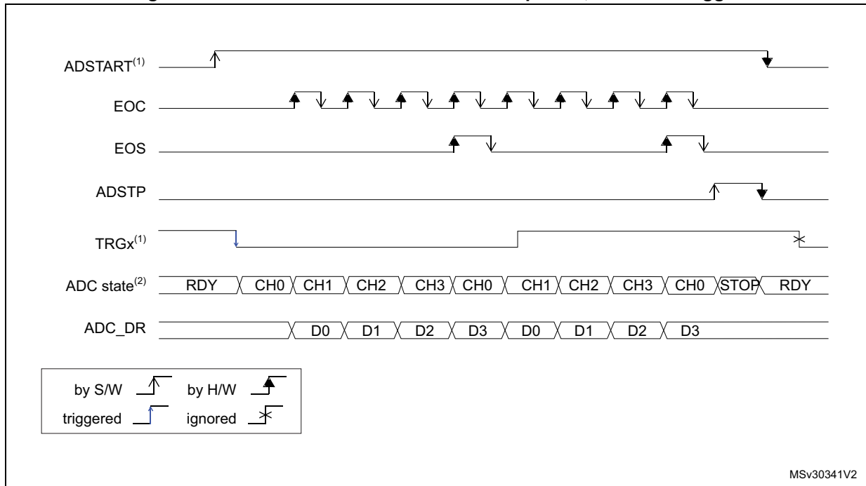
Figure 284. Continuous conversions of a sequence, hardware trigger
