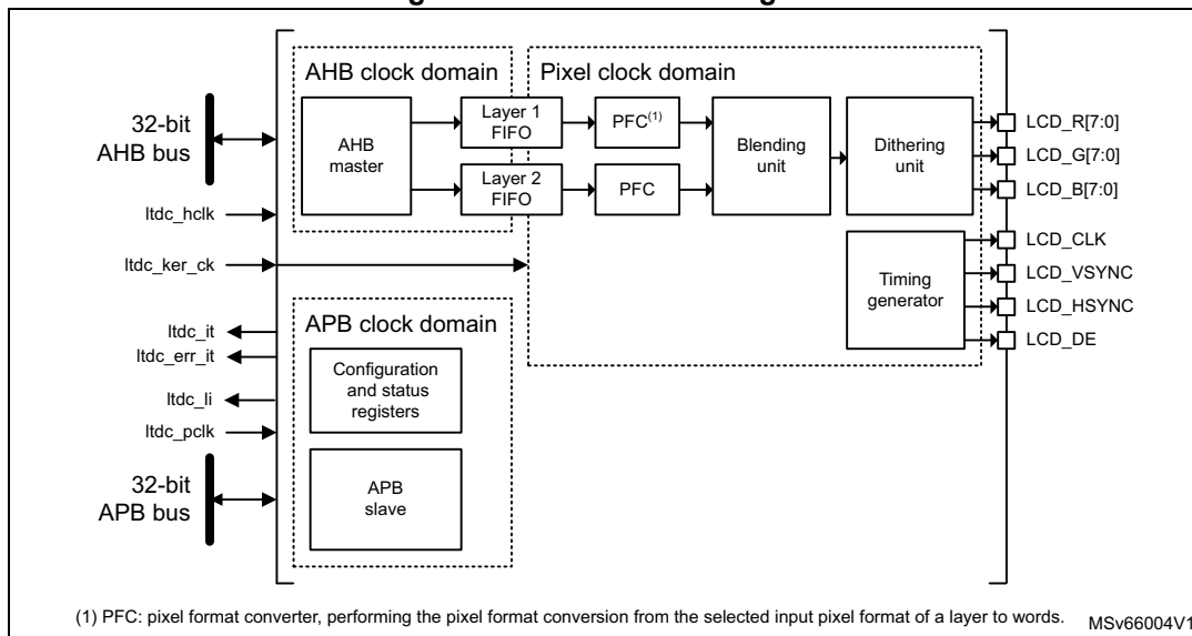
Figure 401. LTDC block diagram
