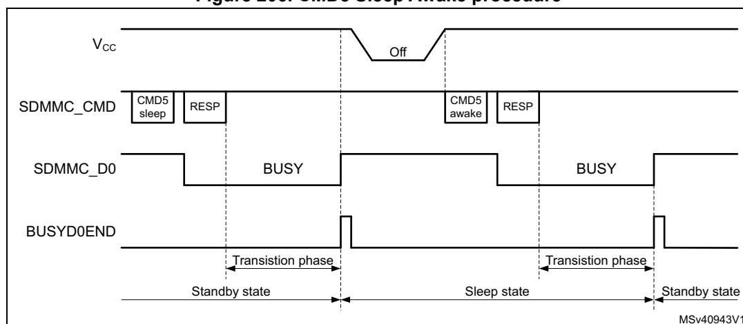
Figure 206. CMD5 Sleep Awake procedure
