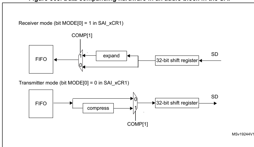
Figure 868. Data companding hardware in an audio block in the SAI
