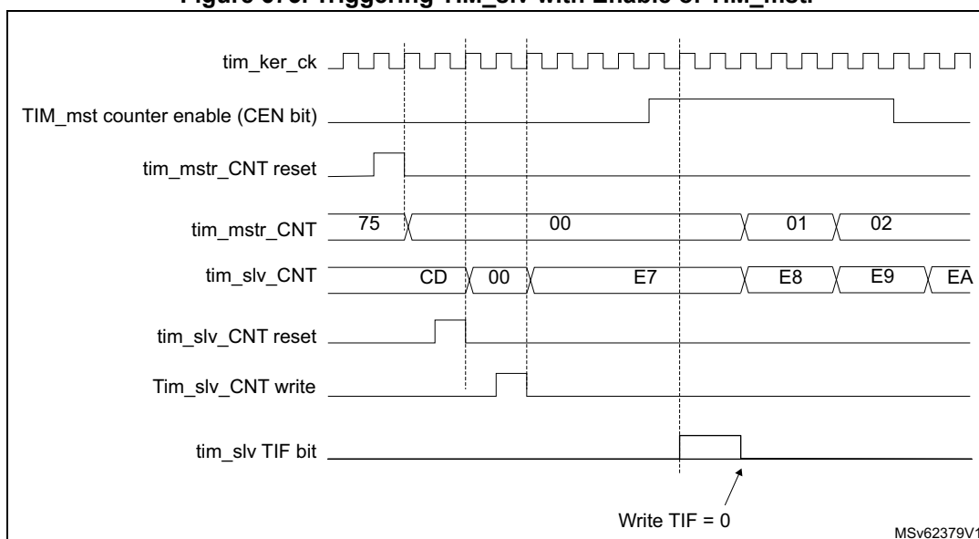
Figure 673. Triggering TIM_slv with Enable of TIM_mstr
