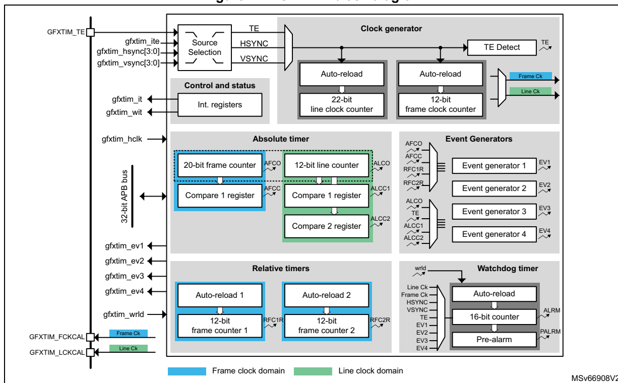
Figure 744. GFXTIM block diagram
