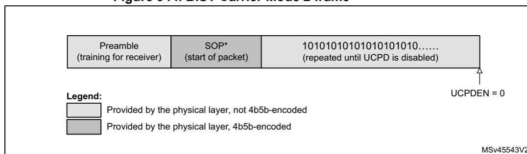
Figure 944. BIST Carrier Mode 2 frame
