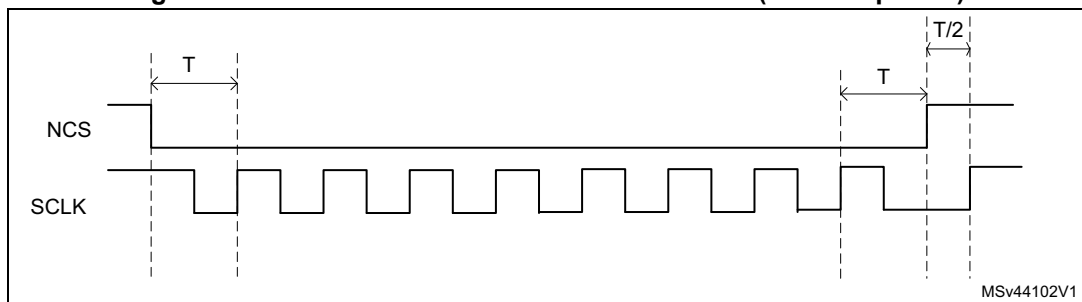
Figure 178. NCS when CKMODE = 1 in DTR mode (T = CLK period)
