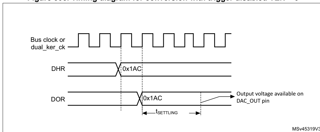
Figure 305. Timing diagram for conversion with trigger disabled TEN = 0
