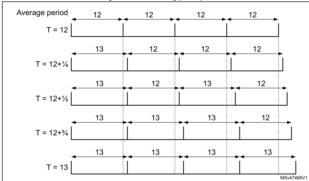
Figure 726. Dithering principle
