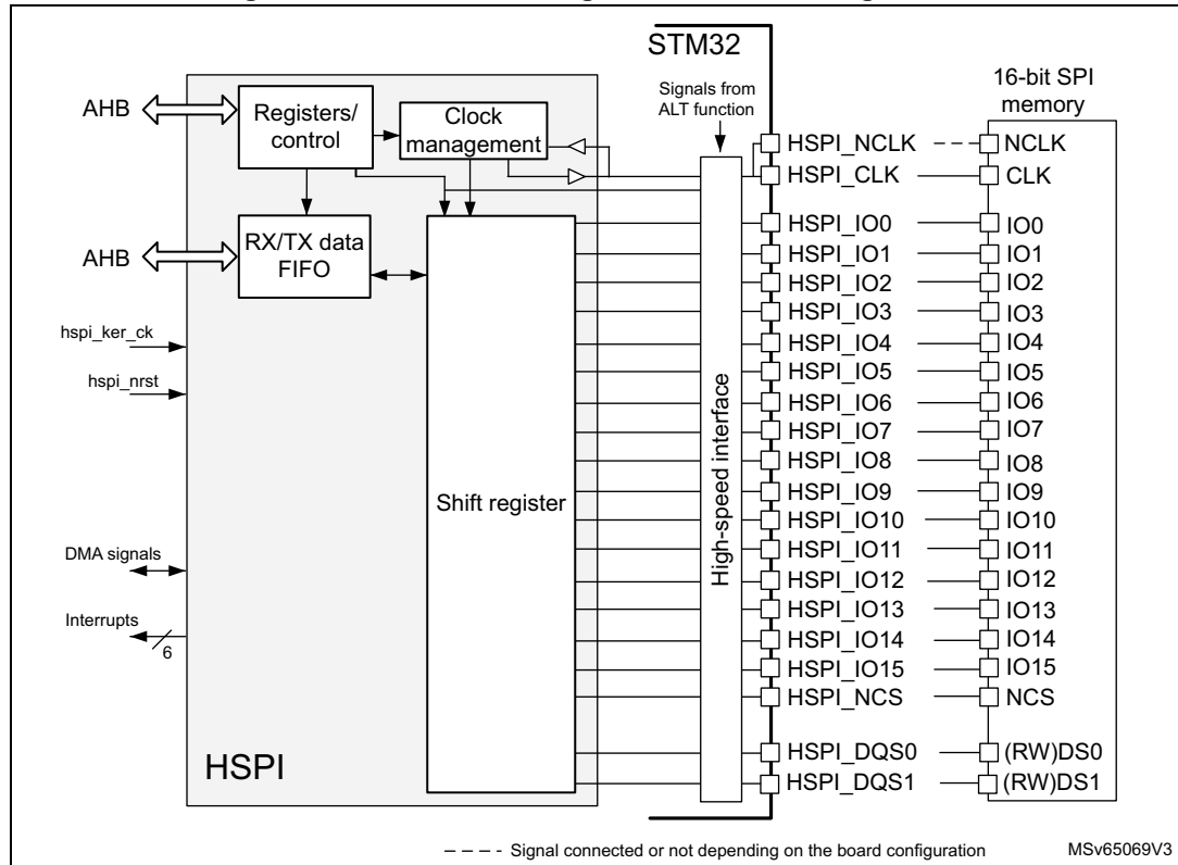
Figure 160. HSPI block diagram for 16-bit configuration
