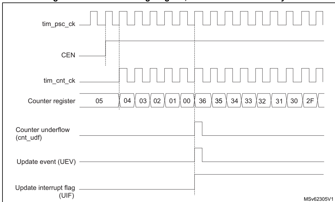
Figure 602. Counter timing diagram, internal clock divided by 1
