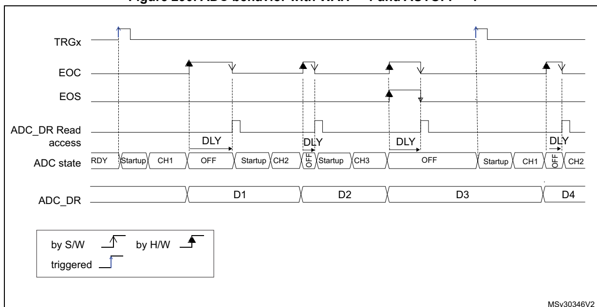
Figure 290. ADC behavior with WAIT = 1 and AUTOFF = 1
