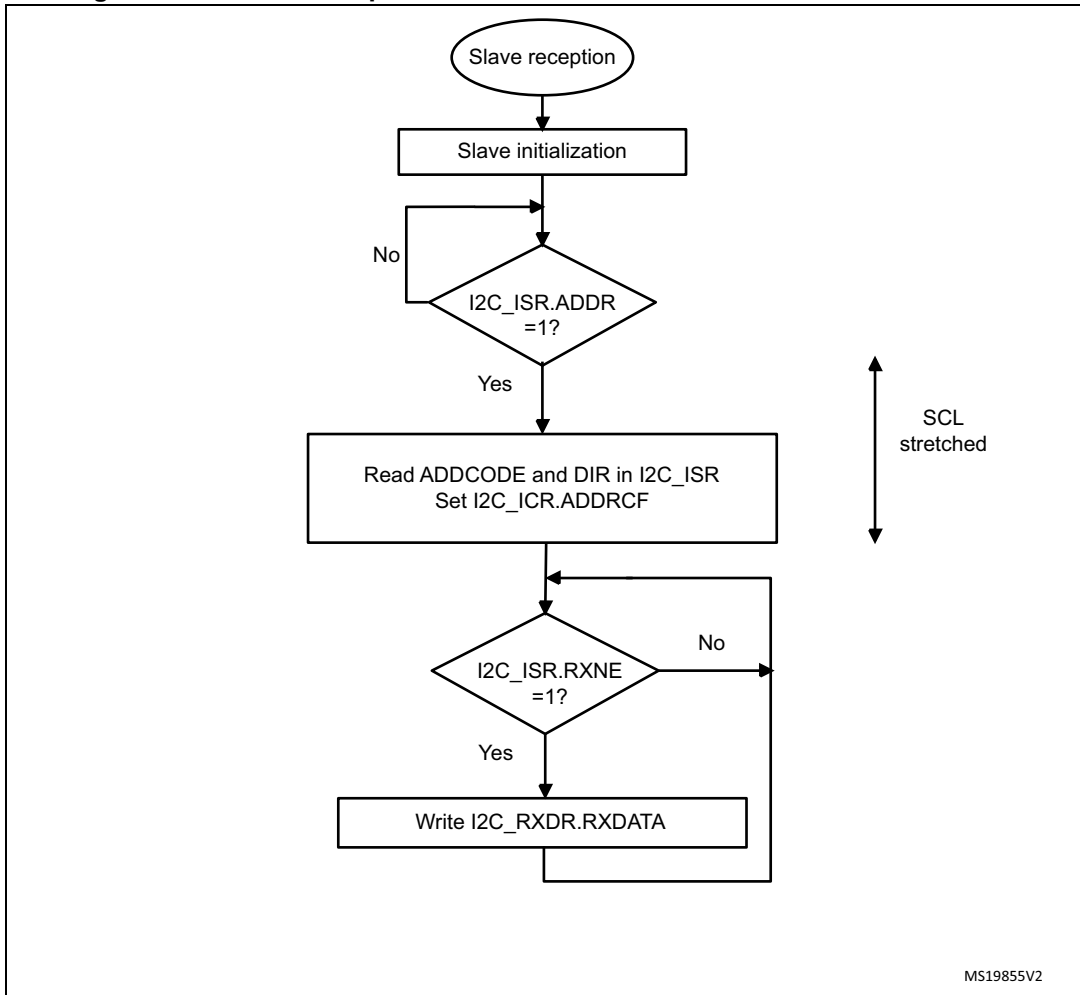
Figure 780. Transfer sequence flow for slave receiver with NOSTRETCH = 0
