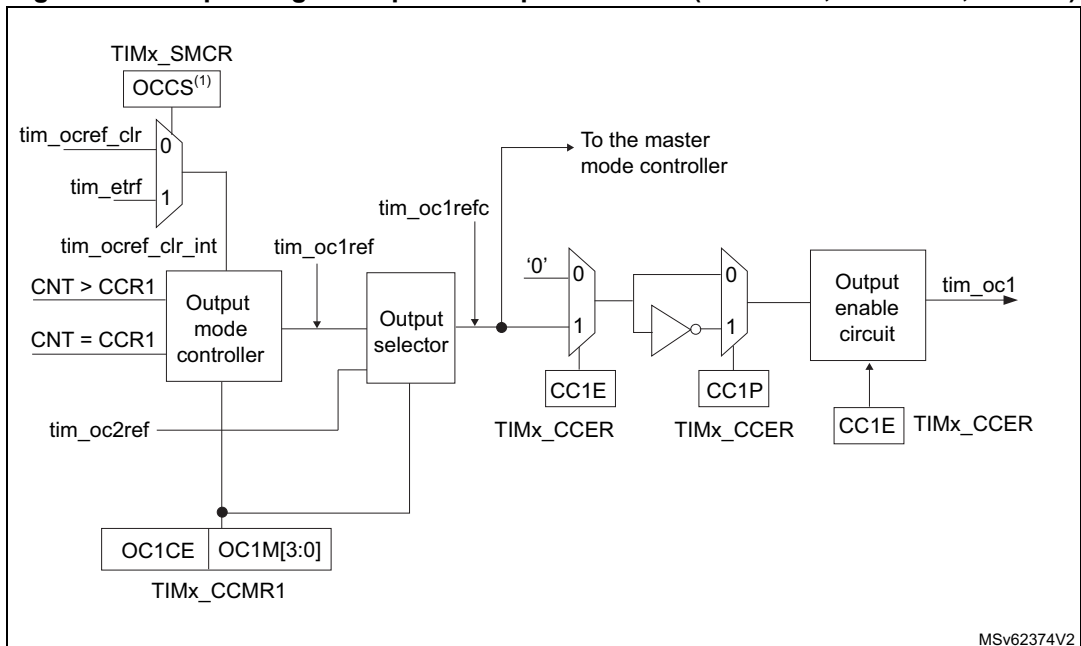
Figure 620. Output stage of capture/compare channel (channel 1, idem ch.2, 3 and 4)
