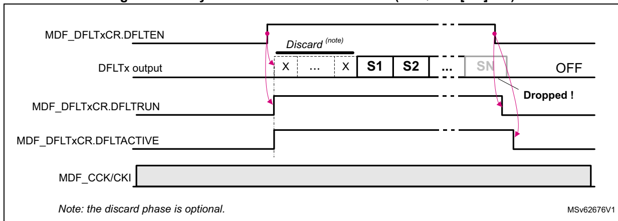
Figure 335. Asynchronous continuous mode (ACQMOD[2:0] = 0)
