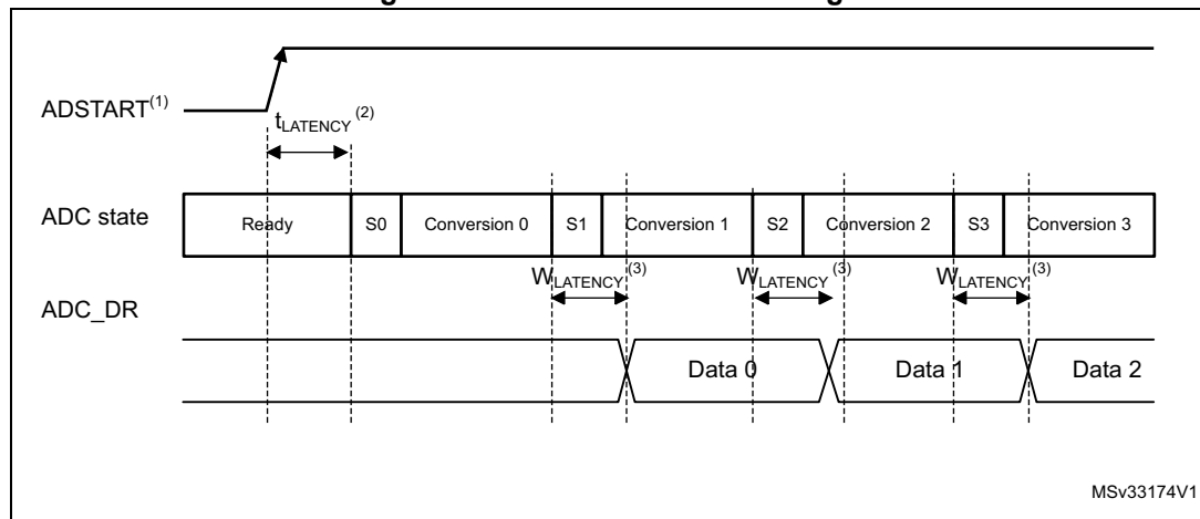
Figure 279. ADC conversion timings
