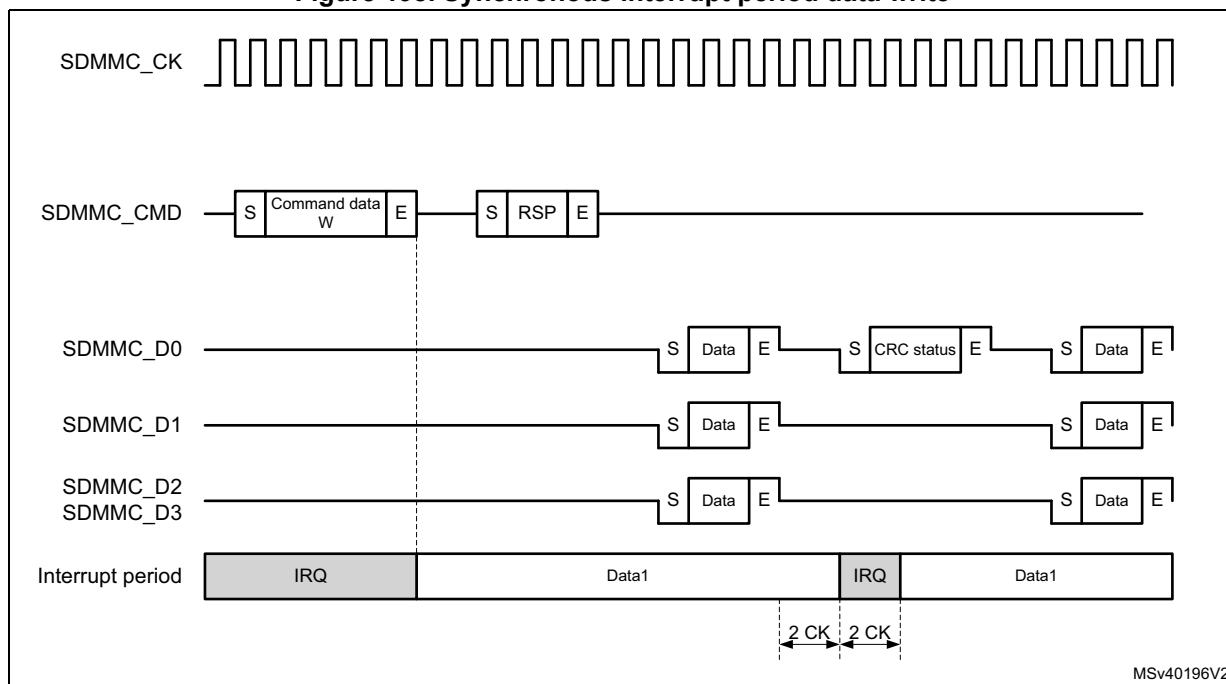
Figure 198. Synchronous interrupt period data write
