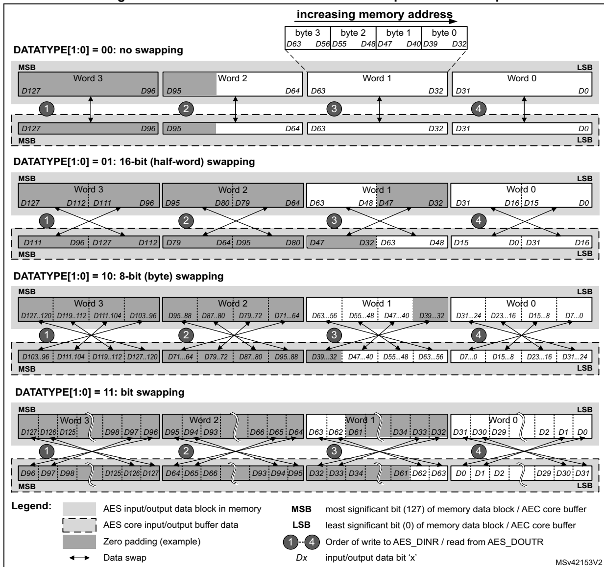
Figure 476. 128-bit block construction with respect to data swap
