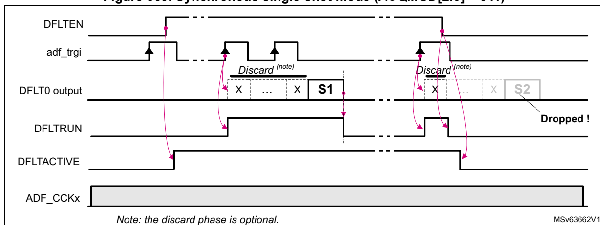
Figure 369. Synchronous single-shot mode ( ACQMOD[2:0] = 011 )
