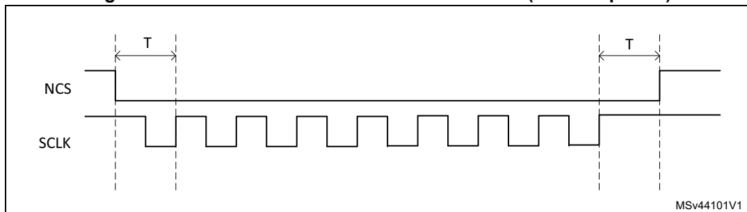
Figure 156. NCS when CKMODE = 1 in SDR mode (T = CLK period)
