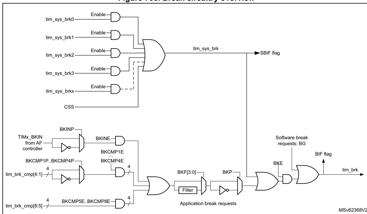
Figure 705. Break circuitry overview
