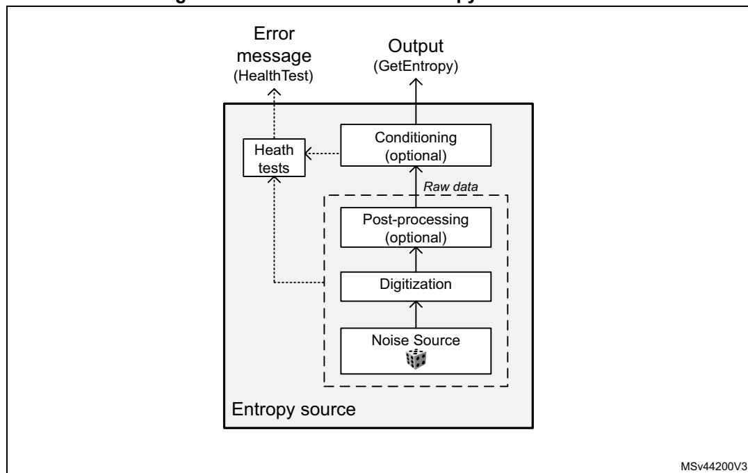
Figure 451. NIST SP800-90B entropy source model
