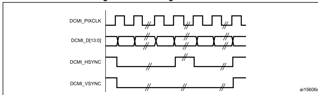
Figure 387. DCMI signal waveforms
