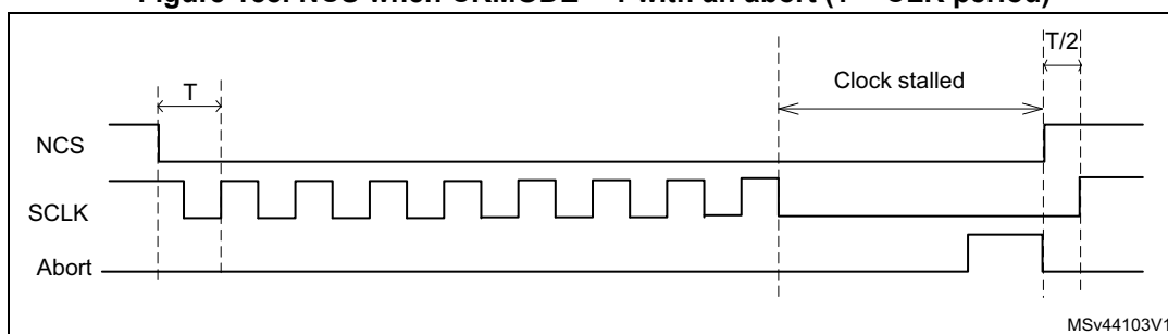
Figure 158. NCS when CKMODE = 1 with an abort (T = CLK period)
