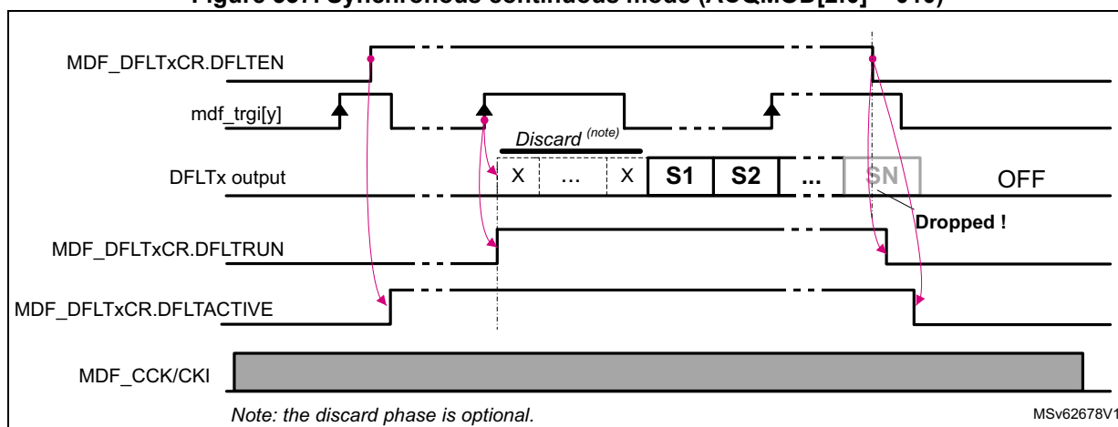
Figure 337. Synchronous continuous mode (ACQMOD[2:0] = 010)
