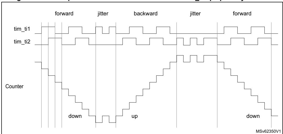
Figure 641. Example of encoder interface mode with tim_ti1fp1 polarity inverted
