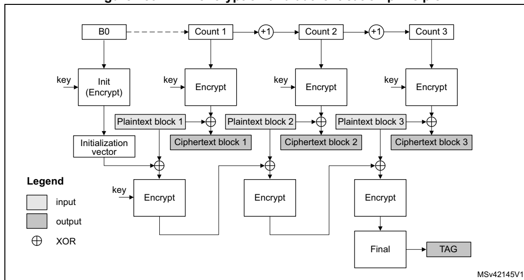
Figure 459. CCM encryption and authentication principle
