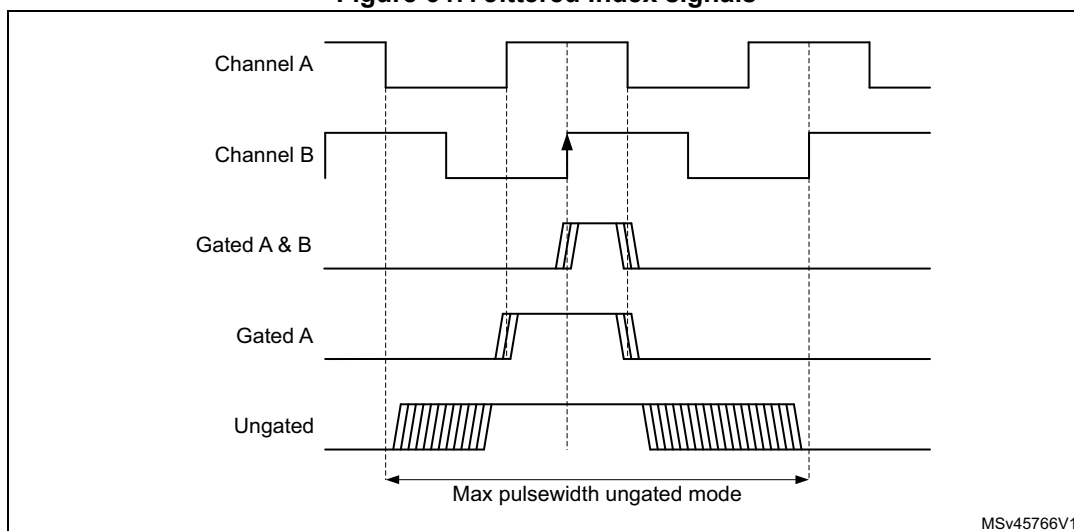
Figure 647. Jittered Index signals
