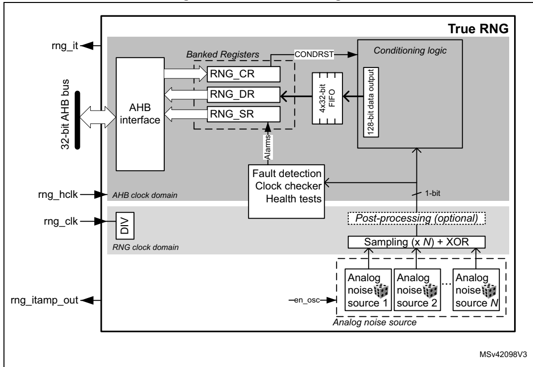
Figure 450. RNG block diagram
