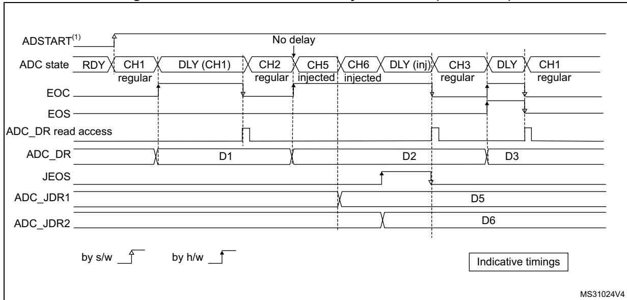
Figure 241. AUTODLY = 1 in auto-injected mode (JAUTO = 1)
