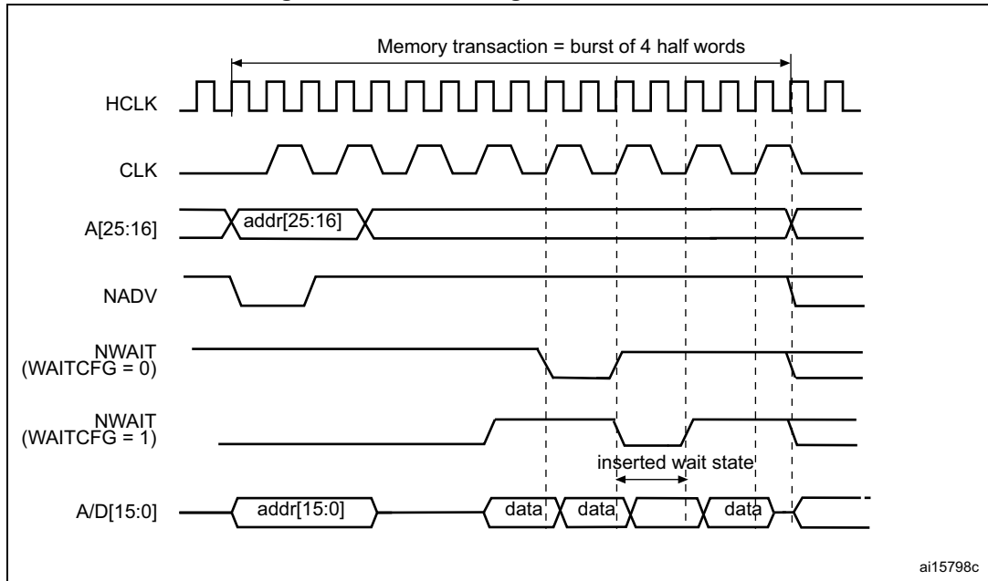
Figure 134. Wait configuration waveforms
