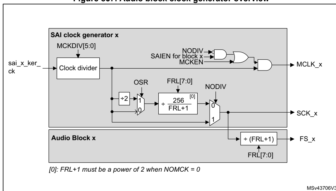
Figure 857. Audio block clock generator overview
