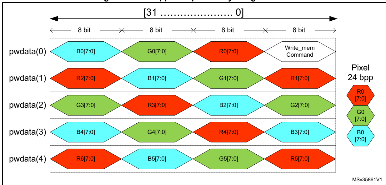
Figure 412. 24 bpp APB pixel to byte organization
