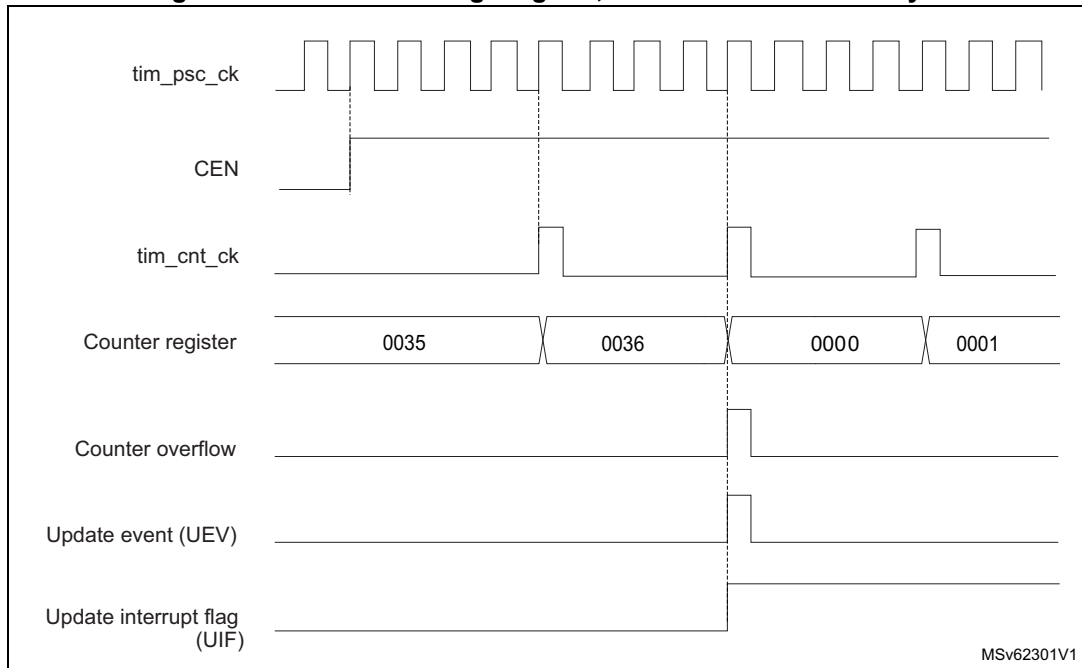
Figure 681. Counter timing diagram, internal clock divided by 4
