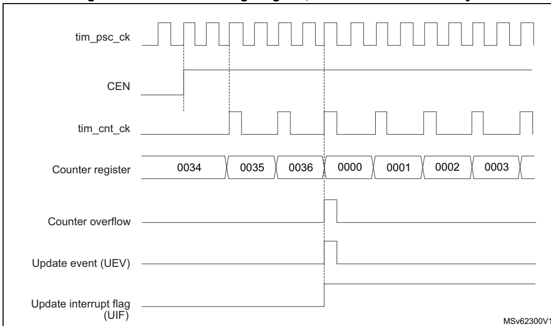
Figure 597. Counter timing diagram, internal clock divided by 2
