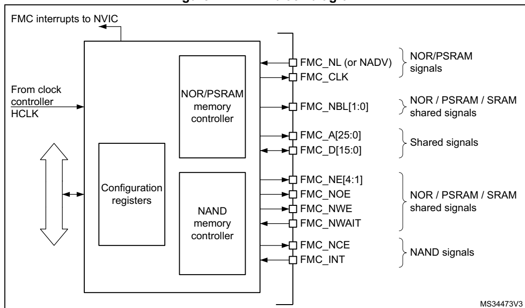
Figure 117. FMC block diagram
