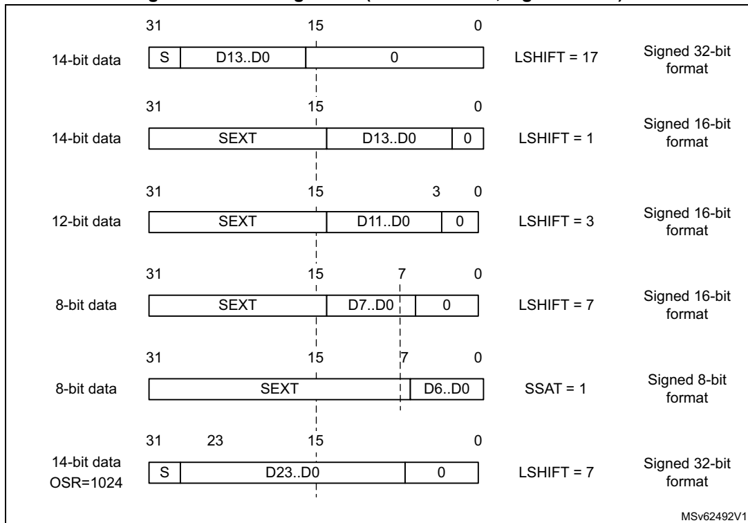
Figure 234. Left alignment (offset enabled, signed value)
