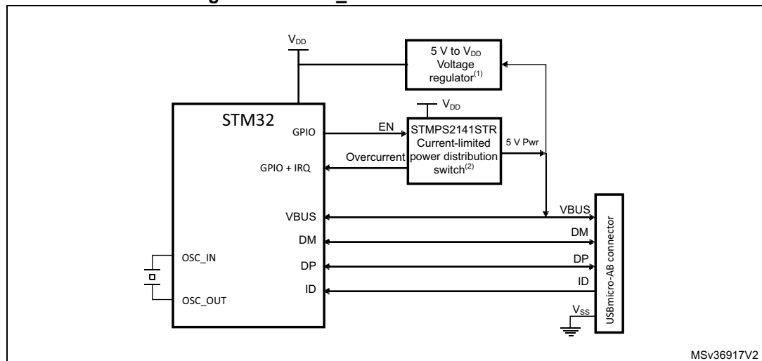
Figure 910. OTG_HS A-B device connection
