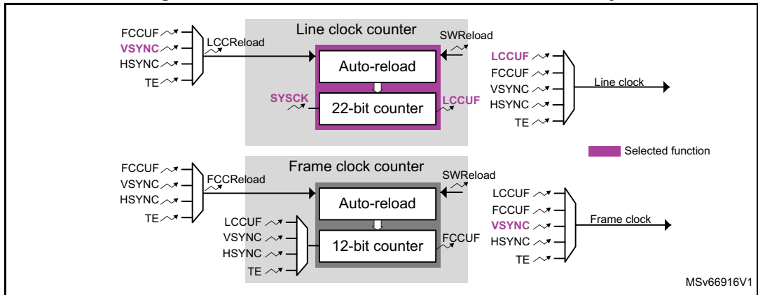
Figure 752. Active counters with external VSYNC only
