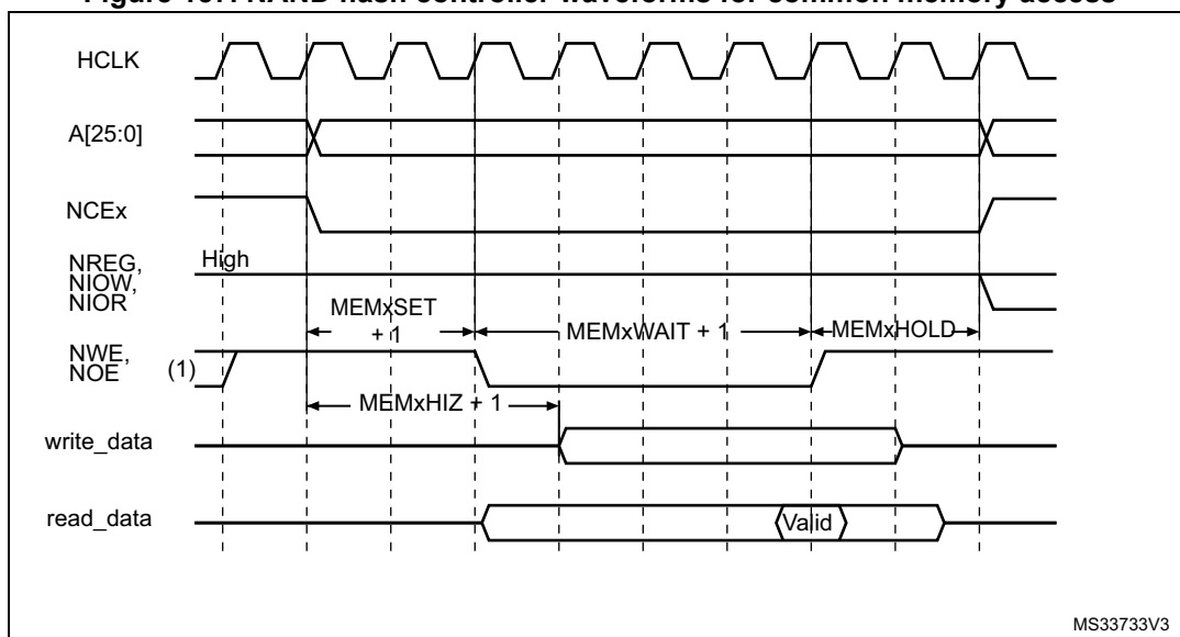
Figure 137. NAND flash controller waveforms for common memory access
