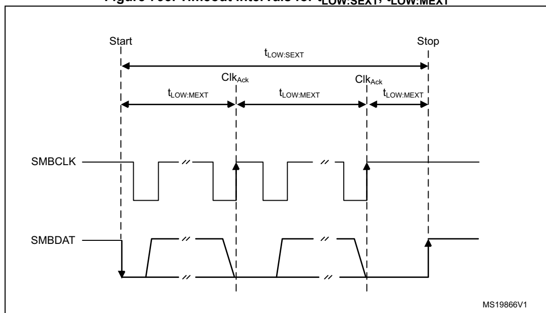
Figure 793. Timeout intervals for t_{\text{LOW:SEXT}} , t_{\text{LOW:MEXT}}
