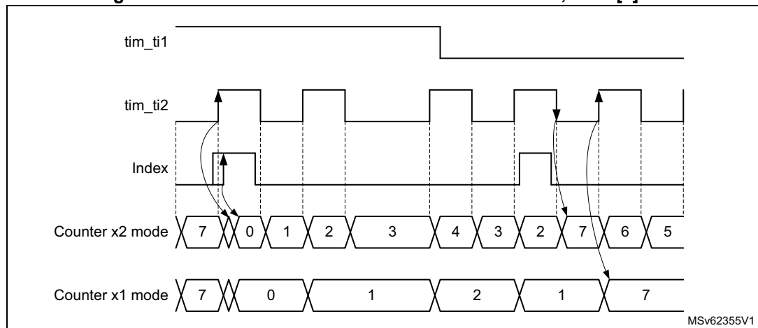
Figure 582. Index behavior in directional clock mode, IPOS[0] = 1
