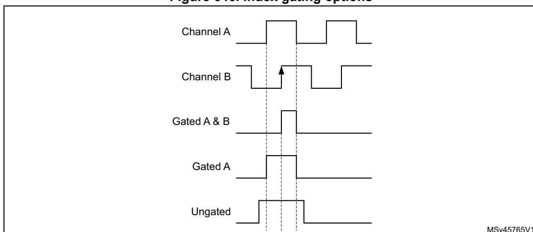
Figure 646. Index gating options
