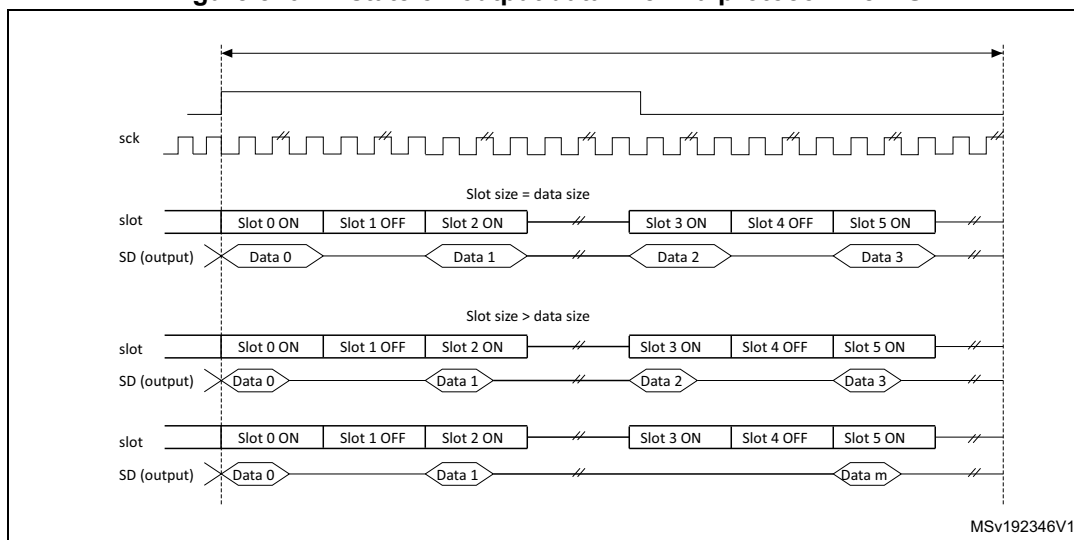
Figure 870. Tristate on output data line in a protocol like I2S
