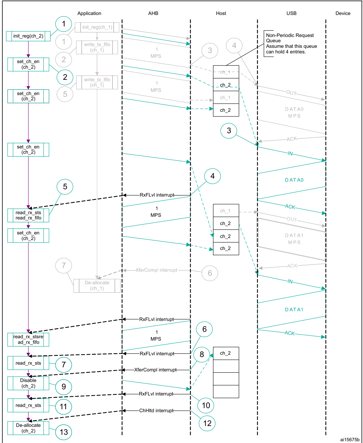
Figure 921. Bulk/control IN transactions
