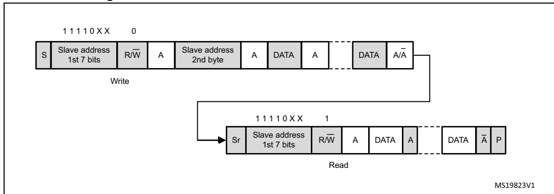
Figure 786. 10-bit address read access with HEAD10R = 1
