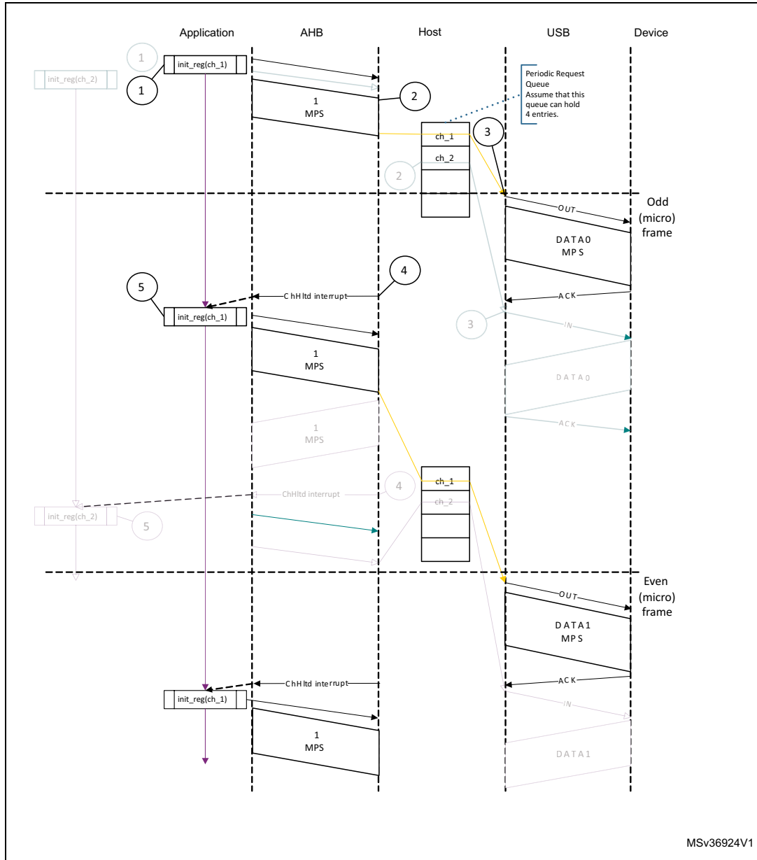
Figure 928. Normal interrupt OUT transactions - DMA mode
