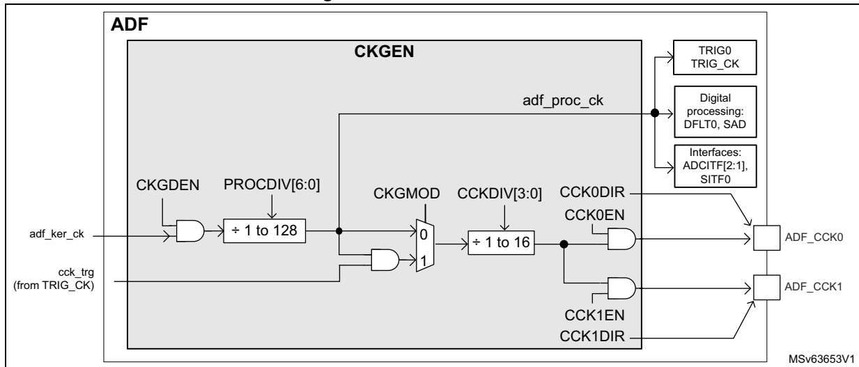
Figure 359. CKGEN overview
