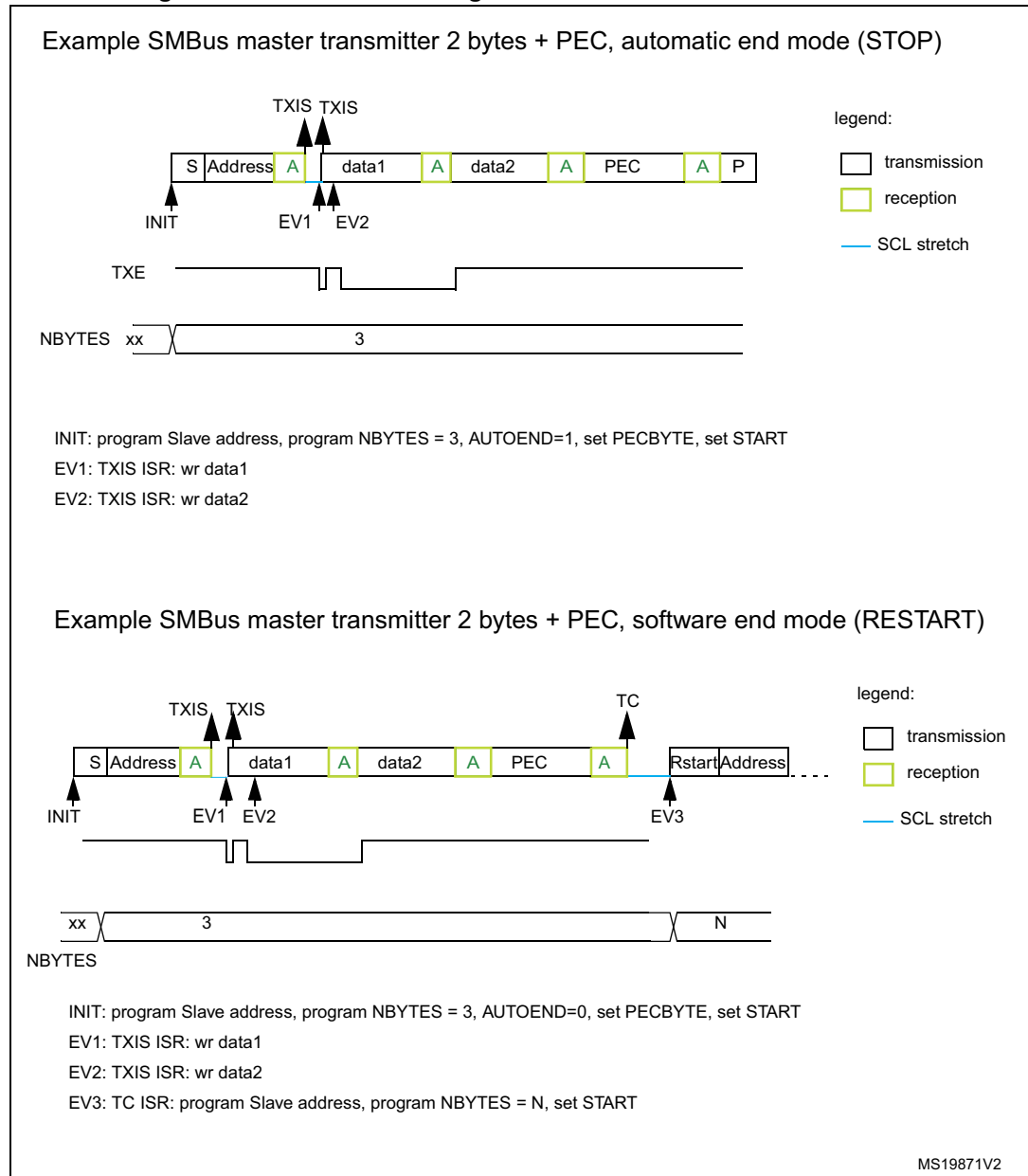
Figure 798. Bus transfer diagrams for SMBus master transmitter
