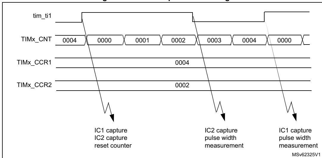
Figure 534. PWM input mode timing
