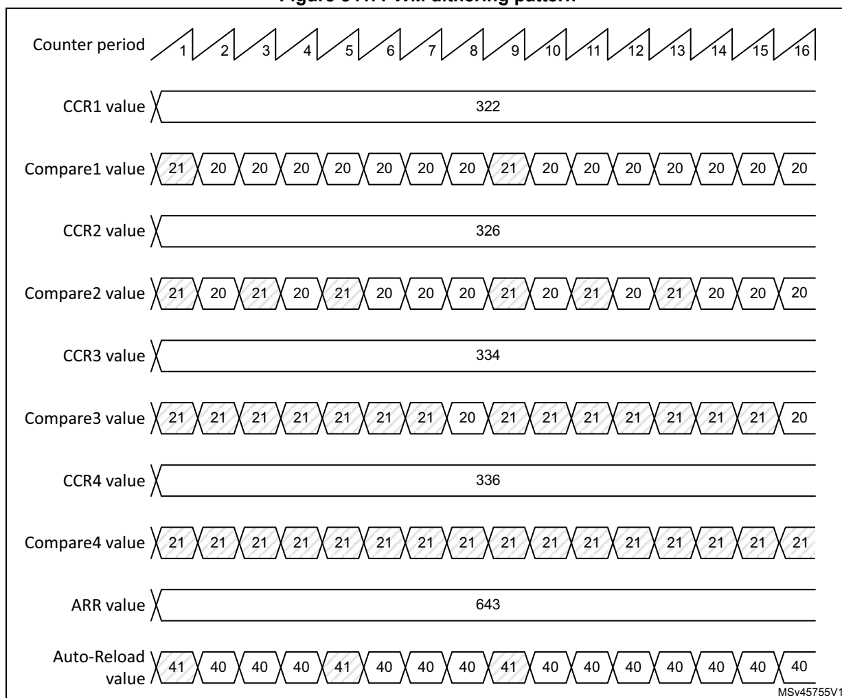
Figure 541. PWM dithering pattern
