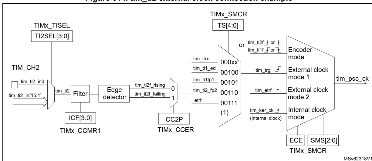
Figure 614. tim_ti2 external clock connection example
