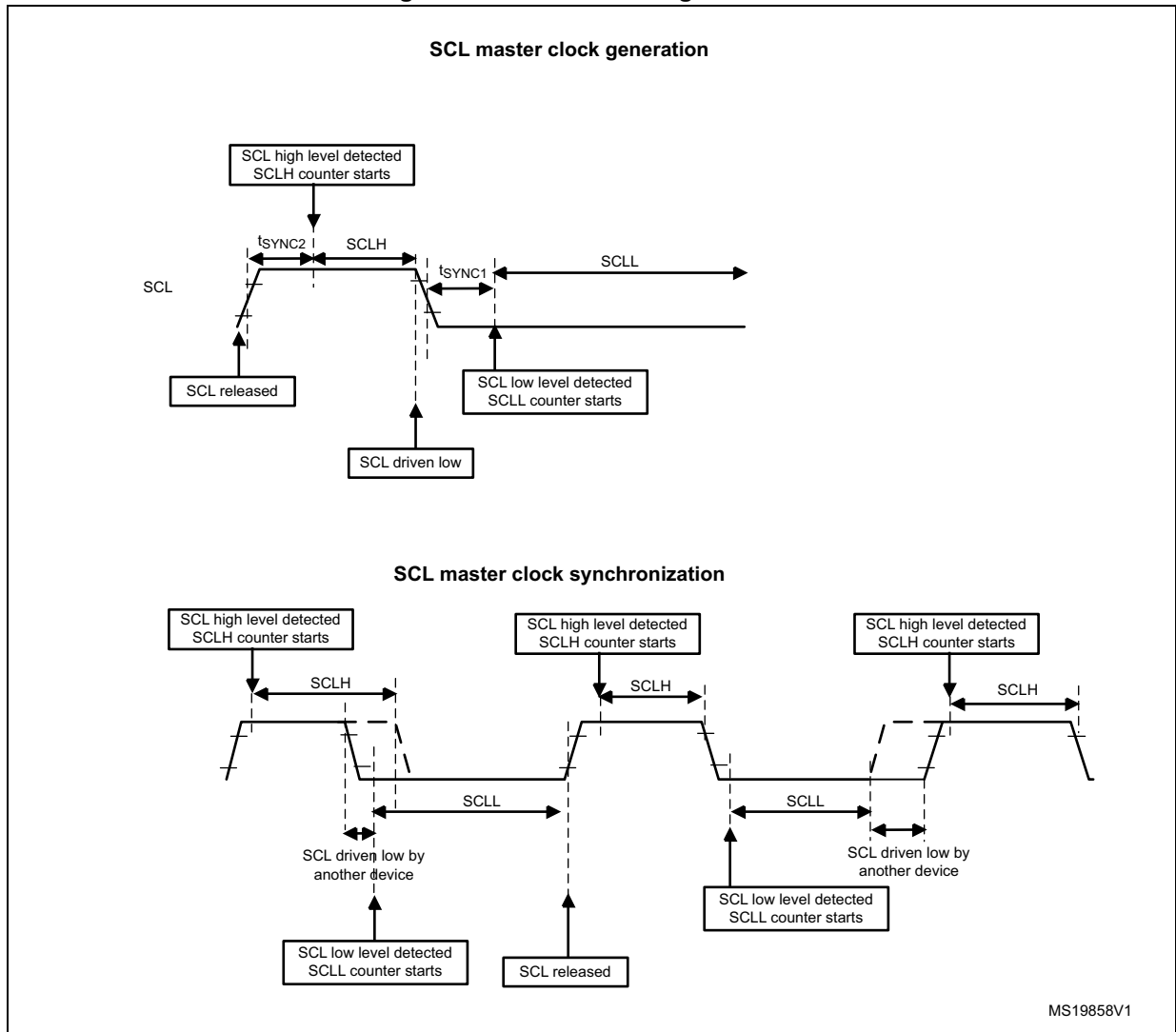
Figure 783. Master clock generation
