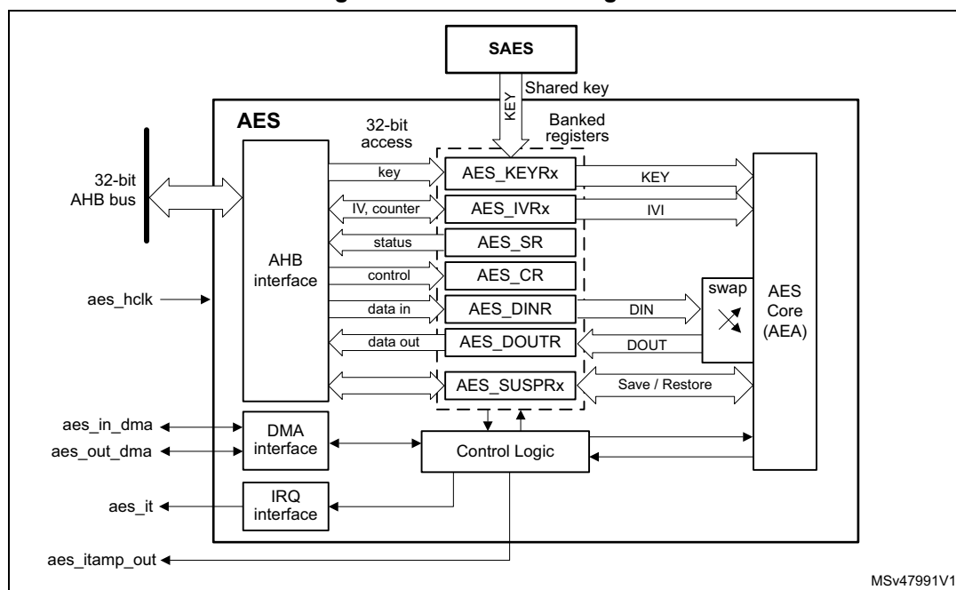
Figure 453. AES block diagram
