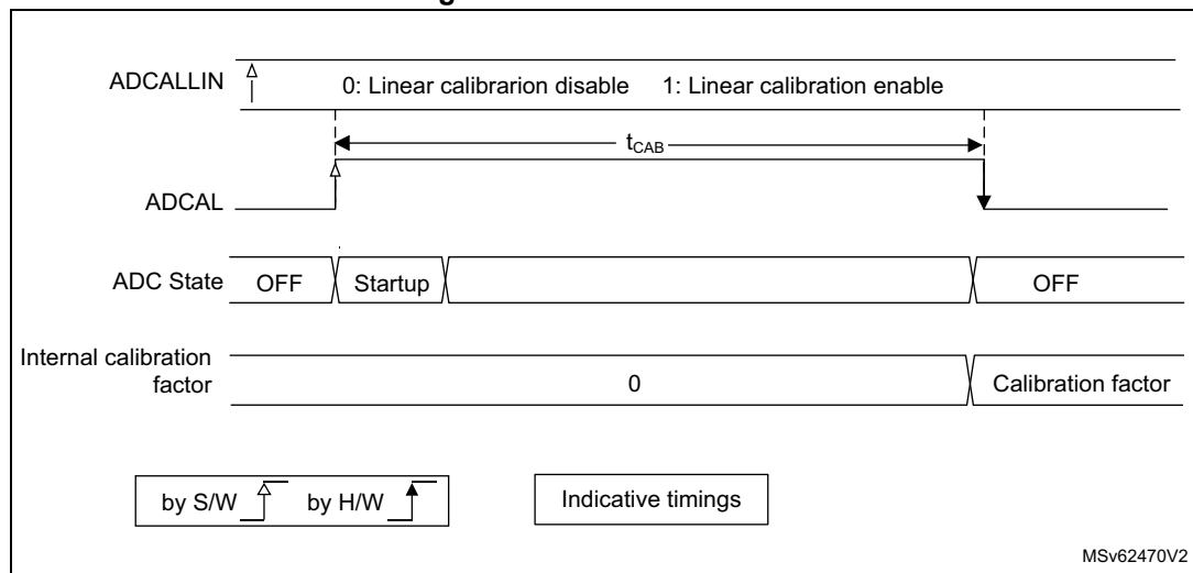
Figure 219. ADC calibration
