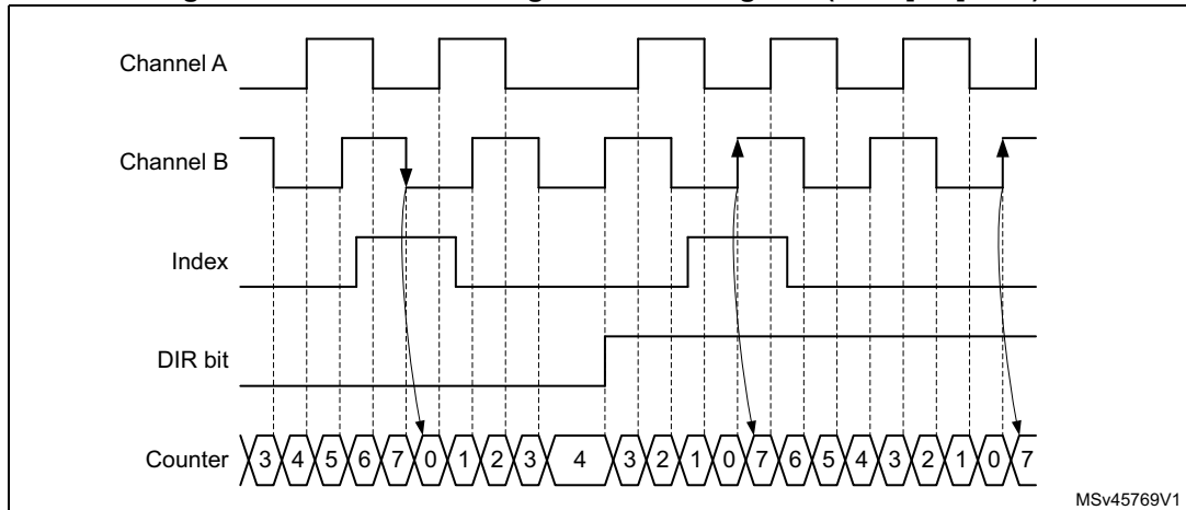
Figure 573. Counter reading with index ungated (IPOS[1:0] = 00)
