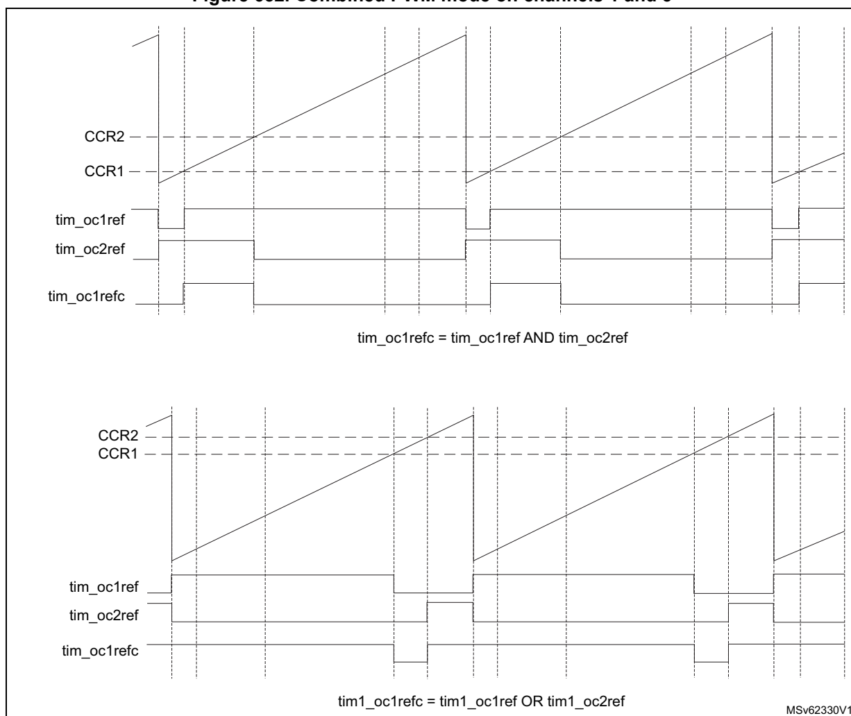
Figure 632. Combined PWM mode on channels 1 and 3
