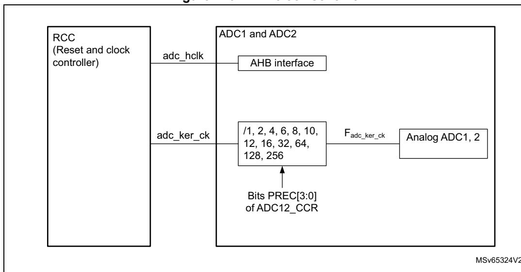
Figure 216. ADC clock scheme
