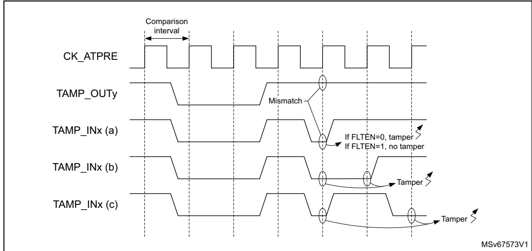
Figure 769. Active tamper filtering
