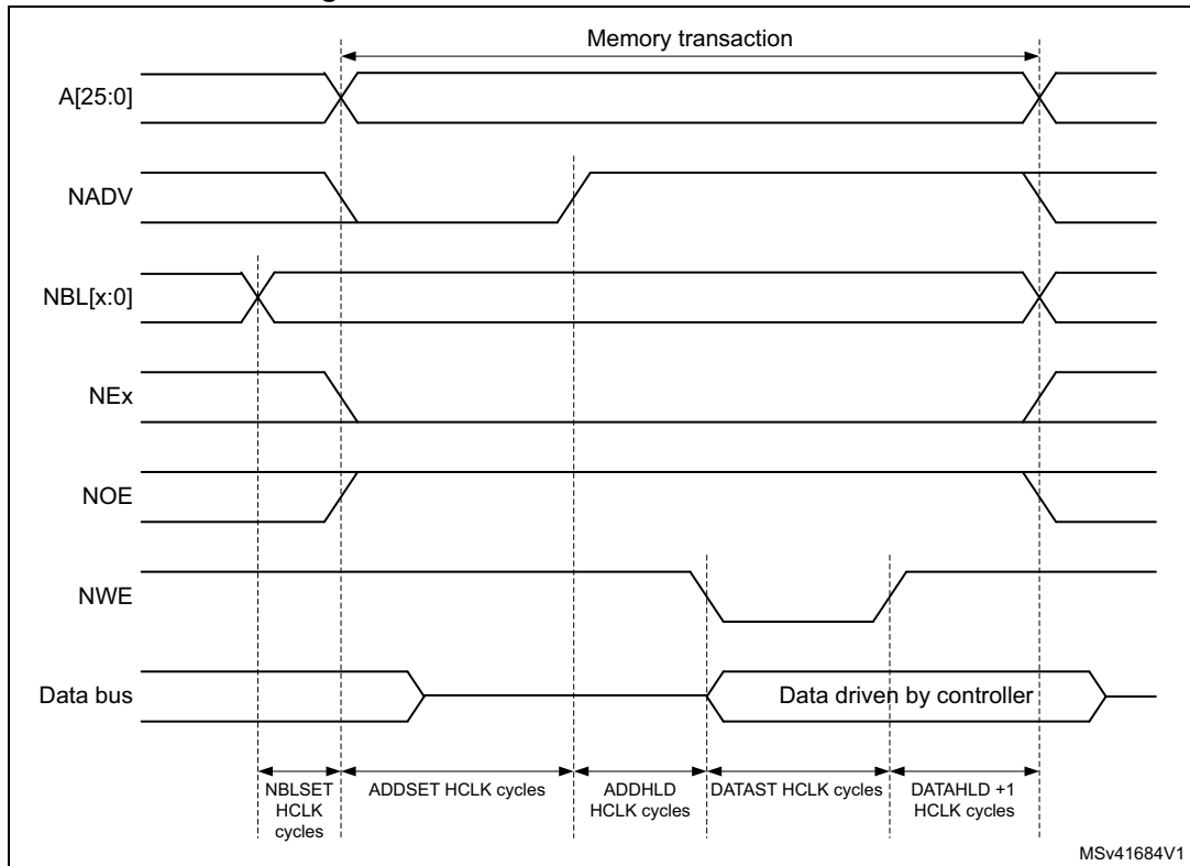
Figure 129. Mode D write access waveforms
