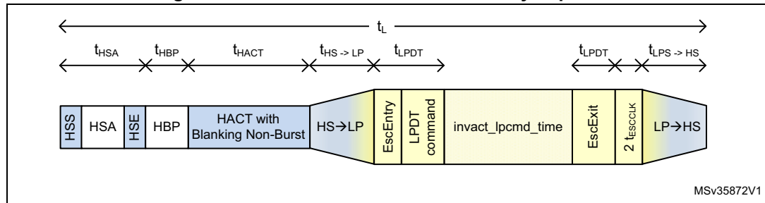
Figure 426. VLPSIZE for non-burst with sync events
