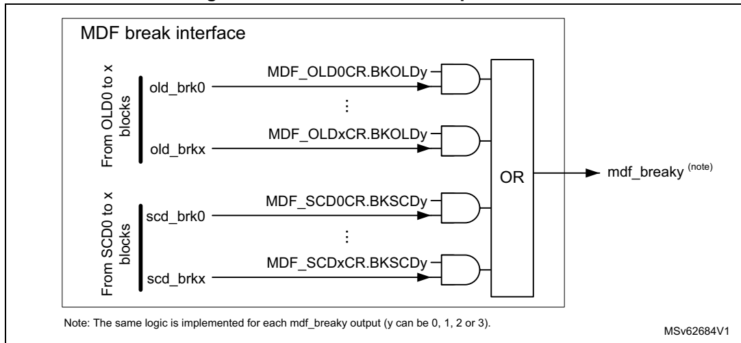
Figure 344. Break interface simplified view
