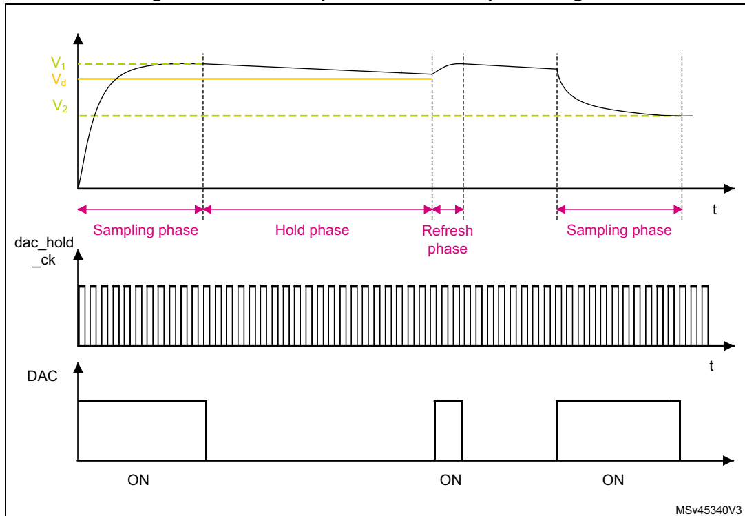
Figure 310. DAC Sample and hold mode phase diagram
