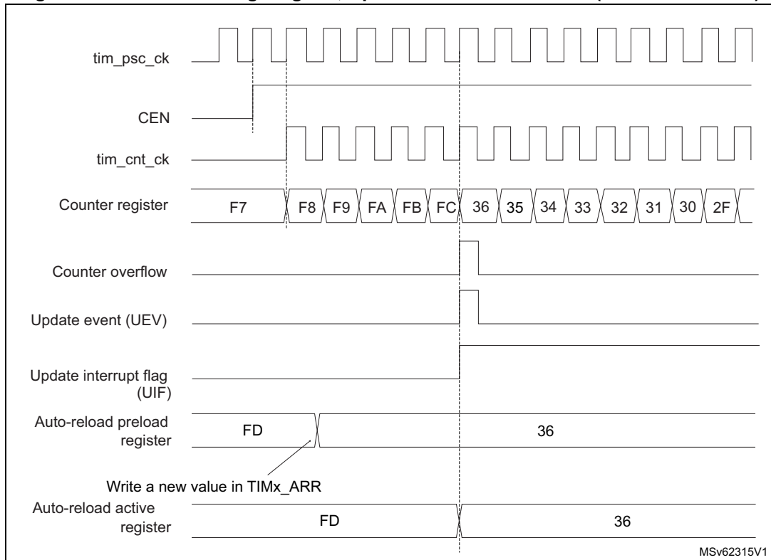
Figure 522. Counter timing diagram, Update event with ARPE=1 (counter overflow)
