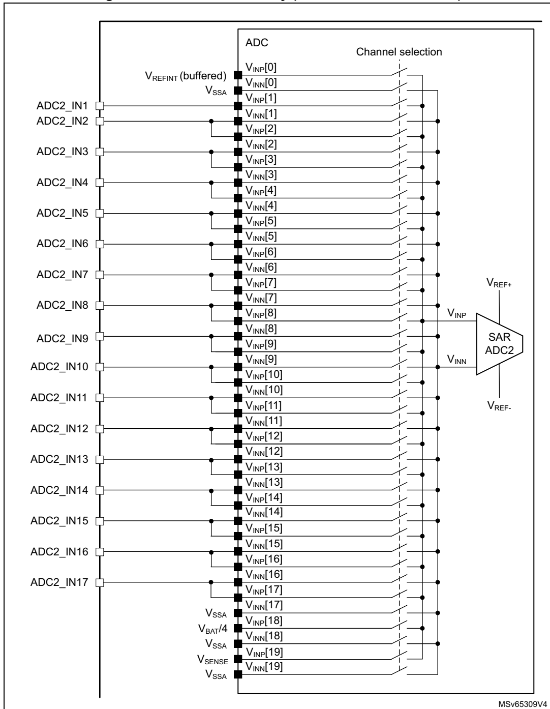
Figure 218. ADC2 connectivity (STM32U59x/5Ax/5Fx/5Gx)
