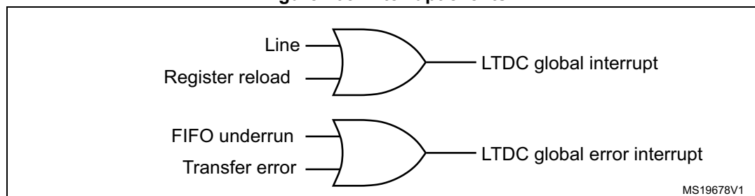
Figure 405. Interrupt events
