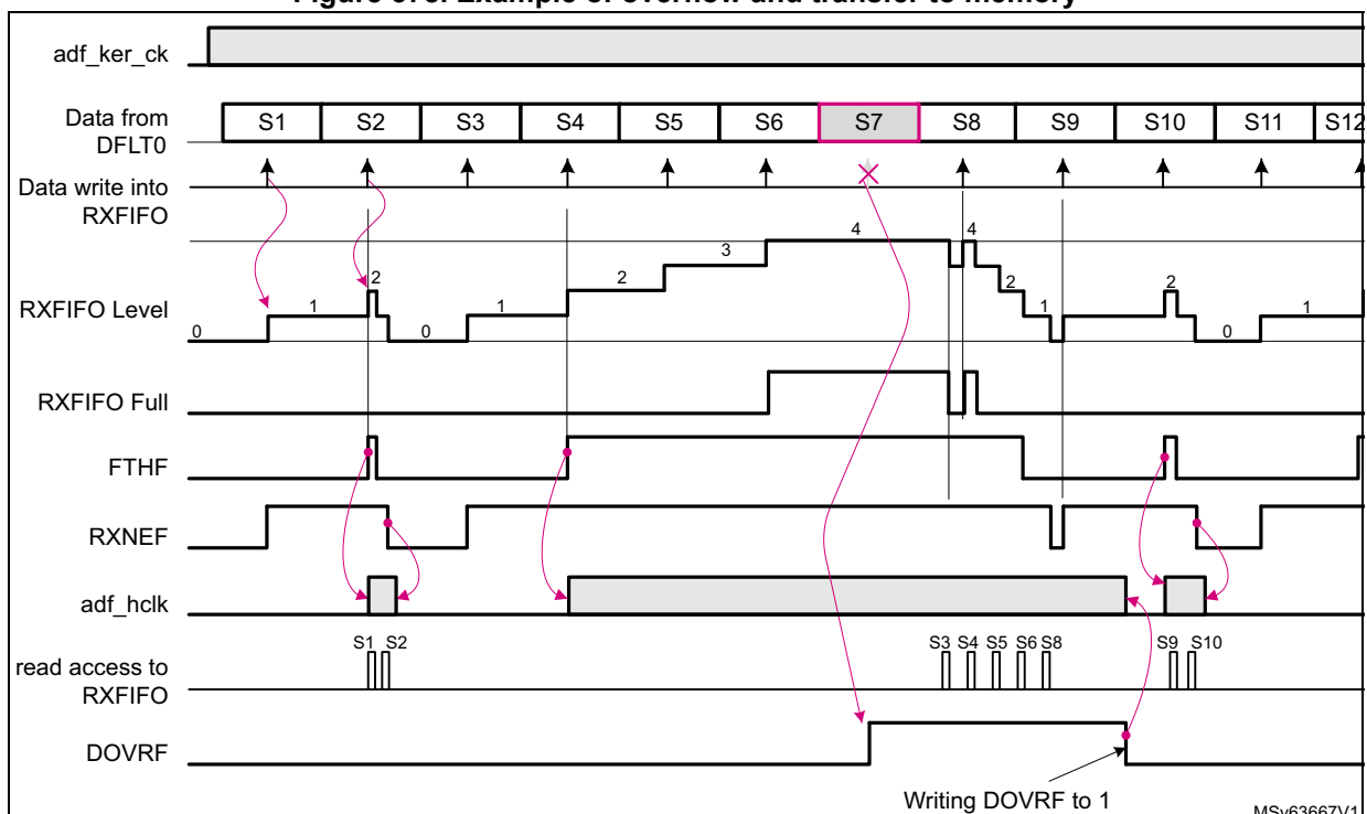
Figure 378. Example of overflow and transfer to memory
