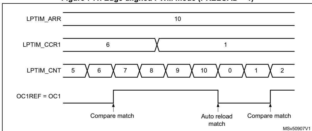
Figure 741. Edge-aligned PWM mode (PRELOAD = 1)
