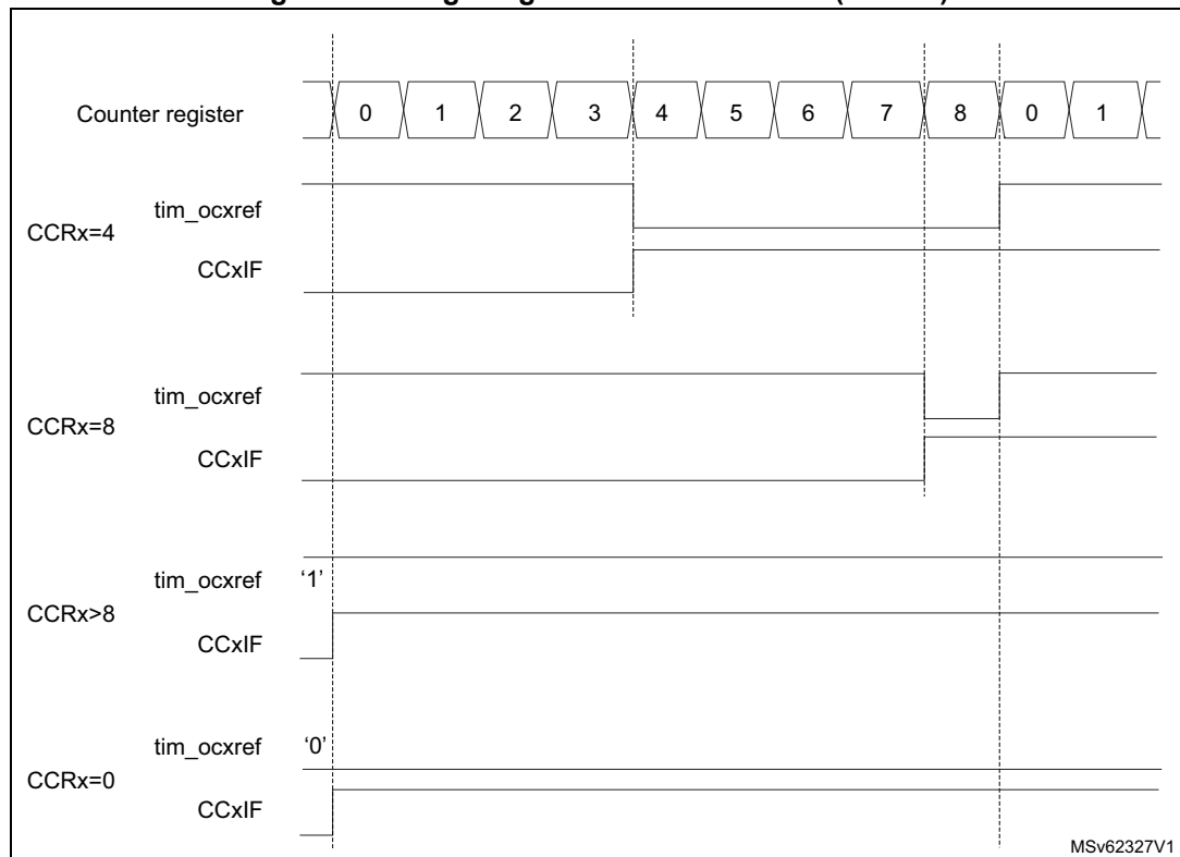
Figure 536. Edge-aligned PWM waveforms (ARR=8)
