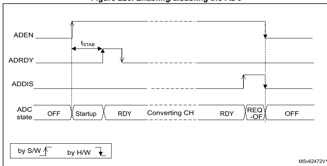
Figure 220. Enabling/disabling the ADC
