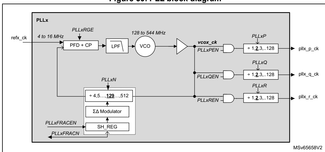
Figure 39. PLL block diagram
