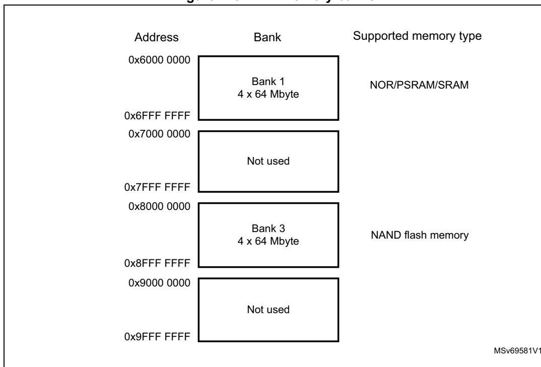
Figure 118. FMC memory banks
