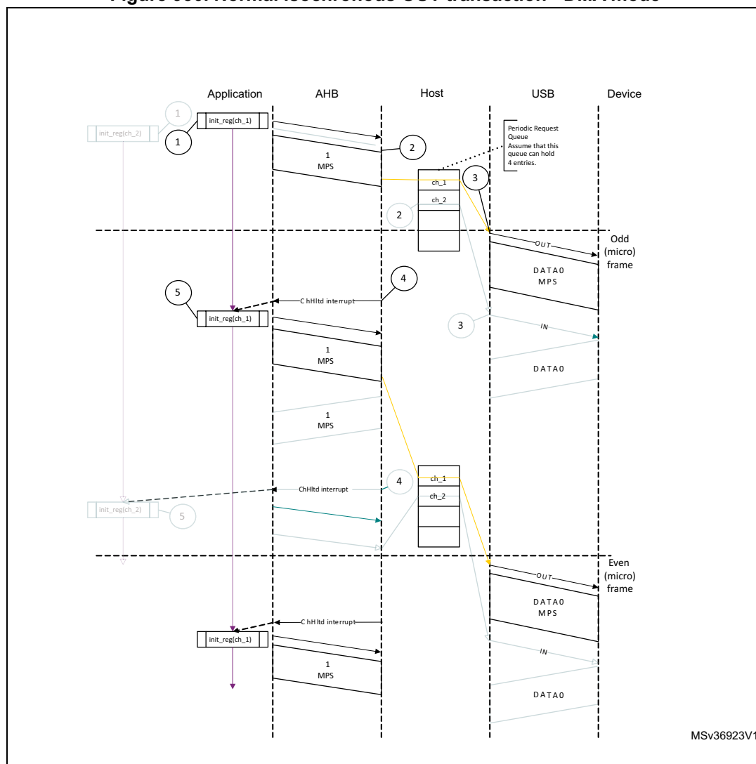
Figure 930. Normal isochronous OUT transaction - DMA mode
