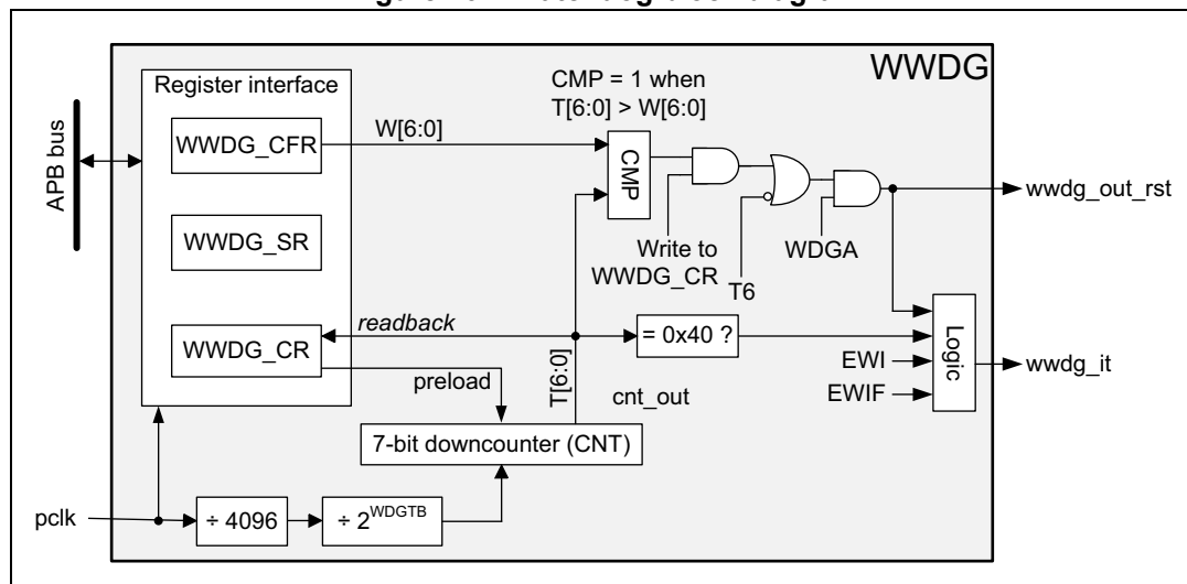
Figure 764. Watchdog block diagram
