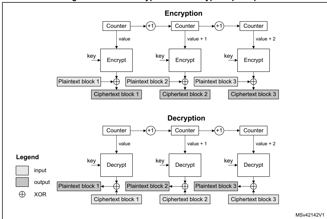
Figure 456. CTR encryption and decryption principle
