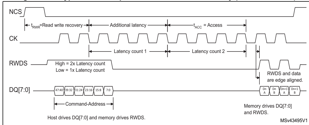
Figure 171. HyperBus read operation with additional latency (8-bit data mode)
