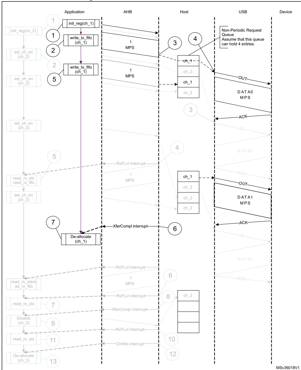
Figure 895. Normal bulk/control OUT/SETUP
