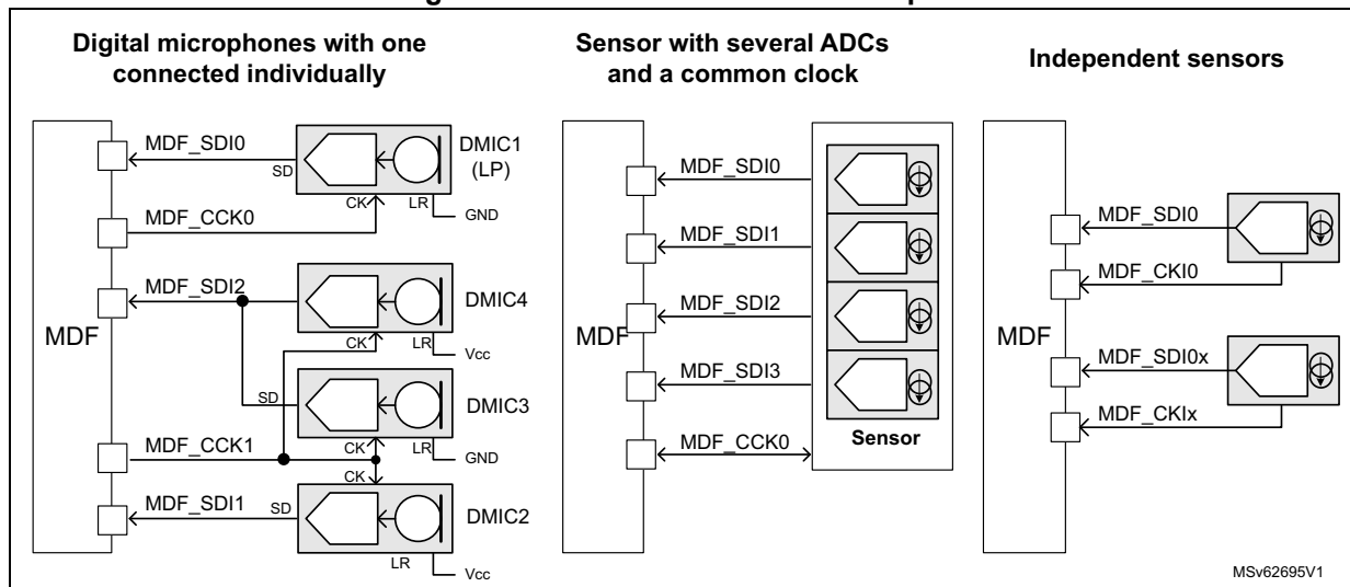
Figure 351. Sensor connection examples
