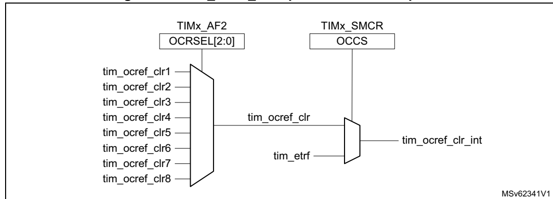
Figure 555. tim_ocref_clr input selection multiplexer
