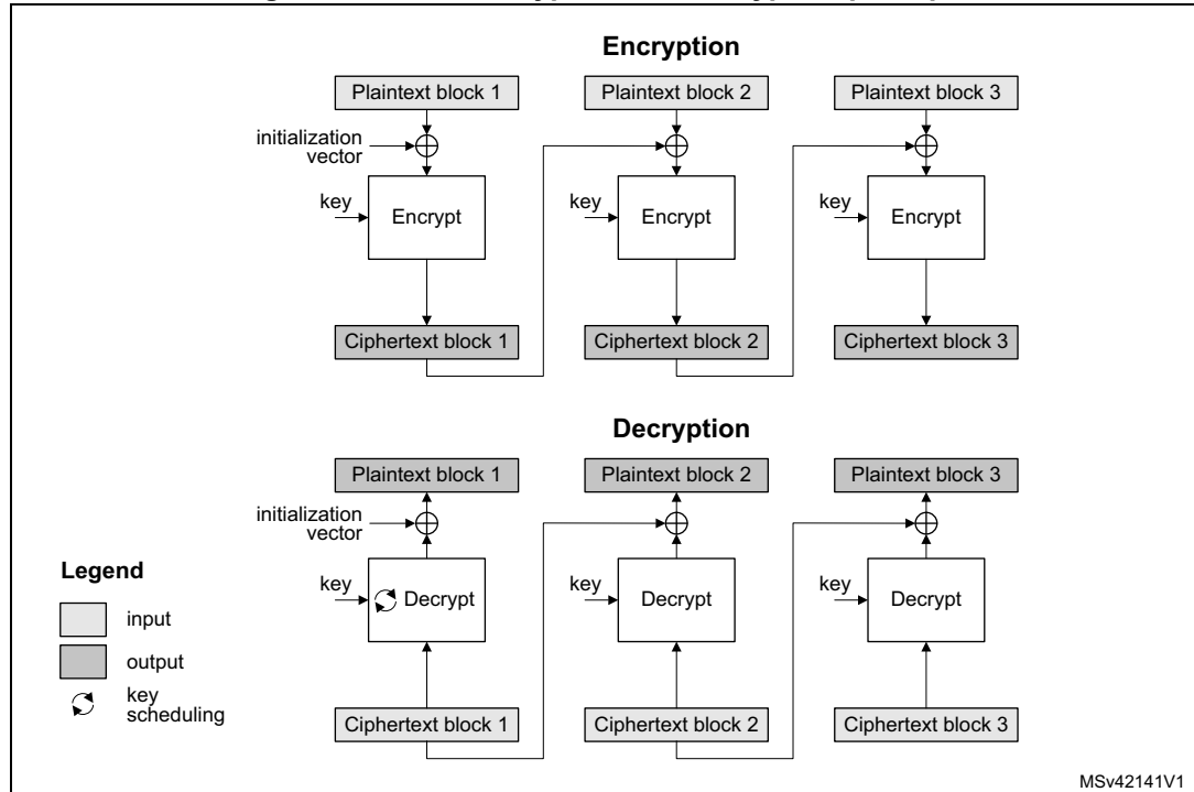
Figure 481. CBC encryption and decryption principle
