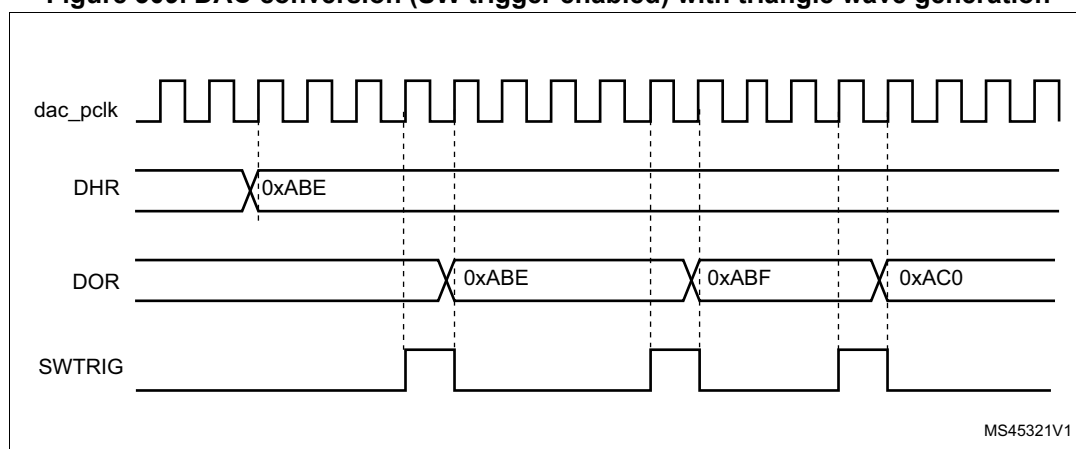
Figure 309. DAC conversion (SW trigger enabled) with triangle wave generation
