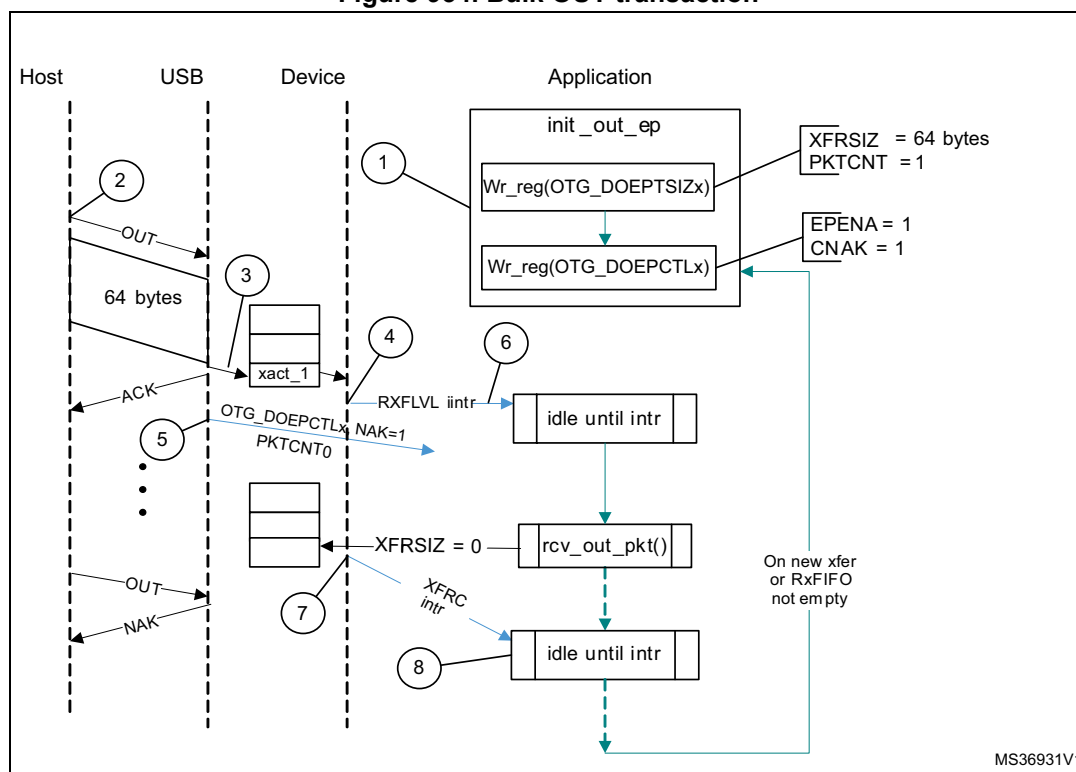
Figure 934. Bulk OUT transaction
