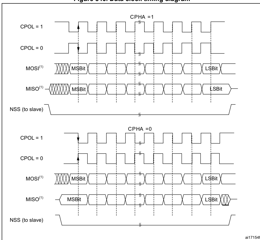
Figure 846. Data clock timing diagram
