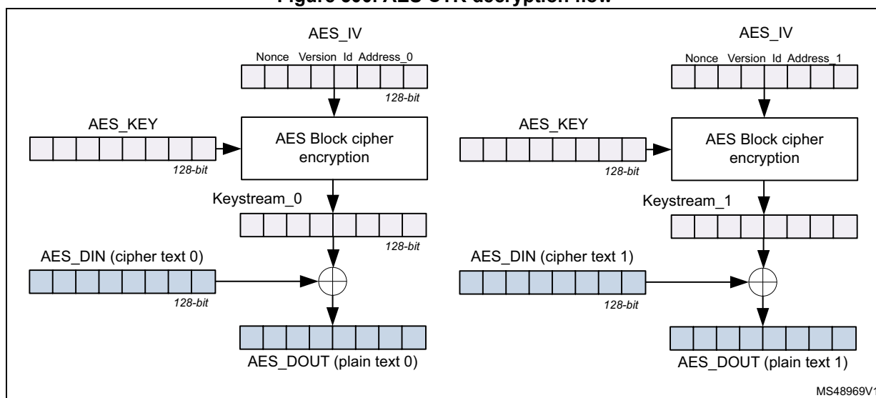
Figure 500. AES CTR decryption flow
