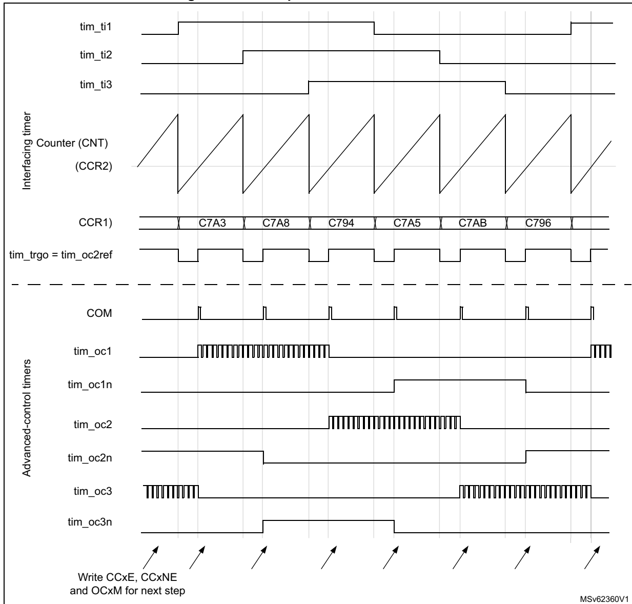
Figure 588. Example of Hall sensor interface
