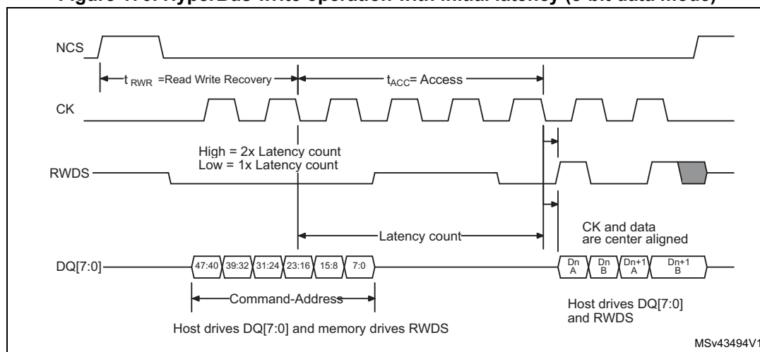
Figure 170. HyperBus write operation with initial latency (8-bit data mode)
