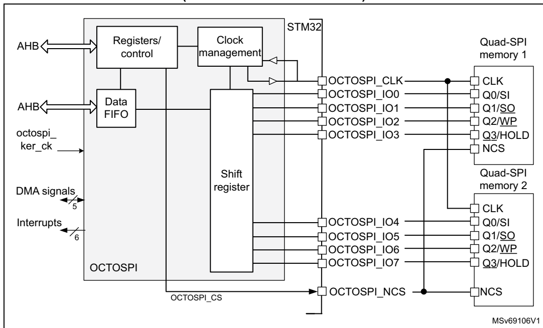
Figure 144. OCTOSPI block diagram in dual-quad configuration (for STM32U535/545 devices)
