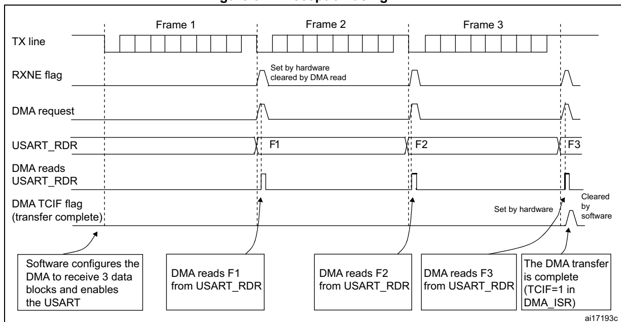
Figure 821. Reception using DMA
