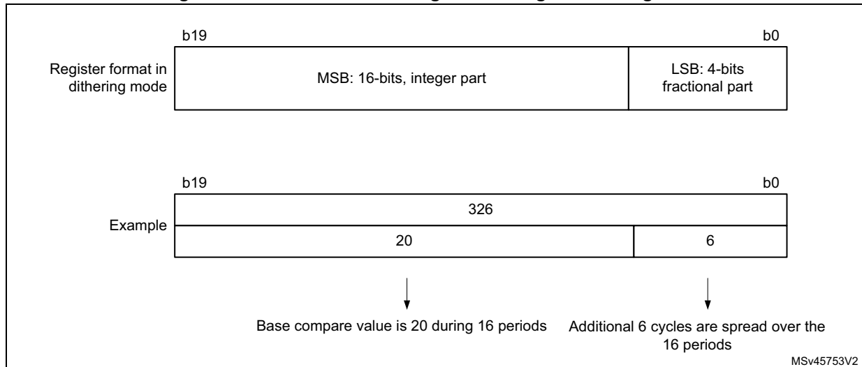
Figure 727. Data format and register coding in dithering mode
