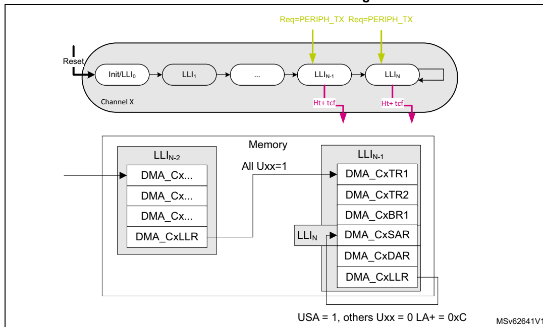
Figure 69. Shared GPDMA channel with circular buffering: update of the memory start address with a linear addressing channel
