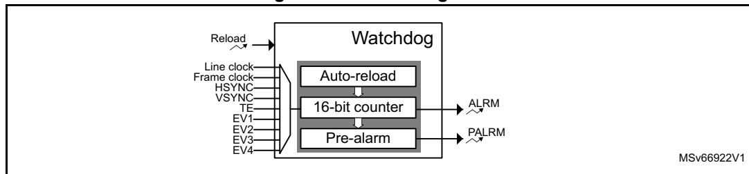
Figure 758. Watchdog timer
