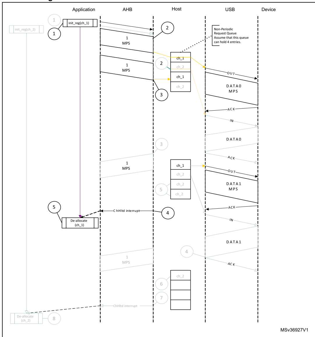
Figure 926. Normal bulk/control OUT/SETUP transactions - DMA
