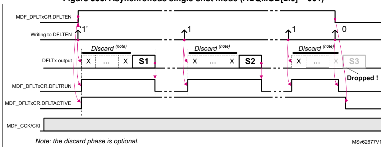
Figure 336. Asynchronous single-shot mode (ACQMOD[2:0] = 001)
