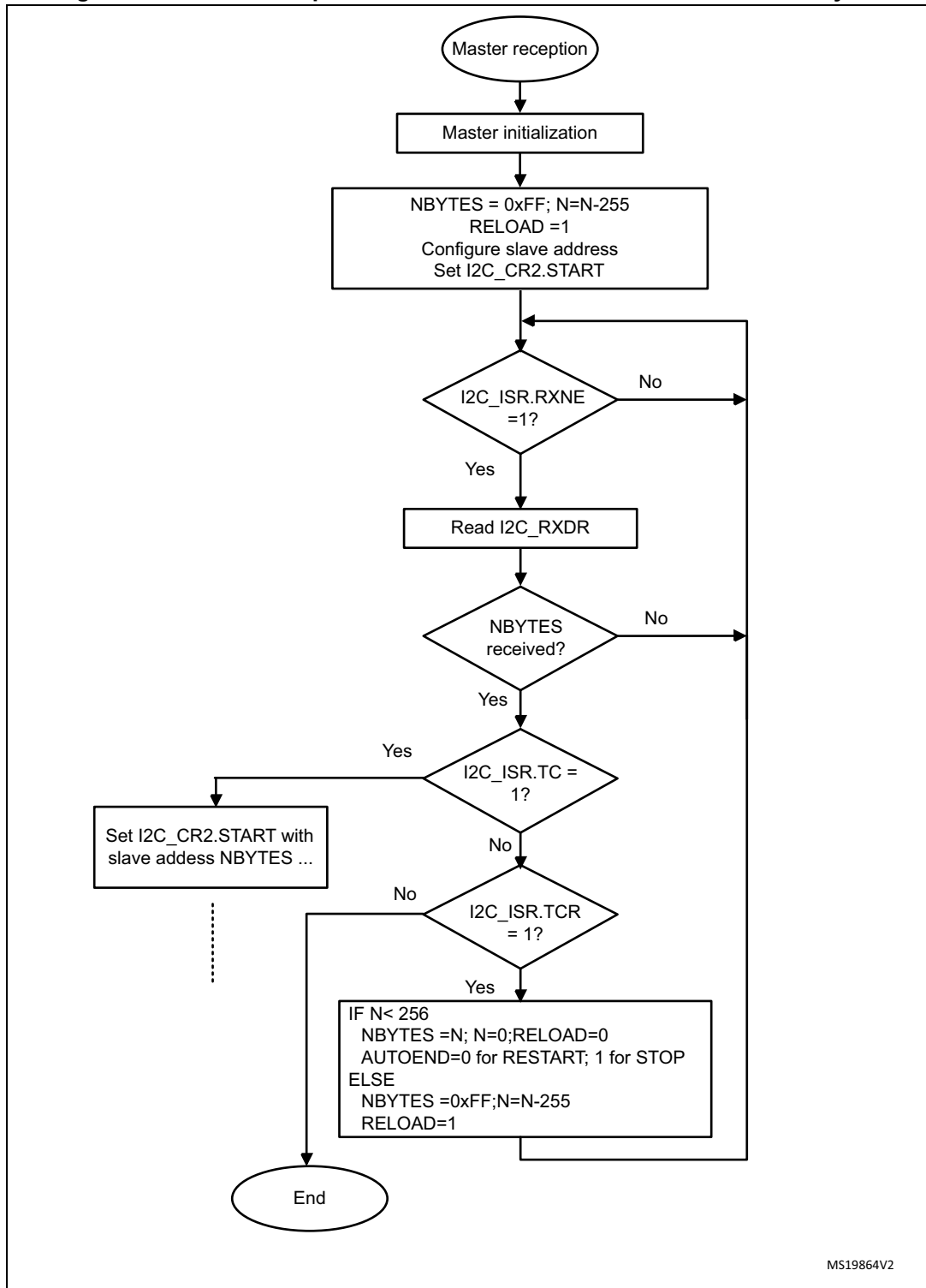
Figure 791. Transfer sequence flow for I2C master receiver for N > 255 bytes
