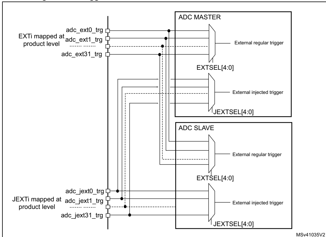
Figure 225. Triggers are shared between ADC master and ADC slave
