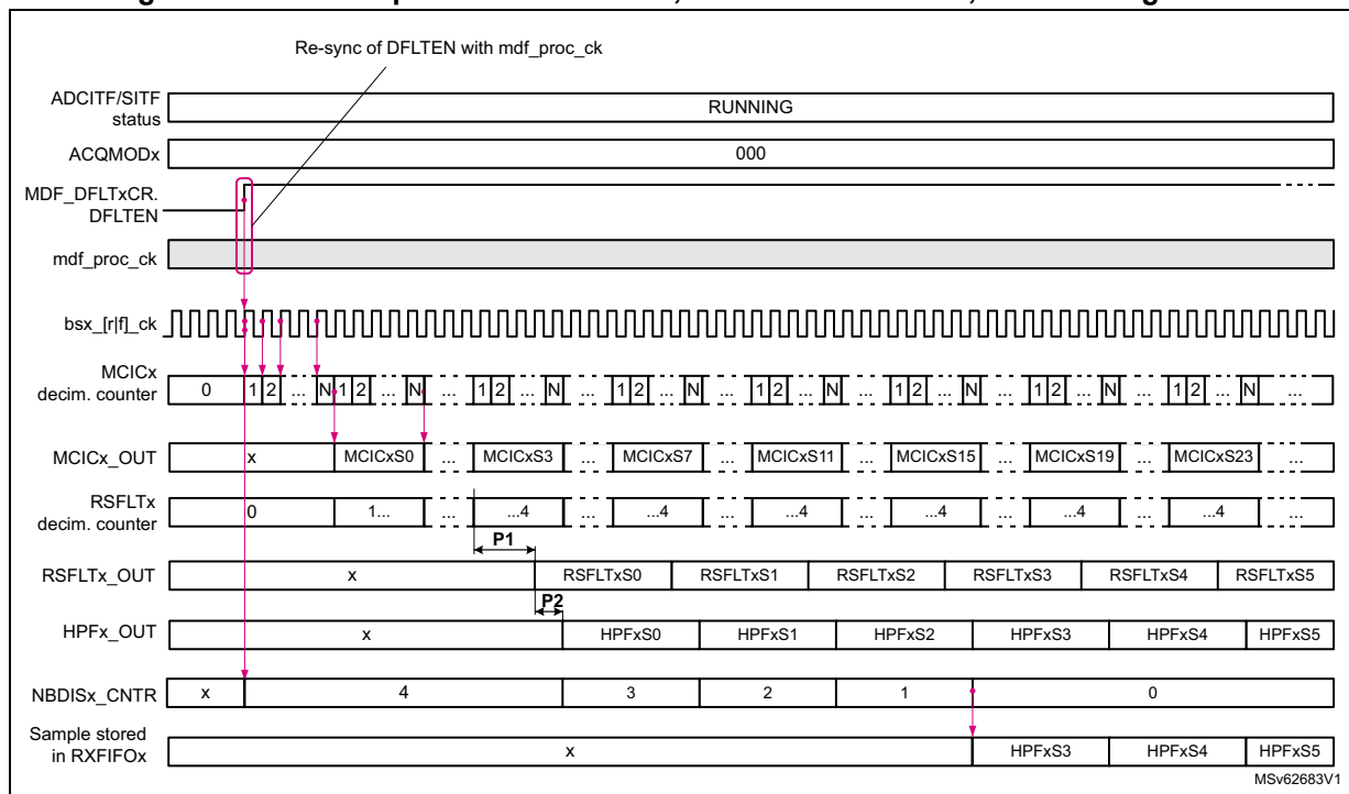
Figure 342. Start sequence with DFLTEN, in continuous mode, audio configuration
