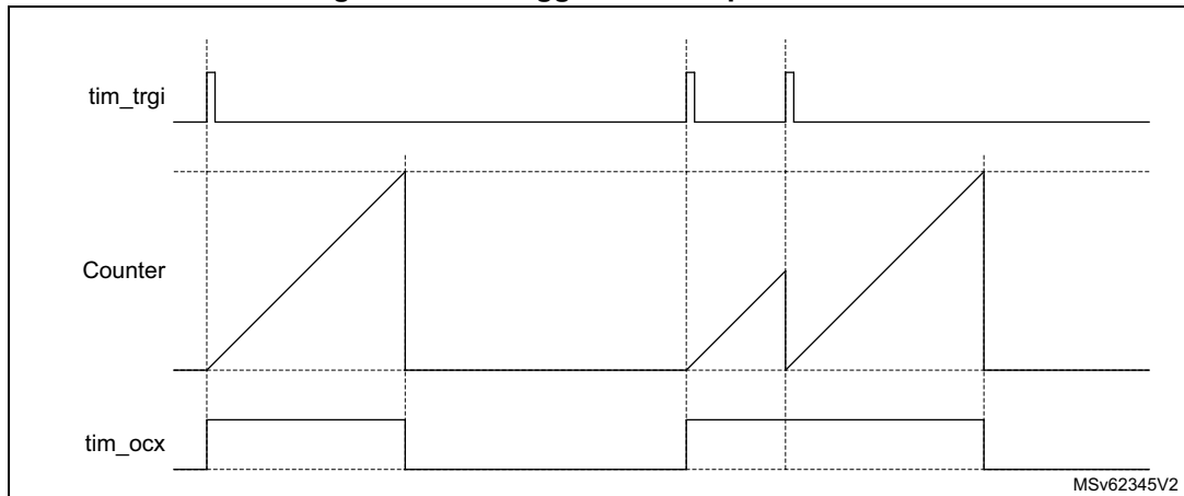
Figure 636. Retriggerable one-pulse mode
