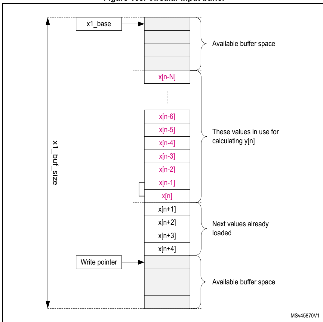
Figure 108. Circular input buffer
