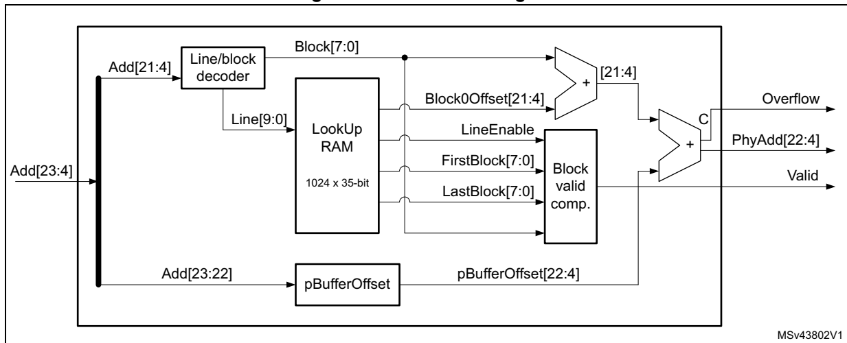
Figure 97. MMU block diagram
