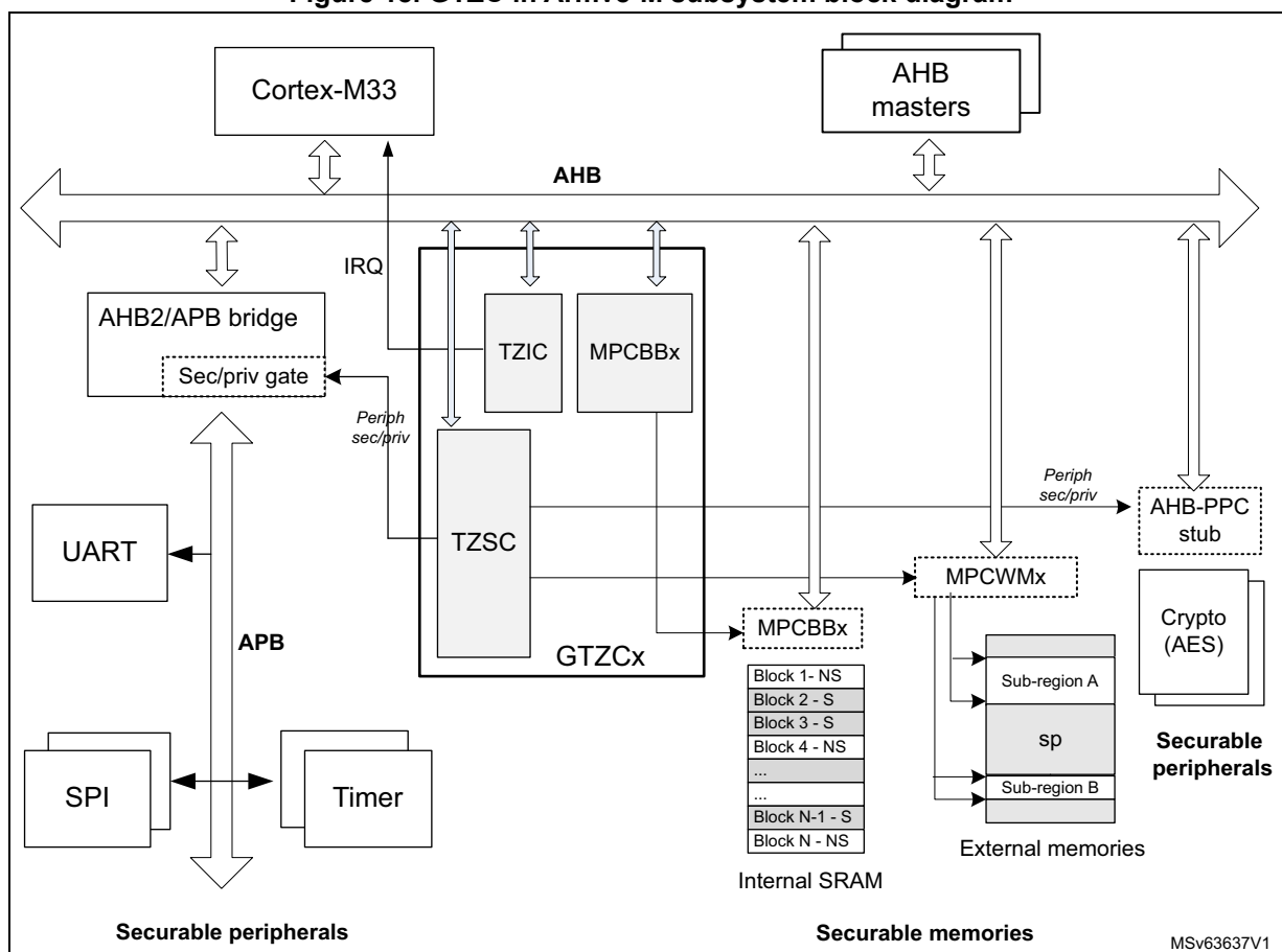
Figure 18. GTZC in Armv8-M subsystem block diagram
