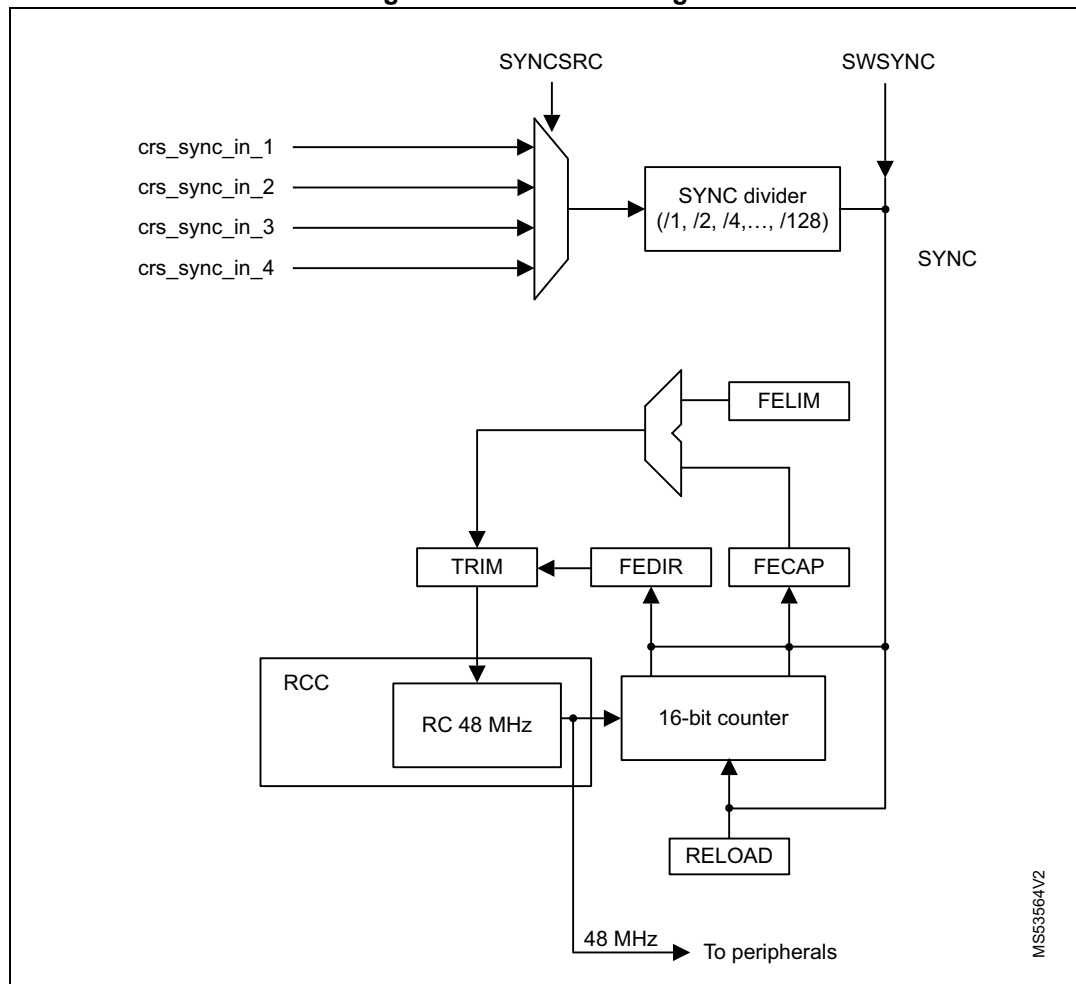
Figure 41. CRS block diagram
