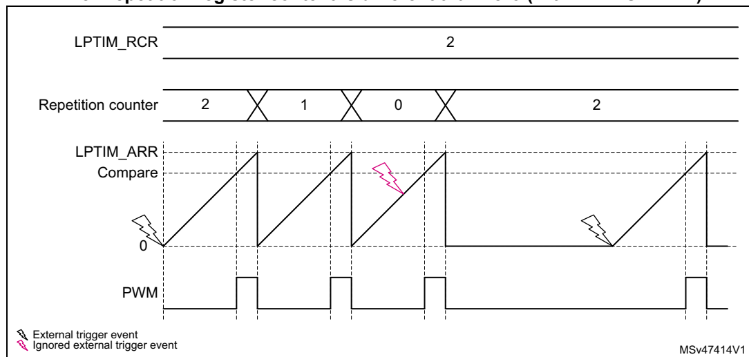
Figure 733. LPTIM output waveform, single counting mode configuration when repetition register content is different than zero (with PRELOAD = 1)
