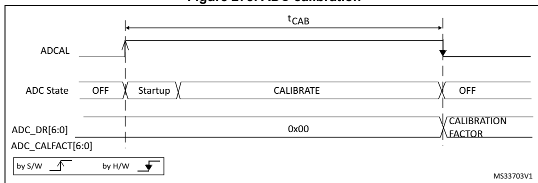
Figure 273. ADC calibration
