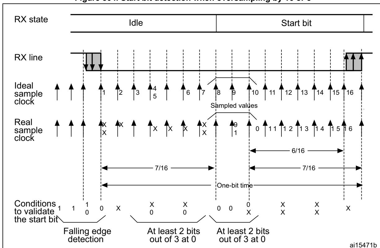
Figure 804. Start bit detection when oversampling by 16 or 8
