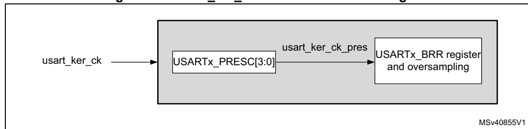
Figure 805. usart_ker_ck clock divider block diagram
