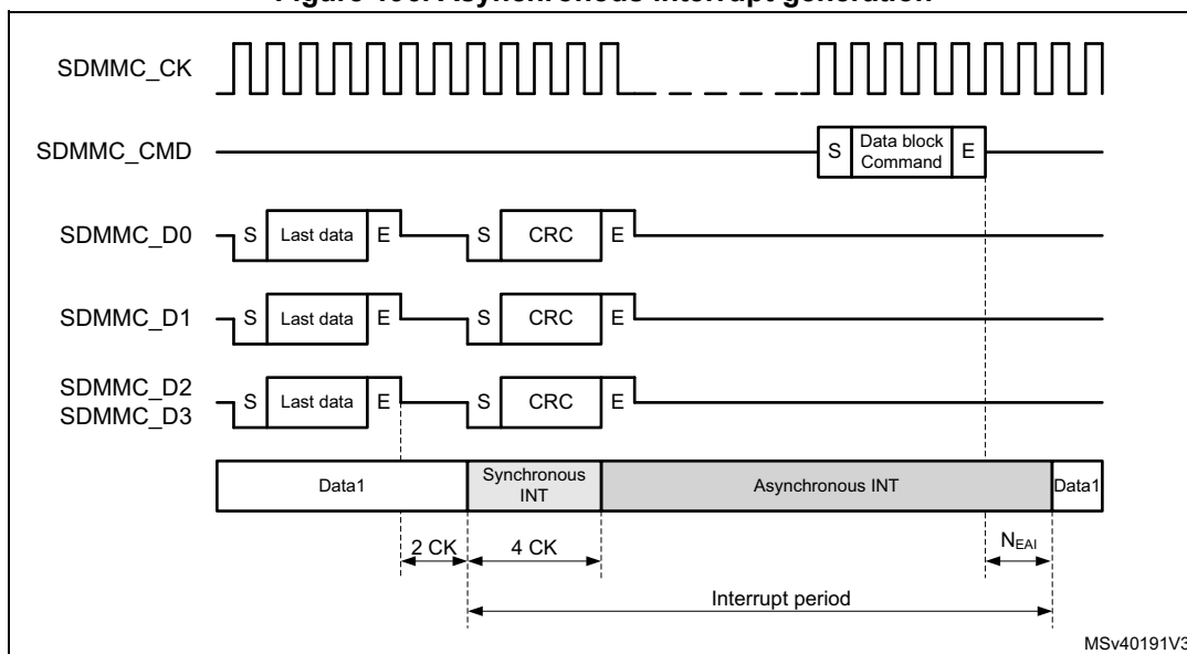
Figure 196. Asynchronous interrupt generation
