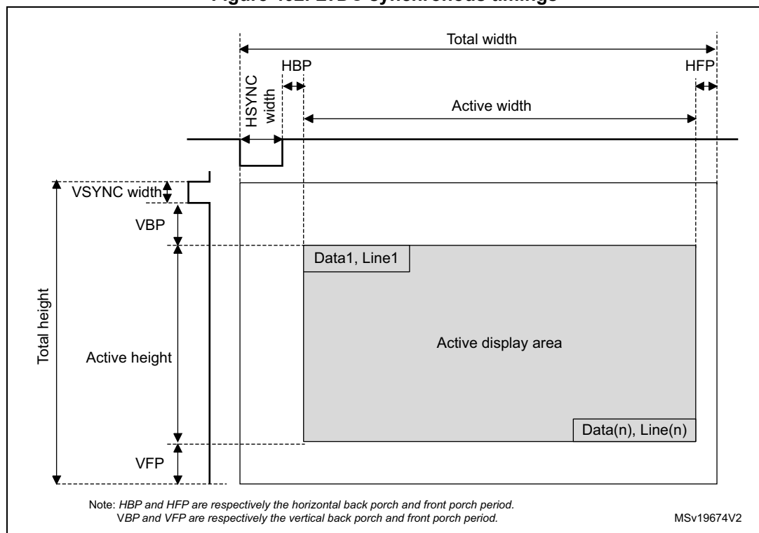
Figure 402. LTDC synchronous timings
