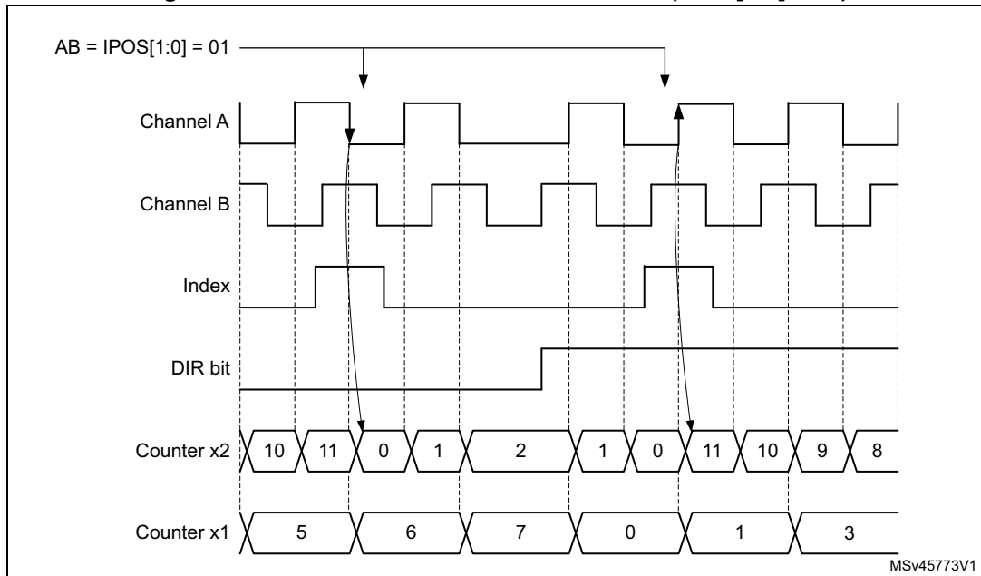
Figure 577. Index behavior in x1 and x2 mode (IPOS[1:0] = 01)
