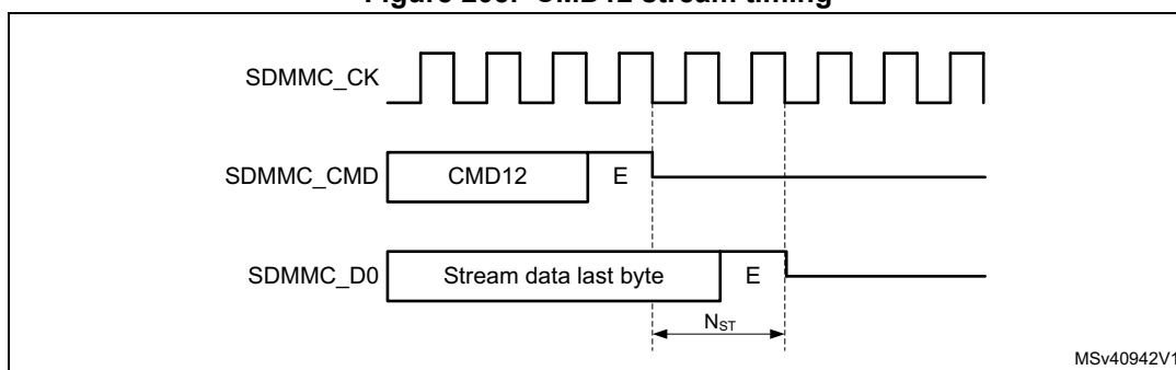
Figure 205. CMD12 stream timing
