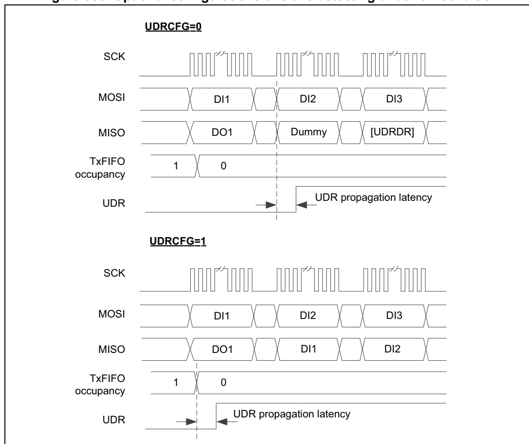
Figure 850. Optional configurations of slave detecting underrun condition
