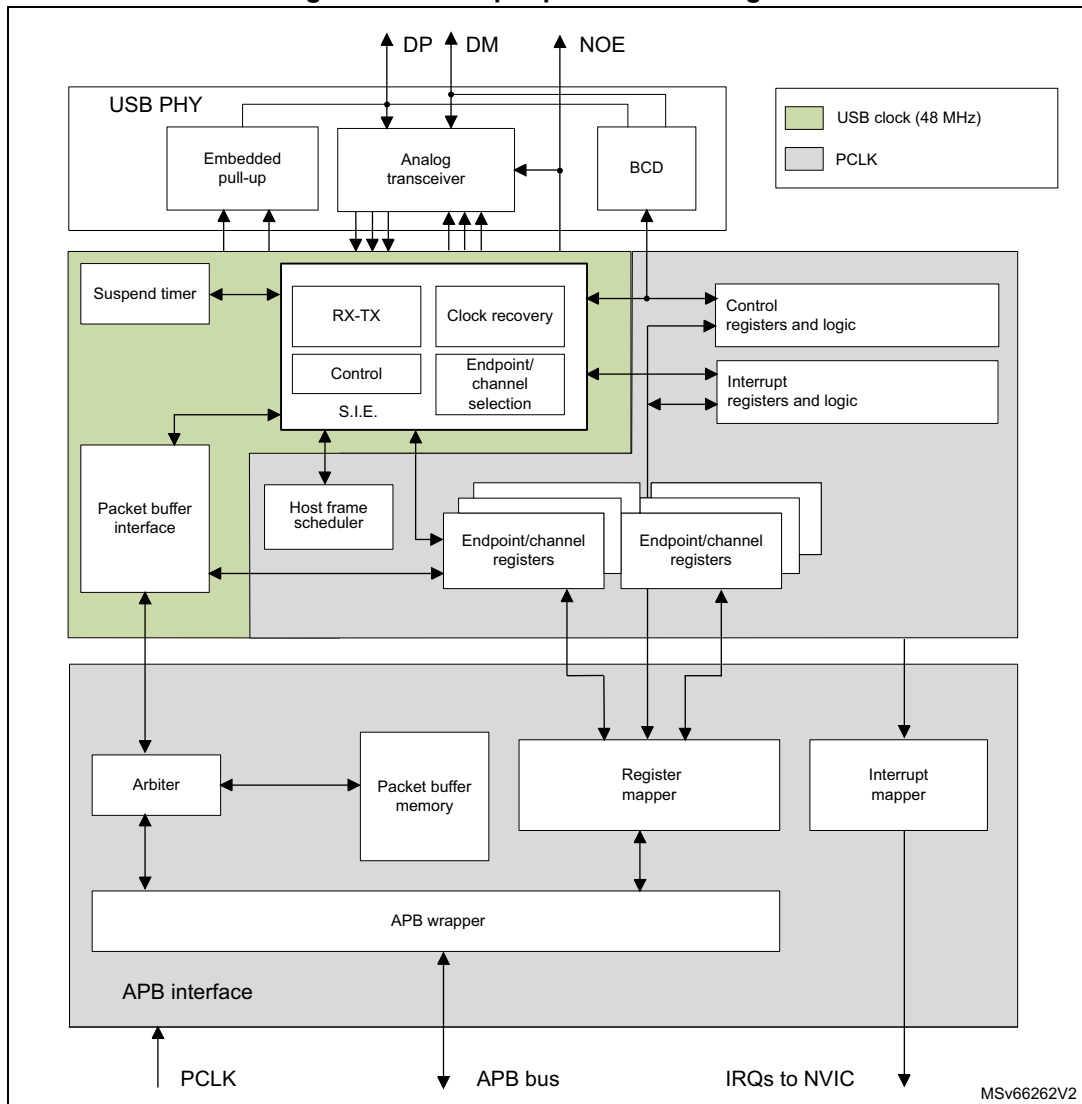
Figure 882. USB peripheral block diagram
