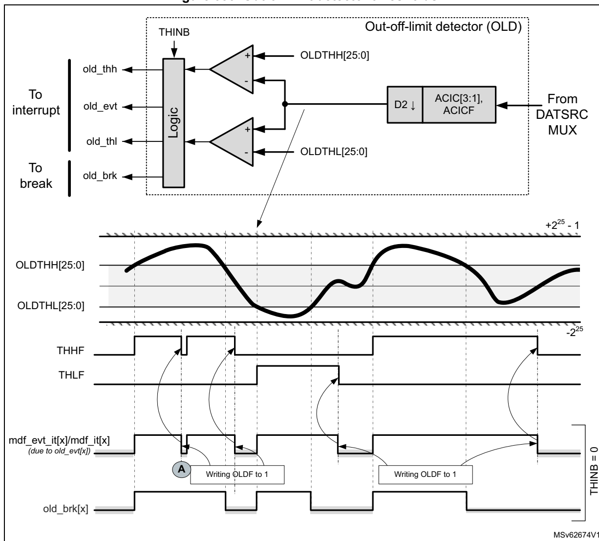
Figure 333. Out-of-limit detector thresholds
