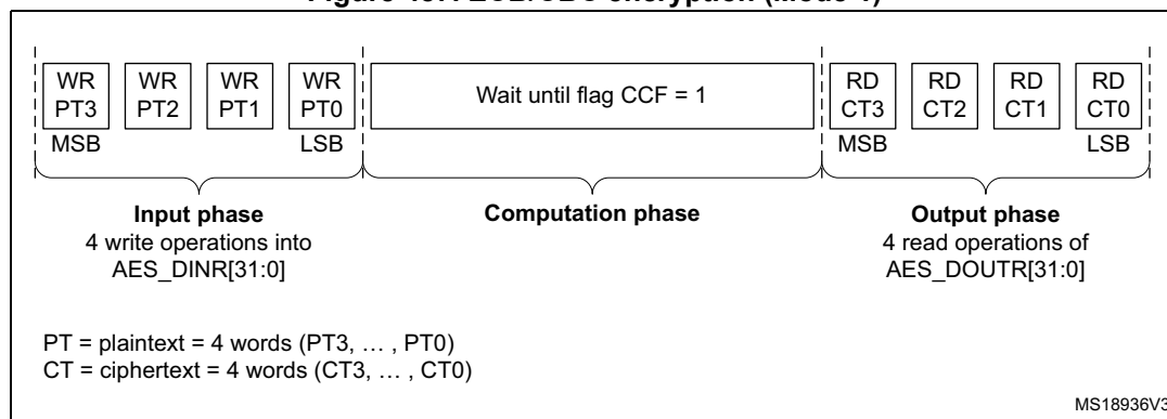
Figure 487. ECB/CBC encryption (Mode 1)
