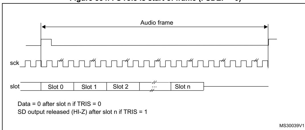
Figure 854. FS role is start of frame (FSDEF = 0)
