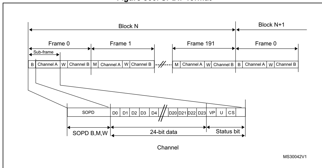
Figure 866. SPDIF format
