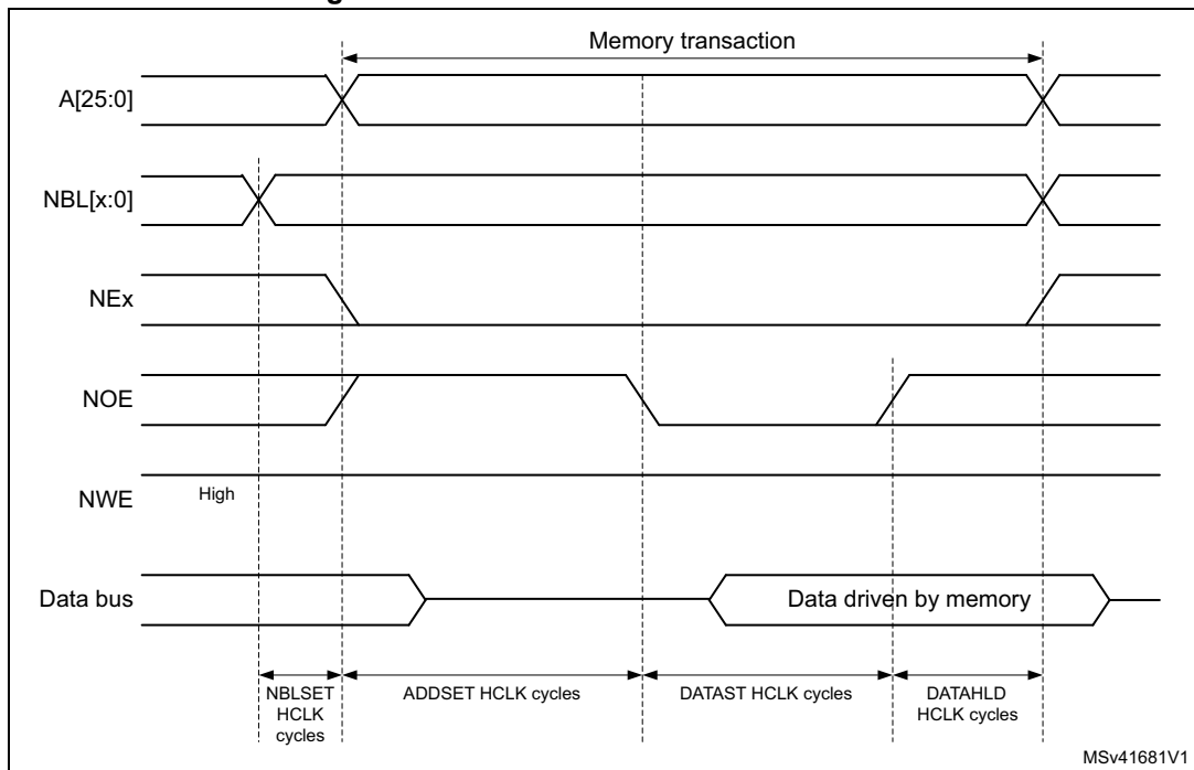
Figure 121. Mode A read access waveforms
