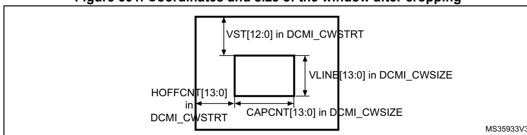
Figure 391. Coordinates and size of the window after cropping
