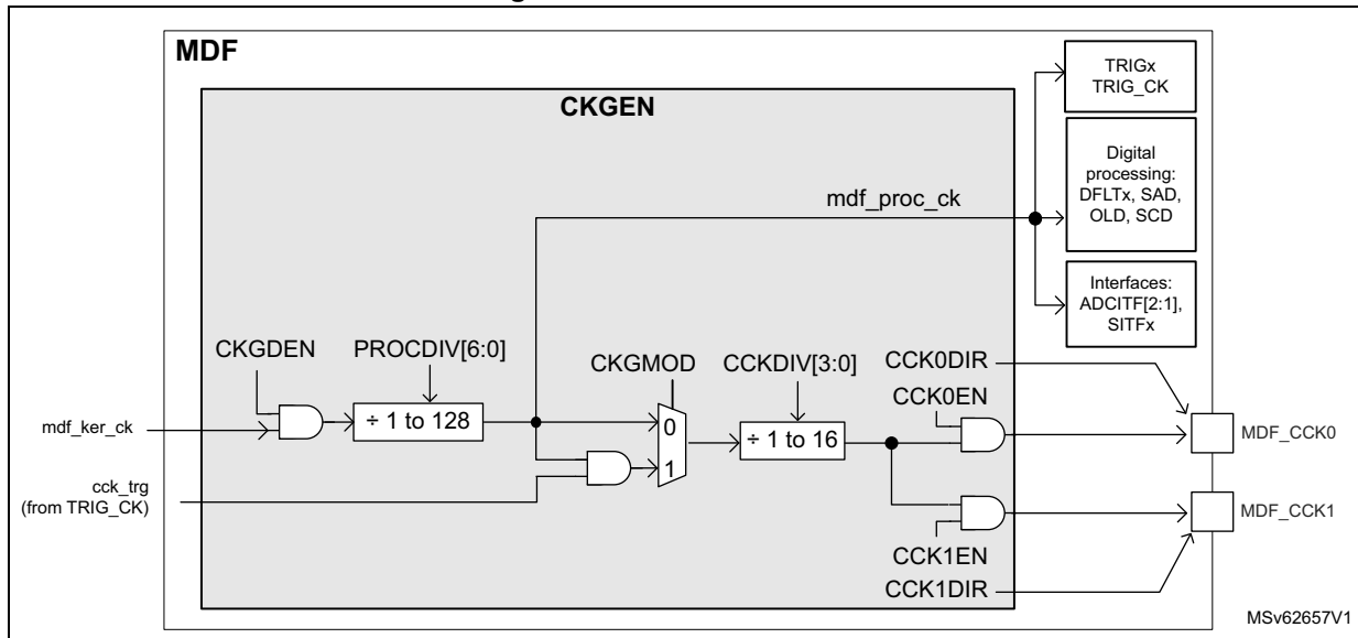
Figure 325. CKGEN overview
