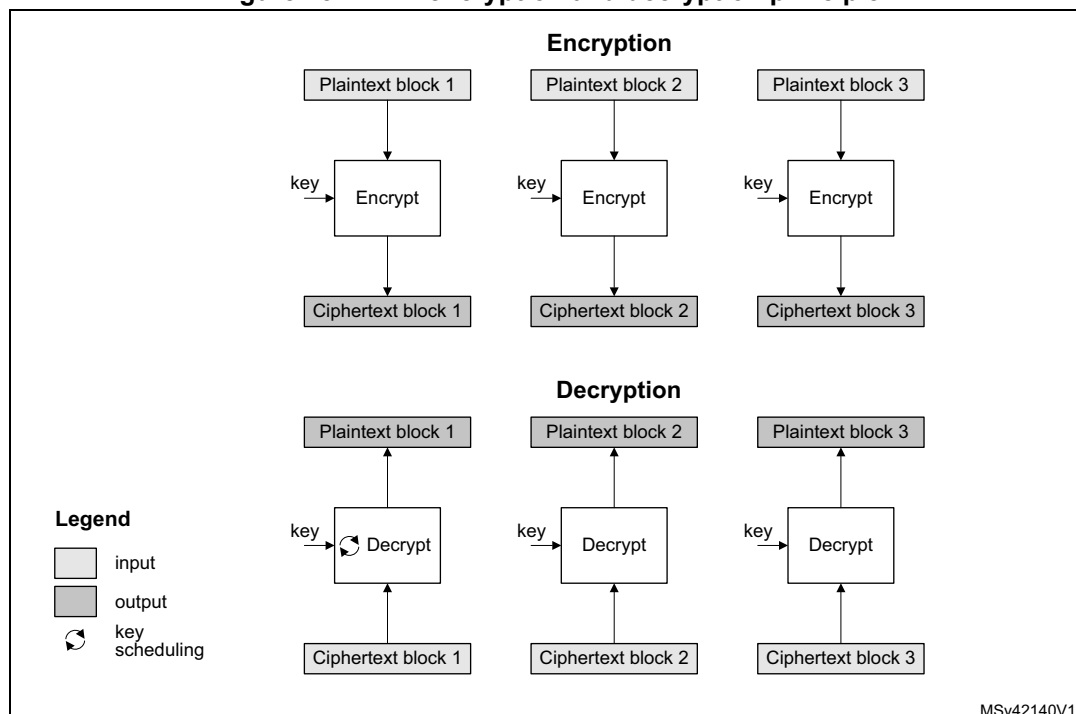
Figure 454. ECB encryption and decryption principle
