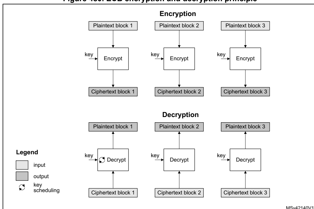
Figure 480. ECB encryption and decryption principle
