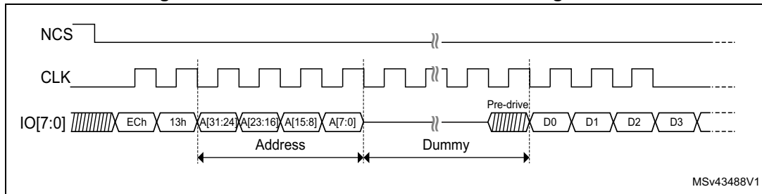
Figure 165. SDR read command in 16-bit configuration
