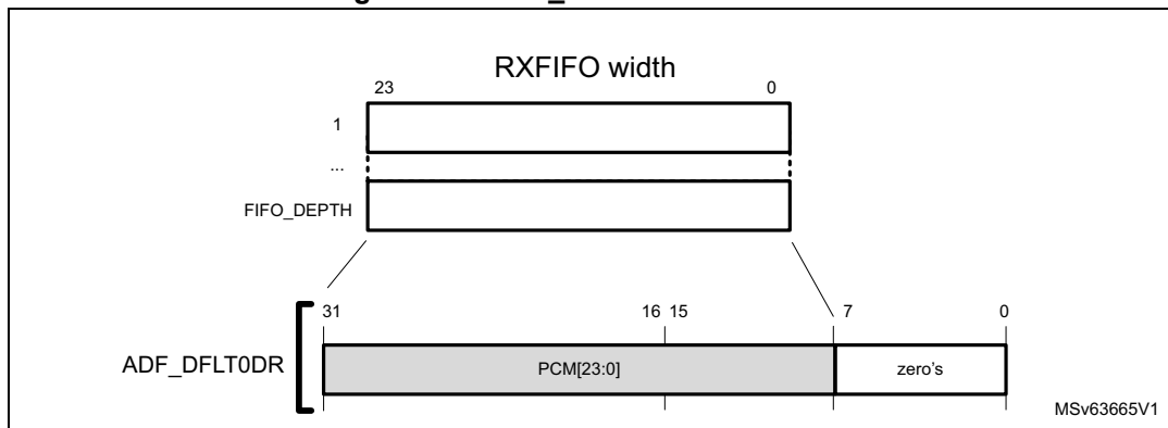
Figure 376. ADF_DFLTxDR data format
