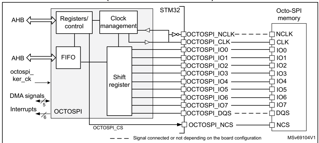
Figure 142. OCTOSPI block diagram in octal configuration (for STM32U535/545 devices)
