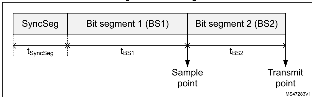
Figure 875. Bit timing
