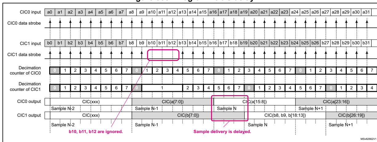
Figure 330. Programmable delay
