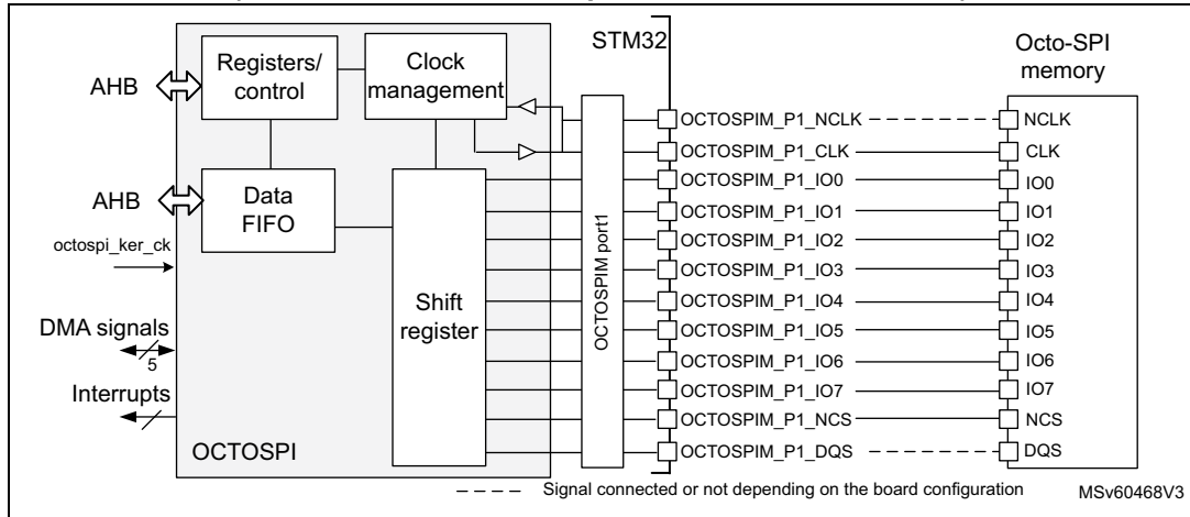
Figure 139. OCTOSPI block diagram in octal configuration (for STM32U5 series except STM32U535/545 devices)
