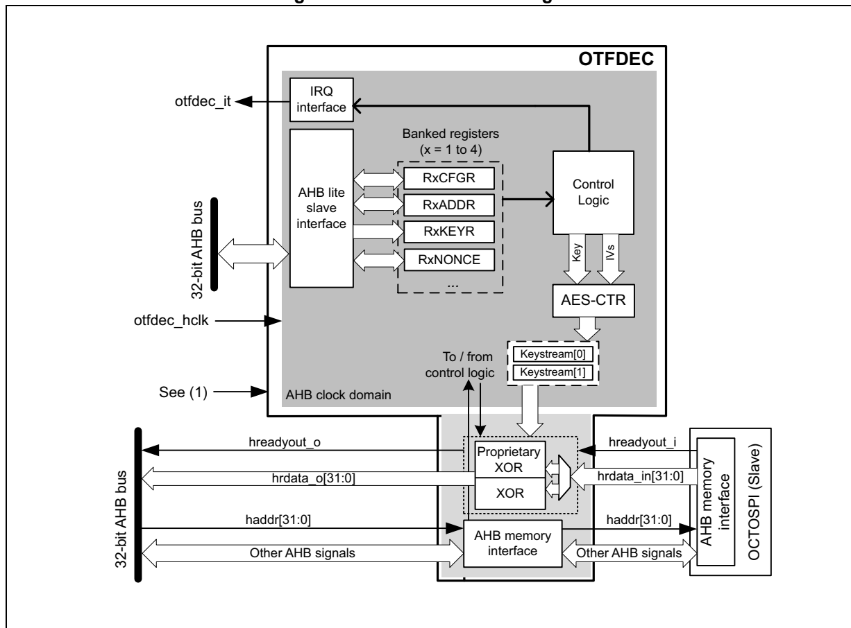
Figure 498. OTFDEC block diagram
