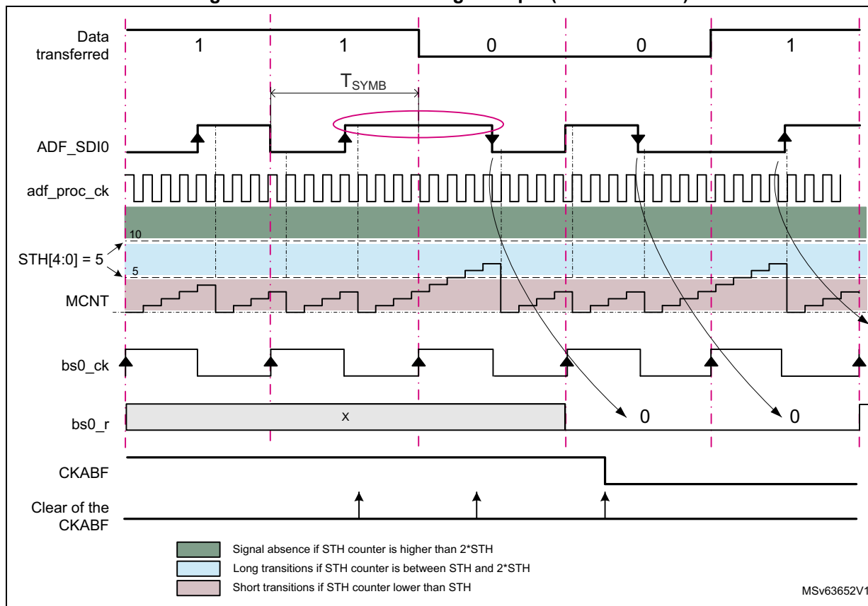
Figure 358. Manchester timing example (SITFMOD = 11)
