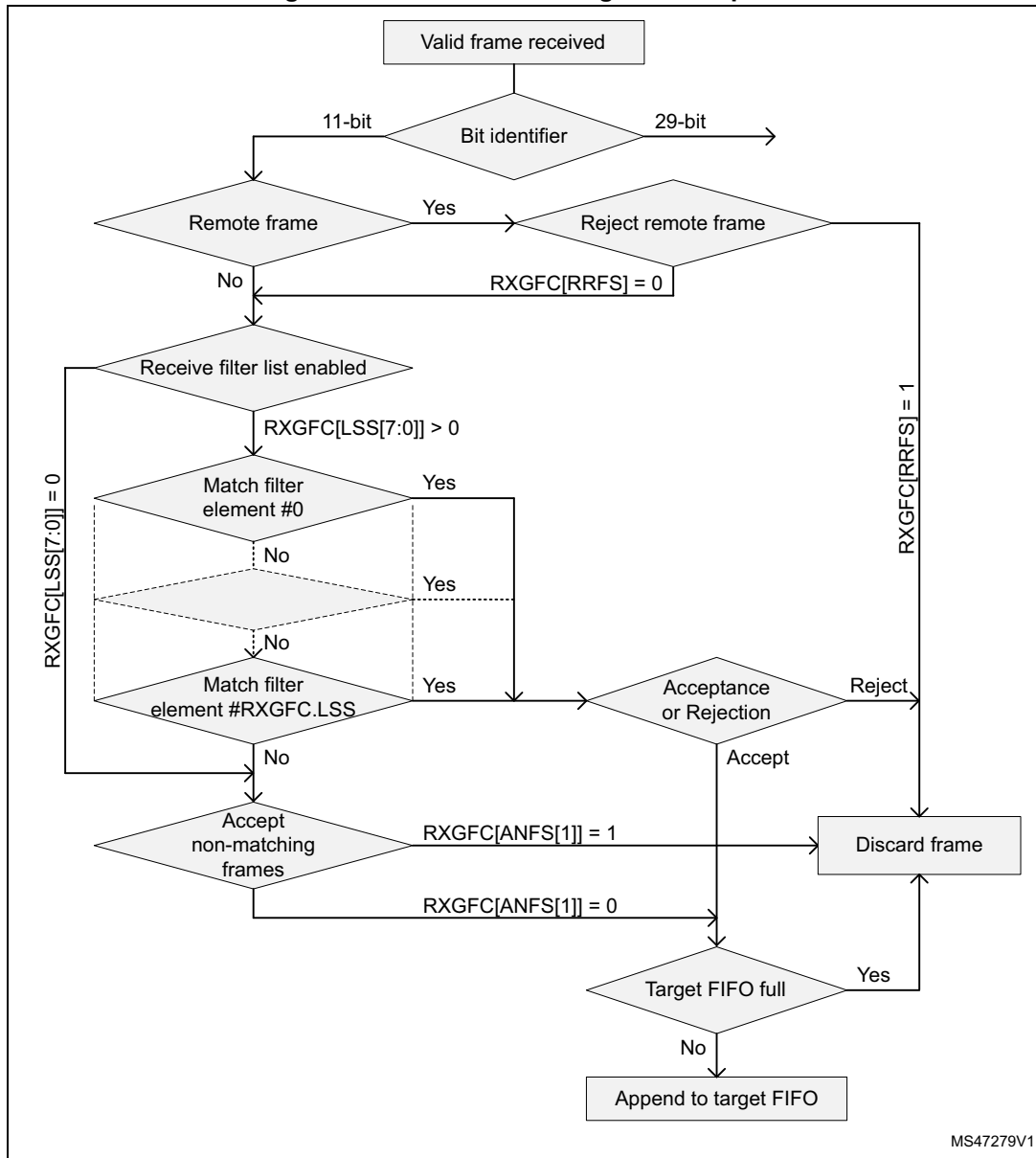
Figure 880. Standard Message ID filter path
