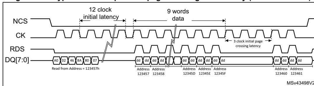
Figure 174. HyperBus read operation page crossing with latency (8-bit data mode)
