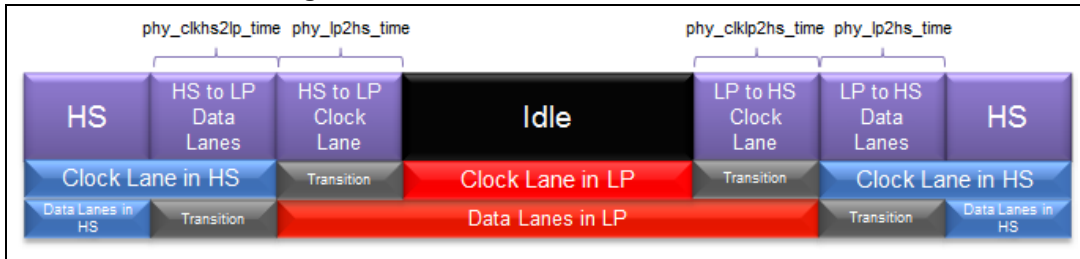
Figure 431. Clock lane and data lane in LP
