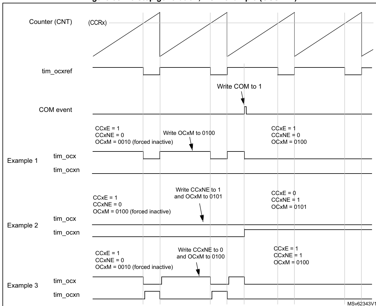
Figure 557. 6-step generation, COM example (OSSR=1)
