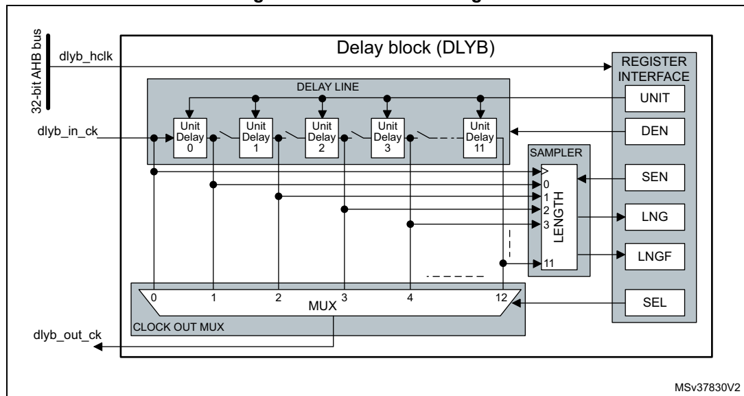
Figure 214. DLYB block diagram
