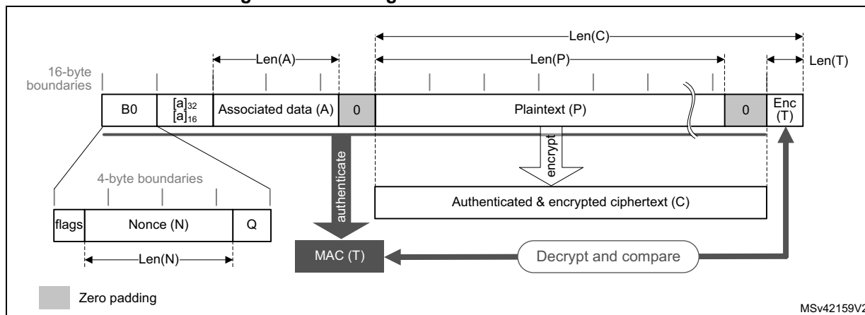
Figure 474. Message construction in CCM mode
