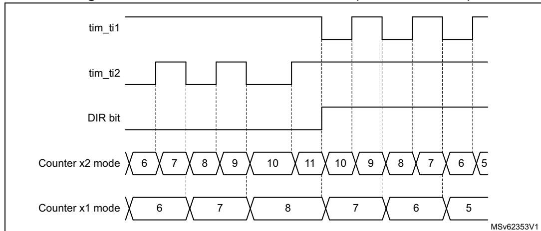
Figure 567. Directional clock encoder mode (CC1P = CC2P = 0)
