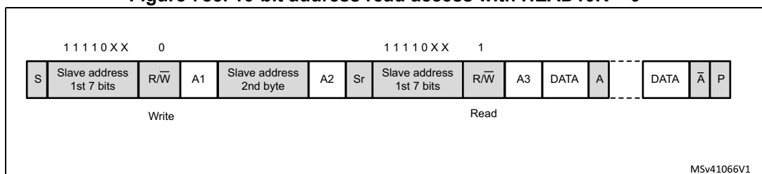
Figure 785. 10-bit address read access with HEAD10R = 0
