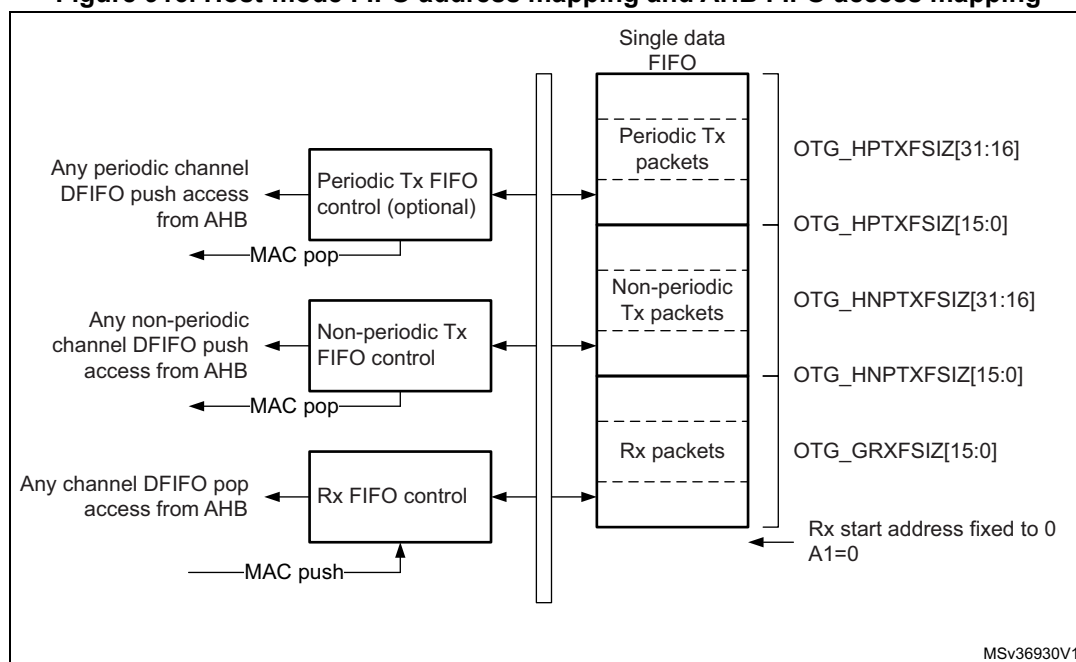
Figure 916. Host-mode FIFO address mapping and AHB FIFO access mapping
