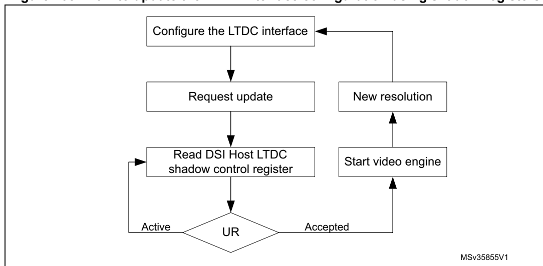
Figure 408. Flow to update the LTDC interface configuration using shadow registers
