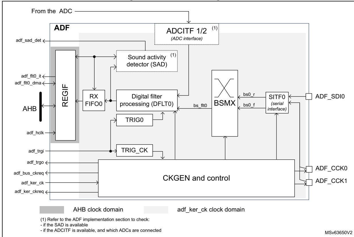
Figure 355. ADF block diagram
