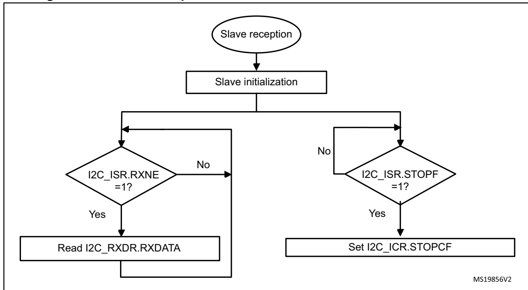
Figure 782. Transfer bus diagrams for I2C slave receiver (mandatory events only)
