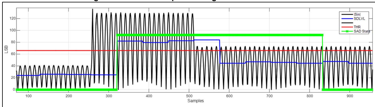
Figure 384. SAD example working with SADM0D = 01
