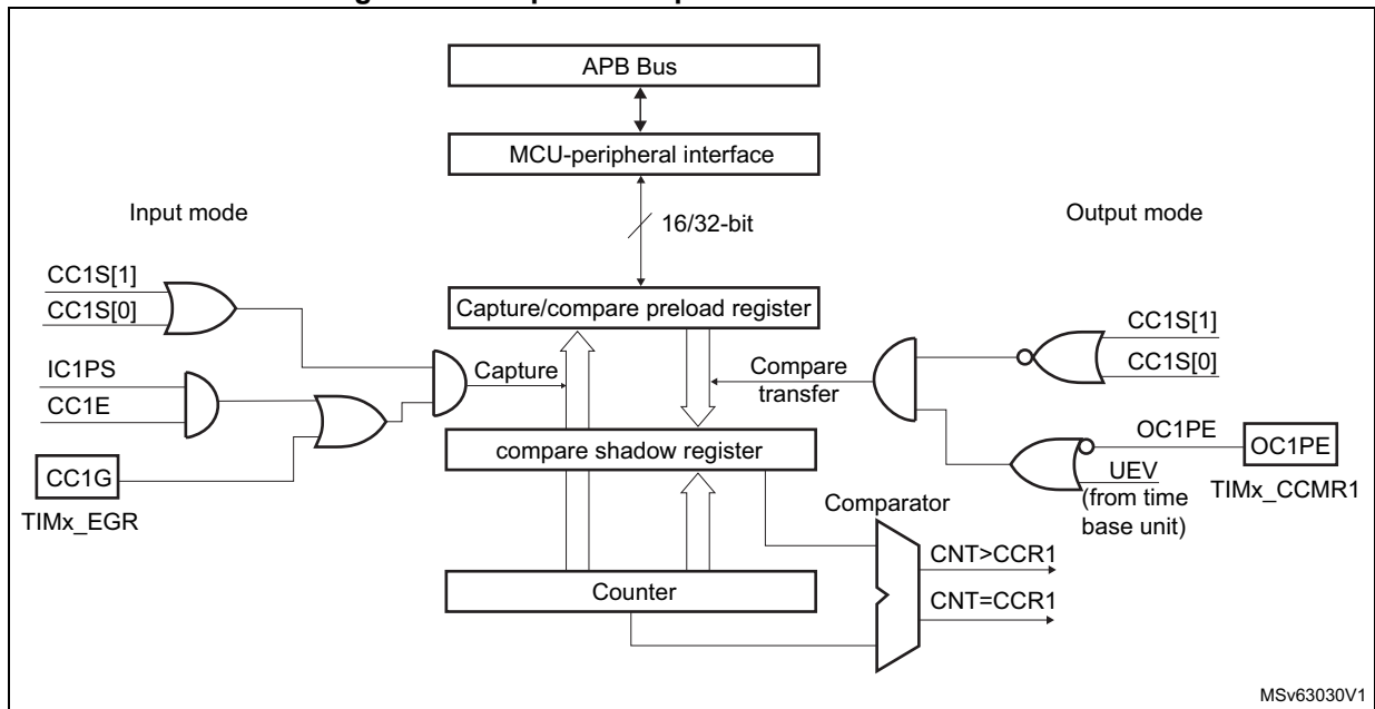
Figure 690. Capture/compare channel 1 main circuit
