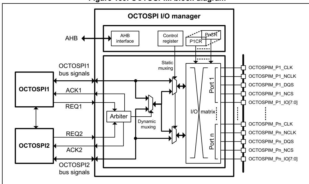
Figure 159. OCTOSPIM block diagram
