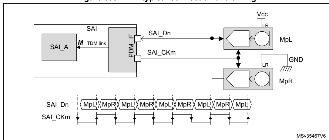
Figure 858. PDM typical connection and timing
