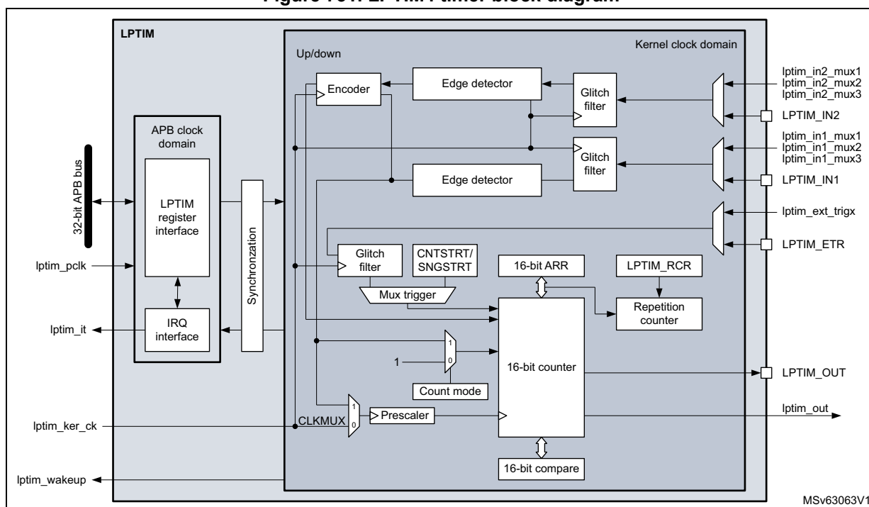
Figure 731. LPTIM4 timer block diagram
