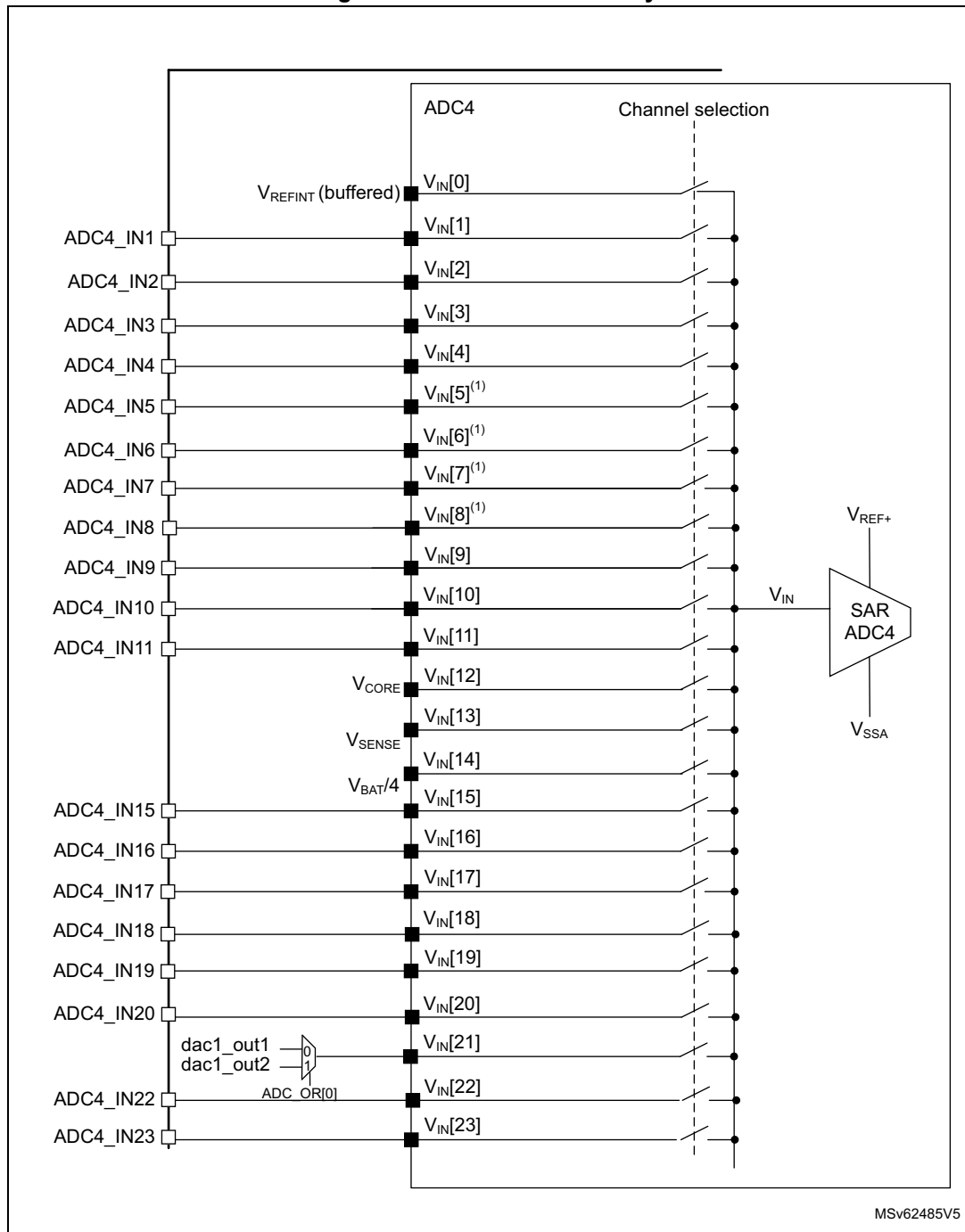
Figure 277. ADC4 connectivity
