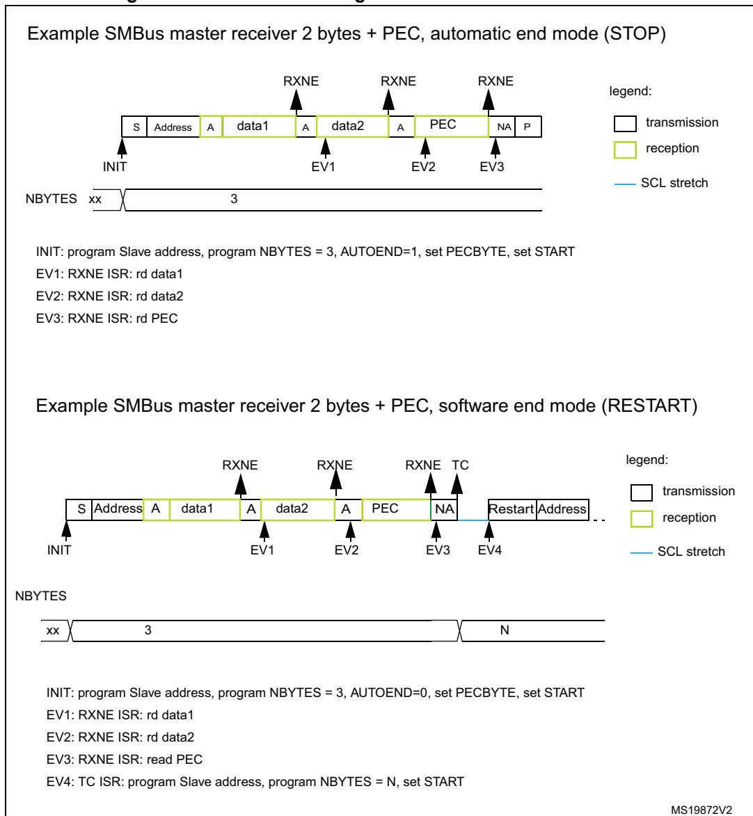
Figure 799. Bus transfer diagrams for SMBus master receiver
