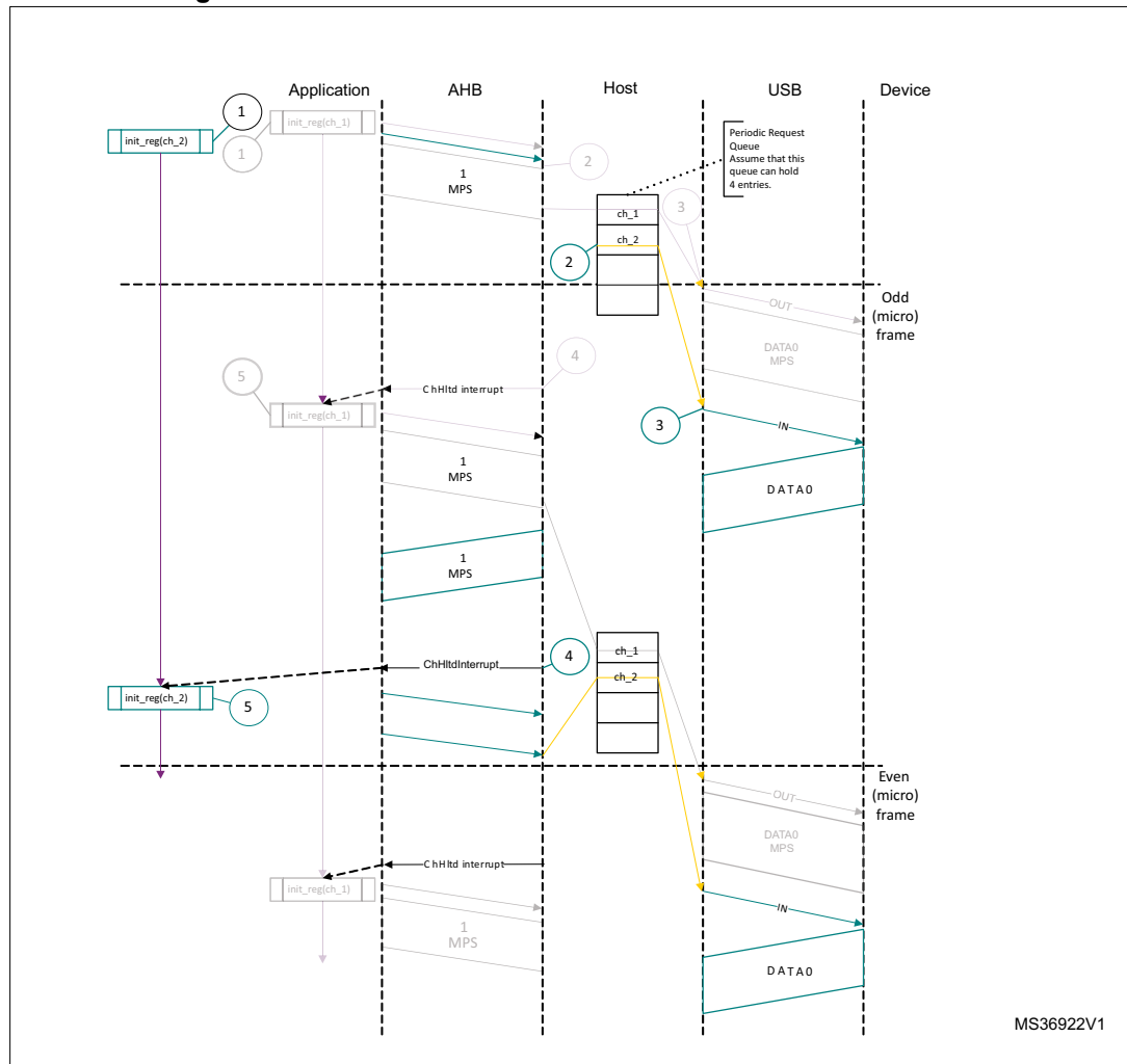
Figure 931. Normal isochronous IN transactions - DMA mode
