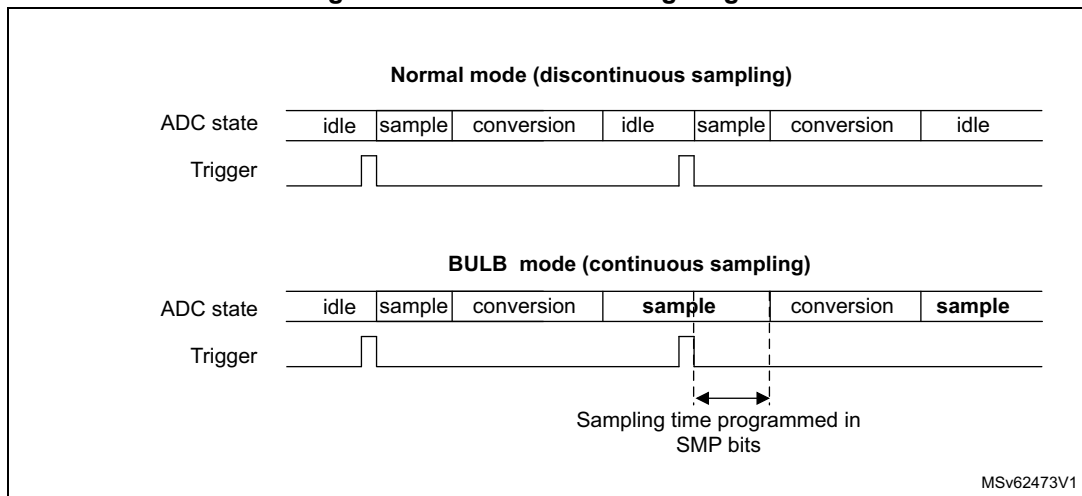
Figure 221. Bulb mode timing diagram
