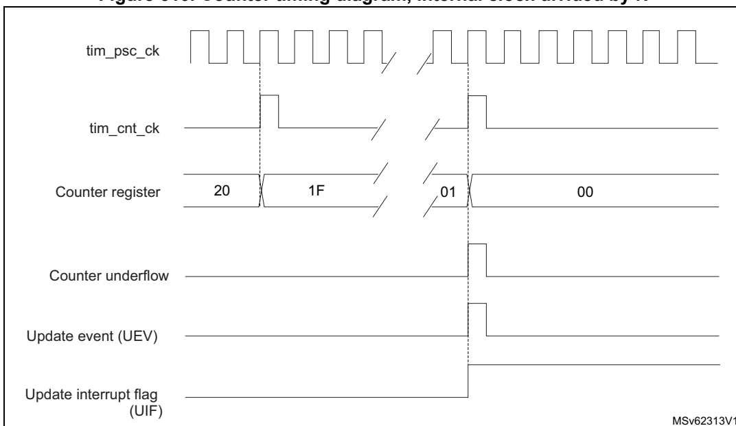
Figure 610. Counter timing diagram, internal clock divided by N
