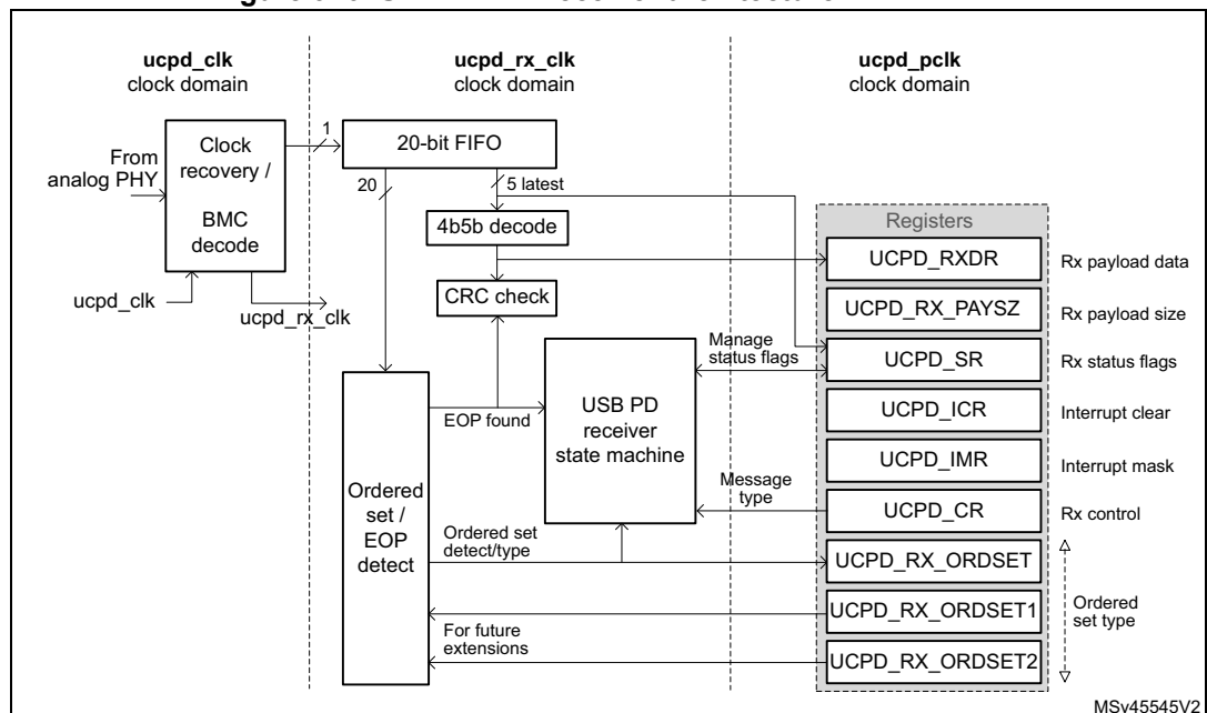
Figure 946. UCPD BMC receiver architecture
