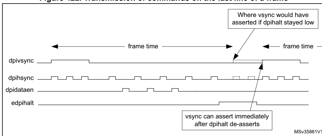
Figure 422. Transmission of commands on the last line of a frame
