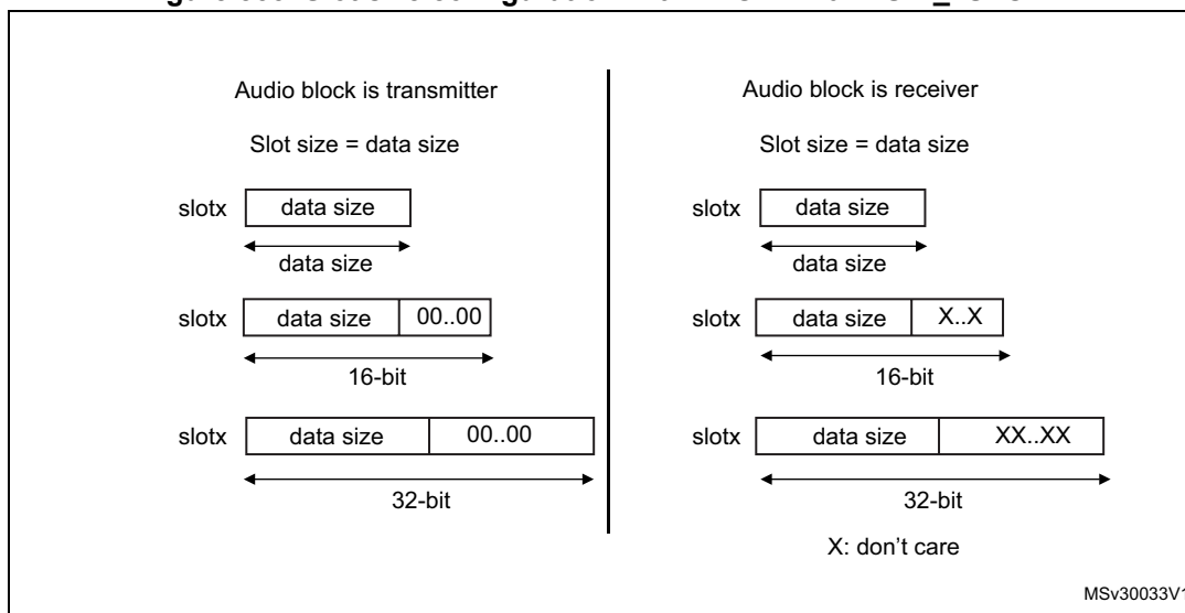
Figure 855. Slot size configuration with FBOFF = 0 in SAI_xSLOTR
