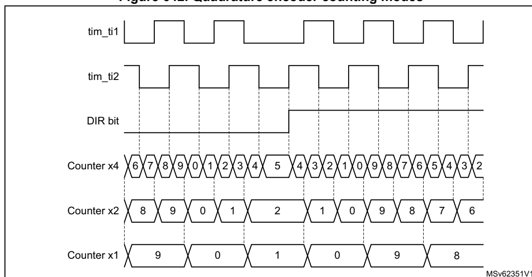
Figure 642. Quadrature encoder counting modes
