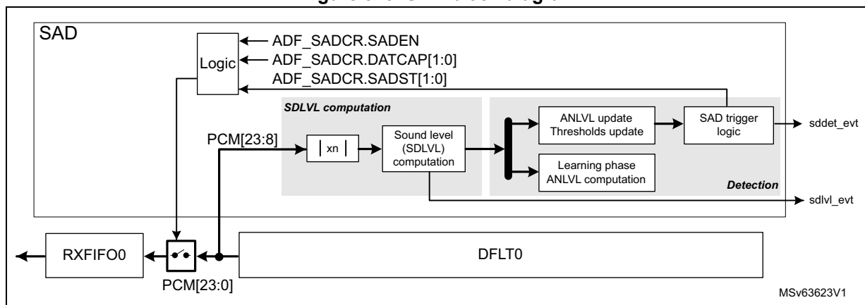
Figure 373. SAD block diagram
