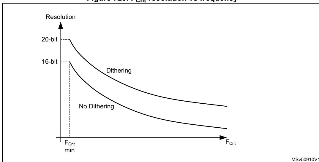
Figure 728. F Cnt resolution vs frequency
