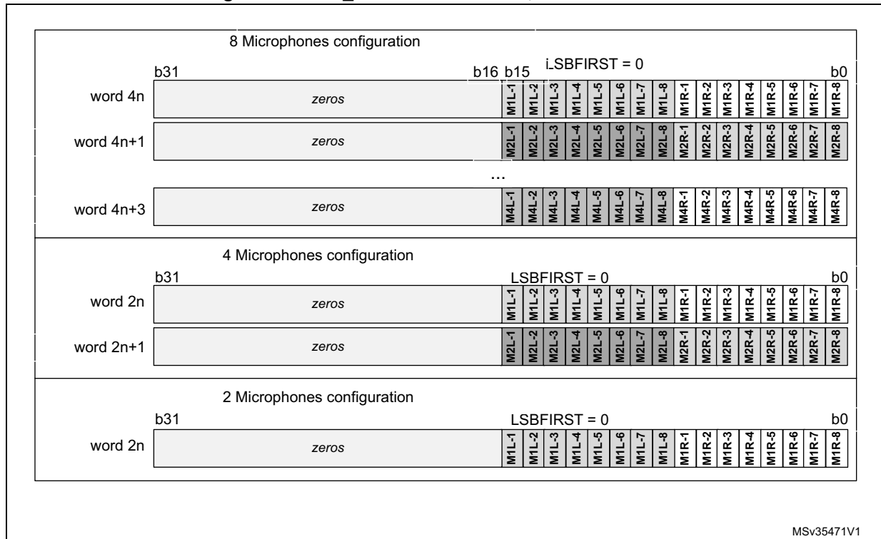
Figure 862. SAI_ADR format in TDM, 16-bit slot width
