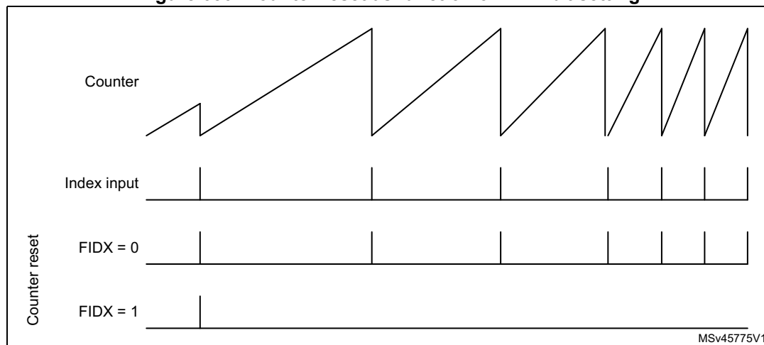
Figure 656. Counter reset as function of FIDX bit setting
