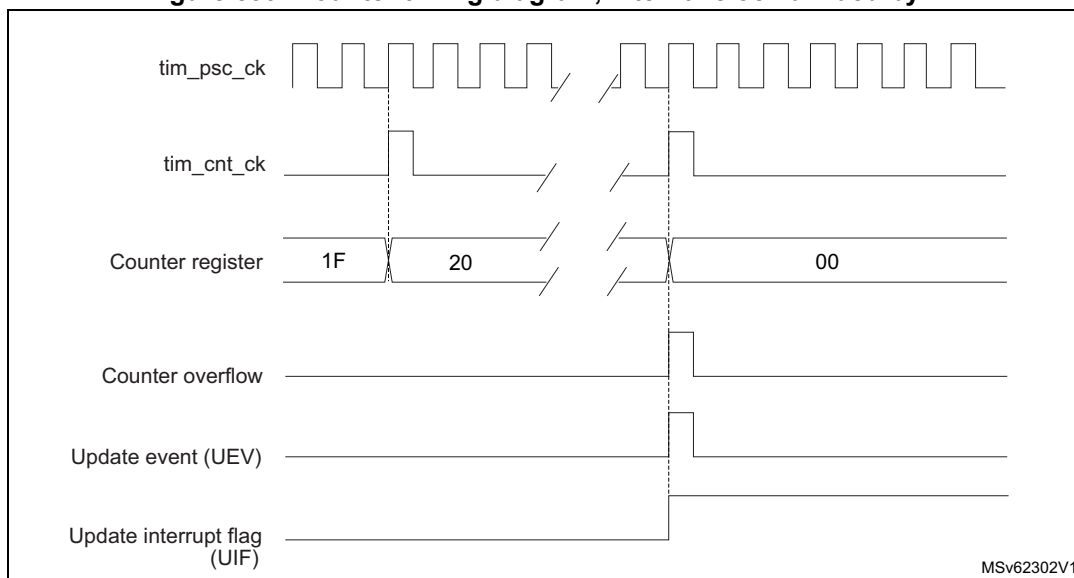
Figure 599. Counter timing diagram, internal clock divided by N
