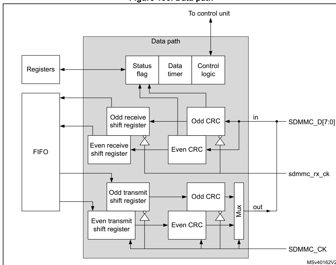
Figure 190. Data path
