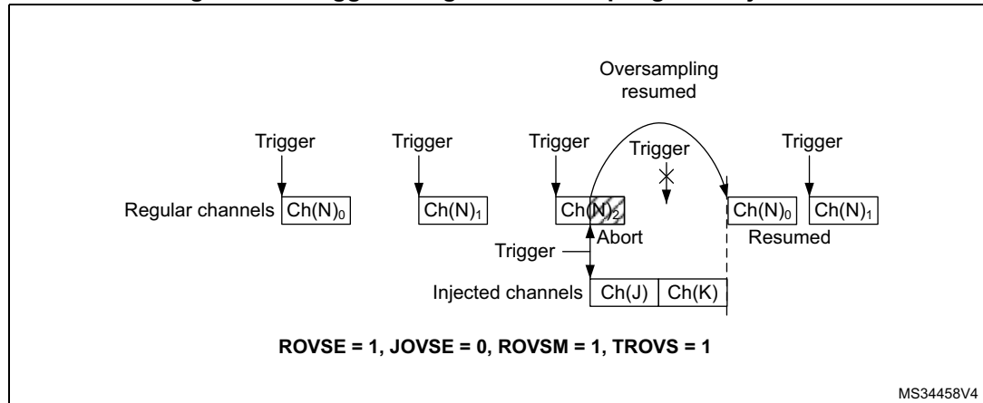
Figure 251. Triggered regular oversampling with injection
