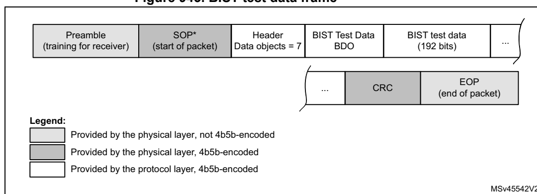
Figure 943. BIST test data frame
