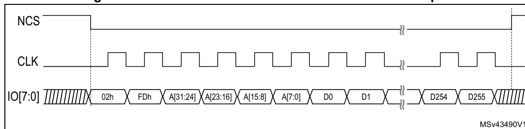
Figure 167. SDR write command in octal-SPI mode example.
