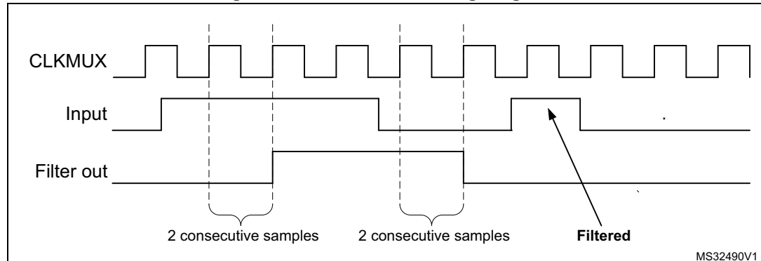
Figure 732. Glitch filter timing diagram
