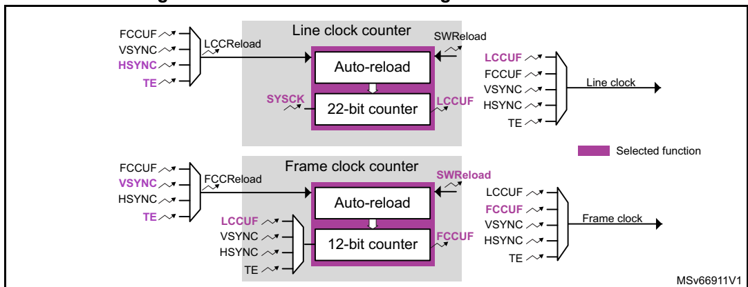
Figure 747. Active counters and signals in standalone
