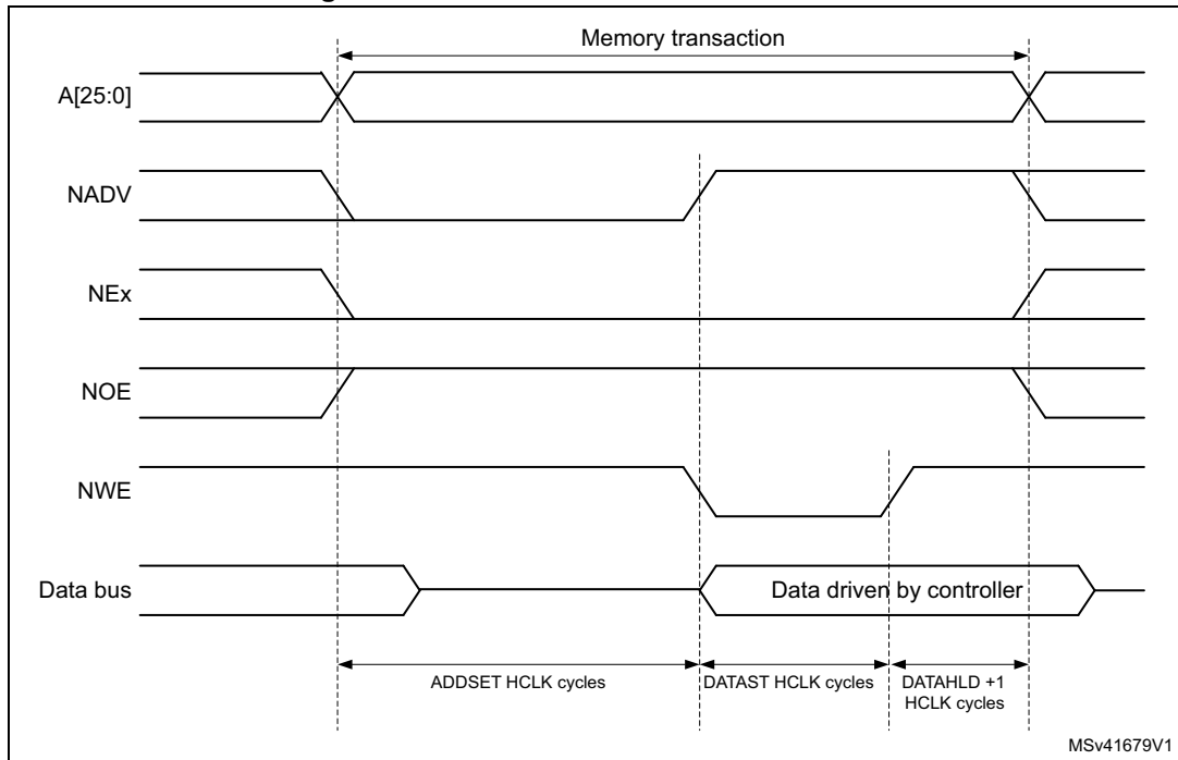
Figure 125. Mode B write access waveforms
