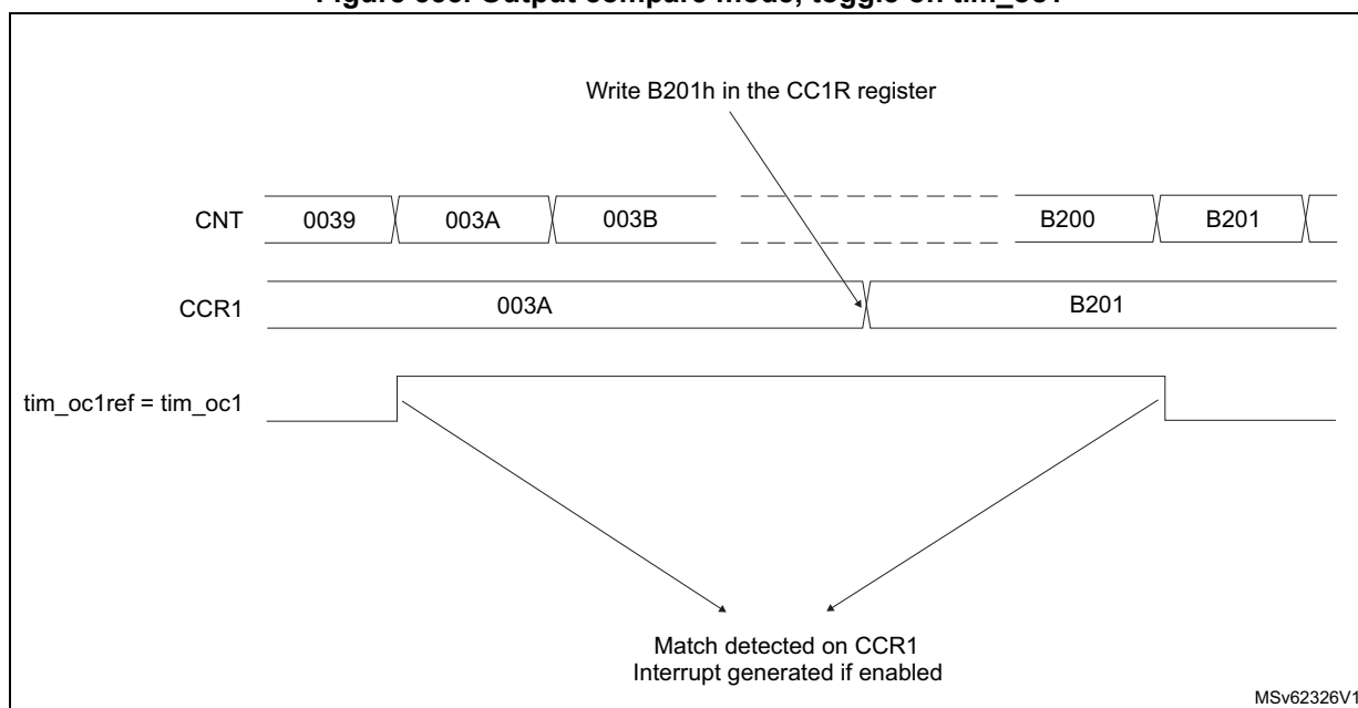
Figure 535. Output compare mode, toggle on tim_oc1
