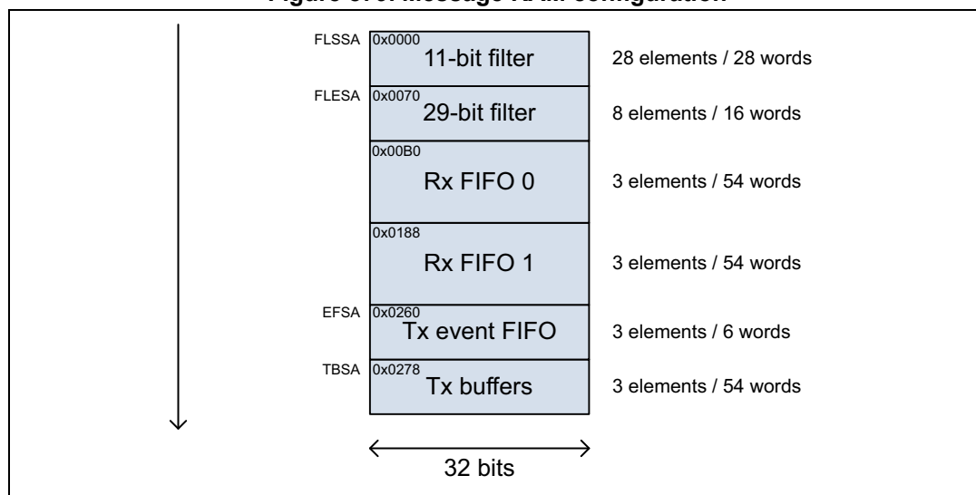
Figure 879. Message RAM configuration
