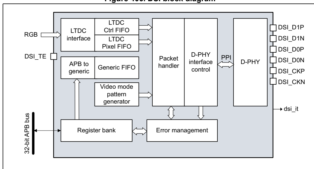
Figure 406. DSI block diagram
