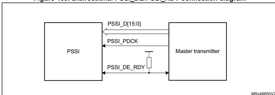
Figure 400. Bidirectional PSSI_DE/PSSI_RDY connection diagram
