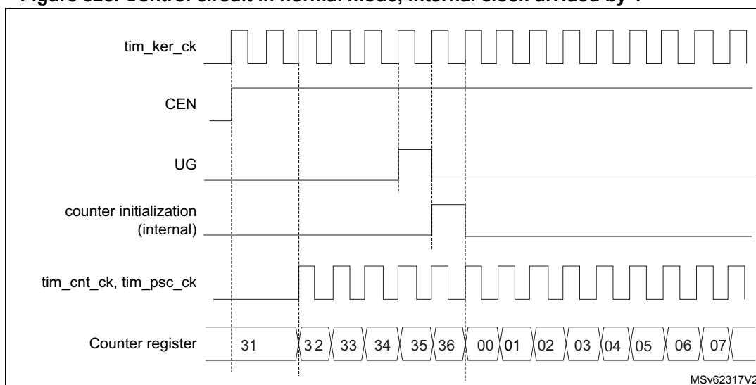
Figure 525. Control circuit in normal mode, internal clock divided by 1
