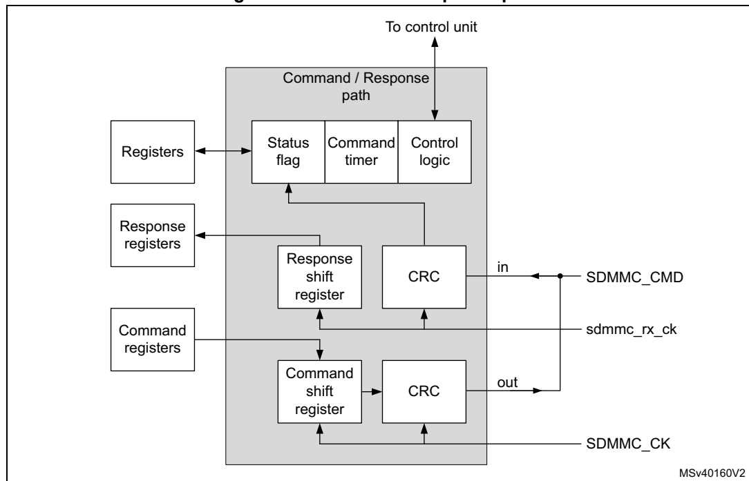
Figure 188. Command/response path
