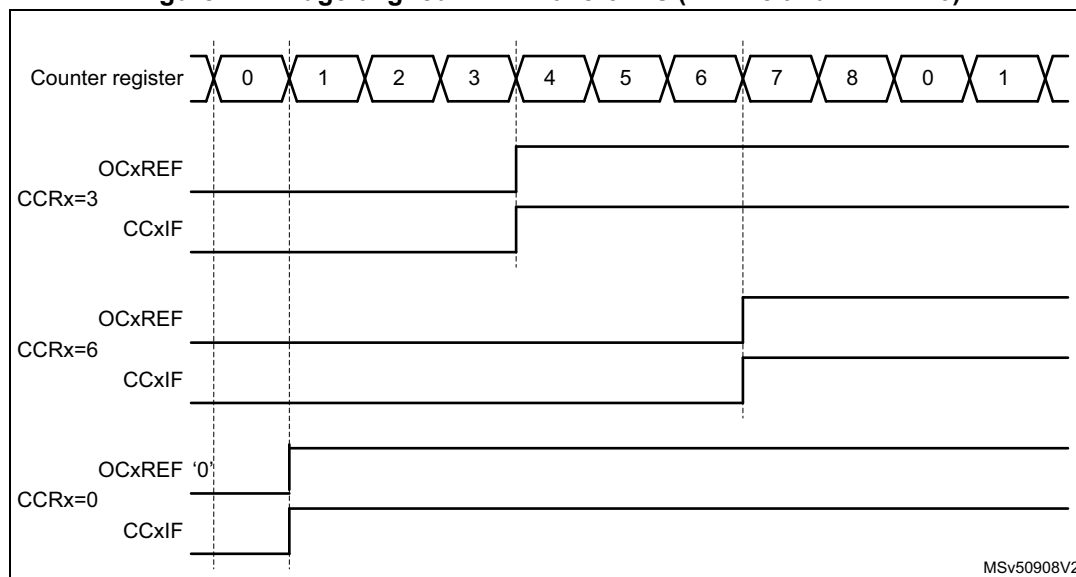
Figure 742. Edge-aligned PWM waveforms (ARR=8 and CCxP = 0)
