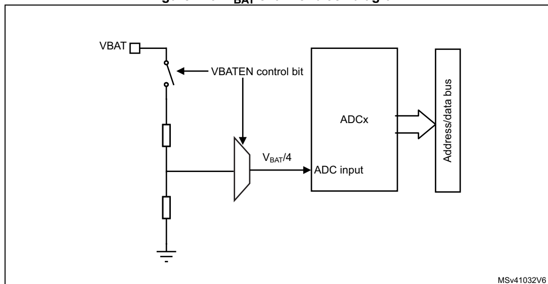
Figure 270. V BAT channel block diagram
