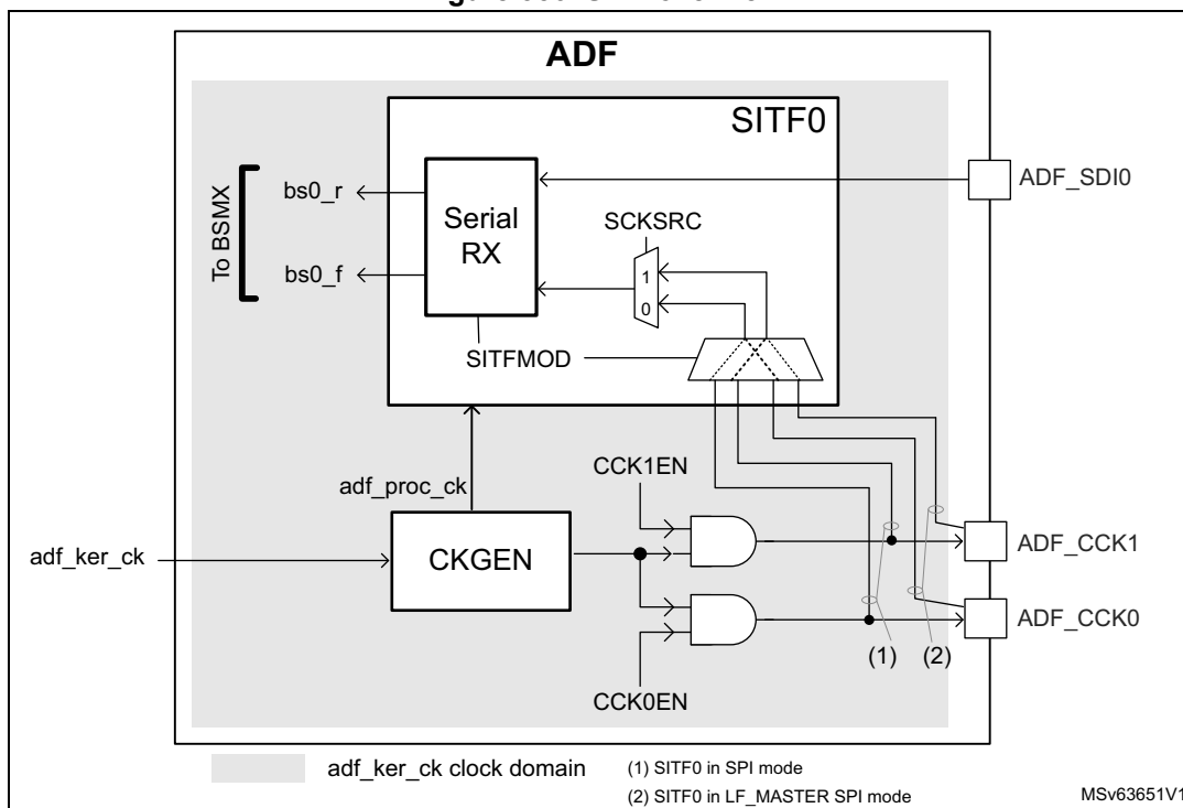
Figure 356. SITF0 overview
