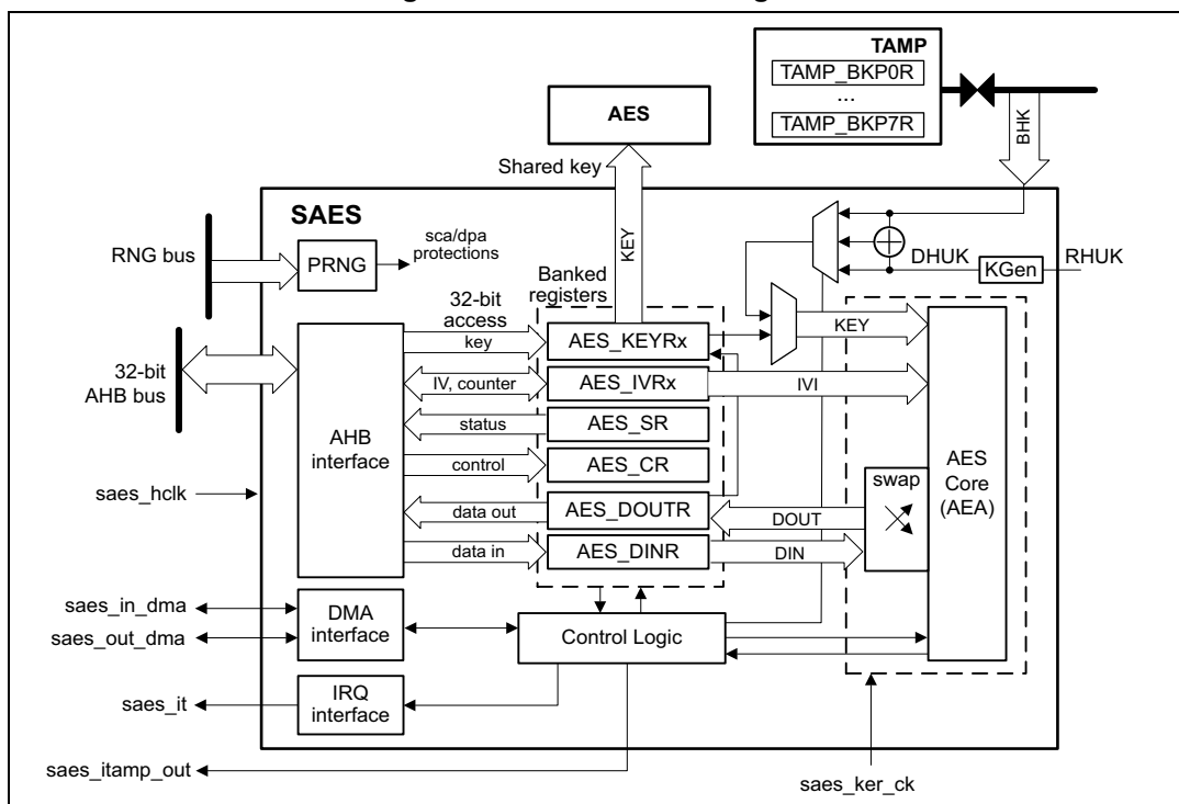
Figure 479. SAES block diagram
