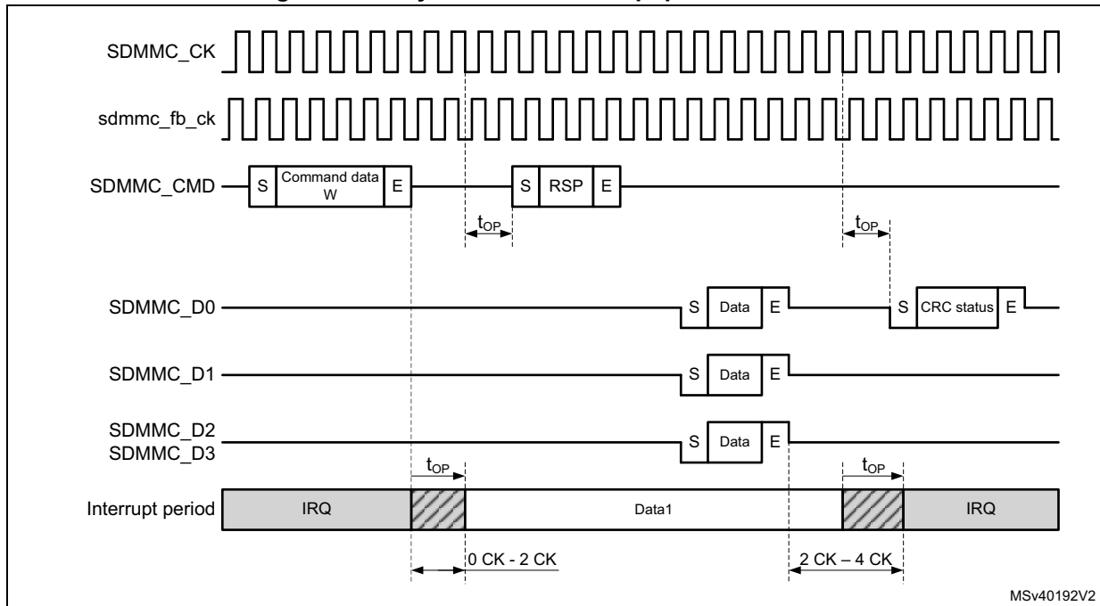
Figure 200. Asynchronous interrupt period data write
