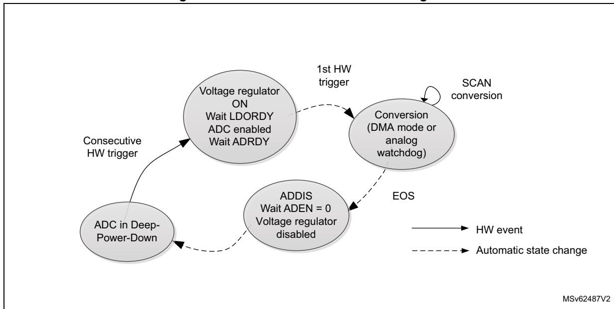
Figure 291. Autonomous mode state diagram
