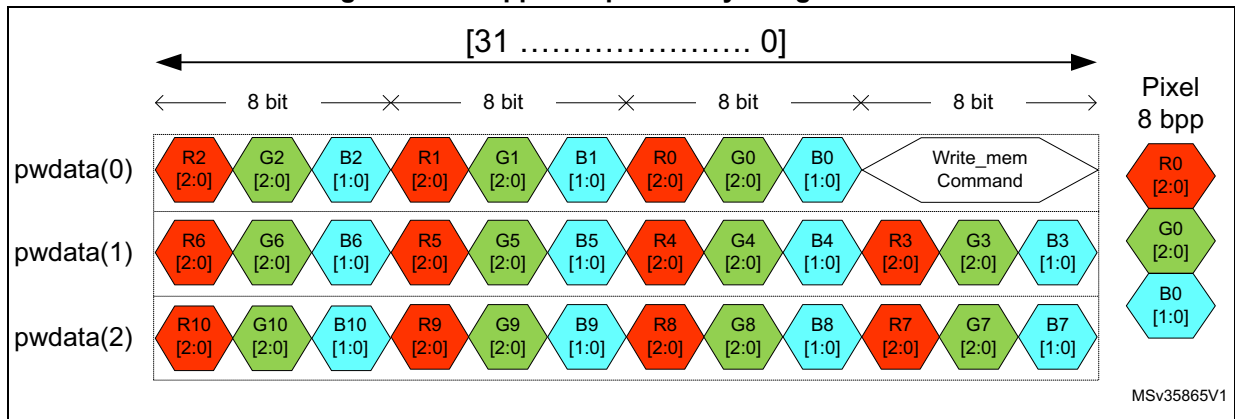
Figure 416. 8 bpp APB pixel to byte organization
