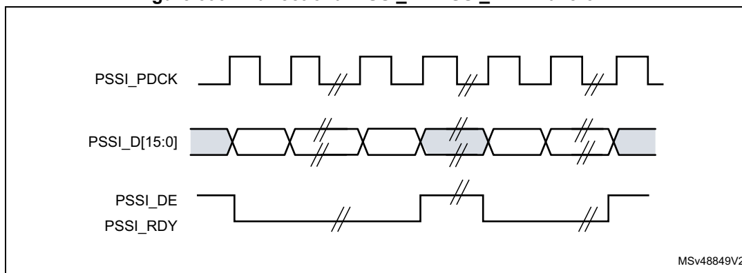
Figure 399. Bidirectional PSSI_DE/PSSI_RDY waveform
