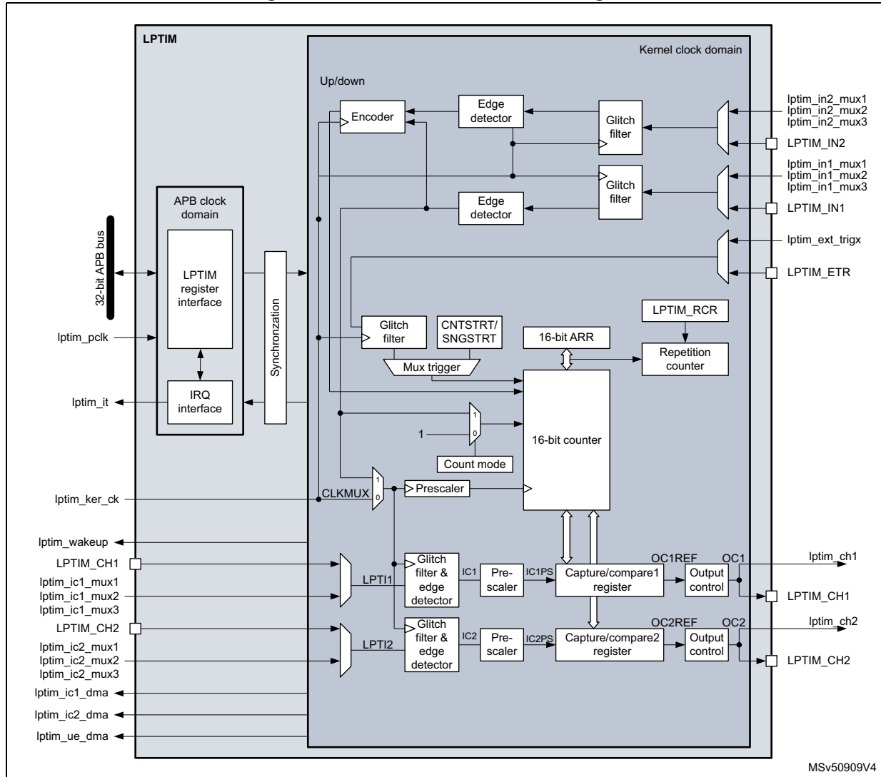
Figure 730. LPTIM1/2/3 timer block diagram
