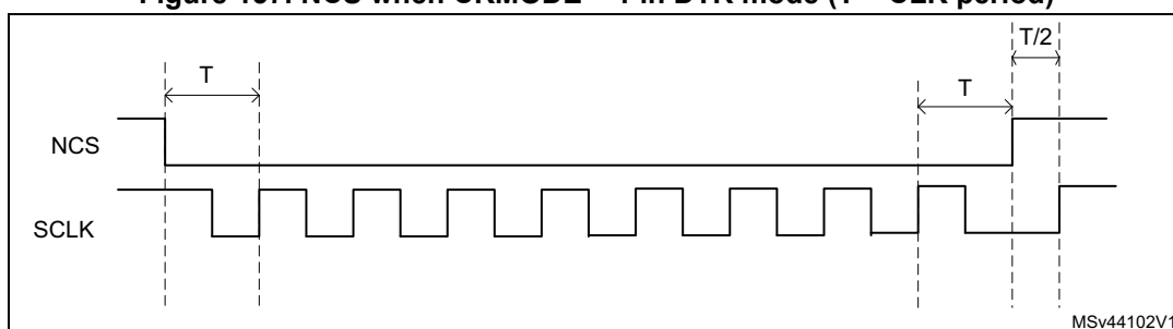
Figure 157. NCS when CKMODE = 1 in DTR mode (T = CLK period)
