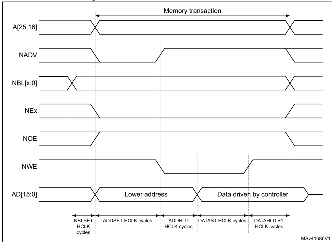
Figure 131. Muxed write access waveforms
