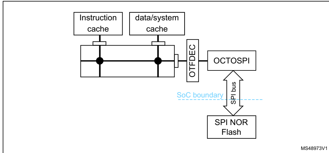
Figure 499. Typical OTFDEC use in a SoC
