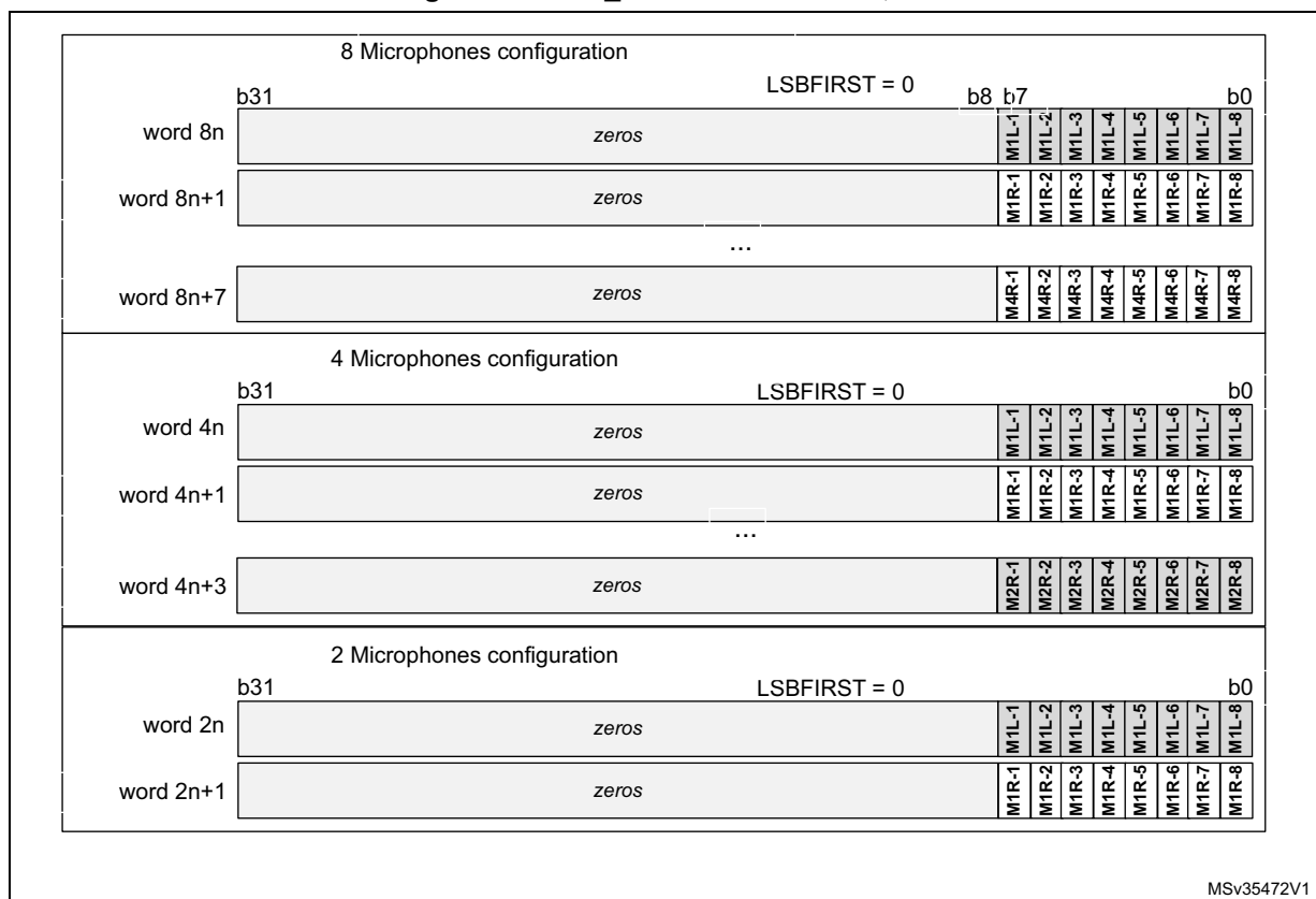
Figure 863. SAI_ADR format in TDM, 8-bit slot width
