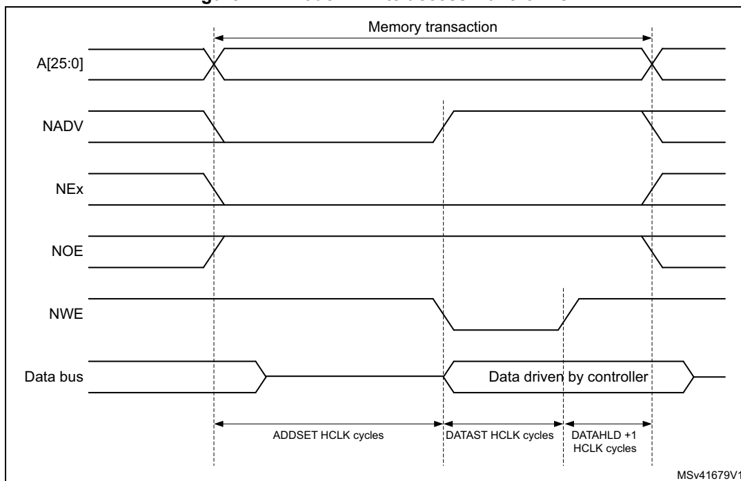
Figure 127. Mode C write access waveforms
