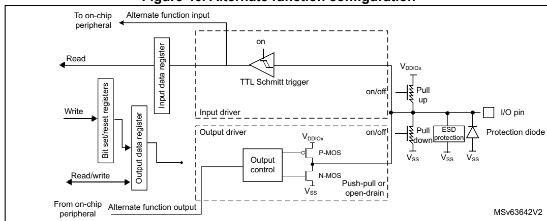
Figure 46. Alternate function configuration
