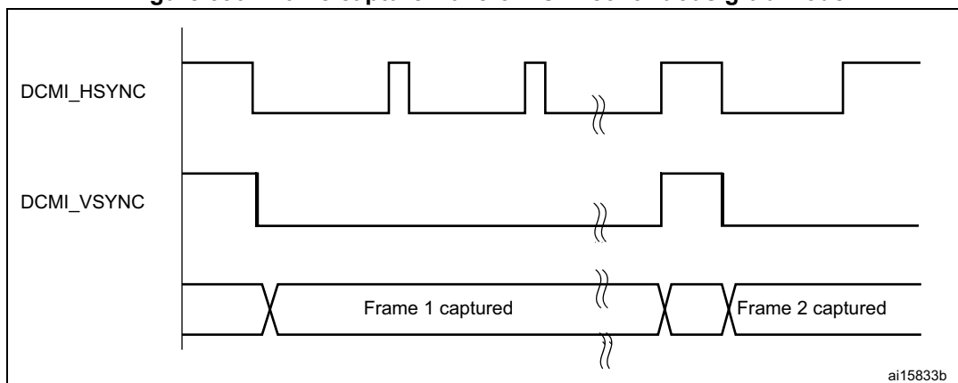
Figure 390. Frame capture waveforms in continuous grab mode
