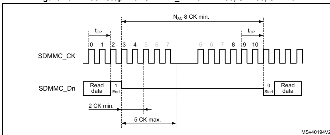
Figure 202. Clock stop with SDMMC_CK for DDR50, SDR50, SDR104
