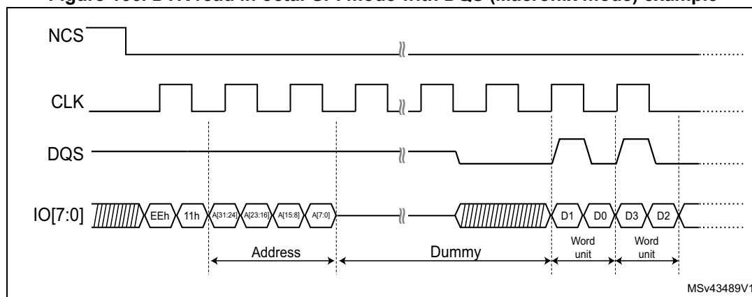
Figure 166. DTR read in octal-SPI mode with DQS (Macronix mode) example
