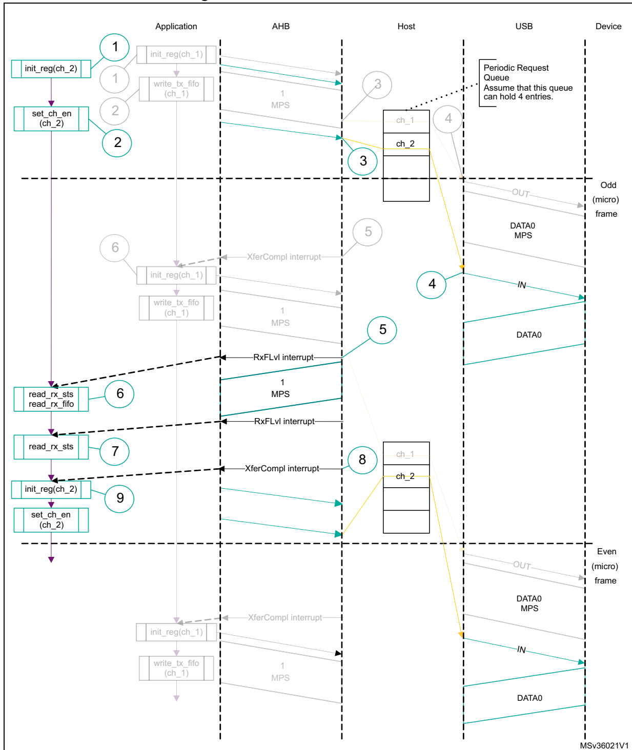
Figure 900. Isochronous IN transactions
