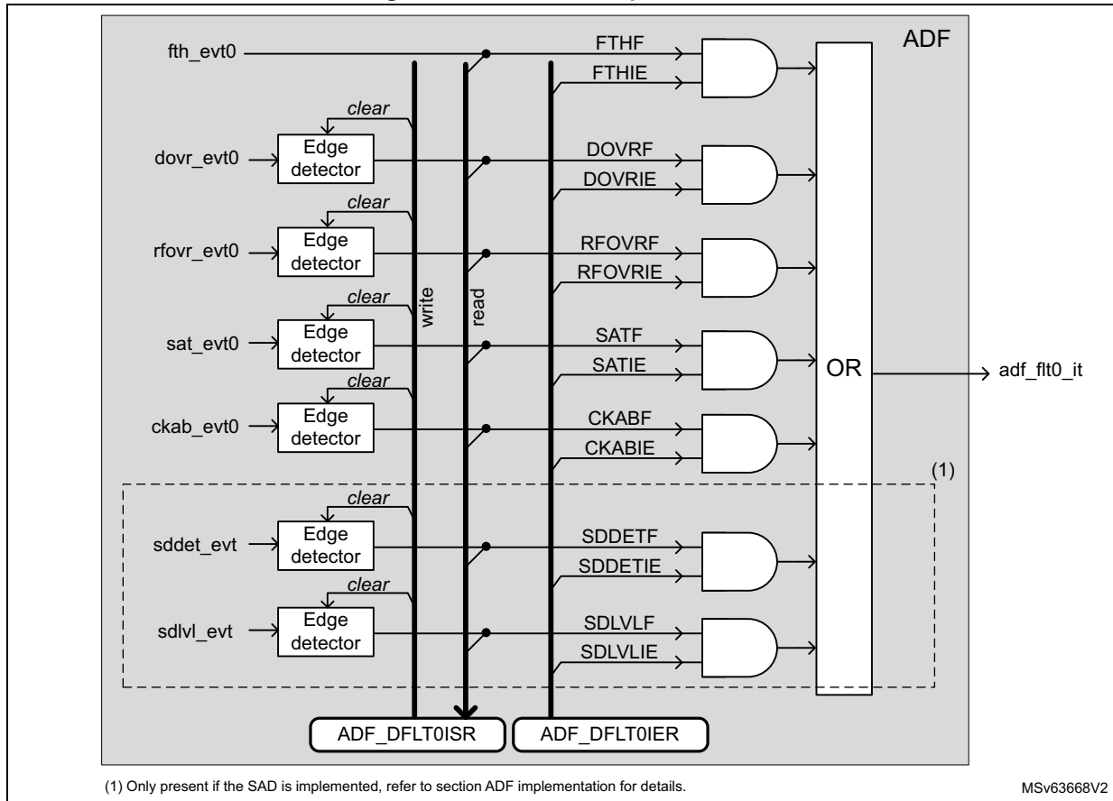
Figure 379. ADF interrupt interface
