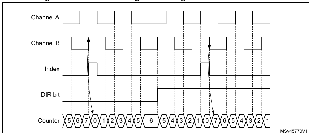
Figure 651. Counter reading with index gated on channel A and B
