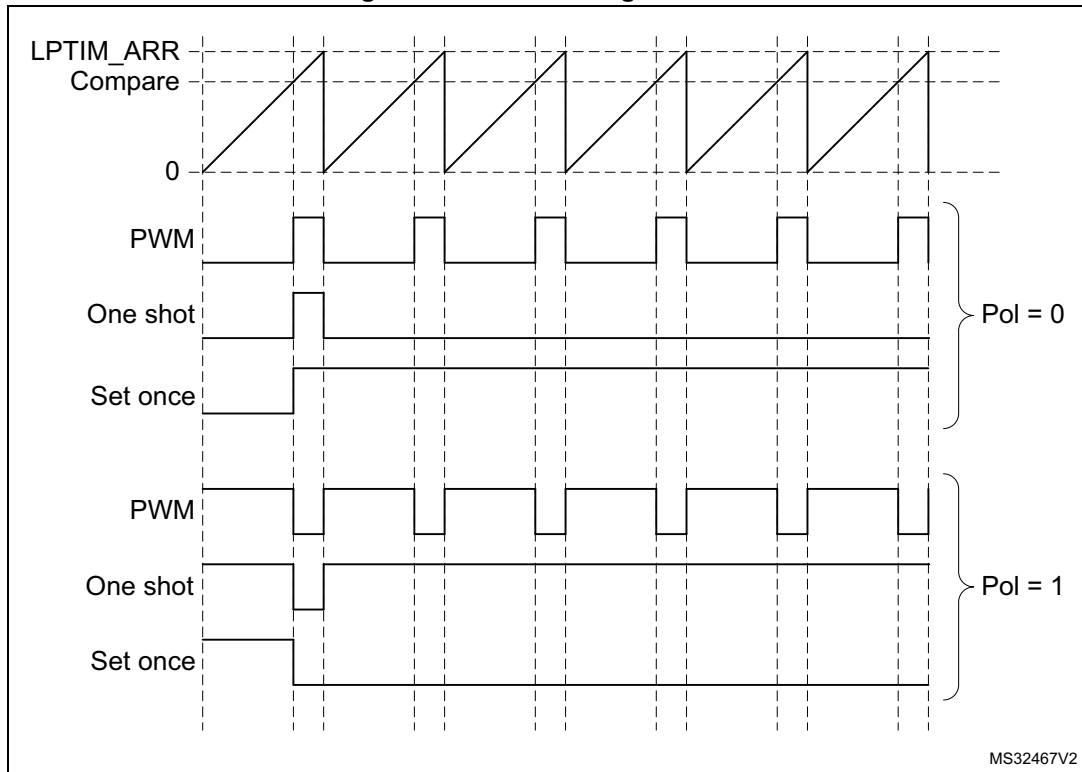
Figure 736. Waveform generation
