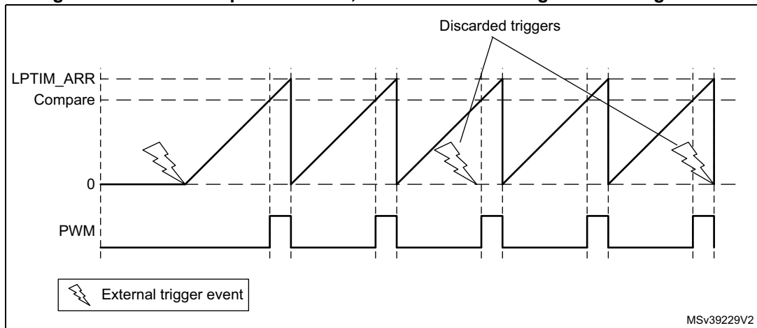
Figure 735. LPTIM output waveform, Continuous counting mode configuration
