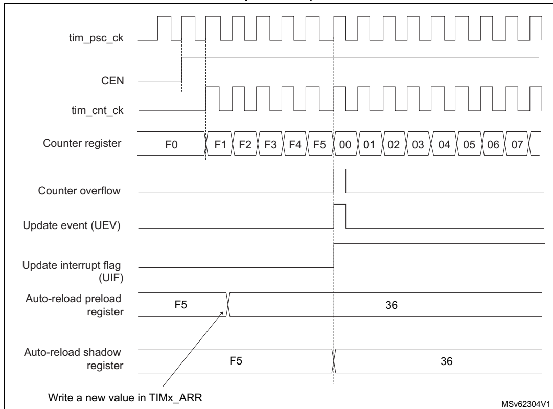
Figure 725. Counter timing diagram, update event when ARPE=1 (TIMx_ARR preloaded)
