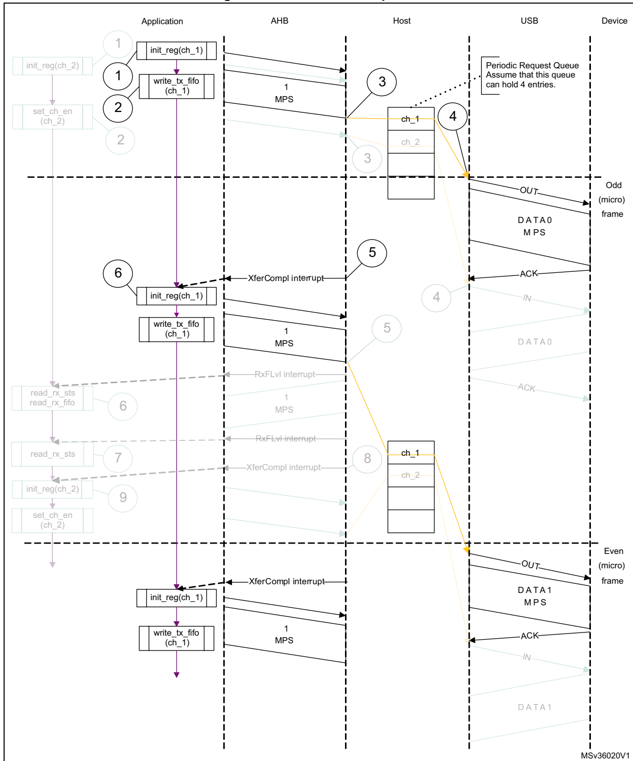
Figure 922. Normal interrupt OUT
