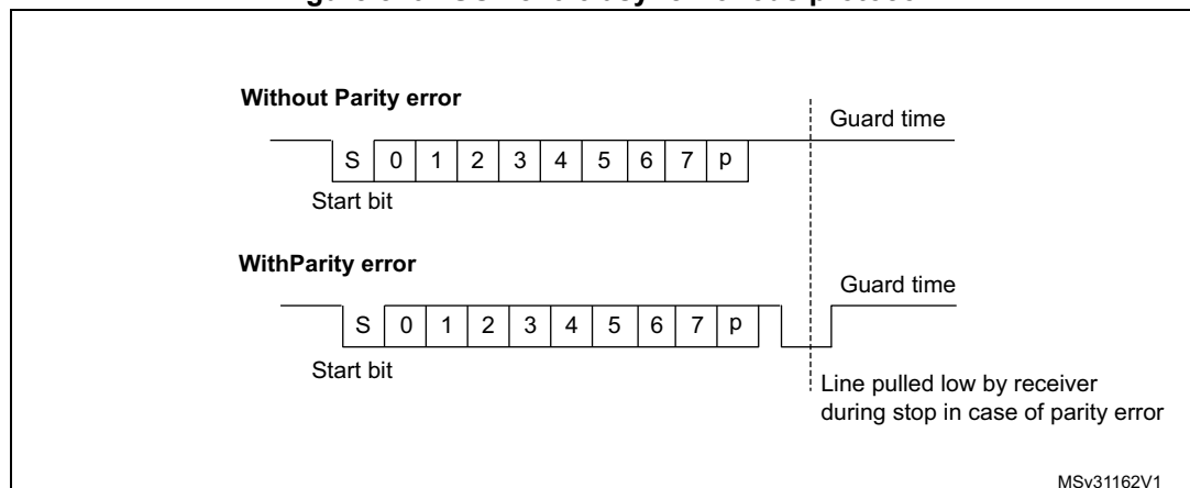
Figure 816. ISO 7816-3 asynchronous protocol
