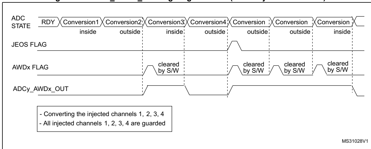
Figure 246. ADC_AWDx_OUT signal generation (on all injected channels)
