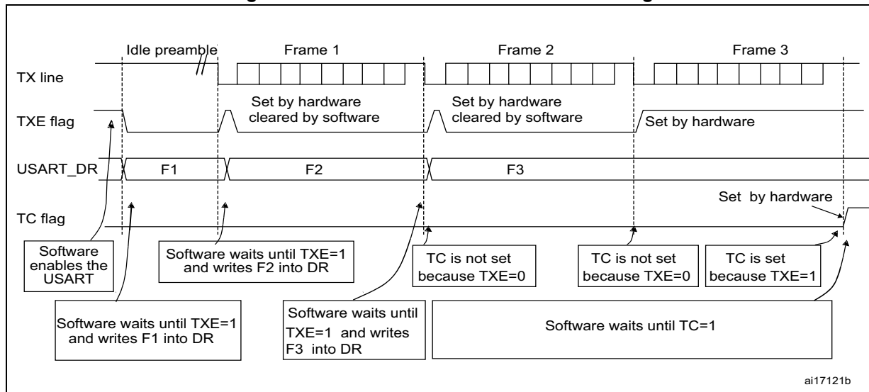
Figure 803. TC/TXE behavior when transmitting
