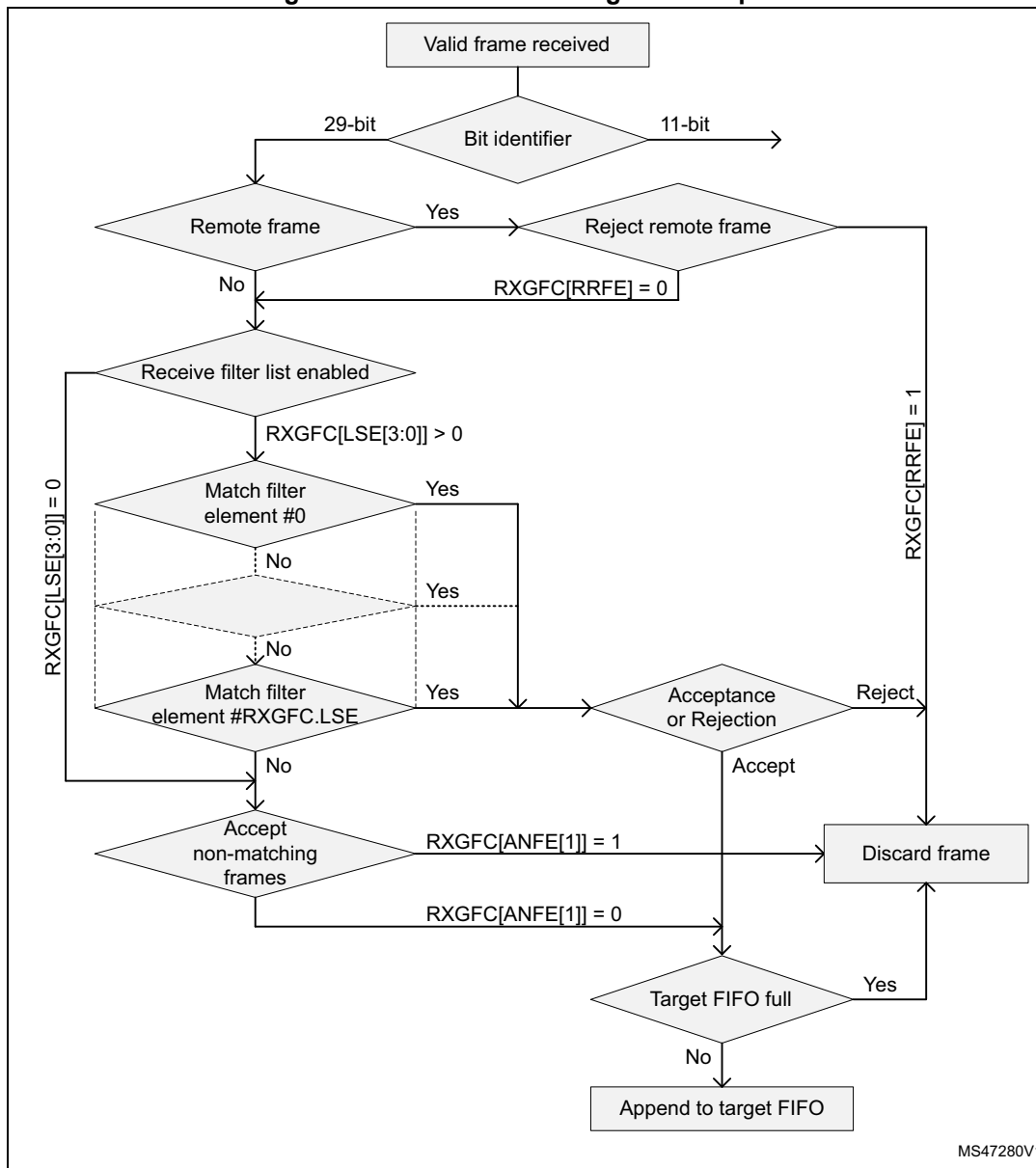
Figure 881. Extended Message ID filter path
