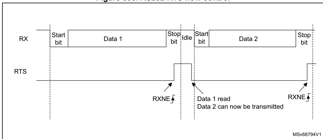
Figure 835. RS232 RTS flow control
