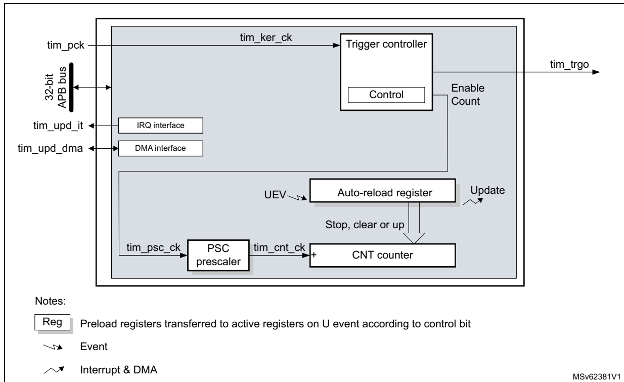
Figure 716. Basic timer block diagram
