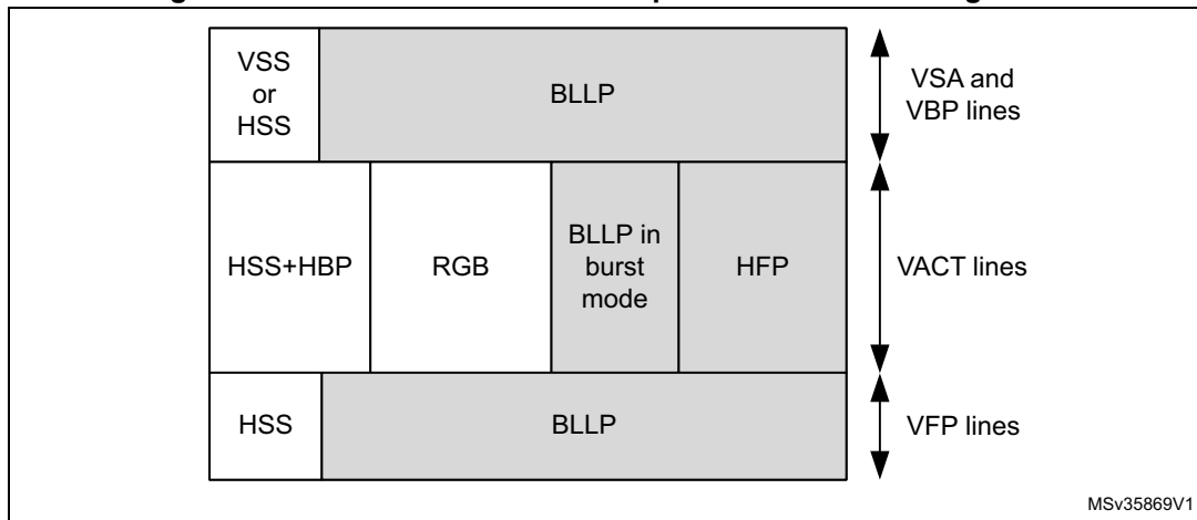
Figure 421. Command transmission periods within the image area
