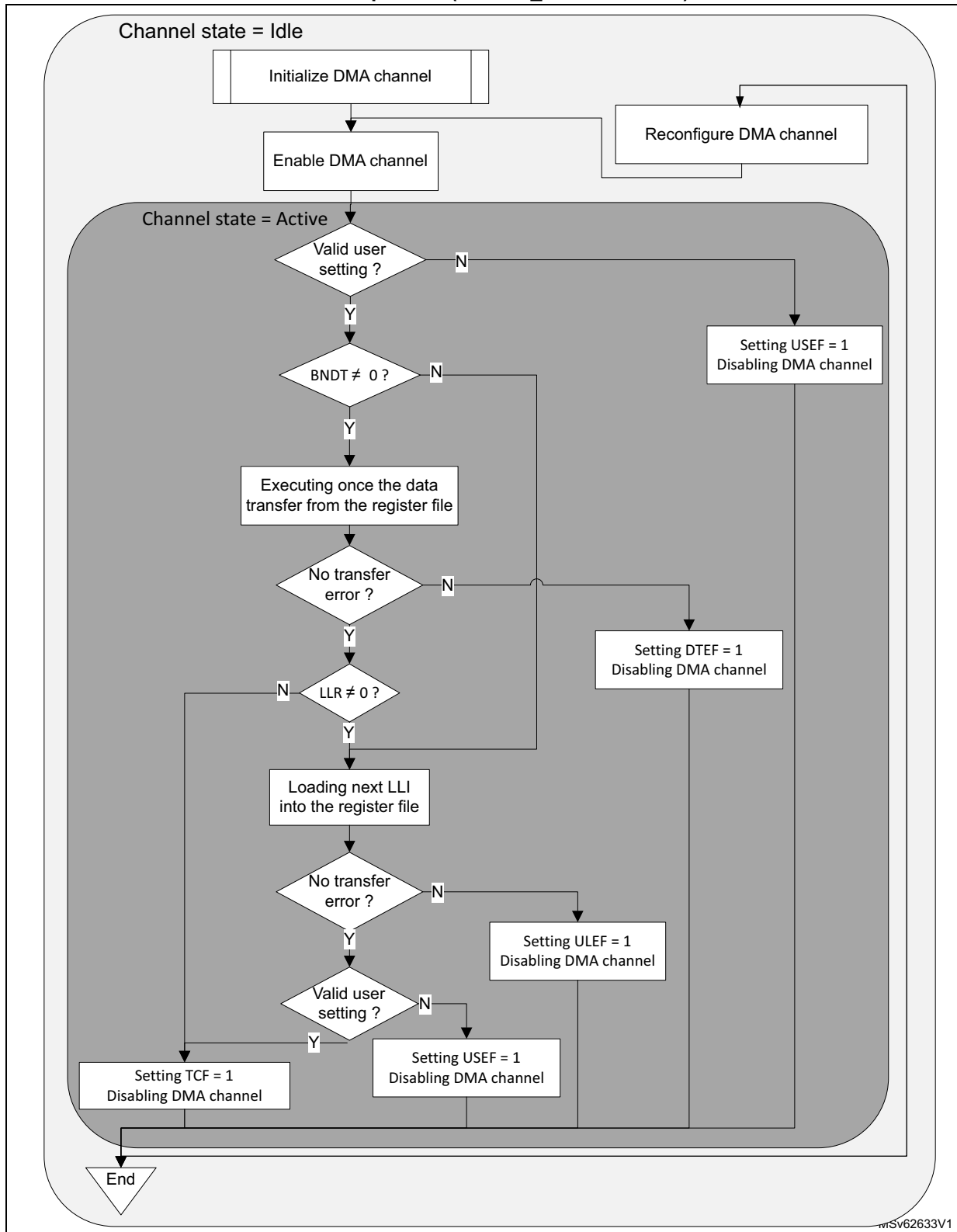
Figure 78. LPDMA channel execution and linked-list programming in link step mode (LPDMA_CxCR.LSM = 1)
