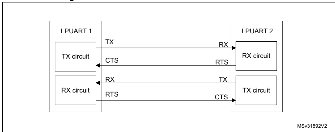
Figure 834. Hardware flow control between 2 LPUARTs
