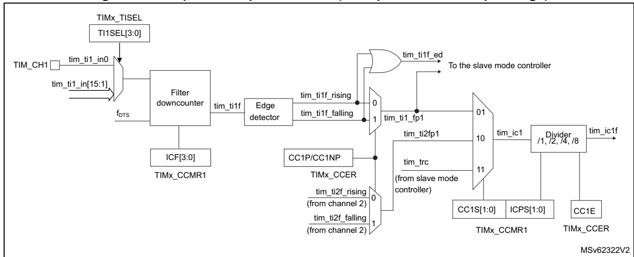
Figure 689. Capture/compare channel (example: channel 1 input stage)
