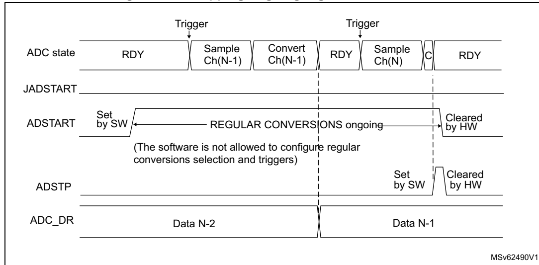
Figure 223. Stopping ongoing regular conversions
