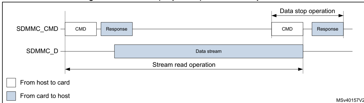
Figure 183. SDMMC (sequential) stream read operation
