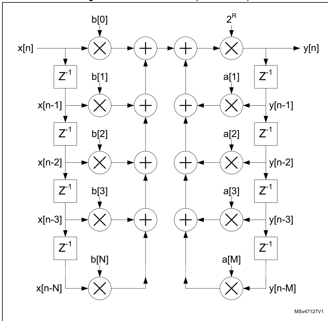
Figure 113. IIR filter structure (direct form 1)
