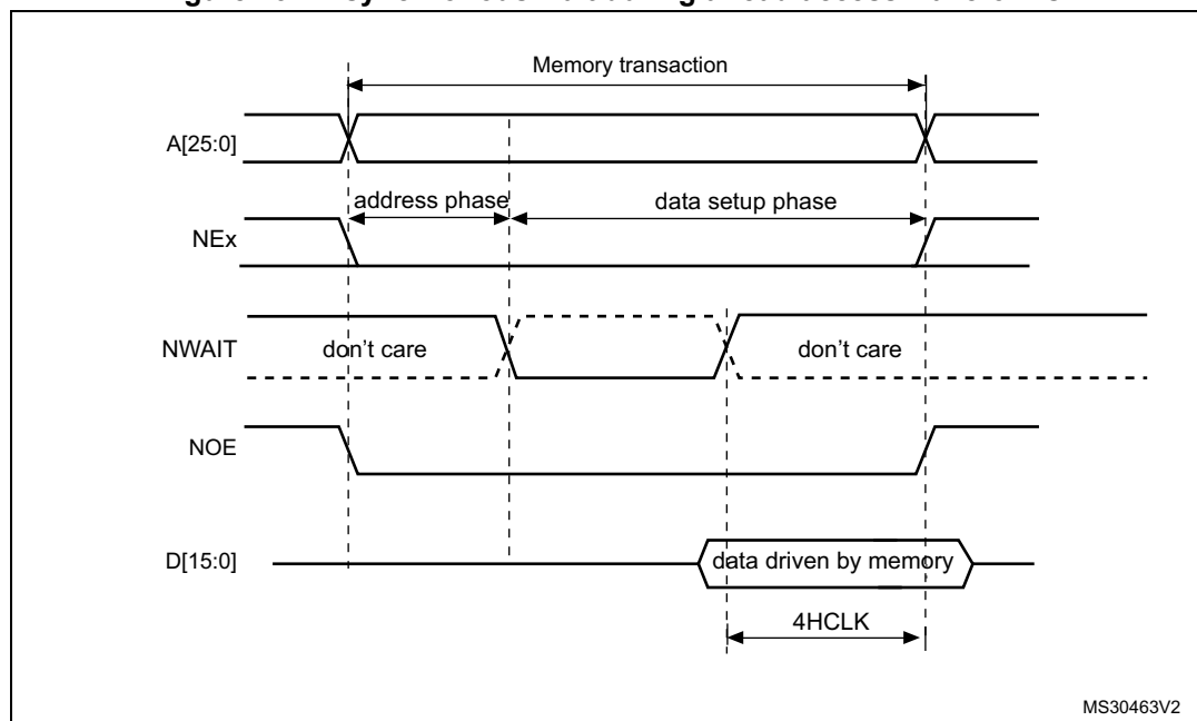
Figure 132. Asynchronous wait during a read access waveforms
