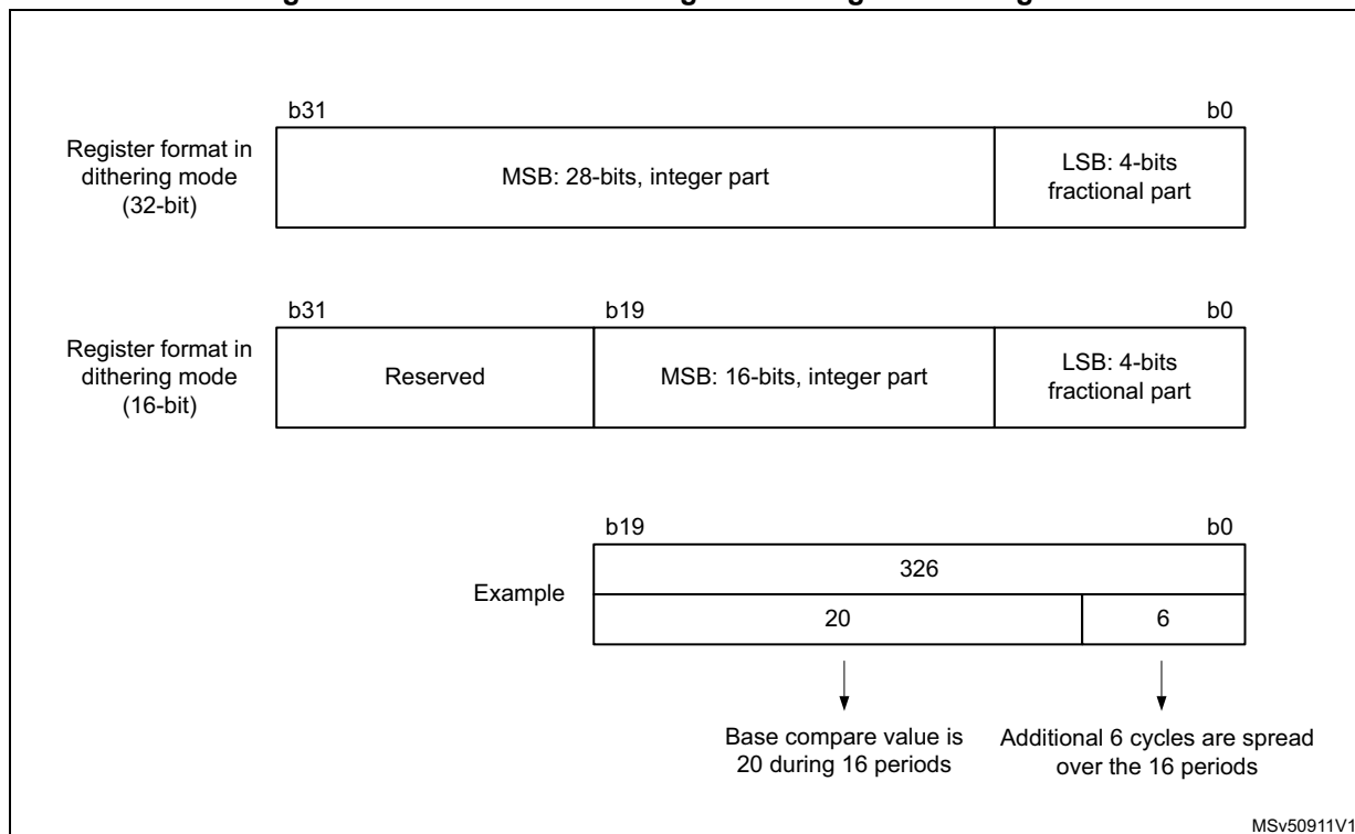
Figure 626. Data format and register coding in dithering mode
