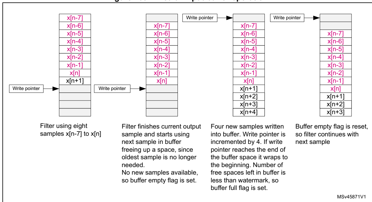
Figure 109. Circular input buffer operation
