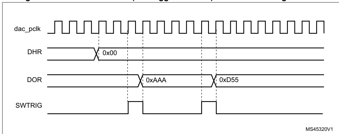
Figure 307. DAC conversion (SW trigger enabled) with LFSR wave generation
