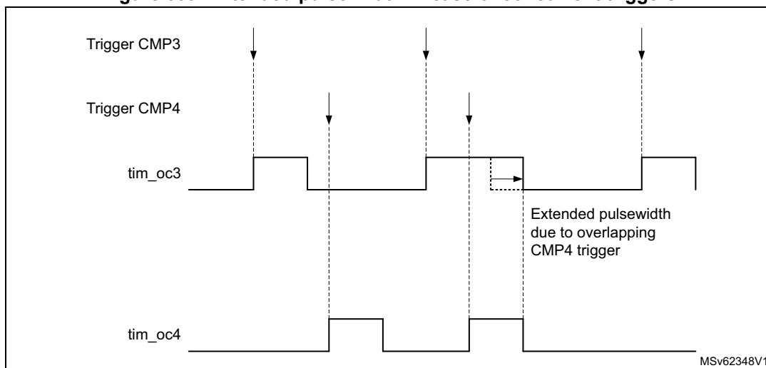
Figure 639. Extended pulse width in case of concurrent triggers
