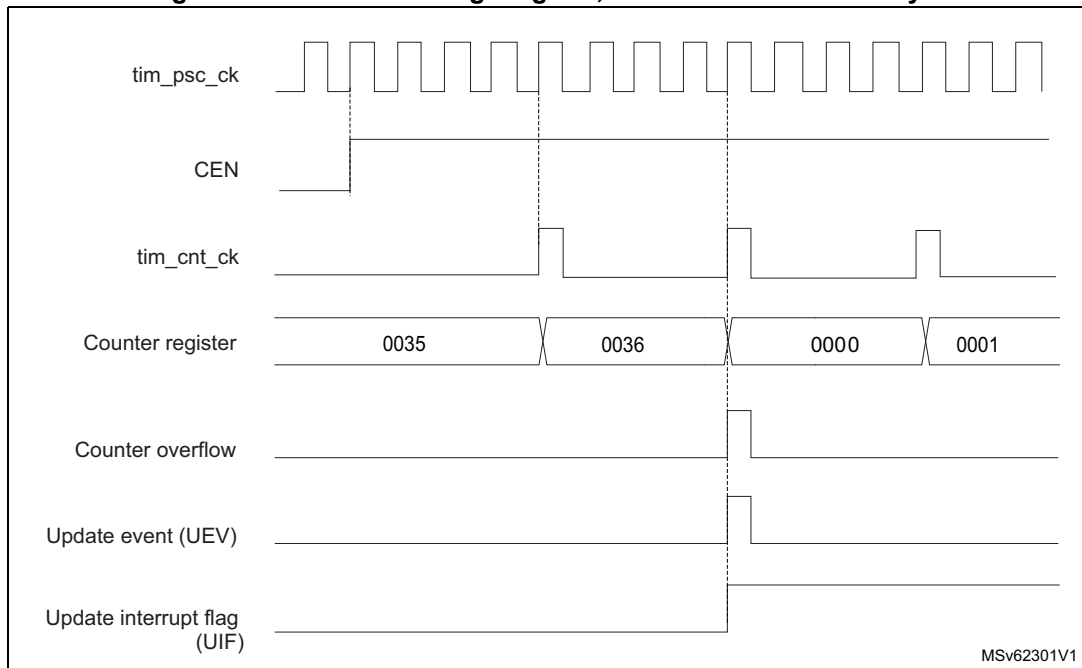
Figure 508. Counter timing diagram, internal clock divided by 4
