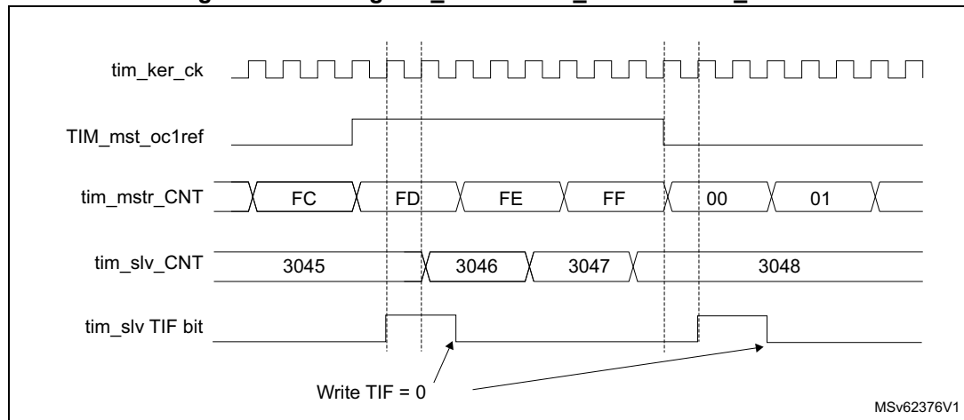
Figure 670. Gating TIM_slv with tim_oc1ref of TIM_mstr
