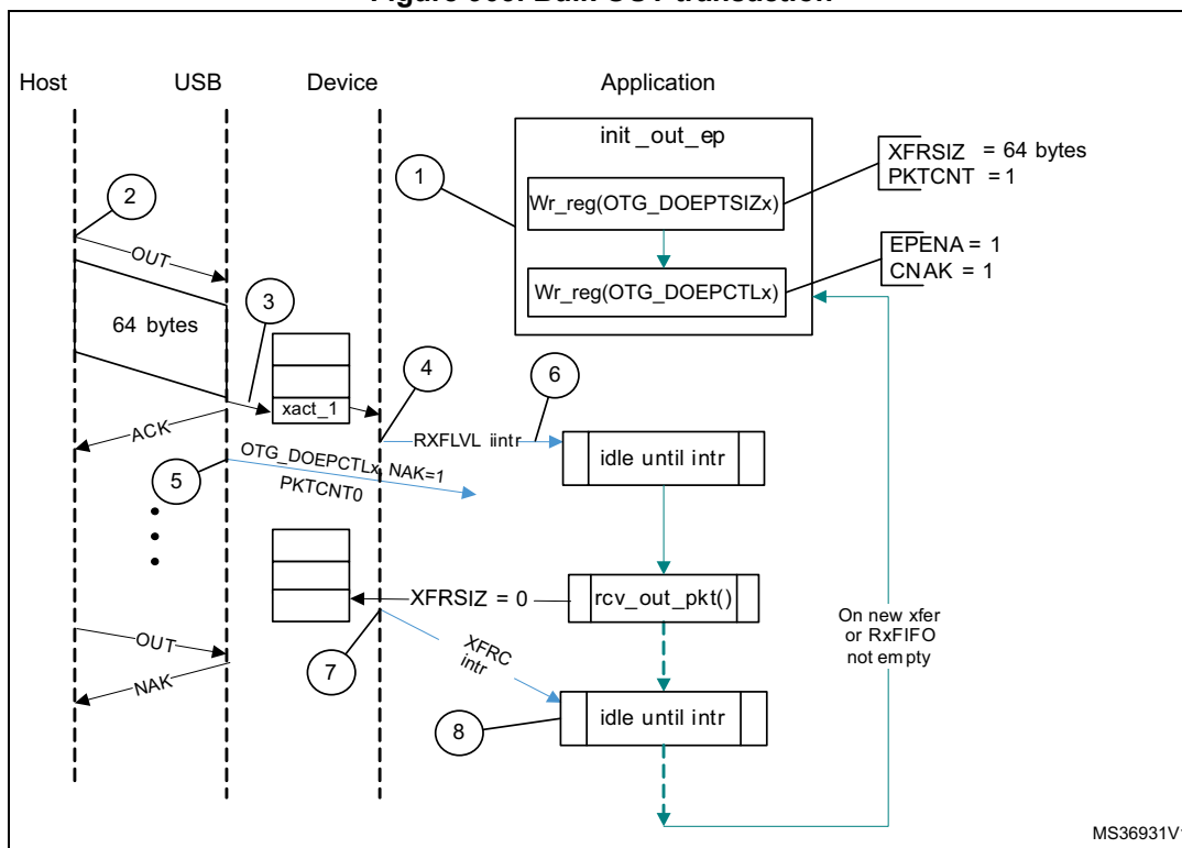
Figure 903. Bulk OUT transaction
