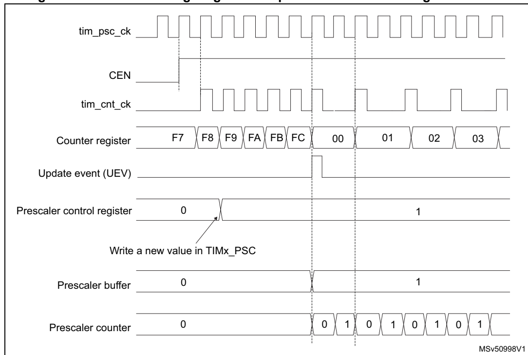
Figure 504. Counter timing diagram with prescaler division change from 1 to 2
