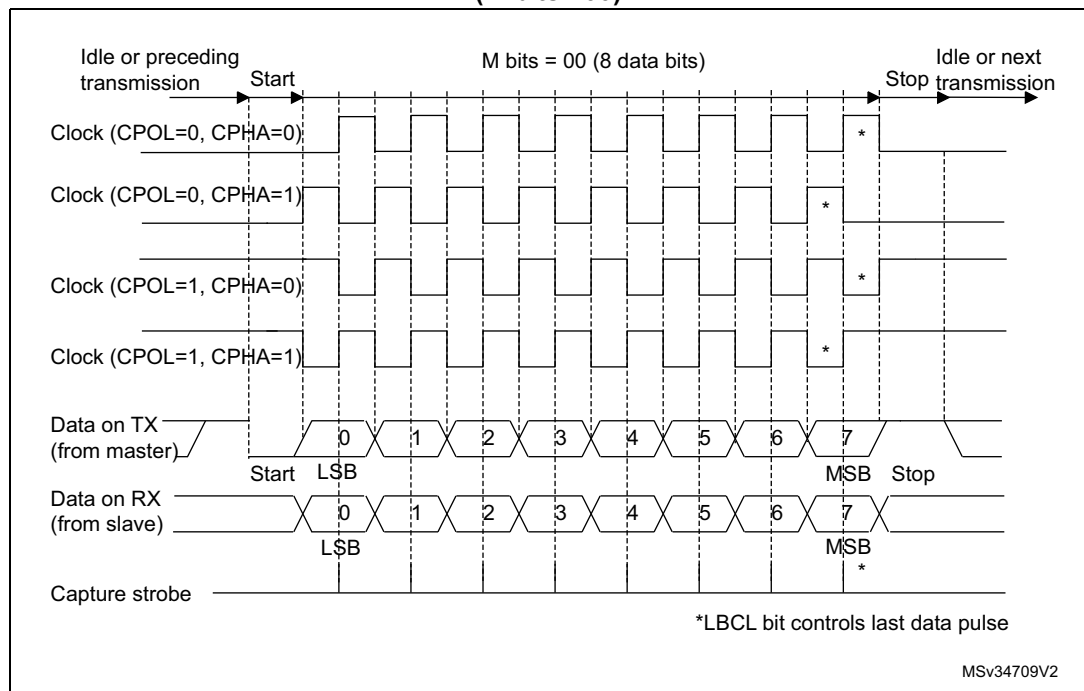
Figure 813. USART data clock timing diagram in Synchronous master mode (M bits = 00)
