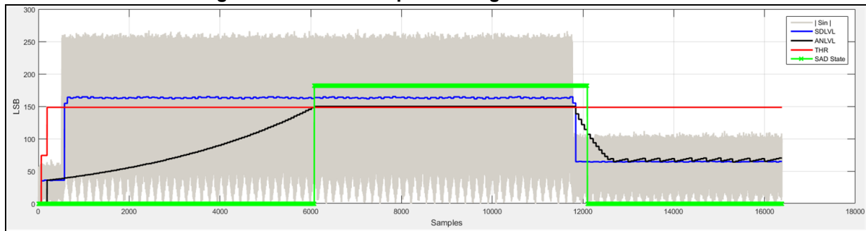
Figure 385. SAD example working with SADMOD = 1x
