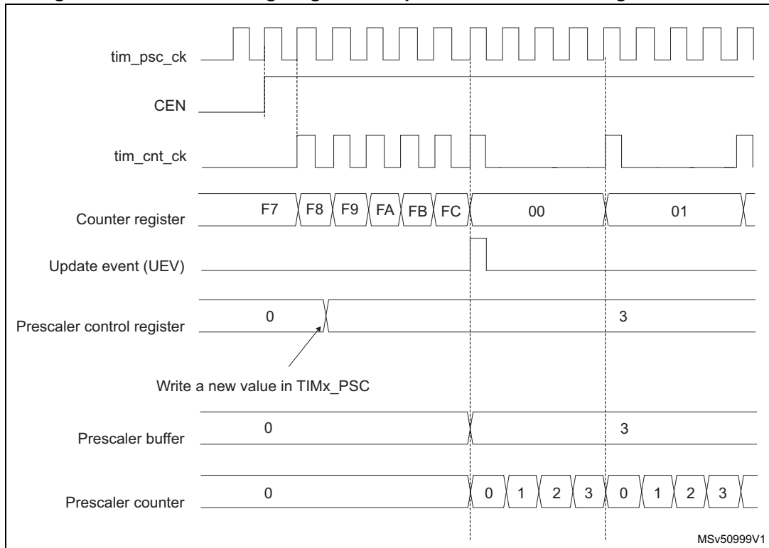
Figure 505. Counter timing diagram with prescaler division change from 1 to 4
