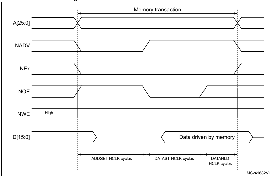
Figure 126. Mode C read access waveforms
