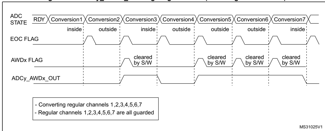
Figure 243. ADCy_AWDx_OUT signal generation (on all regular channels)
