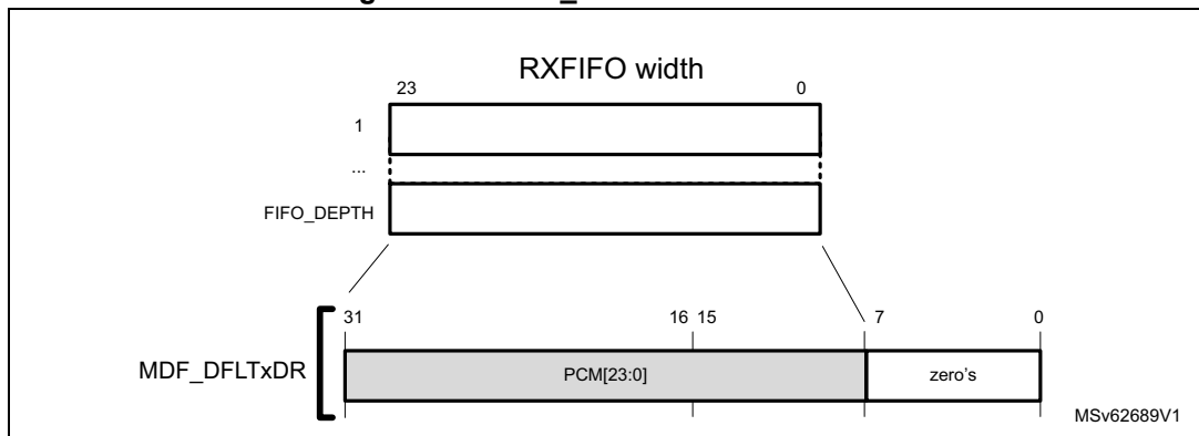
Figure 345. MDF_DFLTxDR data format
