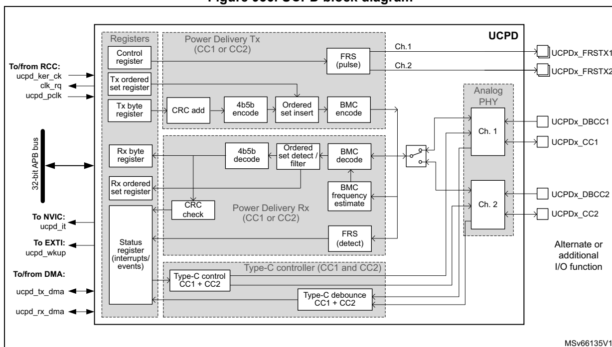
Figure 936. UCPD block diagram
