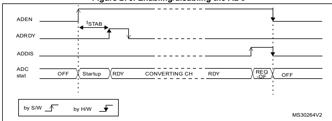
Figure 275. Enabling/disabling the ADC
