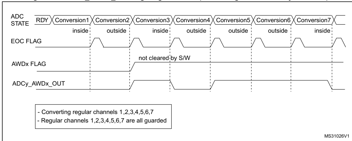
Figure 245. ADC_AWDx_OUT signal generation (on a single regular channel)
