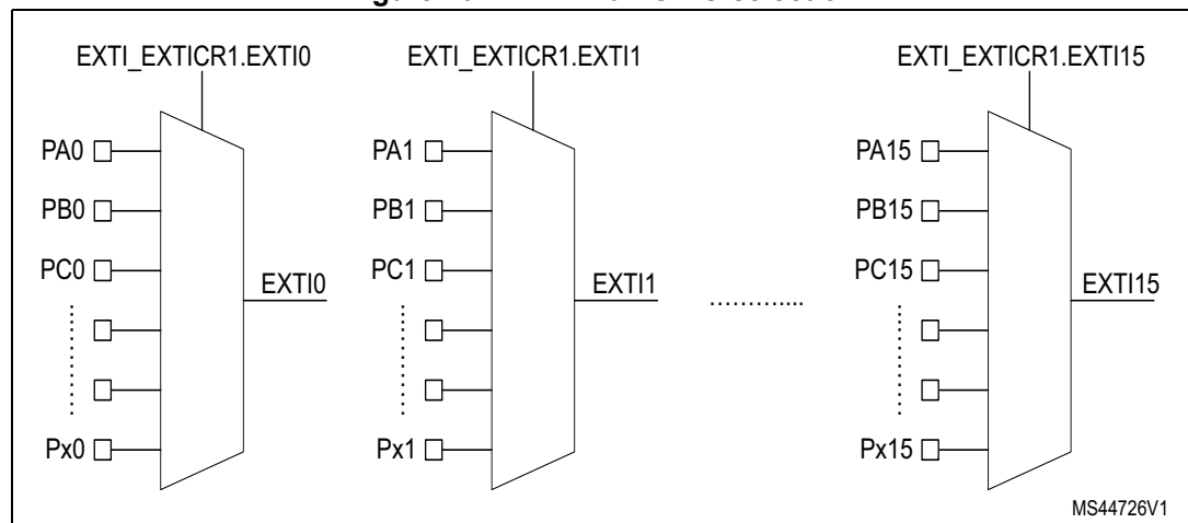
Figure 101. EXTI mux GPIO selection
