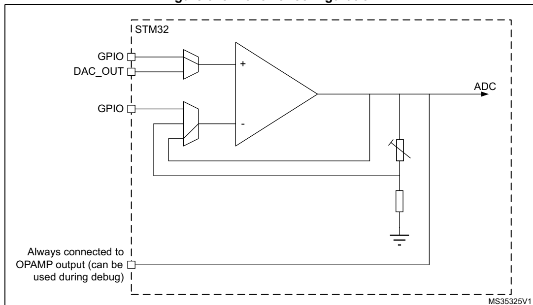
Figure 318. Follower configuration
