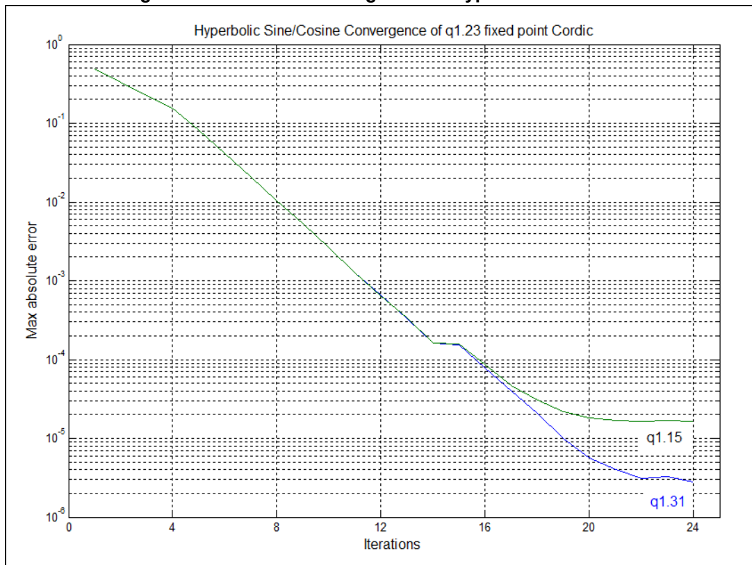
Figure 104. CORDIC convergence for hyperbolic functions
