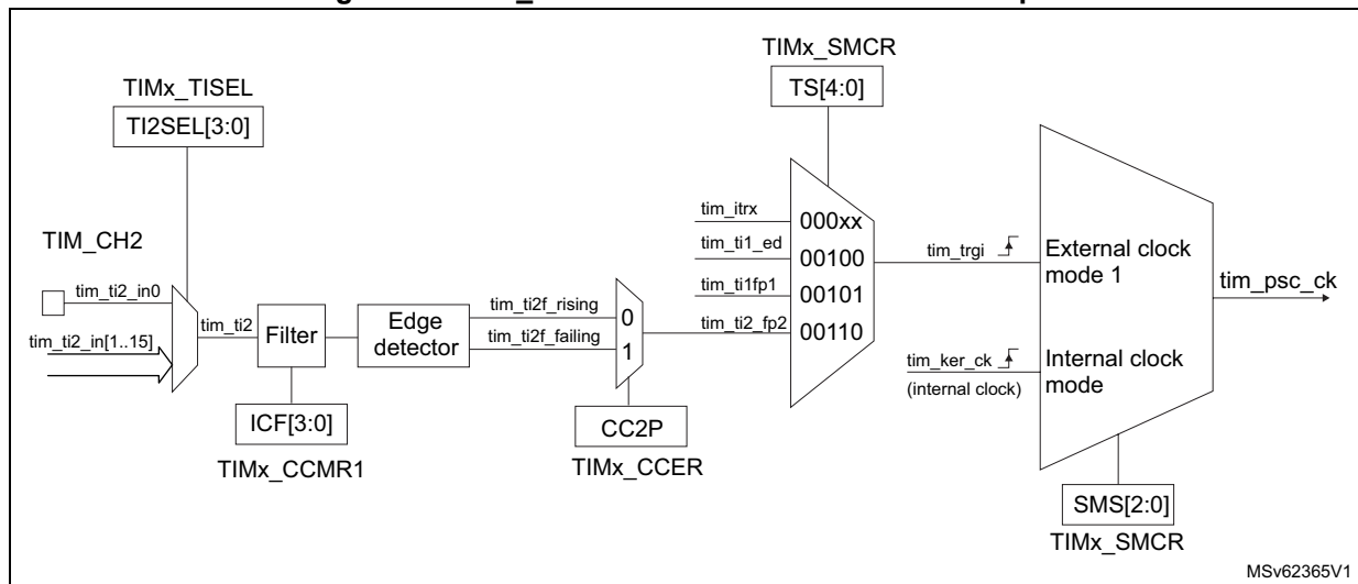
Figure 687. tim_ti2 external clock connection example
