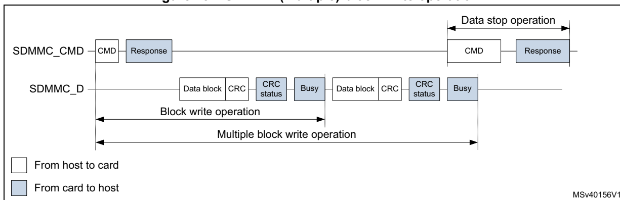
Figure 182. SDMMC (multiple) block write operation
