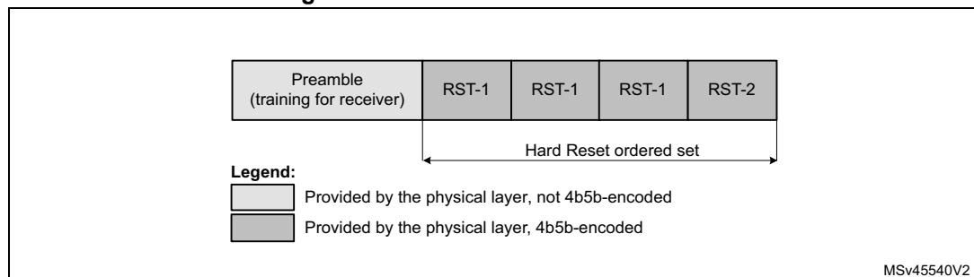
Figure 941. Line format of Hard Reset
