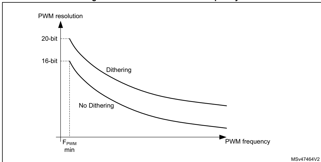
Figure 540. PWM resolution vs frequency
