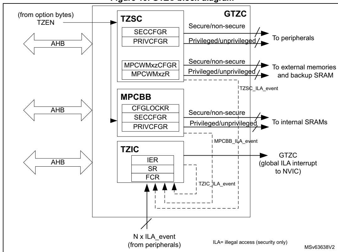
Figure 19. GTZC block diagram
