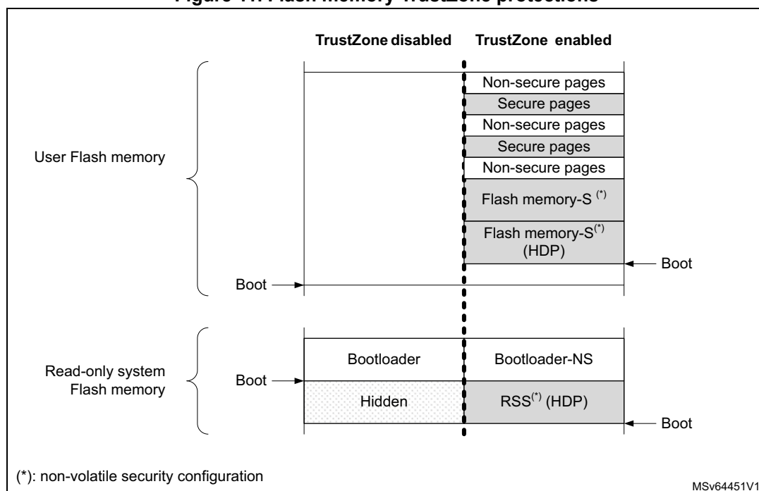
Figure 11. Flash memory TrustZone protections
