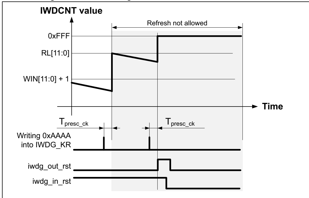
Figure 762. Reset timing due to refresh in the not allowed area
