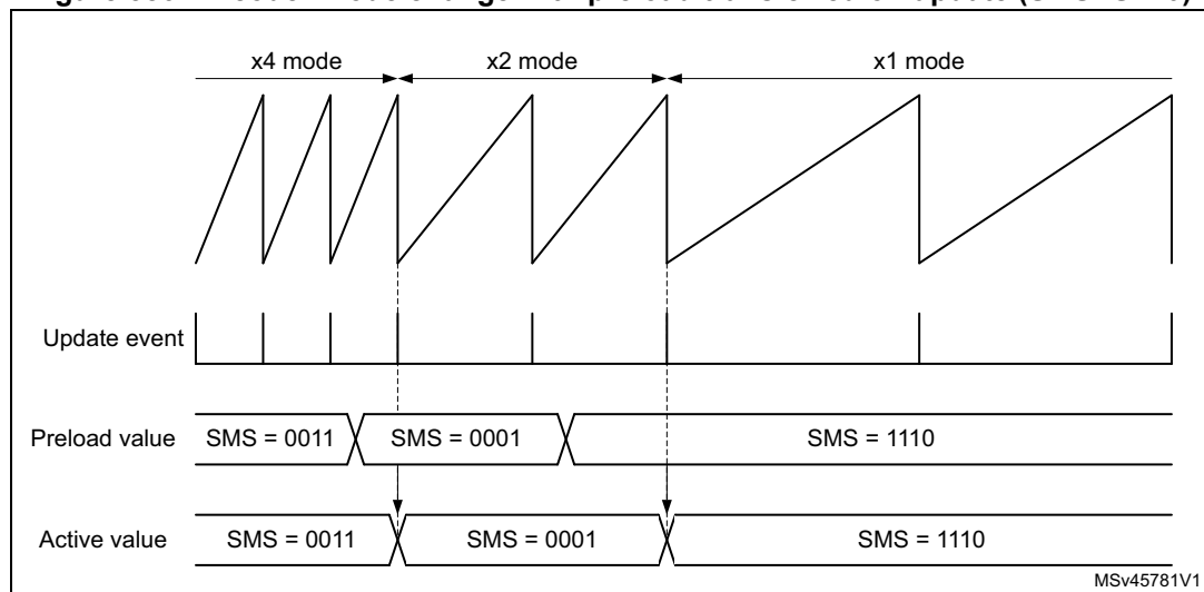
Figure 586. Encoder mode change with preload transferred on update (SMSPS = 0)
