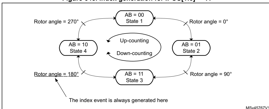
Figure 648. Index generation for IPOS[1:0] = 11
