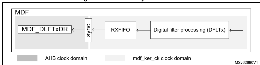
Figure 346. Data re-synchronization
