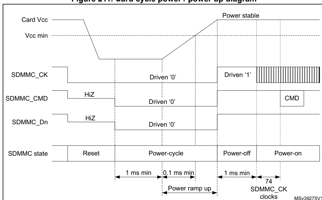
Figure 211. Card cycle power / power up diagram
