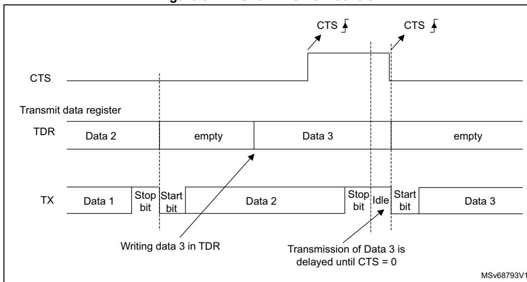
Figure 824. RS232 CTS flow control
