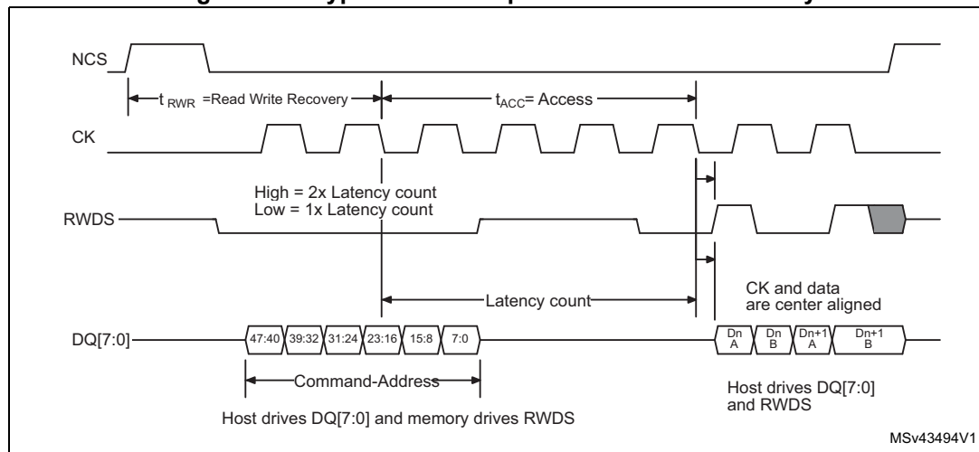
Figure 150. HyperBus write operation with initial latency
