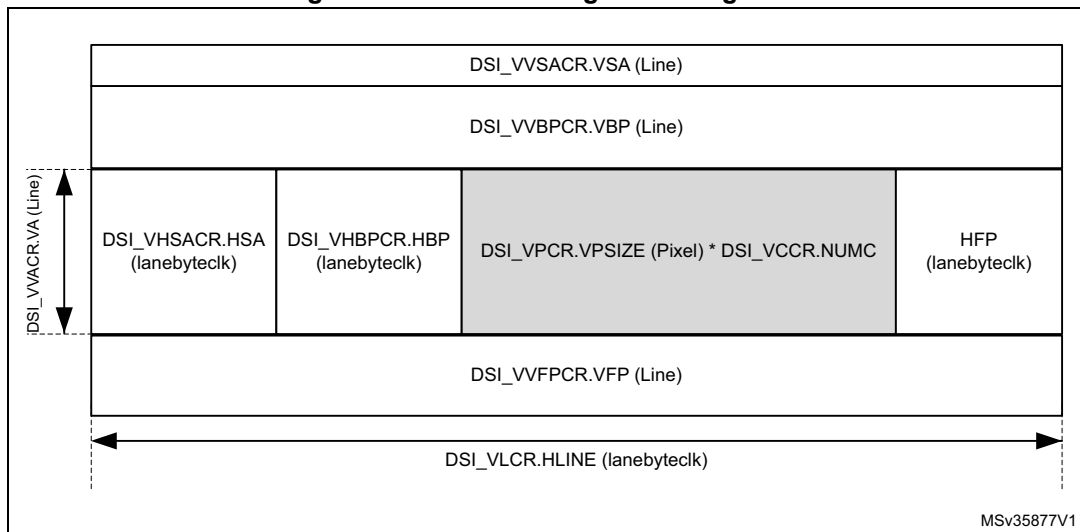
Figure 442. Frame configuration registers
