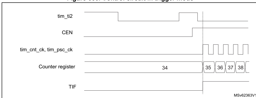
Figure 666. Control circuit in trigger mode
