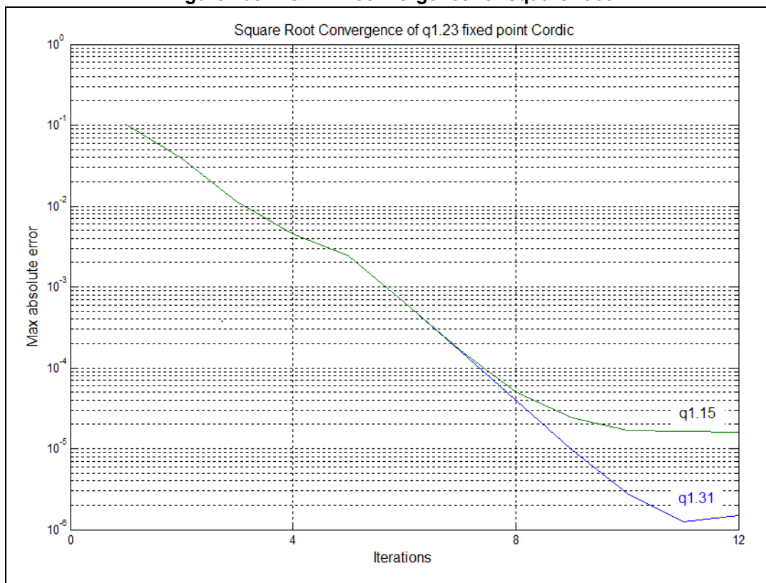
Figure 105. CORDIC convergence for square root
