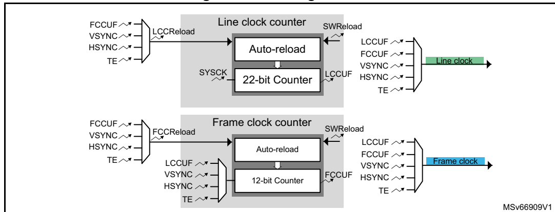
Figure 745. Clock generator
