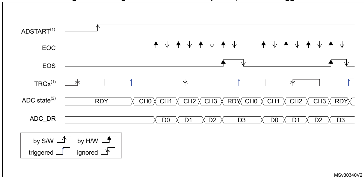
Figure 283. Single conversions of a sequence, hardware trigger
