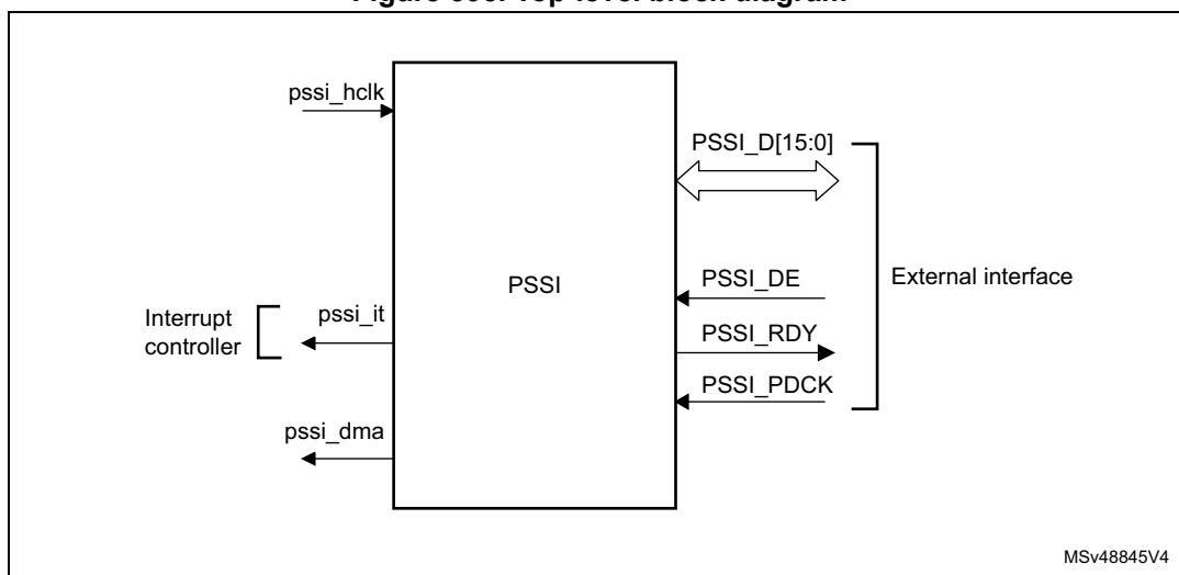
Figure 395. Top-level block diagram
