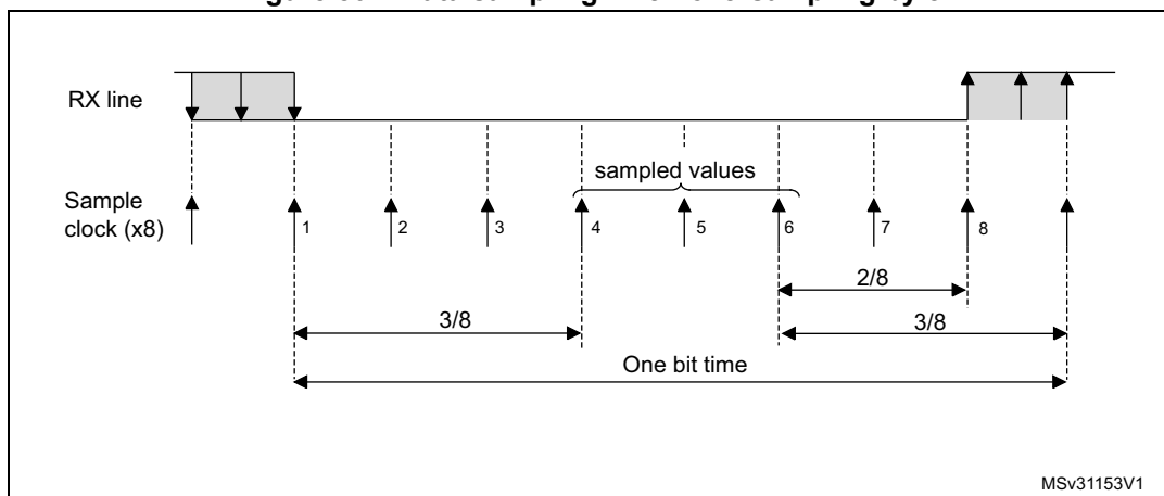
Figure 807. Data sampling when oversampling by 8
