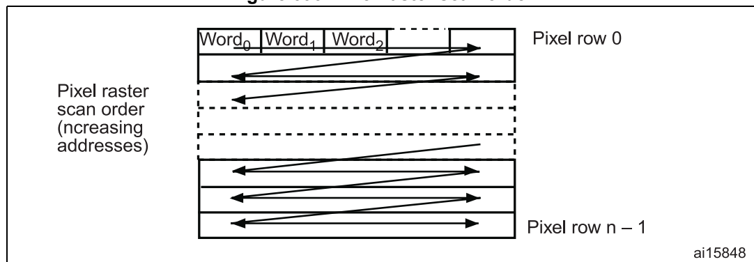
Figure 393. Pixel raster scan order
