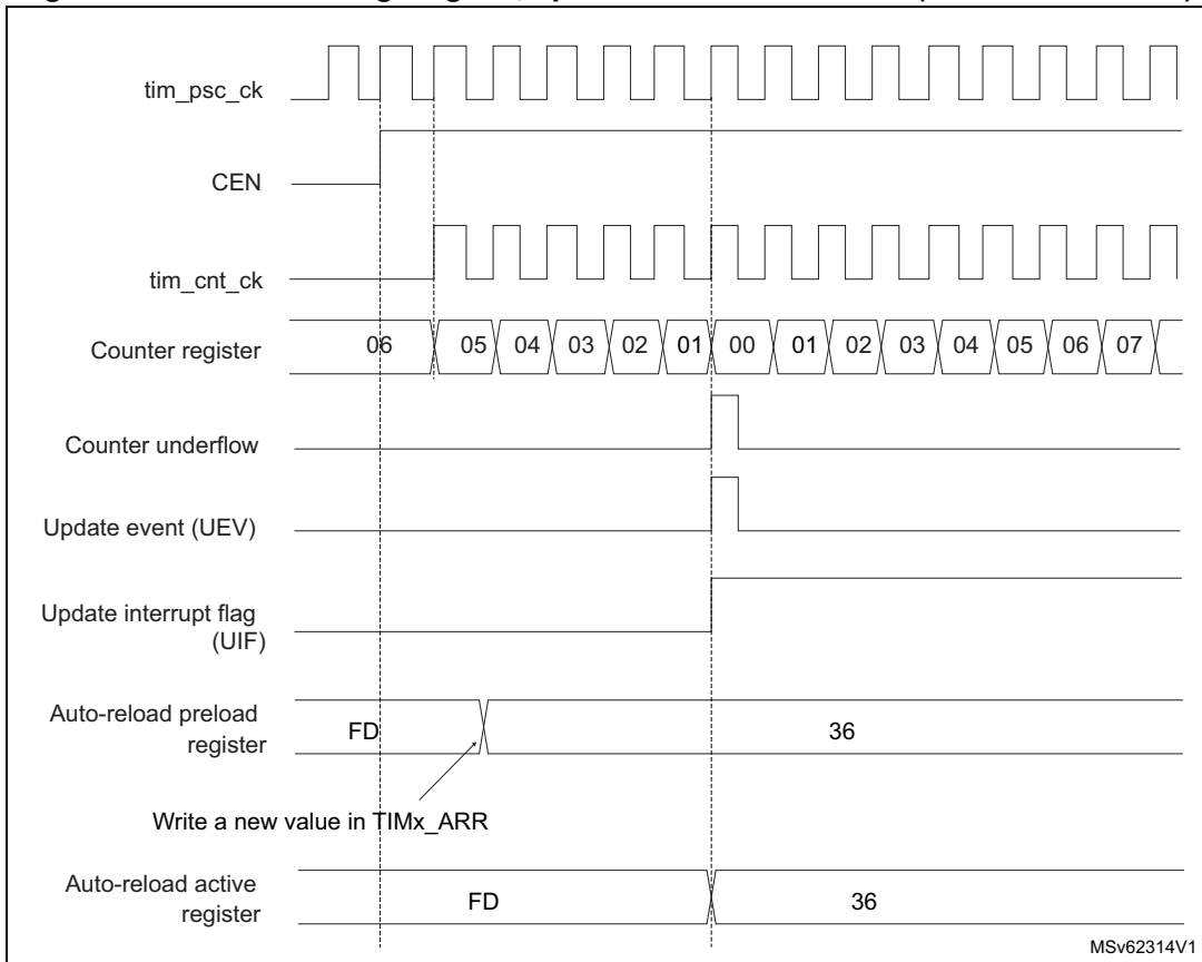
Figure 521. Counter timing diagram, update event with ARPE=1 (counter underflow)
