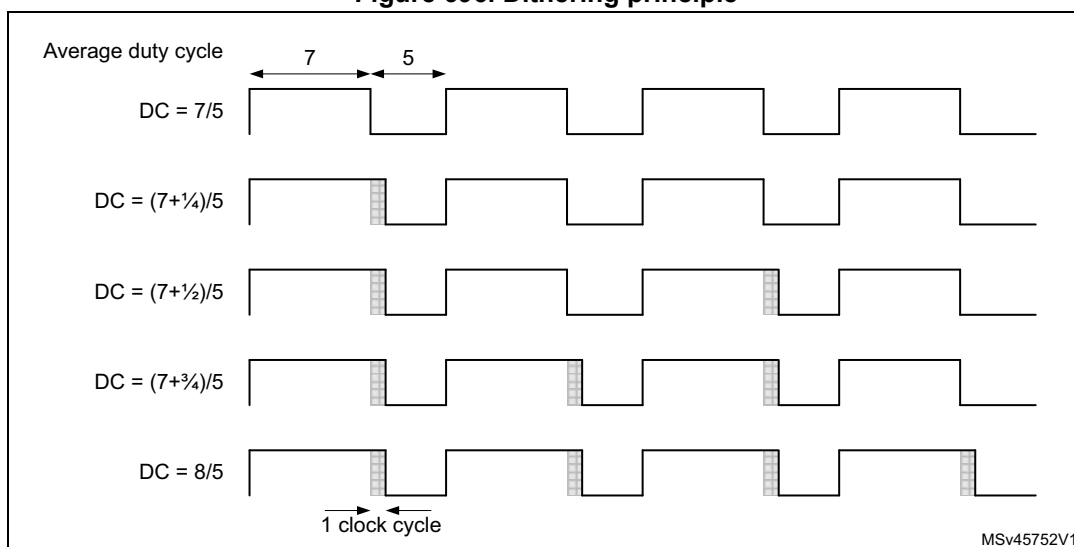
Figure 696. Dithering principle
