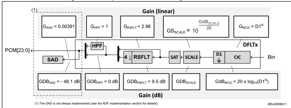
Figure 383. Simplified DFLT view with gain information
