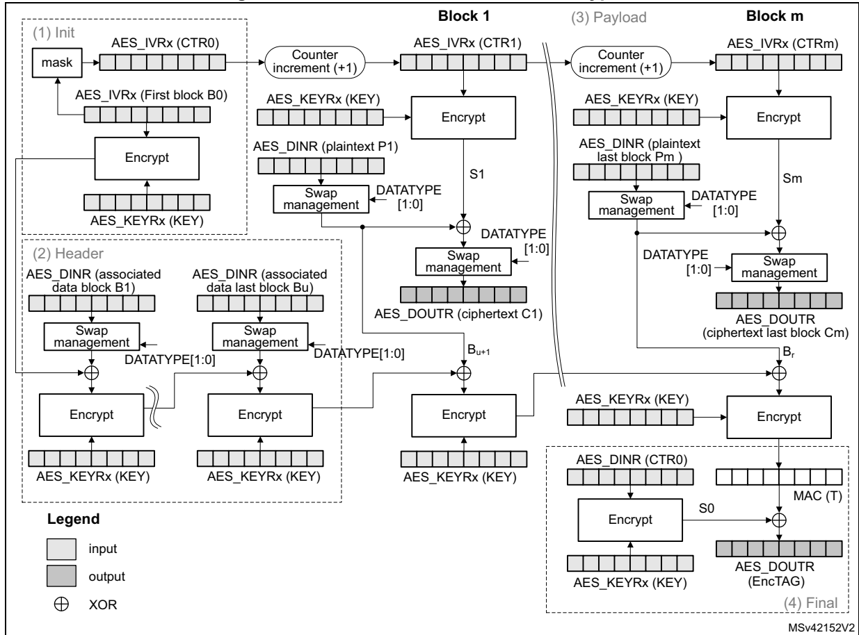
Figure 475. CCM mode authenticated encryption
