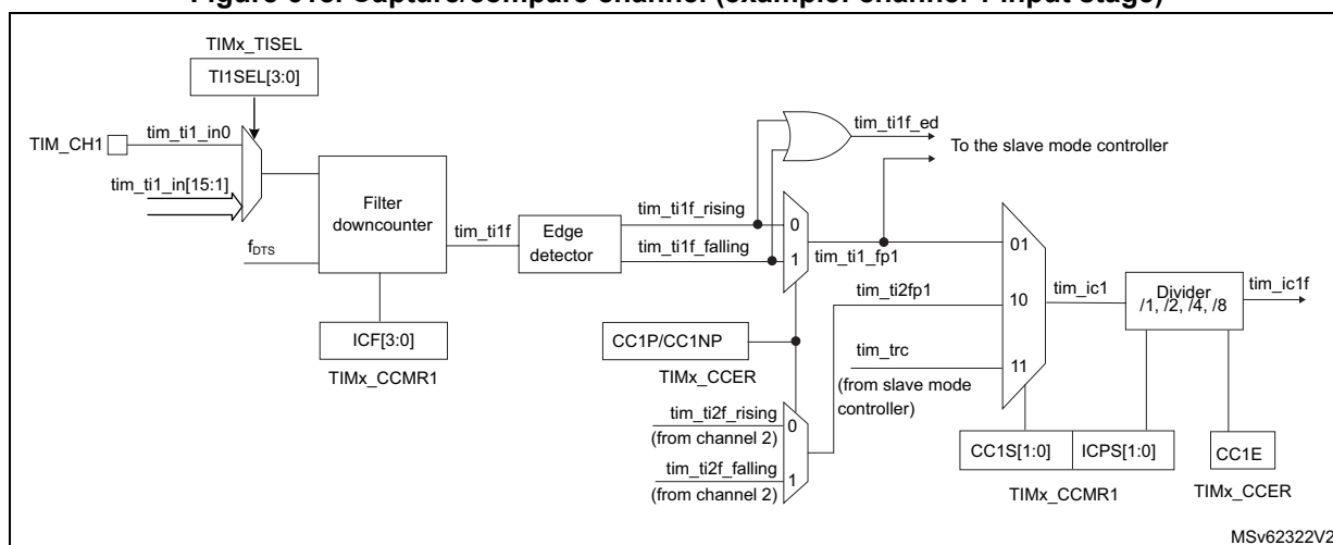
Figure 618. Capture/compare channel (example: channel 1 input stage)
