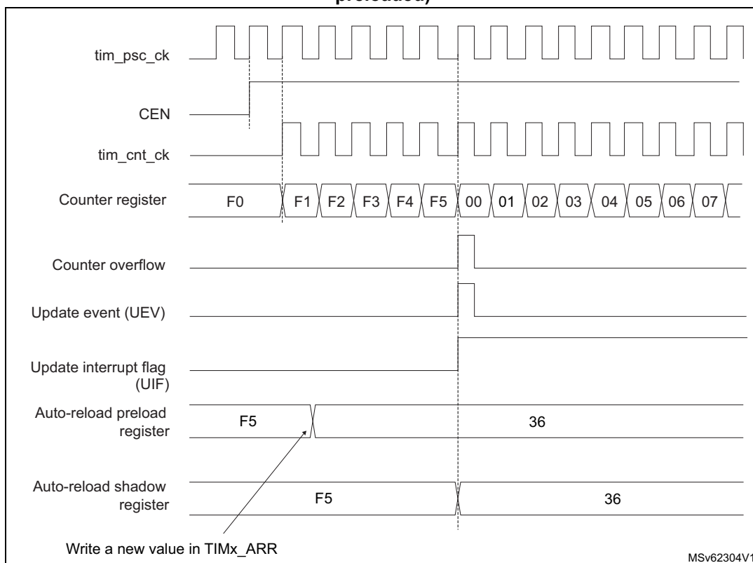
Figure 601. Counter timing diagram, Update event when ARPE=1 (TIMx_ARR preloaded)
