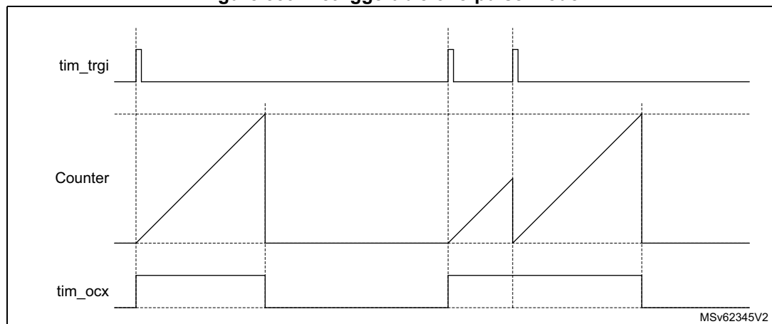
Figure 559. Retriggerable one-pulse mode
