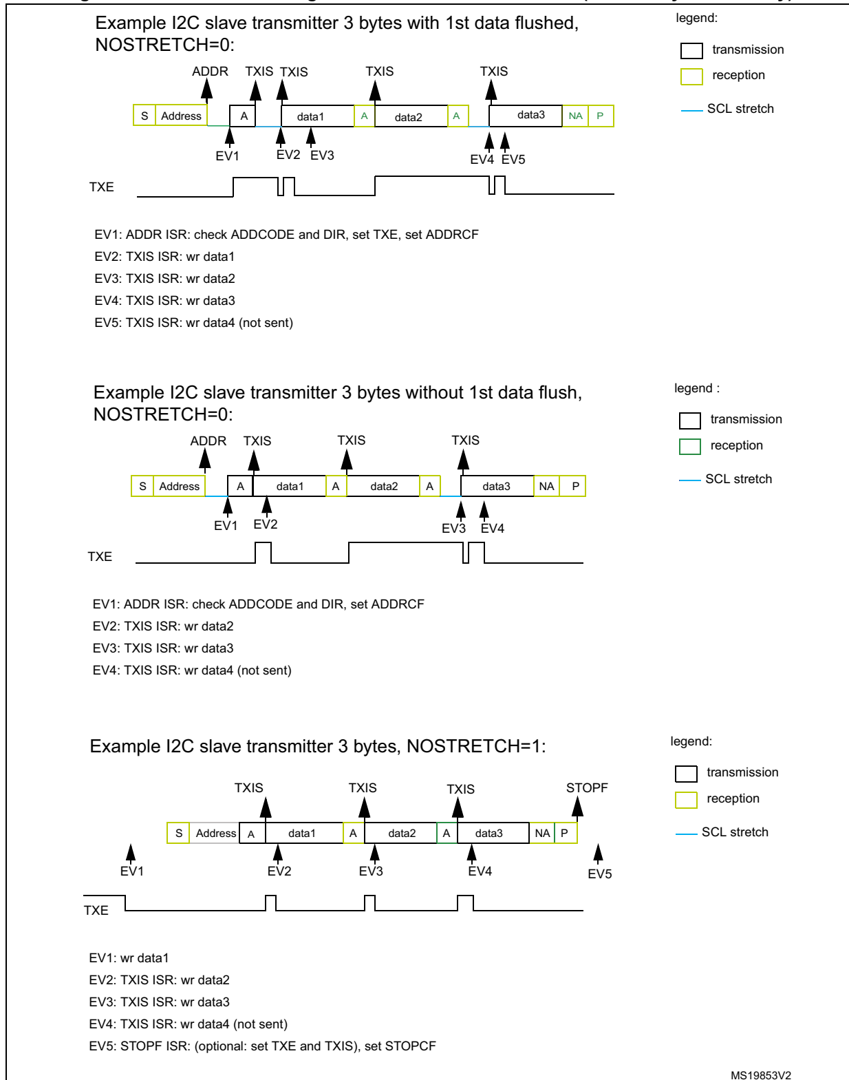
Figure 779. Transfer bus diagrams for I2C slave transmitter (mandatory events only)
