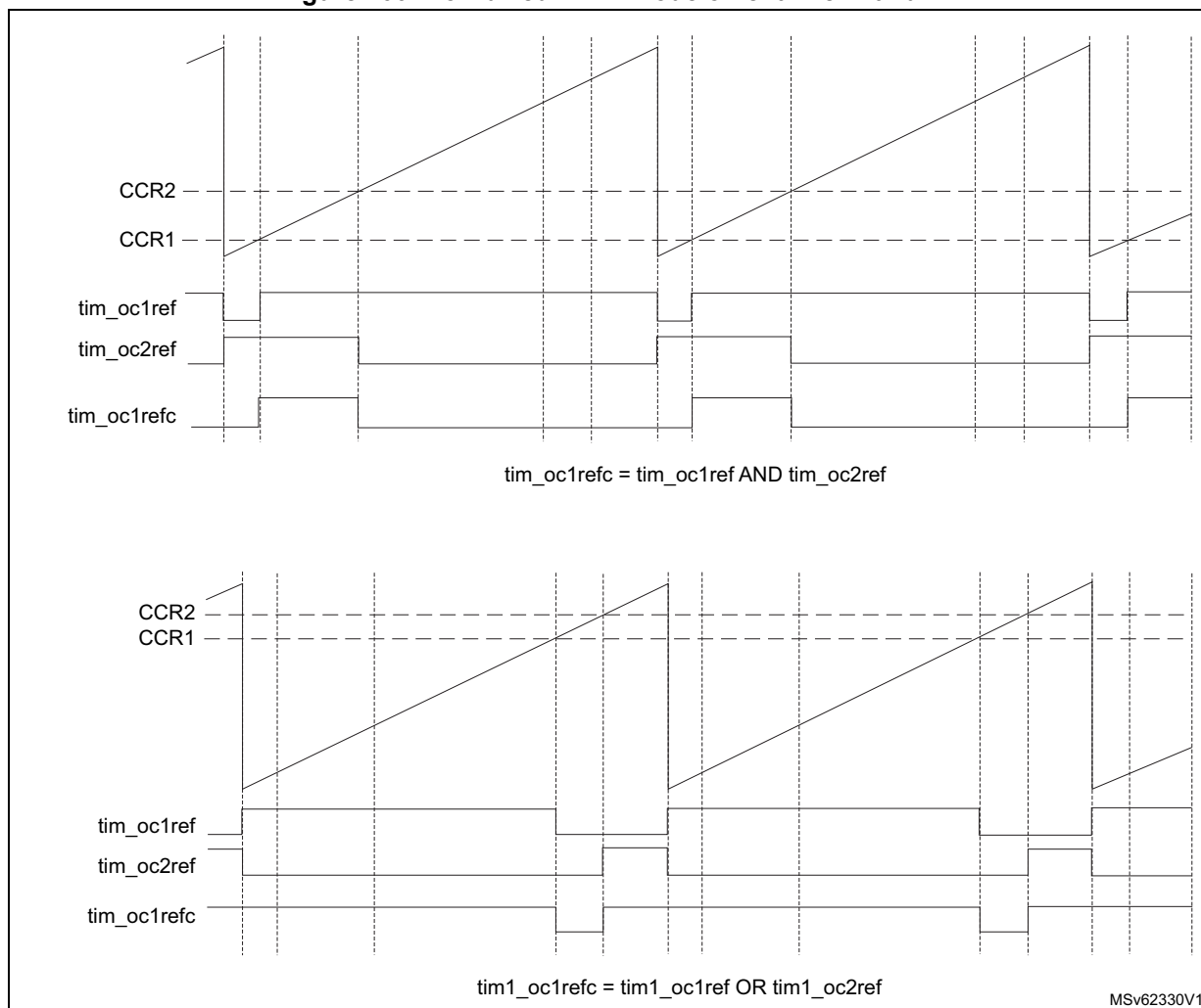
Figure 700. Combined PWM mode on channel 1 and 2
