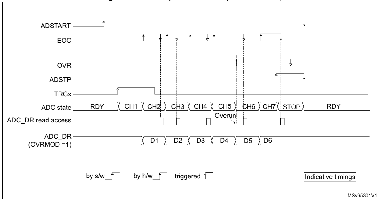
Figure 236. Example of overrun (OVRMOD = 1)
