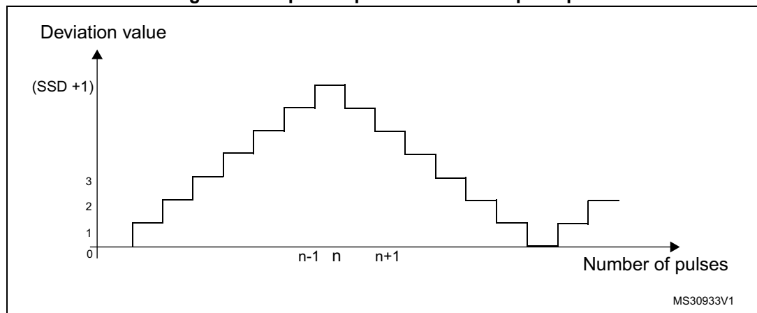
Figure 449. Spread spectrum variation principle
