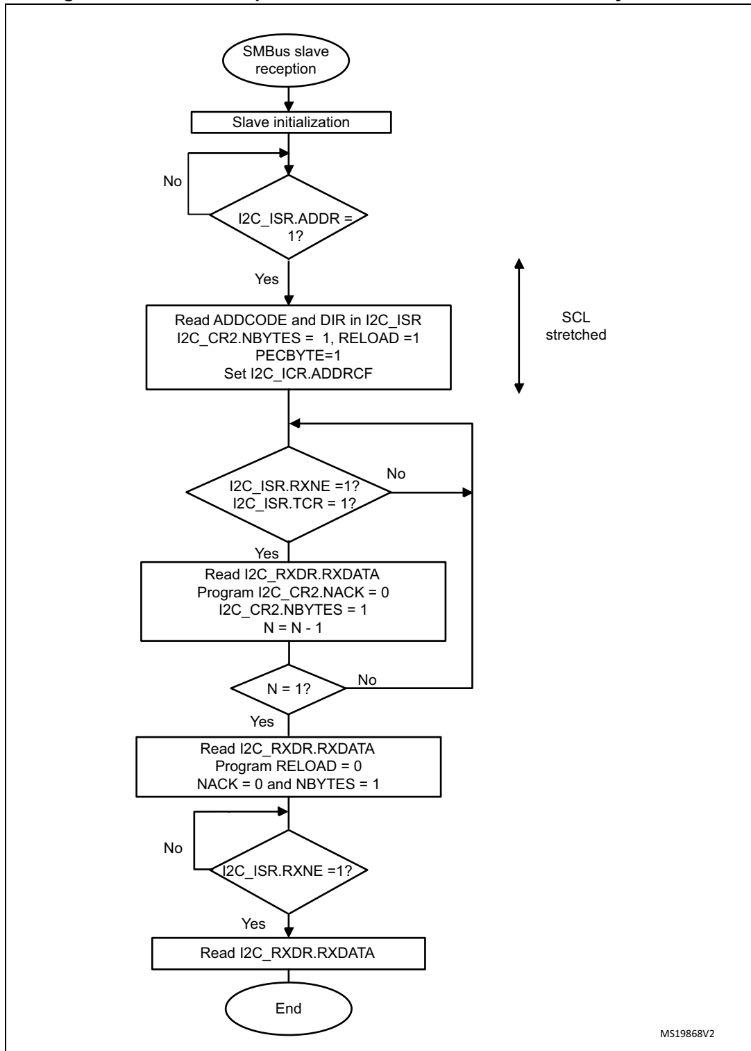
Figure 796. Transfer sequence flow for SMBus slave receiver N bytes + PEC
