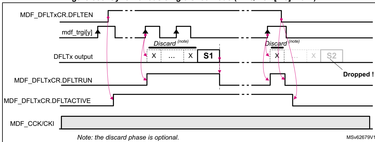
Figure 338. Synchronous single-shot mode (ACQMOD[2:0] = 011)
