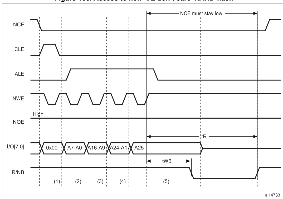
Figure 138. Access to non 'CE don't care' NAND-flash
