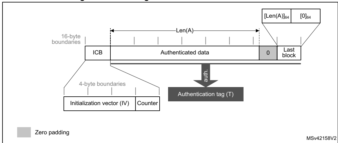
Figure 472. Message construction in GMAC mode
