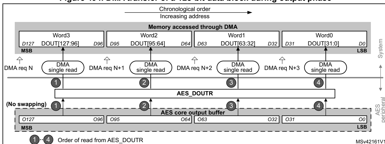
Figure 494. DMA transfer of a 128-bit data block during output phase
