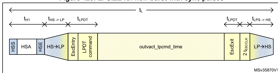
Figure 423. LPSIZE for non-burst with sync pulses
