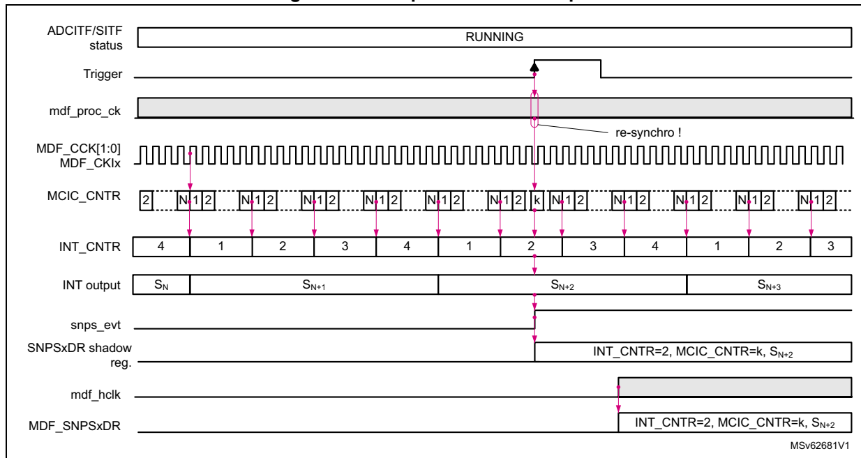
Figure 340. Snapshot mode example
