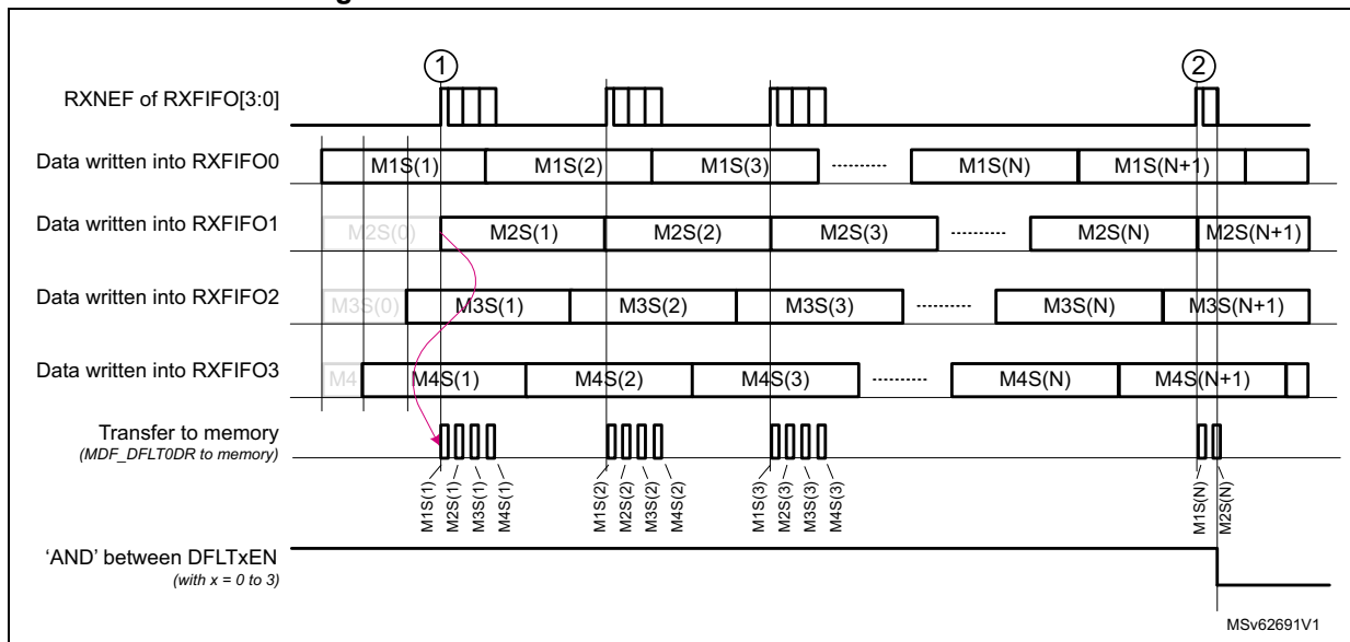
Figure 347. Data transfer in interleaved-transfer mode
