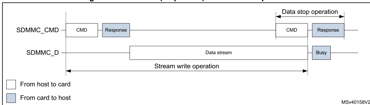
Figure 184. SDMMC (sequential) stream write operation
