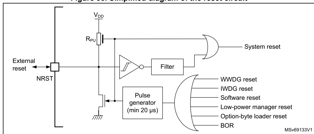
Figure 35. Simplified diagram of the reset circuit
