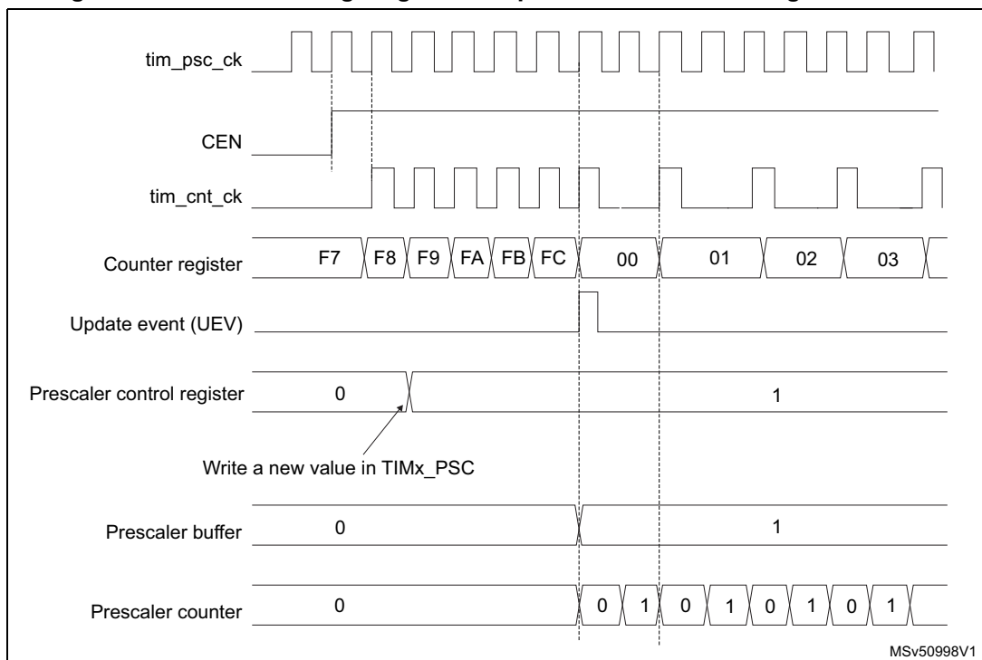
Figure 594. Counter timing diagram with prescaler division change from 1 to 2
