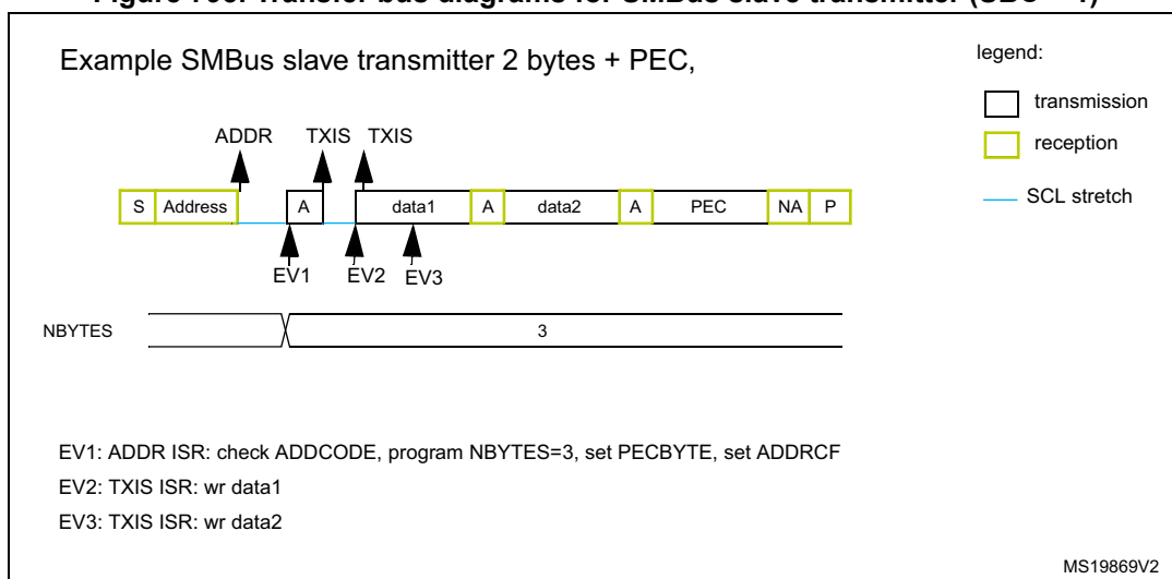
Figure 795. Transfer bus diagrams for SMBus slave transmitter (SBC = 1)
