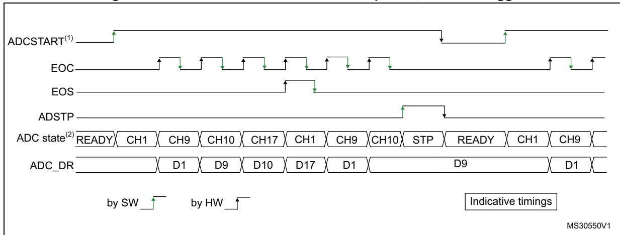
Figure 228. Continuous conversion of a sequence, software trigger
