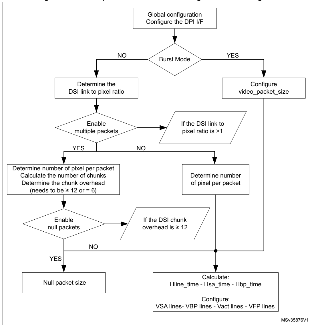
Figure 440. Video packet transmission configuration flow diagram
