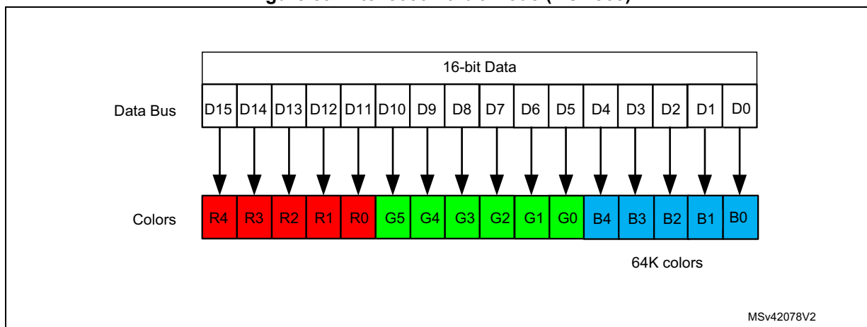
Figure 89. Intel 8080 16-bit mode (RGB565)
