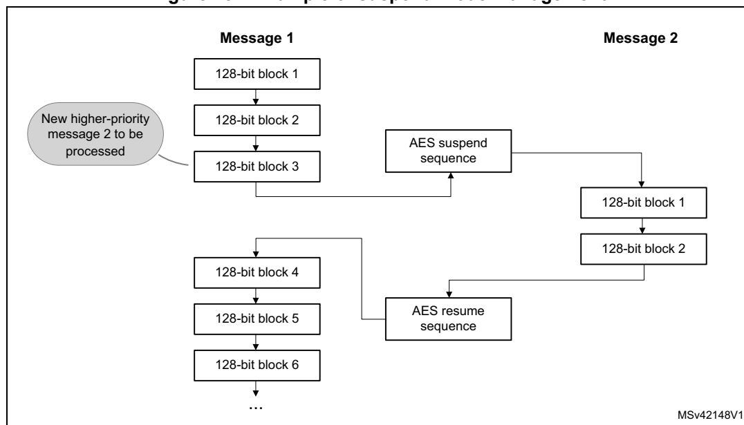
Figure 482. Example of suspend mode management
