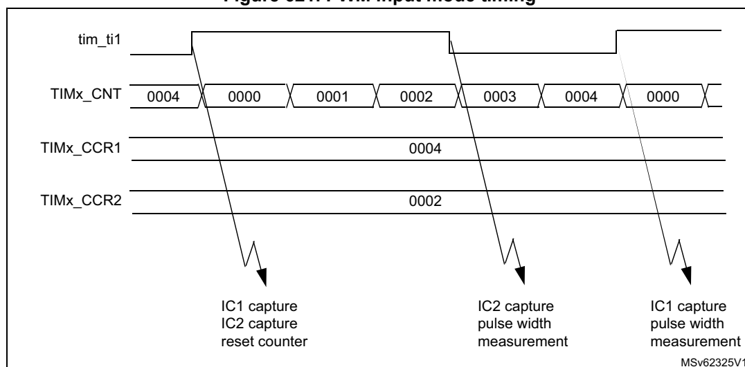
Figure 621. PWM input mode timing
