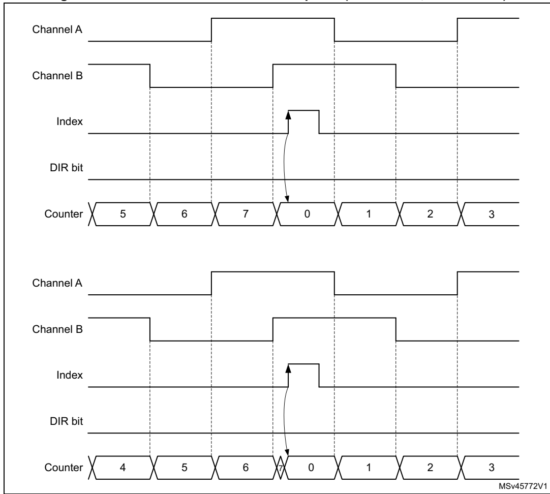
Figure 576. Counter reset Narrow index pulse (closer view, ARR = 0x07)
