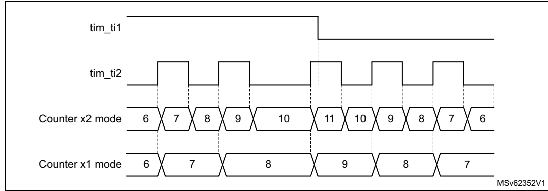
Figure 566. Direction plus clock encoder mode
