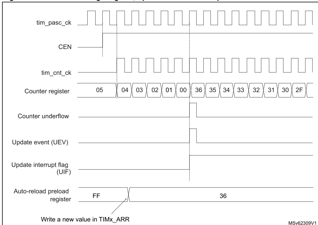
Figure 516. Counter timing diagram, update event when repetition counter is not used
