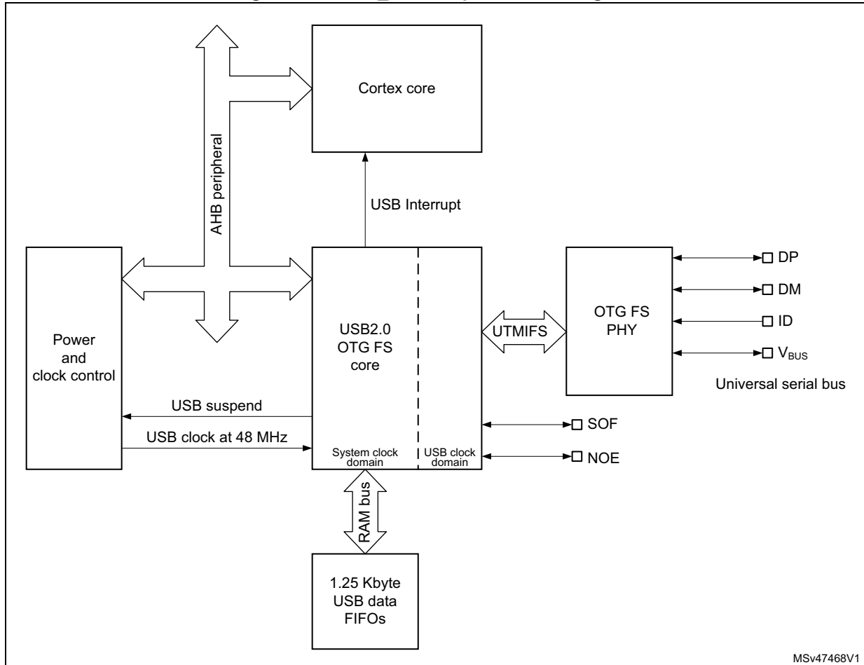
Figure 884. OTG_FS full-speed block diagram
