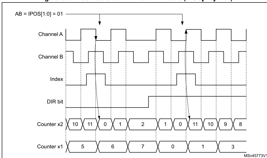
Figure 654. Index behavior in x1 and x2 mode (IPOS[1:0] = 01)
