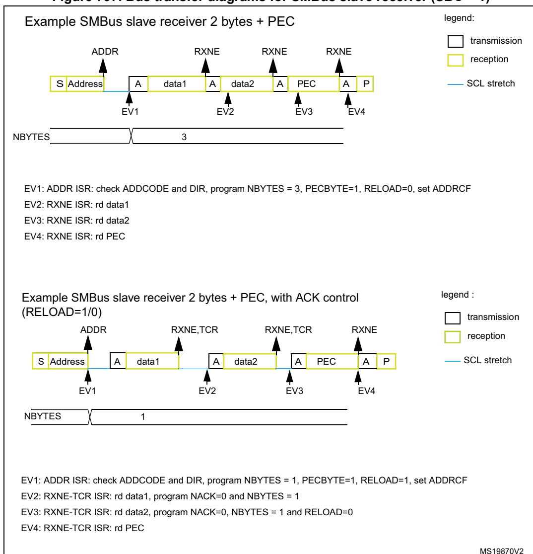
Figure 797. Bus transfer diagrams for SMBus slave receiver (SBC = 1)
