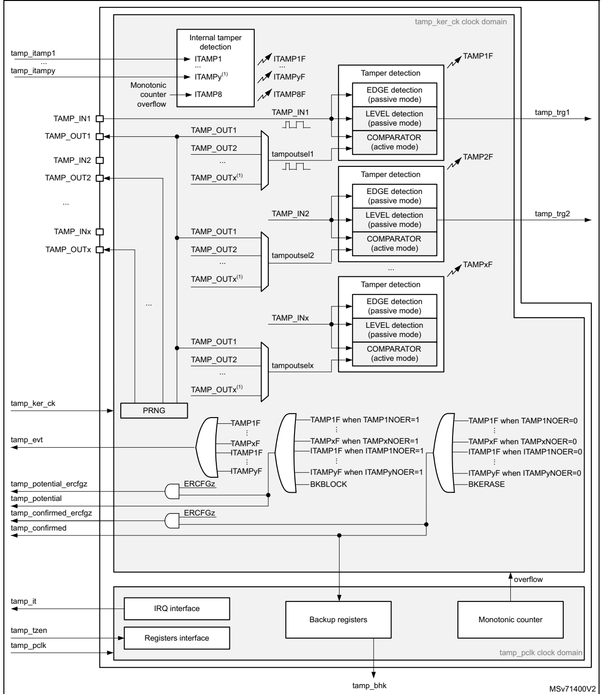
Figure 767. TAMP block diagram
