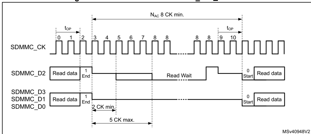
Figure 204. Read Wait with SDMMC_CK ≥ 50 MHz
