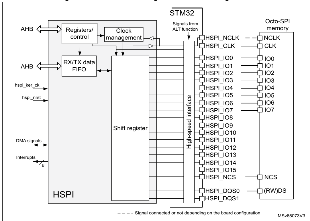
Figure 162. HSPI block diagram for octal configuration
