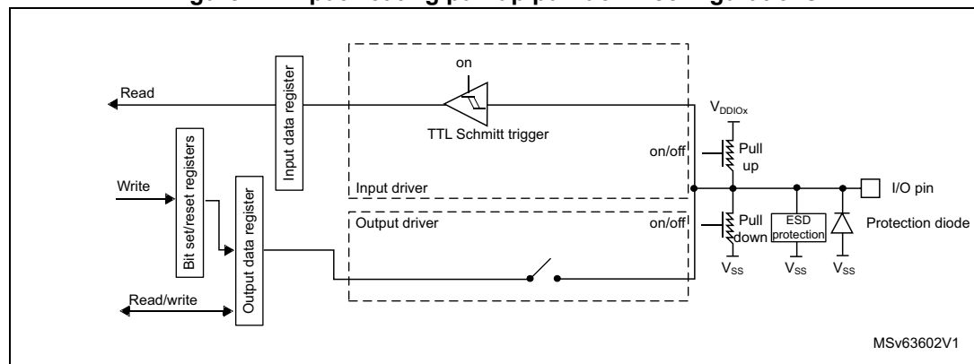
Figure 44. Input floating/pull-up/pull-down configurations
