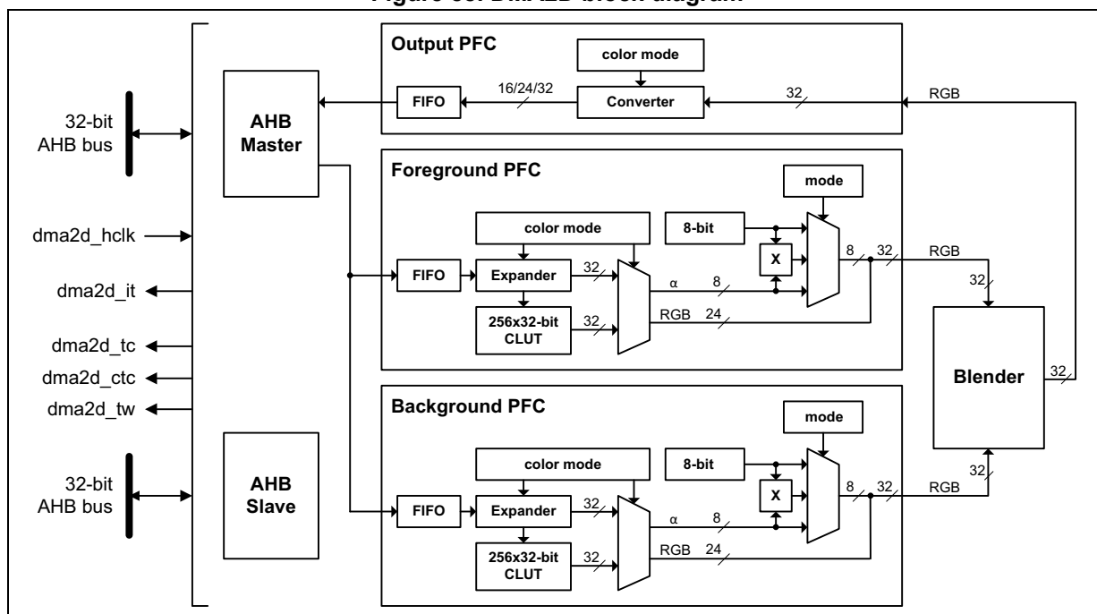
Figure 88. DMA2D block diagram
