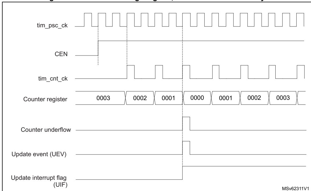
Figure 608. Counter timing diagram, internal clock divided by 2
