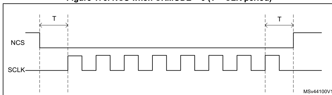
Figure 176. NCS when CKMODE = 0 (T = CLK period)
