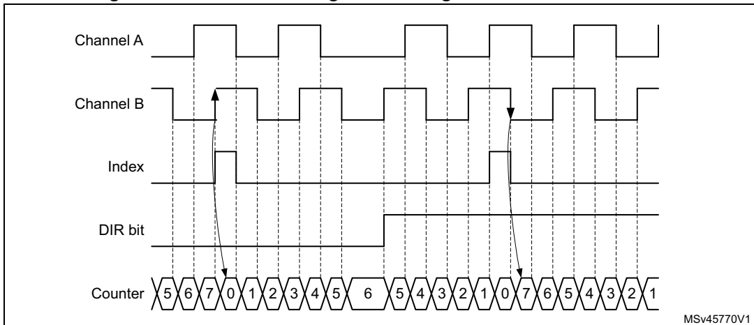
Figure 574. Counter reading with index gated on channel A and B
