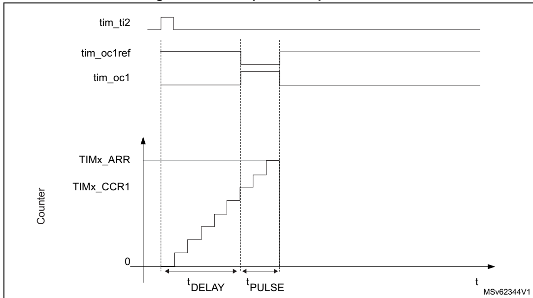
Figure 558. Example of one pulse mode.
