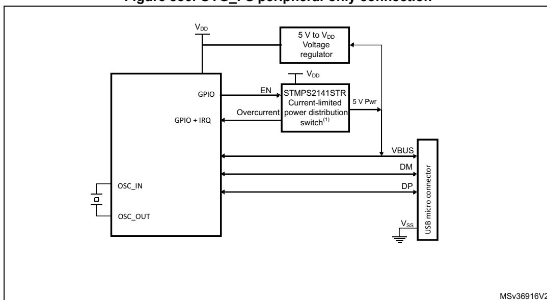
Figure 886. OTG_FS peripheral-only connection
