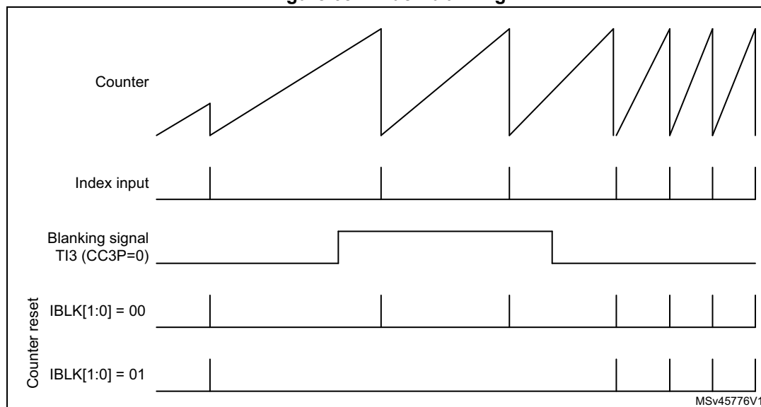
Figure 657. Index blanking
