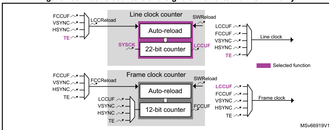
Figure 755. Active counters and signals with external CSYNC only
