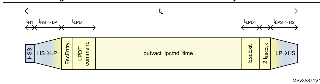
Figure 424. LPSIZE for burst or non-burst with sync events
