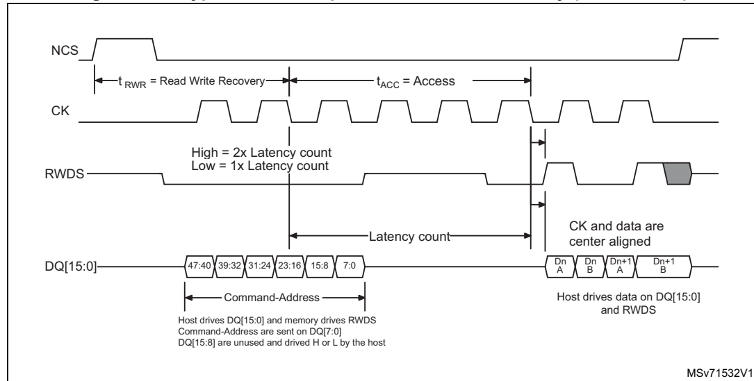
Figure 175. HyperBus write operation with initial latency (16-bit mode)
