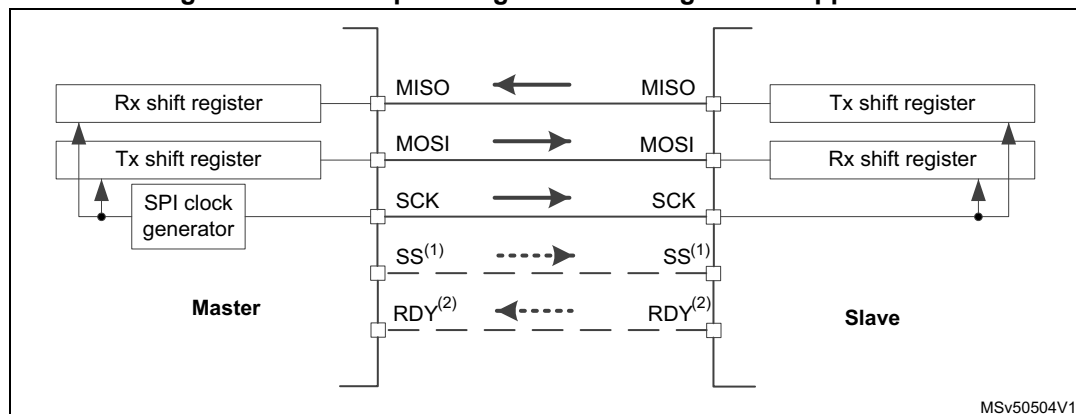
Figure 838. Full-duplex single master/ single slave application
