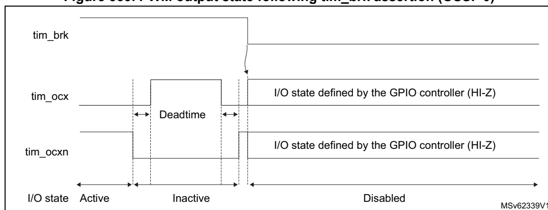
Figure 553. PWM output state following tim_brk assertion (OSSI=0)
