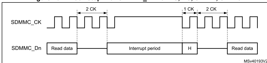
Figure 201. Clock stop with SDMMC_CK for DS, HS, SDR12, SDR25
