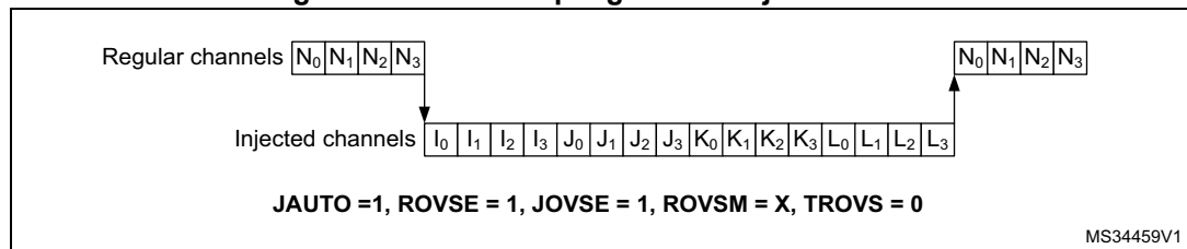
Figure 252. Oversampling in auto-injected mode
