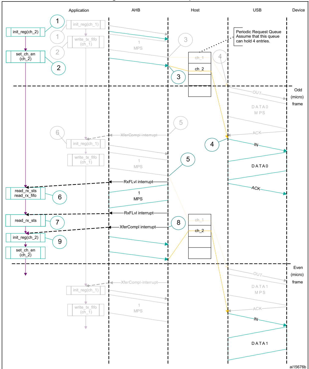
Figure 923. Normal interrupt IN
