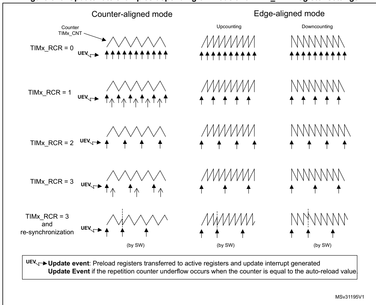
Figure 523. Update rate examples depending on mode and TIMx_RCR register settings
