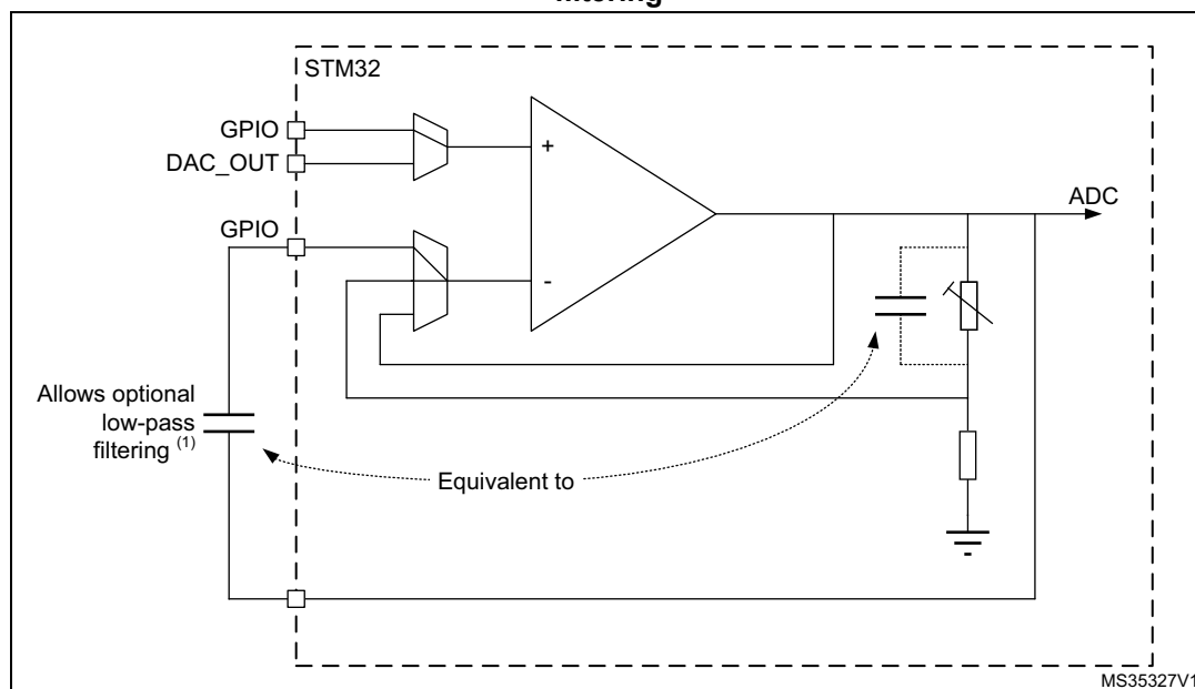
Figure 320. PGA mode, internal gain setting (x2/x4/x8/x16), inverting input used for filtering
