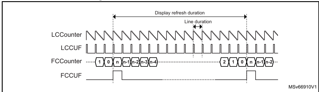
Figure 746. Waveforms in standalone
