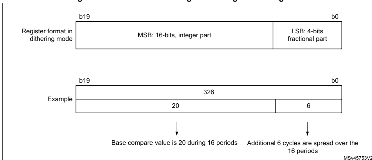
Figure 697. Data format and register coding in dithering mode
