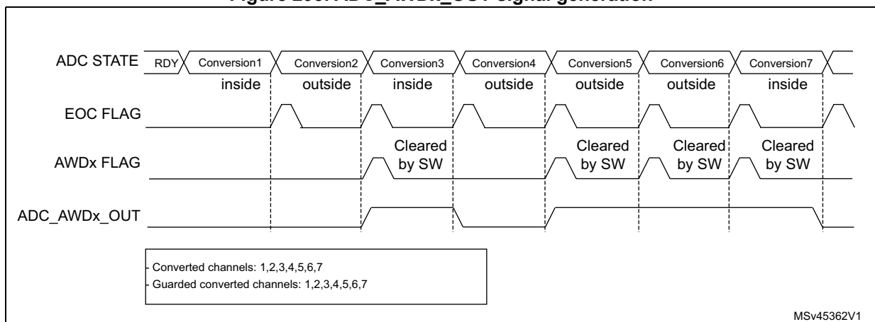
Figure 293. ADC_AWDx_OUT signal generation
