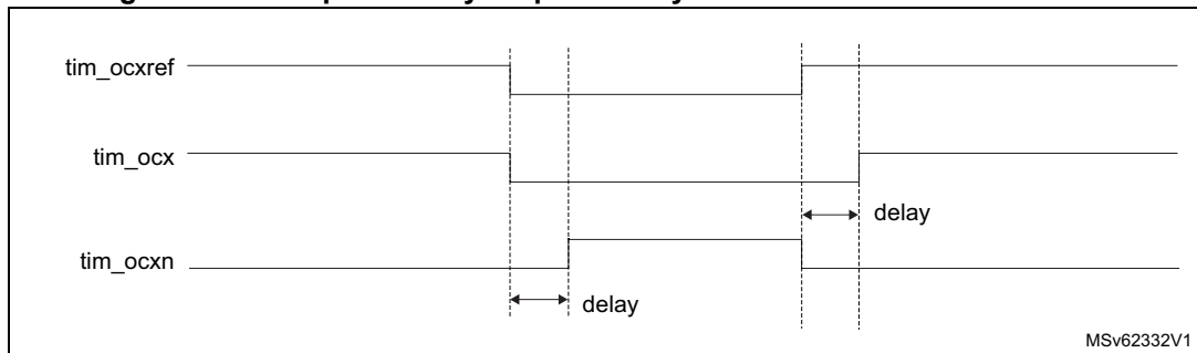
Figure 701. Complementary output with symmetrical dead-time insertion.
