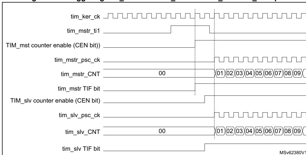
Figure 674. Triggering TIM_mstr and TIM_slv with TIM_mstr tim_ti1 input
