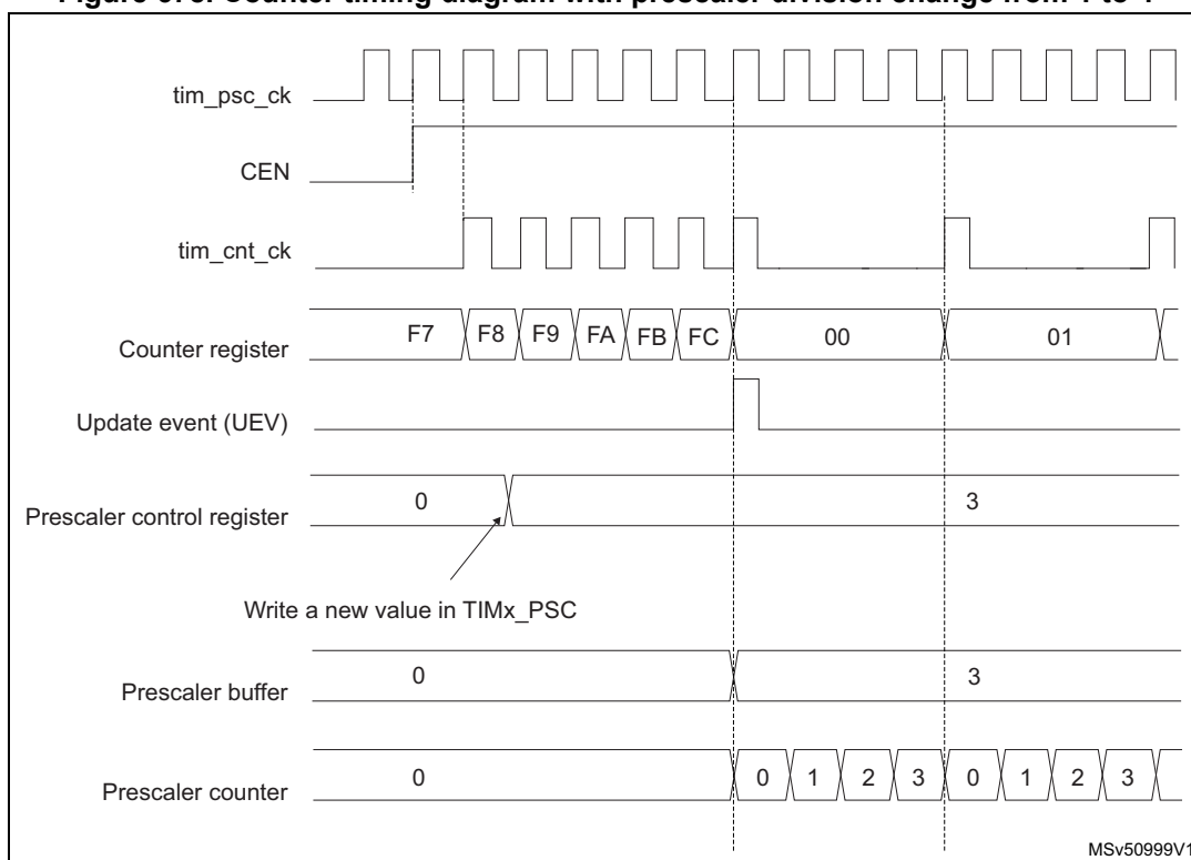
Figure 678. Counter timing diagram with prescaler division change from 1 to 4
