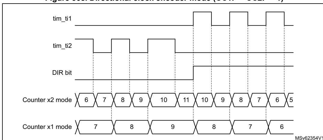
Figure 568. Directional clock encoder mode (CC1P = CC2P = 1)
