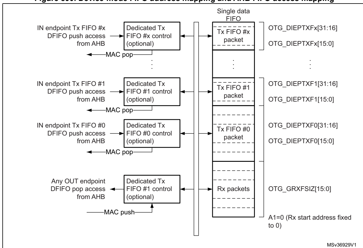
Figure 890. Device-mode FIFO address mapping and AHB FIFO access mapping
