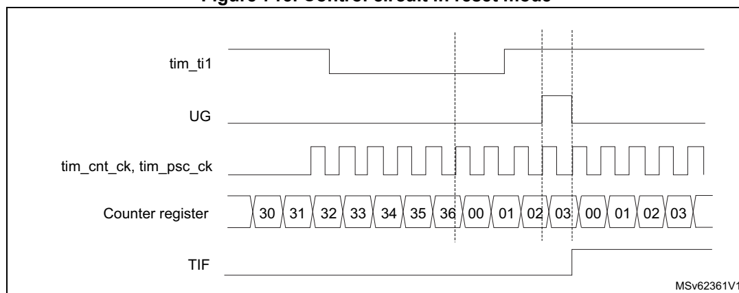
Figure 713. Control circuit in reset mode
