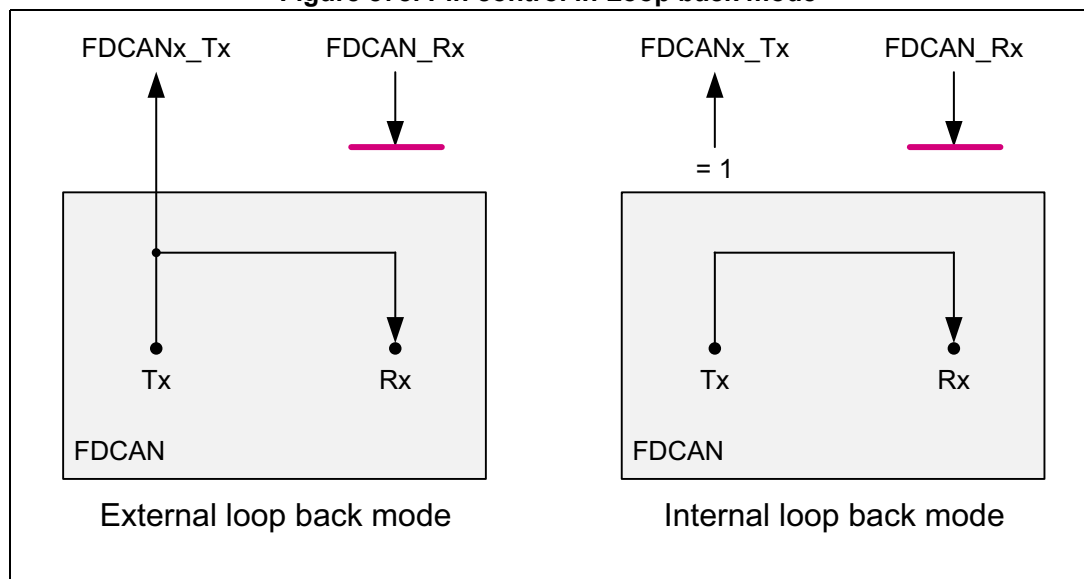
Figure 878. Pin control in Loop back mode
