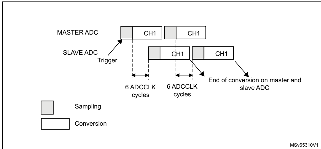
Figure 256. Interleaved mode on one channel in continuous conversion mode: dual ADC mode
