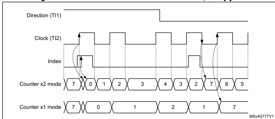
Figure 659. Index behavior in directional clock mode, IPOS[0] = 1
