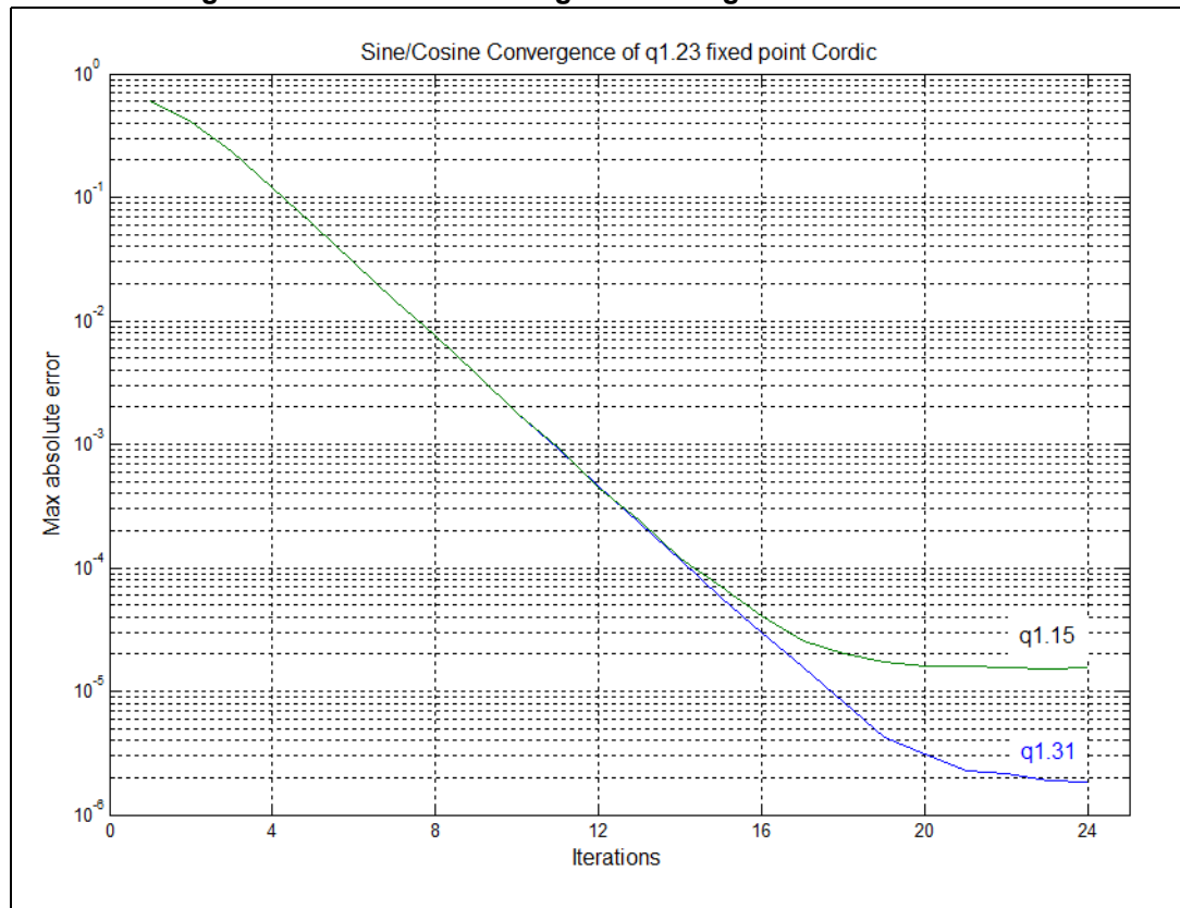
Figure 103. CORDIC convergence for trigonometric functions
