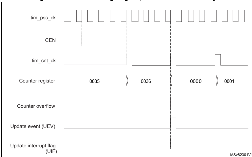
Figure 722. Counter timing diagram, internal clock divided by 4
