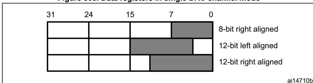
Figure 303. Data registers in single DAC channel mode
