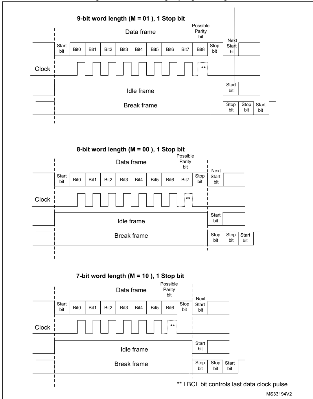
Figure 801. Word length programming
