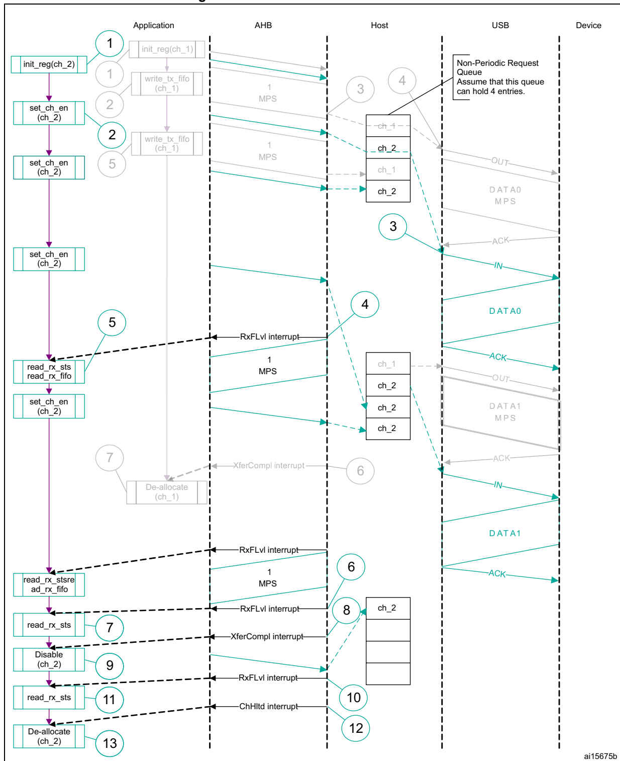
Figure 896. Bulk/control IN transactions
