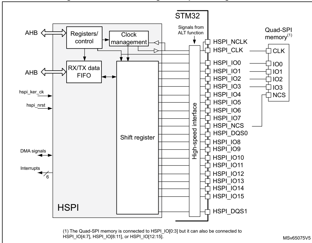
Figure 163. HSPI block diagram in quad configuration
