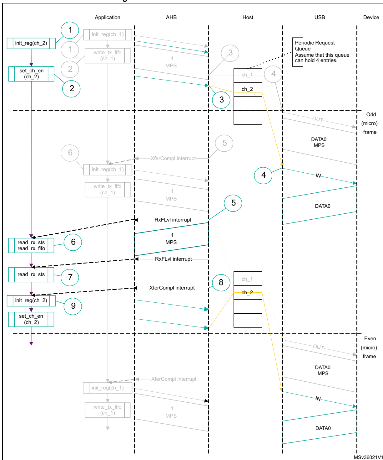
Figure 925. Isochronous IN transactions
