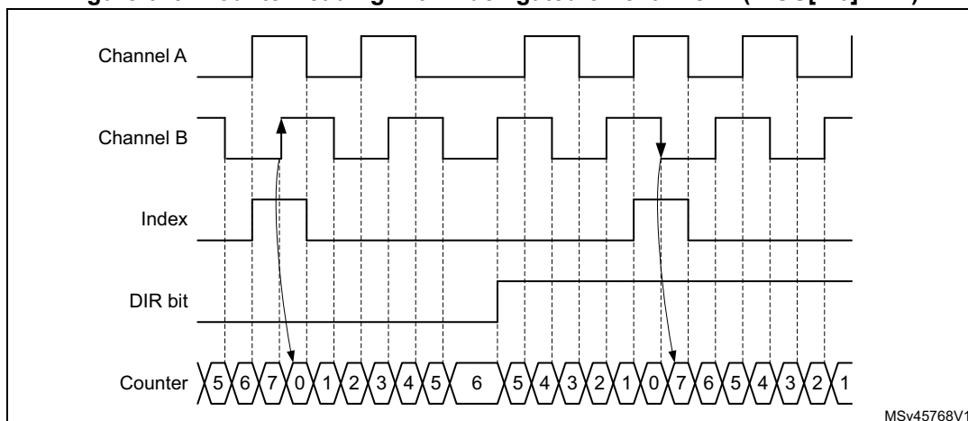
Figure 649. Counter reading with index gated on channel A (IPOS[1:0] = 11)
