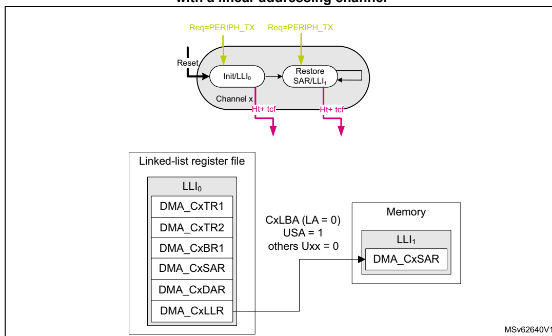
Figure 68. GPDMA circular buffer programming: update of the memory start address with a linear addressing channel
