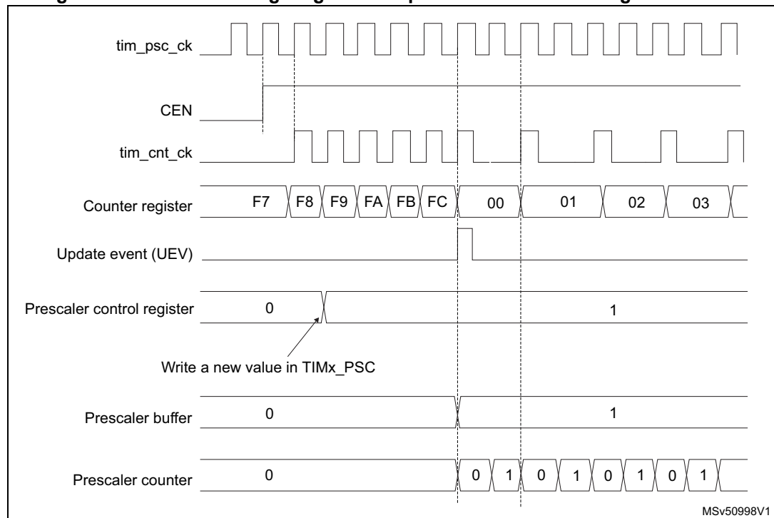
Figure 677. Counter timing diagram with prescaler division change from 1 to 2
