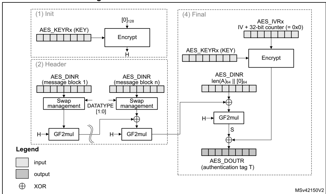
Figure 473. GMAC authentication mode
