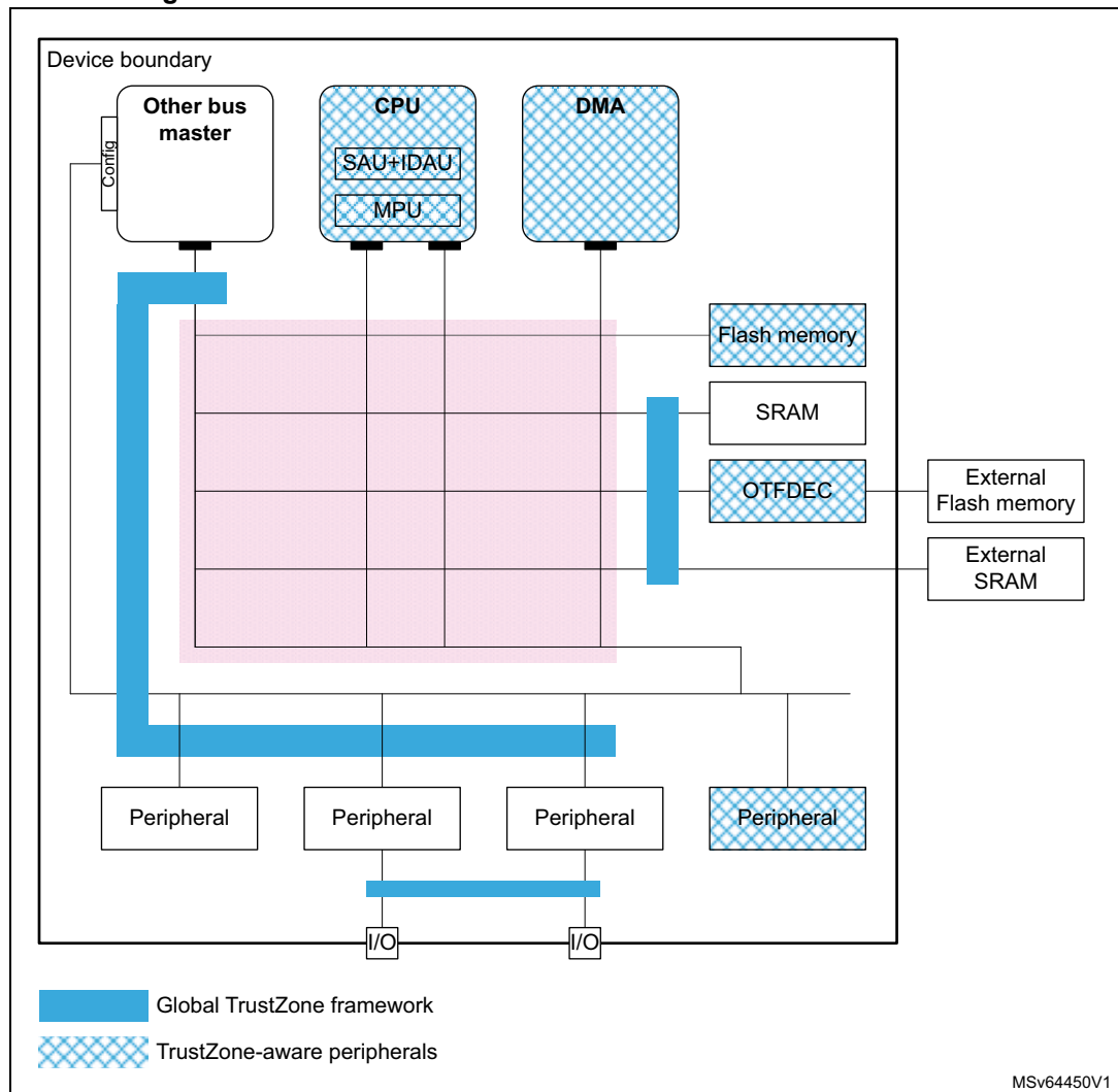
Figure 10. Global TrustZone framework and TrustZone awareness
