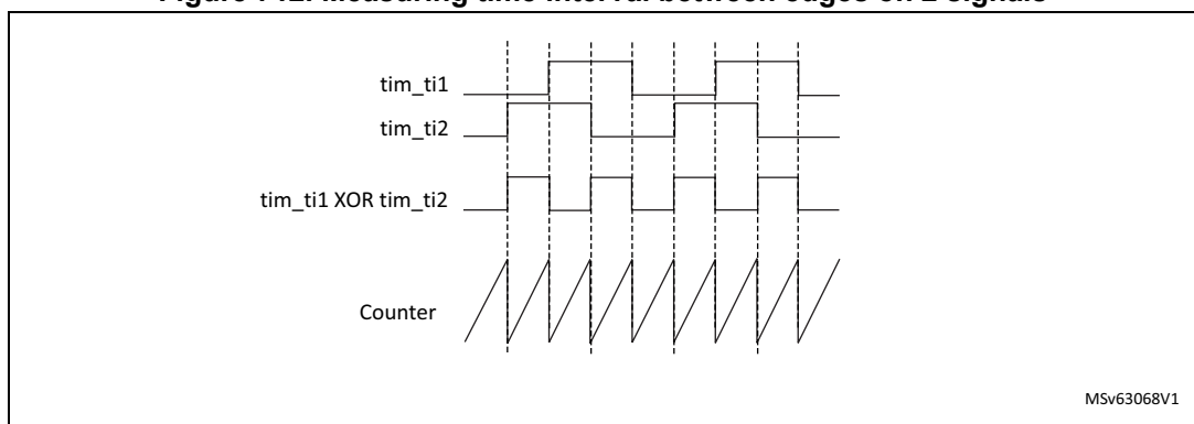
Figure 712. Measuring time interval between edges on 2 signals
