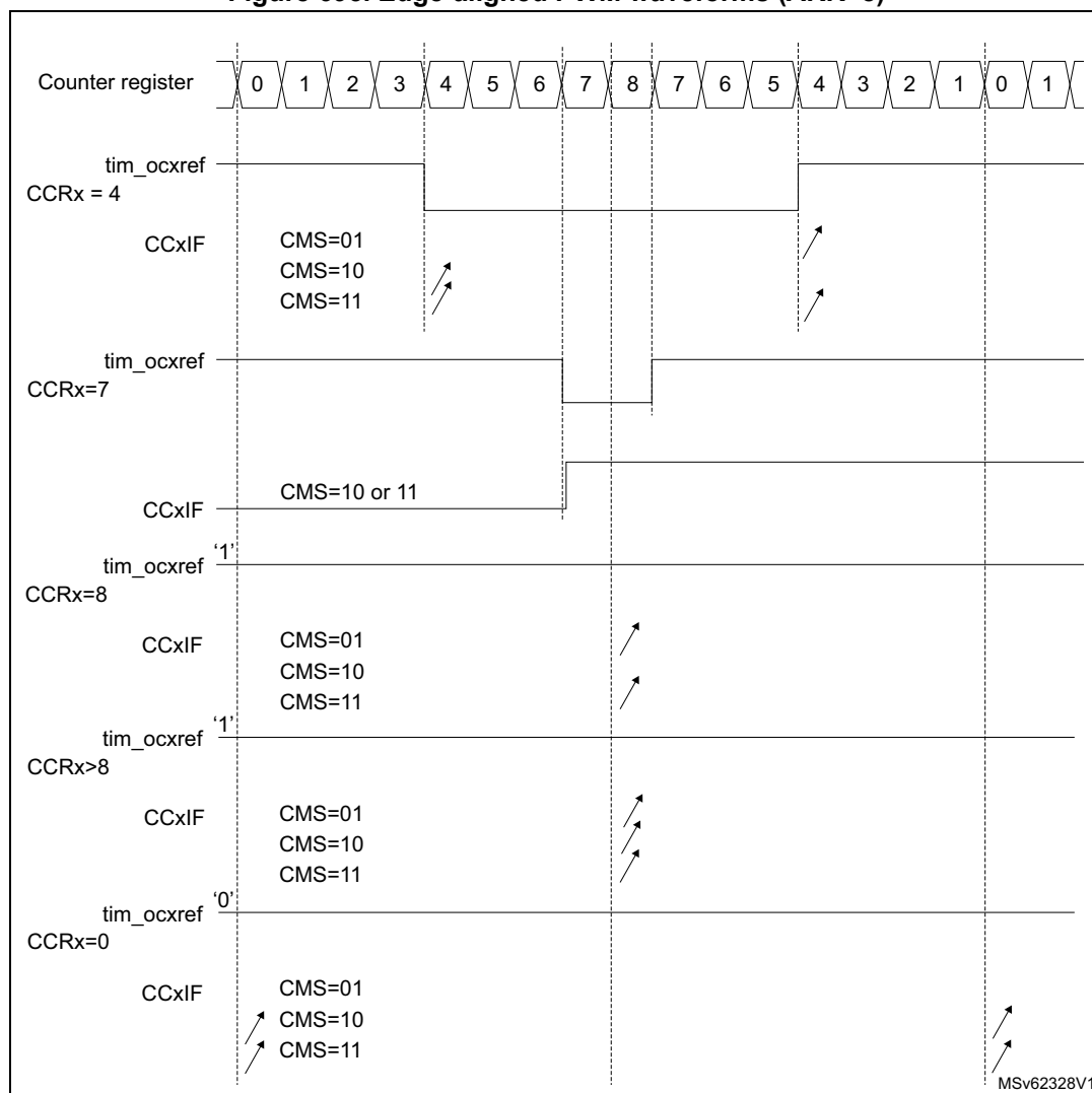
Figure 695. Edge-aligned PWM waveforms (ARR=8)
