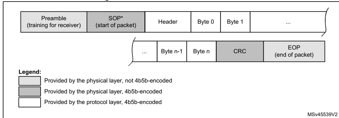
Figure 940. Packet format
