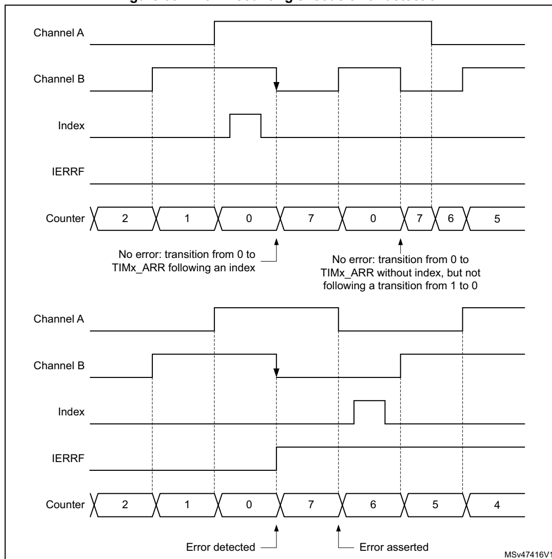
Figure 662. Down-counting encode error detection
