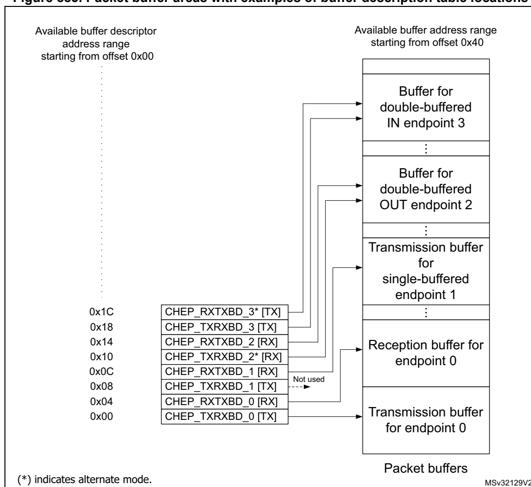
Figure 883. Packet buffer areas with examples of buffer description table locations
