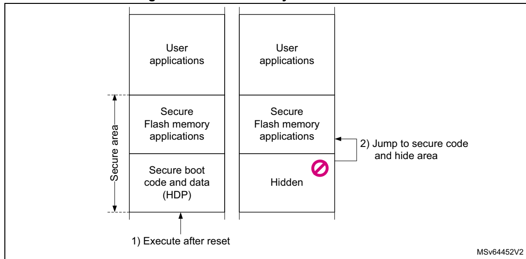
Figure 12. Flash memory secure HDP area
