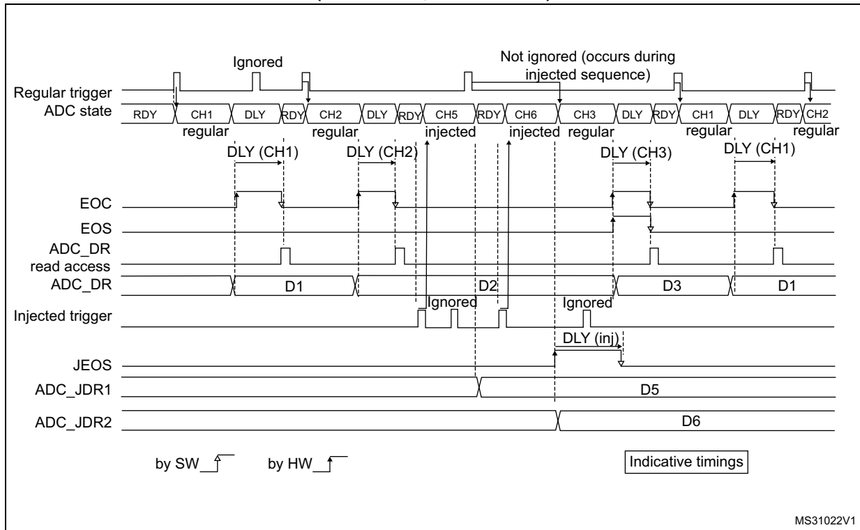
Figure 239. AUTDLY = 1, regular hardware conversions interrupted by injected conversions (DISCEN = 1, JDISCEN = 1)
