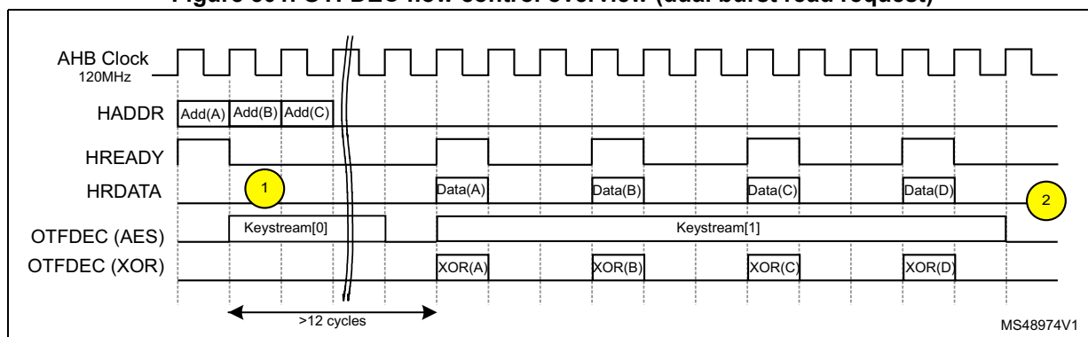
Figure 501. OTFDEC flow control overview (dual burst read request)
