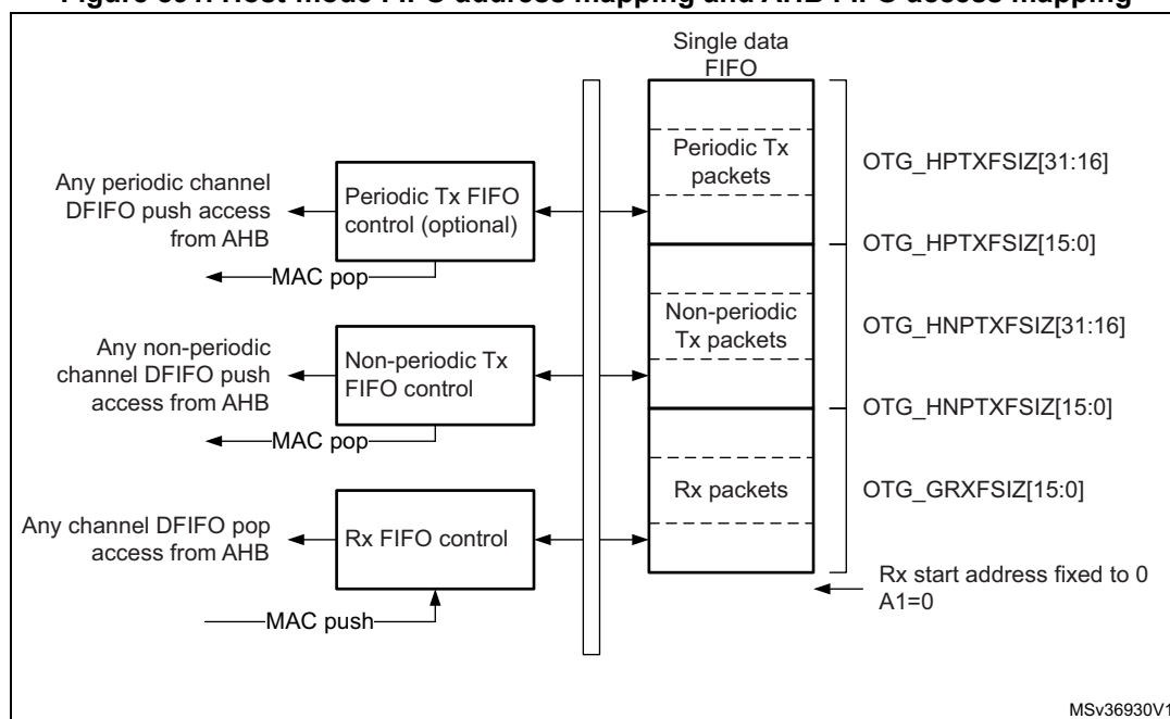
Figure 891. Host-mode FIFO address mapping and AHB FIFO access mapping
