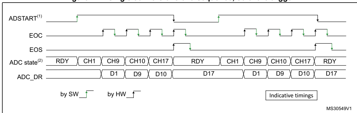
Figure 227. Single conversions of a sequence, software trigger
