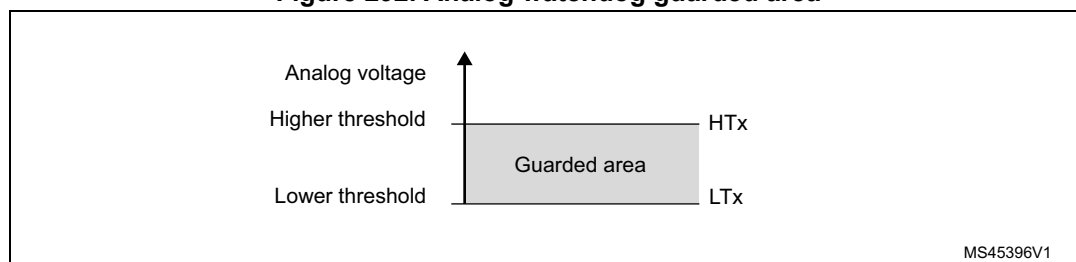
Figure 292. Analog watchdog guarded area
