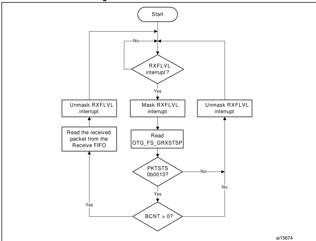
Figure 894. Receive FIFO read task
