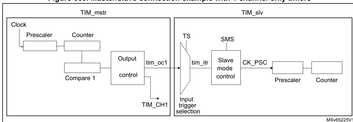
Figure 669. Master/slave connection example with 1 channel only timers
