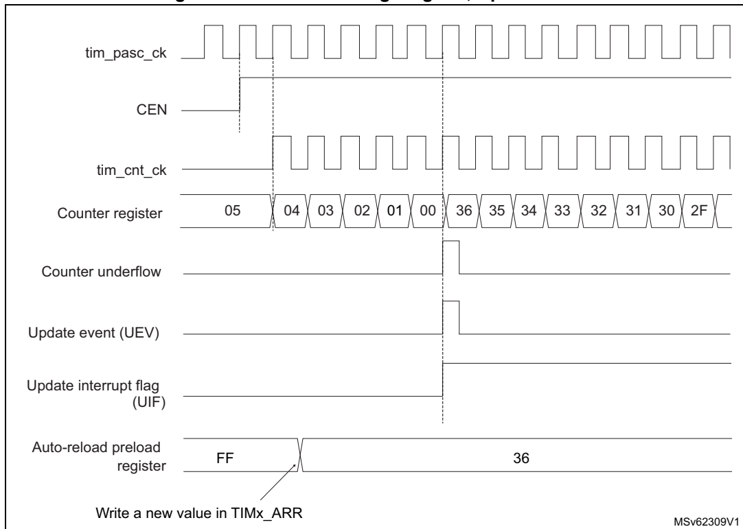
Figure 606. Counter timing diagram, Update event
