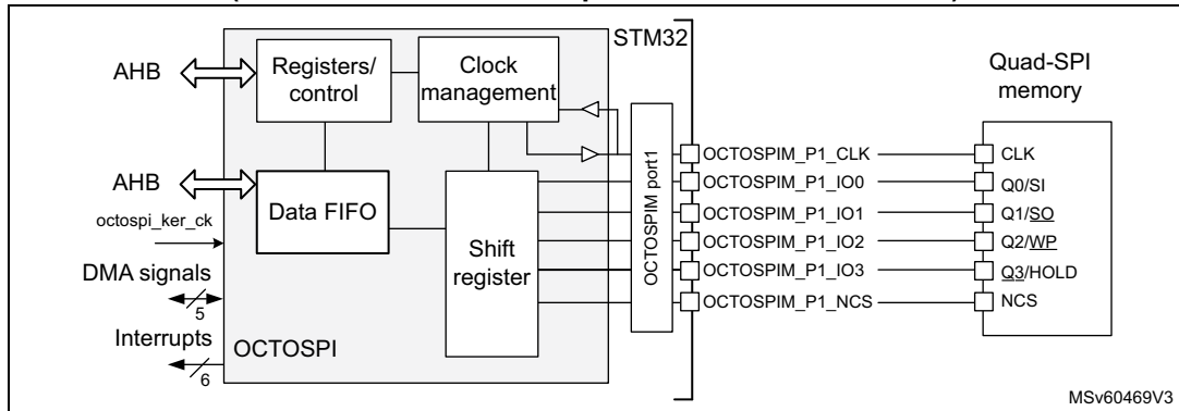
Figure 140. OCTOSPI block diagram in quad configuration (for STM32U5 series except STM32U535/545 devices)
