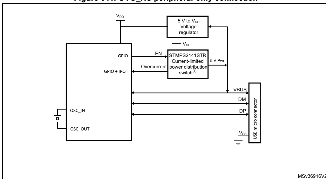
Figure 911. OTG_HS peripheral-only connection
