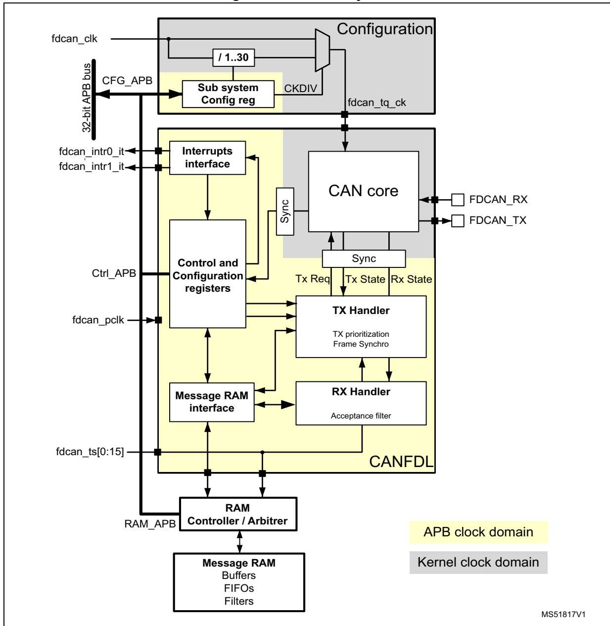
Figure 873. CAN subsystem
