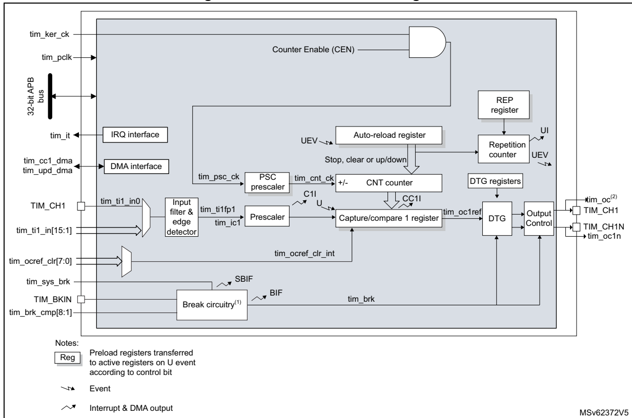
Figure 676. TIM16/TIM17 block diagram
