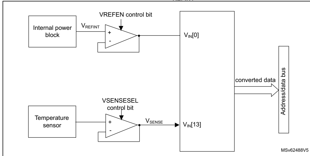
Figure 300. Temperature sensor and V REFINT channel block diagram
