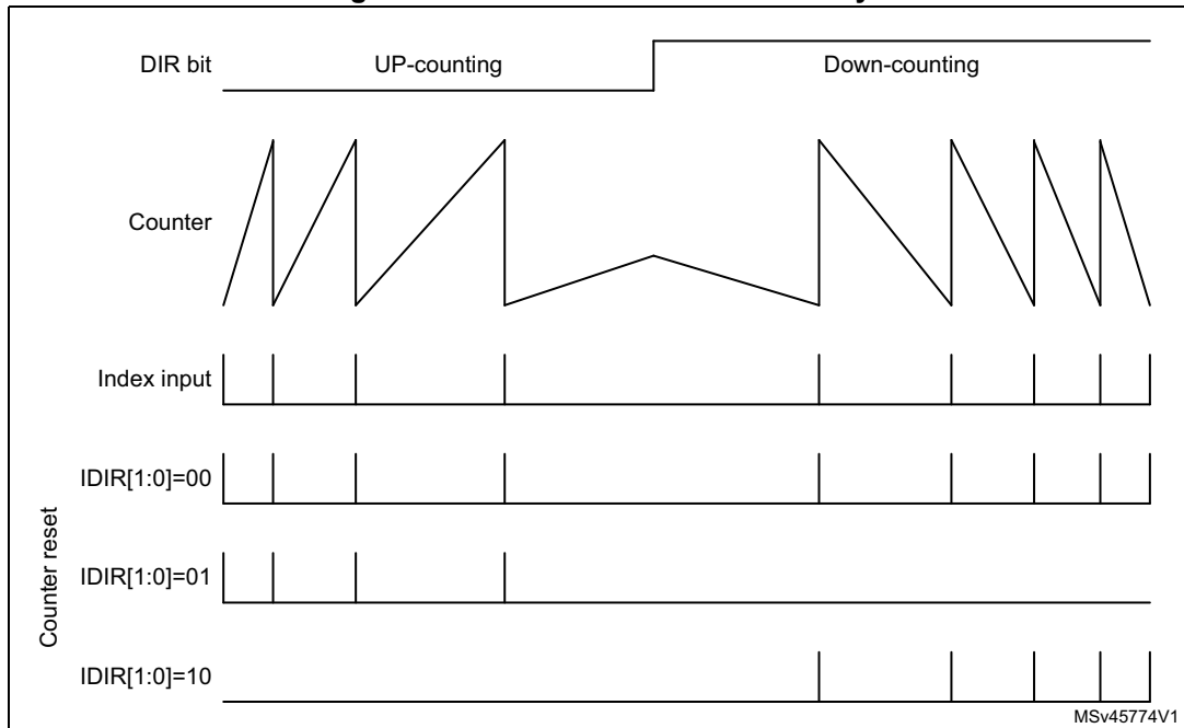
Figure 578. Directional index sensitivity
