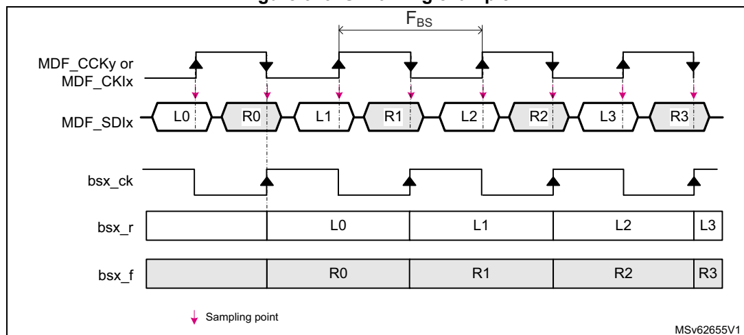
Figure 323. SPI timing example
