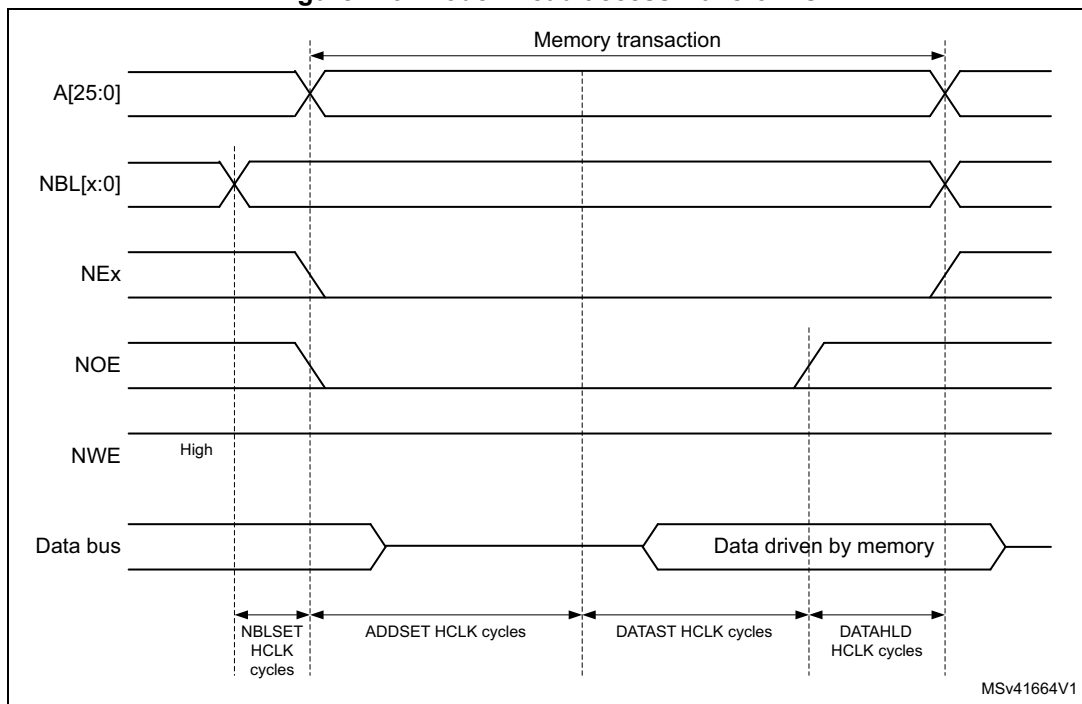
Figure 119. Mode 1 read access waveforms
