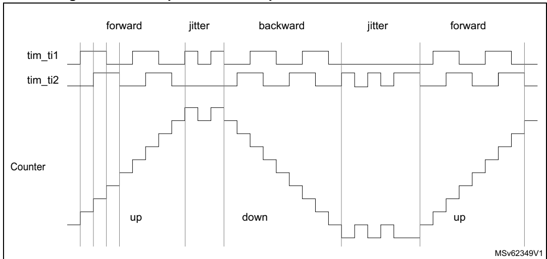
Figure 640. Example of counter operation in encoder interface mode
