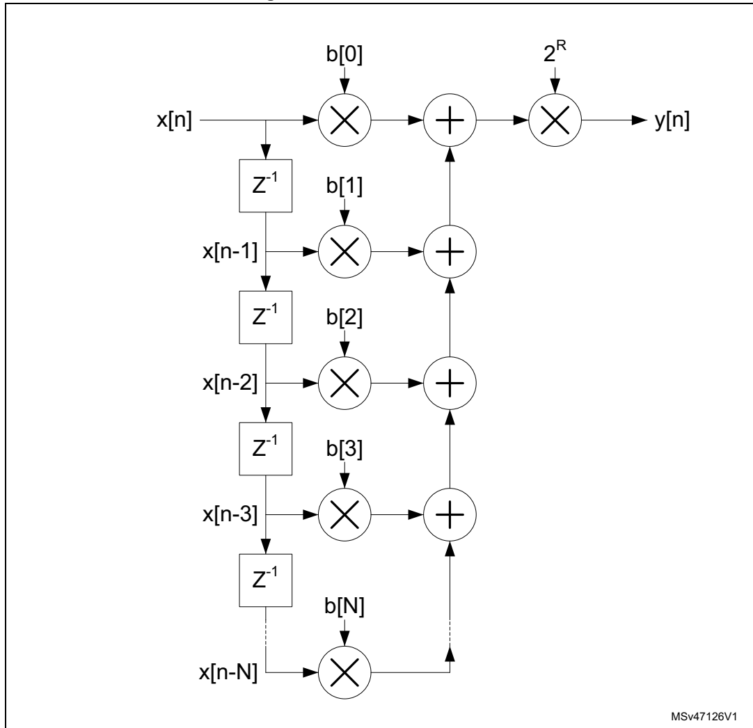
Figure 112. FIR filter structure
