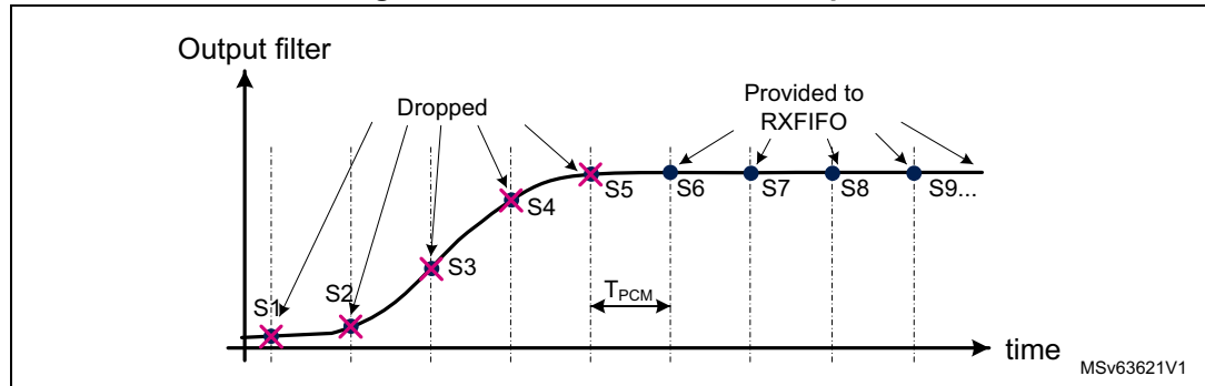
Figure 371. Discard function example
