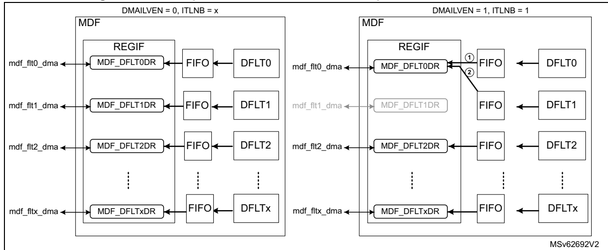
Figure 348. Data path for interleaved- and independent-transfer modes
