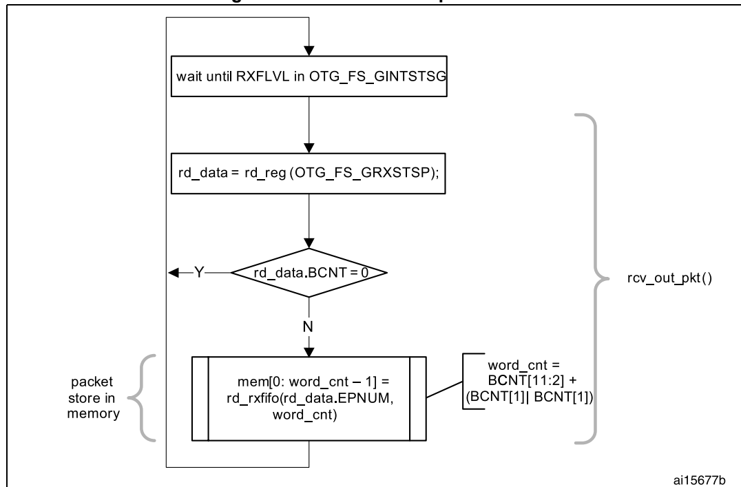
Figure 901. Receive FIFO packet read
