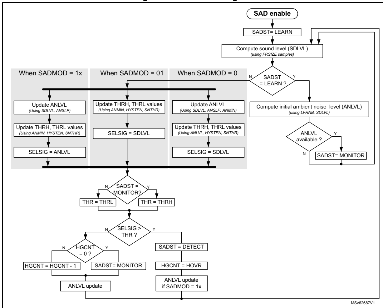
Figure 374. SAD flow diagram
