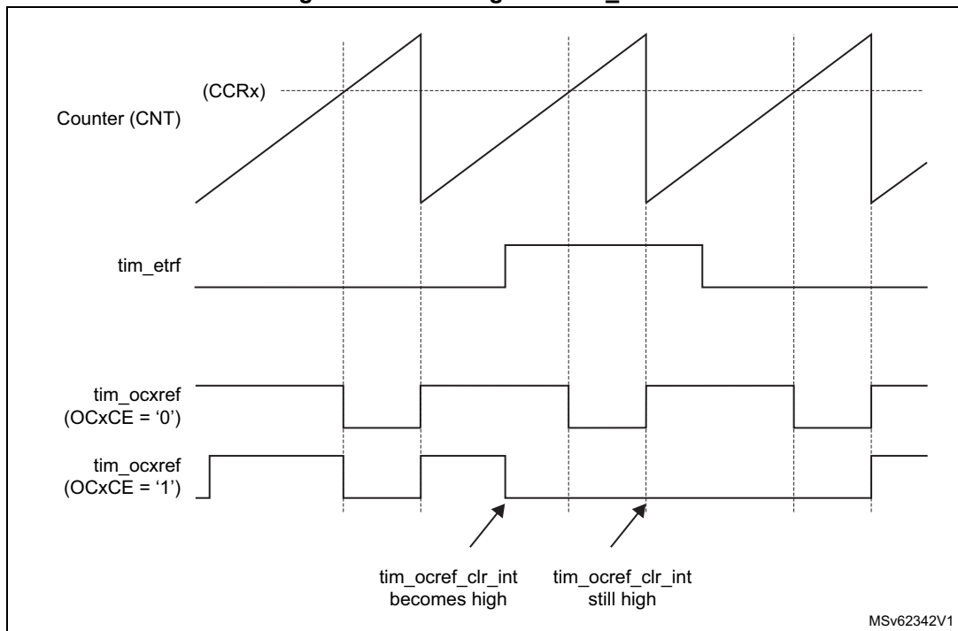
Figure 556. Clearing TIMx tim_ocxref
