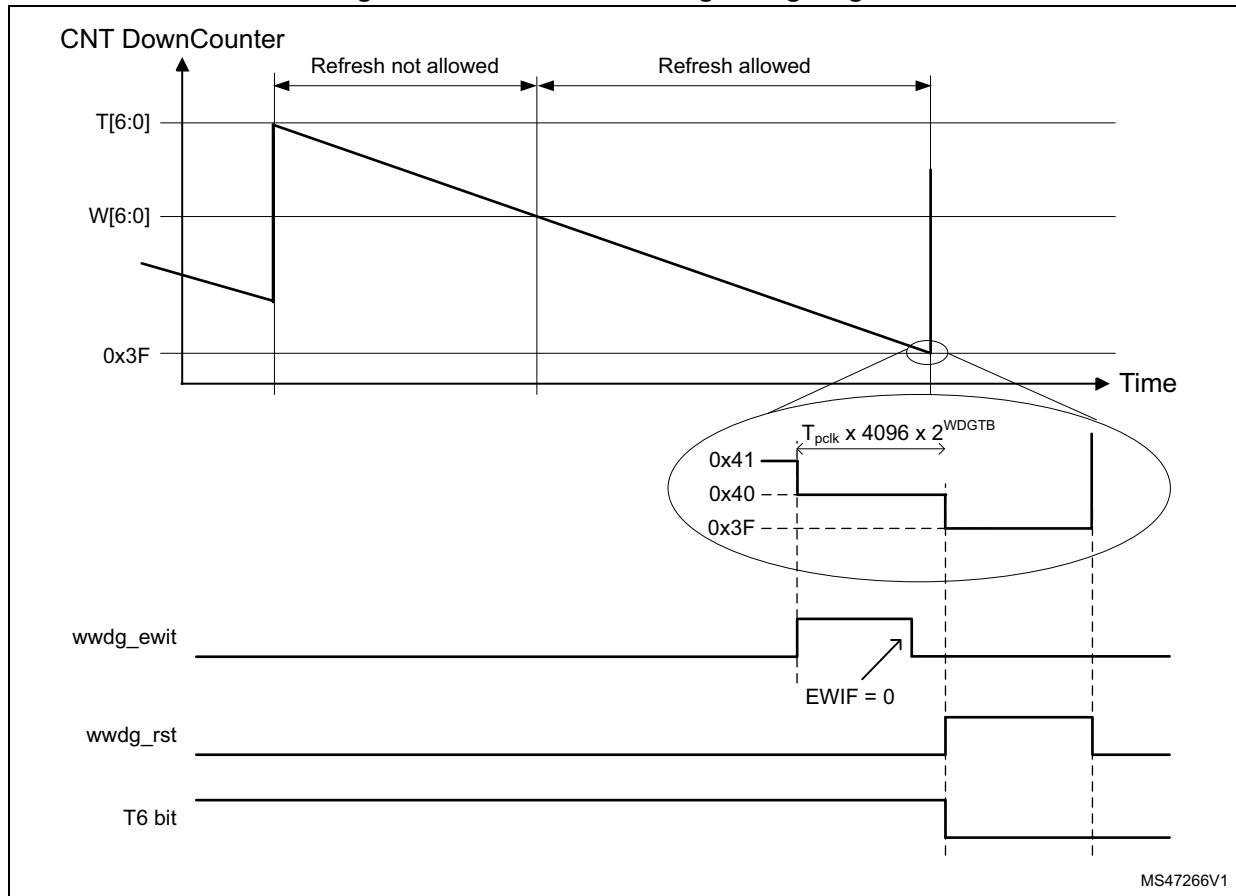
Figure 765. Window watchdog timing diagram
