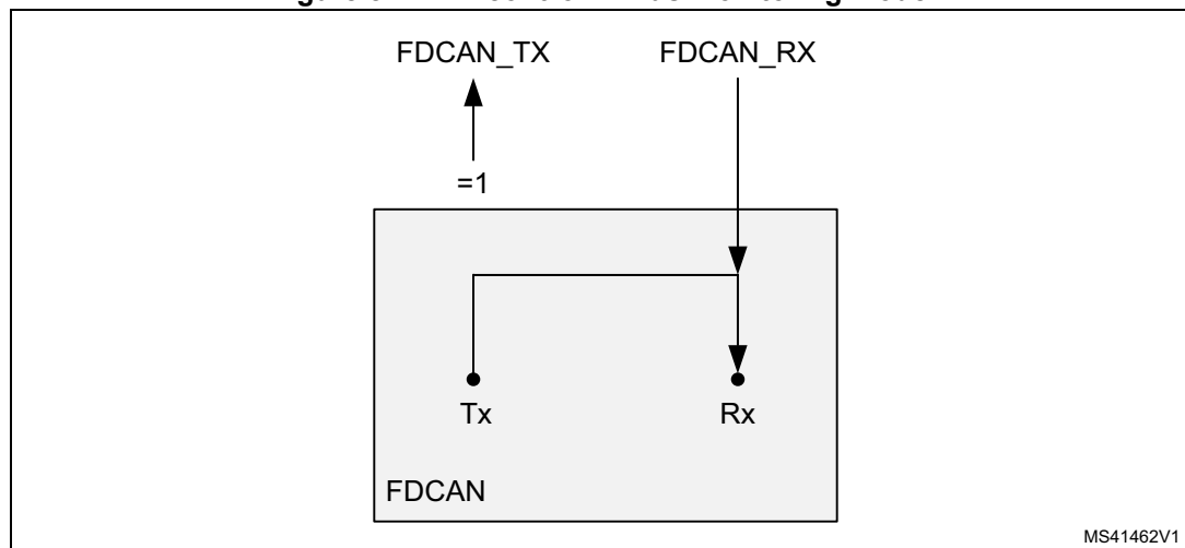
Figure 877. Pin control in Bus monitoring mode
