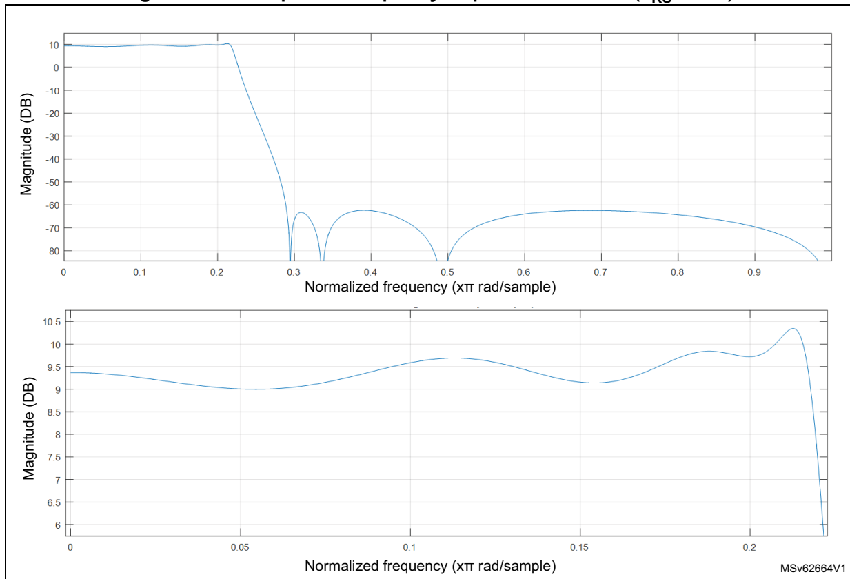
Figure 364. Reshape filter frequency response normalized ( F_{RS} / 2 = 1 )
