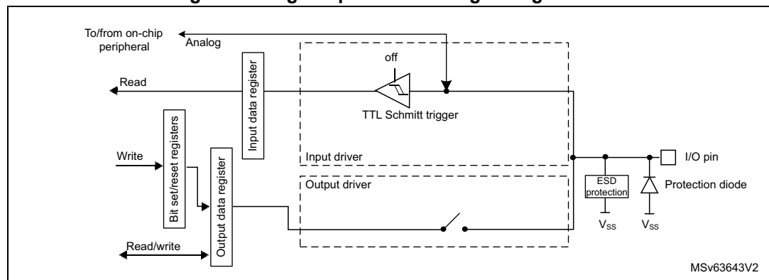
Figure 47. High-impedance analog configuration
