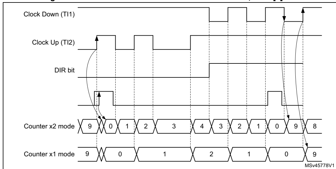
Figure 659. Index behavior in directional clock mode, IPOS[0] = 1
