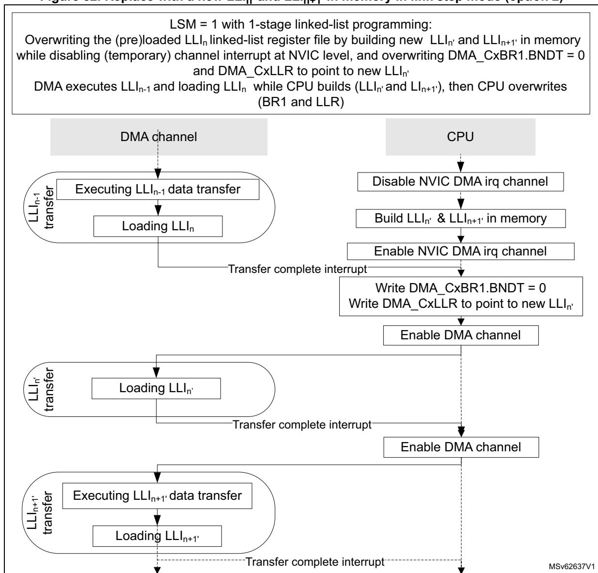
Figure 82. Replace with a new LLI n' and LLI n+1' in memory in link step mode (option 2)
