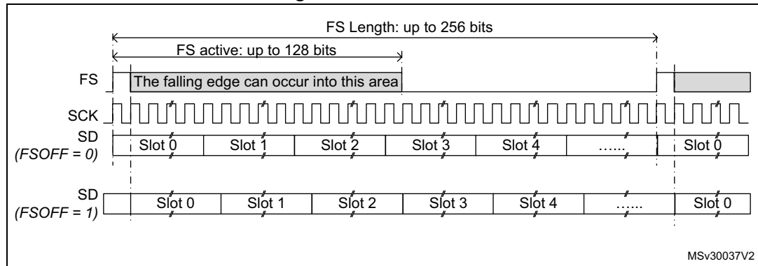
Figure 852. Audio frame
