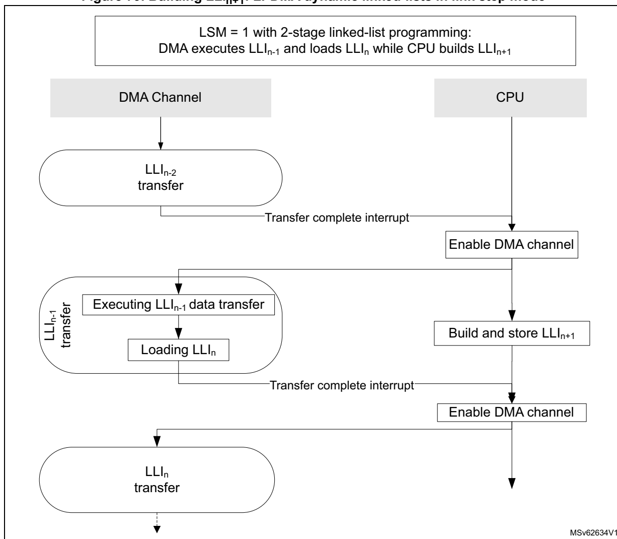
Figure 79. Building LLI_{n+1} : LPDMA dynamic linked-lists in link step mode
