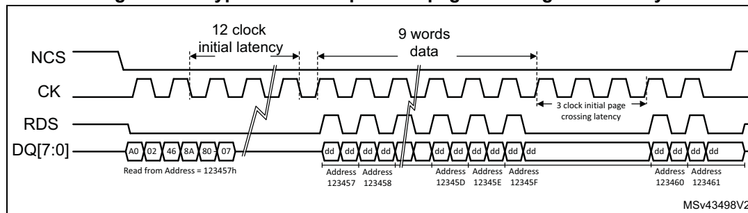
Figure 154. HyperBus read operation page crossing with latency
