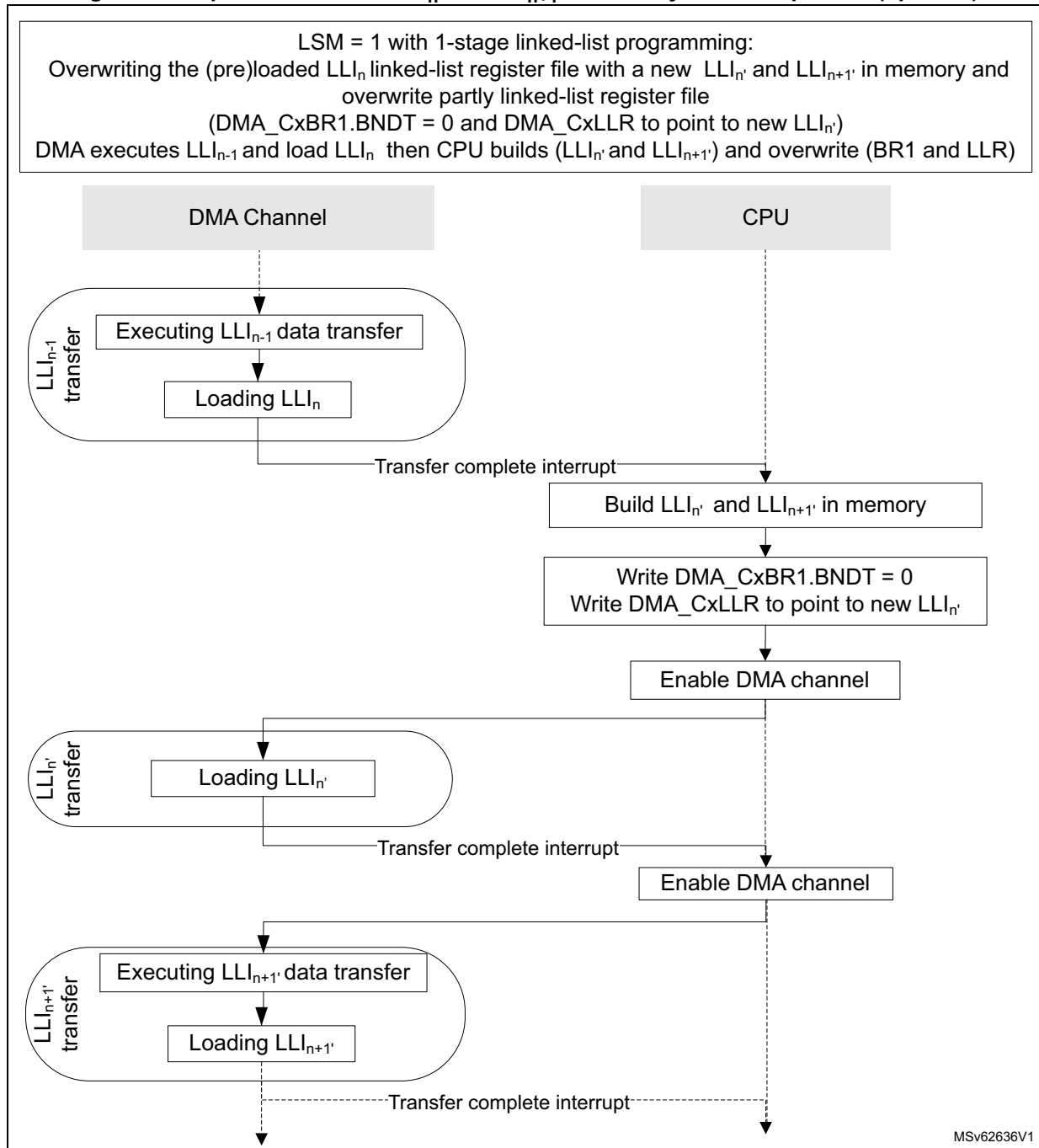
Figure 81. Replace with a new LLI n' and LLI n+1' in memory in link step mode (option 1)
