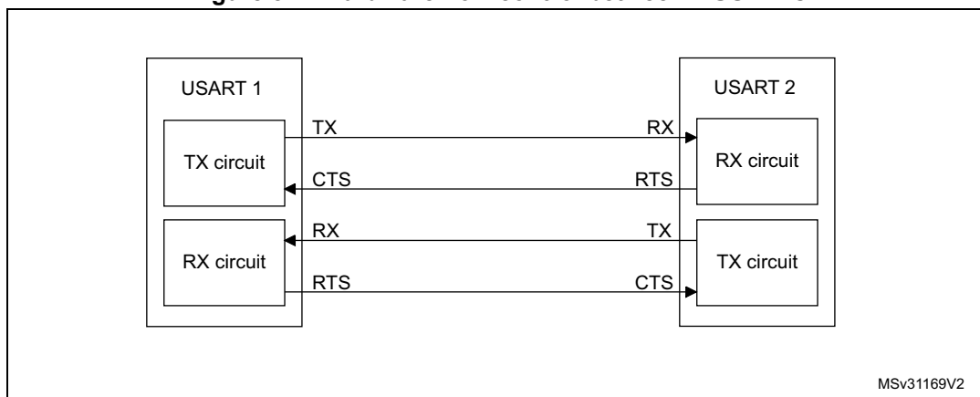
Figure 822. Hardware flow control between 2 USARTs
