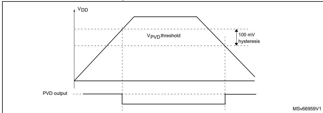
Figure 34. PVD thresholds
