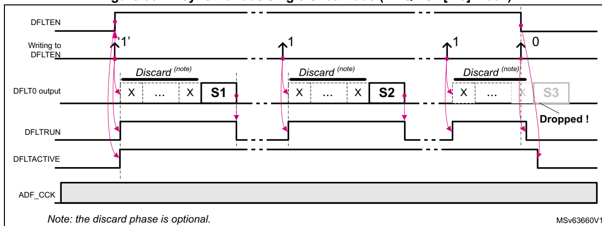
Figure 367. Asynchronous single-shot mode (ACQMOD[2:0] = 001)
