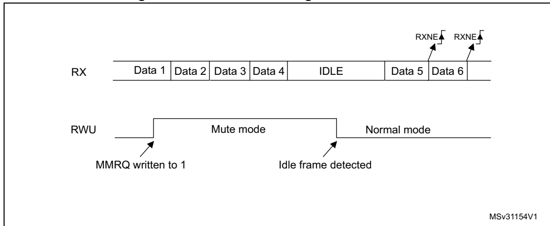
Figure 830. Mute mode using Idle line detection
