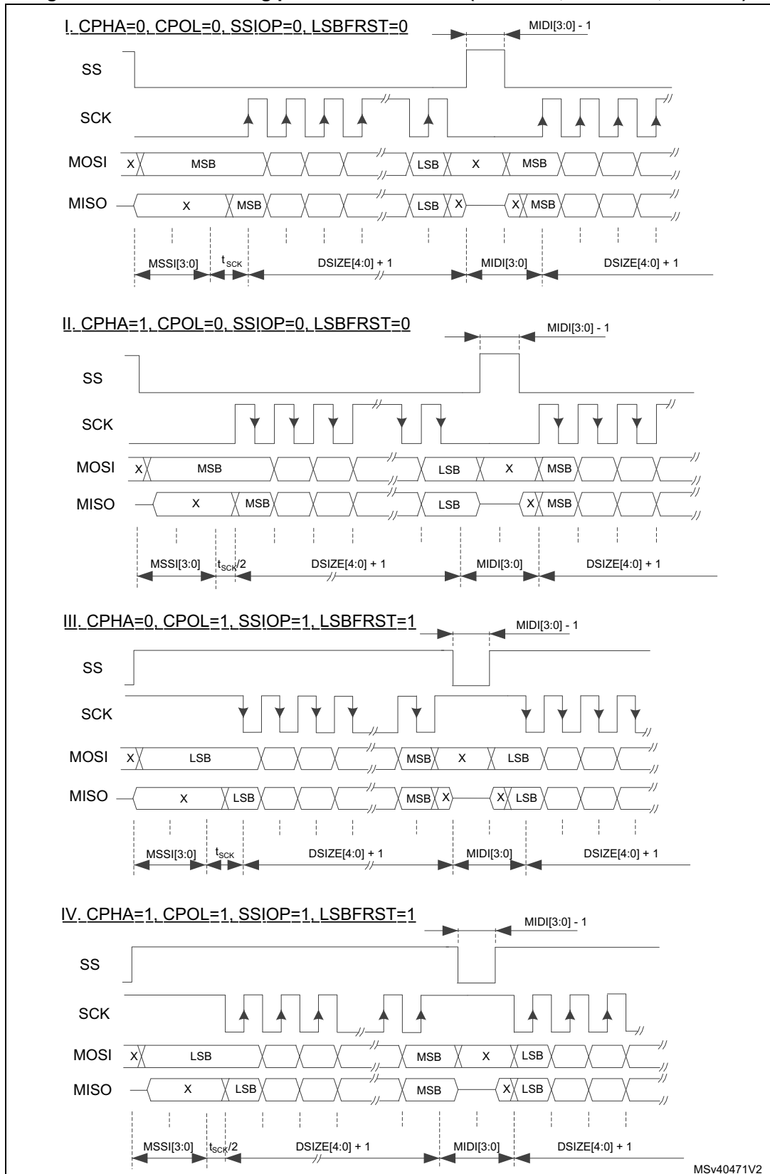
Figure 845. SS interleaving pulses between data (SSOE = 1, SSOM = 1, SSM = 0)
