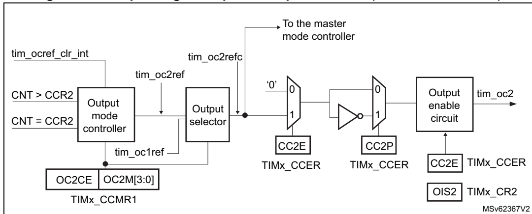
Figure 692. Output stage of capture/compare channel (channel 2 for TIM15)
