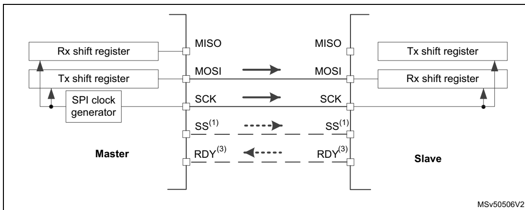
Figure 840. Simplex single master / single slave application (master in transmit-only / slave in receive-only mode)
