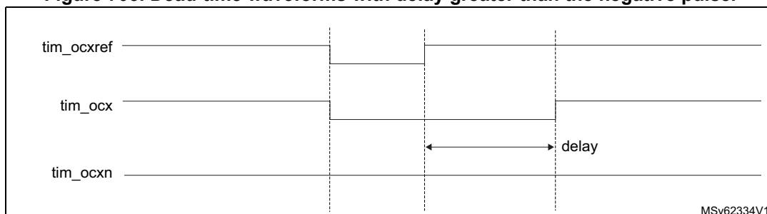
Figure 703. Dead-time waveforms with delay greater than the negative pulse.
