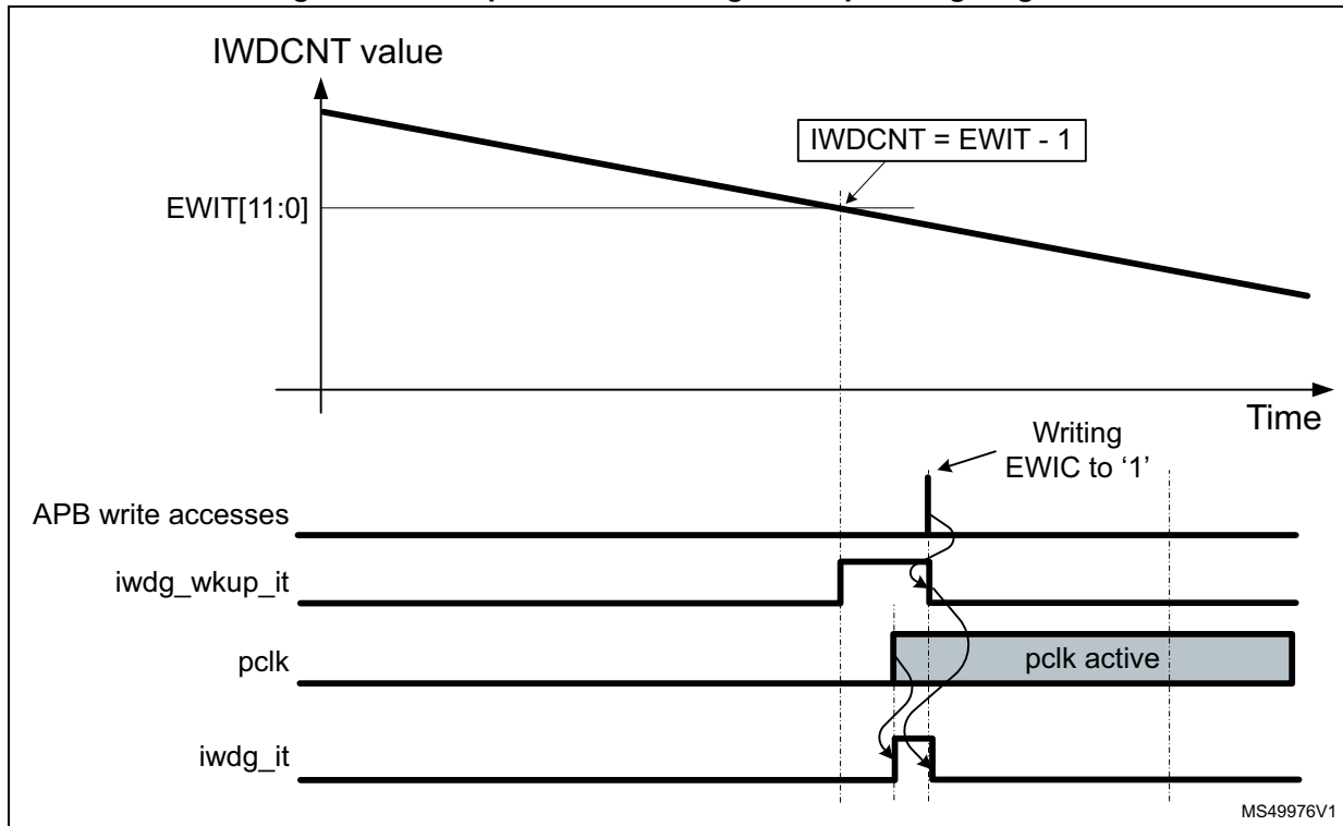
Figure 763. Independent watchdog interrupt timing diagram
