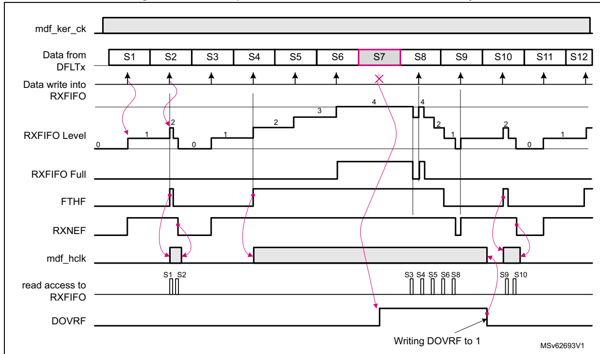
Figure 349. Example of overflow and transfer to memory
