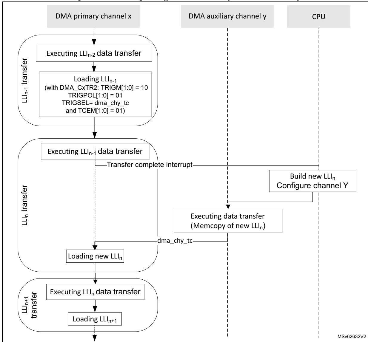
Figure 77. Inserting a LLI n with an auxiliary LPDMA channel y
