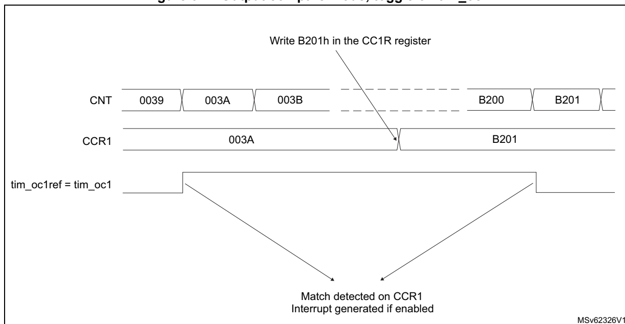
Figure 622. Output compare mode, toggle on tim_oc1
