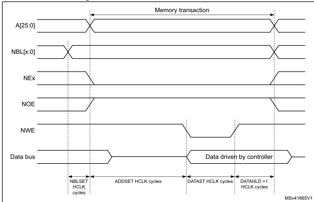
Figure 120. Mode 1 write access waveforms
