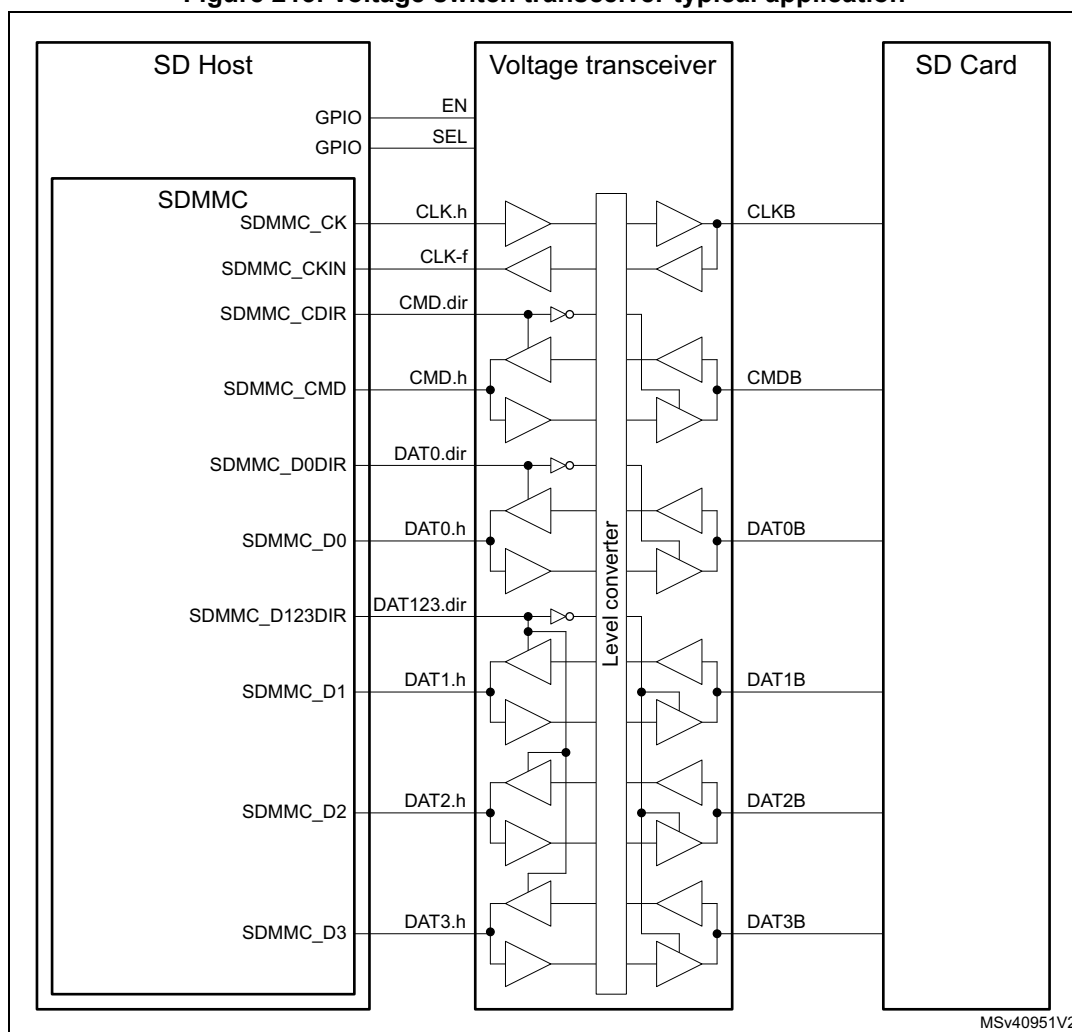
Figure 213. Voltage switch transceiver typical application
