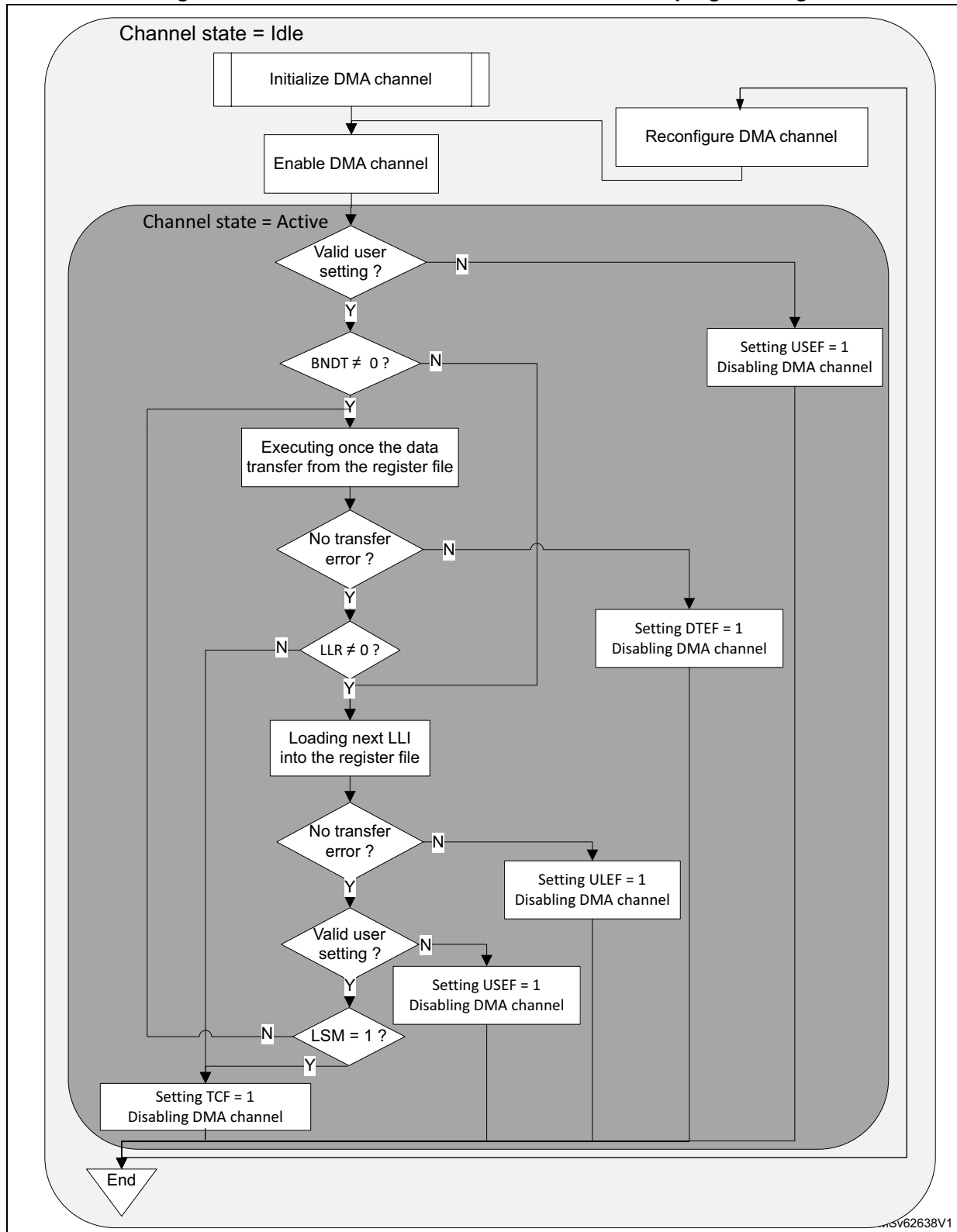
Figure 64. GPDMA channel execution and linked-list programming
