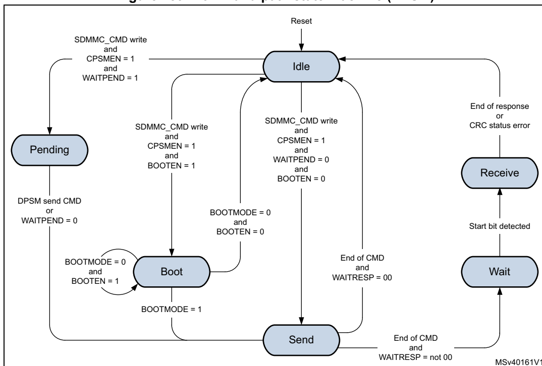
Figure 189. Command path state machine (CPSM)
