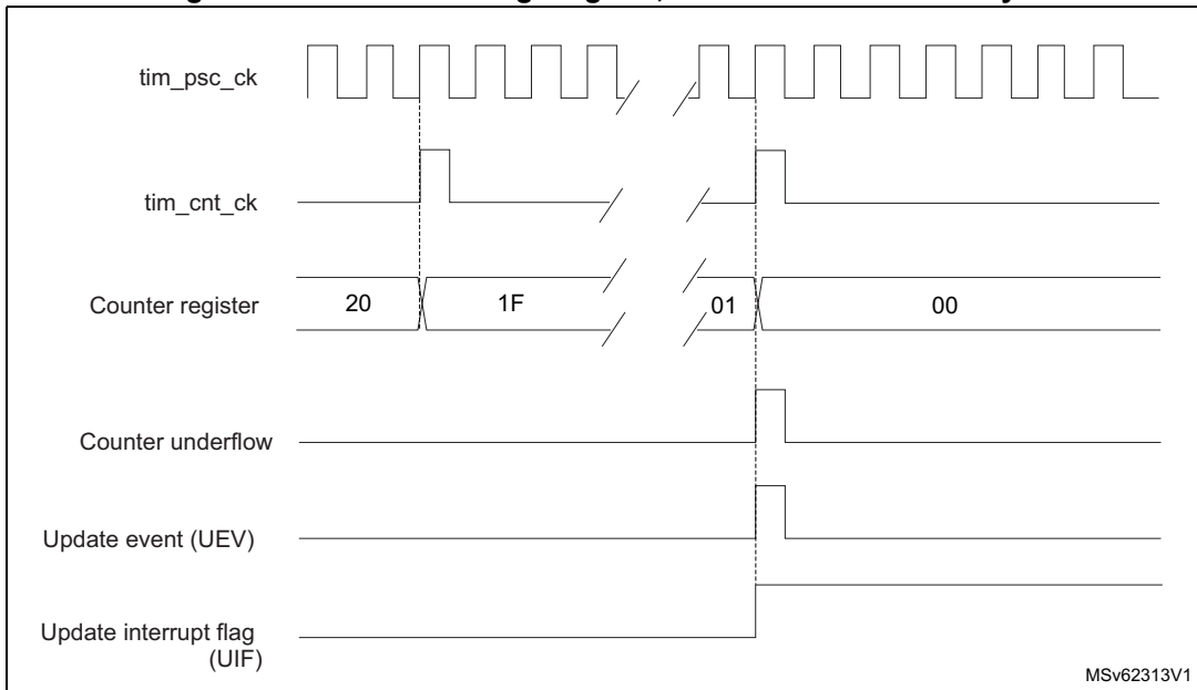
Figure 520. Counter timing diagram, internal clock divided by N
