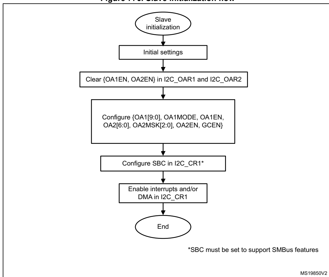
Figure 776. Slave initialization flow
