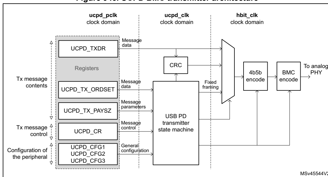
Figure 945. UCPD BMC transmitter architecture
