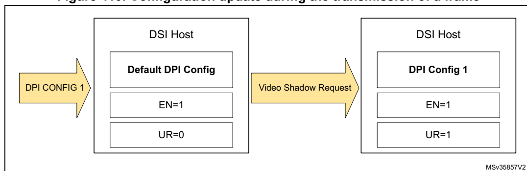
Figure 410. Configuration update during the transmission of a frame
