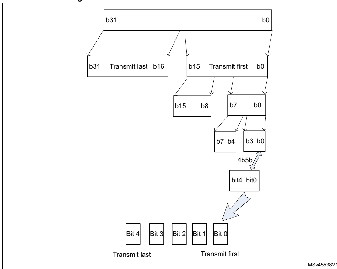
Figure 939. Transmit order for various sizes of data
