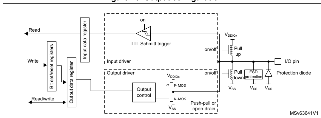
Figure 45. Output configuration
