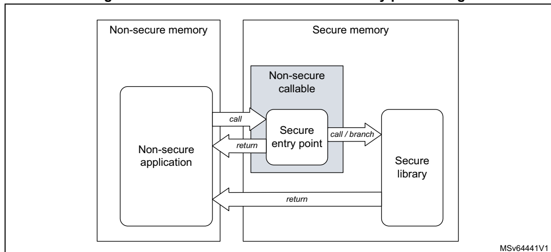
Figure 9. Secure world transition and memory partitioning
