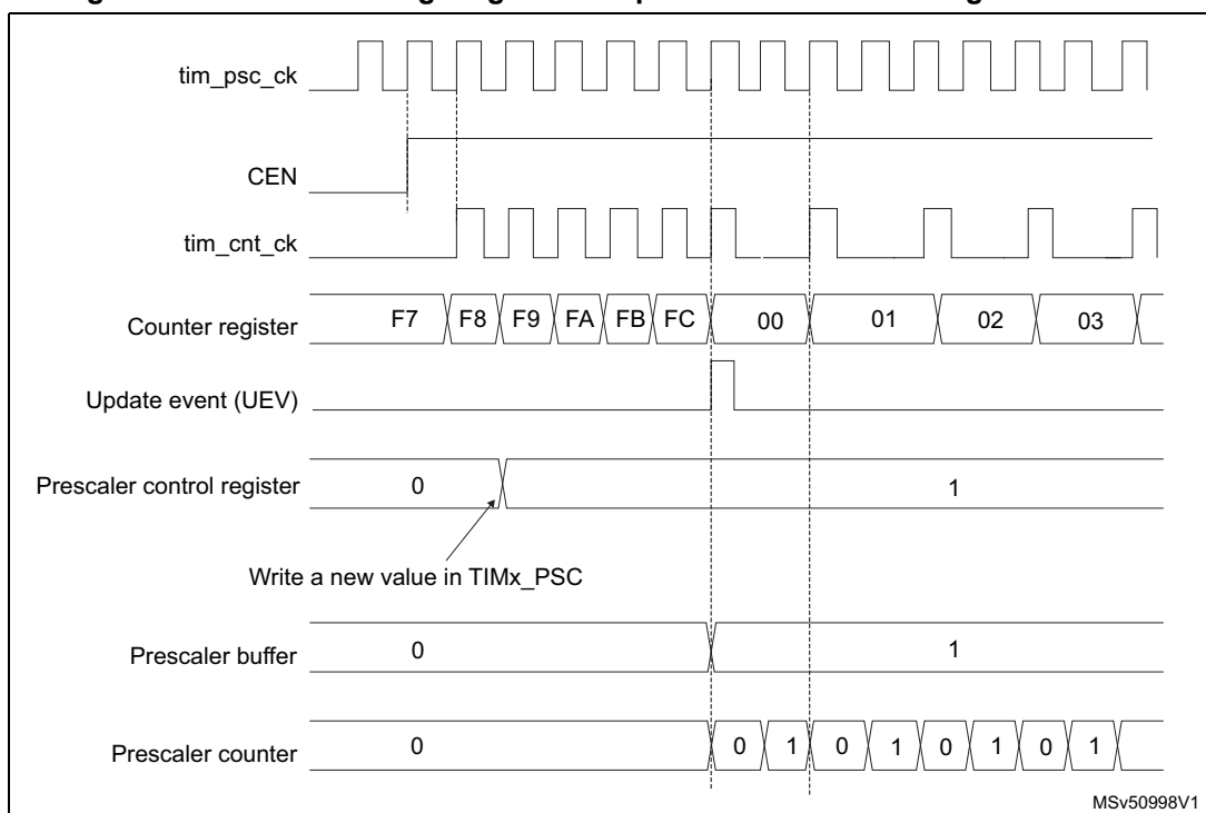
Figure 718. Counter timing diagram with prescaler division change from 1 to 2
