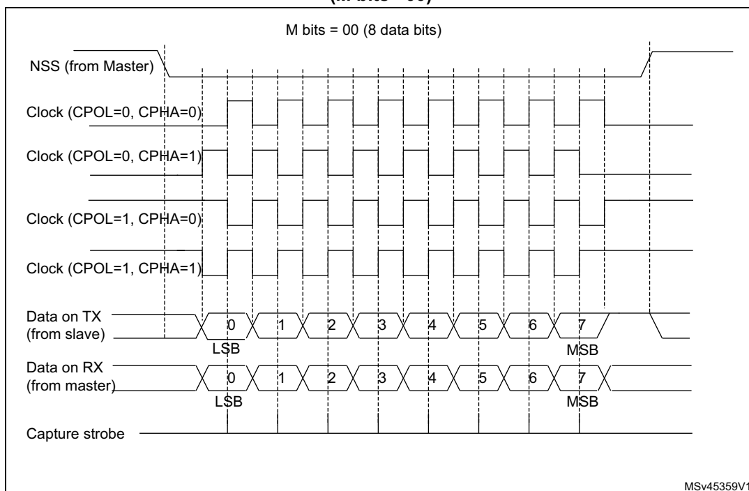
Figure 815. USART data clock timing diagram in Synchronous slave mode (M bits =00)
