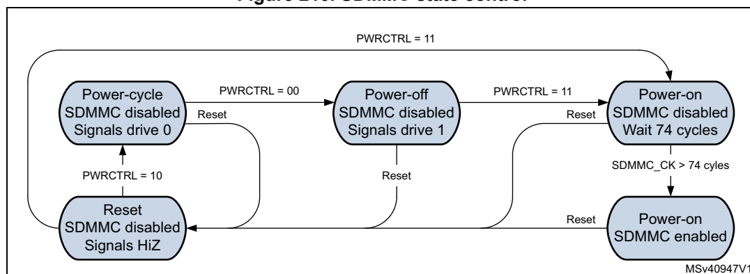
Figure 210. SDMMC state control
