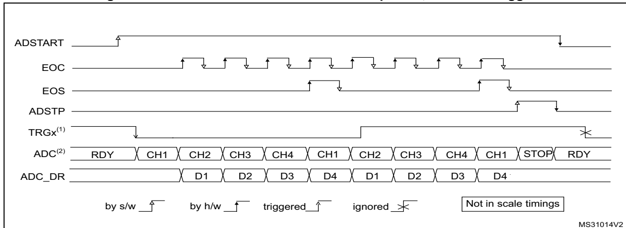
Figure 230. Continuous conversions of a sequence, hardware trigger
